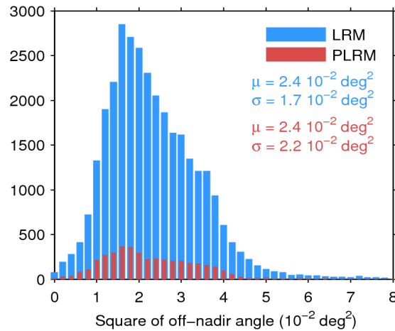
Figure 39. Histogram of flag-valid mispointing over oceans and lakes for LRM (blue) and PLRM (red) for 02/08/2014. Only positive values have been considered. The mean ( \mu ) and standard deviation ( \sigma ) are also shown. Note that values 8 \cdot 10^{-2} \text{ deg}^2 are excluded from the histogram for the sake of readability but not from the computation of \mu and \sigma .
