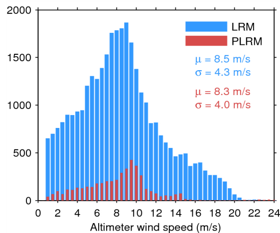
Figure 35. Histogram of science-valid wind over oceans and lakes for LRM (blue) and PLRM (red) for 02/08/2014. The mean ( \mu ) and standard deviation ( \sigma ) are also shown. Note that values larger than 24 m/s are excluded from the histogram for the sake of readability but not from the computation of \mu and \sigma .
