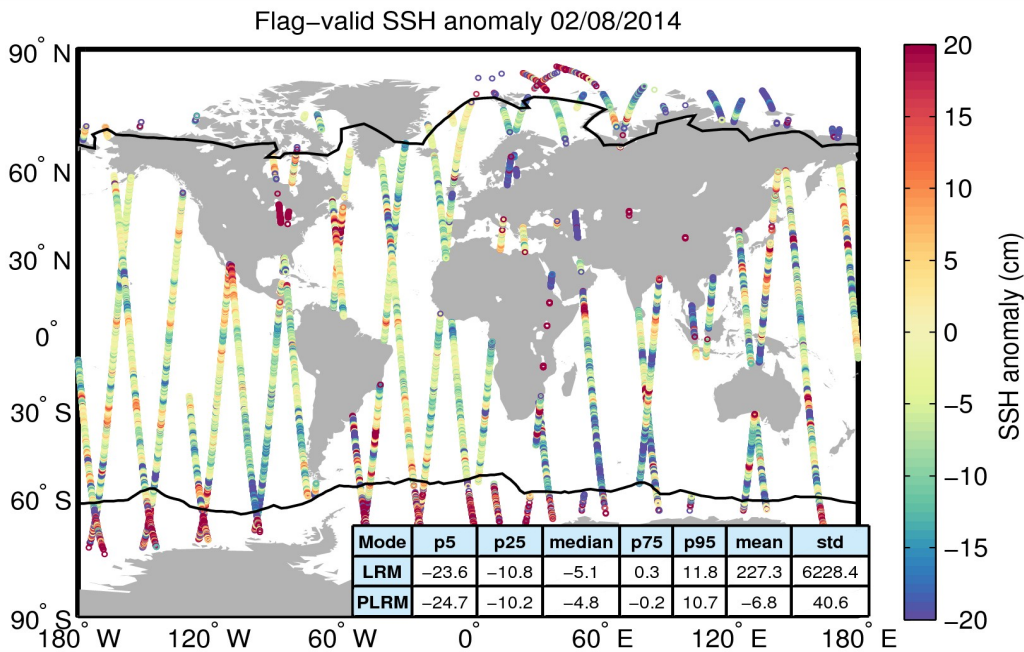
Figure 5. Geographical distribution of flag-valid 1-Hz SSH anomaly data over oceans and lakes for 02/08/2014. The statistical values shown in the table refer to the SSH anomaly in cm and are calculated separately for LRM and PLRM regions. Measurements taken over polar polygons have been excluded from the computation of the statistical values. The black lines mark the outer limit of the Arctic and Antarctic polar polygons.
