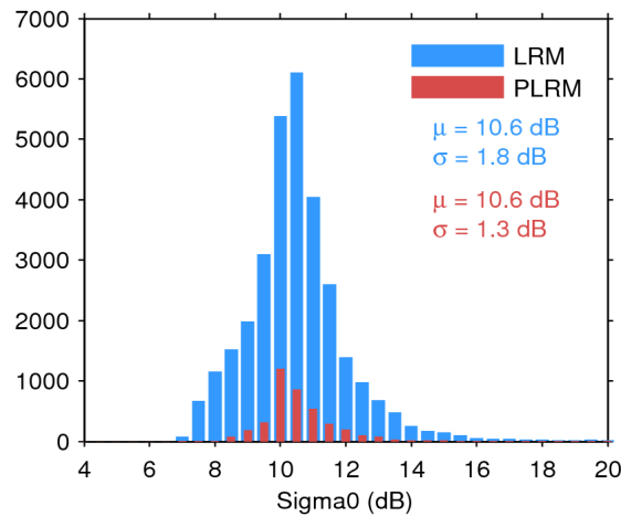
Figure 28. Histogram of science-valid sigma0 over oceans and lakes for LRM (blue) and PLRM (red) for 02/08/2014. The mean ( \mu ) and standard deviation ( \sigma ) are also shown. Note that values outside [4 20] dB are excluded from the histogram for the sake of readability but not from the computation of \mu and \sigma .
