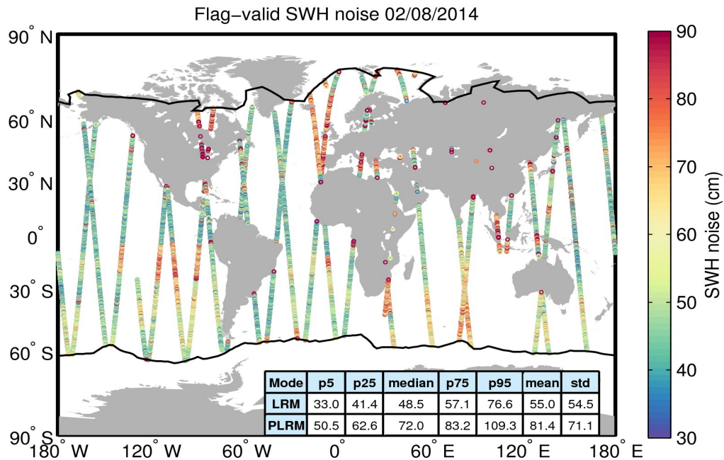
Figure 18. Geographical distribution of flag-valid 20-Hz SWH measurement noise over oceans and lakes for 02/08/2014. The statistical values shown in the table refer to the SWH noise and are calculated separately for LRM and PLRM regions. Measurements taken over polar polygons have been excluded from the computation of the statistical values. The black lines mark the outer limit of the Arctic and Antarctic polar polygons.
