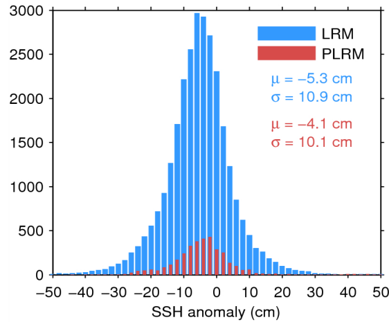
Figure 11. Histogram of science-valid SSH anomaly over oceans and lakes for LRM (blue) and PLRM (red) for 02/08/2014. The mean ( \mu ) and standard deviation ( \sigma ) are also shown. Note that values outside [-50\ 50] cm are excluded from the histogram for the sake of readability but not from the computation of \mu and \sigma .
