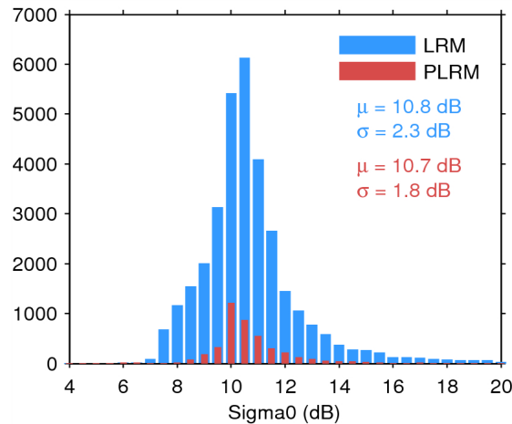
Figure 25. Histogram of flag-valid sigma0 over oceans and lakes for LRM (blue) and PLRM (red) for 02/08/2014. The mean ( \mu ) and standard deviation ( \sigma ) are also shown. Note that values outside [4 20] dB are excluded from the histogram for the sake of readability but not from the computation of \mu and \sigma .
