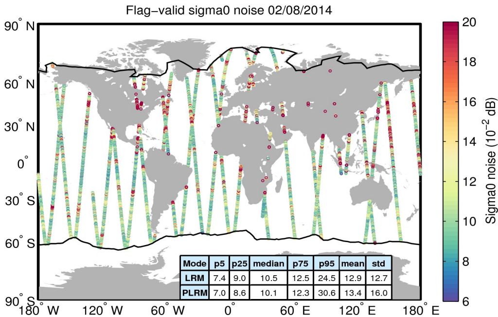
Figure 26. Geographical distribution of flag-valid 20-Hz sigma0 measurement noise over oceans and lakes for 02/08/2014. The statistical values shown in the table refer to the sigma0 noise and are calculated separately for LRM and PLRM regions. Measurements taken over polar polygons have been excluded from the computation of the statistical values. The black lines mark the outer limit of the Arctic and Antarctic polar polygons.
