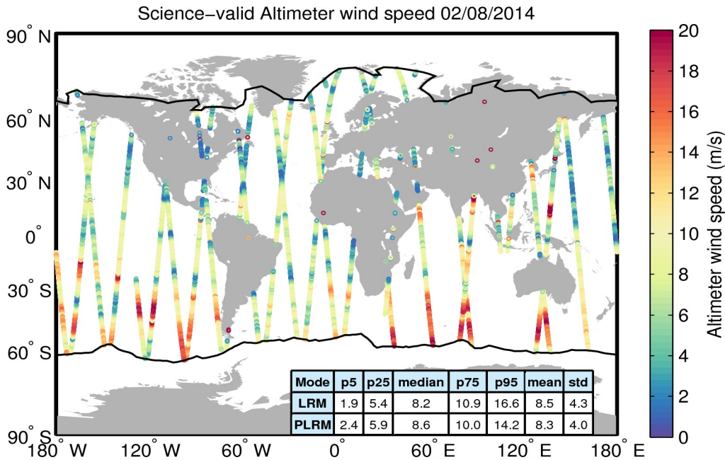
Figure 34. Geographical distribution of science-valid wind data over oceans and lakes for 02/08/2014. The statistical values shown in the table refer to the wind in m/s and are calculated separately for LRM and PLRM regions. The black lines mark the outer limit of the Arctic and Antarctic polar polygons. Gray circles denote records that have been rejected based on the editing criteria described in Table 5.
