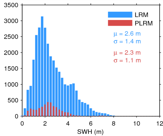
Figure 20. Histogram of science-valid SWH over oceans and lakes for LRM (blue) and PLRM (red) for 02/08/2014. The mean ( \mu ) and standard deviation ( \sigma ) are also shown. Note that values larger than 12 m are excluded from the histogram for the sake of readability but not from the computation of \mu and \sigma .
