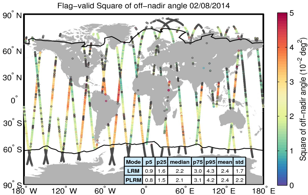
Figure 37. Geographical distribution of flag-valid mispointing data over oceans and lakes for 02/08/2014. The statistical values shown in the table refer to the mispointing in 10^{-2} \text{ deg}^2 and are calculated separately for LRM and PLRM regions. Measurements taken over polar polygons have been excluded from the computation of the statistical values. The black lines mark the outer limit of the Arctic and Antarctic polar polygons. Gray circles denote negative values.
