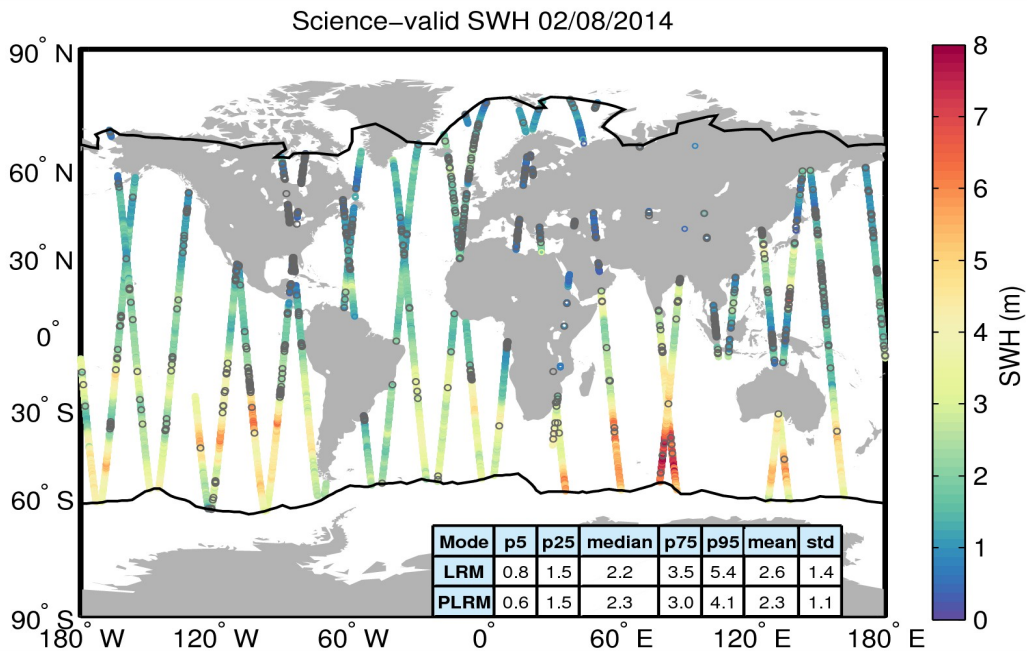
Figure 19. Geographical distribution of science-valid SWH data over oceans and lakes for 02/08/2014. The statistical values shown in the table refer to the SWH in m and are calculated separately for LRM and PLRM regions. The black lines mark the outer limit of the Arctic and Antarctic polar polygons. Gray circles denote records that have been rejected based on the editing criteria described in Table 3.
