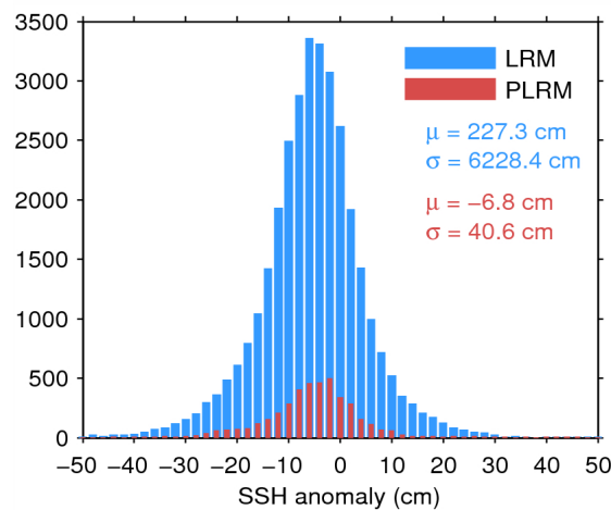
Figure 7. Histogram of flag-valid SSH anomaly over oceans and lakes for LRM (blue) and PLRM (red) for 02/08/2014. The mean ( \mu ) and standard deviation ( \sigma ) are also shown. Note that values outside [-50\ 50] cm are excluded from the histogram for the sake of readability but not from the computation of \mu and \sigma .
