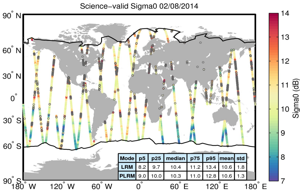
Figure 27. Geographical distribution of science-valid sigma0 data over oceans and lakes for 02/08/2014. The statistical values shown in the table refer to the sigma0 in dB and are calculated separately for LRM and PLRM regions. The black lines mark the outer limit of the Arctic and Antarctic polar polygons. Gray circles denote records that have been rejected based on the editing criteria described in Table 4.
