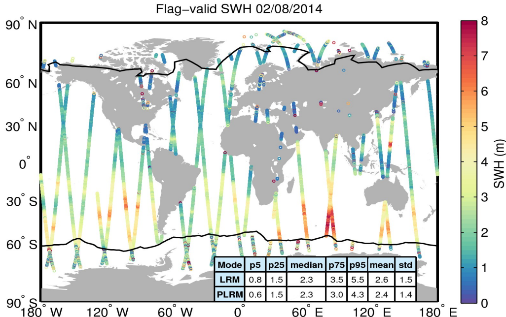
Figure 15. Geographical distribution of flag-valid SWH data over oceans and lakes for 02/08/2014. The statistical values shown in the table refer to the SWH in m and are calculated separately for LRM and PLRM regions. Measurements taken over polar polygons have been excluded from the computation of the statistical values. The black lines mark the outer limit of the Arctic and Antarctic polar polygons.
