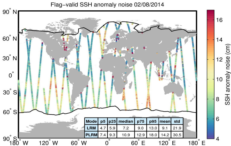
Figure 8. Geographical distribution of flag-valid 20-Hz SSH anomaly measurement noise over oceans and lakes for 02/08/2014. The statistical values shown in the table refer to the SSH anomaly noise and are calculated separately for LRM and PLRM regions. Measurements taken over polar polygons have been excluded from the computation of the statistical values. The black lines mark the outer limit of the Arctic and Antarctic polar polygons.
