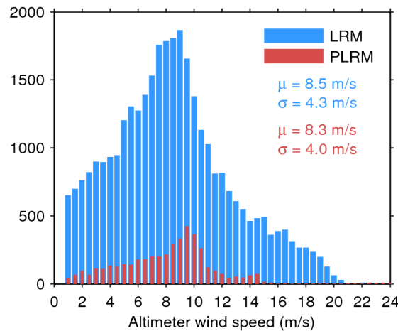
Figure 33. Histogram of flag-valid wind over oceans and lakes for LRM (blue) and PLRM (red) for 02/08/2014. The mean ( \mu ) and standard deviation ( \sigma ) are also shown. Note that values larger than 24 m/s are excluded from the histogram for the sake of readability but not from the computation of \mu and \sigma .
