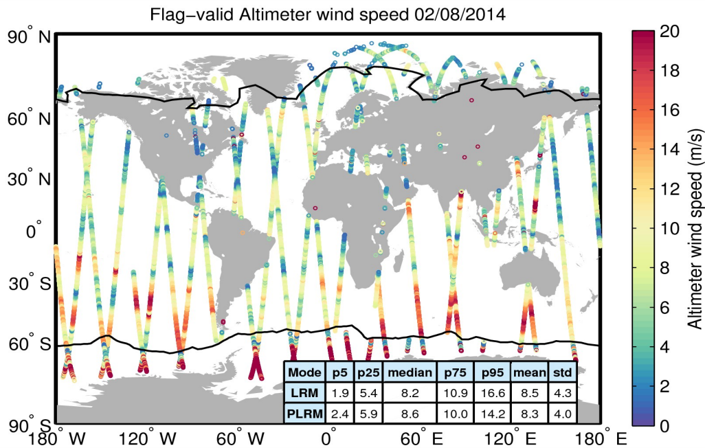
Figure 31. Geographical distribution of flag-valid wind data over oceans and lakes for 02/08/2014. The statistical values shown in the table refer to the wind in m/s and are calculated separately for LRM and PLRM regions. Measurements taken over polar polygons have been excluded from the computation of the statistical values. The black lines mark the outer limit of the Arctic and Antarctic polar polygons.
