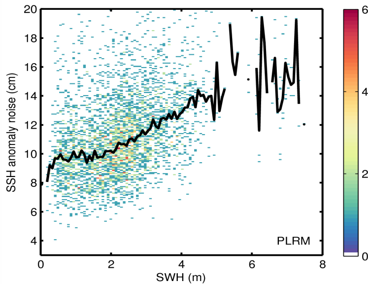
Figure 9. 2D histogram showing flag-valid SSH anomaly noise as a function of SWH for LRM (top) and PLRM (bottom) for 02/08/2014. The black line denotes the median SSH anomaly as a function of SWH.
