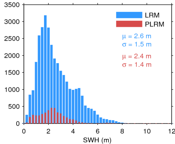
Figure 17. Histogram of flag-valid SWH over oceans and lakes for LRM (blue) and PLRM (red) for 02/08/2014. The mean ( \mu ) and standard deviation ( \sigma ) are also shown. Note that values larger than 12 m are excluded from the histogram for the sake of readability but not from the computation of \mu and \sigma .
