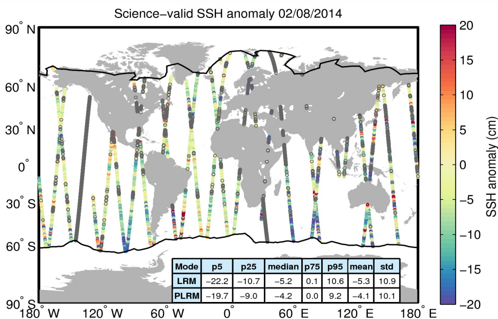
Figure 10. Geographical distribution of science-valid SSH anomaly data over oceans and lakes for 02/08/2014. The statistical values shown in the table refer to the SSH anomaly in cm and are calculated separately for LRM and PLRM regions. The black lines mark the outer limit of the Arctic and Antarctic polar polygons. Gray circles denote records that have been rejected based on the editing criteria described in Table 2.
