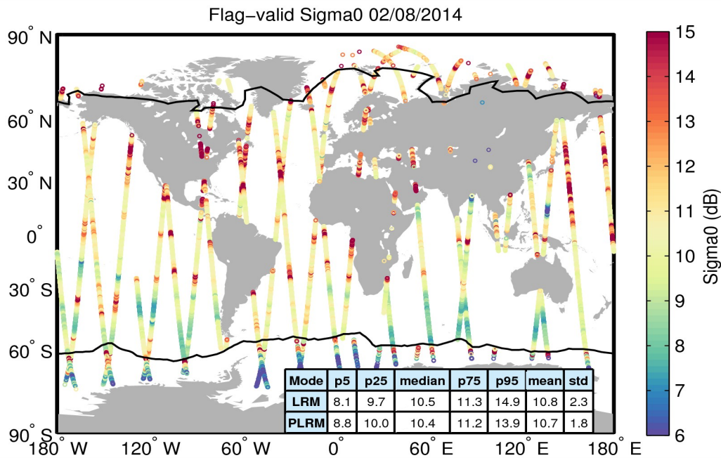
Figure 23. Geographical distribution of flag-valid sigma0 data over oceans and lakes for 02/08/2014. The statistical values shown in the table refer to the sigma0 in dB and are calculated separately for LRM and PLRM regions. Measurements taken over polar polygons have been excluded from the computation of the statistical values. The black lines mark the outer limit of the Arctic and Antarctic polar polygons.
