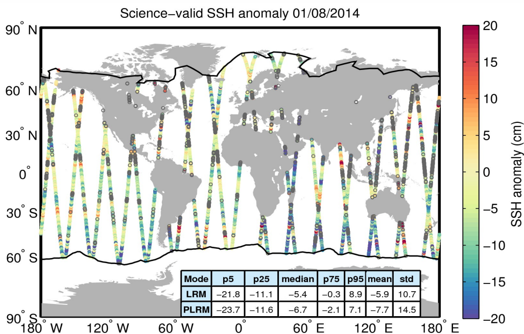
Figure 10. Geographical distribution of science-valid SSH anomaly data over oceans and lakes for 01/08/2014. The statistical values shown in the table refer to the SSH anomaly in cm and are calculated separately for LRM and PLRM regions. The black lines mark the outer limit of the Arctic and Antarctic polar polygons. Gray circles denote records that have been rejected based on the editing criteria described in Table 2.
