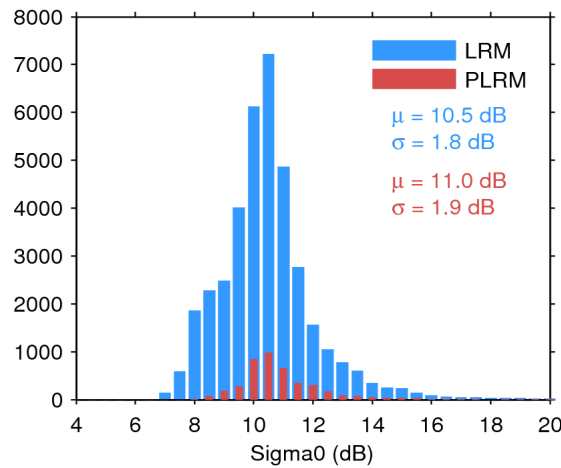
Figure 28. Histogram of science-valid sigma0 over oceans and lakes for LRM (blue) and PLRM (red) for 01/08/2014. The mean ( \mu ) and standard deviation ( \sigma ) are also shown. Note that values outside [4 20] dB are excluded from the histogram for the sake of readability but not from the computation of \mu and \sigma .
