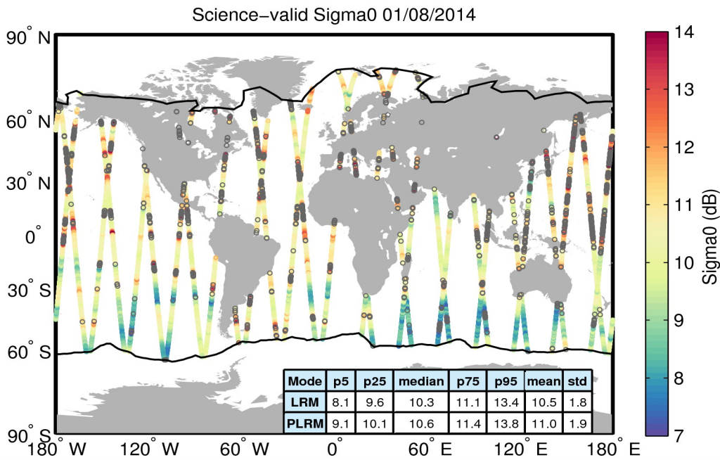
Figure 27. Geographical distribution of science-valid sigma0 data over oceans and lakes for 01/08/2014. The statistical values shown in the table refer to the sigma0 in dB and are calculated separately for LRM and PLRM regions. The black lines mark the outer limit of the Arctic and Antarctic polar polygons. Gray circles denote records that have been rejected based on the editing criteria described in Table 4.
