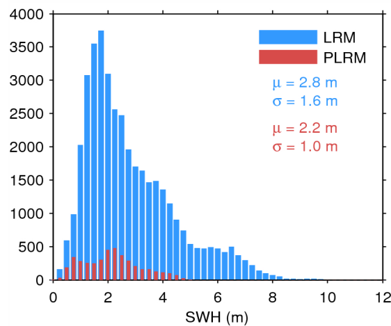
Figure 20. Histogram of science-valid SWH over oceans and lakes for LRM (blue) and PLRM (red) for 01/08/2014. The mean ( \mu ) and standard deviation ( \sigma ) are also shown. Note that values larger than 12 m are excluded from the histogram for the sake of readability but not from the computation of \mu and \sigma .
