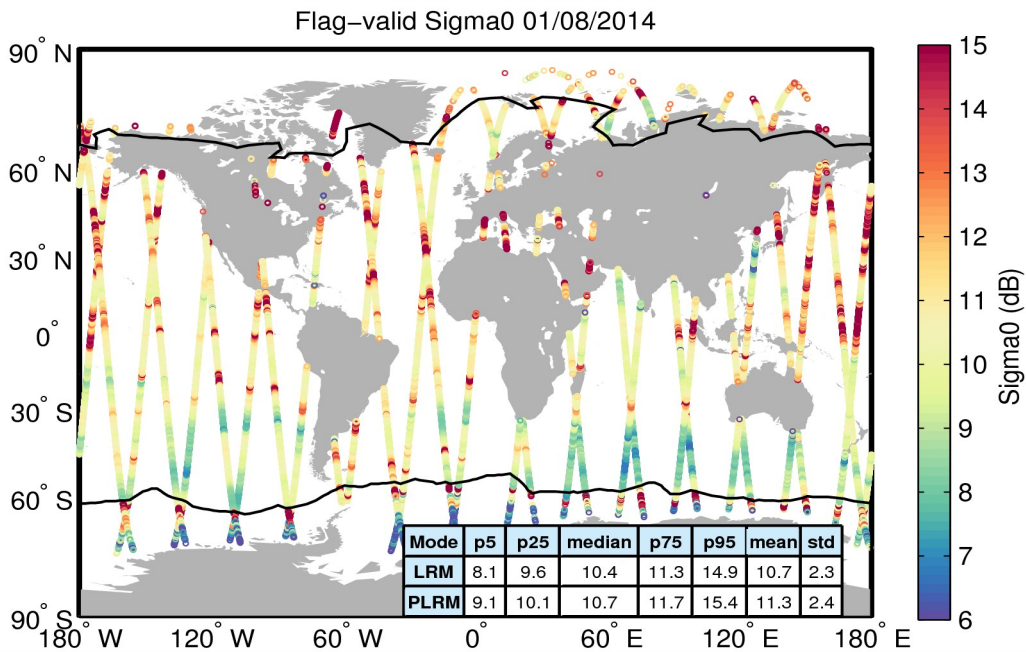
Figure 23. Geographical distribution of flag-valid sigma0 data over oceans and lakes for 01/08/2014. The statistical values shown in the table refer to the sigma0 in dB and are calculated separately for LRM and PLRM regions. Measurements taken over polar polygons have been excluded from the computation of the statistical values. The black lines mark the outer limit of the Arctic and Antarctic polar polygons.
