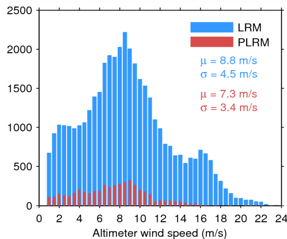
Figure 35. Histogram of science-valid wind over oceans and lakes for LRM (blue) and PLRM (red) for 01/08/2014. The mean ( \mu ) and standard deviation ( \sigma ) are also shown. Note that values larger than 24 m/s are excluded from the histogram for the sake of readability but not from the computation of \mu and \sigma .
