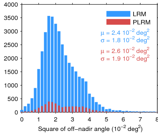
Figure 39. Histogram of flag-valid mispointing over oceans and lakes for LRM (blue) and PLRM (red) for 01/08/2014. Only positive values have been considered. The mean ( \mu ) and standard deviation ( \sigma ) are also shown. Note that values 8 \cdot 10^{-2} \text{ deg}^2 are excluded from the histogram for the sake of readability but not from the computation of \mu and \sigma .
