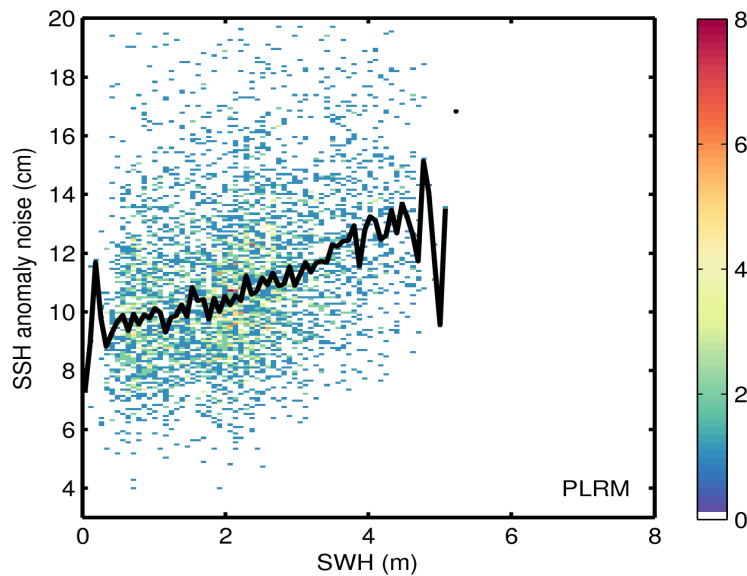
Figure 9. 2D histogram showing flag-valid SSH anomaly noise as a function of SWH for LRM (top) and PLRM (bottom) for 01/08/2014. The black line denotes the median SSH anomaly as a function of SWH.
