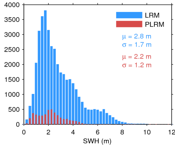
Figure 17. Histogram of flag-valid SWH over oceans and lakes for LRM (blue) and PLRM (red) for 01/08/2014. The mean ( \mu ) and standard deviation ( \sigma ) are also shown. Note that values larger than 12 m are excluded from the histogram for the sake of readability but not from the computation of \mu and \sigma .
