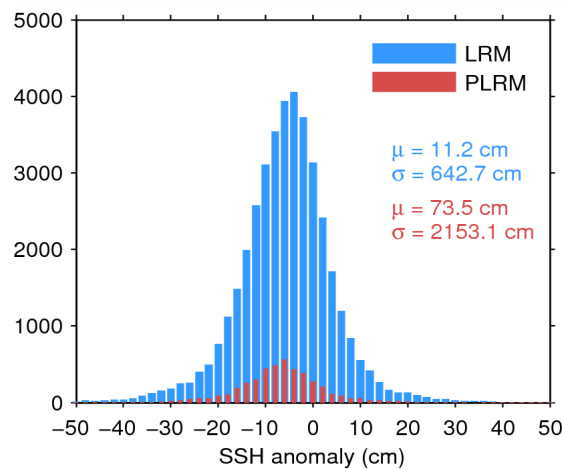
Figure 7. Histogram of flag-valid SSH anomaly over oceans and lakes for LRM (blue) and PLRM (red) for 01/08/2014. The mean ( \mu ) and standard deviation ( \sigma ) are also shown. Note that values outside [-50\ 50] cm are excluded from the histogram for the sake of readability but not from the computation of \mu and \sigma .
