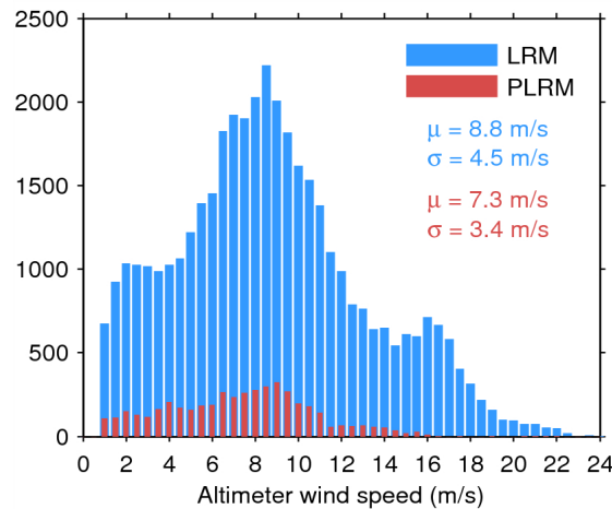
Figure 33. Histogram of flag-valid wind over oceans and lakes for LRM (blue) and PLRM (red) for 01/08/2014. The mean ( \mu ) and standard deviation ( \sigma ) are also shown. Note that values larger than 24 m/s are excluded from the histogram for the sake of readability but not from the computation of \mu and \sigma .
