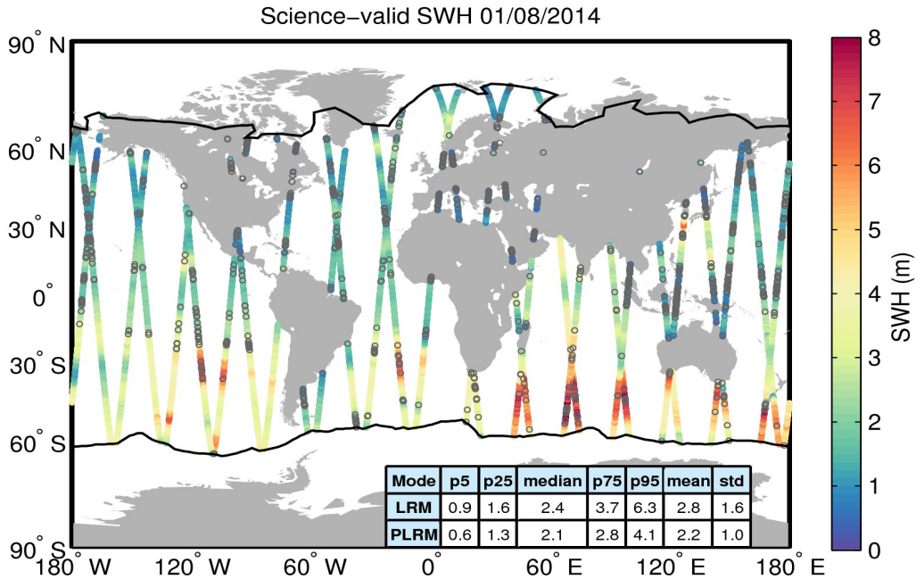
Figure 19. Geographical distribution of science-valid SWH data over oceans and lakes for 01/08/2014. The statistical values shown in the table refer to the SWH in m and are calculated separately for LRM and PLRM regions. The black lines mark the outer limit of the Arctic and Antarctic polar polygons. Gray circles denote records that have been rejected based on the editing criteria described in Table 3.
