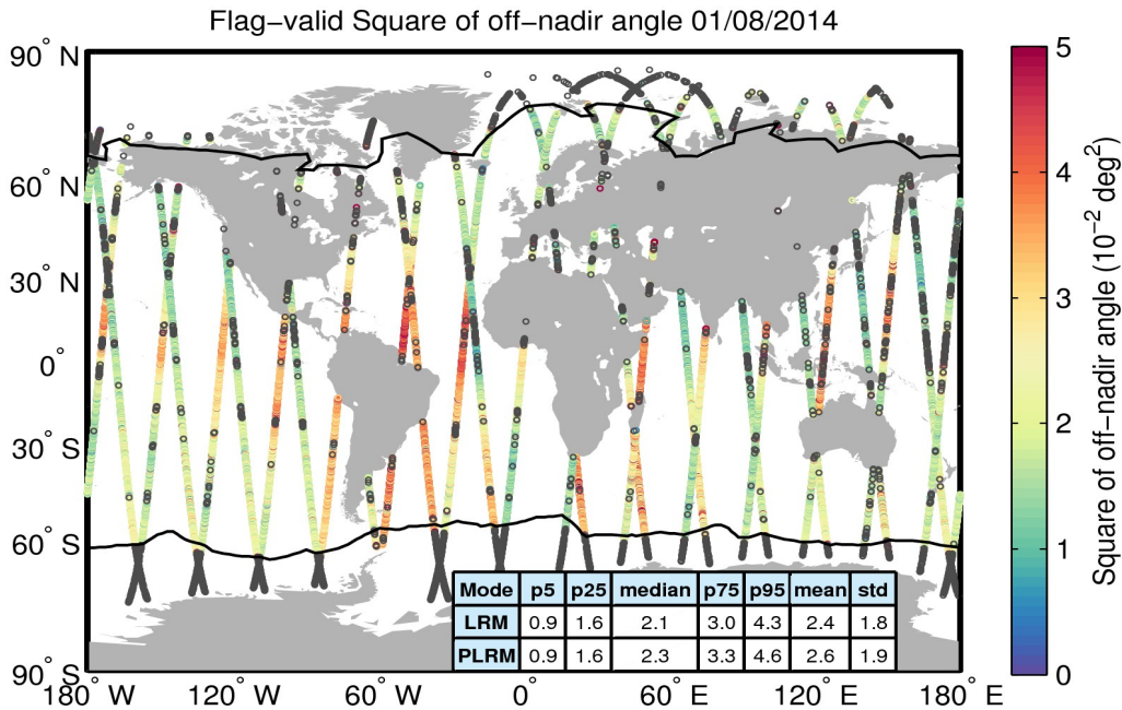
Figure 37. Geographical distribution of flag-valid mispointing data over oceans and lakes for 01/08/2014. The statistical values shown in the table refer to the mispointing in 10^{-2} \text{ deg}^2 and are calculated separately for LRM and PLRM regions. Measurements taken over polar polygons have been excluded from the computation of the statistical values. The black lines mark the outer limit of the Arctic and Antarctic polar polygons. Gray circles denote negative values.
