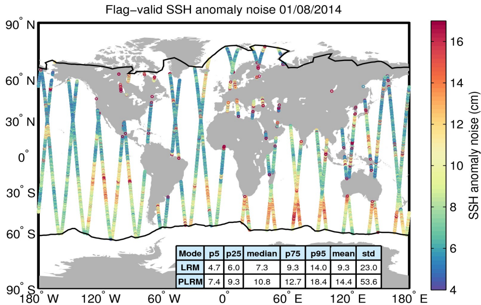
Figure 8. Geographical distribution of flag-valid 20-Hz SSH anomaly measurement noise over oceans and lakes for 01/08/2014. The statistical values shown in the table refer to the SSH anomaly noise and are calculated separately for LRM and PLRM regions. Measurements taken over polar polygons have been excluded from the computation of the statistical values. The black lines mark the outer limit of the Arctic and Antarctic polar polygons.
