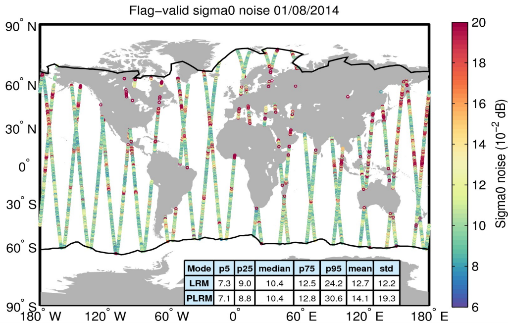
Figure 26. Geographical distribution of flag-valid 20-Hz sigma0 measurement noise over oceans and lakes for 01/08/2014. The statistical values shown in the table refer to the sigma0 noise and are calculated separately for LRM and PLRM regions. Measurements taken over polar polygons have been excluded from the computation of the statistical values. The black lines mark the outer limit of the Arctic and Antarctic polar polygons.
