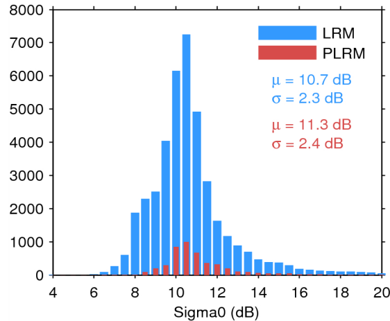
Figure 25. Histogram of flag-valid sigma0 over oceans and lakes for LRM (blue) and PLRM (red) for 01/08/2014. The mean ( \mu ) and standard deviation ( \sigma ) are also shown. Note that values outside [4 20] dB are excluded from the histogram for the sake of readability but not from the computation of \mu and \sigma .
