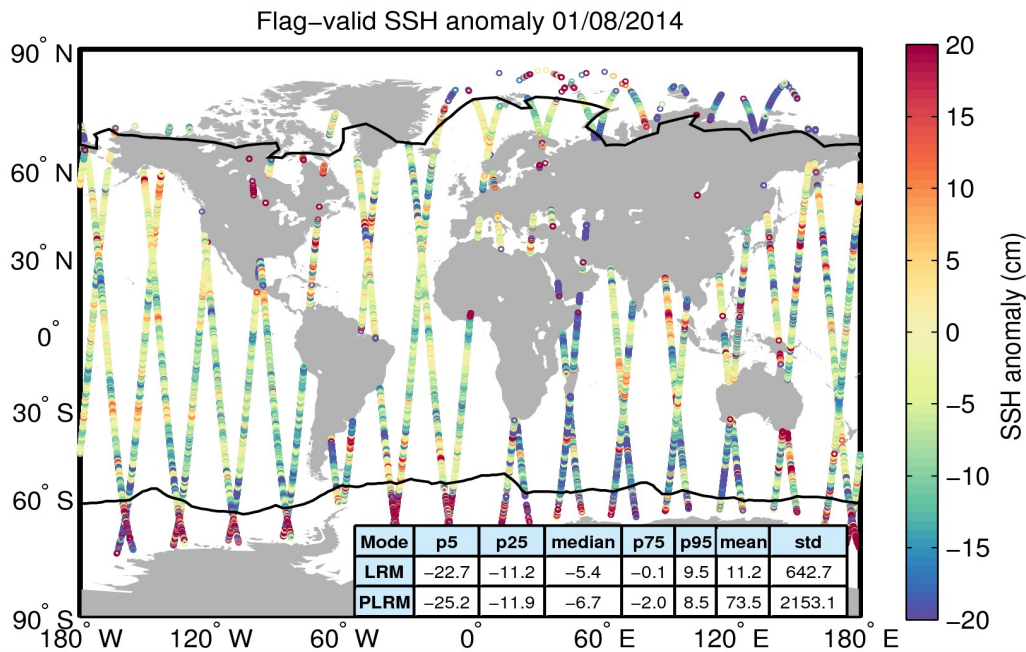
Figure 5. Geographical distribution of flag-valid 1-Hz SSH anomaly data over oceans and lakes for 01/08/2014. The statistical values shown in the table refer to the SSH anomaly in cm and are calculated separately for LRM and PLRM regions. Measurements taken over polar polygons have been excluded from the computation of the statistical values. The black lines mark the outer limit of the Arctic and Antarctic polar polygons.
