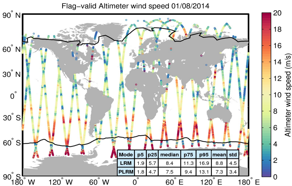
Figure 31. Geographical distribution of flag-valid wind data over oceans and lakes for 01/08/2014. The statistical values shown in the table refer to the wind in m/s and are calculated separately for LRM and PLRM regions. Measurements taken over polar polygons have been excluded from the computation of the statistical values. The black lines mark the outer limit of the Arctic and Antarctic polar polygons.
