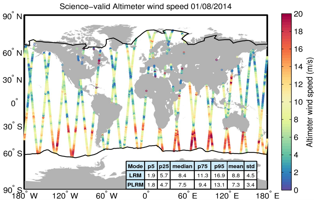
Figure 34. Geographical distribution of science-valid wind data over oceans and lakes for 01/08/2014. The statistical values shown in the table refer to the wind in m/s and are calculated separately for LRM and PLRM regions. The black lines mark the outer limit of the Arctic and Antarctic polar polygons. Gray circles denote records that have been rejected based on the editing criteria described in Table 5.
