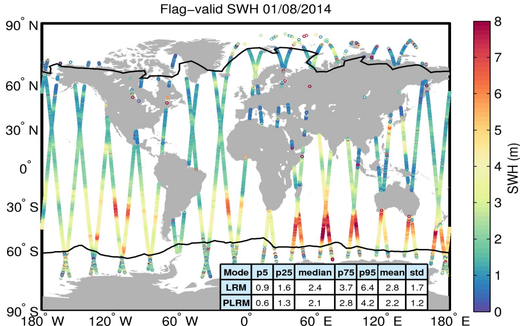
Figure 15. Geographical distribution of flag-valid SWH data over oceans and lakes for 01/08/2014. The statistical values shown in the table refer to the SWH in m and are calculated separately for LRM and PLRM regions. Measurements taken over polar polygons have been excluded from the computation of the statistical values. The black lines mark the outer limit of the Arctic and Antarctic polar polygons.
