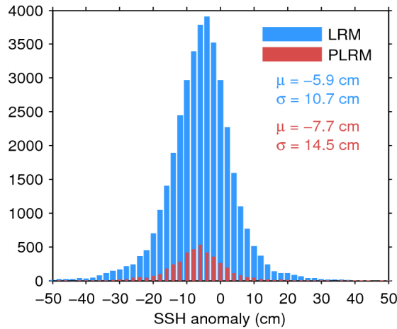
Figure 11. Histogram of science-valid SSH anomaly over oceans and lakes for LRM (blue) and PLRM (red) for 01/08/2014. The mean ( \mu ) and standard deviation ( \sigma ) are also shown. Note that values outside [-50\ 50] cm are excluded from the histogram for the sake of readability but not from the computation of \mu and \sigma .
