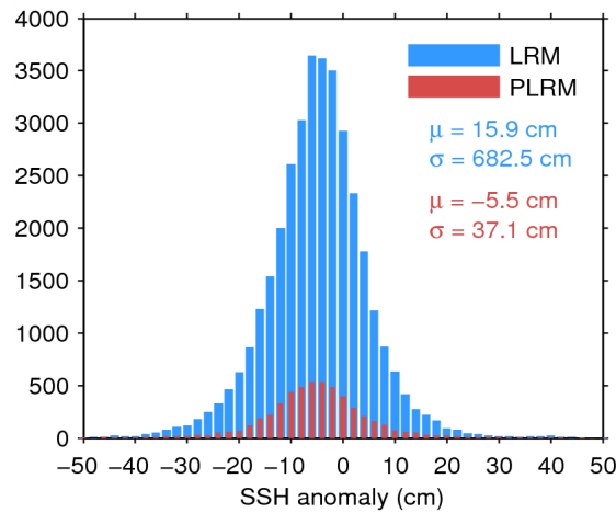
Figure 7. Histogram of flag-valid SSH anomaly over oceans and lakes for LRM (blue) and PLRM (red) for 29/07/2014. The mean ( \mu ) and standard deviation ( \sigma ) are also shown. Note that values outside [-50\ 50] cm are excluded from the histogram for the sake of readability but not from the computation of \mu and \sigma .
