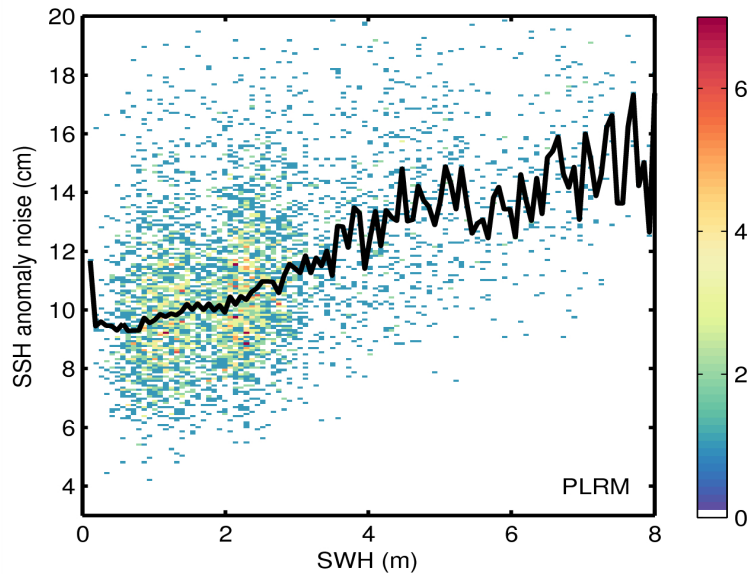
Figure 9. 2D histogram showing flag-valid SSH anomaly noise as a function of SWH for LRM (top) and PLRM (bottom) for 29/07/2014. The black line denotes the median SSH anomaly as a function of SWH.
