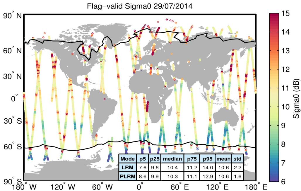
Figure 23. Geographical distribution of flag-valid sigma0 data over oceans and lakes for 29/07/2014. The statistical values shown in the table refer to the sigma0 in dB and are calculated separately for LRM and PLRM regions. Measurements taken over polar polygons have been excluded from the computation of the statistical values. The black lines mark the outer limit of the Arctic and Antarctic polar polygons.
