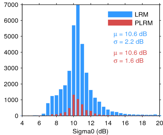
Figure 25. Histogram of flag-valid sigma0 over oceans and lakes for LRM (blue) and PLRM (red) for 29/07/2014. The mean ( \mu ) and standard deviation ( \sigma ) are also shown. Note that values outside [4 20] dB are excluded from the histogram for the sake of readability but not from the computation of \mu and \sigma .
