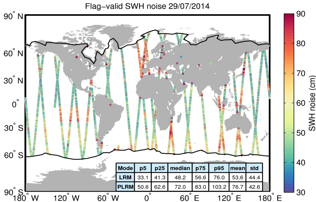
Figure 18. Geographical distribution of flag-valid 20-Hz SWH measurement noise over oceans and lakes for 29/07/2014. The statistical values shown in the table refer to the SWH noise and are calculated separately for LRM and PLRM regions. Measurements taken over polar polygons have been excluded from the computation of the statistical values. The black lines mark the outer limit of the Arctic and Antarctic polar polygons.
