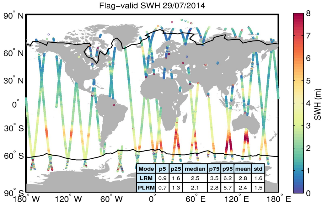
Figure 15. Geographical distribution of flag-valid SWH data over oceans and lakes for 29/07/2014. The statistical values shown in the table refer to the SWH in m and are calculated separately for LRM and PLRM regions. Measurements taken over polar polygons have been excluded from the computation of the statistical values. The black lines mark the outer limit of the Arctic and Antarctic polar polygons.
