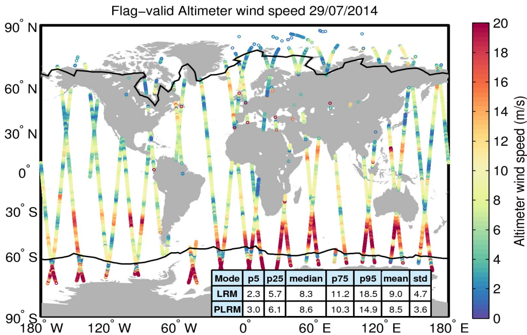
Figure 31. Geographical distribution of flag-valid wind data over oceans and lakes for 29/07/2014. The statistical values shown in the table refer to the wind in m/s and are calculated separately for LRM and PLRM regions. Measurements taken over polar polygons have been excluded from the computation of the statistical values. The black lines mark the outer limit of the Arctic and Antarctic polar polygons.
