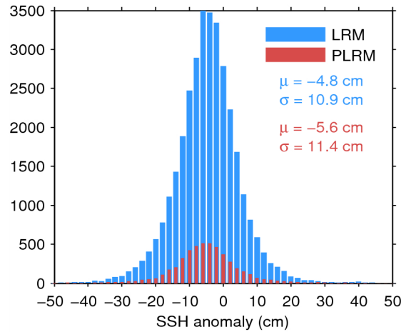
Figure 11. Histogram of science-valid SSH anomaly over oceans and lakes for LRM (blue) and PLRM (red) for 29/07/2014. The mean ( \mu ) and standard deviation ( \sigma ) are also shown. Note that values outside [-50 50] cm are excluded from the histogram for the sake of readability but not from the computation of \mu and \sigma .
