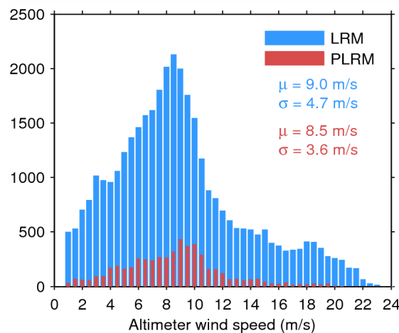
Figure 35. Histogram of science-valid wind over oceans and lakes for LRM (blue) and PLRM (red) for 29/07/2014. The mean ( \mu ) and standard deviation ( \sigma ) are also shown. Note that values larger than 24 m/s are excluded from the histogram for the sake of readability but not from the computation of \mu and \sigma .
