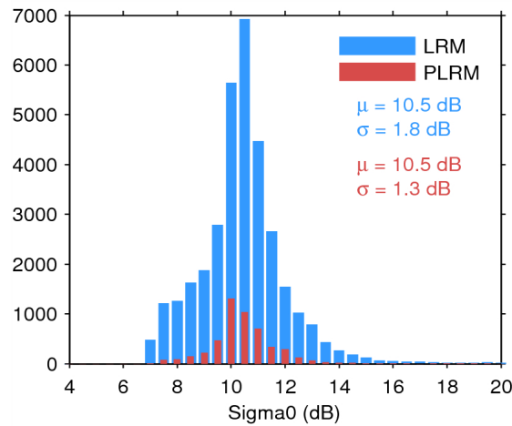
Figure 28. Histogram of science-valid sigma0 over oceans and lakes for LRM (blue) and PLRM (red) for 29/07/2014. The mean ( \mu ) and standard deviation ( \sigma ) are also shown. Note that values outside [4 20] dB are excluded from the histogram for the sake of readability but not from the computation of \mu and \sigma .
