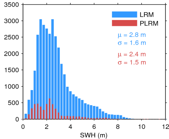
Figure 17. Histogram of flag-valid SWH over oceans and lakes for LRM (blue) and PLRM (red) for 29/07/2014. The mean ( \mu ) and standard deviation ( \sigma ) are also shown. Note that values larger than 12 m are excluded from the histogram for the sake of readability but not from the computation of \mu and \sigma .
