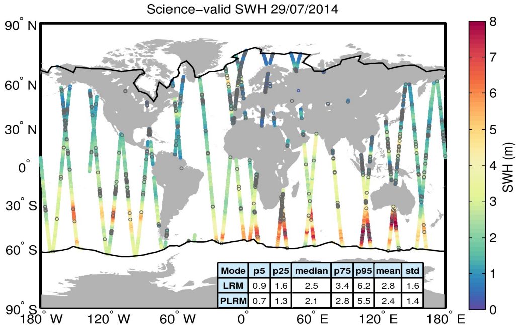
Figure 19. Geographical distribution of science-valid SWH data over oceans and lakes for 29/07/2014. The statistical values shown in the table refer to the SWH in m and are calculated separately for LRM and PLRM regions. The black lines mark the outer limit of the Arctic and Antarctic polar polygons. Gray circles denote records that have been rejected based on the editing criteria described in Table 3.
