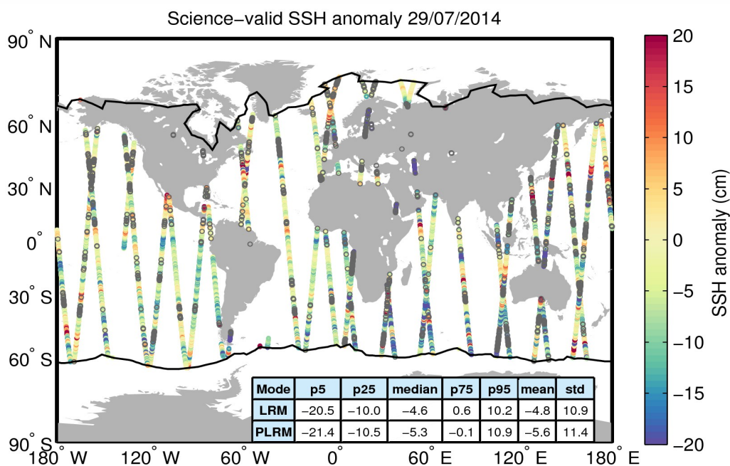
Figure 10. Geographical distribution of science-valid SSH anomaly data over oceans and lakes for 29/07/2014. The statistical values shown in the table refer to the SSH anomaly in cm and are calculated separately for LRM and PLRM regions. The black lines mark the outer limit of the Arctic and Antarctic polar polygons. Gray circles denote records that have been rejected based on the editing criteria described in Table 2.
