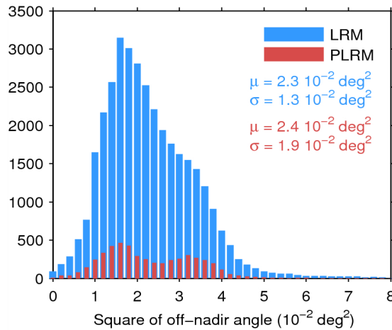
Figure 39. Histogram of flag-valid mispointing over oceans and lakes for LRM (blue) and PLRM (red) for 29/07/2014. Only positive values have been considered. The mean ( \mu ) and standard deviation ( \sigma ) are also shown. Note that values 8 \cdot 10^{-2} \text{ deg}^2 are excluded from the histogram for the sake of readability but not from the computation of \mu and \sigma .
