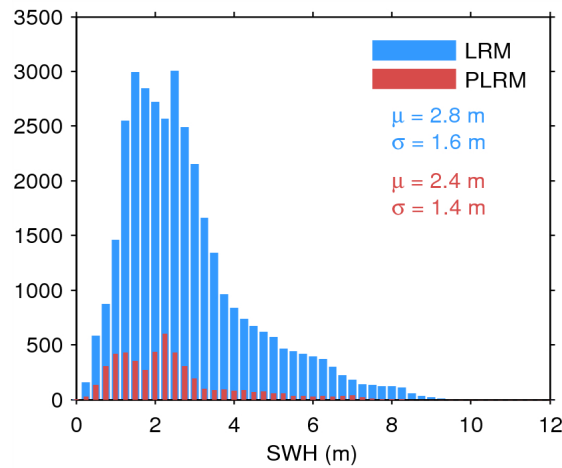
Figure 20. Histogram of science-valid SWH over oceans and lakes for LRM (blue) and PLRM (red) for 29/07/2014. The mean ( \mu ) and standard deviation ( \sigma ) are also shown. Note that values larger than 12 m are excluded from the histogram for the sake of readability but not from the computation of \mu and \sigma .
