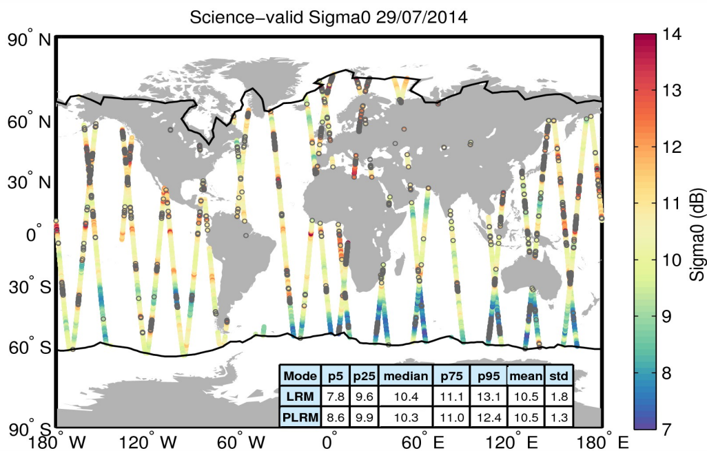
Figure 27. Geographical distribution of science-valid sigma0 data over oceans and lakes for 29/07/2014. The statistical values shown in the table refer to the sigma0 in dB and are calculated separately for LRM and PLRM regions. The black lines mark the outer limit of the Arctic and Antarctic polar polygons. Gray circles denote records that have been rejected based on the editing criteria described in Table 4.
