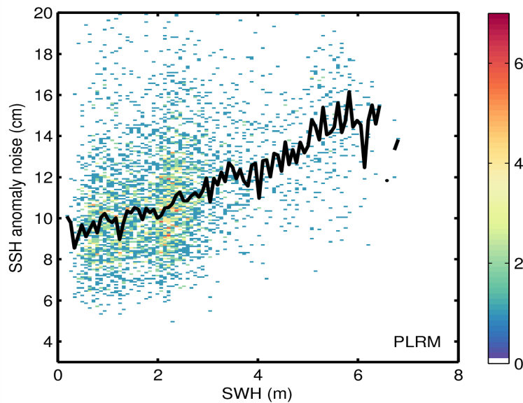
Figure 9. 2D histogram showing flag-valid SSH anomaly noise as a function of SWH for LRM (top) and PLRM (bottom) for 28/07/2014. The black line denotes the median SSH anomaly as a function of SWH.
