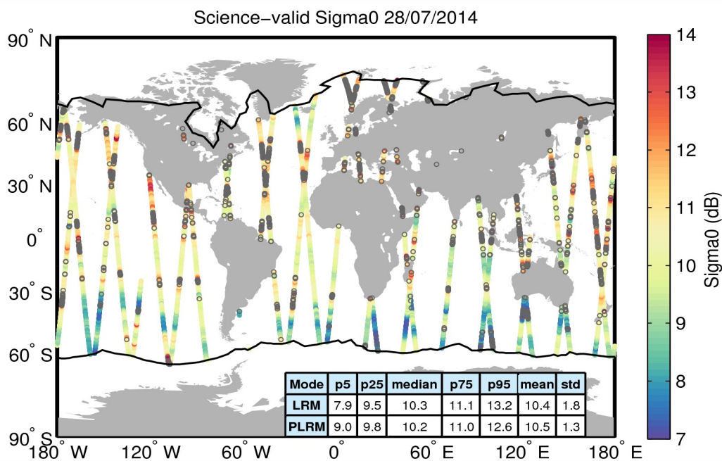
Figure 27. Geographical distribution of science-valid sigma0 data over oceans and lakes for 28/07/2014. The statistical values shown in the table refer to the sigma0 in dB and are calculated separately for LRM and PLRM regions. The black lines mark the outer limit of the Arctic and Antarctic polar polygons. Gray circles denote records that have been rejected based on the editing criteria described in Table 4.
