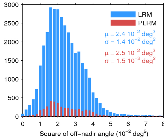
Figure 39. Histogram of flag-valid mispointing over oceans and lakes for LRM (blue) and PLRM (red) for 28/07/2014. Only positive values have been considered. The mean ( \mu ) and standard deviation ( \sigma ) are also shown. Note that values 8 \cdot 10^{-2} \text{ deg}^2 are excluded from the histogram for the sake of readability but not from the computation of \mu and \sigma .
