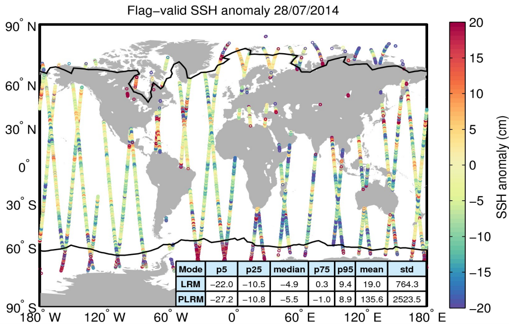
Figure 5. Geographical distribution of flag-valid 1-Hz SSH anomaly data over oceans and lakes for 28/07/2014. The statistical values shown in the table refer to the SSH anomaly in cm and are calculated separately for LRM and PLRM regions. Measurements taken over polar polygons have been excluded from the computation of the statistical values. The black lines mark the outer limit of the Arctic and Antarctic polar polygons.
