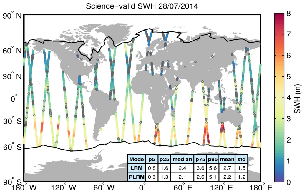
Figure 19. Geographical distribution of science-valid SWH data over oceans and lakes for 28/07/2014. The statistical values shown in the table refer to the SWH in m and are calculated separately for LRM and PLRM regions. The black lines mark the outer limit of the Arctic and Antarctic polar polygons. Gray circles denote records that have been rejected based on the editing criteria described in Table 3.
