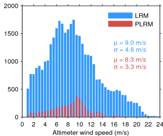
Figure 35. Histogram of science-valid wind over oceans and lakes for LRM (blue) and PLRM (red) for 28/07/2014. The mean ( \mu ) and standard deviation ( \sigma ) are also shown. Note that values larger than 24 m/s are excluded from the histogram for the sake of readability but not from the computation of \mu and \sigma .
