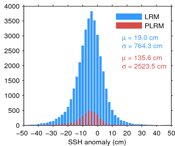
Figure 7. Histogram of flag-valid SSH anomaly over oceans and lakes for LRM (blue) and PLRM (red) for 28/07/2014. The mean ( \mu ) and standard deviation ( \sigma ) are also shown. Note that values outside [-50\ 50] cm are excluded from the histogram for the sake of readability but not from the computation of \mu and \sigma .
