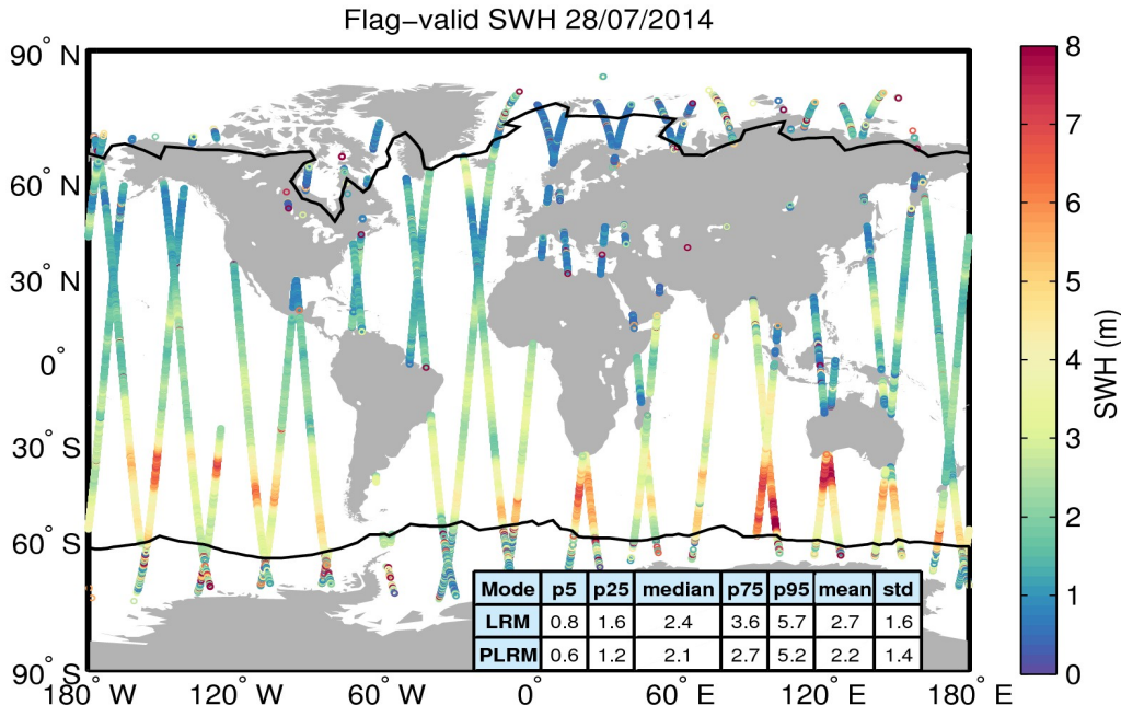
Figure 15. Geographical distribution of flag-valid SWH data over oceans and lakes for 28/07/2014. The statistical values shown in the table refer to the SWH in m and are calculated separately for LRM and PLRM regions. Measurements taken over polar polygons have been excluded from the computation of the statistical values. The black lines mark the outer limit of the Arctic and Antarctic polar polygons.
