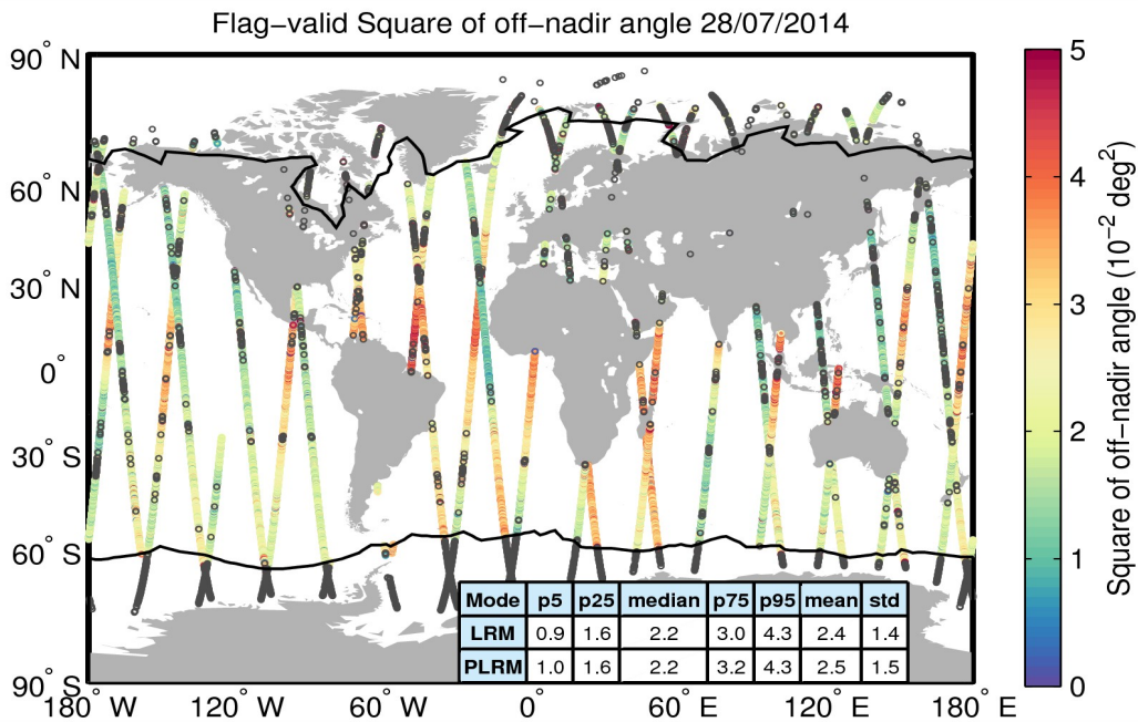
Figure 37. Geographical distribution of flag-valid mispointing data over oceans and lakes for 28/07/2014. The statistical values shown in the table refer to the mispointing in 10^{-2} \text{ deg}^2 and are calculated separately for LRM and PLRM regions. Measurements taken over polar polygons have been excluded from the computation of the statistical values. The black lines mark the outer limit of the Arctic and Antarctic polar polygons. Gray circles denote negative values.
