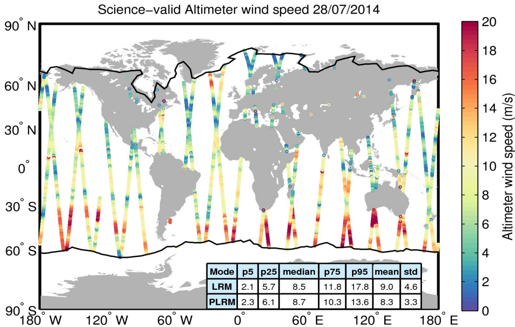
Figure 34. Geographical distribution of science-valid wind data over oceans and lakes for 28/07/2014. The statistical values shown in the table refer to the wind in m/s and are calculated separately for LRM and PLRM regions. The black lines mark the outer limit of the Arctic and Antarctic polar polygons. Gray circles denote records that have been rejected based on the editing criteria described in Table 5.
