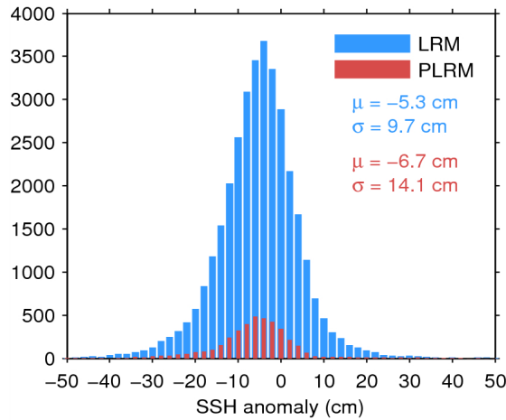
Figure 11. Histogram of science-valid SSH anomaly over oceans and lakes for LRM (blue) and PLRM (red) for 28/07/2014. The mean ( \mu ) and standard deviation ( \sigma ) are also shown. Note that values outside [-50 50] cm are excluded from the histogram for the sake of readability but not from the computation of \mu and \sigma .
