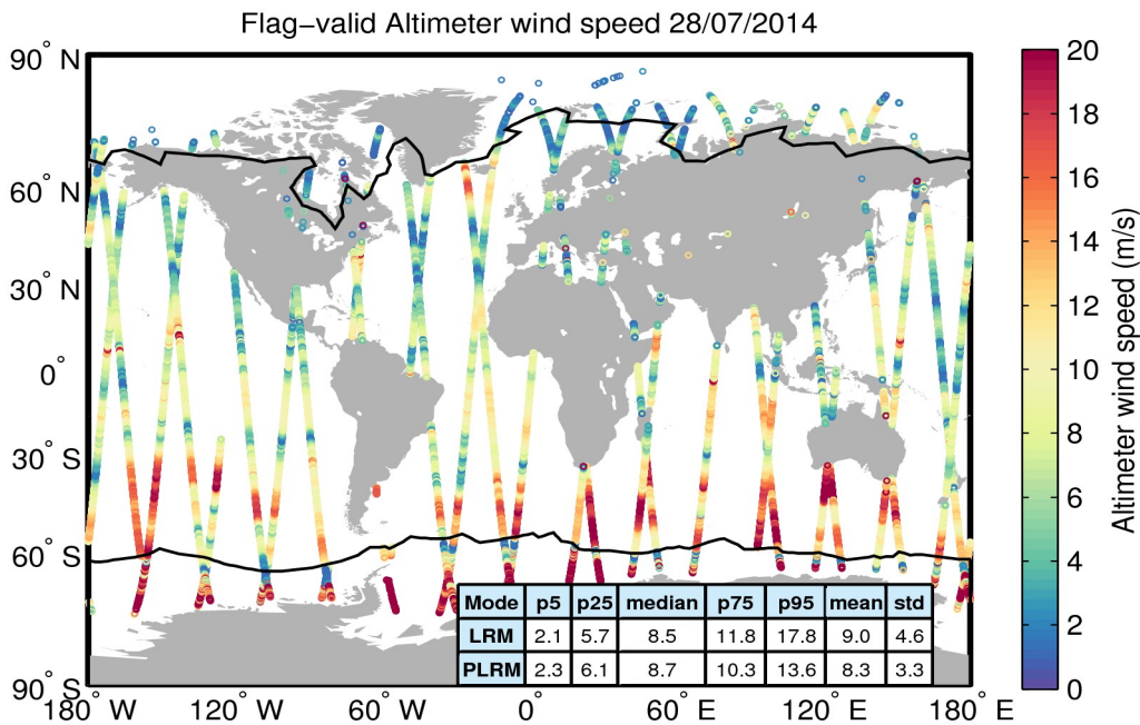
Figure 31. Geographical distribution of flag-valid wind data over oceans and lakes for 28/07/2014. The statistical values shown in the table refer to the wind in m/s and are calculated separately for LRM and PLRM regions. Measurements taken over polar polygons have been excluded from the computation of the statistical values. The black lines mark the outer limit of the Arctic and Antarctic polar polygons.
