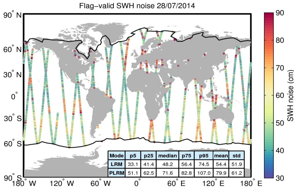
Figure 18. Geographical distribution of flag-valid 20-Hz SWH measurement noise over oceans and lakes for 28/07/2014. The statistical values shown in the table refer to the SWH noise and are calculated separately for LRM and PLRM regions. Measurements taken over polar polygons have been excluded from the computation of the statistical values. The black lines mark the outer limit of the Arctic and Antarctic polar polygons.
