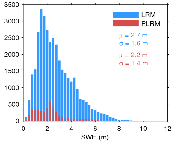
Figure 17. Histogram of flag-valid SWH over oceans and lakes for LRM (blue) and PLRM (red) for 28/07/2014. The mean ( \mu ) and standard deviation ( \sigma ) are also shown. Note that values larger than 12 m are excluded from the histogram for the sake of readability but not from the computation of \mu and \sigma .
