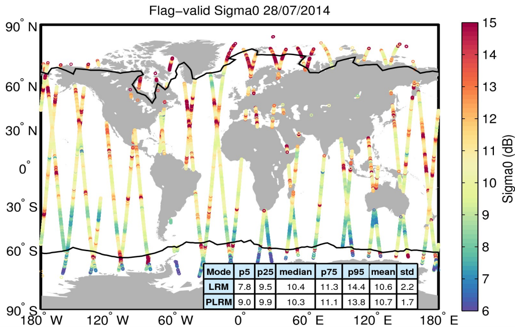
Figure 23. Geographical distribution of flag-valid sigma0 data over oceans and lakes for 28/07/2014. The statistical values shown in the table refer to the sigma0 in dB and are calculated separately for LRM and PLRM regions. Measurements taken over polar polygons have been excluded from the computation of the statistical values. The black lines mark the outer limit of the Arctic and Antarctic polar polygons.
