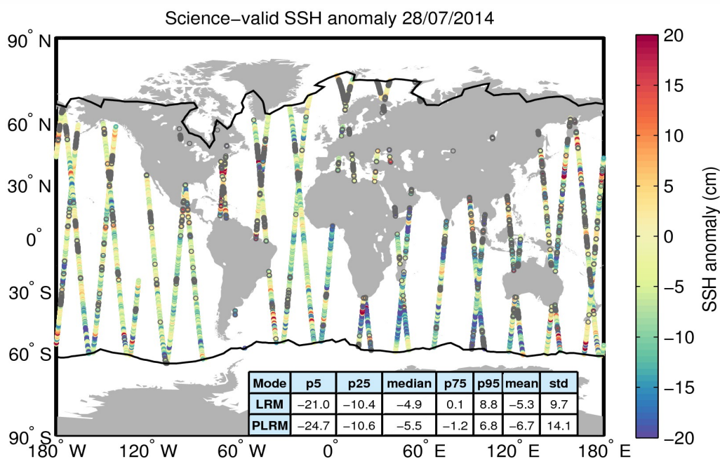
Figure 10. Geographical distribution of science-valid SSH anomaly data over oceans and lakes for 28/07/2014. The statistical values shown in the table refer to the SSH anomaly in cm and are calculated separately for LRM and PLRM regions. The black lines mark the outer limit of the Arctic and Antarctic polar polygons. Gray circles denote records that have been rejected based on the editing criteria described in Table 2.
