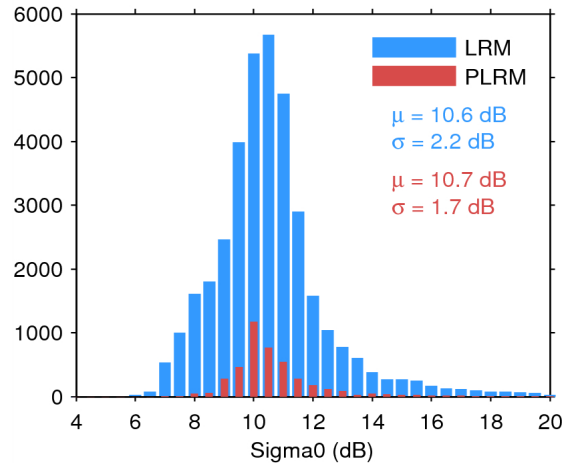
Figure 25. Histogram of flag-valid sigma0 over oceans and lakes for LRM (blue) and PLRM (red) for 28/07/2014. The mean ( \mu ) and standard deviation ( \sigma ) are also shown. Note that values outside [4 20] dB are excluded from the histogram for the sake of readability but not from the computation of \mu and \sigma .
