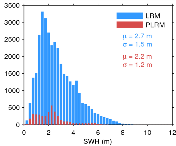
Figure 20. Histogram of science-valid SWH over oceans and lakes for LRM (blue) and PLRM (red) for 28/07/2014. The mean ( \mu ) and standard deviation ( \sigma ) are also shown. Note that values larger than 12 m are excluded from the histogram for the sake of readability but not from the computation of \mu and \sigma .
