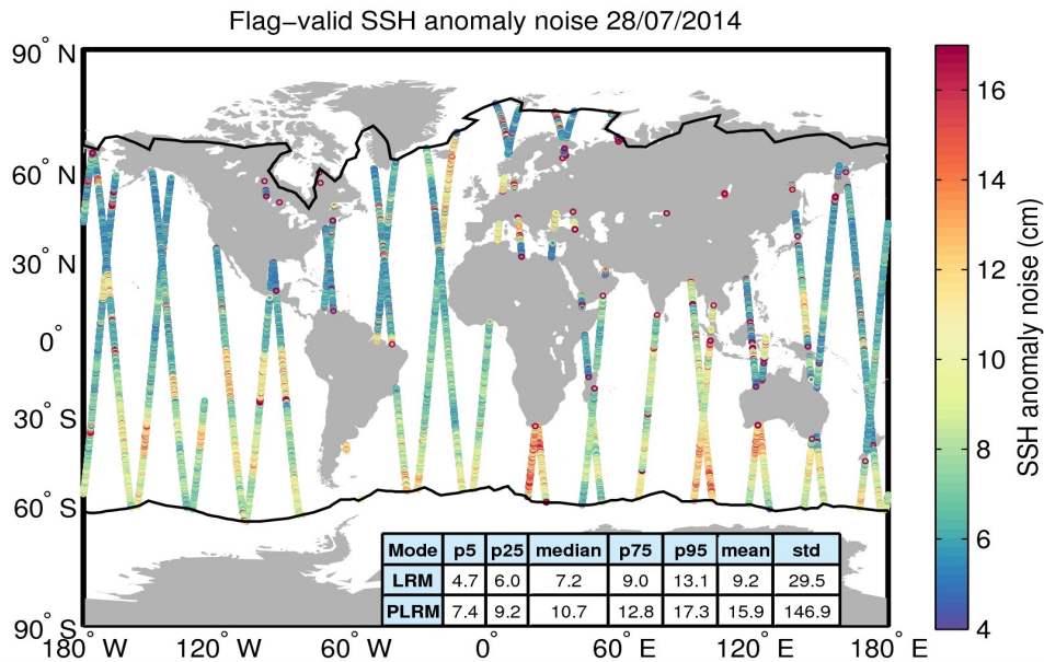
Figure 8. Geographical distribution of flag-valid 20-Hz SSH anomaly measurement noise over oceans and lakes for 28/07/2014. The statistical values shown in the table refer to the SSH anomaly noise and are calculated separately for LRM and PLRM regions. Measurements taken over polar polygons have been excluded from the computation of the statistical values. The black lines mark the outer limit of the Arctic and Antarctic polar polygons.
