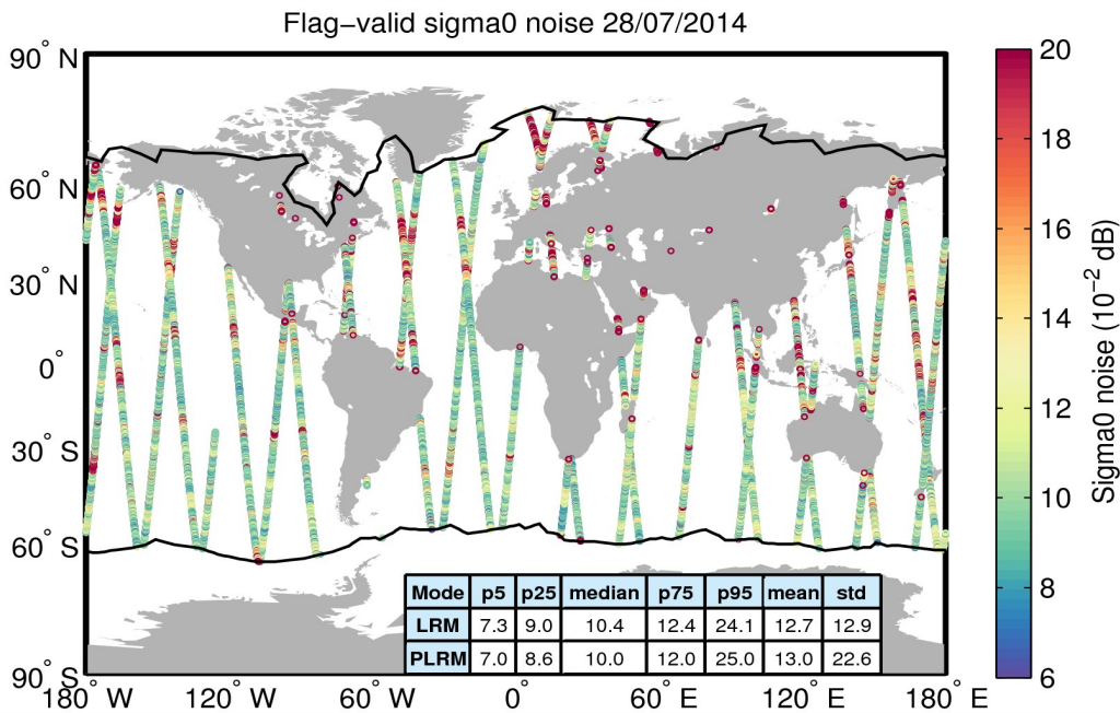
Figure 26. Geographical distribution of flag-valid 20-Hz sigma0 measurement noise over oceans and lakes for 28/07/2014. The statistical values shown in the table refer to the sigma0 noise and are calculated separately for LRM and PLRM regions. Measurements taken over polar polygons have been excluded from the computation of the statistical values. The black lines mark the outer limit of the Arctic and Antarctic polar polygons.
