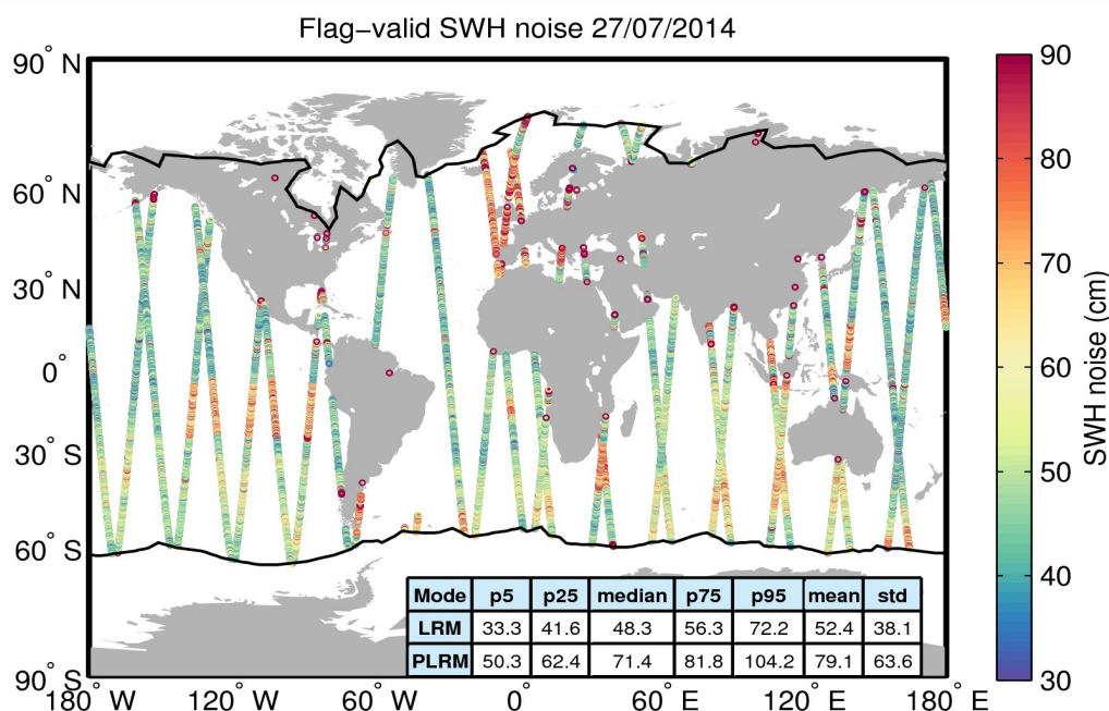
Figure 18. Geographical distribution of flag-valid 20-Hz SWH measurement noise over oceans and lakes for 27/07/2014. The statistical values shown in the table refer to the SWH noise and are calculated separately for LRM and PLRM regions. Measurements taken over polar polygons have been excluded from the computation of the statistical values. The black lines mark the outer limit of the Arctic and Antarctic polar polygons.
