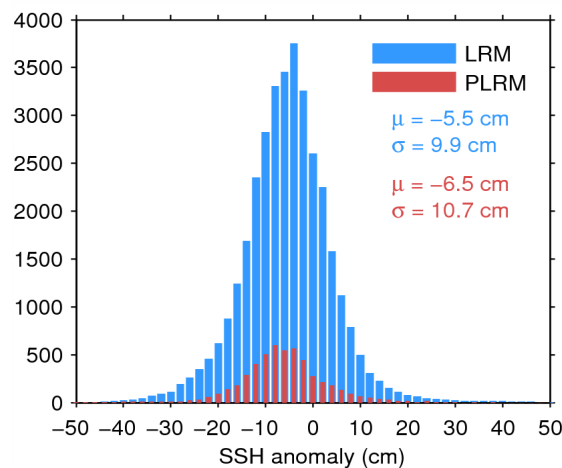
Figure 11. Histogram of science-valid SSH anomaly over oceans and lakes for LRM (blue) and PLRM (red) for 27/07/2014. The mean ( \mu ) and standard deviation ( \sigma ) are also shown. Note that values outside [-50 50] cm are excluded from the histogram for the sake of readability but not from the computation of \mu and \sigma .
