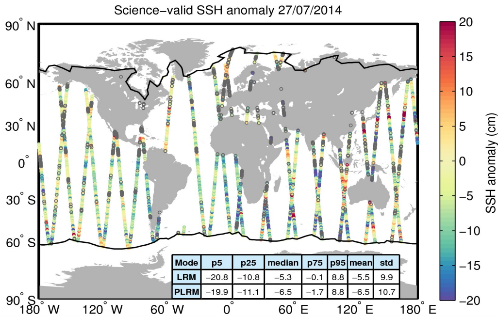
Figure 10. Geographical distribution of science-valid SSH anomaly data over oceans and lakes for 27/07/2014. The statistical values shown in the table refer to the SSH anomaly in cm and are calculated separately for LRM and PLRM regions. The black lines mark the outer limit of the Arctic and Antarctic polar polygons. Gray circles denote records that have been rejected based on the editing criteria described in Table 2.
