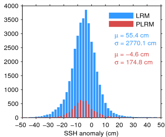
Figure 7. Histogram of flag-valid SSH anomaly over oceans and lakes for LRM (blue) and PLRM (red) for 27/07/2014. The mean ( \mu ) and standard deviation ( \sigma ) are also shown. Note that values outside [-50 50] cm are excluded from the histogram for the sake of readability but not from the computation of \mu and \sigma .
