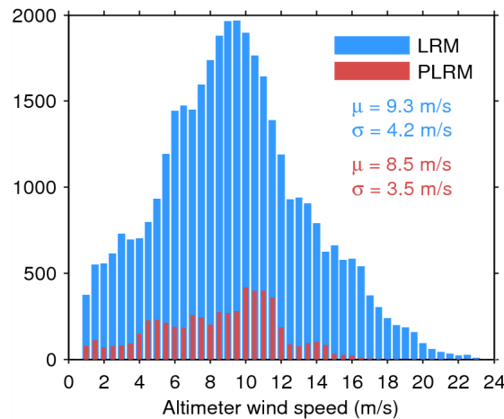
Figure 33. Histogram of flag-valid wind over oceans and lakes for LRM (blue) and PLRM (red) for 27/07/2014. The mean ( \mu ) and standard deviation ( \sigma ) are also shown. Note that values larger than 24 m/s are excluded from the histogram for the sake of readability but not from the computation of \mu and \sigma .
