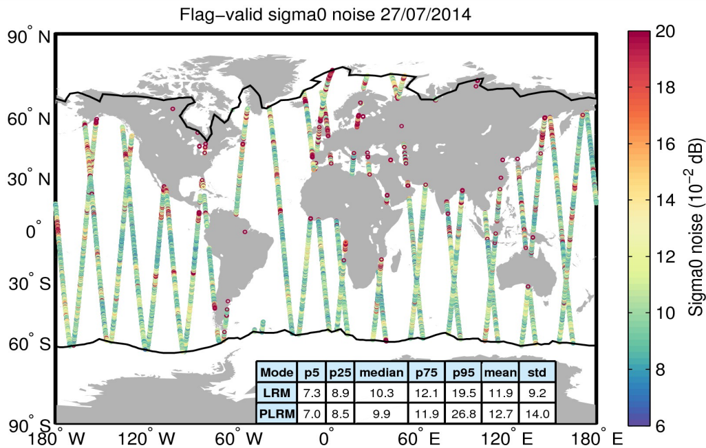
Figure 26. Geographical distribution of flag-valid 20-Hz sigma0 measurement noise over oceans and lakes for 27/07/2014. The statistical values shown in the table refer to the sigma0 noise and are calculated separately for LRM and PLRM regions. Measurements taken over polar polygons have been excluded from the computation of the statistical values. The black lines mark the outer limit of the Arctic and Antarctic polar polygons.
