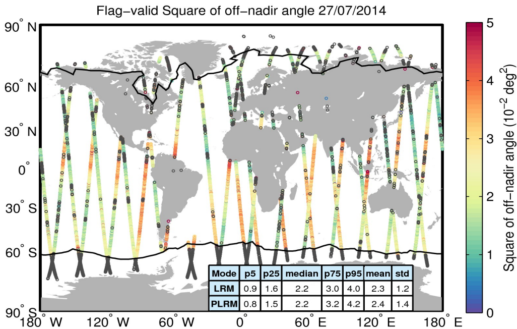
Figure 37. Geographical distribution of flag-valid mispointing data over oceans and lakes for 27/07/2014. The statistical values shown in the table refer to the mispointing in 10^{-2} \text{ deg}^2 and are calculated separately for LRM and PLRM regions. Measurements taken over polar polygons have been excluded from the computation of the statistical values. The black lines mark the outer limit of the Arctic and Antarctic polar polygons. Gray circles denote negative values.
