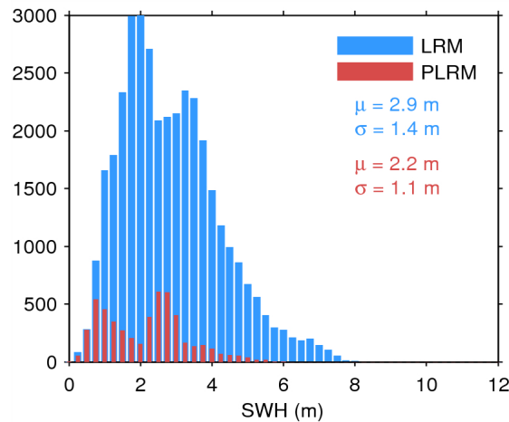
Figure 20. Histogram of science-valid SWH over oceans and lakes for LRM (blue) and PLRM (red) for 27/07/2014. The mean ( \mu ) and standard deviation ( \sigma ) are also shown. Note that values larger than 12 m are excluded from the histogram for the sake of readability but not from the computation of \mu and \sigma .
