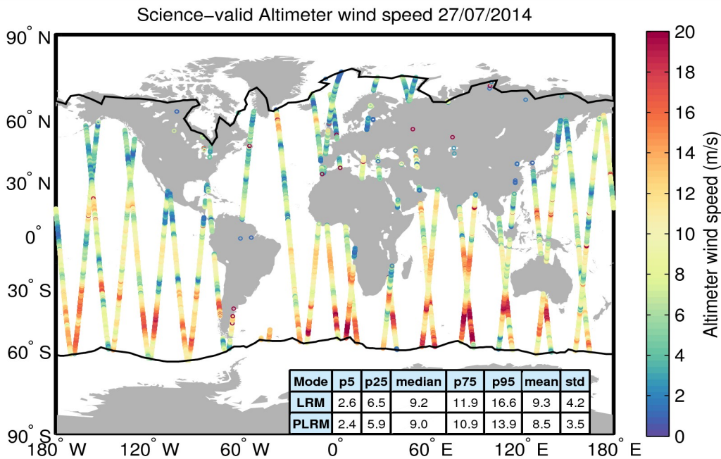
Figure 34. Geographical distribution of science-valid wind data over oceans and lakes for 27/07/2014. The statistical values shown in the table refer to the wind in m/s and are calculated separately for LRM and PLRM regions. The black lines mark the outer limit of the Arctic and Antarctic polar polygons. Gray circles denote records that have been rejected based on the editing criteria described in Table 5.
