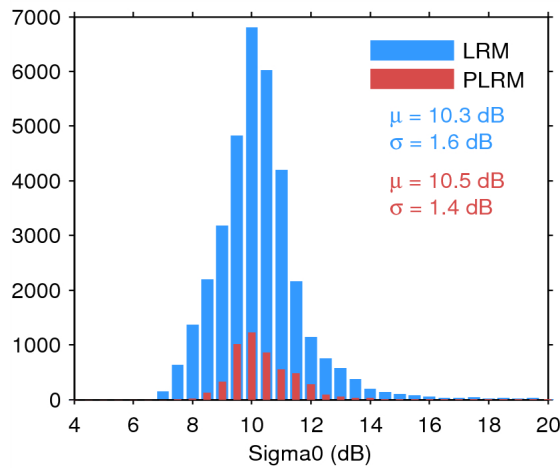
Figure 28. Histogram of science-valid sigma0 over oceans and lakes for LRM (blue) and PLRM (red) for 27/07/2014. The mean ( \mu ) and standard deviation ( \sigma ) are also shown. Note that values outside [4 20] dB are excluded from the histogram for the sake of readability but not from the computation of \mu and \sigma .
