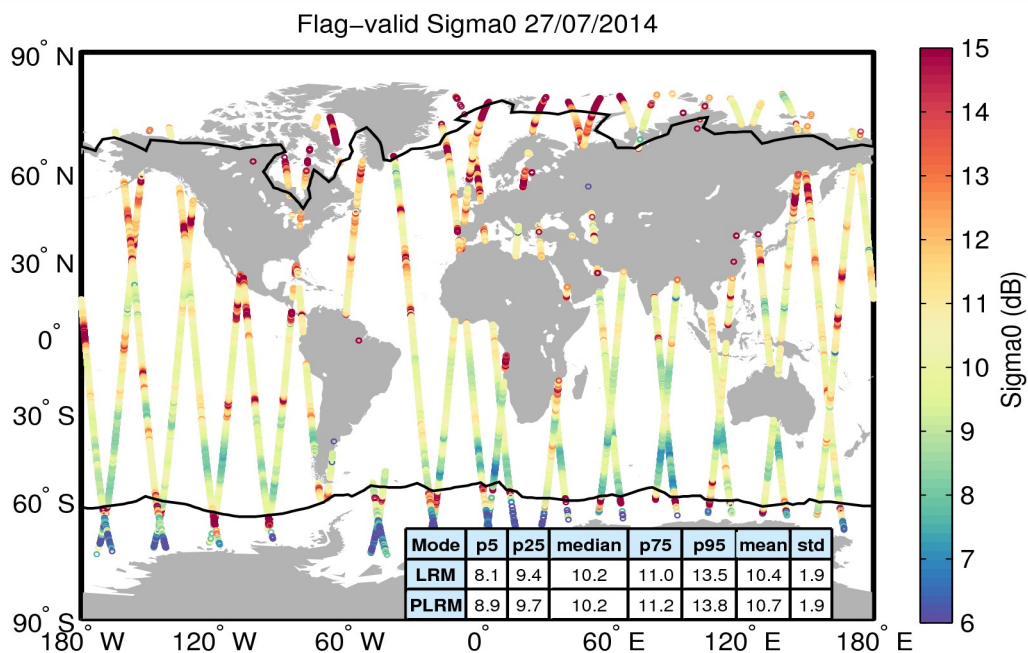
Figure 23. Geographical distribution of flag-valid sigma0 data over oceans and lakes for 27/07/2014. The statistical values shown in the table refer to the sigma0 in dB and are calculated separately for LRM and PLRM regions. Measurements taken over polar polygons have been excluded from the computation of the statistical values. The black lines mark the outer limit of the Arctic and Antarctic polar polygons.
