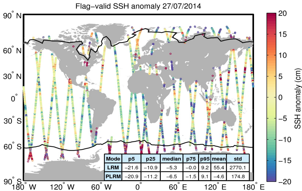
Figure 5. Geographical distribution of flag-valid 1-Hz SSH anomaly data over oceans and lakes for 27/07/2014. The statistical values shown in the table refer to the SSH anomaly in cm and are calculated separately for LRM and PLRM regions. Measurements taken over polar polygons have been excluded from the computation of the statistical values. The black lines mark the outer limit of the Arctic and Antarctic polar polygons.
