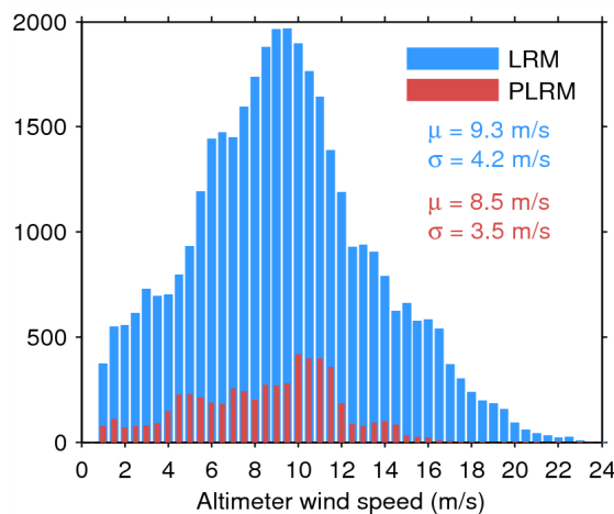
Figure 35. Histogram of science-valid wind over oceans and lakes for LRM (blue) and PLRM (red) for 27/07/2014. The mean ( \mu ) and standard deviation ( \sigma ) are also shown. Note that values larger than 24 m/s are excluded from the histogram for the sake of readability but not from the computation of \mu and \sigma .
