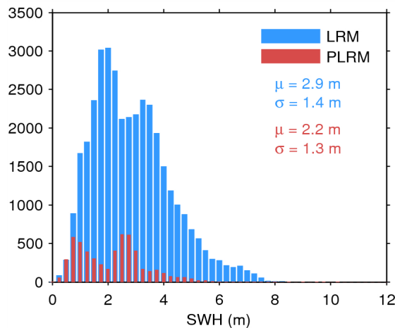
Figure 17. Histogram of flag-valid SWH over oceans and lakes for LRM (blue) and PLRM (red) for 27/07/2014. The mean ( \mu ) and standard deviation ( \sigma ) are also shown. Note that values larger than 12 m are excluded from the histogram for the sake of readability but not from the computation of \mu and \sigma .
