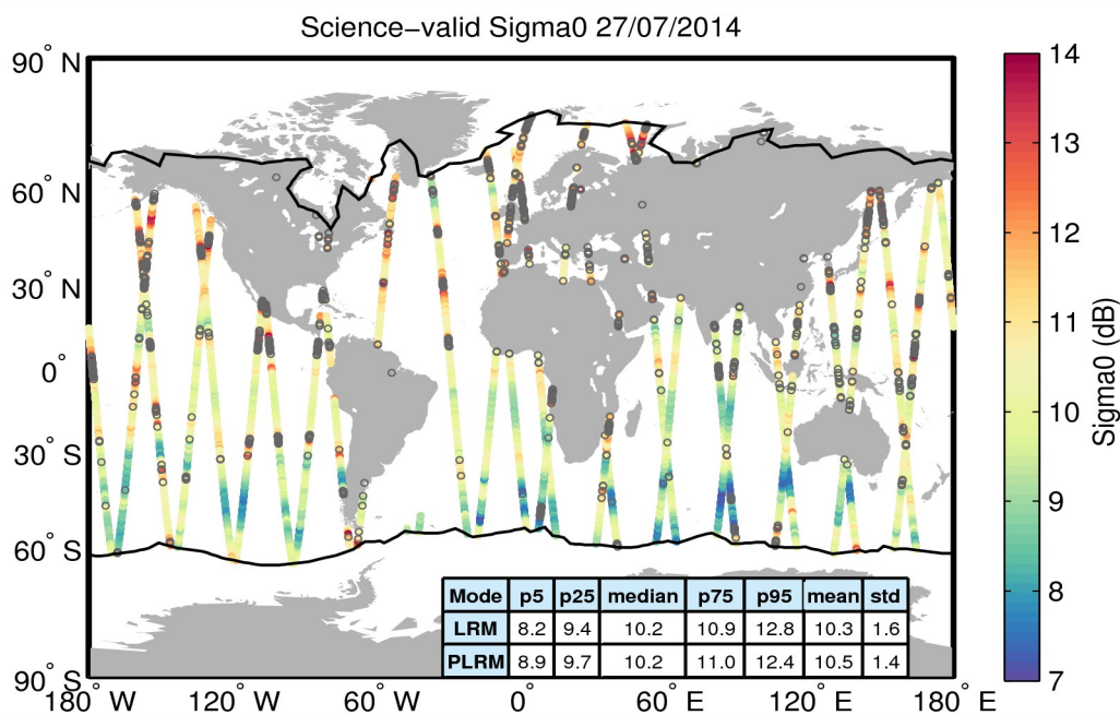
Figure 27. Geographical distribution of science-valid sigma0 data over oceans and lakes for 27/07/2014. The statistical values shown in the table refer to the sigma0 in dB and are calculated separately for LRM and PLRM regions. The black lines mark the outer limit of the Arctic and Antarctic polar polygons. Gray circles denote records that have been rejected based on the editing criteria described in Table 4.
