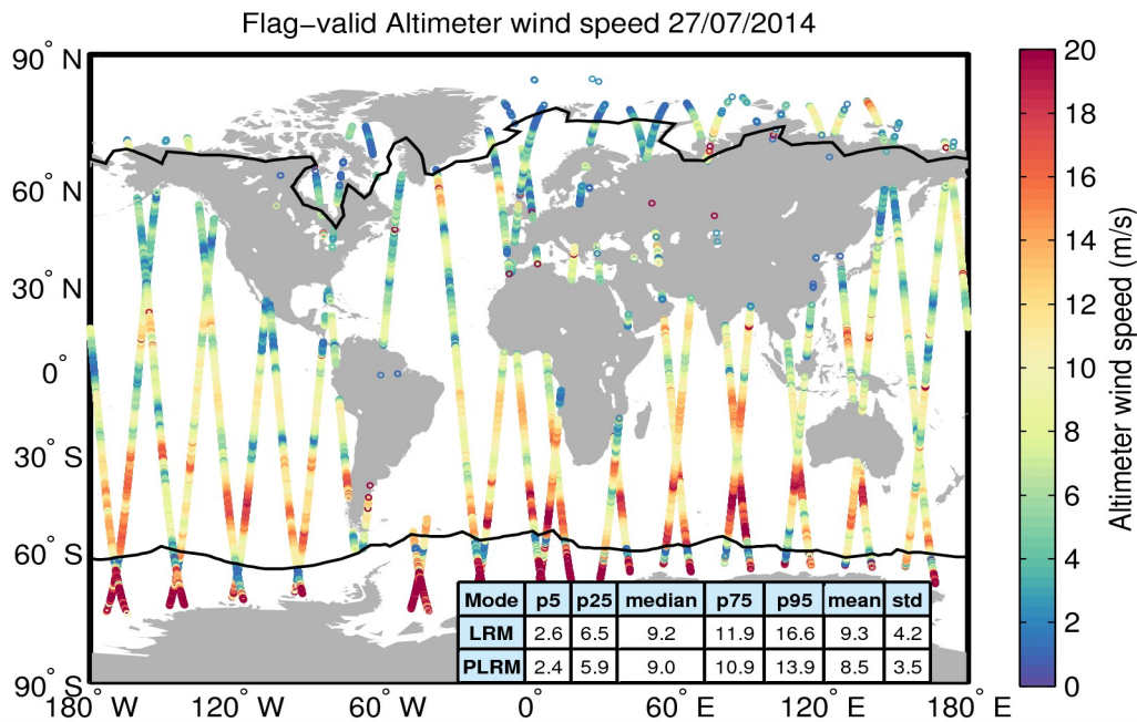
Figure 31. Geographical distribution of flag-valid wind data over oceans and lakes for 27/07/2014. The statistical values shown in the table refer to the wind in m/s and are calculated separately for LRM and PLRM regions. Measurements taken over polar polygons have been excluded from the computation of the statistical values. The black lines mark the outer limit of the Arctic and Antarctic polar polygons.
