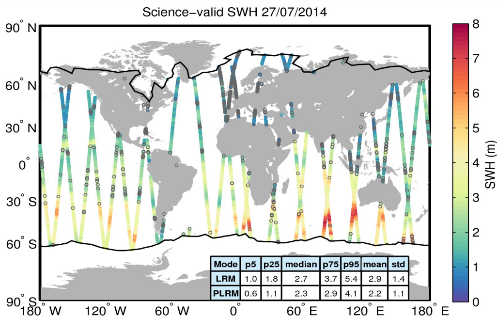
Figure 19. Geographical distribution of science-valid SWH data over oceans and lakes for 27/07/2014. The statistical values shown in the table refer to the SWH in m and are calculated separately for LRM and PLRM regions. The black lines mark the outer limit of the Arctic and Antarctic polar polygons. Gray circles denote records that have been rejected based on the editing criteria described in Table 3.
