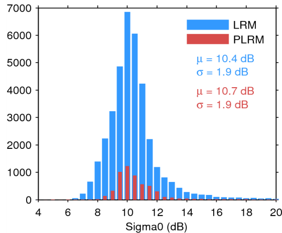
Figure 25. Histogram of flag-valid sigma0 over oceans and lakes for LRM (blue) and PLRM (red) for 27/07/2014. The mean ( \mu ) and standard deviation ( \sigma ) are also shown. Note that values outside [4 20] dB are excluded from the histogram for the sake of readability but not from the computation of \mu and \sigma .
