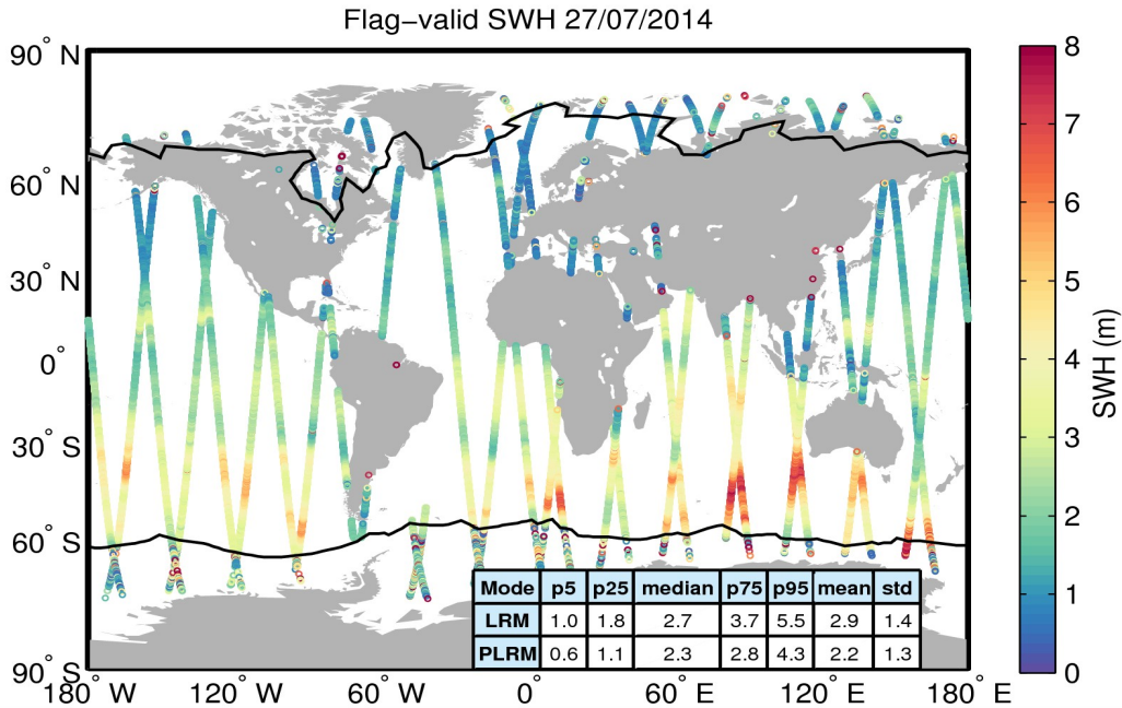
Figure 15. Geographical distribution of flag-valid SWH data over oceans and lakes for 27/07/2014. The statistical values shown in the table refer to the SWH in m and are calculated separately for LRM and PLRM regions. Measurements taken over polar polygons have been excluded from the computation of the statistical values. The black lines mark the outer limit of the Arctic and Antarctic polar polygons.
