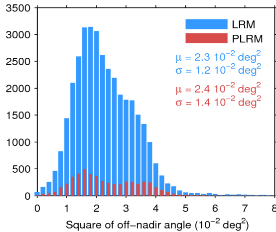
Figure 39. Histogram of flag-valid mispointing over oceans and lakes for LRM (blue) and PLRM (red) for 27/07/2014. Only positive values have been considered. The mean ( \mu ) and standard deviation ( \sigma ) are also shown. Note that values 8 \cdot 10^{-2} \text{ deg}^2 are excluded from the histogram for the sake of readability but not from the computation of \mu and \sigma .
