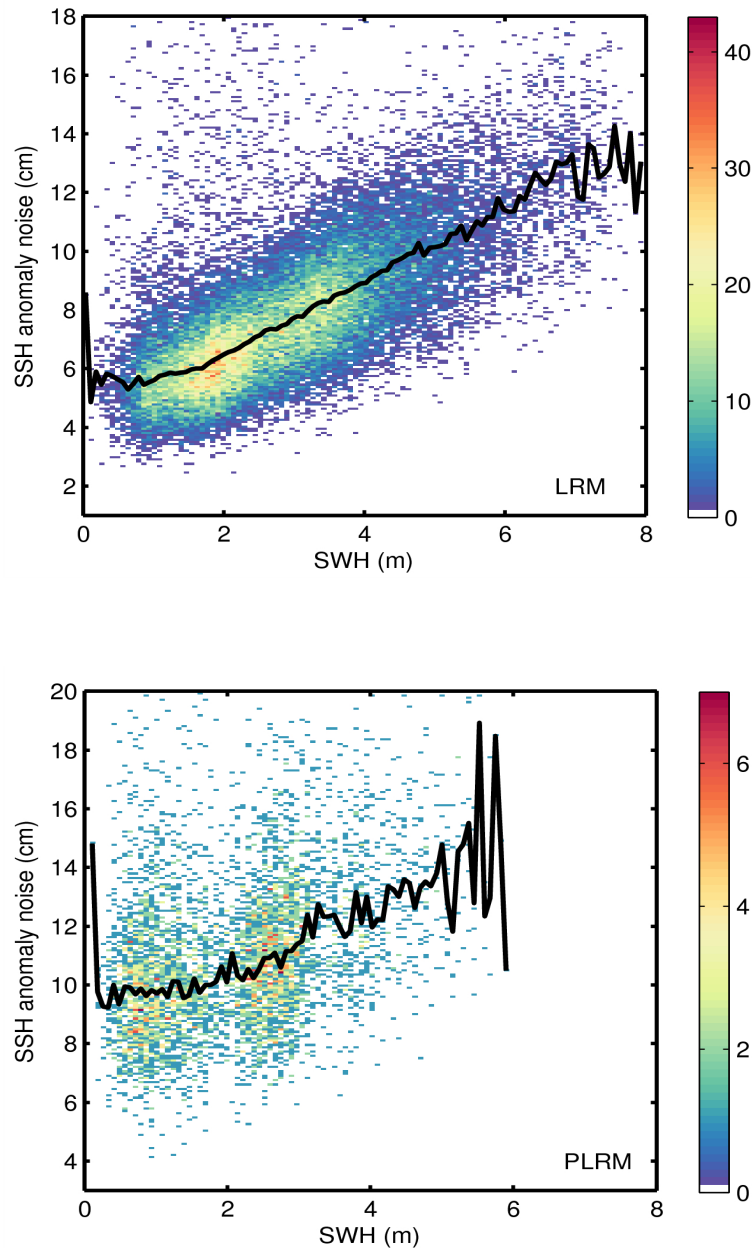
Figure 9. 2D histogram showing flag-valid SSH anomaly noise as a function of SWH for LRM (top) and PLRM (bottom) for 27/07/2014. The black line denotes the median SSH anomaly as a function of SWH.
