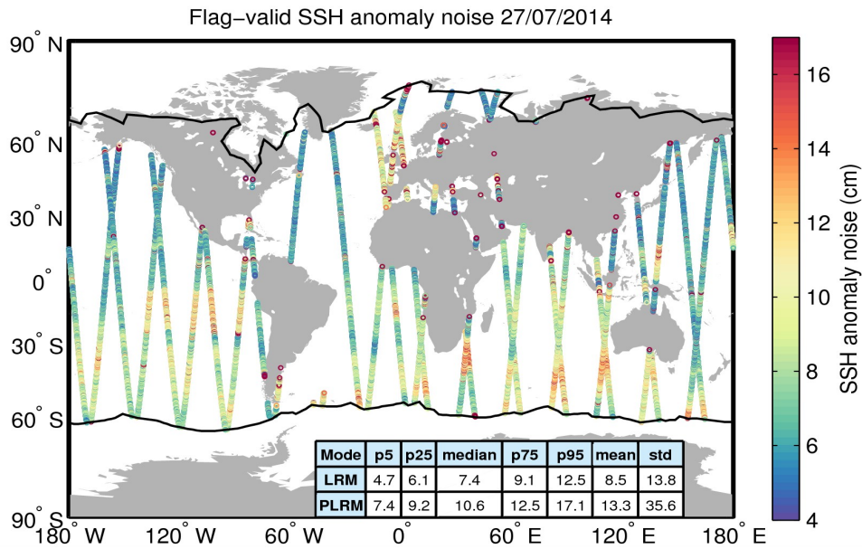
Figure 8. Geographical distribution of flag-valid 20-Hz SSH anomaly measurement noise over oceans and lakes for 27/07/2014. The statistical values shown in the table refer to the SSH anomaly noise and are calculated separately for LRM and PLRM regions. Measurements taken over polar polygons have been excluded from the computation of the statistical values. The black lines mark the outer limit of the Arctic and Antarctic polar polygons.
