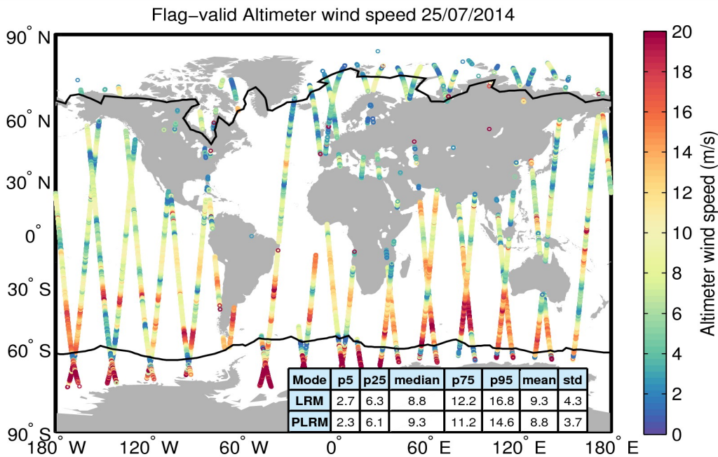
Figure 31. Geographical distribution of flag-valid wind data over oceans and lakes for 25/07/2014. The statistical values shown in the table refer to the wind in m/s and are calculated separately for LRM and PLRM regions. Measurements taken over polar polygons have been excluded from the computation of the statistical values. The black lines mark the outer limit of the Arctic and Antarctic polar polygons.
