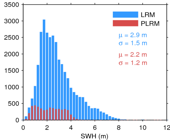
Figure 17. Histogram of flag-valid SWH over oceans and lakes for LRM (blue) and PLRM (red) for 25/07/2014. The mean ( \mu ) and standard deviation ( \sigma ) are also shown. Note that values larger than 12 m are excluded from the histogram for the sake of readability but not from the computation of \mu and \sigma .
