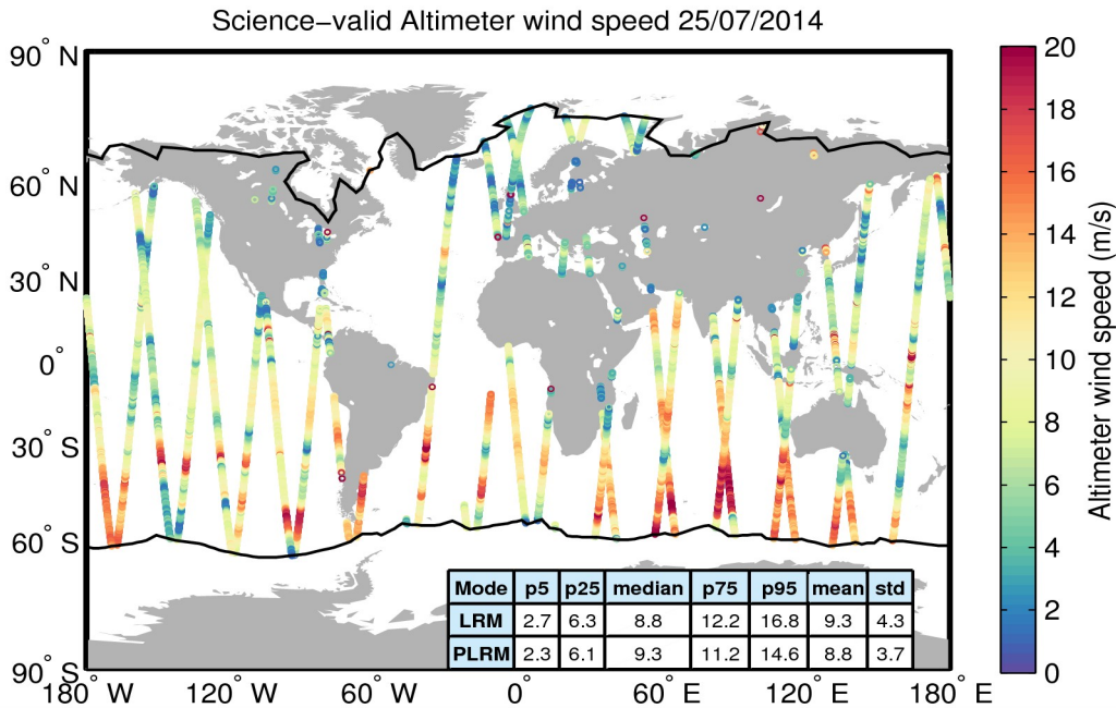
Figure 34. Geographical distribution of science-valid wind data over oceans and lakes for 25/07/2014. The statistical values shown in the table refer to the wind in m/s and are calculated separately for LRM and PLRM regions. The black lines mark the outer limit of the Arctic and Antarctic polar polygons. Gray circles denote records that have been rejected based on the editing criteria described in Table 5.
