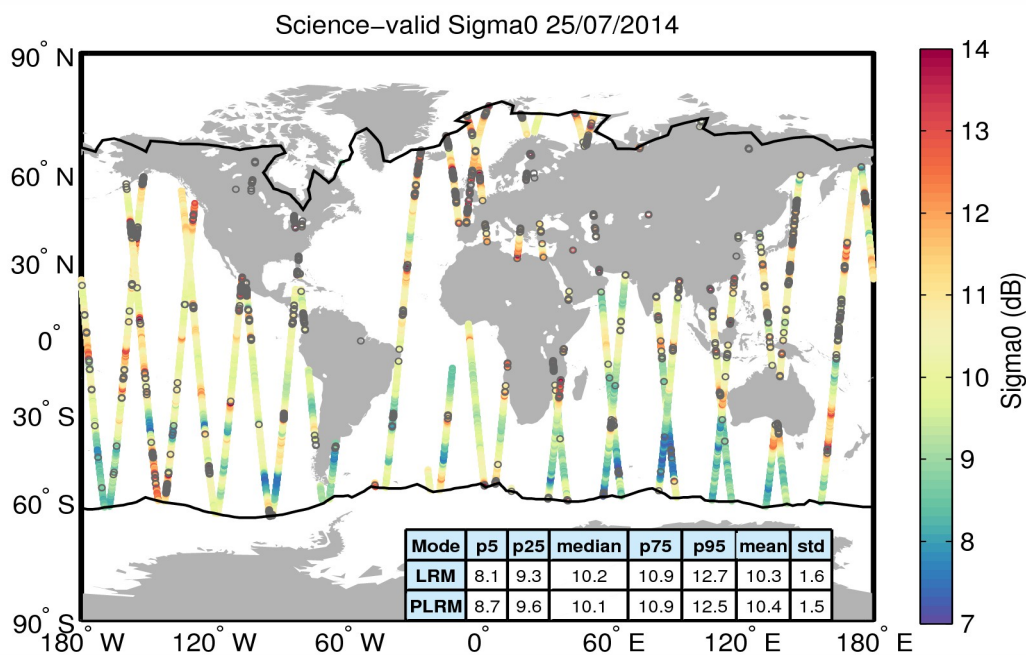
Figure 27. Geographical distribution of science-valid sigma0 data over oceans and lakes for 25/07/2014. The statistical values shown in the table refer to the sigma0 in dB and are calculated separately for LRM and PLRM regions. The black lines mark the outer limit of the Arctic and Antarctic polar polygons. Gray circles denote records that have been rejected based on the editing criteria described in Table 4.
