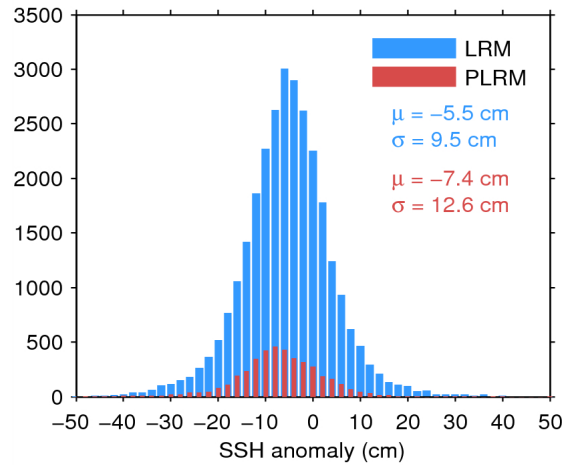
Figure 11. Histogram of science-valid SSH anomaly over oceans and lakes for LRM (blue) and PLRM (red) for 25/07/2014. The mean ( \mu ) and standard deviation ( \sigma ) are also shown. Note that values outside [-50 50] cm are excluded from the histogram for the sake of readability but not from the computation of \mu and \sigma .
