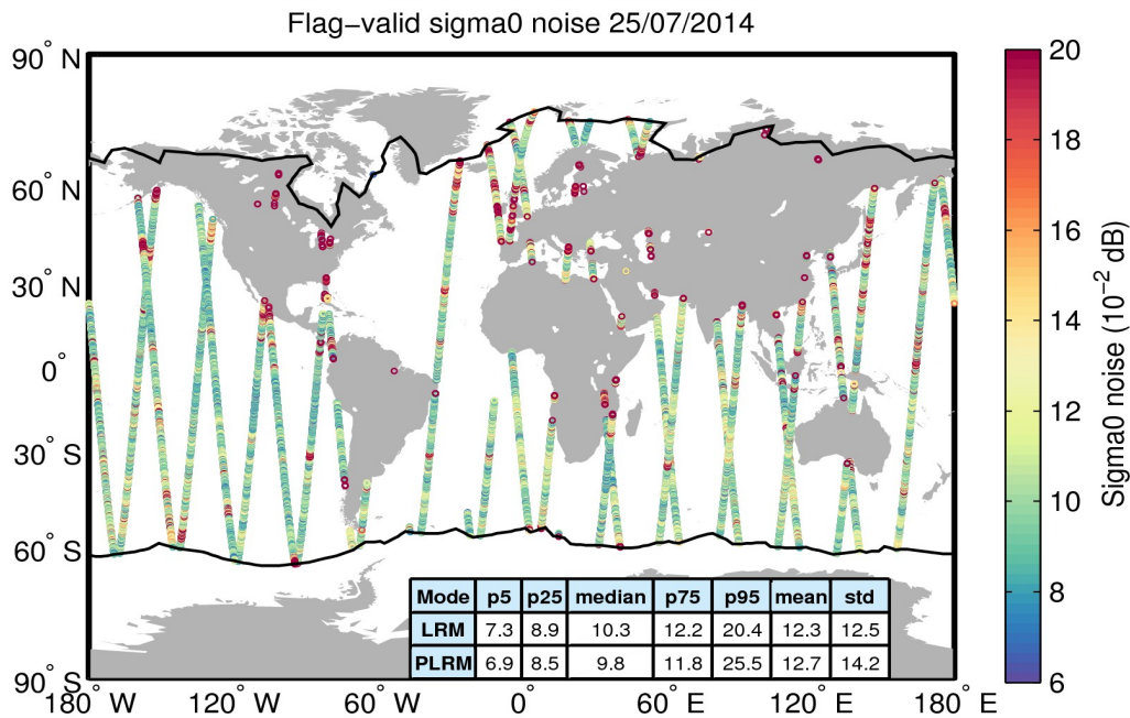
Figure 26. Geographical distribution of flag-valid 20-Hz sigma0 measurement noise over oceans and lakes for 25/07/2014. The statistical values shown in the table refer to the sigma0 noise and are calculated separately for LRM and PLRM regions. Measurements taken over polar polygons have been excluded from the computation of the statistical values. The black lines mark the outer limit of the Arctic and Antarctic polar polygons.
