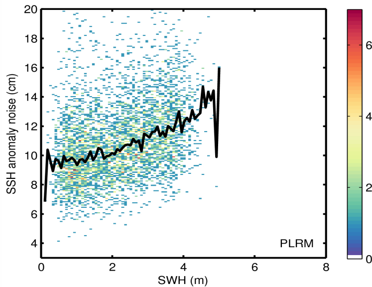
Figure 9. 2D histogram showing flag-valid SSH anomaly noise as a function of SWH for LRM (top) and PLRM (bottom) for 25/07/2014. The black line denotes the median SSH anomaly as a function of SWH.
