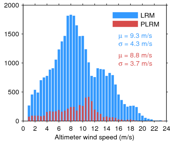
Figure 33. Histogram of flag-valid wind over oceans and lakes for LRM (blue) and PLRM (red) for 25/07/2014. The mean ( \mu ) and standard deviation ( \sigma ) are also shown. Note that values larger than 24 m/s are excluded from the histogram for the sake of readability but not from the computation of \mu and \sigma .
