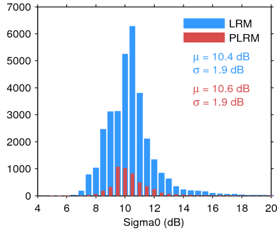
Figure 25. Histogram of flag-valid sigma0 over oceans and lakes for LRM (blue) and PLRM (red) for 25/07/2014. The mean ( \mu ) and standard deviation ( \sigma ) are also shown. Note that values outside [4 20] dB are excluded from the histogram for the sake of readability but not from the computation of \mu and \sigma .
