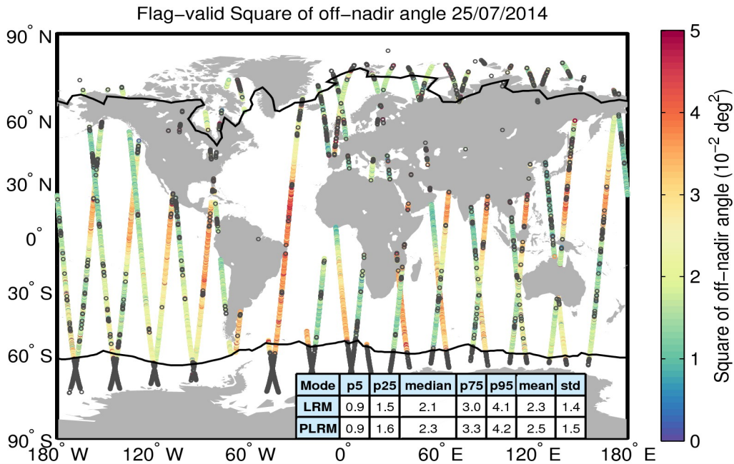
Figure 37. Geographical distribution of flag-valid mispointing data over oceans and lakes for 25/07/2014. The statistical values shown in the table refer to the mispointing in 10^{-2} \text{ deg}^2 and are calculated separately for LRM and PLRM regions. Measurements taken over polar polygons have been excluded from the computation of the statistical values. The black lines mark the outer limit of the Arctic and Antarctic polar polygons. Gray circles denote negative values.
