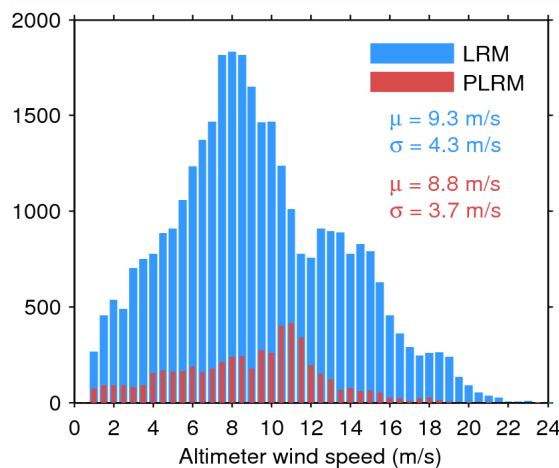
Figure 35. Histogram of science-valid wind over oceans and lakes for LRM (blue) and PLRM (red) for 25/07/2014. The mean ( \mu ) and standard deviation ( \sigma ) are also shown. Note that values larger than 24 m/s are excluded from the histogram for the sake of readability but not from the computation of \mu and \sigma .
