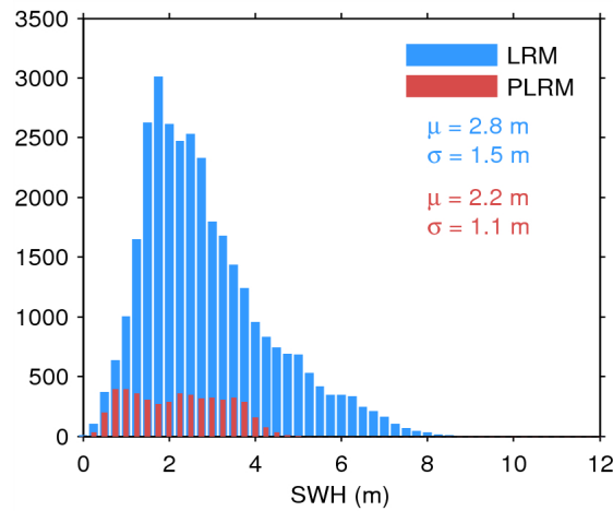
Figure 20. Histogram of science-valid SWH over oceans and lakes for LRM (blue) and PLRM (red) for 25/07/2014. The mean ( \mu ) and standard deviation ( \sigma ) are also shown. Note that values larger than 12 m are excluded from the histogram for the sake of readability but not from the computation of \mu and \sigma .
