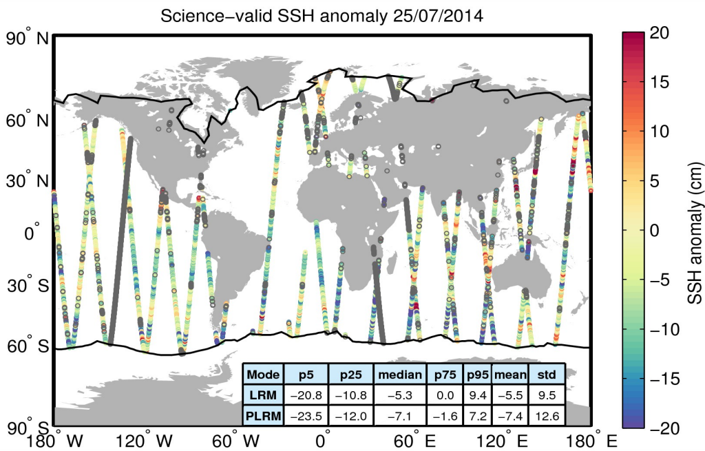
Figure 10. Geographical distribution of science-valid SSH anomaly data over oceans and lakes for 25/07/2014. The statistical values shown in the table refer to the SSH anomaly in cm and are calculated separately for LRM and PLRM regions. The black lines mark the outer limit of the Arctic and Antarctic polar polygons. Gray circles denote records that have been rejected based on the editing criteria described in Table 2.
