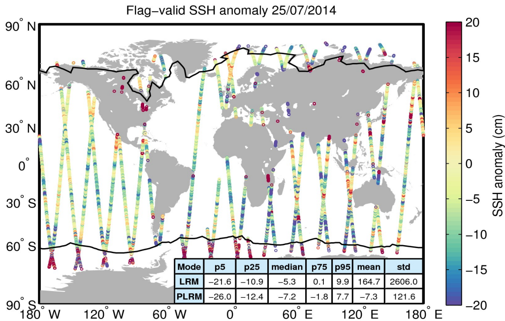
Figure 5. Geographical distribution of flag-valid 1-Hz SSH anomaly data over oceans and lakes for 25/07/2014. The statistical values shown in the table refer to the SSH anomaly in cm and are calculated separately for LRM and PLRM regions. Measurements taken over polar polygons have been excluded from the computation of the statistical values. The black lines mark the outer limit of the Arctic and Antarctic polar polygons.
