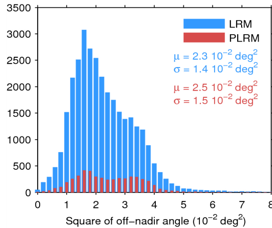
Figure 39. Histogram of flag-valid mispointing over oceans and lakes for LRM (blue) and PLRM (red) for 25/07/2014. Only positive values have been considered. The mean ( \mu ) and standard deviation ( \sigma ) are also shown. Note that values 8 \cdot 10^{-2} \text{ deg}^2 are excluded from the histogram for the sake of readability but not from the computation of \mu and \sigma .
