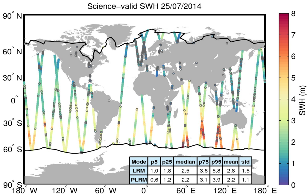
Figure 19. Geographical distribution of science-valid SWH data over oceans and lakes for 25/07/2014. The statistical values shown in the table refer to the SWH in m and are calculated separately for LRM and PLRM regions. The black lines mark the outer limit of the Arctic and Antarctic polar polygons. Gray circles denote records that have been rejected based on the editing criteria described in Table 3.
