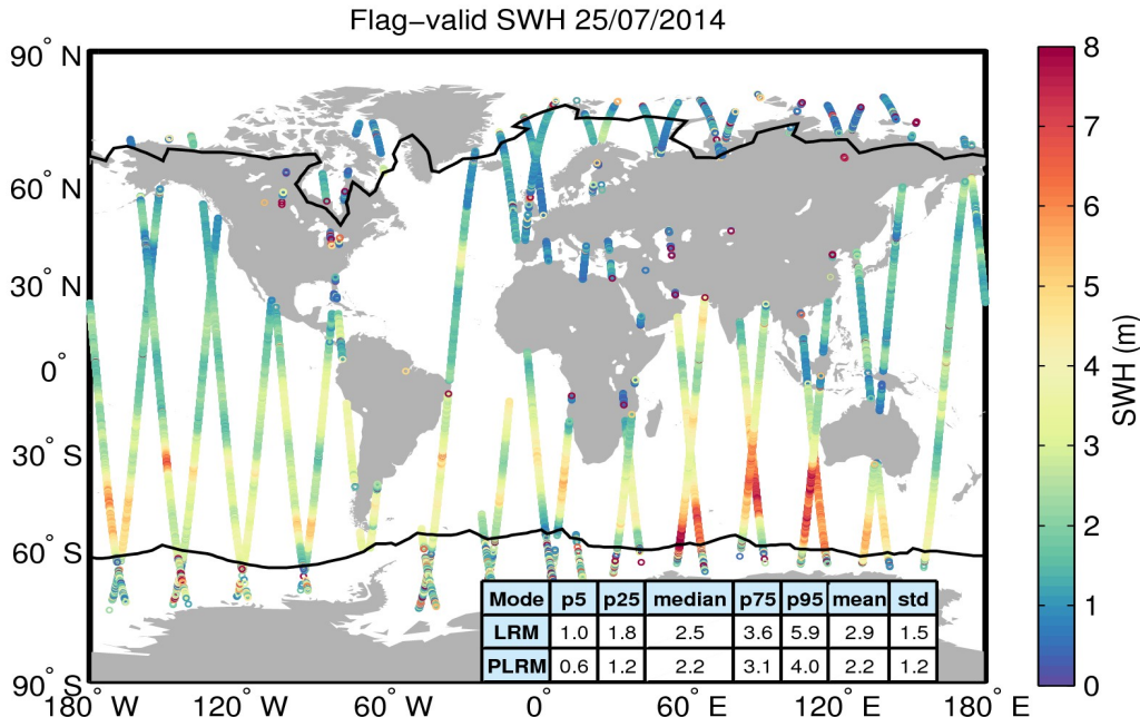
Figure 15. Geographical distribution of flag-valid SWH data over oceans and lakes for 25/07/2014. The statistical values shown in the table refer to the SWH in m and are calculated separately for LRM and PLRM regions. Measurements taken over polar polygons have been excluded from the computation of the statistical values. The black lines mark the outer limit of the Arctic and Antarctic polar polygons.
