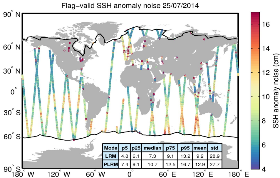
Figure 8. Geographical distribution of flag-valid 20-Hz SSH anomaly measurement noise over oceans and lakes for 25/07/2014. The statistical values shown in the table refer to the SSH anomaly noise and are calculated separately for LRM and PLRM regions. Measurements taken over polar polygons have been excluded from the computation of the statistical values. The black lines mark the outer limit of the Arctic and Antarctic polar polygons.
