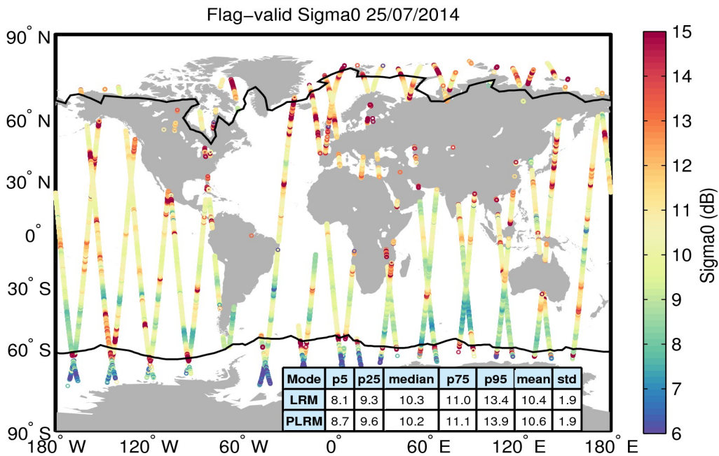
Figure 23. Geographical distribution of flag-valid sigma0 data over oceans and lakes for 25/07/2014. The statistical values shown in the table refer to the sigma0 in dB and are calculated separately for LRM and PLRM regions. Measurements taken over polar polygons have been excluded from the computation of the statistical values. The black lines mark the outer limit of the Arctic and Antarctic polar polygons.
