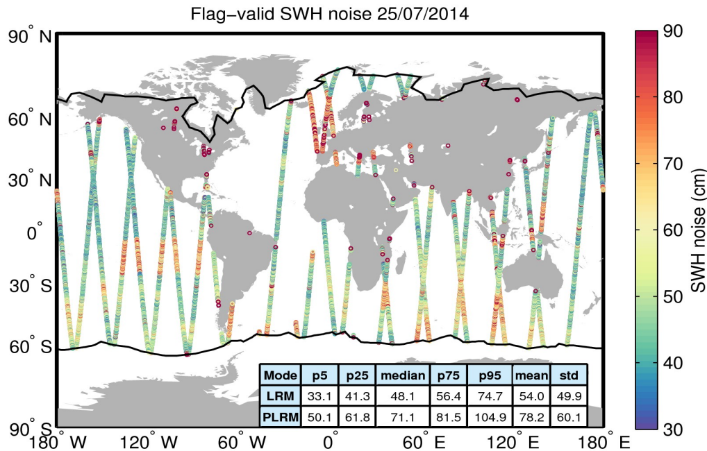
Figure 18. Geographical distribution of flag-valid 20-Hz SWH measurement noise over oceans and lakes for 25/07/2014. The statistical values shown in the table refer to the SWH noise and are calculated separately for LRM and PLRM regions. Measurements taken over polar polygons have been excluded from the computation of the statistical values. The black lines mark the outer limit of the Arctic and Antarctic polar polygons.
