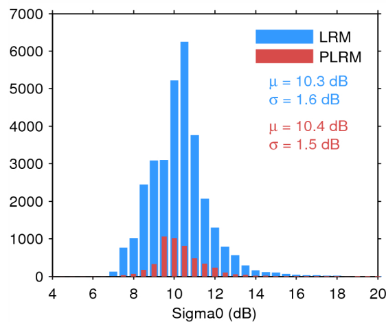
Figure 28. Histogram of science-valid sigma0 over oceans and lakes for LRM (blue) and PLRM (red) for 25/07/2014. The mean ( \mu ) and standard deviation ( \sigma ) are also shown. Note that values outside [4 20] dB are excluded from the histogram for the sake of readability but not from the computation of \mu and \sigma .
