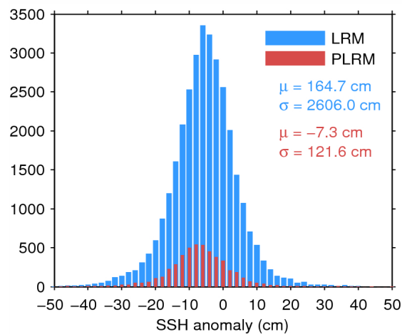
Figure 7. Histogram of flag-valid SSH anomaly over oceans and lakes for LRM (blue) and PLRM (red) for 25/07/2014. The mean ( \mu ) and standard deviation ( \sigma ) are also shown. Note that values outside [-50 \ 50] cm are excluded from the histogram for the sake of readability but not from the computation of \mu and \sigma .
