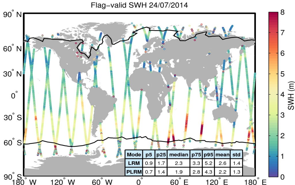
Figure 15. Geographical distribution of flag-valid SWH data over oceans and lakes for 24/07/2014. The statistical values shown in the table refer to the SWH in m and are calculated separately for LRM and PLRM regions. Measurements taken over polar polygons have been excluded from the computation of the statistical values. The black lines mark the outer limit of the Arctic and Antarctic polar polygons.
