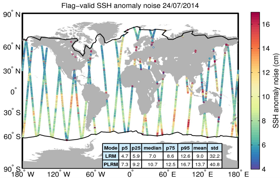
Figure 8. Geographical distribution of flag-valid 20-Hz SSH anomaly measurement noise over oceans and lakes for 24/07/2014. The statistical values shown in the table refer to the SSH anomaly noise and are calculated separately for LRM and PLRM regions. Measurements taken over polar polygons have been excluded from the computation of the statistical values. The black lines mark the outer limit of the Arctic and Antarctic polar polygons.
