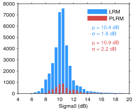
Figure 25. Histogram of flag-valid sigma0 over oceans and lakes for LRM (blue) and PLRM (red) for 24/07/2014. The mean ( \mu ) and standard deviation ( \sigma ) are also shown. Note that values outside [4 20] dB are excluded from the histogram for the sake of readability but not from the computation of \mu and \sigma .
