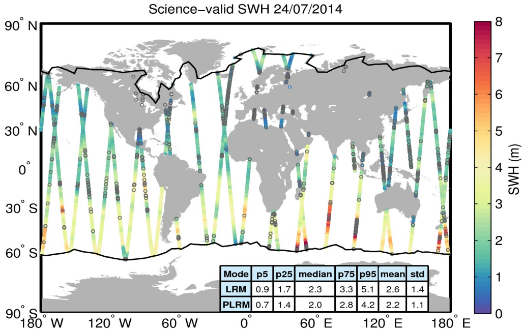
Figure 19. Geographical distribution of science-valid SWH data over oceans and lakes for 24/07/2014. The statistical values shown in the table refer to the SWH in m and are calculated separately for LRM and PLRM regions. The black lines mark the outer limit of the Arctic and Antarctic polar polygons. Gray circles denote records that have been rejected based on the editing criteria described in Table 3.
