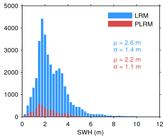
Figure 20. Histogram of science-valid SWH over oceans and lakes for LRM (blue) and PLRM (red) for 24/07/2014. The mean ( \mu ) and standard deviation ( \sigma ) are also shown. Note that values larger than 12 m are excluded from the histogram for the sake of readability but not from the computation of \mu and \sigma .
