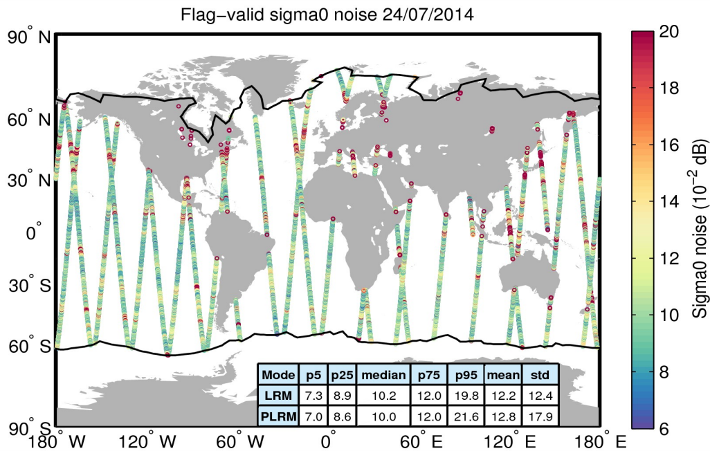
Figure 26. Geographical distribution of flag-valid 20-Hz sigma0 measurement noise over oceans and lakes for 24/07/2014. The statistical values shown in the table refer to the sigma0 noise and are calculated separately for LRM and PLRM regions. Measurements taken over polar polygons have been excluded from the computation of the statistical values. The black lines mark the outer limit of the Arctic and Antarctic polar polygons.
