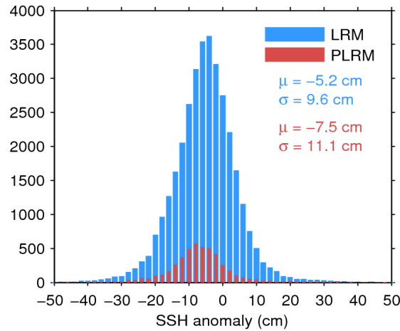
Figure 11. Histogram of science-valid SSH anomaly over oceans and lakes for LRM (blue) and PLRM (red) for 24/07/2014. The mean ( \mu ) and standard deviation ( \sigma ) are also shown. Note that values outside [-50\ 50] cm are excluded from the histogram for the sake of readability but not from the computation of \mu and \sigma .
