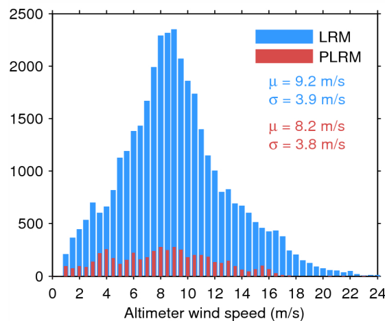
Figure 35. Histogram of science-valid wind over oceans and lakes for LRM (blue) and PLRM (red) for 24/07/2014. The mean ( \mu ) and standard deviation ( \sigma ) are also shown. Note that values larger than 24 m/s are excluded from the histogram for the sake of readability but not from the computation of \mu and \sigma .
