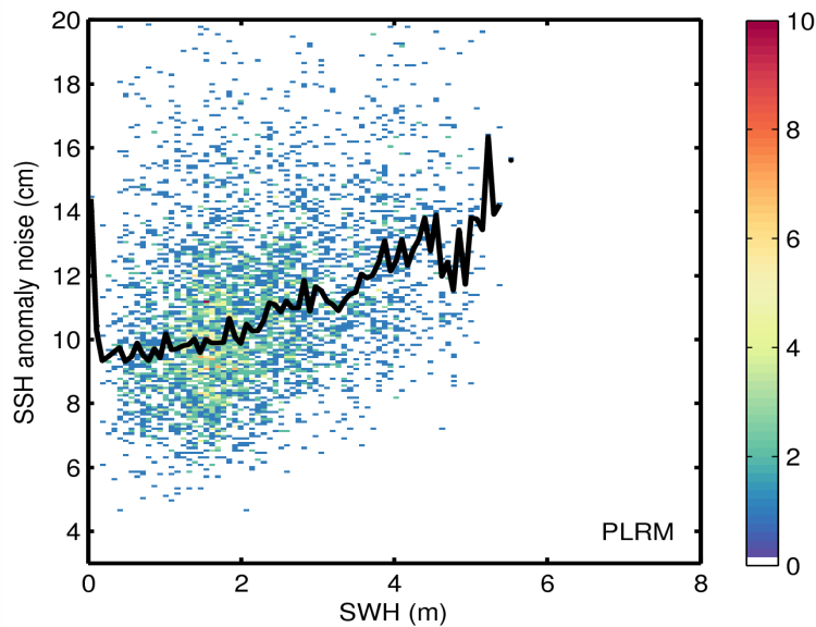
Figure 9. 2D histogram showing flag-valid SSH anomaly noise as a function of SWH for LRM (top) and PLRM (bottom) for 24/07/2014. The black line denotes the median SSH anomaly as a function of SWH.
