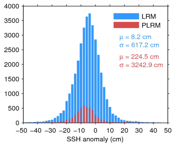
Figure 7. Histogram of flag-valid SSH anomaly over oceans and lakes for LRM (blue) and PLRM (red) for 24/07/2014. The mean ( \mu ) and standard deviation ( \sigma ) are also shown. Note that values outside [-50 \ 50] cm are excluded from the histogram for the sake of readability but not from the computation of \mu and \sigma .
