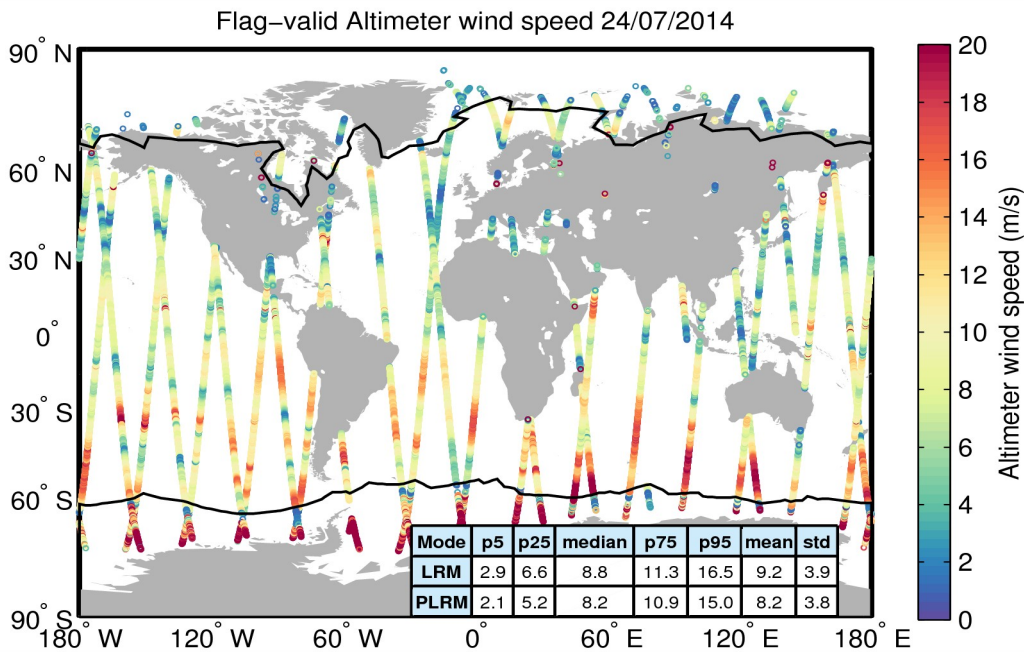
Figure 31. Geographical distribution of flag-valid wind data over oceans and lakes for 24/07/2014. The statistical values shown in the table refer to the wind in m/s and are calculated separately for LRM and PLRM regions. Measurements taken over polar polygons have been excluded from the computation of the statistical values. The black lines mark the outer limit of the Arctic and Antarctic polar polygons.
