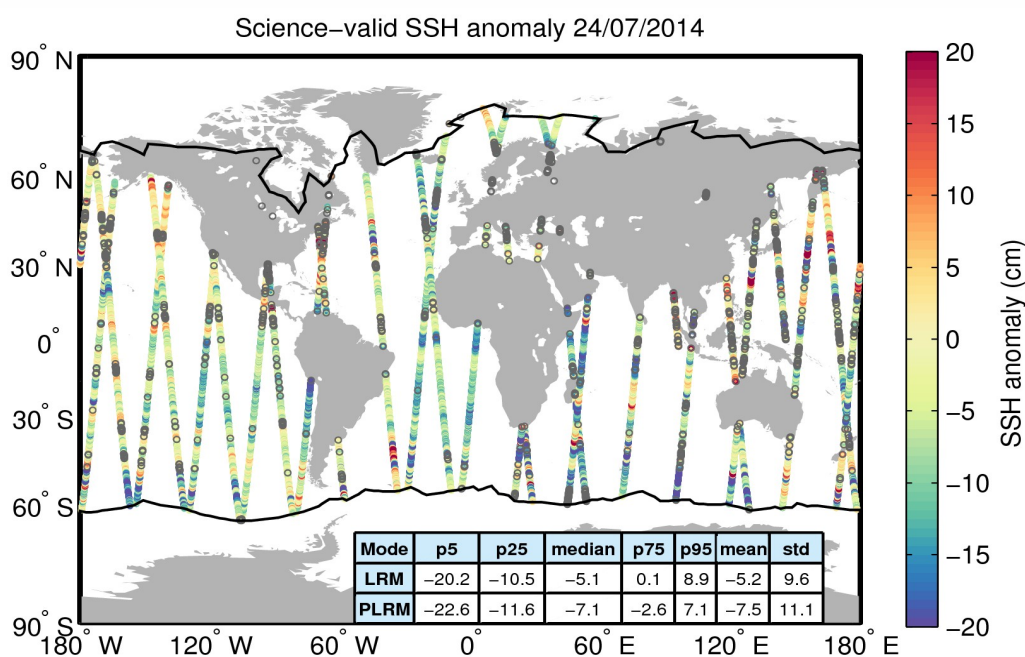
Figure 10. Geographical distribution of science-valid SSH anomaly data over oceans and lakes for 24/07/2014. The statistical values shown in the table refer to the SSH anomaly in cm and are calculated separately for LRM and PLRM regions. The black lines mark the outer limit of the Arctic and Antarctic polar polygons. Gray circles denote records that have been rejected based on the editing criteria described in Table 2.
