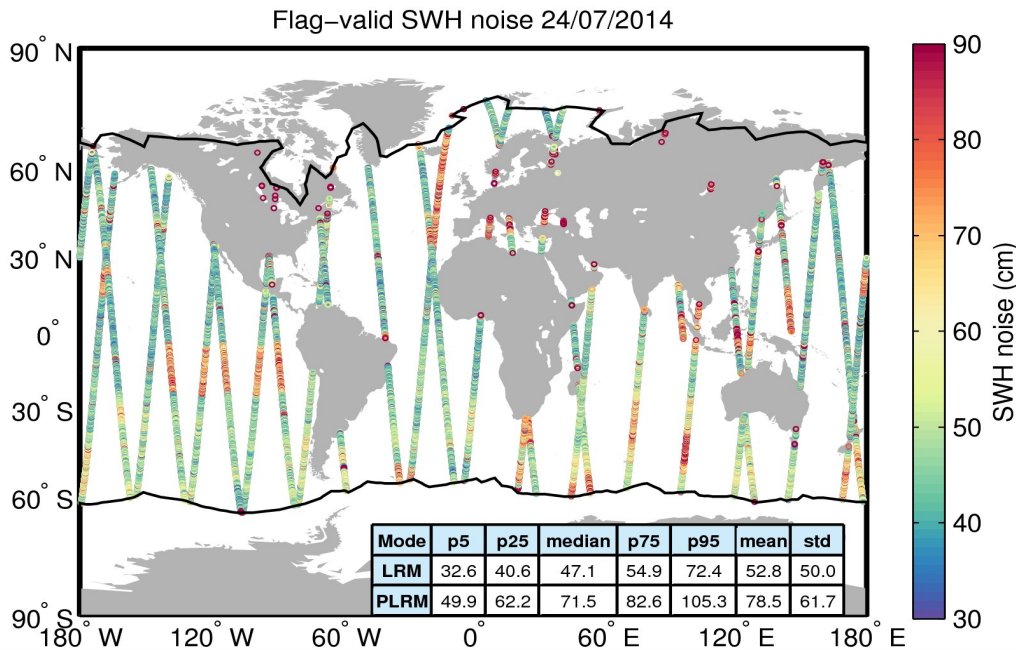
Figure 18. Geographical distribution of flag-valid 20-Hz SWH measurement noise over oceans and lakes for 24/07/2014. The statistical values shown in the table refer to the SWH noise and are calculated separately for LRM and PLRM regions. Measurements taken over polar polygons have been excluded from the computation of the statistical values. The black lines mark the outer limit of the Arctic and Antarctic polar polygons.
