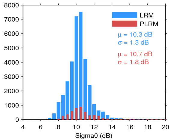
Figure 28. Histogram of science-valid sigma0 over oceans and lakes for LRM (blue) and PLRM (red) for 24/07/2014. The mean ( \mu ) and standard deviation ( \sigma ) are also shown. Note that values outside [4 20] dB are excluded from the histogram for the sake of readability but not from the computation of \mu and \sigma .
