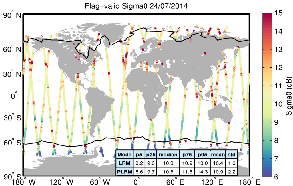
Figure 23. Geographical distribution of flag-valid sigma0 data over oceans and lakes for 24/07/2014. The statistical values shown in the table refer to the sigma0 in dB and are calculated separately for LRM and PLRM regions. Measurements taken over polar polygons have been excluded from the computation of the statistical values. The black lines mark the outer limit of the Arctic and Antarctic polar polygons.
