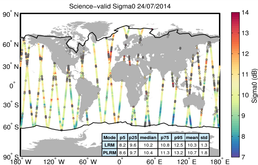
Figure 27. Geographical distribution of science-valid sigma0 data over oceans and lakes for 24/07/2014. The statistical values shown in the table refer to the sigma0 in dB and are calculated separately for LRM and PLRM regions. The black lines mark the outer limit of the Arctic and Antarctic polar polygons. Gray circles denote records that have been rejected based on the editing criteria described in Table 4.
