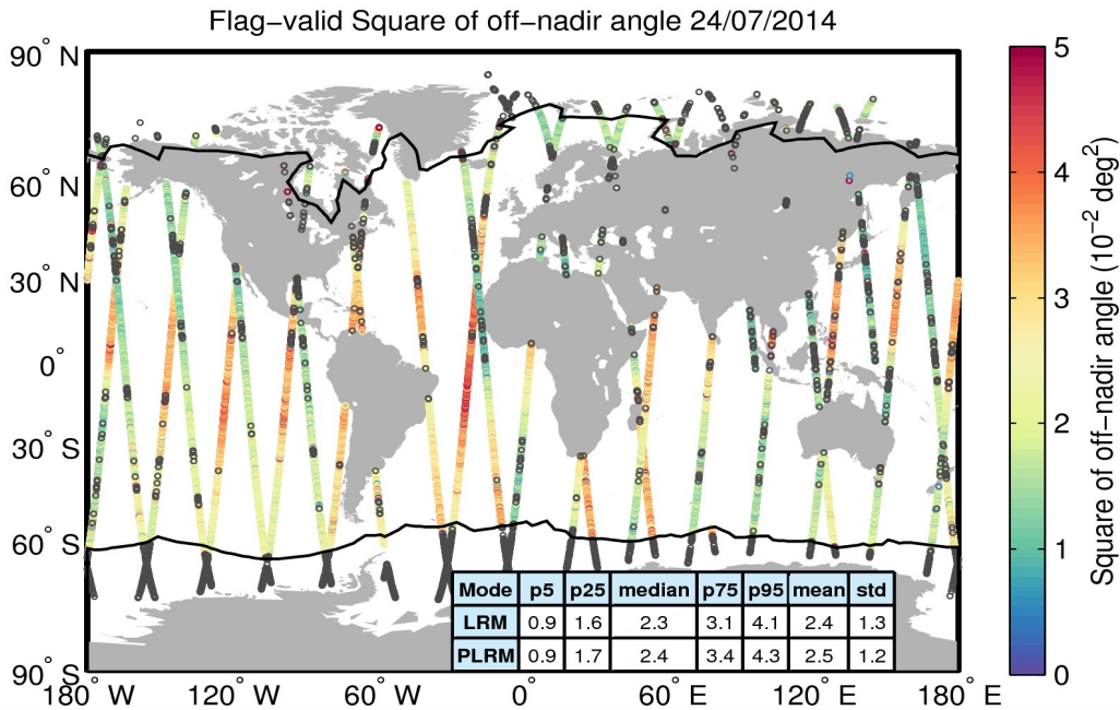
Figure 37. Geographical distribution of flag-valid mispointing data over oceans and lakes for 24/07/2014. The statistical values shown in the table refer to the mispointing in 10^{-2} deg 2 and are calculated separately for LRM and PLRM regions. Measurements taken over polar polygons have been excluded from the computation of the statistical values. The black lines mark the outer limit of the Arctic and Antarctic polar polygons. Gray circles denote negative values.
