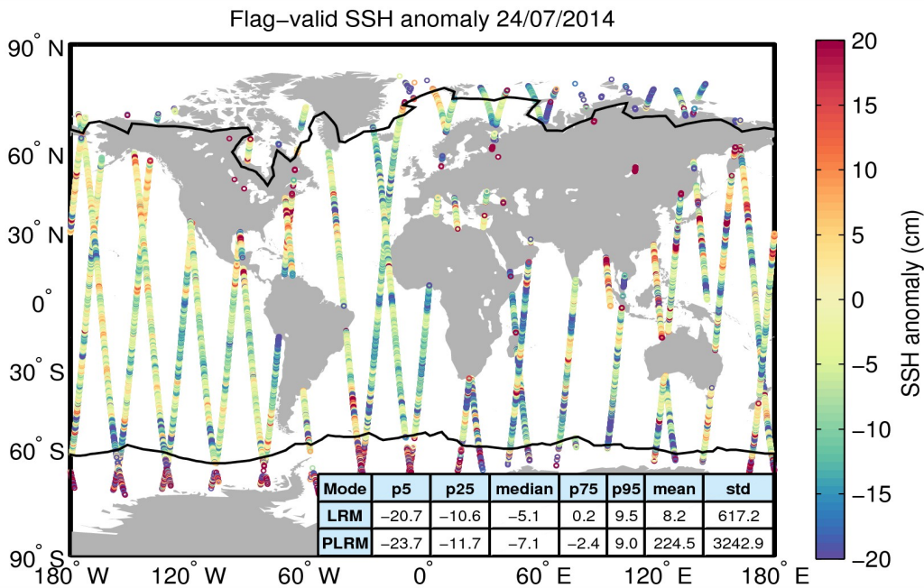
Figure 5. Geographical distribution of flag-valid 1-Hz SSH anomaly data over oceans and lakes for 24/07/2014. The statistical values shown in the table refer to the SSH anomaly in cm and are calculated separately for LRM and PLRM regions. Measurements taken over polar polygons have been excluded from the computation of the statistical values. The black lines mark the outer limit of the Arctic and Antarctic polar polygons.
