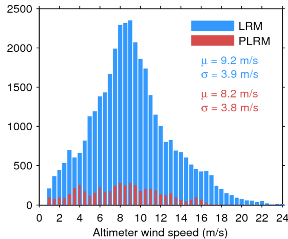
Figure 33. Histogram of flag-valid wind over oceans and lakes for LRM (blue) and PLRM (red) for 24/07/2014. The mean ( \mu ) and standard deviation ( \sigma ) are also shown. Note that values larger than 24 m/s are excluded from the histogram for the sake of readability but not from the computation of \mu and \sigma .
