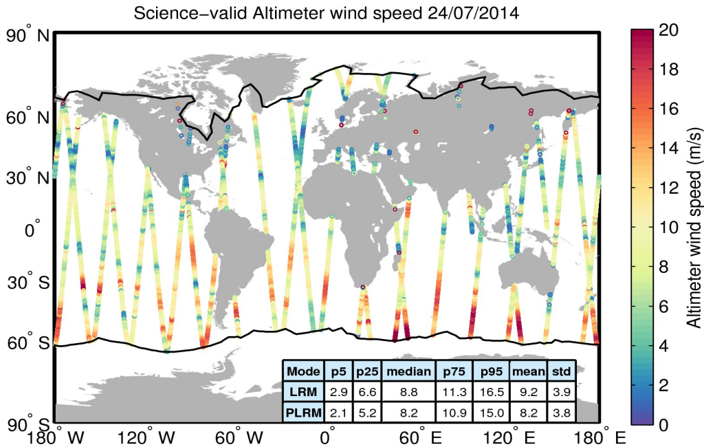
Figure 34. Geographical distribution of science-valid wind data over oceans and lakes for 24/07/2014. The statistical values shown in the table refer to the wind in m/s and are calculated separately for LRM and PLRM regions. The black lines mark the outer limit of the Arctic and Antarctic polar polygons. Gray circles denote records that have been rejected based on the editing criteria described in Table 5.
