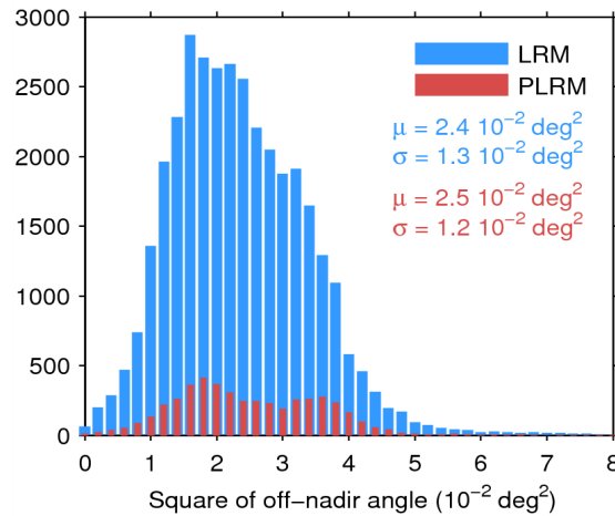
Figure 39. Histogram of flag-valid mispointing over oceans and lakes for LRM (blue) and PLRM (red) for 24/07/2014. Only positive values have been considered. The mean ( \mu ) and standard deviation ( \sigma ) are also shown. Note that values 8 \cdot 10^{-2} \text{ deg}^2 are excluded from the histogram for the sake of readability but not from the computation of \mu and \sigma .
