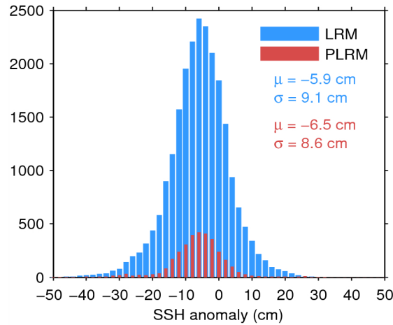
Figure 11. Histogram of science-valid SSH anomaly over oceans and lakes for LRM (blue) and PLRM (red) for 23/07/2014. The mean ( \mu ) and standard deviation ( \sigma ) are also shown. Note that values outside [-50\ 50] cm are excluded from the histogram for the sake of readability but not from the computation of \mu and \sigma .
