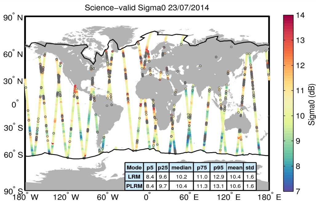
Figure 27. Geographical distribution of science-valid sigma0 data over oceans and lakes for 23/07/2014. The statistical values shown in the table refer to the sigma0 in dB and are calculated separately for LRM and PLRM regions. The black lines mark the outer limit of the Arctic and Antarctic polar polygons. Gray circles denote records that have been rejected based on the editing criteria described in Table 4.
