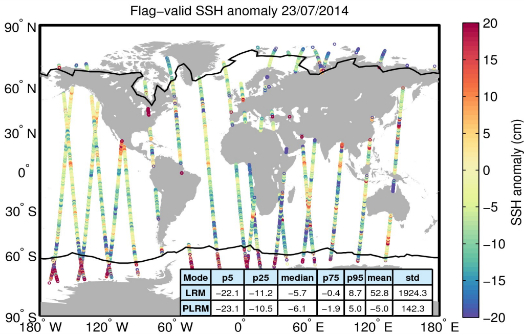
Figure 5. Geographical distribution of flag-valid 1-Hz SSH anomaly data over oceans and lakes for 23/07/2014. The statistical values shown in the table refer to the SSH anomaly in cm and are calculated separately for LRM and PLRM regions. Measurements taken over polar polygons have been excluded from the computation of the statistical values. The black lines mark the outer limit of the Arctic and Antarctic polar polygons.
