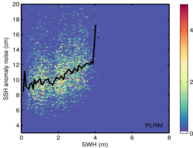
Figure 9. 2D histogram showing flag-valid SSH anomaly noise as a function of SWH for LRM (top) and PLRM (bottom) for 23/07/2014. The black line denotes the median SSH anomaly as a function of SWH.
