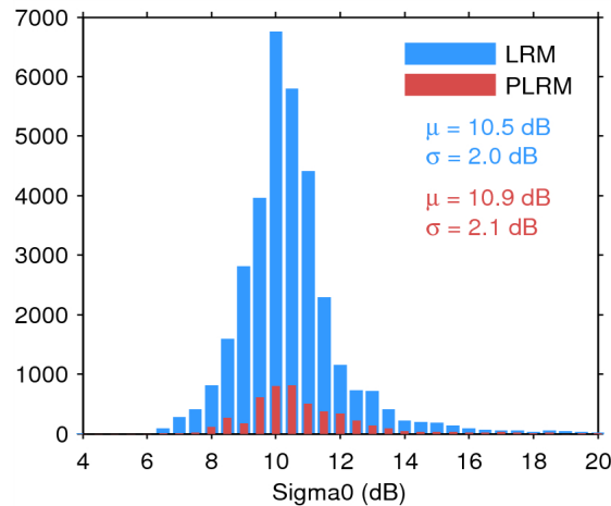
Figure 25. Histogram of flag-valid sigma0 over oceans and lakes for LRM (blue) and PLRM (red) for 23/07/2014. The mean ( \mu ) and standard deviation ( \sigma ) are also shown. Note that values outside [4 20] dB are excluded from the histogram for the sake of readability but not from the computation of \mu and \sigma .
