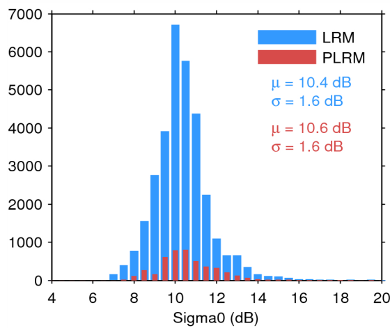
Figure 28. Histogram of science-valid sigma0 over oceans and lakes for LRM (blue) and PLRM (red) for 23/07/2014. The mean ( \mu ) and standard deviation ( \sigma ) are also shown. Note that values outside [4 20] dB are excluded from the histogram for the sake of readability but not from the computation of \mu and \sigma .
