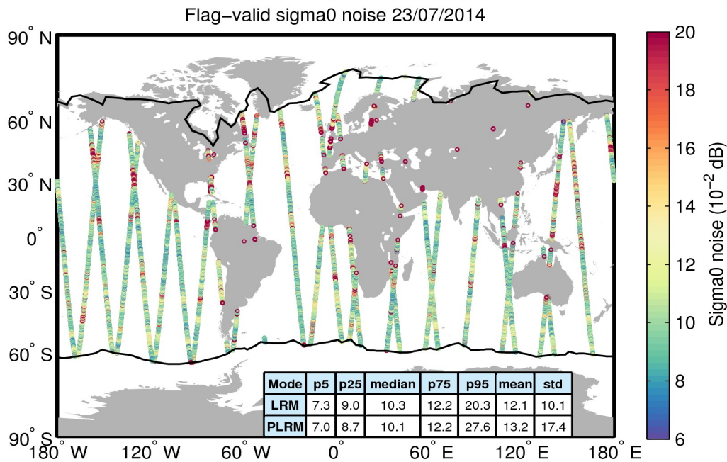
Figure 26. Geographical distribution of flag-valid 20-Hz sigma0 measurement noise over oceans and lakes for 23/07/2014. The statistical values shown in the table refer to the sigma0 noise and are calculated separately for LRM and PLRM regions. Measurements taken over polar polygons have been excluded from the computation of the statistical values. The black lines mark the outer limit of the Arctic and Antarctic polar polygons.
