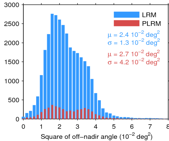
Figure 39. Histogram of flag-valid mispointing over oceans and lakes for LRM (blue) and PLRM (red) for 23/07/2014. Only positive values have been considered. The mean ( \mu ) and standard deviation ( \sigma ) are also shown. Note that values 8 \cdot 10^{-2} \text{ deg}^2 are excluded from the histogram for the sake of readability but not from the computation of \mu and \sigma .
