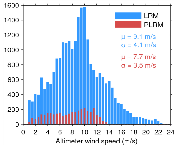
Figure 33. Histogram of flag-valid wind over oceans and lakes for LRM (blue) and PLRM (red) for 23/07/2014. The mean ( \mu ) and standard deviation ( \sigma ) are also shown. Note that values larger than 24 m/s are excluded from the histogram for the sake of readability but not from the computation of \mu and \sigma .
