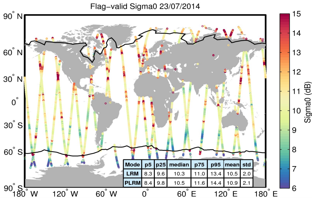
Figure 23. Geographical distribution of flag-valid sigma0 data over oceans and lakes for 23/07/2014. The statistical values shown in the table refer to the sigma0 in dB and are calculated separately for LRM and PLRM regions. Measurements taken over polar polygons have been excluded from the computation of the statistical values. The black lines mark the outer limit of the Arctic and Antarctic polar polygons.
