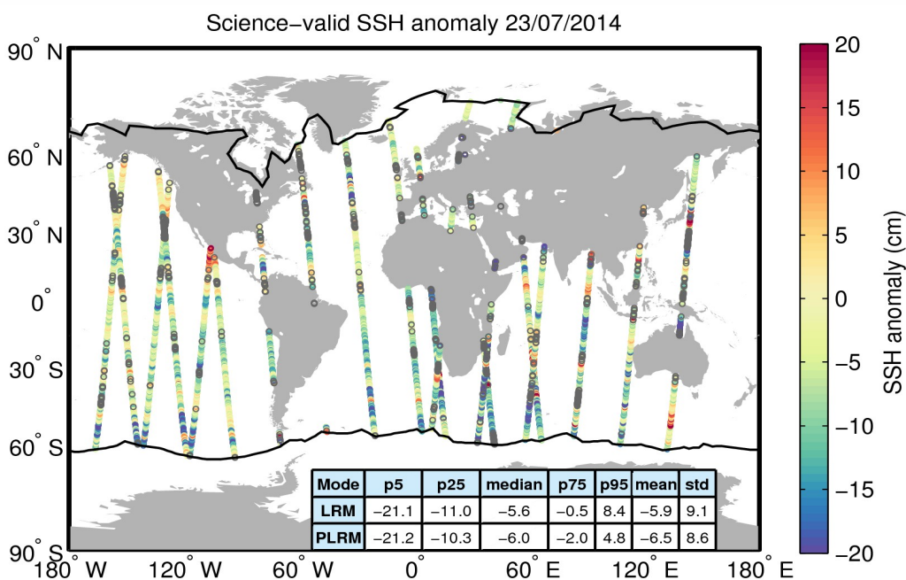
Figure 10. Geographical distribution of science-valid SSH anomaly data over oceans and lakes for 23/07/2014. The statistical values shown in the table refer to the SSH anomaly in cm and are calculated separately for LRM and PLRM regions. The black lines mark the outer limit of the Arctic and Antarctic polar polygons. Gray circles denote records that have been rejected based on the editing criteria described in Table 2.
