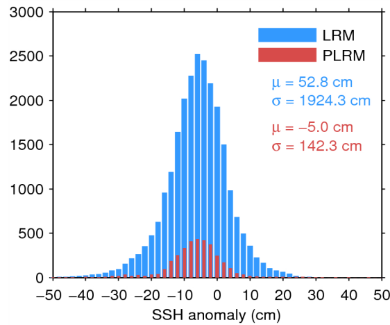
Figure 7. Histogram of flag-valid SSH anomaly over oceans and lakes for LRM (blue) and PLRM (red) for 23/07/2014. The mean ( \mu ) and standard deviation ( \sigma ) are also shown. Note that values outside [-50 50] cm are excluded from the histogram for the sake of readability but not from the computation of \mu and \sigma .
