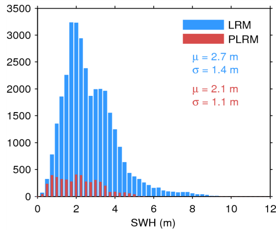
Figure 20. Histogram of science-valid SWH over oceans and lakes for LRM (blue) and PLRM (red) for 23/07/2014. The mean ( \mu ) and standard deviation ( \sigma ) are also shown. Note that values larger than 12 m are excluded from the histogram for the sake of readability but not from the computation of \mu and \sigma .
