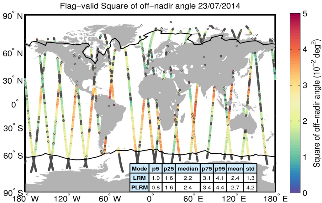
Figure 37. Geographical distribution of flag-valid mispointing data over oceans and lakes for 23/07/2014. The statistical values shown in the table refer to the mispointing in 10^{-2} deg 2 and are calculated separately for LRM and PLRM regions. Measurements taken over polar polygons have been excluded from the computation of the statistical values. The black lines mark the outer limit of the Arctic and Antarctic polar polygons. Gray circles denote negative values.
