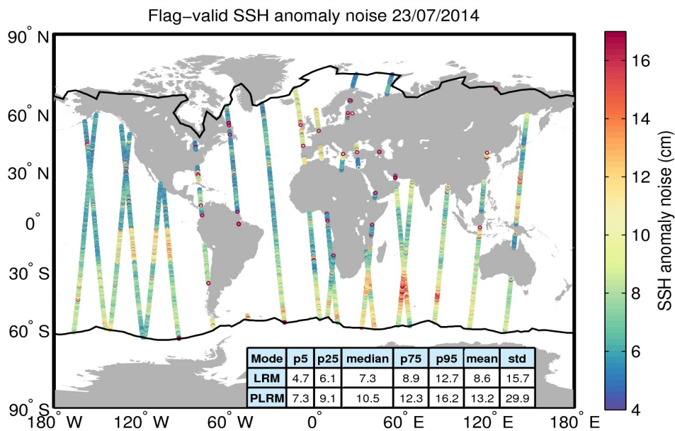
Figure 8. Geographical distribution of flag-valid 20-Hz SSH anomaly measurement noise over oceans and lakes for 23/07/2014. The statistical values shown in the table refer to the SSH anomaly noise and are calculated separately for LRM and PLRM regions. Measurements taken over polar polygons have been excluded from the computation of the statistical values. The black lines mark the outer limit of the Arctic and Antarctic polar polygons.
