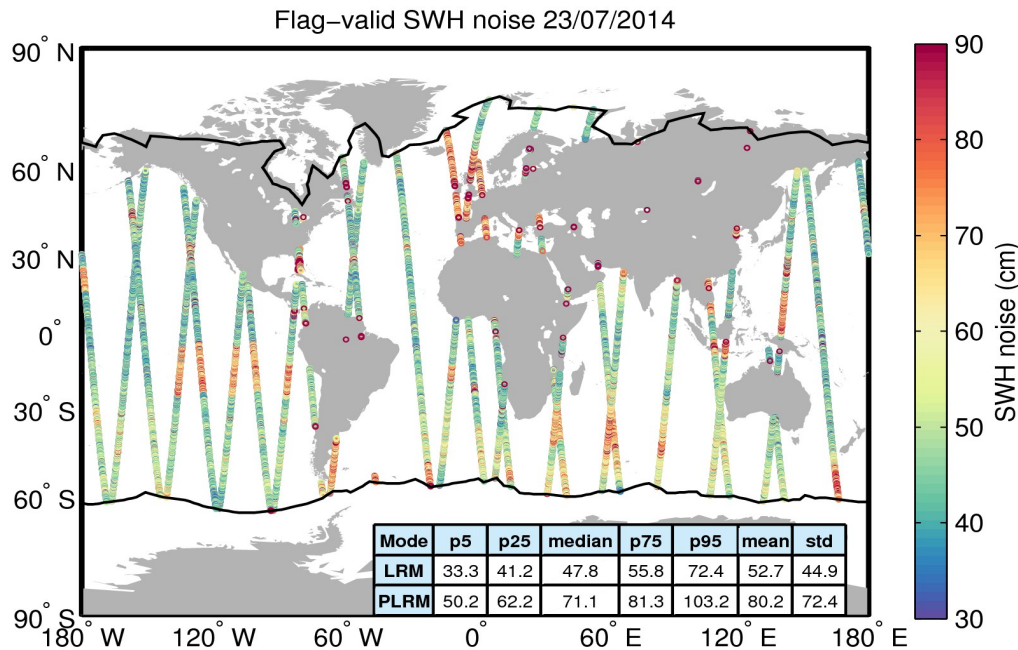
Figure 18. Geographical distribution of flag-valid 20-Hz SWH measurement noise over oceans and lakes for 23/07/2014. The statistical values shown in the table refer to the SWH noise and are calculated separately for LRM and PLRM regions. Measurements taken over polar polygons have been excluded from the computation of the statistical values. The black lines mark the outer limit of the Arctic and Antarctic polar polygons.
