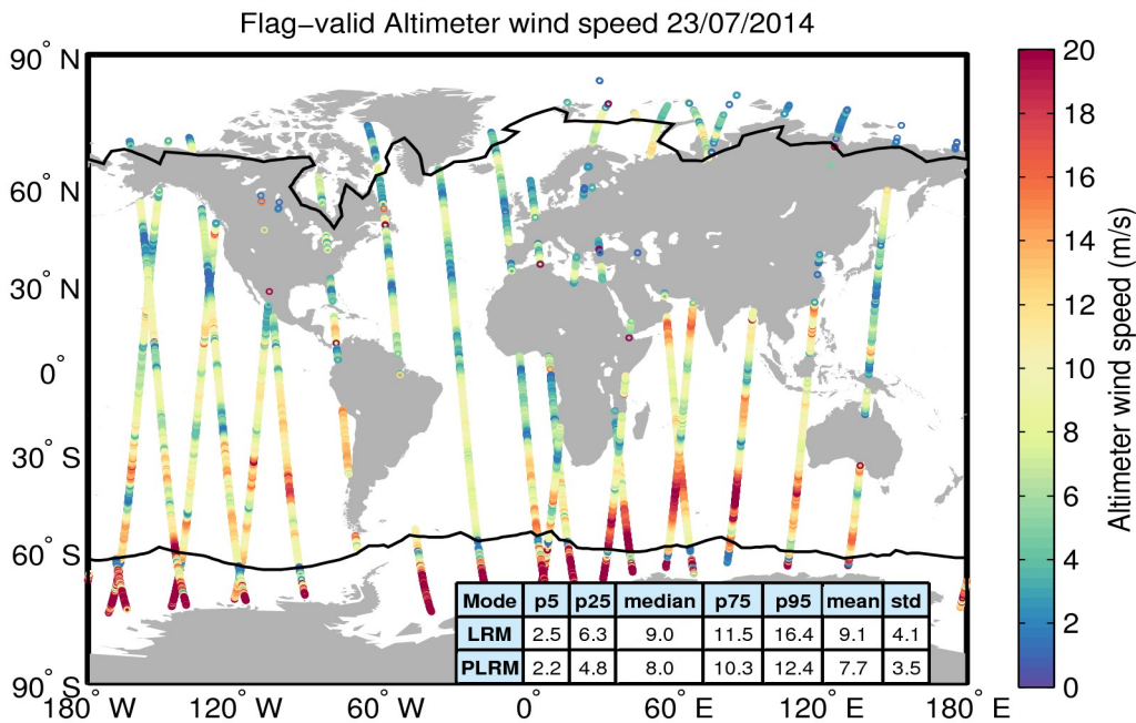
Figure 31. Geographical distribution of flag-valid wind data over oceans and lakes for 23/07/2014. The statistical values shown in the table refer to the wind in m/s and are calculated separately for LRM and PLRM regions. Measurements taken over polar polygons have been excluded from the computation of the statistical values. The black lines mark the outer limit of the Arctic and Antarctic polar polygons.
