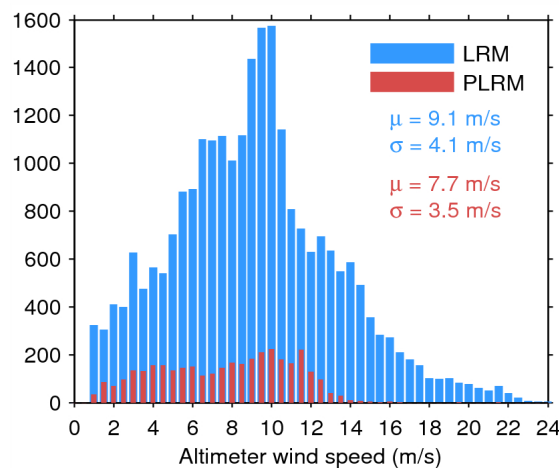
Figure 35. Histogram of science-valid wind over oceans and lakes for LRM (blue) and PLRM (red) for 23/07/2014. The mean ( \mu ) and standard deviation ( \sigma ) are also shown. Note that values larger than 24 m/s are excluded from the histogram for the sake of readability but not from the computation of \mu and \sigma .
