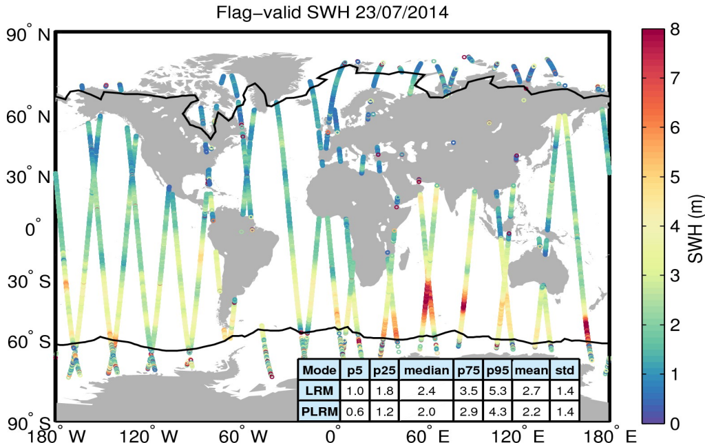
Figure 15. Geographical distribution of flag-valid SWH data over oceans and lakes for 23/07/2014. The statistical values shown in the table refer to the SWH in m and are calculated separately for LRM and PLRM regions. Measurements taken over polar polygons have been excluded from the computation of the statistical values. The black lines mark the outer limit of the Arctic and Antarctic polar polygons.
