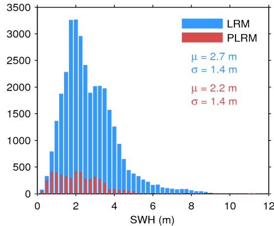
Figure 17. Histogram of flag-valid SWH over oceans and lakes for LRM (blue) and PLRM (red) for 23/07/2014. The mean ( \mu ) and standard deviation ( \sigma ) are also shown. Note that values larger than 12 m are excluded from the histogram for the sake of readability but not from the computation of \mu and \sigma .
