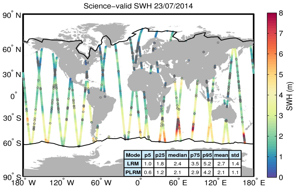
Figure 19. Geographical distribution of science-valid SWH data over oceans and lakes for 23/07/2014. The statistical values shown in the table refer to the SWH in m and are calculated separately for LRM and PLRM regions. The black lines mark the outer limit of the Arctic and Antarctic polar polygons. Gray circles denote records that have been rejected based on the editing criteria described in Table 3.
