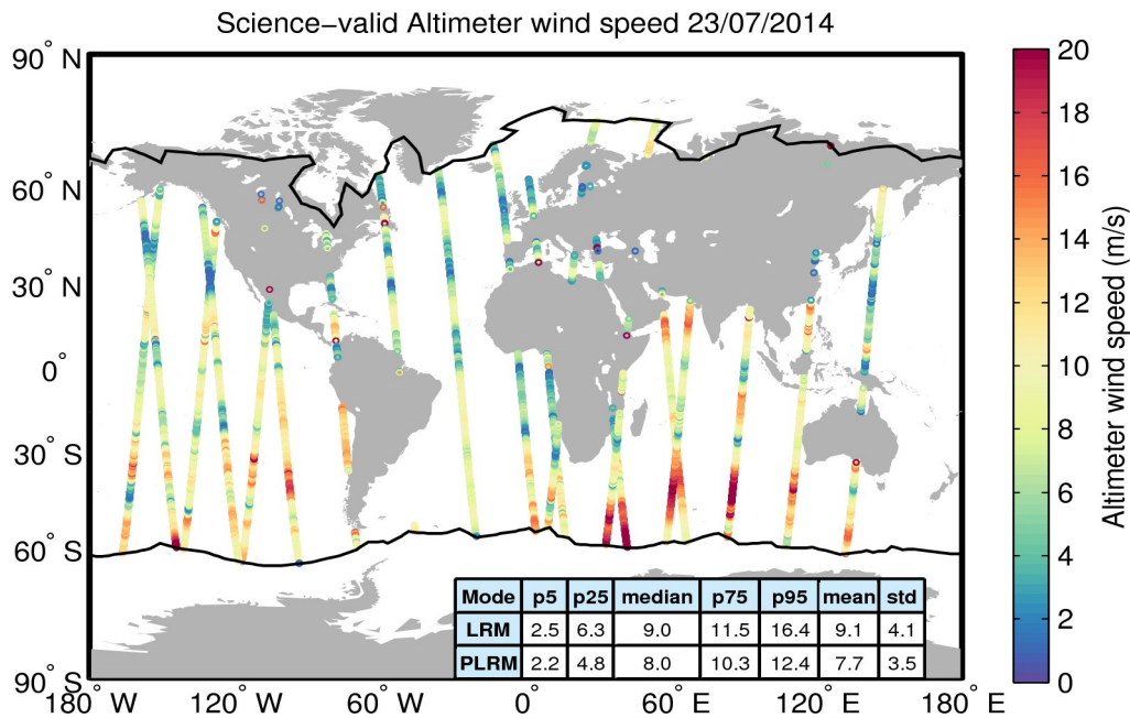
Figure 34. Geographical distribution of science-valid wind data over oceans and lakes for 23/07/2014. The statistical values shown in the table refer to the wind in m/s and are calculated separately for LRM and PLRM regions. The black lines mark the outer limit of the Arctic and Antarctic polar polygons. Gray circles denote records that have been rejected based on the editing criteria described in Table 5.
