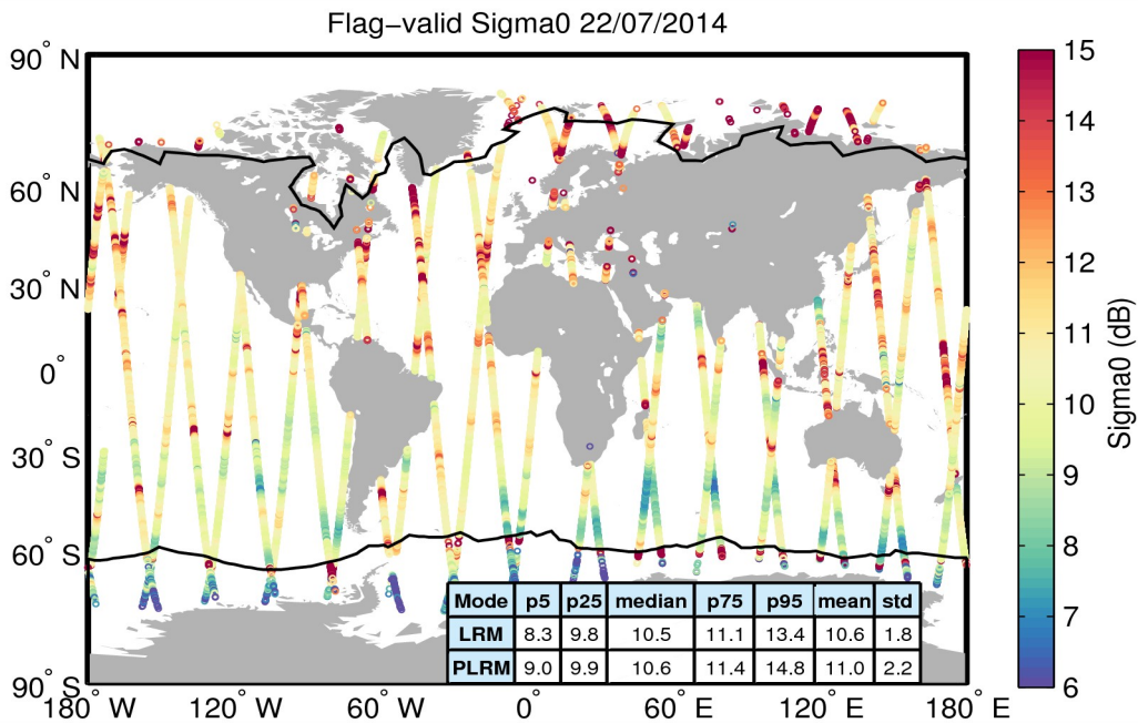
Figure 23. Geographical distribution of flag-valid sigma0 data over oceans and lakes for 22/07/2014. The statistical values shown in the table refer to the sigma0 in dB and are calculated separately for LRM and PLRM regions. Measurements taken over polar polygons have been excluded from the computation of the statistical values. The black lines mark the outer limit of the Arctic and Antarctic polar polygons.
