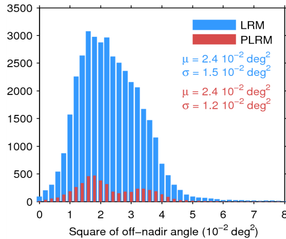
Figure 39. Histogram of flag-valid mispointing over oceans and lakes for LRM (blue) and PLRM (red) for 22/07/2014. Only positive values have been considered. The mean ( \mu ) and standard deviation ( \sigma ) are also shown. Note that values 8 \cdot 10^{-2} \text{ deg}^2 are excluded from the histogram for the sake of readability but not from the computation of \mu and \sigma .
