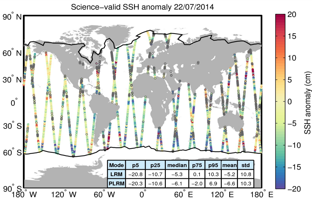
Figure 10. Geographical distribution of science-valid SSH anomaly data over oceans and lakes for 22/07/2014. The statistical values shown in the table refer to the SSH anomaly in cm and are calculated separately for LRM and PLRM regions. The black lines mark the outer limit of the Arctic and Antarctic polar polygons. Gray circles denote records that have been rejected based on the editing criteria described in Table 2.
