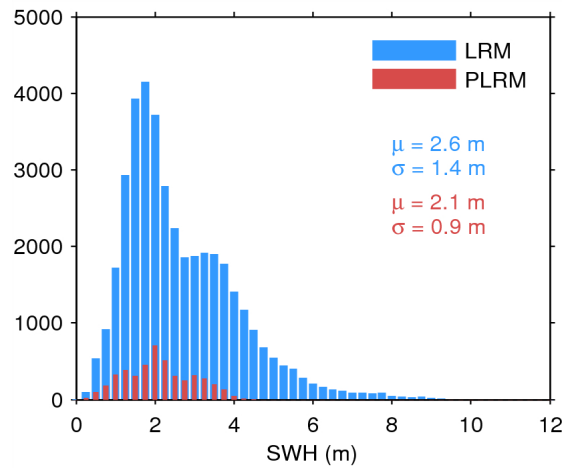
Figure 20. Histogram of science-valid SWH over oceans and lakes for LRM (blue) and PLRM (red) for 22/07/2014. The mean ( \mu ) and standard deviation ( \sigma ) are also shown. Note that values larger than 12 m are excluded from the histogram for the sake of readability but not from the computation of \mu and \sigma .
