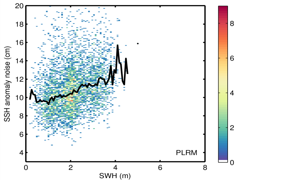
Figure 9. 2D histogram showing flag-valid SSH anomaly noise as a function of SWH for LRM (top) and PLRM (bottom) for 22/07/2014. The black line denotes the median SSH anomaly as a function of SWH.
