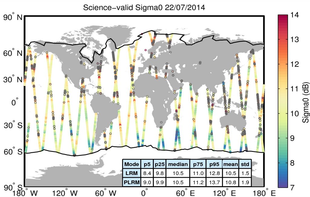
Figure 27. Geographical distribution of science-valid sigma0 data over oceans and lakes for 22/07/2014. The statistical values shown in the table refer to the sigma0 in dB and are calculated separately for LRM and PLRM regions. The black lines mark the outer limit of the Arctic and Antarctic polar polygons. Gray circles denote records that have been rejected based on the editing criteria described in Table 4.
