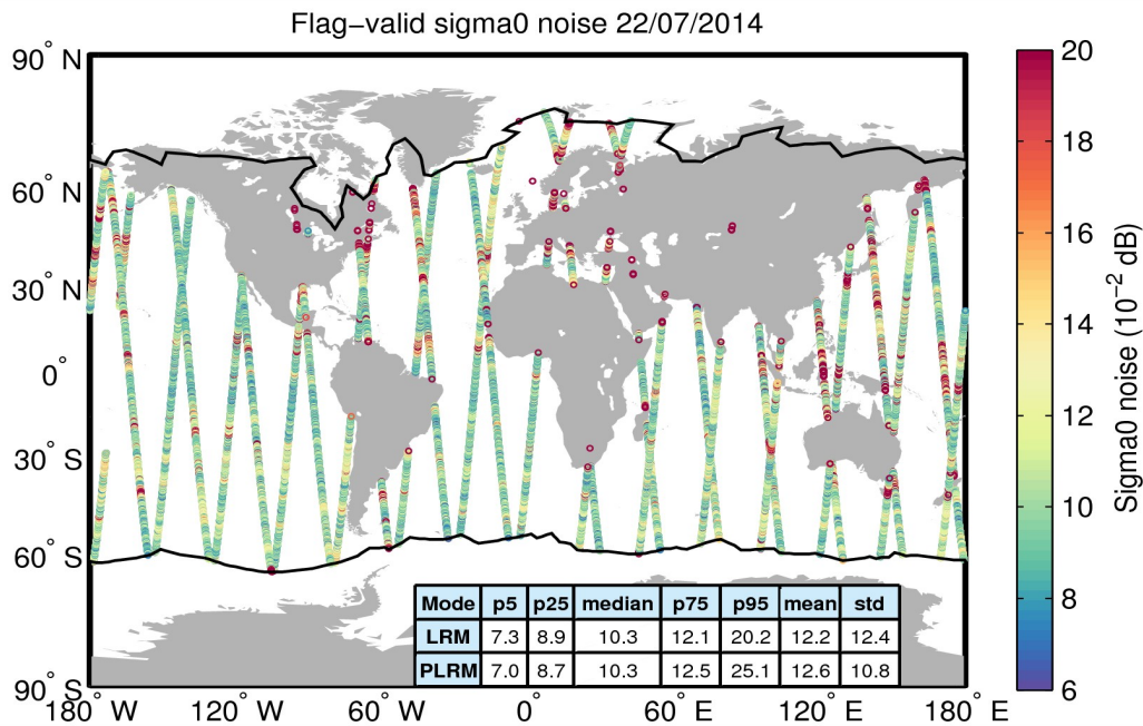
Figure 26. Geographical distribution of flag-valid 20-Hz sigma0 measurement noise over oceans and lakes for 22/07/2014. The statistical values shown in the table refer to the sigma0 noise and are calculated separately for LRM and PLRM regions. Measurements taken over polar polygons have been excluded from the computation of the statistical values. The black lines mark the outer limit of the Arctic and Antarctic polar polygons.
