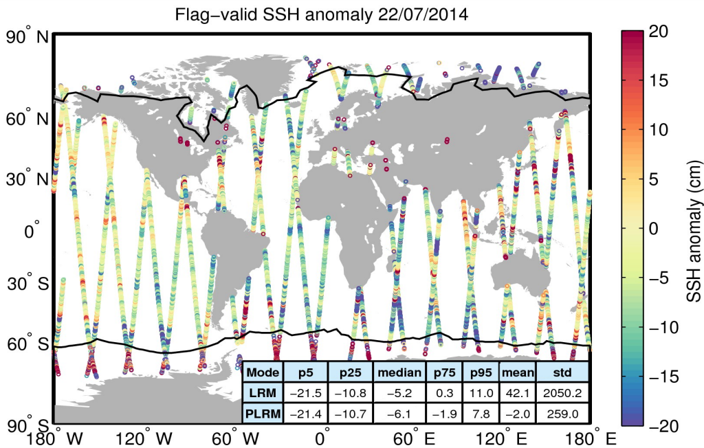
Figure 5. Geographical distribution of flag-valid 1-Hz SSH anomaly data over oceans and lakes for 22/07/2014. The statistical values shown in the table refer to the SSH anomaly in cm and are calculated separately for LRM and PLRM regions. Measurements taken over polar polygons have been excluded from the computation of the statistical values. The black lines mark the outer limit of the Arctic and Antarctic polar polygons.
