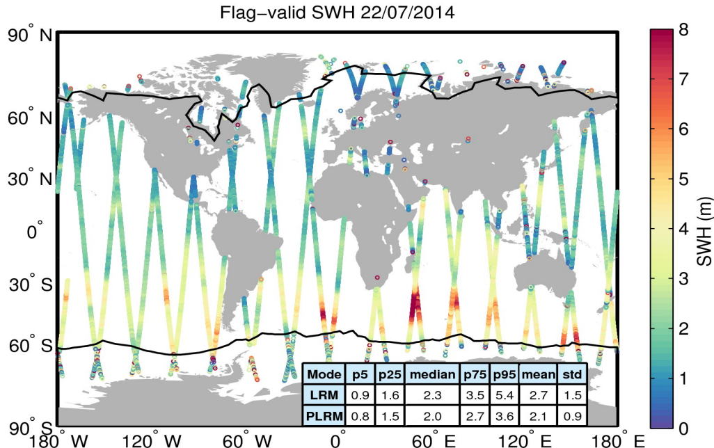
Figure 15. Geographical distribution of flag-valid SWH data over oceans and lakes for 22/07/2014. The statistical values shown in the table refer to the SWH in m and are calculated separately for LRM and PLRM regions. Measurements taken over polar polygons have been excluded from the computation of the statistical values. The black lines mark the outer limit of the Arctic and Antarctic polar polygons.
