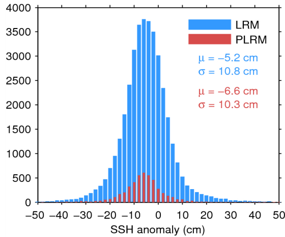
Figure 11. Histogram of science-valid SSH anomaly over oceans and lakes for LRM (blue) and PLRM (red) for 22/07/2014. The mean ( \mu ) and standard deviation ( \sigma ) are also shown. Note that values outside [-50 50] cm are excluded from the histogram for the sake of readability but not from the computation of \mu and \sigma .
