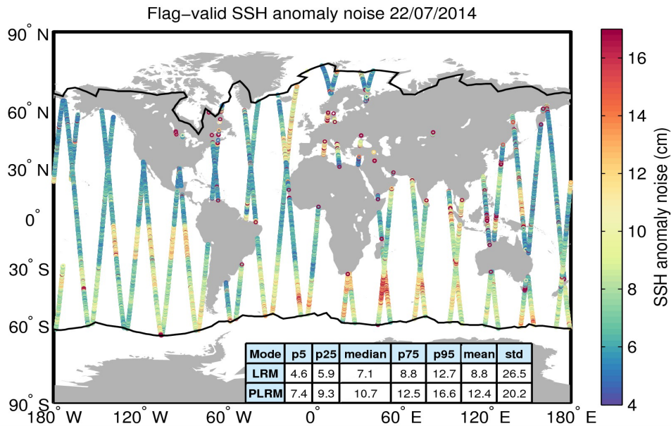
Figure 8. Geographical distribution of flag-valid 20-Hz SSH anomaly measurement noise over oceans and lakes for 22/07/2014. The statistical values shown in the table refer to the SSH anomaly noise and are calculated separately for LRM and PLRM regions. Measurements taken over polar polygons have been excluded from the computation of the statistical values. The black lines mark the outer limit of the Arctic and Antarctic polar polygons.
