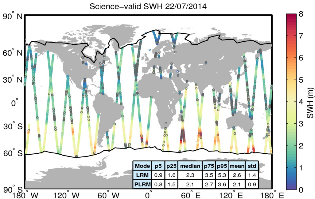
Figure 19. Geographical distribution of science-valid SWH data over oceans and lakes for 22/07/2014. The statistical values shown in the table refer to the SWH in m and are calculated separately for LRM and PLRM regions. The black lines mark the outer limit of the Arctic and Antarctic polar polygons. Gray circles denote records that have been rejected based on the editing criteria described in Table 3.
