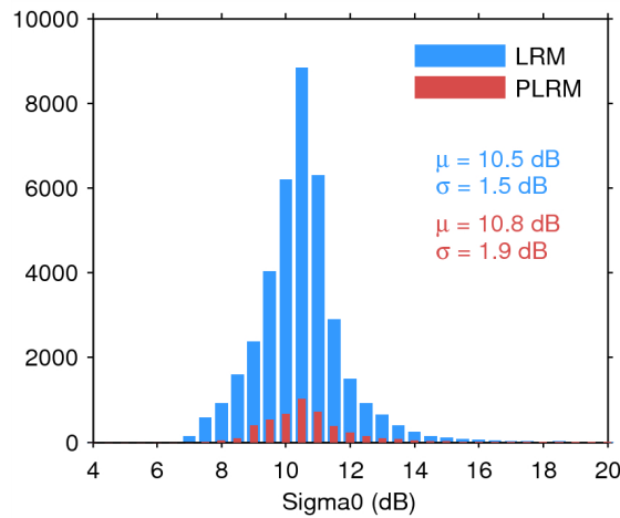
Figure 28. Histogram of science-valid sigma0 over oceans and lakes for LRM (blue) and PLRM (red) for 22/07/2014. The mean ( \mu ) and standard deviation ( \sigma ) are also shown. Note that values outside [4 20] dB are excluded from the histogram for the sake of readability but not from the computation of \mu and \sigma .
