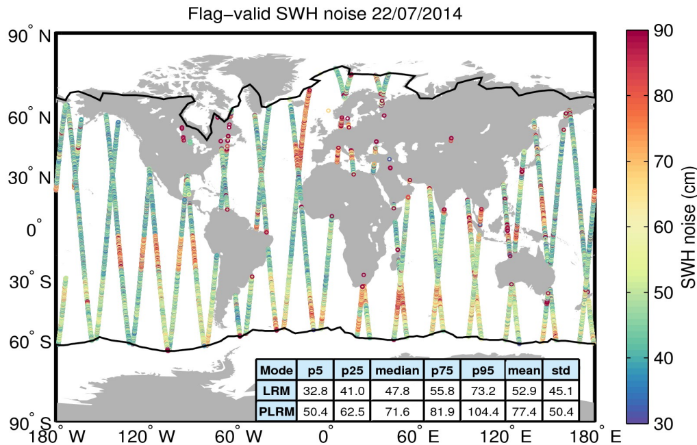
Figure 18. Geographical distribution of flag-valid 20-Hz SWH measurement noise over oceans and lakes for 22/07/2014. The statistical values shown in the table refer to the SWH noise and are calculated separately for LRM and PLRM regions. Measurements taken over polar polygons have been excluded from the computation of the statistical values. The black lines mark the outer limit of the Arctic and Antarctic polar polygons.
