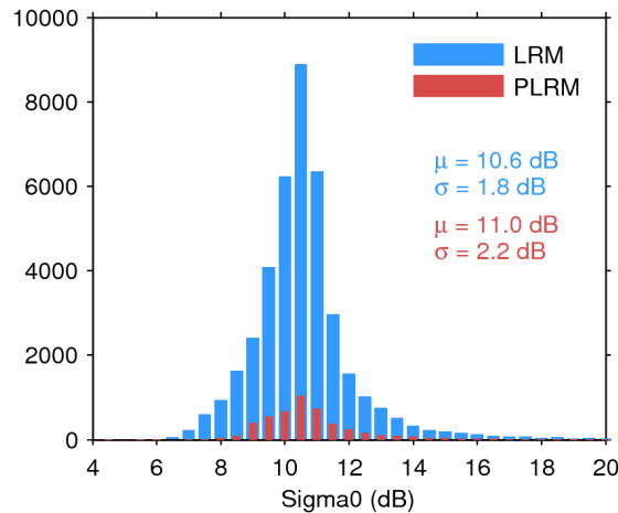
Figure 25. Histogram of flag-valid sigma0 over oceans and lakes for LRM (blue) and PLRM (red) for 22/07/2014. The mean ( \mu ) and standard deviation ( \sigma ) are also shown. Note that values outside [4 20] dB are excluded from the histogram for the sake of readability but not from the computation of \mu and \sigma .
