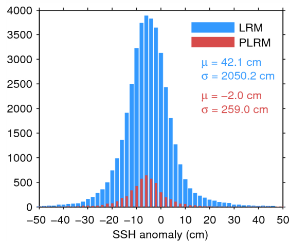
Figure 7. Histogram of flag-valid SSH anomaly over oceans and lakes for LRM (blue) and PLRM (red) for 22/07/2014. The mean ( \mu ) and standard deviation ( \sigma ) are also shown. Note that values outside [-50 \ 50] cm are excluded from the histogram for the sake of readability but not from the computation of \mu and \sigma .
