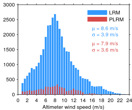
Figure 33. Histogram of flag-valid wind over oceans and lakes for LRM (blue) and PLRM (red) for 22/07/2014. The mean ( \mu ) and standard deviation ( \sigma ) are also shown. Note that values larger than 24 m/s are excluded from the histogram for the sake of readability but not from the computation of \mu and \sigma .
