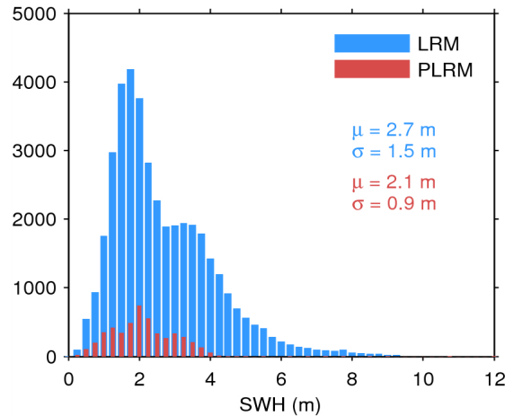
Figure 17. Histogram of flag-valid SWH over oceans and lakes for LRM (blue) and PLRM (red) for 22/07/2014. The mean ( \mu ) and standard deviation ( \sigma ) are also shown. Note that values larger than 12 m are excluded from the histogram for the sake of readability but not from the computation of \mu and \sigma .
