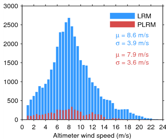
Figure 35. Histogram of science-valid wind over oceans and lakes for LRM (blue) and PLRM (red) for 22/07/2014. The mean ( \mu ) and standard deviation ( \sigma ) are also shown. Note that values larger than 24 m/s are excluded from the histogram for the sake of readability but not from the computation of \mu and \sigma .
