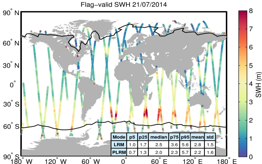
Figure 15. Geographical distribution of flag-valid SWH data over oceans and lakes for 21/07/2014. The statistical values shown in the table refer to the SWH in m and are calculated separately for LRM and PLRM regions. Measurements taken over polar polygons have been excluded from the computation of the statistical values. The black lines mark the outer limit of the Arctic and Antarctic polar polygons.
