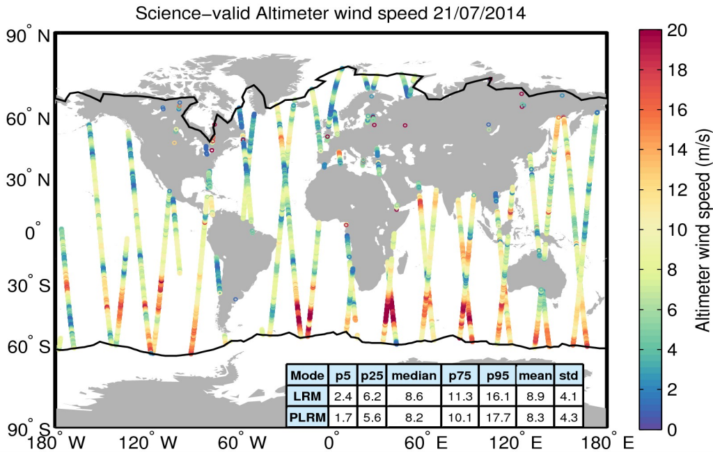
Figure 34. Geographical distribution of science-valid wind data over oceans and lakes for 21/07/2014. The statistical values shown in the table refer to the wind in m/s and are calculated separately for LRM and PLRM regions. The black lines mark the outer limit of the Arctic and Antarctic polar polygons. Gray circles denote records that have been rejected based on the editing criteria described in Table 5.
