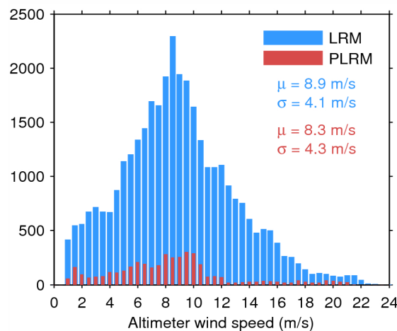
Figure 35. Histogram of science-valid wind over oceans and lakes for LRM (blue) and PLRM (red) for 21/07/2014. The mean ( \mu ) and standard deviation ( \sigma ) are also shown. Note that values larger than 24 m/s are excluded from the histogram for the sake of readability but not from the computation of \mu and \sigma .
