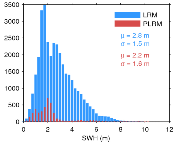
Figure 17. Histogram of flag-valid SWH over oceans and lakes for LRM (blue) and PLRM (red) for 21/07/2014. The mean ( \mu ) and standard deviation ( \sigma ) are also shown. Note that values larger than 12 m are excluded from the histogram for the sake of readability but not from the computation of \mu and \sigma .
