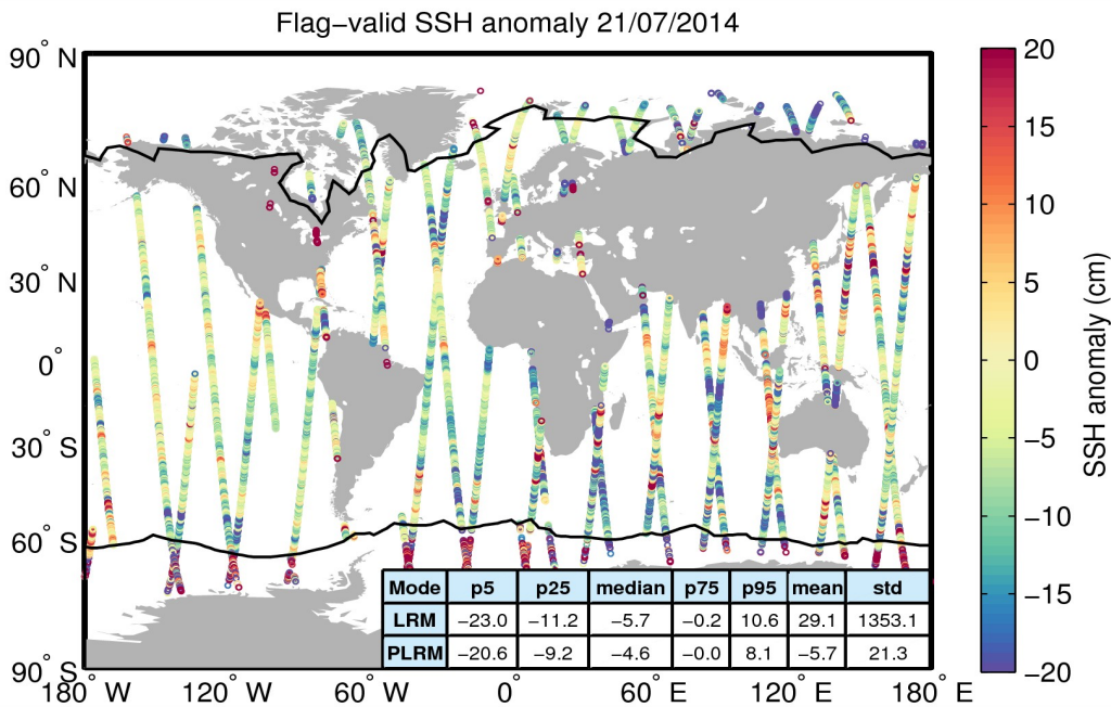
Figure 5. Geographical distribution of flag-valid 1-Hz SSH anomaly data over oceans and lakes for 21/07/2014. The statistical values shown in the table refer to the SSH anomaly in cm and are calculated separately for LRM and PLRM regions. Measurements taken over polar polygons have been excluded from the computation of the statistical values. The black lines mark the outer limit of the Arctic and Antarctic polar polygons.
