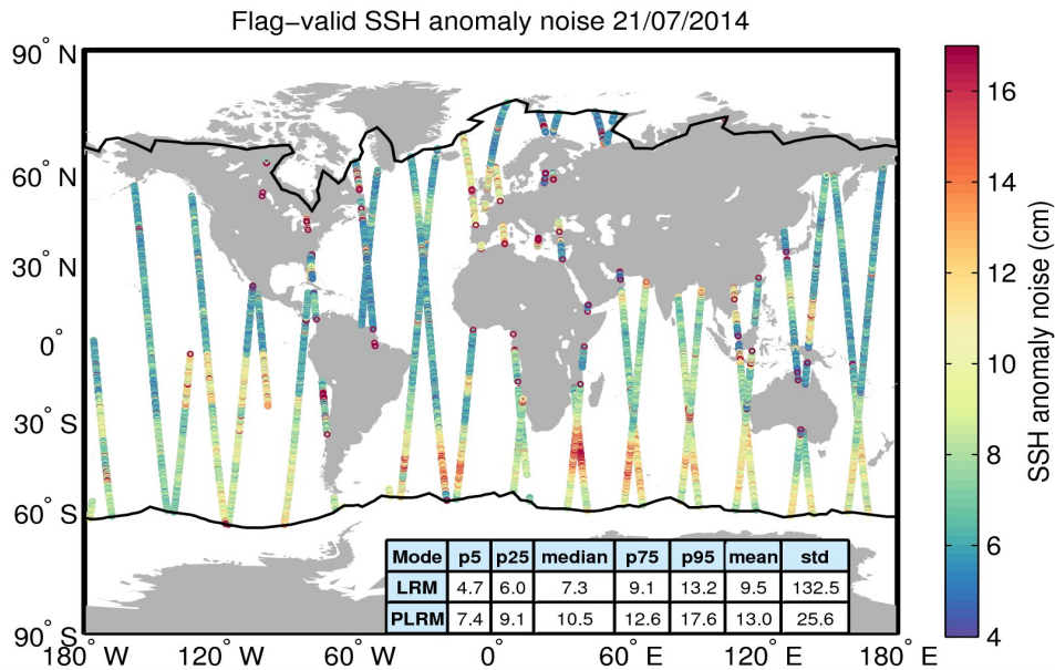
Figure 8. Geographical distribution of flag-valid 20-Hz SSH anomaly measurement noise over oceans and lakes for 21/07/2014. The statistical values shown in the table refer to the SSH anomaly noise and are calculated separately for LRM and PLRM regions. Measurements taken over polar polygons have been excluded from the computation of the statistical values. The black lines mark the outer limit of the Arctic and Antarctic polar polygons.
