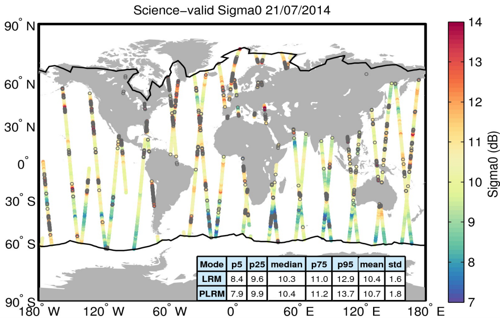
Figure 27. Geographical distribution of science-valid sigma0 data over oceans and lakes for 21/07/2014. The statistical values shown in the table refer to the sigma0 in dB and are calculated separately for LRM and PLRM regions. The black lines mark the outer limit of the Arctic and Antarctic polar polygons. Gray circles denote records that have been rejected based on the editing criteria described in Table 4.
