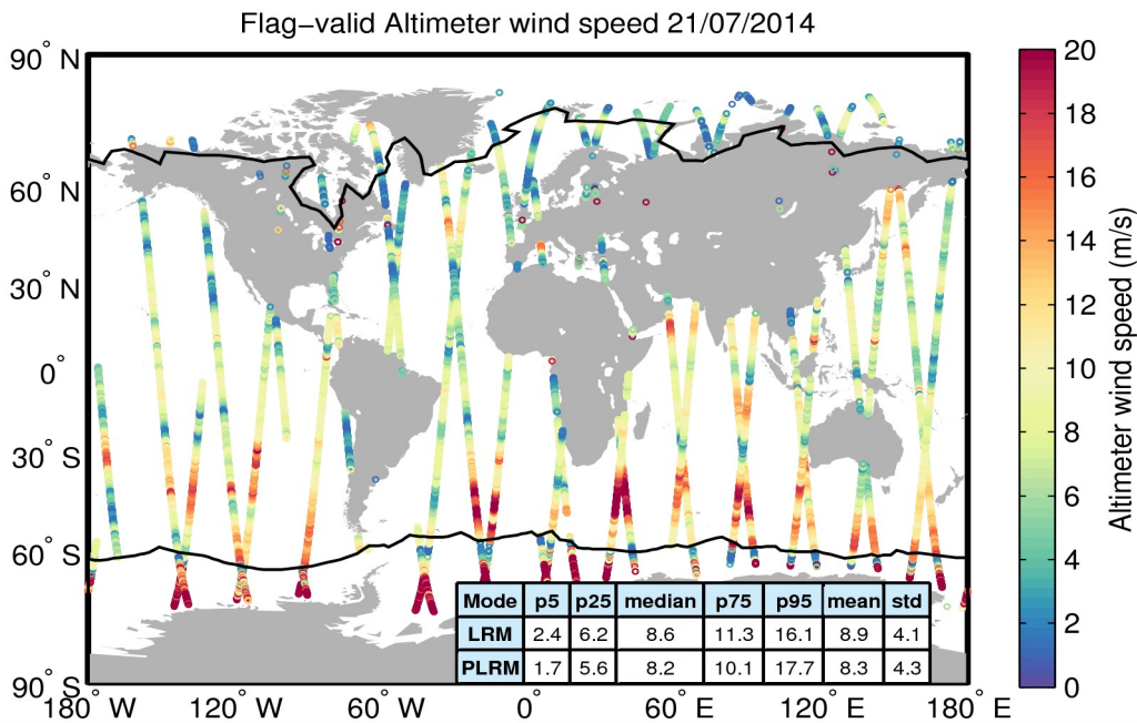
Figure 31. Geographical distribution of flag-valid wind data over oceans and lakes for 21/07/2014. The statistical values shown in the table refer to the wind in m/s and are calculated separately for LRM and PLRM regions. Measurements taken over polar polygons have been excluded from the computation of the statistical values. The black lines mark the outer limit of the Arctic and Antarctic polar polygons.
