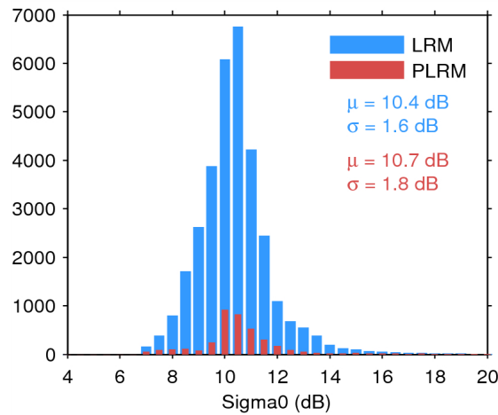
Figure 28. Histogram of science-valid sigma0 over oceans and lakes for LRM (blue) and PLRM (red) for 21/07/2014. The mean ( \mu ) and standard deviation ( \sigma ) are also shown. Note that values outside [4 20] dB are excluded from the histogram for the sake of readability but not from the computation of \mu and \sigma .
