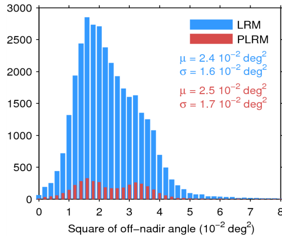
Figure 39. Histogram of flag-valid mispointing over oceans and lakes for LRM (blue) and PLRM (red) for 21/07/2014. Only positive values have been considered. The mean ( \mu ) and standard deviation ( \sigma ) are also shown. Note that values 8 \cdot 10^{-2} \text{ deg}^2 are excluded from the histogram for the sake of readability but not from the computation of \mu and \sigma .
