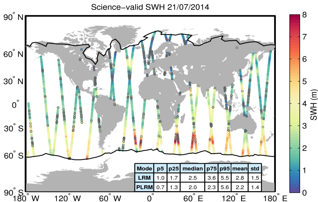
Figure 19. Geographical distribution of science-valid SWH data over oceans and lakes for 21/07/2014. The statistical values shown in the table refer to the SWH in m and are calculated separately for LRM and PLRM regions. The black lines mark the outer limit of the Arctic and Antarctic polar polygons. Gray circles denote records that have been rejected based on the editing criteria described in Table 3.
