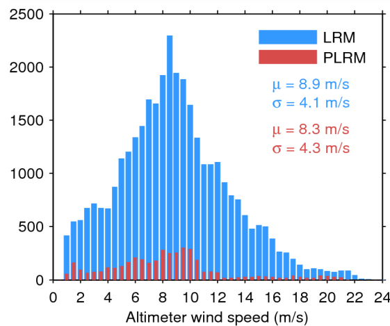
Figure 33. Histogram of flag-valid wind over oceans and lakes for LRM (blue) and PLRM (red) for 21/07/2014. The mean ( \mu ) and standard deviation ( \sigma ) are also shown. Note that values larger than 24 m/s are excluded from the histogram for the sake of readability but not from the computation of \mu and \sigma .
