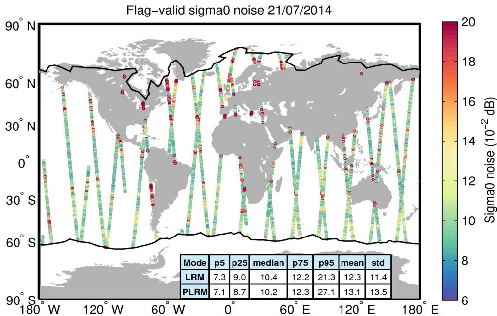
Figure 26. Geographical distribution of flag-valid 20-Hz sigma0 measurement noise over oceans and lakes for 21/07/2014. The statistical values shown in the table refer to the sigma0 noise and are calculated separately for LRM and PLRM regions. Measurements taken over polar polygons have been excluded from the computation of the statistical values. The black lines mark the outer limit of the Arctic and Antarctic polar polygons.
