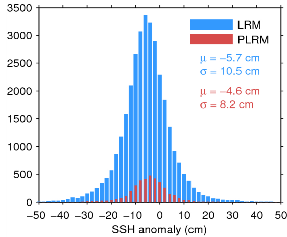
Figure 11. Histogram of science-valid SSH anomaly over oceans and lakes for LRM (blue) and PLRM (red) for 21/07/2014. The mean ( \mu ) and standard deviation ( \sigma ) are also shown. Note that values outside [-50\ 50] cm are excluded from the histogram for the sake of readability but not from the computation of \mu and \sigma .
