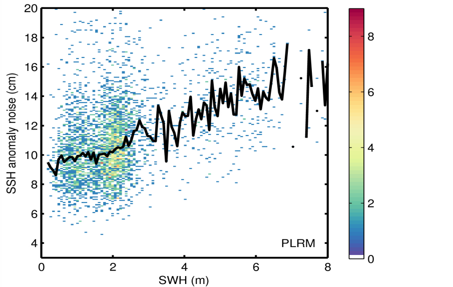
Figure 9. 2D histogram showing flag-valid SSH anomaly noise as a function of SWH for LRM (top) and PLRM (bottom) for 21/07/2014. The black line denotes the median SSH anomaly as a function of SWH.
