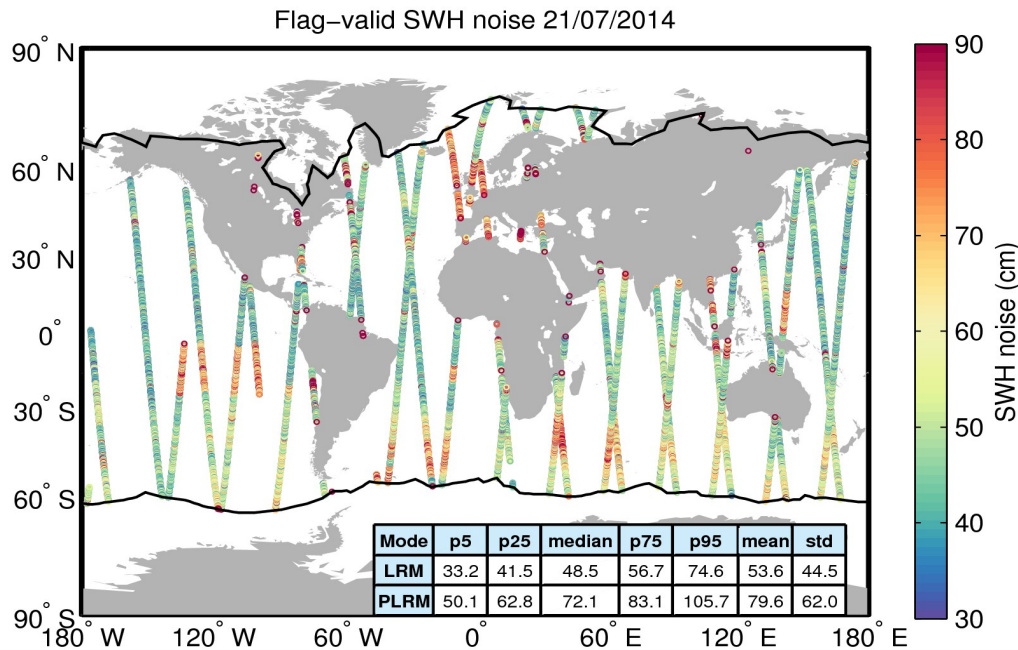
Figure 18. Geographical distribution of flag-valid 20-Hz SWH measurement noise over oceans and lakes for 21/07/2014. The statistical values shown in the table refer to the SWH noise and are calculated separately for LRM and PLRM regions. Measurements taken over polar polygons have been excluded from the computation of the statistical values. The black lines mark the outer limit of the Arctic and Antarctic polar polygons.
