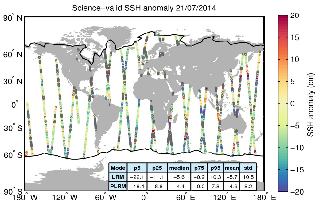
Figure 10. Geographical distribution of science-valid SSH anomaly data over oceans and lakes for 21/07/2014. The statistical values shown in the table refer to the SSH anomaly in cm and are calculated separately for LRM and PLRM regions. The black lines mark the outer limit of the Arctic and Antarctic polar polygons. Gray circles denote records that have been rejected based on the editing criteria described in Table 2.
