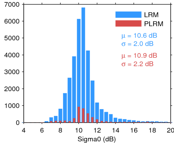
Figure 25. Histogram of flag-valid sigma0 over oceans and lakes for LRM (blue) and PLRM (red) for 21/07/2014. The mean ( \mu ) and standard deviation ( \sigma ) are also shown. Note that values outside [4 20] dB are excluded from the histogram for the sake of readability but not from the computation of \mu and \sigma .
