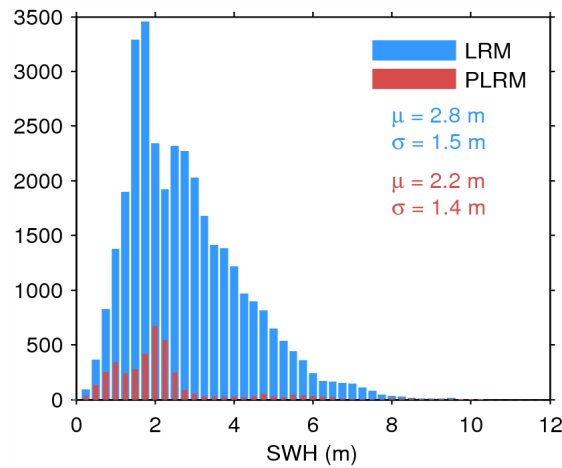
Figure 20. Histogram of science-valid SWH over oceans and lakes for LRM (blue) and PLRM (red) for 21/07/2014. The mean ( \mu ) and standard deviation ( \sigma ) are also shown. Note that values larger than 12 m are excluded from the histogram for the sake of readability but not from the computation of \mu and \sigma .
