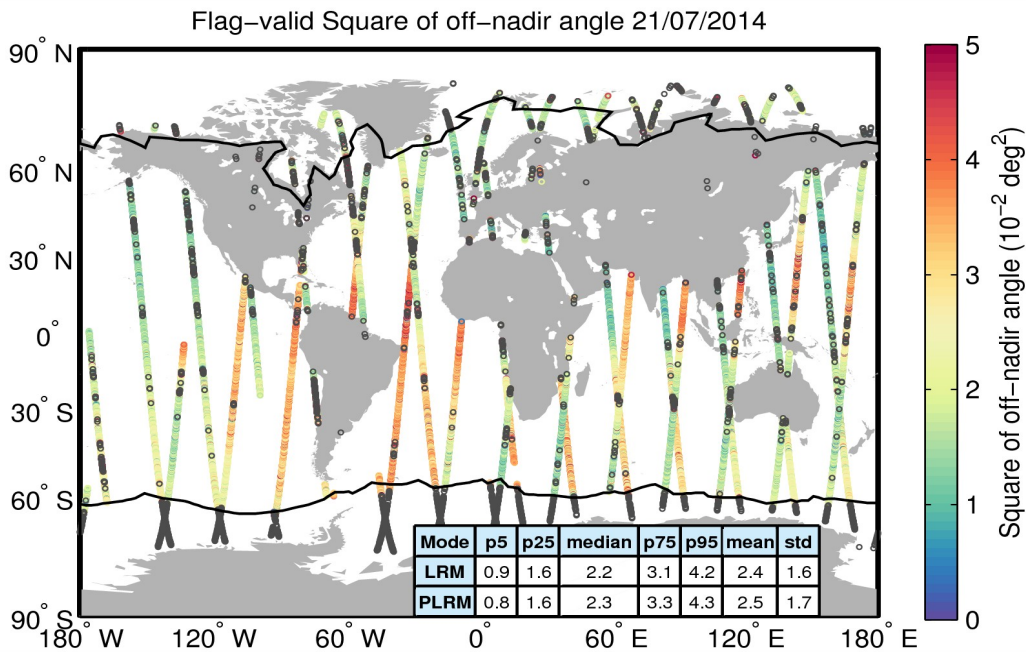
Figure 37. Geographical distribution of flag-valid mispointing data over oceans and lakes for 21/07/2014. The statistical values shown in the table refer to the mispointing in 10^{-2} \text{ deg}^2 and are calculated separately for LRM and PLRM regions. Measurements taken over polar polygons have been excluded from the computation of the statistical values. The black lines mark the outer limit of the Arctic and Antarctic polar polygons. Gray circles denote negative values.
