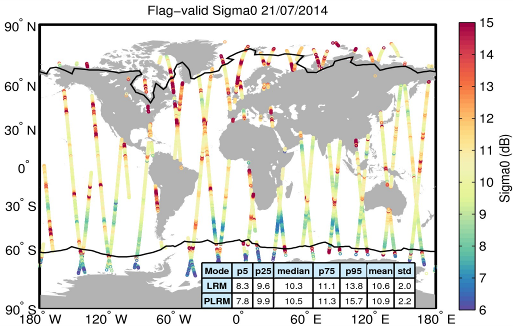
Figure 23. Geographical distribution of flag-valid sigma0 data over oceans and lakes for 21/07/2014. The statistical values shown in the table refer to the sigma0 in dB and are calculated separately for LRM and PLRM regions. Measurements taken over polar polygons have been excluded from the computation of the statistical values. The black lines mark the outer limit of the Arctic and Antarctic polar polygons.
