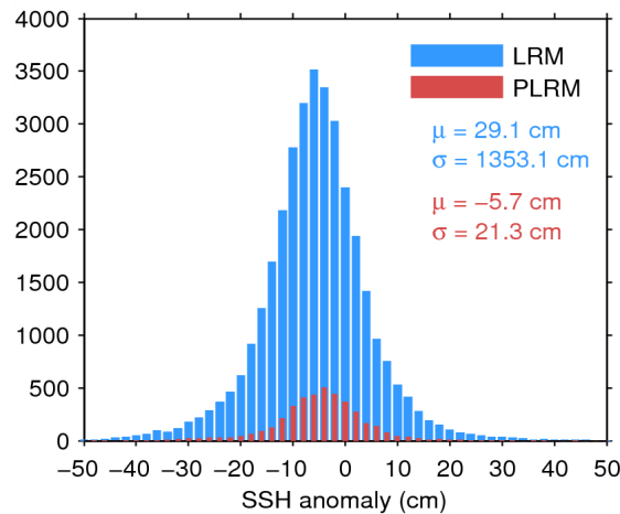
Figure 7. Histogram of flag-valid SSH anomaly over oceans and lakes for LRM (blue) and PLRM (red) for 21/07/2014. The mean ( \mu ) and standard deviation ( \sigma ) are also shown. Note that values outside [-50\ 50] cm are excluded from the histogram for the sake of readability but not from the computation of \mu and \sigma .
