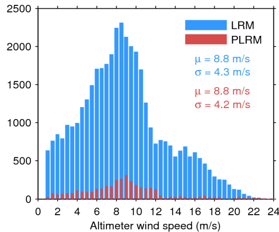
Figure 33. Histogram of flag-valid wind over oceans and lakes for LRM (blue) and PLRM (red) for 19/07/2014. The mean ( \mu ) and standard deviation ( \sigma ) are also shown. Note that values larger than 24 m/s are excluded from the histogram for the sake of readability but not from the computation of \mu and \sigma .
