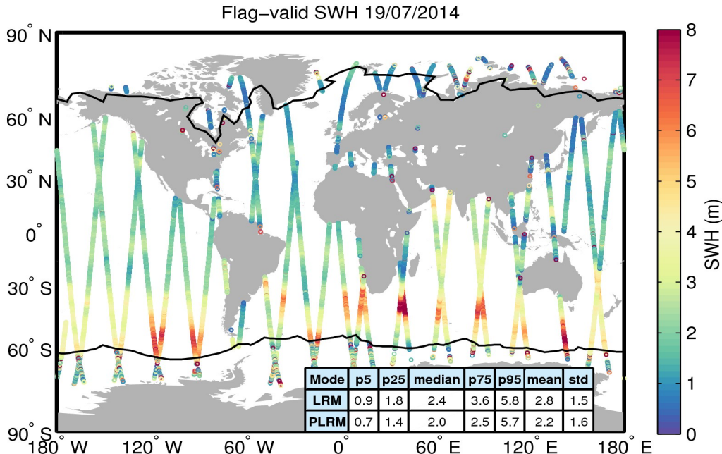
Figure 15. Geographical distribution of flag-valid SWH data over oceans and lakes for 19/07/2014. The statistical values shown in the table refer to the SWH in m and are calculated separately for LRM and PLRM regions. Measurements taken over polar polygons have been excluded from the computation of the statistical values. The black lines mark the outer limit of the Arctic and Antarctic polar polygons.
