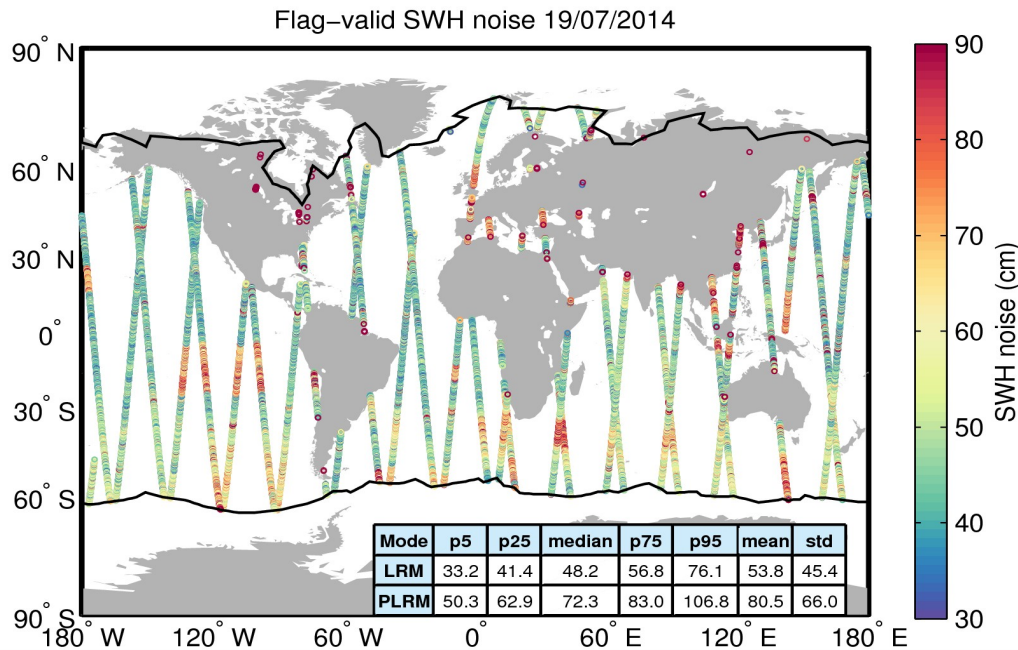
Figure 18. Geographical distribution of flag-valid 20-Hz SWH measurement noise over oceans and lakes for 19/07/2014. The statistical values shown in the table refer to the SWH noise and are calculated separately for LRM and PLRM regions. Measurements taken over polar polygons have been excluded from the computation of the statistical values. The black lines mark the outer limit of the Arctic and Antarctic polar polygons.
