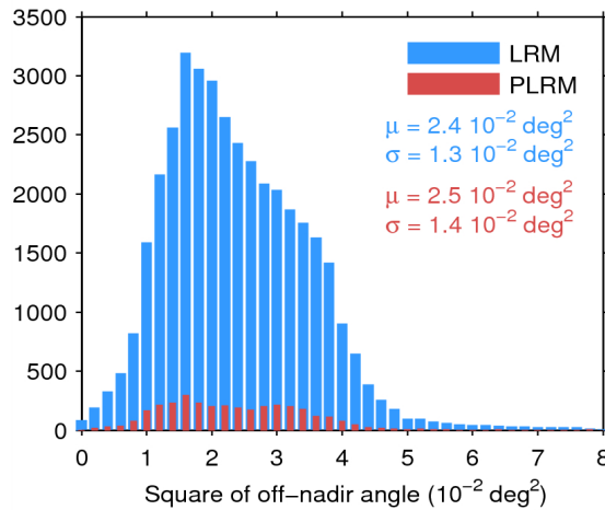
Figure 39. Histogram of flag-valid mispointing over oceans and lakes for LRM (blue) and PLRM (red) for 19/07/2014. Only positive values have been considered. The mean ( \mu ) and standard deviation ( \sigma ) are also shown. Note that values 8 \cdot 10^{-2} \text{ deg}^2 are excluded from the histogram for the sake of readability but not from the computation of \mu and \sigma .
