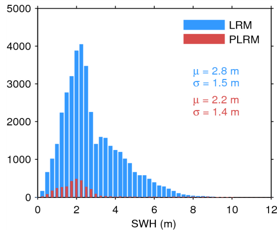
Figure 20. Histogram of science-valid SWH over oceans and lakes for LRM (blue) and PLRM (red) for 19/07/2014. The mean ( \mu ) and standard deviation ( \sigma ) are also shown. Note that values larger than 12 m are excluded from the histogram for the sake of readability but not from the computation of \mu and \sigma .
