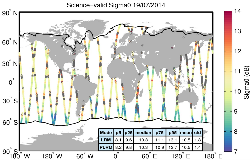
Figure 27. Geographical distribution of science-valid sigma0 data over oceans and lakes for 19/07/2014. The statistical values shown in the table refer to the sigma0 in dB and are calculated separately for LRM and PLRM regions. The black lines mark the outer limit of the Arctic and Antarctic polar polygons. Gray circles denote records that have been rejected based on the editing criteria described in Table 4.
