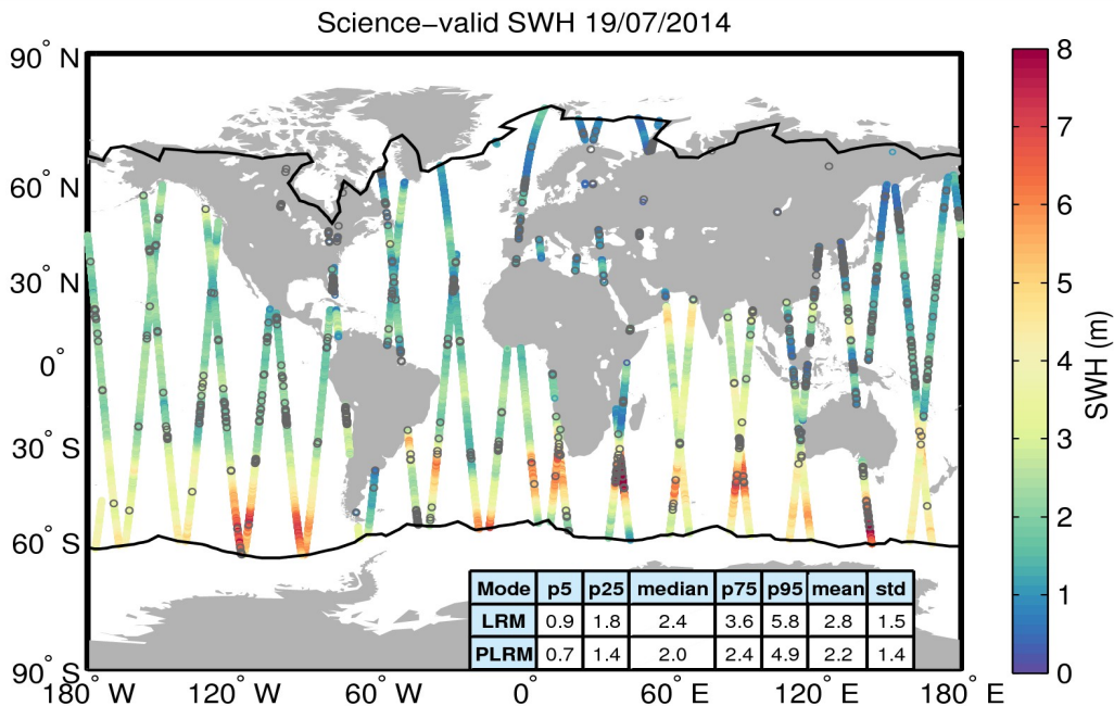
Figure 19. Geographical distribution of science-valid SWH data over oceans and lakes for 19/07/2014. The statistical values shown in the table refer to the SWH in m and are calculated separately for LRM and PLRM regions. The black lines mark the outer limit of the Arctic and Antarctic polar polygons. Gray circles denote records that have been rejected based on the editing criteria described in Table 3.
