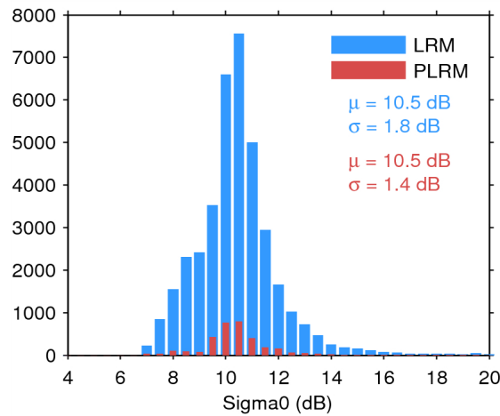
Figure 28. Histogram of science-valid sigma0 over oceans and lakes for LRM (blue) and PLRM (red) for 19/07/2014. The mean ( \mu ) and standard deviation ( \sigma ) are also shown. Note that values outside [4 20] dB are excluded from the histogram for the sake of readability but not from the computation of \mu and \sigma .
