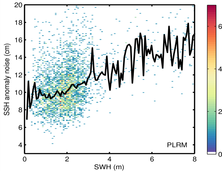
Figure 9. 2D histogram showing flag-valid SSH anomaly noise as a function of SWH for LRM (top) and PLRM (bottom) for 19/07/2014. The black line denotes the median SSH anomaly as a function of SWH.
