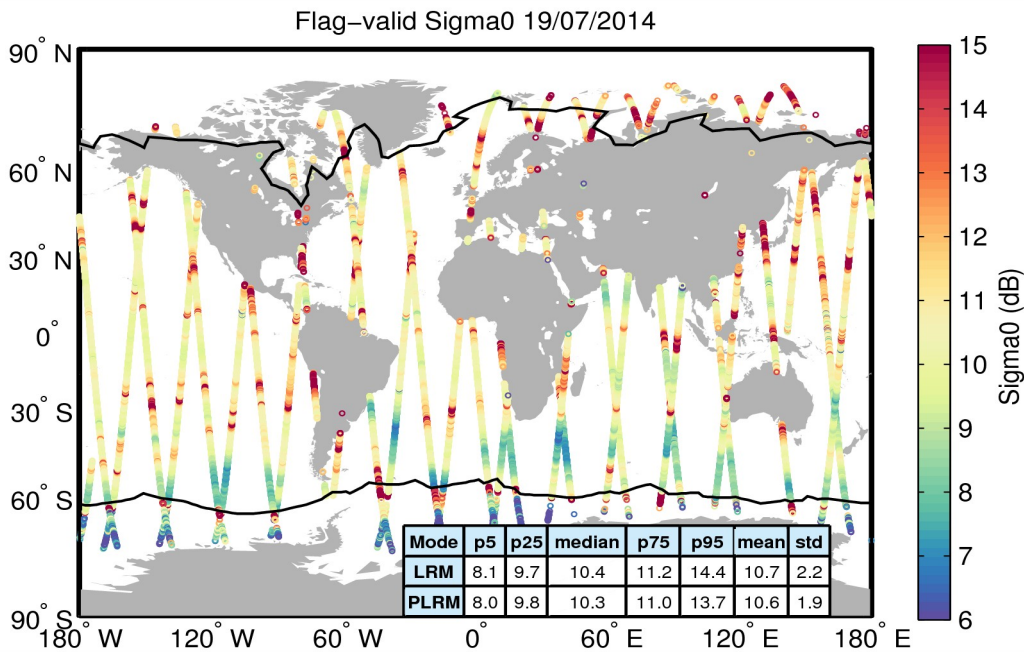
Figure 23. Geographical distribution of flag-valid sigma0 data over oceans and lakes for 19/07/2014. The statistical values shown in the table refer to the sigma0 in dB and are calculated separately for LRM and PLRM regions. Measurements taken over polar polygons have been excluded from the computation of the statistical values. The black lines mark the outer limit of the Arctic and Antarctic polar polygons.
