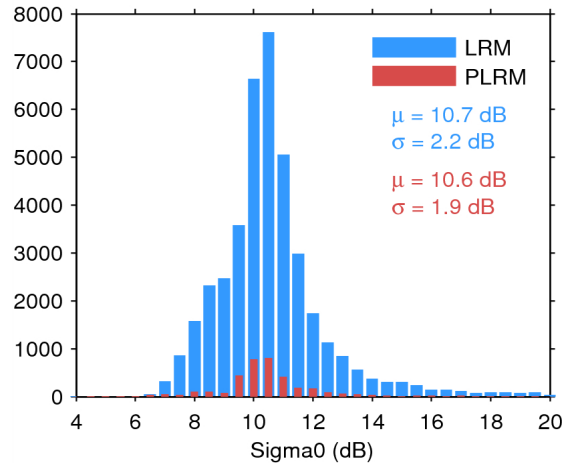
Figure 25. Histogram of flag-valid sigma0 over oceans and lakes for LRM (blue) and PLRM (red) for 19/07/2014. The mean ( \mu ) and standard deviation ( \sigma ) are also shown. Note that values outside [4 20] dB are excluded from the histogram for the sake of readability but not from the computation of \mu and \sigma .
