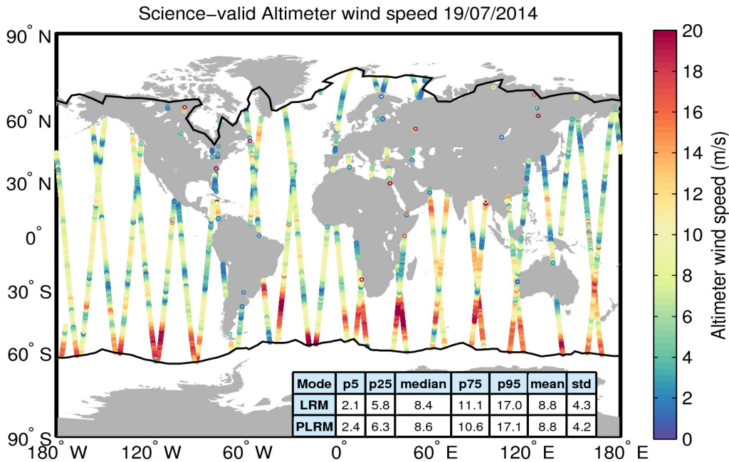
Figure 34. Geographical distribution of science-valid wind data over oceans and lakes for 19/07/2014. The statistical values shown in the table refer to the wind in m/s and are calculated separately for LRM and PLRM regions. The black lines mark the outer limit of the Arctic and Antarctic polar polygons. Gray circles denote records that have been rejected based on the editing criteria described in Table 5.
