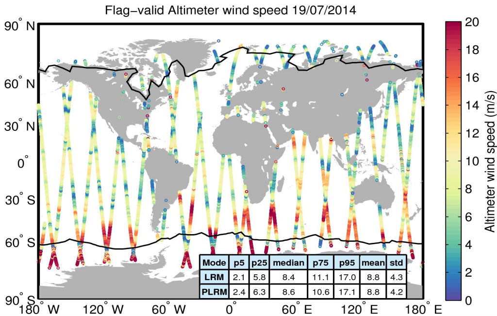
Figure 31. Geographical distribution of flag-valid wind data over oceans and lakes for 19/07/2014. The statistical values shown in the table refer to the wind in m/s and are calculated separately for LRM and PLRM regions. Measurements taken over polar polygons have been excluded from the computation of the statistical values. The black lines mark the outer limit of the Arctic and Antarctic polar polygons.
