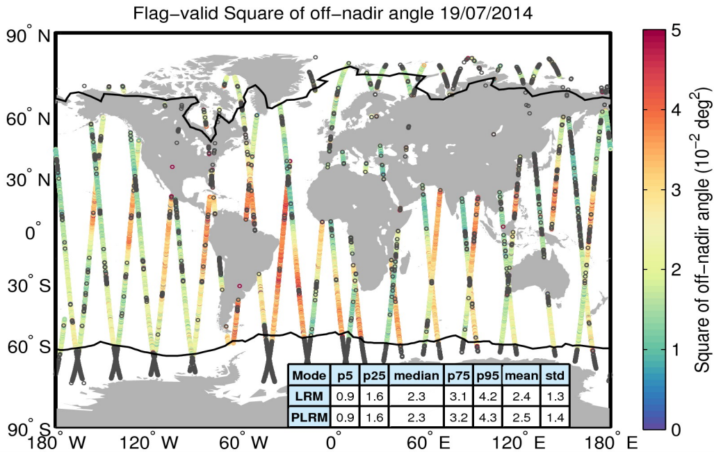
Figure 37. Geographical distribution of flag-valid mispointing data over oceans and lakes for 19/07/2014. The statistical values shown in the table refer to the mispointing in 10^{-2} deg 2 and are calculated separately for LRM and PLRM regions. Measurements taken over polar polygons have been excluded from the computation of the statistical values. The black lines mark the outer limit of the Arctic and Antarctic polar polygons. Gray circles denote negative values.
