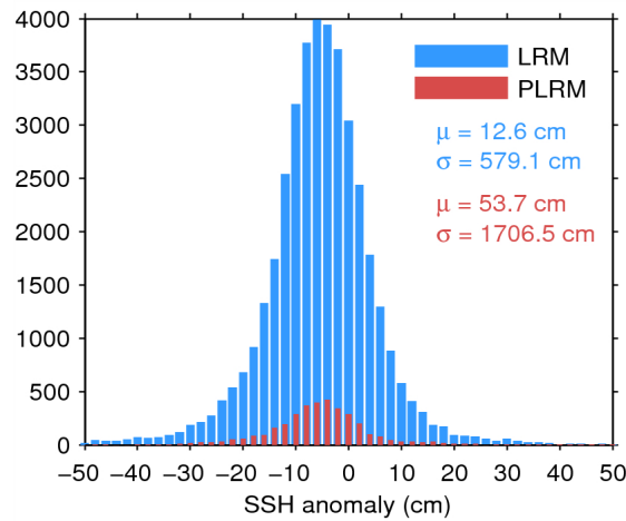
Figure 7. Histogram of flag-valid SSH anomaly over oceans and lakes for LRM (blue) and PLRM (red) for 19/07/2014. The mean ( \mu ) and standard deviation ( \sigma ) are also shown. Note that values outside [-50\ 50] cm are excluded from the histogram for the sake of readability but not from the computation of \mu and \sigma .
