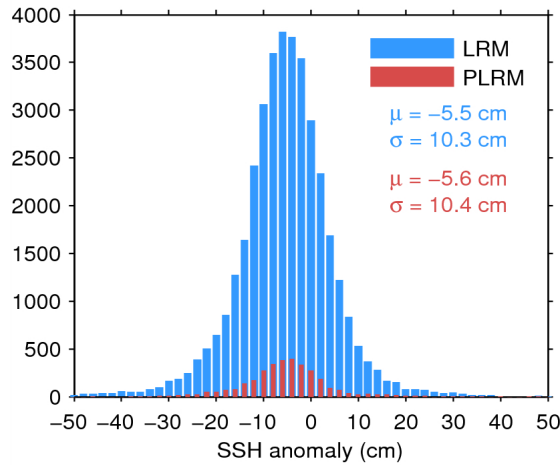
Figure 11. Histogram of science-valid SSH anomaly over oceans and lakes for LRM (blue) and PLRM (red) for 19/07/2014. The mean ( \mu ) and standard deviation ( \sigma ) are also shown. Note that values outside [-50 50] cm are excluded from the histogram for the sake of readability but not from the computation of \mu and \sigma .
