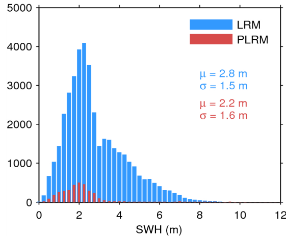
Figure 17. Histogram of flag-valid SWH over oceans and lakes for LRM (blue) and PLRM (red) for 19/07/2014. The mean ( \mu ) and standard deviation ( \sigma ) are also shown. Note that values larger than 12 m are excluded from the histogram for the sake of readability but not from the computation of \mu and \sigma .
