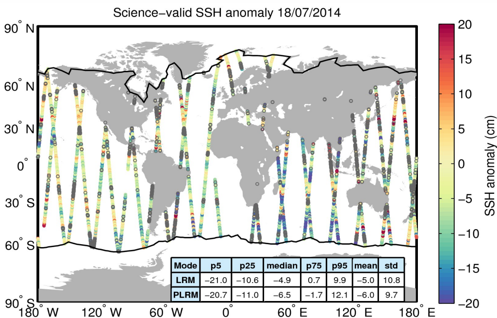
Figure 10. Geographical distribution of science-valid SSH anomaly data over oceans and lakes for 18/07/2014. The statistical values shown in the table refer to the SSH anomaly in cm and are calculated separately for LRM and PLRM regions. The black lines mark the outer limit of the Arctic and Antarctic polar polygons. Gray circles denote records that have been rejected based on the editing criteria described in Table 2.
