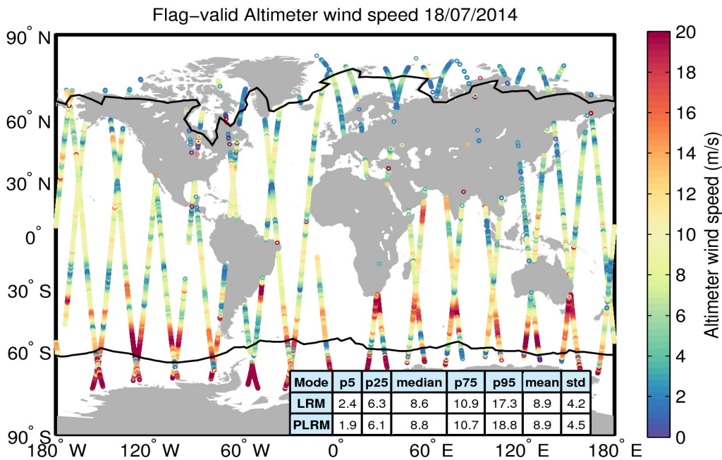
Figure 31. Geographical distribution of flag-valid wind data over oceans and lakes for 18/07/2014. The statistical values shown in the table refer to the wind in m/s and are calculated separately for LRM and PLRM regions. Measurements taken over polar polygons have been excluded from the computation of the statistical values. The black lines mark the outer limit of the Arctic and Antarctic polar polygons.
