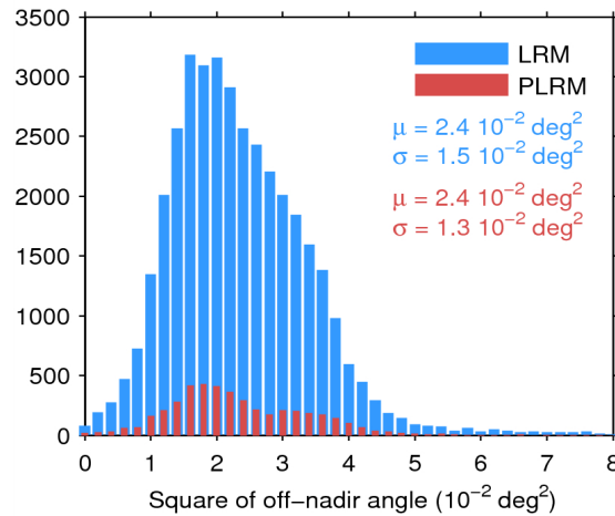
Figure 39. Histogram of flag-valid mispointing over oceans and lakes for LRM (blue) and PLRM (red) for 18/07/2014. Only positive values have been considered. The mean ( \mu ) and standard deviation ( \sigma ) are also shown. Note that values 8 \cdot 10^{-2} \text{ deg}^2 are excluded from the histogram for the sake of readability but not from the computation of \mu and \sigma .
