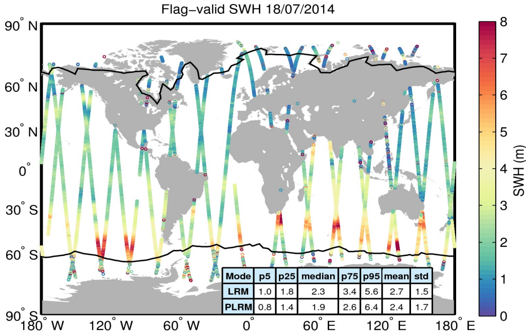
Figure 15. Geographical distribution of flag-valid SWH data over oceans and lakes for 18/07/2014. The statistical values shown in the table refer to the SWH in m and are calculated separately for LRM and PLRM regions. Measurements taken over polar polygons have been excluded from the computation of the statistical values. The black lines mark the outer limit of the Arctic and Antarctic polar polygons.
