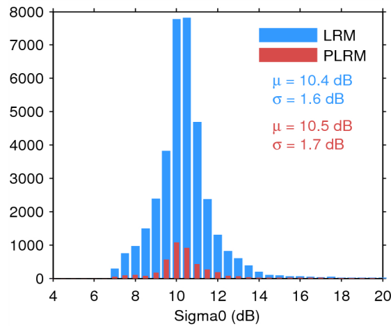
Figure 28. Histogram of science-valid sigma0 over oceans and lakes for LRM (blue) and PLRM (red) for 18/07/2014. The mean ( \mu ) and standard deviation ( \sigma ) are also shown. Note that values outside [4 20] dB are excluded from the histogram for the sake of readability but not from the computation of \mu and \sigma .
