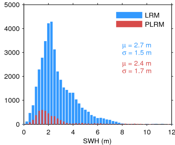
Figure 17. Histogram of flag-valid SWH over oceans and lakes for LRM (blue) and PLRM (red) for 18/07/2014. The mean ( \mu ) and standard deviation ( \sigma ) are also shown. Note that values larger than 12 m are excluded from the histogram for the sake of readability but not from the computation of \mu and \sigma .
