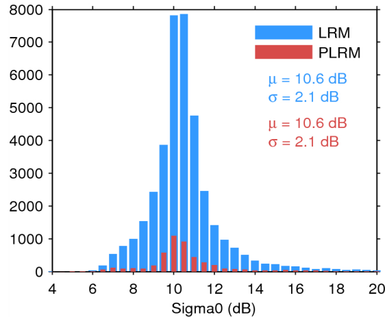
Figure 25. Histogram of flag-valid sigma0 over oceans and lakes for LRM (blue) and PLRM (red) for 18/07/2014. The mean ( \mu ) and standard deviation ( \sigma ) are also shown. Note that values outside [4 20] dB are excluded from the histogram for the sake of readability but not from the computation of \mu and \sigma .
