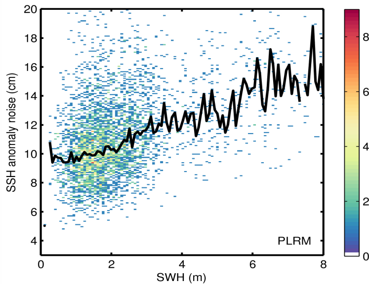
Figure 9. 2D histogram showing flag-valid SSH anomaly noise as a function of SWH for LRM (top) and PLRM (bottom) for 18/07/2014. The black line denotes the median SSH anomaly as a function of SWH.
