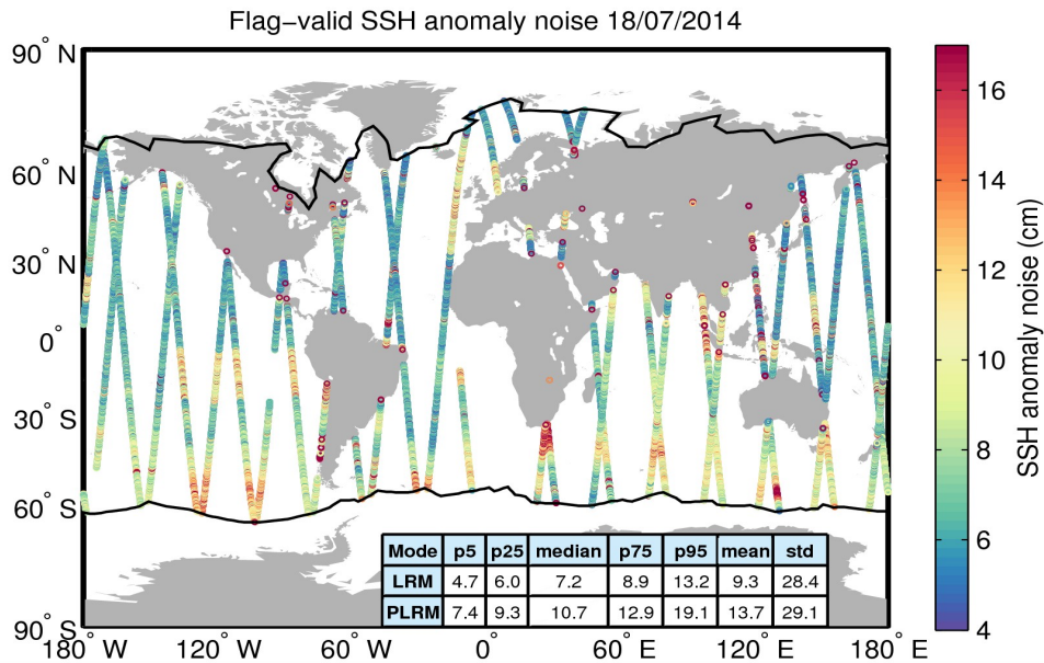
Figure 8. Geographical distribution of flag-valid 20-Hz SSH anomaly measurement noise over oceans and lakes for 18/07/2014. The statistical values shown in the table refer to the SSH anomaly noise and are calculated separately for LRM and PLRM regions. Measurements taken over polar polygons have been excluded from the computation of the statistical values. The black lines mark the outer limit of the Arctic and Antarctic polar polygons.
