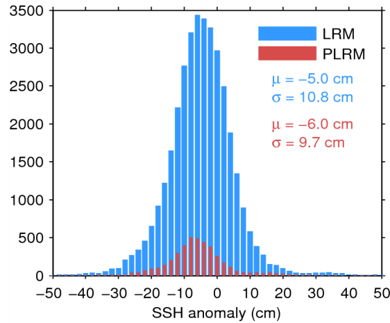
Figure 11. Histogram of science-valid SSH anomaly over oceans and lakes for LRM (blue) and PLRM (red) for 18/07/2014. The mean ( \mu ) and standard deviation ( \sigma ) are also shown. Note that values outside [-50\ 50] cm are excluded from the histogram for the sake of readability but not from the computation of \mu and \sigma .
