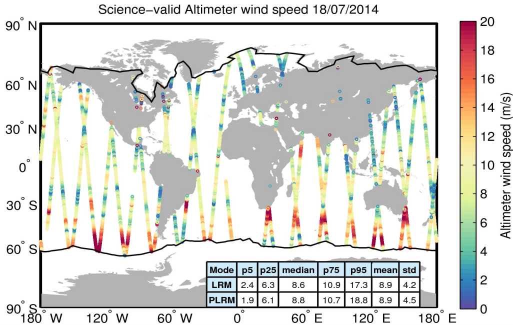
Figure 34. Geographical distribution of science-valid wind data over oceans and lakes for 18/07/2014. The statistical values shown in the table refer to the wind in m/s and are calculated separately for LRM and PLRM regions. The black lines mark the outer limit of the Arctic and Antarctic polar polygons. Gray circles denote records that have been rejected based on the editing criteria described in Table 5.
