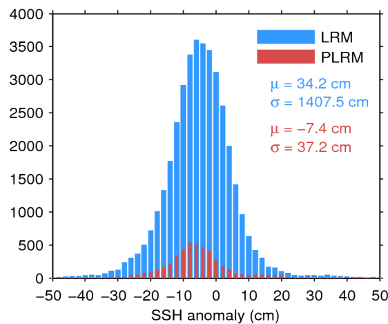
Figure 7. Histogram of flag-valid SSH anomaly over oceans and lakes for LRM (blue) and PLRM (red) for 18/07/2014. The mean ( \mu ) and standard deviation ( \sigma ) are also shown. Note that values outside [-50 \ 50] cm are excluded from the histogram for the sake of readability but not from the computation of \mu and \sigma .
