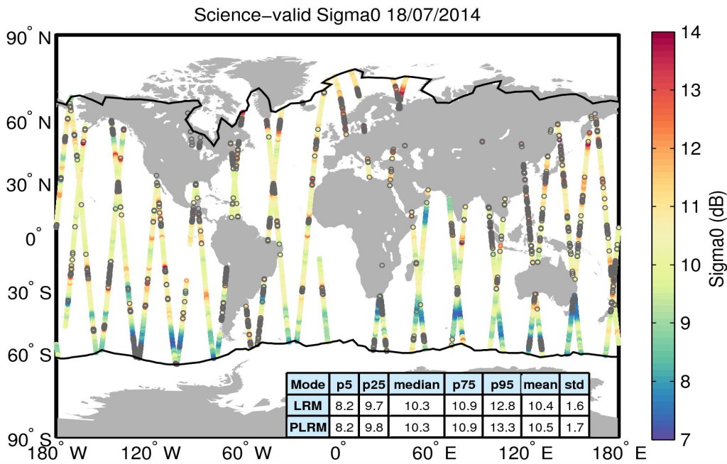
Figure 27. Geographical distribution of science-valid sigma0 data over oceans and lakes for 18/07/2014. The statistical values shown in the table refer to the sigma0 in dB and are calculated separately for LRM and PLRM regions. The black lines mark the outer limit of the Arctic and Antarctic polar polygons. Gray circles denote records that have been rejected based on the editing criteria described in Table 4.
