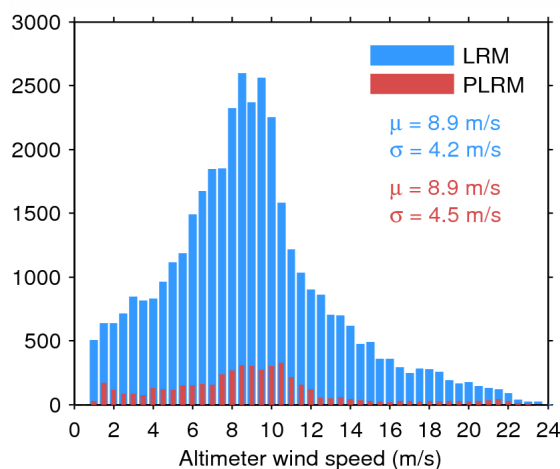
Figure 33. Histogram of flag-valid wind over oceans and lakes for LRM (blue) and PLRM (red) for 18/07/2014. The mean ( \mu ) and standard deviation ( \sigma ) are also shown. Note that values larger than 24 m/s are excluded from the histogram for the sake of readability but not from the computation of \mu and \sigma .
