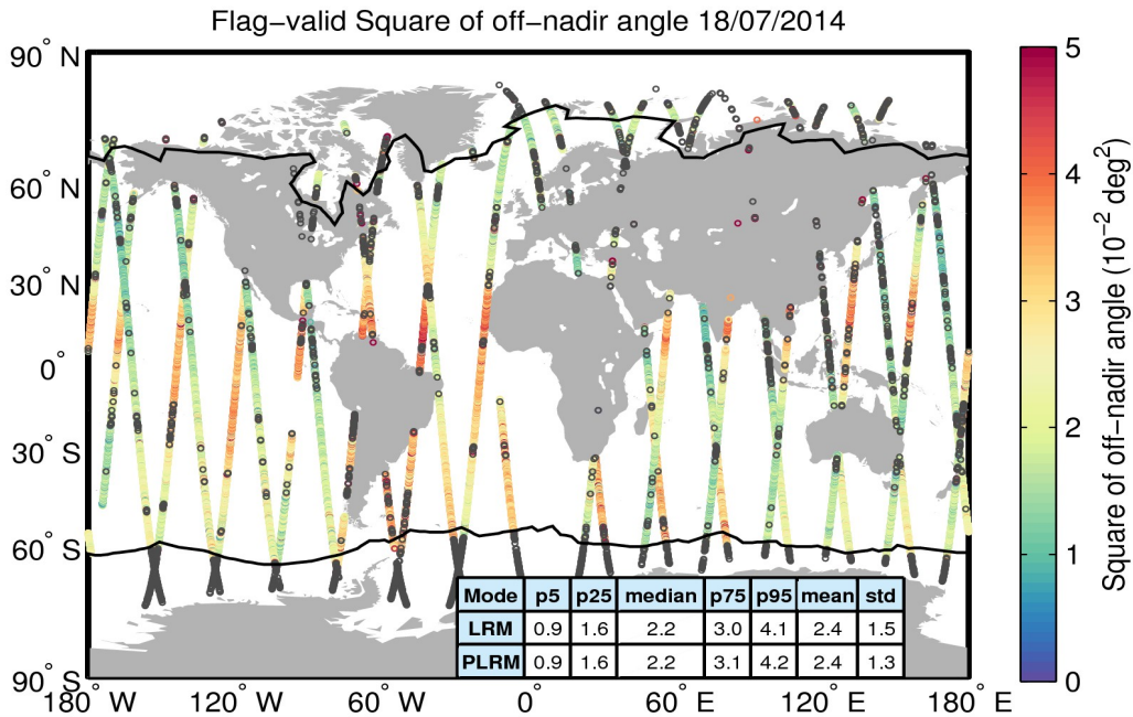
Figure 37. Geographical distribution of flag-valid mispointing data over oceans and lakes for 18/07/2014. The statistical values shown in the table refer to the mispointing in 10^{-2} \text{ deg}^2 and are calculated separately for LRM and PLRM regions. Measurements taken over polar polygons have been excluded from the computation of the statistical values. The black lines mark the outer limit of the Arctic and Antarctic polar polygons. Gray circles denote negative values.
