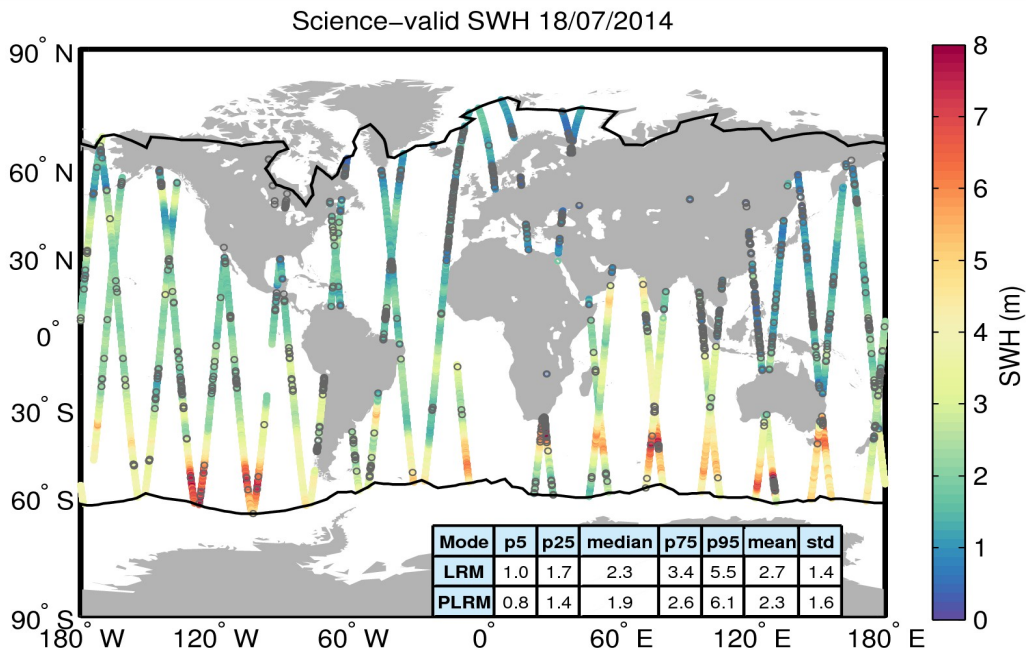
Figure 19. Geographical distribution of science-valid SWH data over oceans and lakes for 18/07/2014. The statistical values shown in the table refer to the SWH in m and are calculated separately for LRM and PLRM regions. The black lines mark the outer limit of the Arctic and Antarctic polar polygons. Gray circles denote records that have been rejected based on the editing criteria described in Table 3.
