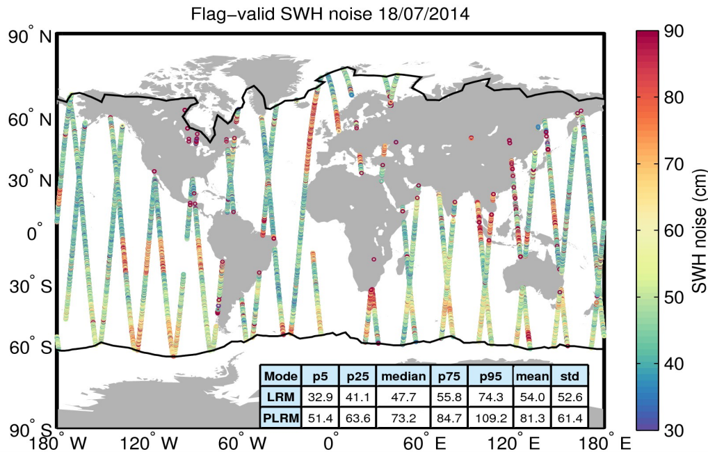
Figure 18. Geographical distribution of flag-valid 20-Hz SWH measurement noise over oceans and lakes for 18/07/2014. The statistical values shown in the table refer to the SWH noise and are calculated separately for LRM and PLRM regions. Measurements taken over polar polygons have been excluded from the computation of the statistical values. The black lines mark the outer limit of the Arctic and Antarctic polar polygons.
