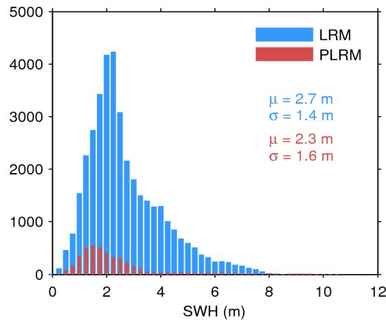
Figure 20. Histogram of science-valid SWH over oceans and lakes for LRM (blue) and PLRM (red) for 18/07/2014. The mean ( \mu ) and standard deviation ( \sigma ) are also shown. Note that values larger than 12 m are excluded from the histogram for the sake of readability but not from the computation of \mu and \sigma .
