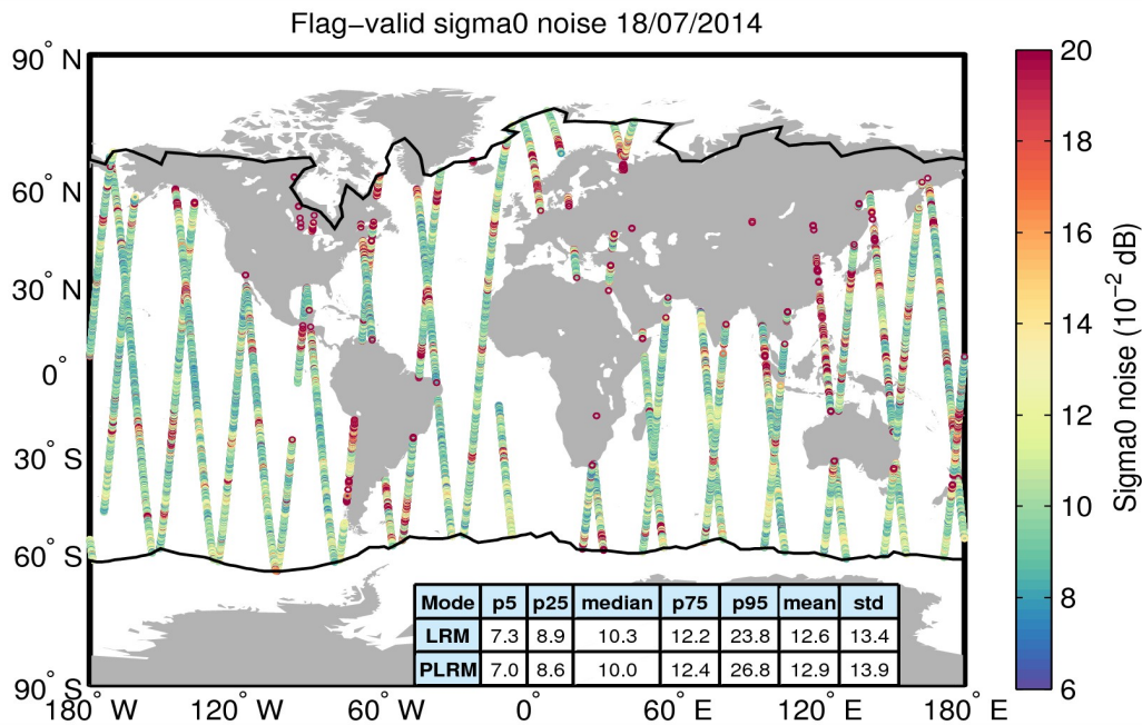
Figure 26. Geographical distribution of flag-valid 20-Hz sigma0 measurement noise over oceans and lakes for 18/07/2014. The statistical values shown in the table refer to the sigma0 noise and are calculated separately for LRM and PLRM regions. Measurements taken over polar polygons have been excluded from the computation of the statistical values. The black lines mark the outer limit of the Arctic and Antarctic polar polygons.
