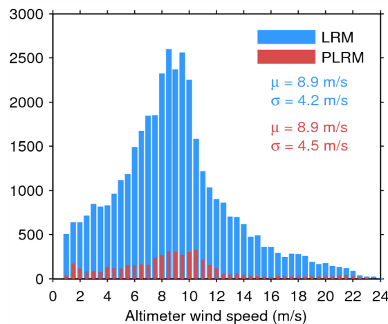
Figure 35. Histogram of science-valid wind over oceans and lakes for LRM (blue) and PLRM (red) for 18/07/2014. The mean ( \mu ) and standard deviation ( \sigma ) are also shown. Note that values larger than 24 m/s are excluded from the histogram for the sake of readability but not from the computation of \mu and \sigma .
