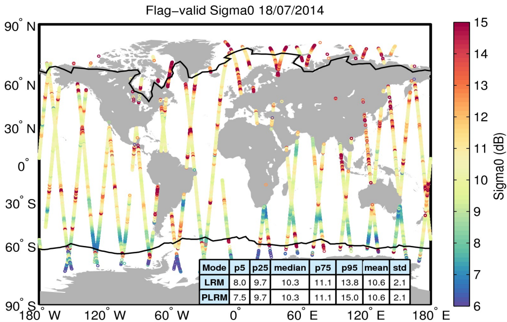
Figure 23. Geographical distribution of flag-valid sigma0 data over oceans and lakes for 18/07/2014. The statistical values shown in the table refer to the sigma0 in dB and are calculated separately for LRM and PLRM regions. Measurements taken over polar polygons have been excluded from the computation of the statistical values. The black lines mark the outer limit of the Arctic and Antarctic polar polygons.
