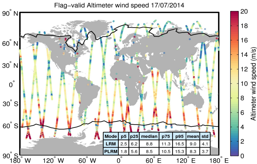
Figure 31. Geographical distribution of flag-valid wind data over oceans and lakes for 17/07/2014. The statistical values shown in the table refer to the wind in m/s and are calculated separately for LRM and PLRM regions. Measurements taken over polar polygons have been excluded from the computation of the statistical values. The black lines mark the outer limit of the Arctic and Antarctic polar polygons.
