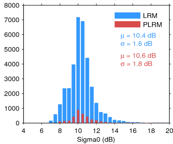
Figure 28. Histogram of science-valid sigma0 over oceans and lakes for LRM (blue) and PLRM (red) for 17/07/2014. The mean ( \mu ) and standard deviation ( \sigma ) are also shown. Note that values outside [4 20] dB are excluded from the histogram for the sake of readability but not from the computation of \mu and \sigma .
