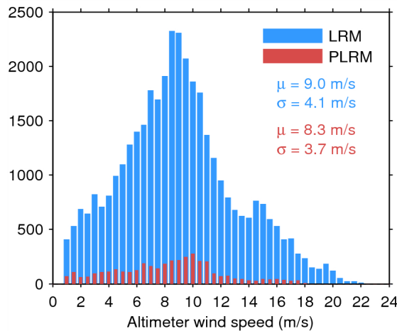
Figure 33. Histogram of flag-valid wind over oceans and lakes for LRM (blue) and PLRM (red) for 17/07/2014. The mean ( \mu ) and standard deviation ( \sigma ) are also shown. Note that values larger than 24 m/s are excluded from the histogram for the sake of readability but not from the computation of \mu and \sigma .
