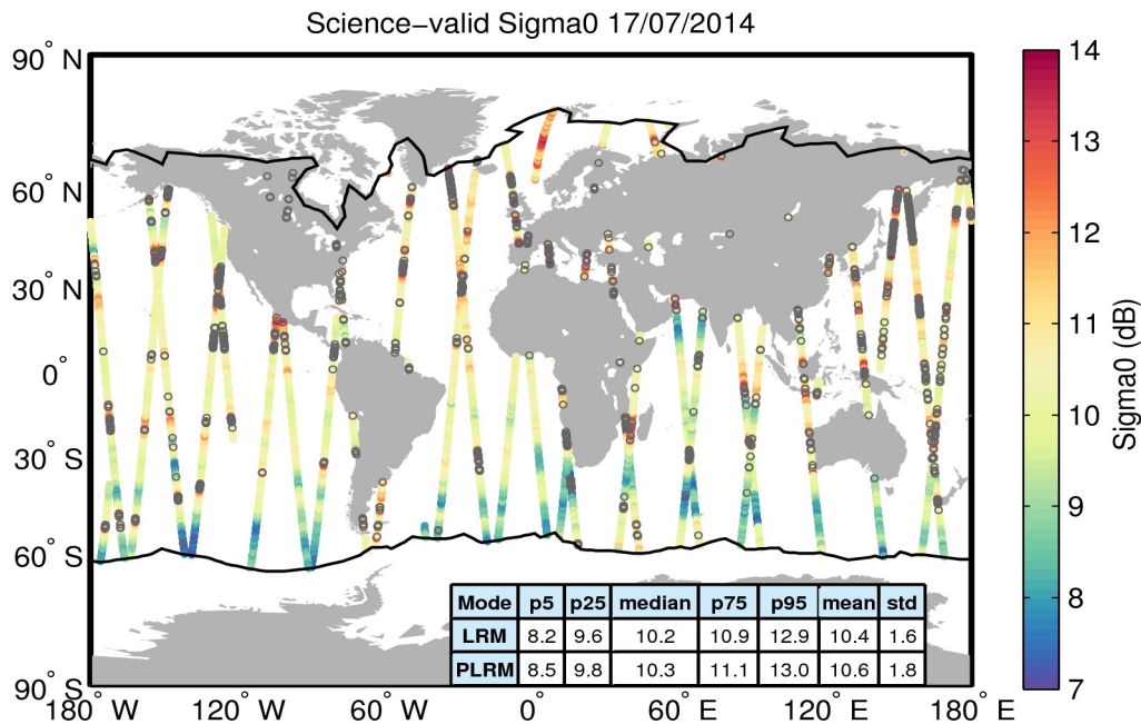
Figure 27. Geographical distribution of science-valid sigma0 data over oceans and lakes for 17/07/2014. The statistical values shown in the table refer to the sigma0 in dB and are calculated separately for LRM and PLRM regions. The black lines mark the outer limit of the Arctic and Antarctic polar polygons. Gray circles denote records that have been rejected based on the editing criteria described in Table 4.
