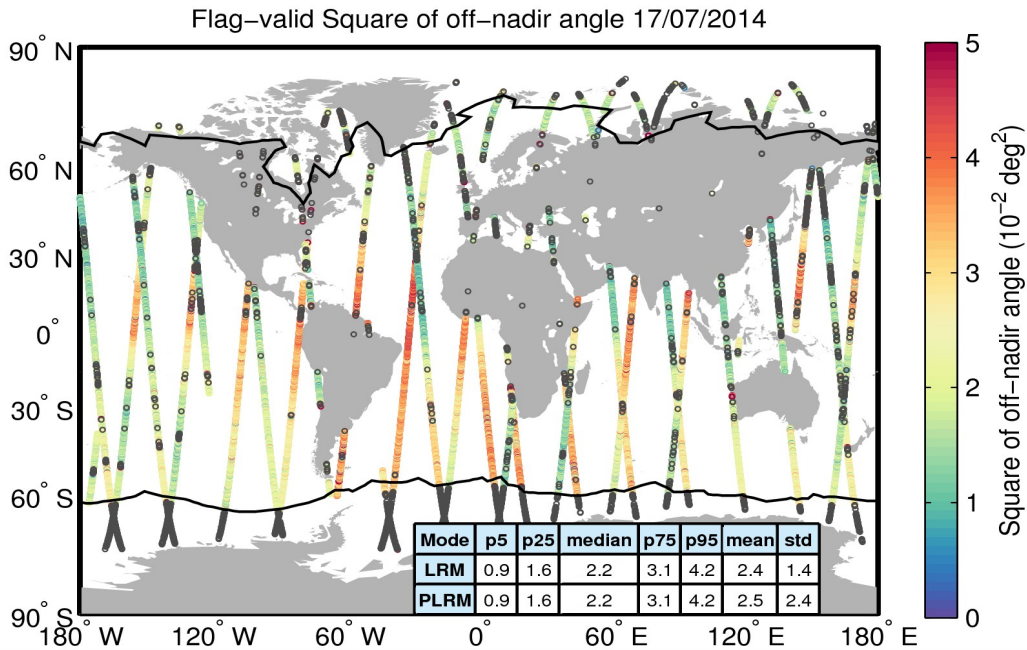
Figure 37. Geographical distribution of flag-valid mispointing data over oceans and lakes for 17/07/2014. The statistical values shown in the table refer to the mispointing in 10^{-2} deg 2 and are calculated separately for LRM and PLRM regions. Measurements taken over polar polygons have been excluded from the computation of the statistical values. The black lines mark the outer limit of the Arctic and Antarctic polar polygons. Gray circles denote negative values.
