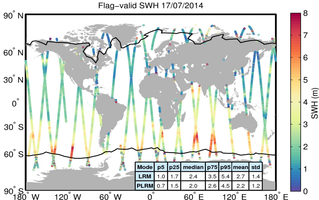
Figure 15. Geographical distribution of flag-valid SWH data over oceans and lakes for 17/07/2014. The statistical values shown in the table refer to the SWH in m and are calculated separately for LRM and PLRM regions. Measurements taken over polar polygons have been excluded from the computation of the statistical values. The black lines mark the outer limit of the Arctic and Antarctic polar polygons.
