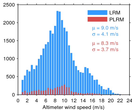
Figure 35. Histogram of science-valid wind over oceans and lakes for LRM (blue) and PLRM (red) for 17/07/2014. The mean ( \mu ) and standard deviation ( \sigma ) are also shown. Note that values larger than 24 m/s are excluded from the histogram for the sake of readability but not from the computation of \mu and \sigma .
