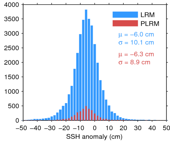
Figure 11. Histogram of science-valid SSH anomaly over oceans and lakes for LRM (blue) and PLRM (red) for 17/07/2014. The mean ( \mu ) and standard deviation ( \sigma ) are also shown. Note that values outside [-50\ 50] cm are excluded from the histogram for the sake of readability but not from the computation of \mu and \sigma .
