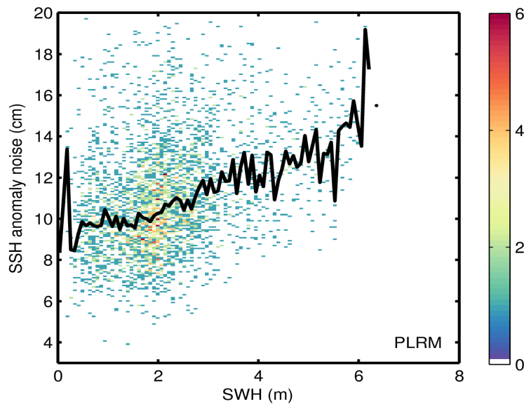
Figure 9. 2D histogram showing flag-valid SSH anomaly noise as a function of SWH for LRM (top) and PLRM (bottom) for 17/07/2014. The black line denotes the median SSH anomaly as a function of SWH.
