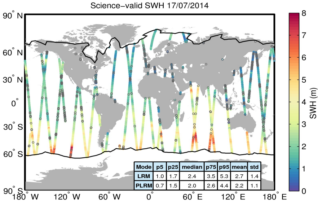
Figure 19. Geographical distribution of science-valid SWH data over oceans and lakes for 17/07/2014. The statistical values shown in the table refer to the SWH in m and are calculated separately for LRM and PLRM regions. The black lines mark the outer limit of the Arctic and Antarctic polar polygons. Gray circles denote records that have been rejected based on the editing criteria described in Table 3.
