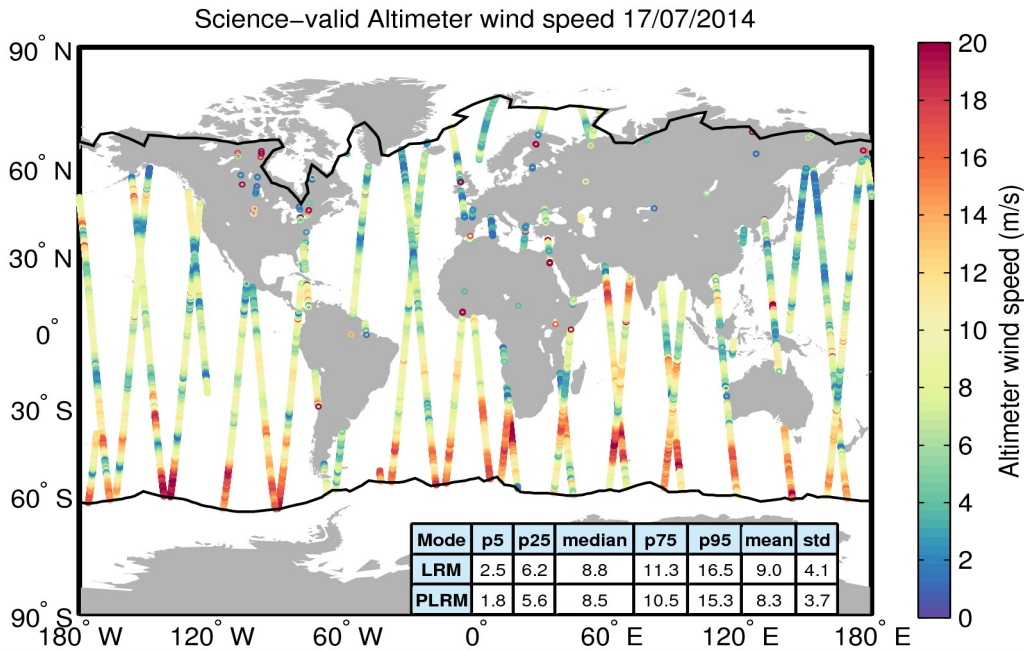
Figure 34. Geographical distribution of science-valid wind data over oceans and lakes for 17/07/2014. The statistical values shown in the table refer to the wind in m/s and are calculated separately for LRM and PLRM regions. The black lines mark the outer limit of the Arctic and Antarctic polar polygons. Gray circles denote records that have been rejected based on the editing criteria described in Table 5.
