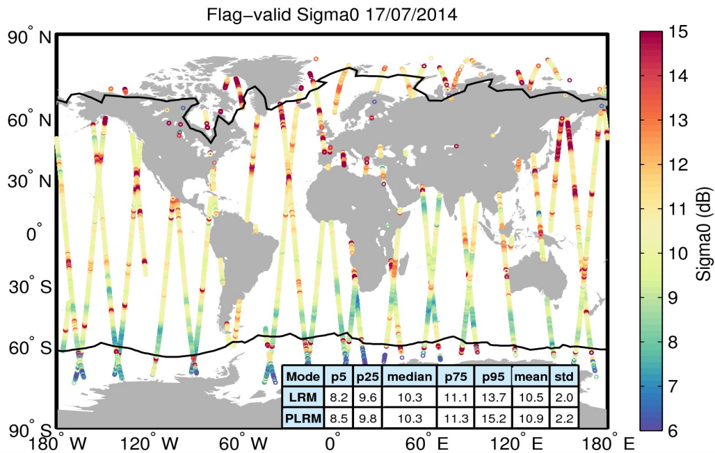
Figure 23. Geographical distribution of flag-valid sigma0 data over oceans and lakes for 17/07/2014. The statistical values shown in the table refer to the sigma0 in dB and are calculated separately for LRM and PLRM regions. Measurements taken over polar polygons have been excluded from the computation of the statistical values. The black lines mark the outer limit of the Arctic and Antarctic polar polygons.
