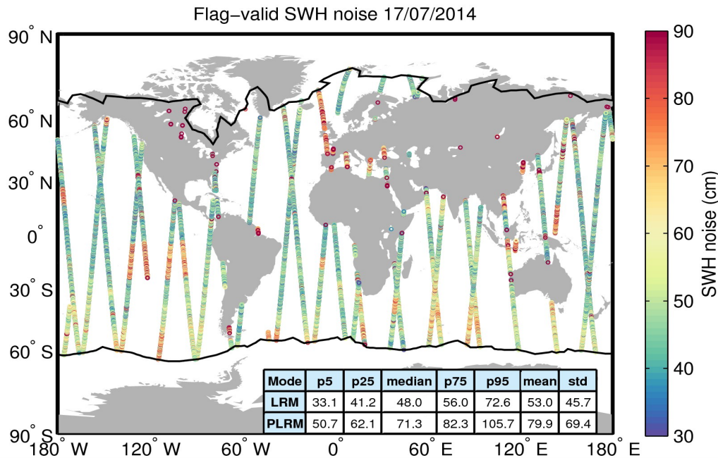
Figure 18. Geographical distribution of flag-valid 20-Hz SWH measurement noise over oceans and lakes for 17/07/2014. The statistical values shown in the table refer to the SWH noise and are calculated separately for LRM and PLRM regions. Measurements taken over polar polygons have been excluded from the computation of the statistical values. The black lines mark the outer limit of the Arctic and Antarctic polar polygons.
