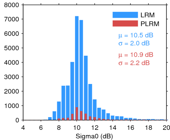
Figure 25. Histogram of flag-valid sigma0 over oceans and lakes for LRM (blue) and PLRM (red) for 17/07/2014. The mean ( \mu ) and standard deviation ( \sigma ) are also shown. Note that values outside [4 20] dB are excluded from the histogram for the sake of readability but not from the computation of \mu and \sigma .
