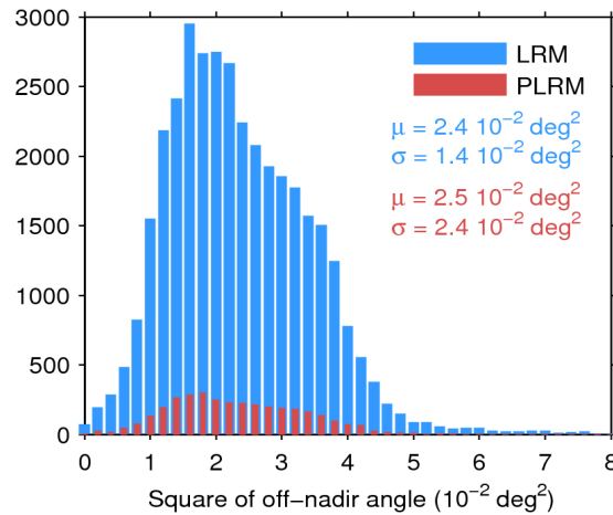
Figure 39. Histogram of flag-valid mispointing over oceans and lakes for LRM (blue) and PLRM (red) for 17/07/2014. Only positive values have been considered. The mean ( \mu ) and standard deviation ( \sigma ) are also shown. Note that values 8 \cdot 10^{-2} \text{ deg}^2 are excluded from the histogram for the sake of readability but not from the computation of \mu and \sigma .
