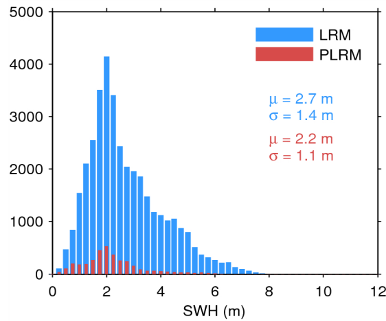
Figure 20. Histogram of science-valid SWH over oceans and lakes for LRM (blue) and PLRM (red) for 17/07/2014. The mean ( \mu ) and standard deviation ( \sigma ) are also shown. Note that values larger than 12 m are excluded from the histogram for the sake of readability but not from the computation of \mu and \sigma .
