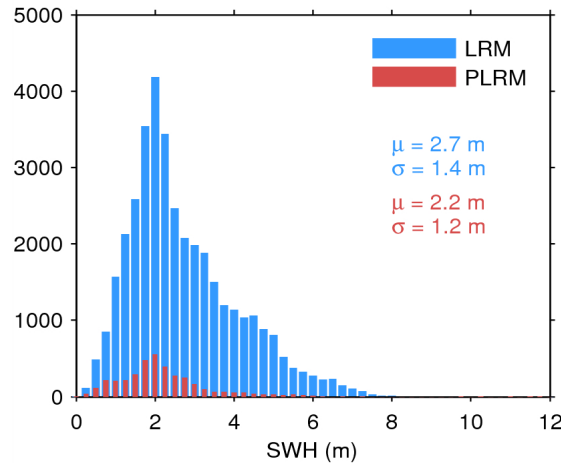
Figure 17. Histogram of flag-valid SWH over oceans and lakes for LRM (blue) and PLRM (red) for 17/07/2014. The mean ( \mu ) and standard deviation ( \sigma ) are also shown. Note that values larger than 12 m are excluded from the histogram for the sake of readability but not from the computation of \mu and \sigma .
