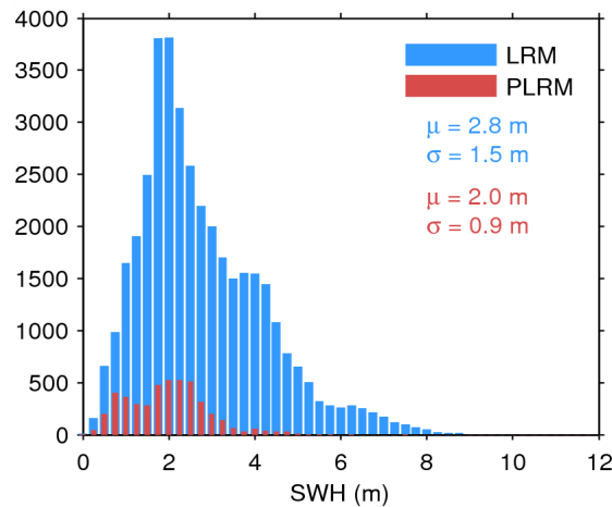
Figure 20. Histogram of science-valid SWH over oceans and lakes for LRM (blue) and PLRM (red) for 16/07/2014. The mean ( \mu ) and standard deviation ( \sigma ) are also shown. Note that values larger than 12 m are excluded from the histogram for the sake of readability but not from the computation of \mu and \sigma .
