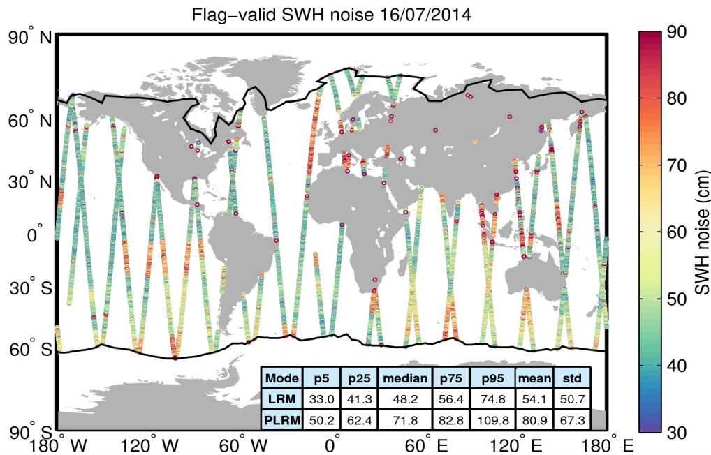
Figure 18. Geographical distribution of flag-valid 20-Hz SWH measurement noise over oceans and lakes for 16/07/2014. The statistical values shown in the table refer to the SWH noise and are calculated separately for LRM and PLRM regions. Measurements taken over polar polygons have been excluded from the computation of the statistical values. The black lines mark the outer limit of the Arctic and Antarctic polar polygons.
