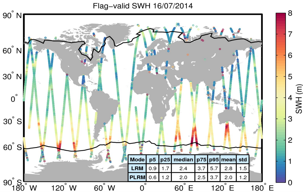
Figure 15. Geographical distribution of flag-valid SWH data over oceans and lakes for 16/07/2014. The statistical values shown in the table refer to the SWH in m and are calculated separately for LRM and PLRM regions. Measurements taken over polar polygons have been excluded from the computation of the statistical values. The black lines mark the outer limit of the Arctic and Antarctic polar polygons.
