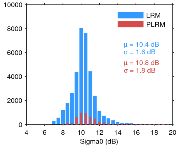
Figure 28. Histogram of science-valid sigma0 over oceans and lakes for LRM (blue) and PLRM (red) for 16/07/2014. The mean ( \mu ) and standard deviation ( \sigma ) are also shown. Note that values outside [4 20] dB are excluded from the histogram for the sake of readability but not from the computation of \mu and \sigma .
