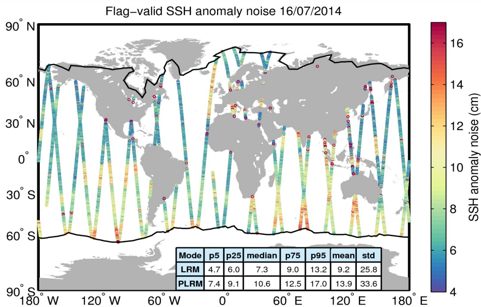
Figure 8. Geographical distribution of flag-valid 20-Hz SSH anomaly measurement noise over oceans and lakes for 16/07/2014. The statistical values shown in the table refer to the SSH anomaly noise and are calculated separately for LRM and PLRM regions. Measurements taken over polar polygons have been excluded from the computation of the statistical values. The black lines mark the outer limit of the Arctic and Antarctic polar polygons.
