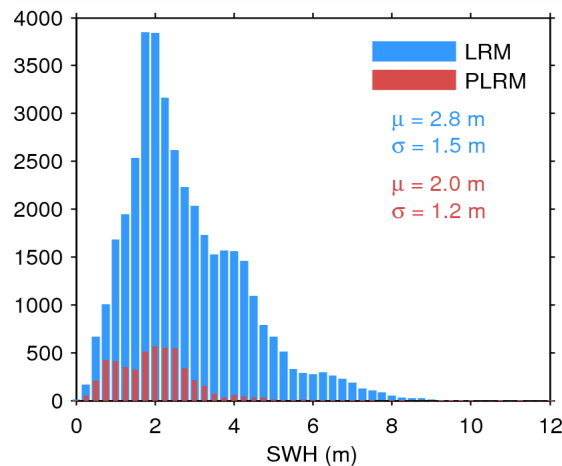
Figure 17. Histogram of flag-valid SWH over oceans and lakes for LRM (blue) and PLRM (red) for 16/07/2014. The mean ( \mu ) and standard deviation ( \sigma ) are also shown. Note that values larger than 12 m are excluded from the histogram for the sake of readability but not from the computation of \mu and \sigma .
