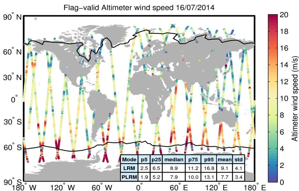
Figure 31. Geographical distribution of flag-valid wind data over oceans and lakes for 16/07/2014. The statistical values shown in the table refer to the wind in m/s and are calculated separately for LRM and PLRM regions. Measurements taken over polar polygons have been excluded from the computation of the statistical values. The black lines mark the outer limit of the Arctic and Antarctic polar polygons.
