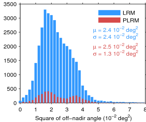
Figure 39. Histogram of flag-valid mispointing over oceans and lakes for LRM (blue) and PLRM (red) for 16/07/2014. Only positive values have been considered. The mean ( \mu ) and standard deviation ( \sigma ) are also shown. Note that values 8 \cdot 10^{-2} \text{ deg}^2 are excluded from the histogram for the sake of readability but not from the computation of \mu and \sigma .
