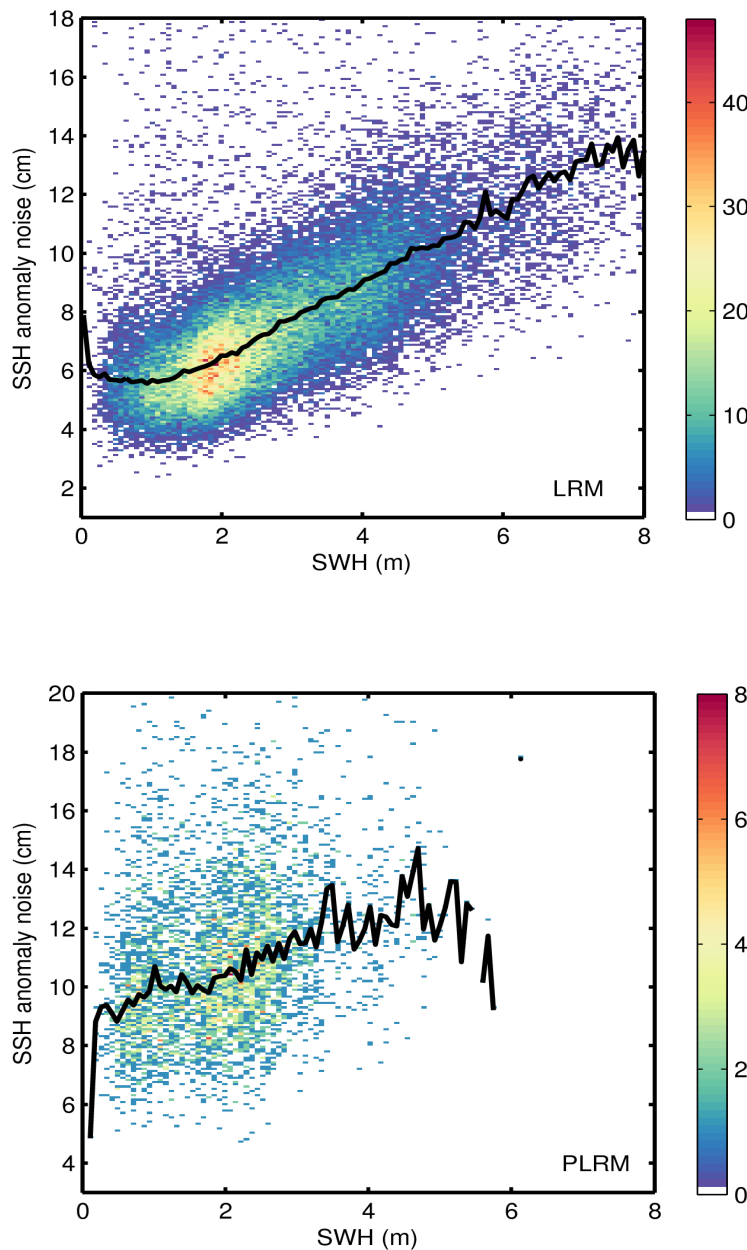
Figure 9. 2D histogram showing flag-valid SSH anomaly noise as a function of SWH for LRM (top) and PLRM (bottom) for 16/07/2014. The black line denotes the median SSH anomaly as a function of SWH.
