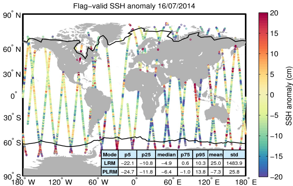
Figure 5. Geographical distribution of flag-valid 1-Hz SSH anomaly data over oceans and lakes for 16/07/2014. The statistical values shown in the table refer to the SSH anomaly in cm and are calculated separately for LRM and PLRM regions. Measurements taken over polar polygons have been excluded from the computation of the statistical values. The black lines mark the outer limit of the Arctic and Antarctic polar polygons.
