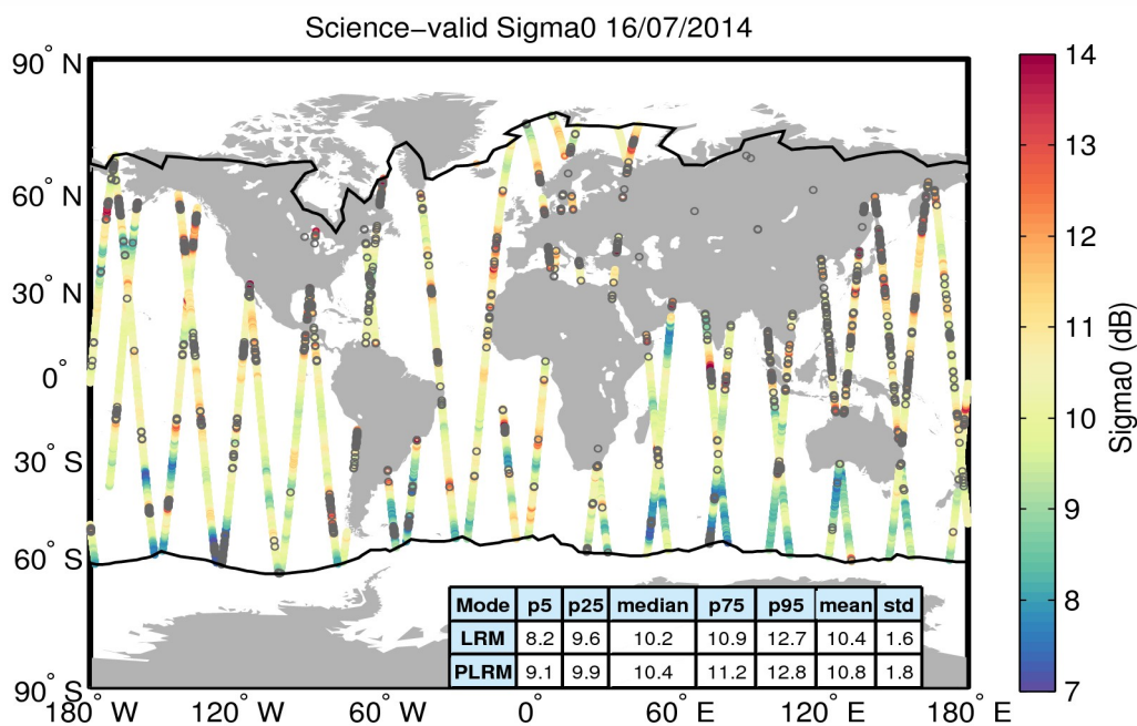
Figure 27. Geographical distribution of science-valid sigma0 data over oceans and lakes for 16/07/2014. The statistical values shown in the table refer to the sigma0 in dB and are calculated separately for LRM and PLRM regions. The black lines mark the outer limit of the Arctic and Antarctic polar polygons. Gray circles denote records that have been rejected based on the editing criteria described in Table 4.
