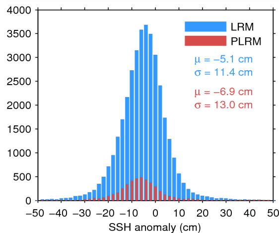
Figure 11. Histogram of science-valid SSH anomaly over oceans and lakes for LRM (blue) and PLRM (red) for 16/07/2014. The mean ( \mu ) and standard deviation ( \sigma ) are also shown. Note that values outside [-50 50] cm are excluded from the histogram for the sake of readability but not from the computation of \mu and \sigma .
