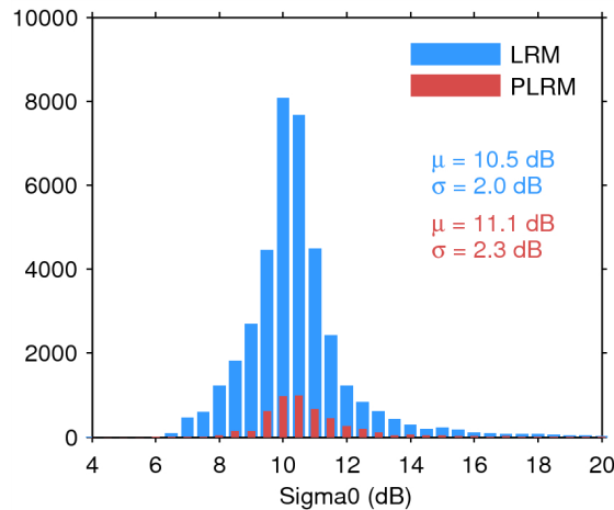
Figure 25. Histogram of flag-valid sigma0 over oceans and lakes for LRM (blue) and PLRM (red) for 16/07/2014. The mean ( \mu ) and standard deviation ( \sigma ) are also shown. Note that values outside [4 20] dB are excluded from the histogram for the sake of readability but not from the computation of \mu and \sigma .
