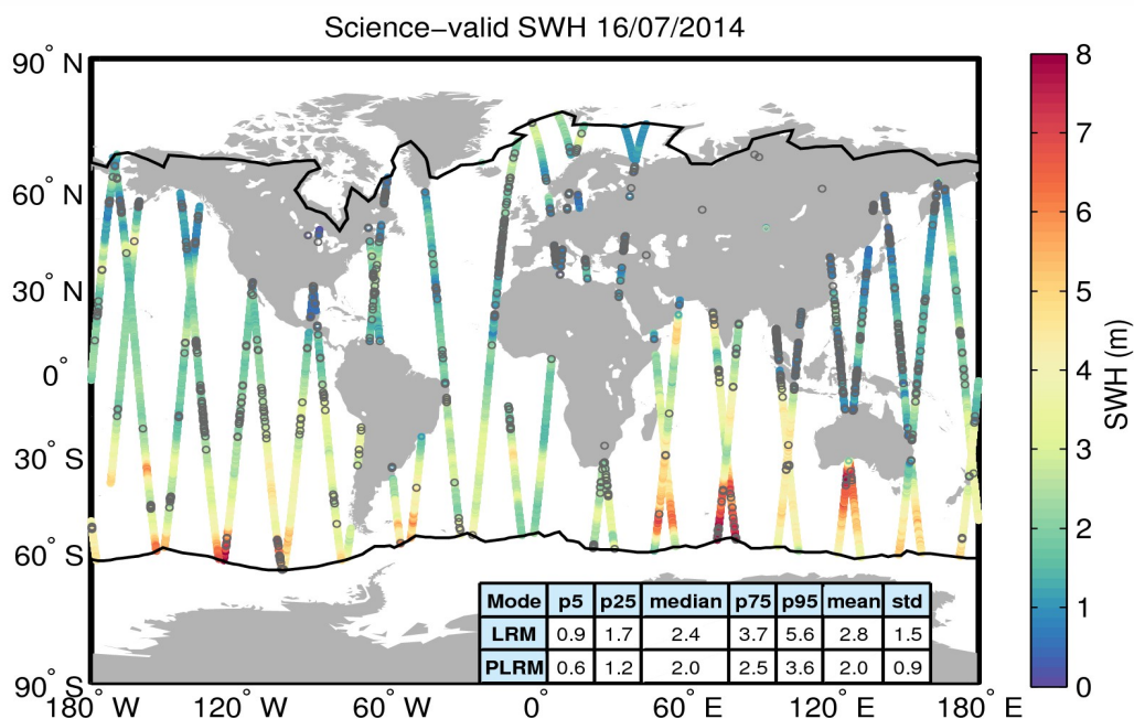
Figure 19. Geographical distribution of science-valid SWH data over oceans and lakes for 16/07/2014. The statistical values shown in the table refer to the SWH in m and are calculated separately for LRM and PLRM regions. The black lines mark the outer limit of the Arctic and Antarctic polar polygons. Gray circles denote records that have been rejected based on the editing criteria described in Table 3.
