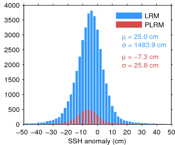
Figure 7. Histogram of flag-valid SSH anomaly over oceans and lakes for LRM (blue) and PLRM (red) for 16/07/2014. The mean ( \mu ) and standard deviation ( \sigma ) are also shown. Note that values outside [-50\ 50] cm are excluded from the histogram for the sake of readability but not from the computation of \mu and \sigma .
