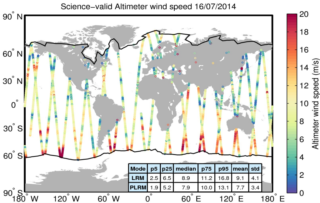
Figure 34. Geographical distribution of science-valid wind data over oceans and lakes for 16/07/2014. The statistical values shown in the table refer to the wind in m/s and are calculated separately for LRM and PLRM regions. The black lines mark the outer limit of the Arctic and Antarctic polar polygons. Gray circles denote records that have been rejected based on the editing criteria described in Table 5.
