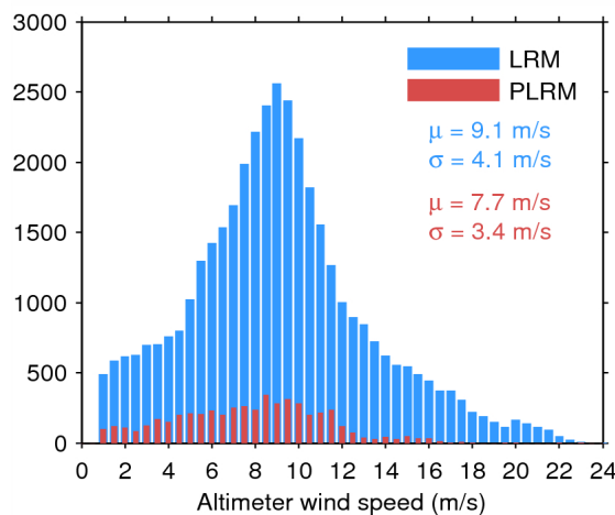
Figure 35. Histogram of science-valid wind over oceans and lakes for LRM (blue) and PLRM (red) for 16/07/2014. The mean ( \mu ) and standard deviation ( \sigma ) are also shown. Note that values larger than 24 m/s are excluded from the histogram for the sake of readability but not from the computation of \mu and \sigma .
