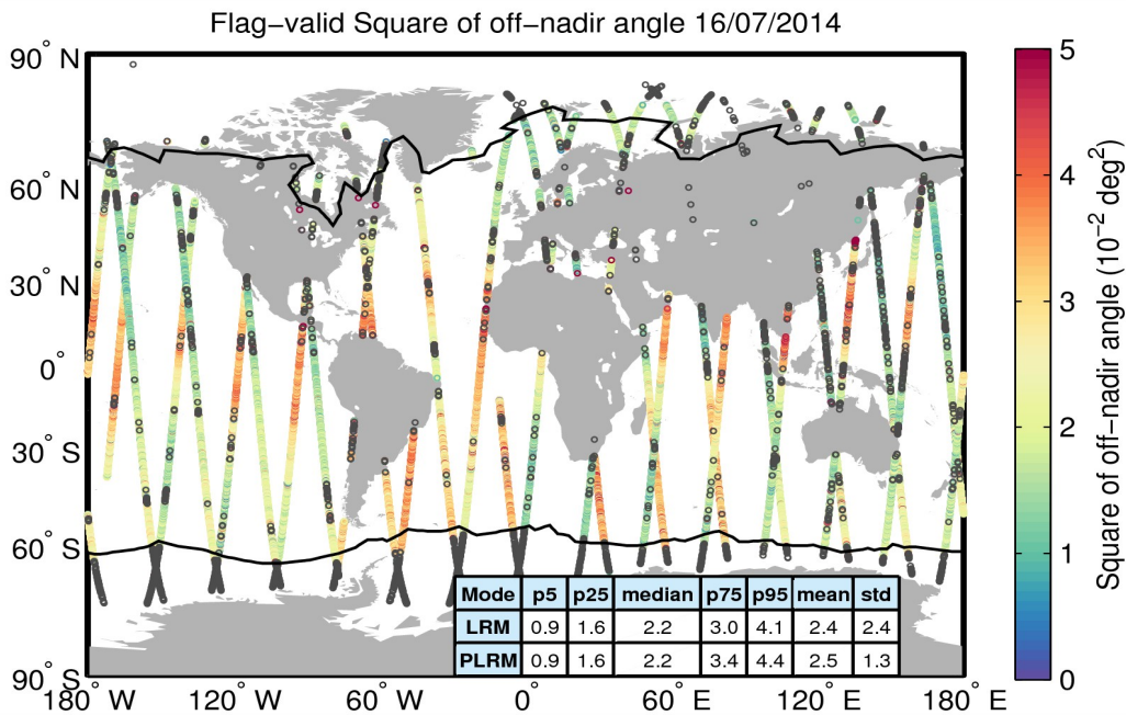
Figure 37. Geographical distribution of flag-valid mispointing data over oceans and lakes for 16/07/2014. The statistical values shown in the table refer to the mispointing in 10^{-2} \text{ deg}^2 and are calculated separately for LRM and PLRM regions. Measurements taken over polar polygons have been excluded from the computation of the statistical values. The black lines mark the outer limit of the Arctic and Antarctic polar polygons. Gray circles denote negative values.
