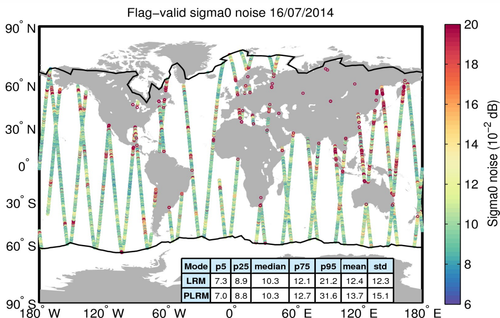
Figure 26. Geographical distribution of flag-valid 20-Hz sigma0 measurement noise over oceans and lakes for 16/07/2014. The statistical values shown in the table refer to the sigma0 noise and are calculated separately for LRM and PLRM regions. Measurements taken over polar polygons have been excluded from the computation of the statistical values. The black lines mark the outer limit of the Arctic and Antarctic polar polygons.
