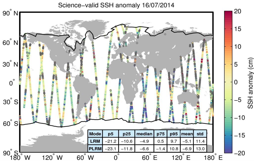
Figure 10. Geographical distribution of science-valid SSH anomaly data over oceans and lakes for 16/07/2014. The statistical values shown in the table refer to the SSH anomaly in cm and are calculated separately for LRM and PLRM regions. The black lines mark the outer limit of the Arctic and Antarctic polar polygons. Gray circles denote records that have been rejected based on the editing criteria described in Table 2.
