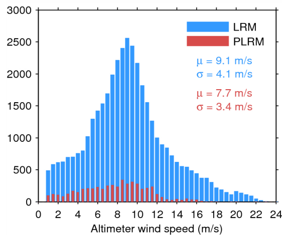
Figure 33. Histogram of flag-valid wind over oceans and lakes for LRM (blue) and PLRM (red) for 16/07/2014. The mean ( \mu ) and standard deviation ( \sigma ) are also shown. Note that values larger than 24 m/s are excluded from the histogram for the sake of readability but not from the computation of \mu and \sigma .
