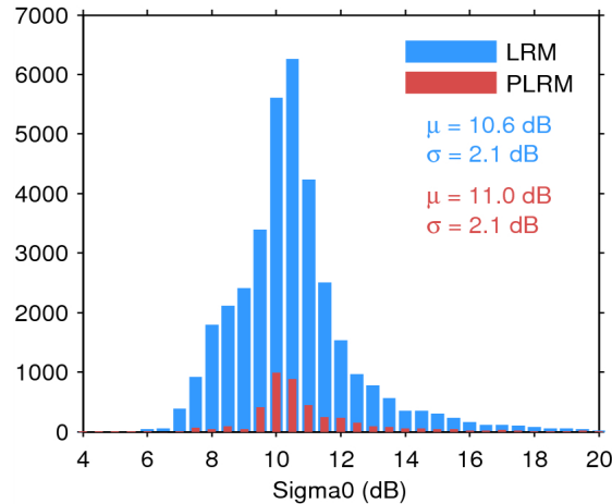
Figure 25. Histogram of flag-valid sigma0 over oceans and lakes for LRM (blue) and PLRM (red) for 13/07/2014. The mean ( \mu ) and standard deviation ( \sigma ) are also shown. Note that values outside [4 20] dB are excluded from the histogram for the sake of readability but not from the computation of \mu and \sigma .
