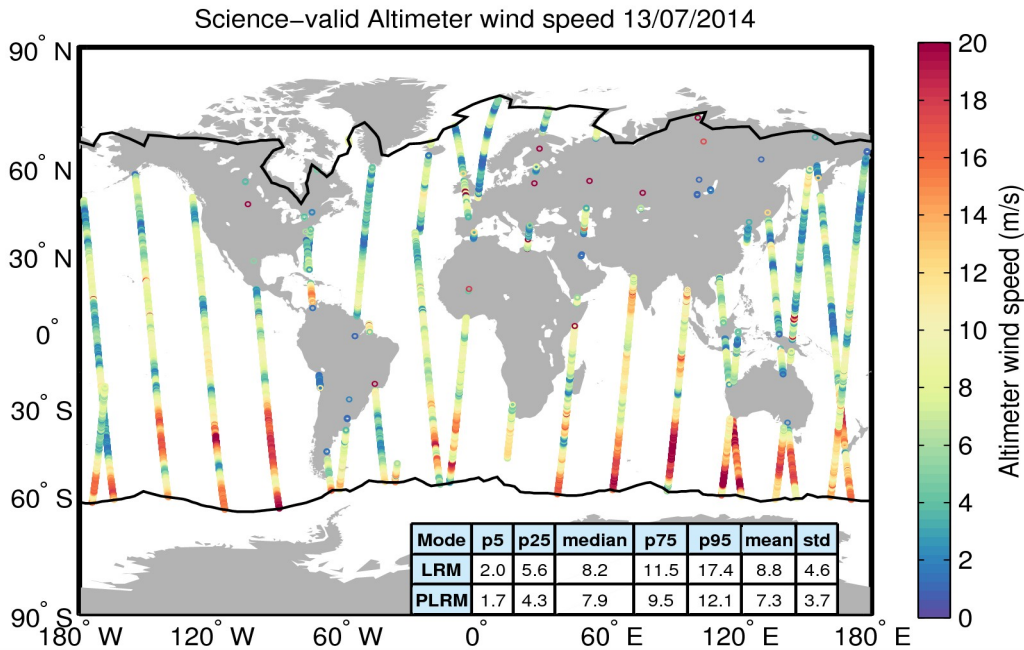
Figure 34. Geographical distribution of science-valid wind data over oceans and lakes for 13/07/2014. The statistical values shown in the table refer to the wind in m/s and are calculated separately for LRM and PLRM regions. The black lines mark the outer limit of the Arctic and Antarctic polar polygons. Gray circles denote records that have been rejected based on the editing criteria described in Table 5.
