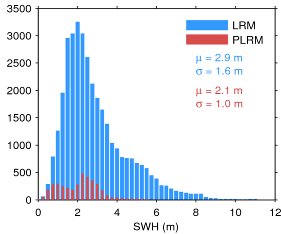
Figure 20. Histogram of science-valid SWH over oceans and lakes for LRM (blue) and PLRM (red) for 13/07/2014. The mean ( \mu ) and standard deviation ( \sigma ) are also shown. Note that values larger than 12 m are excluded from the histogram for the sake of readability but not from the computation of \mu and \sigma .
