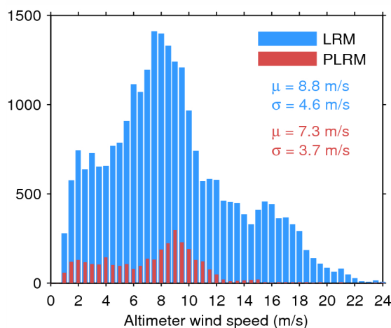
Figure 33. Histogram of flag-valid wind over oceans and lakes for LRM (blue) and PLRM (red) for 13/07/2014. The mean ( \mu ) and standard deviation ( \sigma ) are also shown. Note that values larger than 24 m/s are excluded from the histogram for the sake of readability but not from the computation of \mu and \sigma .
