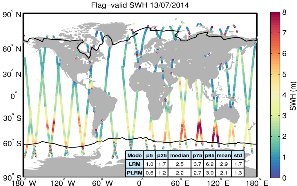
Figure 15. Geographical distribution of flag-valid SWH data over oceans and lakes for 13/07/2014. The statistical values shown in the table refer to the SWH in m and are calculated separately for LRM and PLRM regions. Measurements taken over polar polygons have been excluded from the computation of the statistical values. The black lines mark the outer limit of the Arctic and Antarctic polar polygons.
