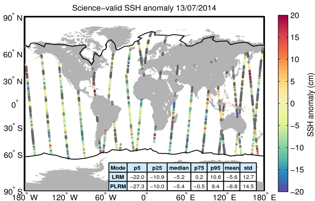
Figure 10. Geographical distribution of science-valid SSH anomaly data over oceans and lakes for 13/07/2014. The statistical values shown in the table refer to the SSH anomaly in cm and are calculated separately for LRM and PLRM regions. The black lines mark the outer limit of the Arctic and Antarctic polar polygons. Gray circles denote records that have been rejected based on the editing criteria described in Table 2.
