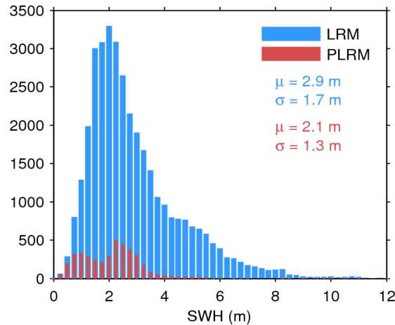
Figure 17. Histogram of flag-valid SWH over oceans and lakes for LRM (blue) and PLRM (red) for 13/07/2014. The mean ( \mu ) and standard deviation ( \sigma ) are also shown. Note that values larger than 12 m are excluded from the histogram for the sake of readability but not from the computation of \mu and \sigma .
