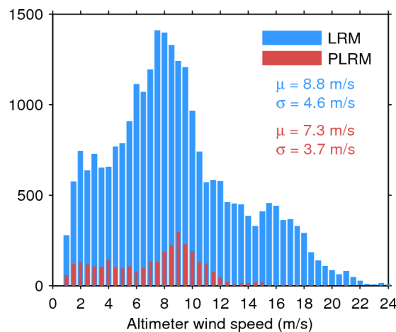
Figure 35. Histogram of science-valid wind over oceans and lakes for LRM (blue) and PLRM (red) for 13/07/2014. The mean ( \mu ) and standard deviation ( \sigma ) are also shown. Note that values larger than 24 m/s are excluded from the histogram for the sake of readability but not from the computation of \mu and \sigma .
