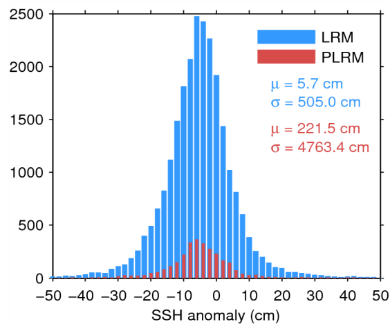
Figure 7. Histogram of flag-valid SSH anomaly over oceans and lakes for LRM (blue) and PLRM (red) for 13/07/2014. The mean ( \mu ) and standard deviation ( \sigma ) are also shown. Note that values outside [-50 \ 50] cm are excluded from the histogram for the sake of readability but not from the computation of \mu and \sigma .
