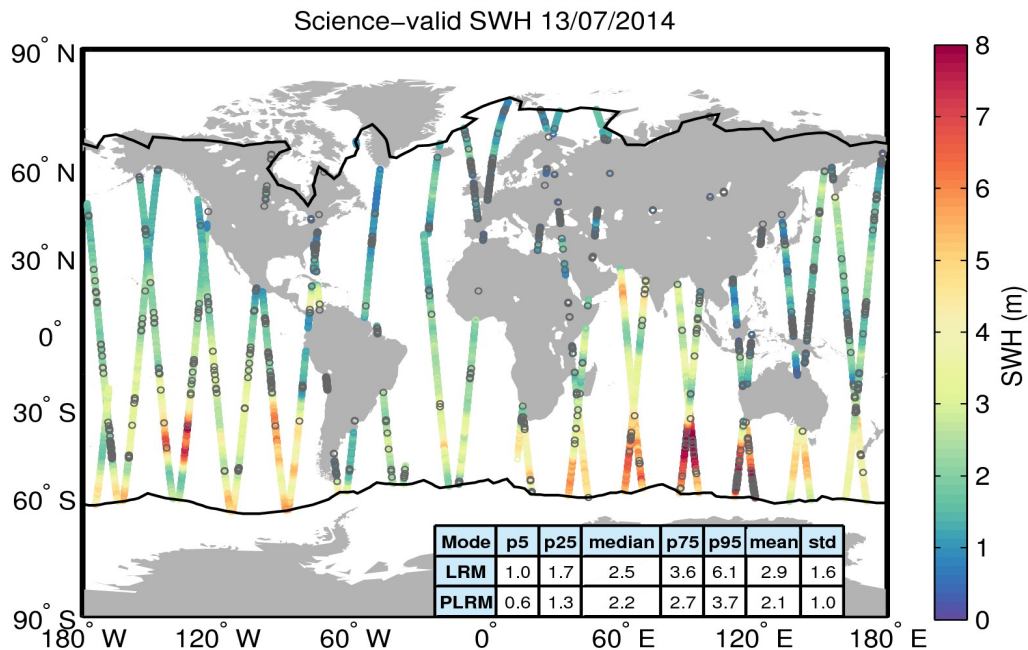
Figure 19. Geographical distribution of science-valid SWH data over oceans and lakes for 13/07/2014. The statistical values shown in the table refer to the SWH in m and are calculated separately for LRM and PLRM regions. The black lines mark the outer limit of the Arctic and Antarctic polar polygons. Gray circles denote records that have been rejected based on the editing criteria described in Table 3.
