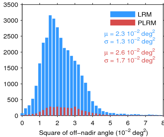
Figure 39. Histogram of flag-valid mispointing over oceans and lakes for LRM (blue) and PLRM (red) for 13/07/2014. Only positive values have been considered. The mean ( \mu ) and standard deviation ( \sigma ) are also shown. Note that values 8 \cdot 10^{-2} \text{ deg}^2 are excluded from the histogram for the sake of readability but not from the computation of \mu and \sigma .
