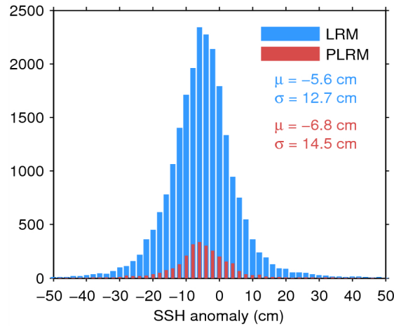
Figure 11. Histogram of science-valid SSH anomaly over oceans and lakes for LRM (blue) and PLRM (red) for 13/07/2014. The mean ( \mu ) and standard deviation ( \sigma ) are also shown. Note that values outside [-50\ 50] cm are excluded from the histogram for the sake of readability but not from the computation of \mu and \sigma .
