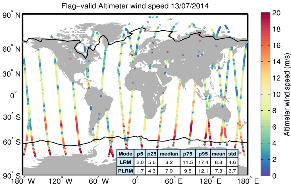
Figure 31. Geographical distribution of flag-valid wind data over oceans and lakes for 13/07/2014. The statistical values shown in the table refer to the wind in m/s and are calculated separately for LRM and PLRM regions. Measurements taken over polar polygons have been excluded from the computation of the statistical values. The black lines mark the outer limit of the Arctic and Antarctic polar polygons.
