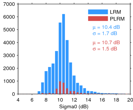
Figure 28. Histogram of science-valid sigma0 over oceans and lakes for LRM (blue) and PLRM (red) for 13/07/2014. The mean ( \mu ) and standard deviation ( \sigma ) are also shown. Note that values outside [4 20] dB are excluded from the histogram for the sake of readability but not from the computation of \mu and \sigma .
