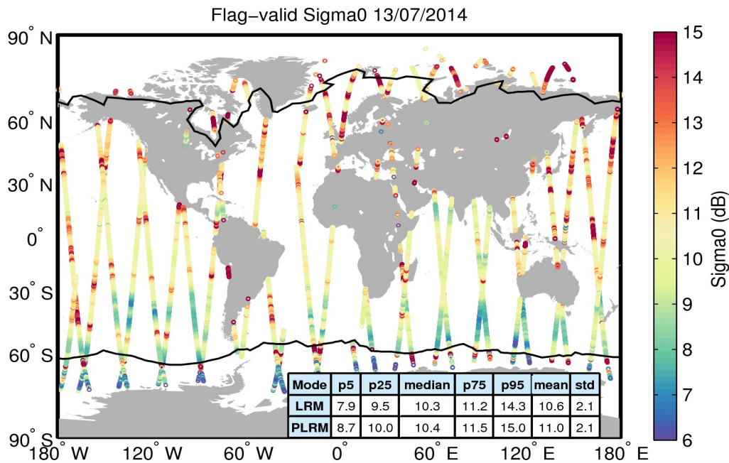
Figure 23. Geographical distribution of flag-valid sigma0 data over oceans and lakes for 13/07/2014. The statistical values shown in the table refer to the sigma0 in dB and are calculated separately for LRM and PLRM regions. Measurements taken over polar polygons have been excluded from the computation of the statistical values. The black lines mark the outer limit of the Arctic and Antarctic polar polygons.
