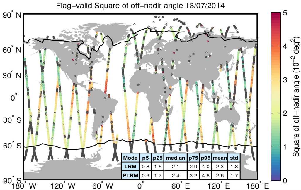
Figure 37. Geographical distribution of flag-valid mispointing data over oceans and lakes for 13/07/2014. The statistical values shown in the table refer to the mispointing in 10^{-2} \text{ deg}^2 and are calculated separately for LRM and PLRM regions. Measurements taken over polar polygons have been excluded from the computation of the statistical values. The black lines mark the outer limit of the Arctic and Antarctic polar polygons. Gray circles denote negative values.
