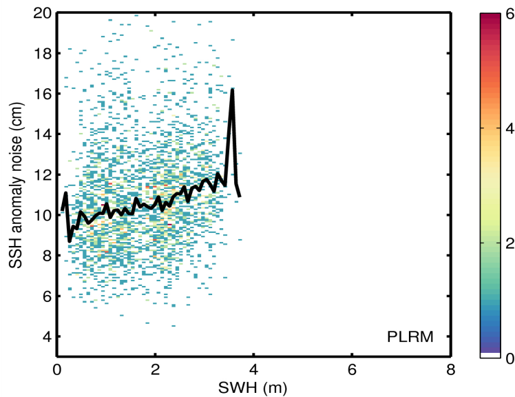
Figure 9. 2D histogram showing flag-valid SSH anomaly noise as a function of SWH for LRM (top) and PLRM (bottom) for 13/07/2014. The black line denotes the median SSH anomaly as a function of SWH.
