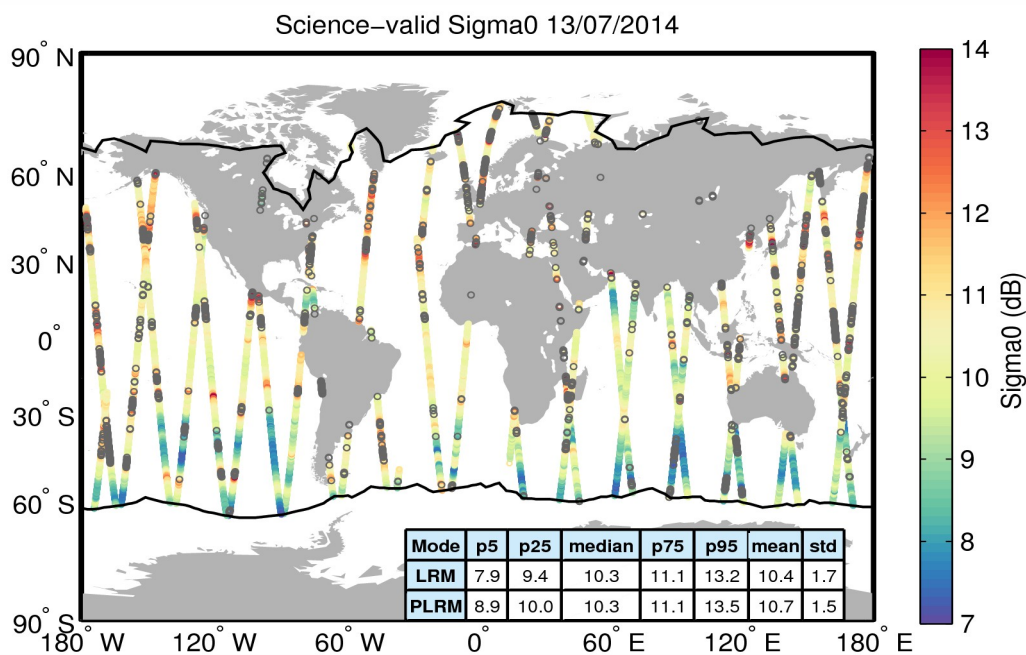
Figure 27. Geographical distribution of science-valid sigma0 data over oceans and lakes for 13/07/2014. The statistical values shown in the table refer to the sigma0 in dB and are calculated separately for LRM and PLRM regions. The black lines mark the outer limit of the Arctic and Antarctic polar polygons. Gray circles denote records that have been rejected based on the editing criteria described in Table 4.
