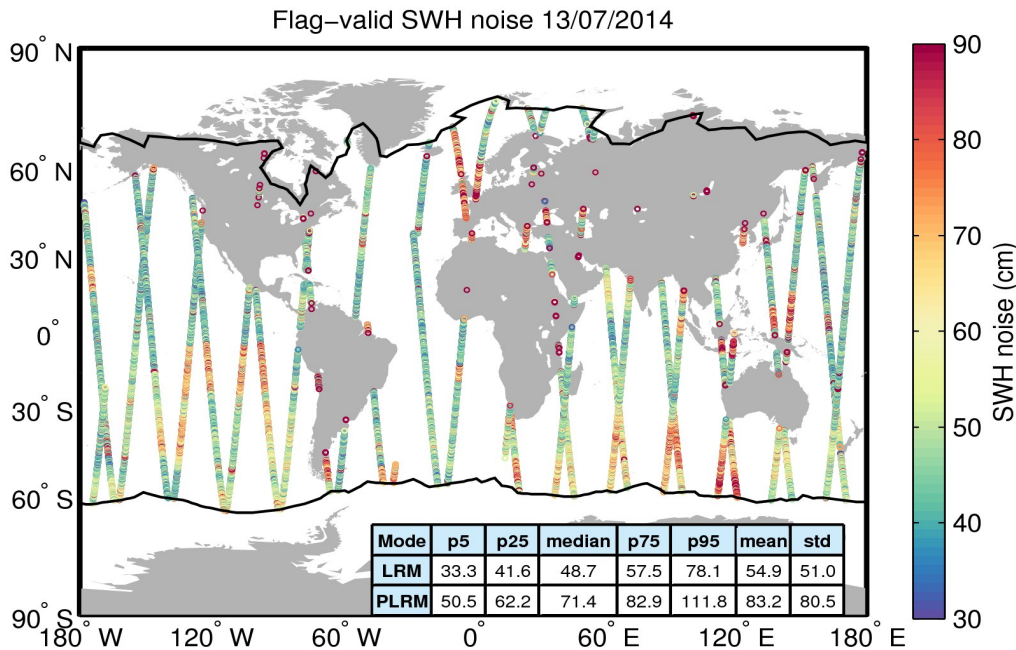
Figure 18. Geographical distribution of flag-valid 20-Hz SWH measurement noise over oceans and lakes for 13/07/2014. The statistical values shown in the table refer to the SWH noise and are calculated separately for LRM and PLRM regions. Measurements taken over polar polygons have been excluded from the computation of the statistical values. The black lines mark the outer limit of the Arctic and Antarctic polar polygons.
