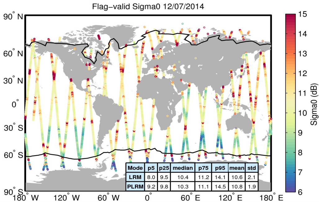
Figure 23. Geographical distribution of flag-valid sigma0 data over oceans and lakes for 12/07/2014. The statistical values shown in the table refer to the sigma0 in dB and are calculated separately for LRM and PLRM regions. Measurements taken over polar polygons have been excluded from the computation of the statistical values. The black lines mark the outer limit of the Arctic and Antarctic polar polygons.
