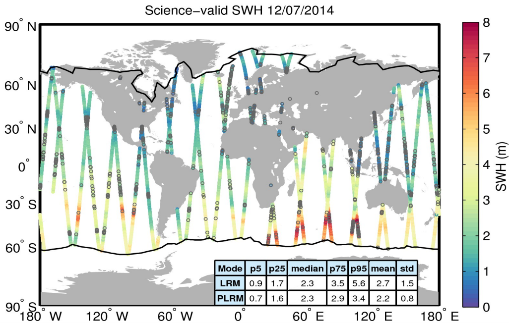
Figure 19. Geographical distribution of science-valid SWH data over oceans and lakes for 12/07/2014. The statistical values shown in the table refer to the SWH in m and are calculated separately for LRM and PLRM regions. The black lines mark the outer limit of the Arctic and Antarctic polar polygons. Gray circles denote records that have been rejected based on the editing criteria described in Table 3.
