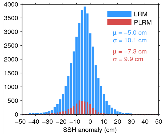
Figure 11. Histogram of science-valid SSH anomaly over oceans and lakes for LRM (blue) and PLRM (red) for 12/07/2014. The mean ( \mu ) and standard deviation ( \sigma ) are also shown. Note that values outside [-50\ 50] cm are excluded from the histogram for the sake of readability but not from the computation of \mu and \sigma .
