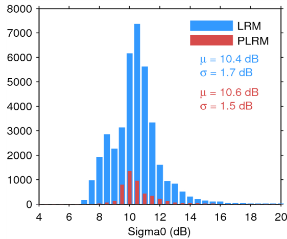
Figure 28. Histogram of science-valid sigma0 over oceans and lakes for LRM (blue) and PLRM (red) for 12/07/2014. The mean ( \mu ) and standard deviation ( \sigma ) are also shown. Note that values outside [4 20] dB are excluded from the histogram for the sake of readability but not from the computation of \mu and \sigma .
