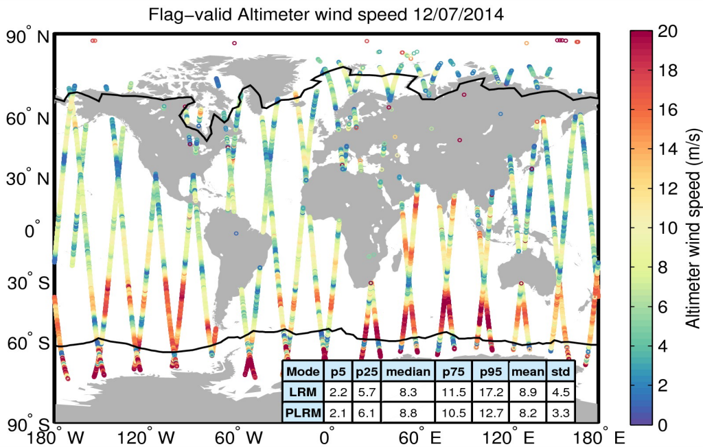
Figure 31. Geographical distribution of flag-valid wind data over oceans and lakes for 12/07/2014. The statistical values shown in the table refer to the wind in m/s and are calculated separately for LRM and PLRM regions. Measurements taken over polar polygons have been excluded from the computation of the statistical values. The black lines mark the outer limit of the Arctic and Antarctic polar polygons.
