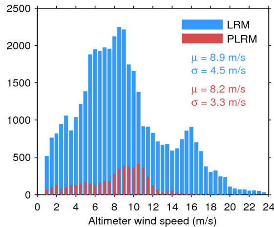
Figure 33. Histogram of flag-valid wind over oceans and lakes for LRM (blue) and PLRM (red) for 12/07/2014. The mean ( \mu ) and standard deviation ( \sigma ) are also shown. Note that values larger than 24 m/s are excluded from the histogram for the sake of readability but not from the computation of \mu and \sigma .
