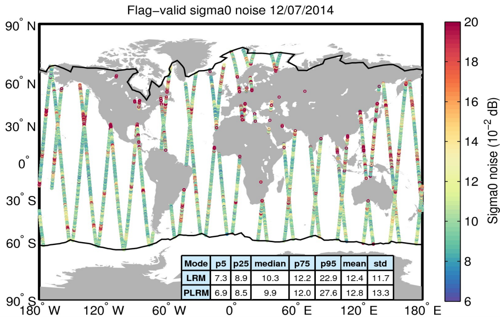
Figure 26. Geographical distribution of flag-valid 20-Hz sigma0 measurement noise over oceans and lakes for 12/07/2014. The statistical values shown in the table refer to the sigma0 noise and are calculated separately for LRM and PLRM regions. Measurements taken over polar polygons have been excluded from the computation of the statistical values. The black lines mark the outer limit of the Arctic and Antarctic polar polygons.
