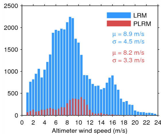
Figure 35. Histogram of science-valid wind over oceans and lakes for LRM (blue) and PLRM (red) for 12/07/2014. The mean ( \mu ) and standard deviation ( \sigma ) are also shown. Note that values larger than 24 m/s are excluded from the histogram for the sake of readability but not from the computation of \mu and \sigma .
