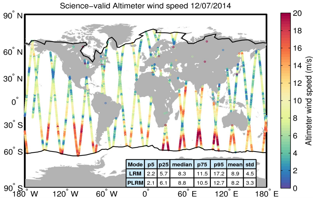
Figure 34. Geographical distribution of science-valid wind data over oceans and lakes for 12/07/2014. The statistical values shown in the table refer to the wind in m/s and are calculated separately for LRM and PLRM regions. The black lines mark the outer limit of the Arctic and Antarctic polar polygons. Gray circles denote records that have been rejected based on the editing criteria described in Table 5.
