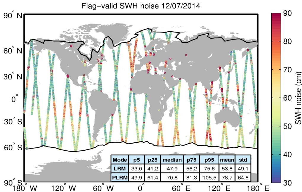
Figure 18. Geographical distribution of flag-valid 20-Hz SWH measurement noise over oceans and lakes for 12/07/2014. The statistical values shown in the table refer to the SWH noise and are calculated separately for LRM and PLRM regions. Measurements taken over polar polygons have been excluded from the computation of the statistical values. The black lines mark the outer limit of the Arctic and Antarctic polar polygons.
