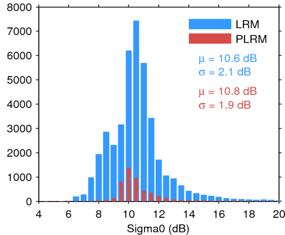
Figure 25. Histogram of flag-valid sigma0 over oceans and lakes for LRM (blue) and PLRM (red) for 12/07/2014. The mean ( \mu ) and standard deviation ( \sigma ) are also shown. Note that values outside [4 20] dB are excluded from the histogram for the sake of readability but not from the computation of \mu and \sigma .
