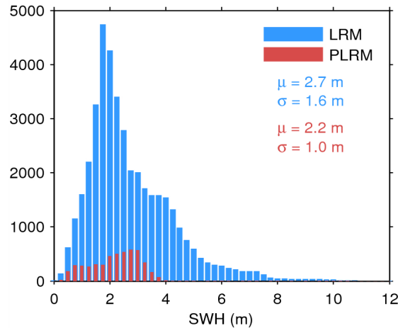
Figure 17. Histogram of flag-valid SWH over oceans and lakes for LRM (blue) and PLRM (red) for 12/07/2014. The mean ( \mu ) and standard deviation ( \sigma ) are also shown. Note that values larger than 12 m are excluded from the histogram for the sake of readability but not from the computation of \mu and \sigma .
