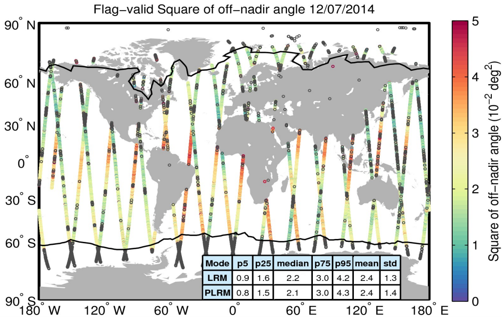
Figure 37. Geographical distribution of flag-valid mispointing data over oceans and lakes for 12/07/2014. The statistical values shown in the table refer to the mispointing in 10^{-2} deg 2 and are calculated separately for LRM and PLRM regions. Measurements taken over polar polygons have been excluded from the computation of the statistical values. The black lines mark the outer limit of the Arctic and Antarctic polar polygons. Gray circles denote negative values.
