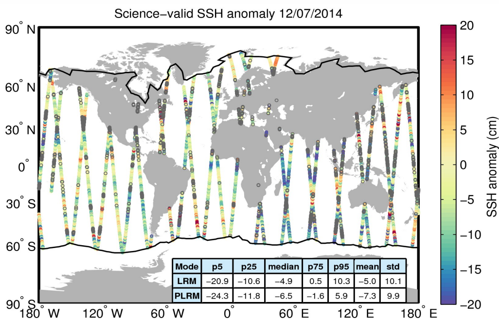
Figure 10. Geographical distribution of science-valid SSH anomaly data over oceans and lakes for 12/07/2014. The statistical values shown in the table refer to the SSH anomaly in cm and are calculated separately for LRM and PLRM regions. The black lines mark the outer limit of the Arctic and Antarctic polar polygons. Gray circles denote records that have been rejected based on the editing criteria described in Table 2.
