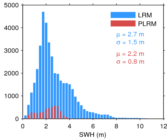
Figure 20. Histogram of science-valid SWH over oceans and lakes for LRM (blue) and PLRM (red) for 12/07/2014. The mean ( \mu ) and standard deviation ( \sigma ) are also shown. Note that values larger than 12 m are excluded from the histogram for the sake of readability but not from the computation of \mu and \sigma .
