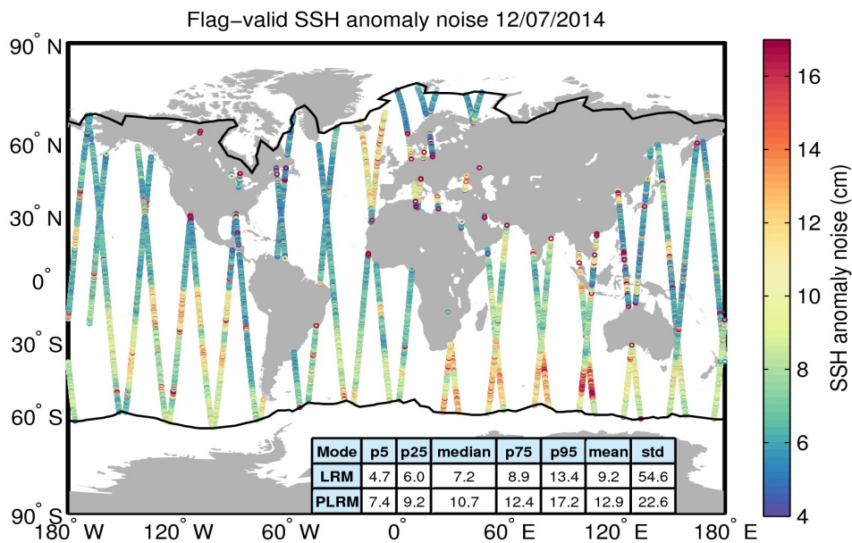
Figure 8. Geographical distribution of flag-valid 20-Hz SSH anomaly measurement noise over oceans and lakes for 12/07/2014. The statistical values shown in the table refer to the SSH anomaly noise and are calculated separately for LRM and PLRM regions. Measurements taken over polar polygons have been excluded from the computation of the statistical values. The black lines mark the outer limit of the Arctic and Antarctic polar polygons.
