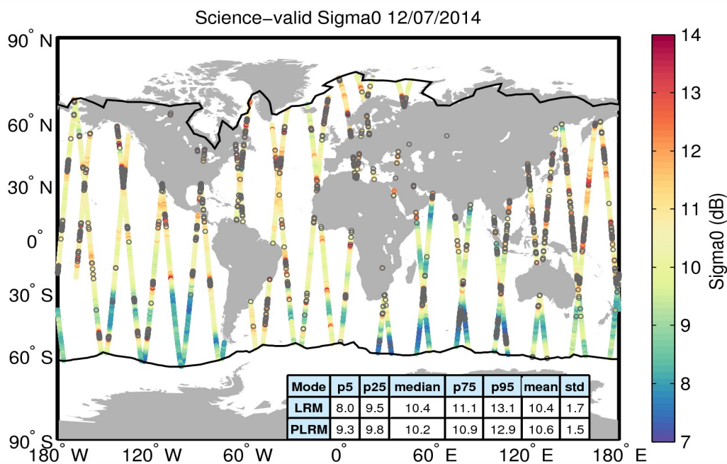
Figure 27. Geographical distribution of science-valid sigma0 data over oceans and lakes for 12/07/2014. The statistical values shown in the table refer to the sigma0 in dB and are calculated separately for LRM and PLRM regions. The black lines mark the outer limit of the Arctic and Antarctic polar polygons. Gray circles denote records that have been rejected based on the editing criteria described in Table 4.
