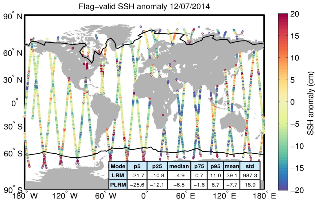
Figure 5. Geographical distribution of flag-valid 1-Hz SSH anomaly data over oceans and lakes for 12/07/2014. The statistical values shown in the table refer to the SSH anomaly in cm and are calculated separately for LRM and PLRM regions. Measurements taken over polar polygons have been excluded from the computation of the statistical values. The black lines mark the outer limit of the Arctic and Antarctic polar polygons.
