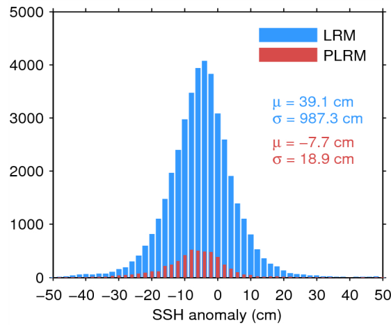
Figure 7. Histogram of flag-valid SSH anomaly over oceans and lakes for LRM (blue) and PLRM (red) for 12/07/2014. The mean ( \mu ) and standard deviation ( \sigma ) are also shown. Note that values outside [-50\ 50] cm are excluded from the histogram for the sake of readability but not from the computation of \mu and \sigma .
