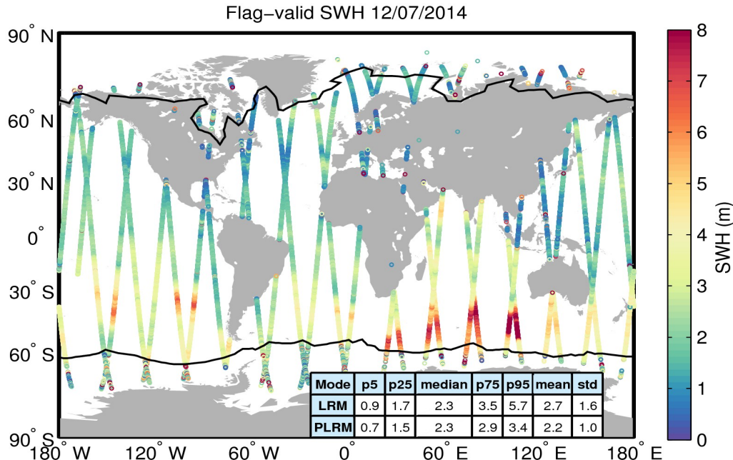
Figure 15. Geographical distribution of flag-valid SWH data over oceans and lakes for 12/07/2014. The statistical values shown in the table refer to the SWH in m and are calculated separately for LRM and PLRM regions. Measurements taken over polar polygons have been excluded from the computation of the statistical values. The black lines mark the outer limit of the Arctic and Antarctic polar polygons.
