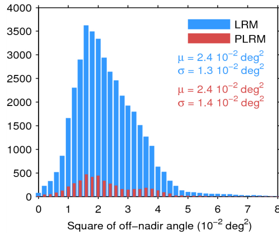
Figure 39. Histogram of flag-valid mispointing over oceans and lakes for LRM (blue) and PLRM (red) for 12/07/2014. Only positive values have been considered. The mean ( \mu ) and standard deviation ( \sigma ) are also shown. Note that values 8 \cdot 10^{-2} \text{ deg}^2 are excluded from the histogram for the sake of readability but not from the computation of \mu and \sigma .
