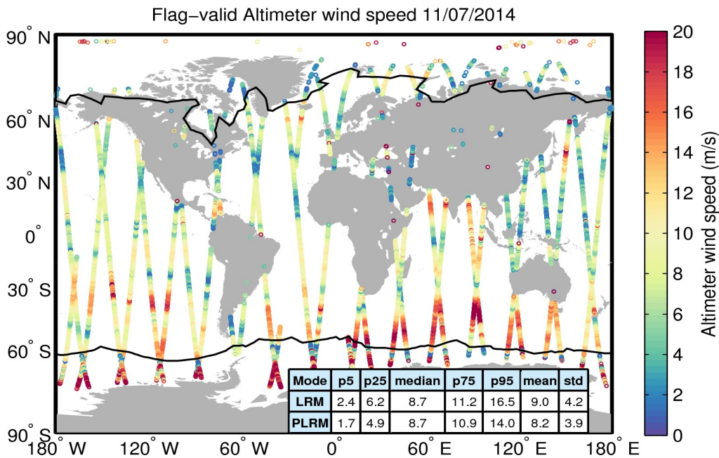
Figure 31. Geographical distribution of flag-valid wind data over oceans and lakes for 11/07/2014. The statistical values shown in the table refer to the wind in m/s and are calculated separately for LRM and PLRM regions. Measurements taken over polar polygons have been excluded from the computation of the statistical values. The black lines mark the outer limit of the Arctic and Antarctic polar polygons.
