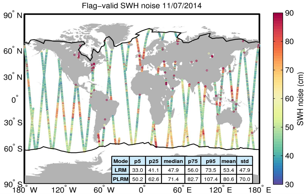
Figure 18. Geographical distribution of flag-valid 20-Hz SWH measurement noise over oceans and lakes for 11/07/2014. The statistical values shown in the table refer to the SWH noise and are calculated separately for LRM and PLRM regions. Measurements taken over polar polygons have been excluded from the computation of the statistical values. The black lines mark the outer limit of the Arctic and Antarctic polar polygons.
