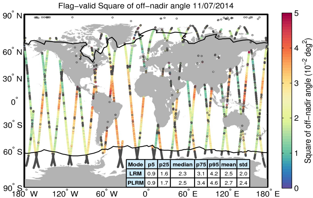
Figure 37. Geographical distribution of flag-valid mispointing data over oceans and lakes for 11/07/2014. The statistical values shown in the table refer to the mispointing in 10^{-2} deg 2 and are calculated separately for LRM and PLRM regions. Measurements taken over polar polygons have been excluded from the computation of the statistical values. The black lines mark the outer limit of the Arctic and Antarctic polar polygons. Gray circles denote negative values.
