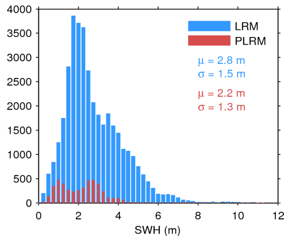
Figure 17. Histogram of flag-valid SWH over oceans and lakes for LRM (blue) and PLRM (red) for 11/07/2014. The mean ( \mu ) and standard deviation ( \sigma ) are also shown. Note that values larger than 12 m are excluded from the histogram for the sake of readability but not from the computation of \mu and \sigma .
