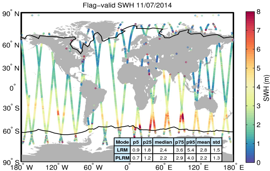
Figure 15. Geographical distribution of flag-valid SWH data over oceans and lakes for 11/07/2014. The statistical values shown in the table refer to the SWH in m and are calculated separately for LRM and PLRM regions. Measurements taken over polar polygons have been excluded from the computation of the statistical values. The black lines mark the outer limit of the Arctic and Antarctic polar polygons.
