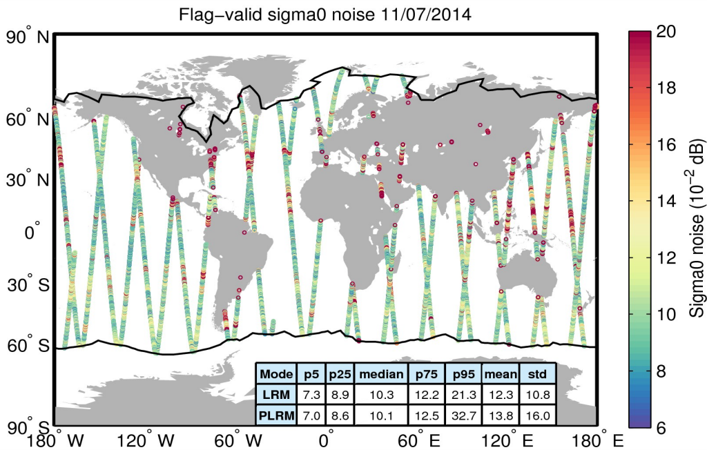
Figure 26. Geographical distribution of flag-valid 20-Hz sigma0 measurement noise over oceans and lakes for 11/07/2014. The statistical values shown in the table refer to the sigma0 noise and are calculated separately for LRM and PLRM regions. Measurements taken over polar polygons have been excluded from the computation of the statistical values. The black lines mark the outer limit of the Arctic and Antarctic polar polygons.
