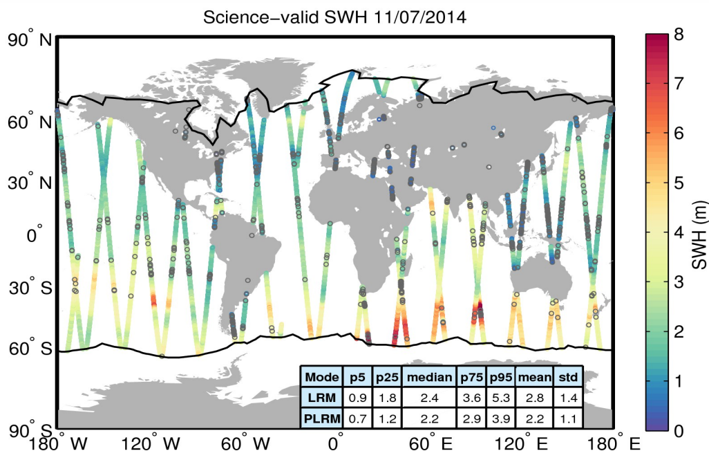
Figure 19. Geographical distribution of science-valid SWH data over oceans and lakes for 11/07/2014. The statistical values shown in the table refer to the SWH in m and are calculated separately for LRM and PLRM regions. The black lines mark the outer limit of the Arctic and Antarctic polar polygons. Gray circles denote records that have been rejected based on the editing criteria described in Table 3.
