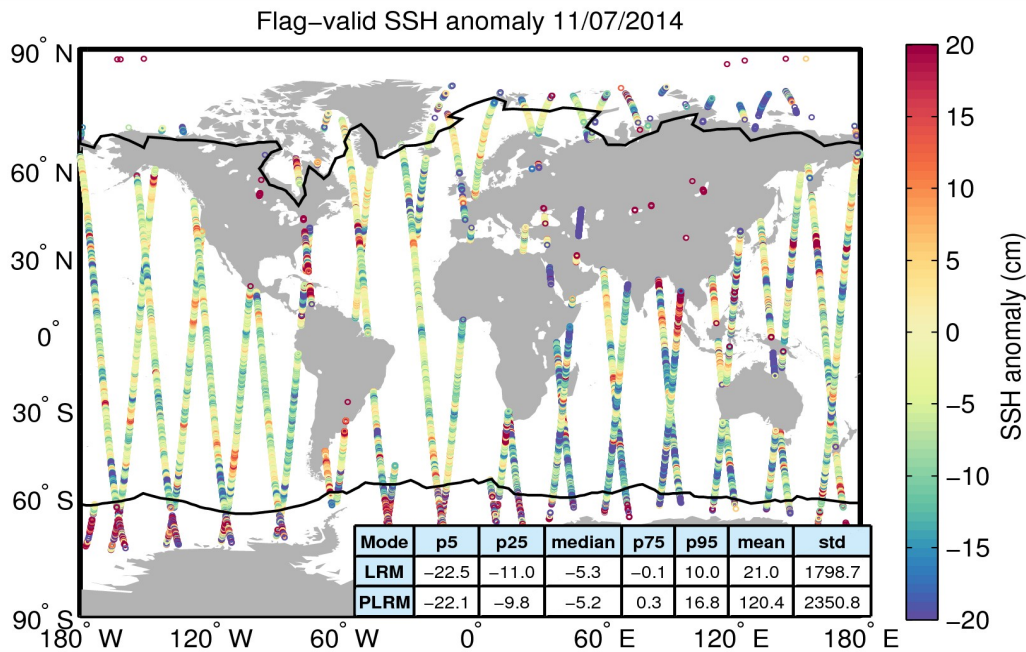
Figure 5. Geographical distribution of flag-valid 1-Hz SSH anomaly data over oceans and lakes for 11/07/2014. The statistical values shown in the table refer to the SSH anomaly in cm and are calculated separately for LRM and PLRM regions. Measurements taken over polar polygons have been excluded from the computation of the statistical values. The black lines mark the outer limit of the Arctic and Antarctic polar polygons.
