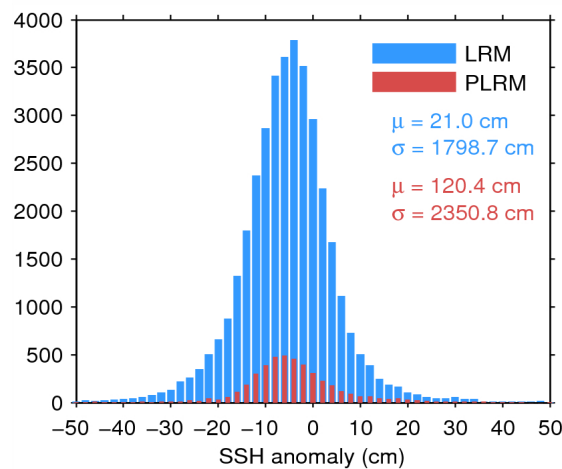
Figure 7. Histogram of flag-valid SSH anomaly over oceans and lakes for LRM (blue) and PLRM (red) for 11/07/2014. The mean ( \mu ) and standard deviation ( \sigma ) are also shown. Note that values outside [-50\ 50] cm are excluded from the histogram for the sake of readability but not from the computation of \mu and \sigma .
