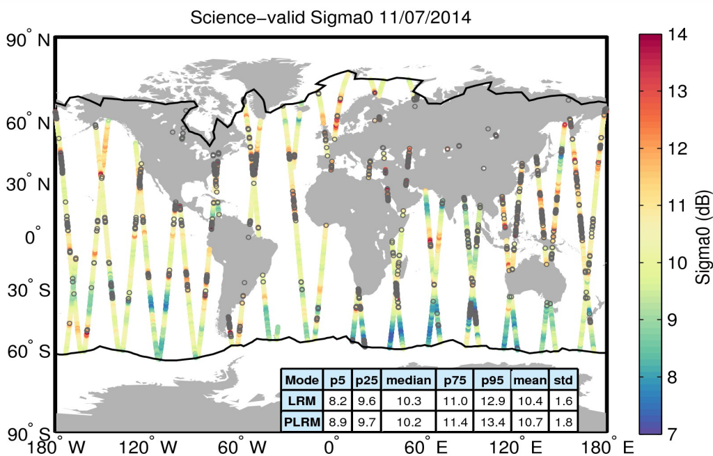
Figure 27. Geographical distribution of science-valid sigma0 data over oceans and lakes for 11/07/2014. The statistical values shown in the table refer to the sigma0 in dB and are calculated separately for LRM and PLRM regions. The black lines mark the outer limit of the Arctic and Antarctic polar polygons. Gray circles denote records that have been rejected based on the editing criteria described in Table 4.
