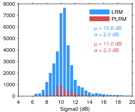
Figure 25. Histogram of flag-valid sigma0 over oceans and lakes for LRM (blue) and PLRM (red) for 11/07/2014. The mean ( \mu ) and standard deviation ( \sigma ) are also shown. Note that values outside [4 20] dB are excluded from the histogram for the sake of readability but not from the computation of \mu and \sigma .
