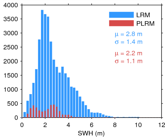
Figure 20. Histogram of science-valid SWH over oceans and lakes for LRM (blue) and PLRM (red) for 11/07/2014. The mean ( \mu ) and standard deviation ( \sigma ) are also shown. Note that values larger than 12 m are excluded from the histogram for the sake of readability but not from the computation of \mu and \sigma .
