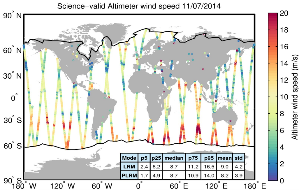
Figure 34. Geographical distribution of science-valid wind data over oceans and lakes for 11/07/2014. The statistical values shown in the table refer to the wind in m/s and are calculated separately for LRM and PLRM regions. The black lines mark the outer limit of the Arctic and Antarctic polar polygons. Gray circles denote records that have been rejected based on the editing criteria described in Table 5.
