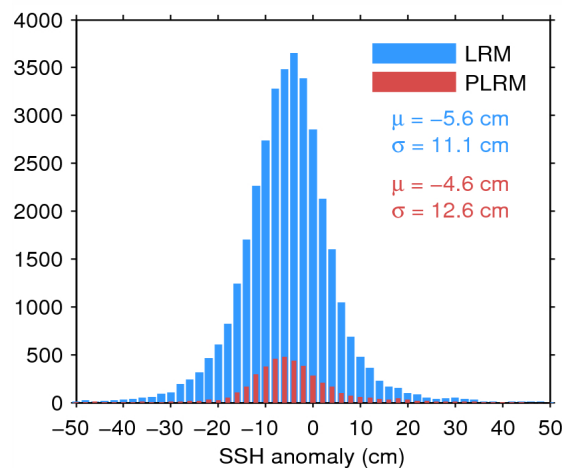
Figure 11. Histogram of science-valid SSH anomaly over oceans and lakes for LRM (blue) and PLRM (red) for 11/07/2014. The mean ( \mu ) and standard deviation ( \sigma ) are also shown. Note that values outside [-50 50] cm are excluded from the histogram for the sake of readability but not from the computation of \mu and \sigma .
