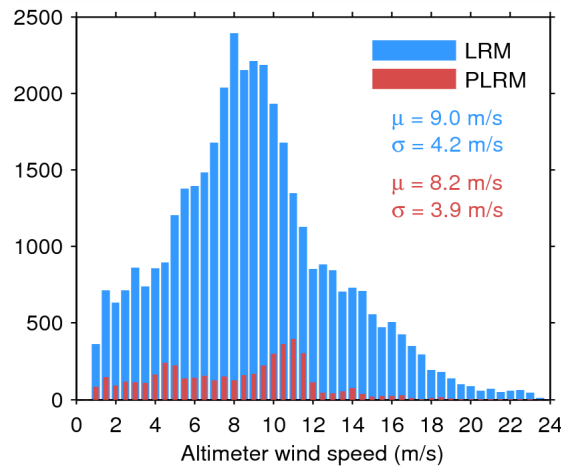
Figure 33. Histogram of flag-valid wind over oceans and lakes for LRM (blue) and PLRM (red) for 11/07/2014. The mean ( \mu ) and standard deviation ( \sigma ) are also shown. Note that values larger than 24 m/s are excluded from the histogram for the sake of readability but not from the computation of \mu and \sigma .
