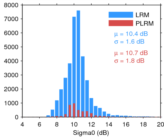
Figure 28. Histogram of science-valid sigma0 over oceans and lakes for LRM (blue) and PLRM (red) for 11/07/2014. The mean ( \mu ) and standard deviation ( \sigma ) are also shown. Note that values outside [4 20] dB are excluded from the histogram for the sake of readability but not from the computation of \mu and \sigma .
