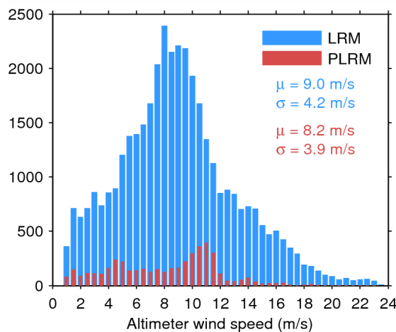
Figure 35. Histogram of science-valid wind over oceans and lakes for LRM (blue) and PLRM (red) for 11/07/2014. The mean ( \mu ) and standard deviation ( \sigma ) are also shown. Note that values larger than 24 m/s are excluded from the histogram for the sake of readability but not from the computation of \mu and \sigma .
