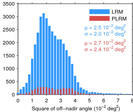
Figure 39. Histogram of flag-valid mispointing over oceans and lakes for LRM (blue) and PLRM (red) for 11/07/2014. Only positive values have been considered. The mean ( \mu ) and standard deviation ( \sigma ) are also shown. Note that values 8 \cdot 10^{-2} \text{ deg}^2 are excluded from the histogram for the sake of readability but not from the computation of \mu and \sigma .
