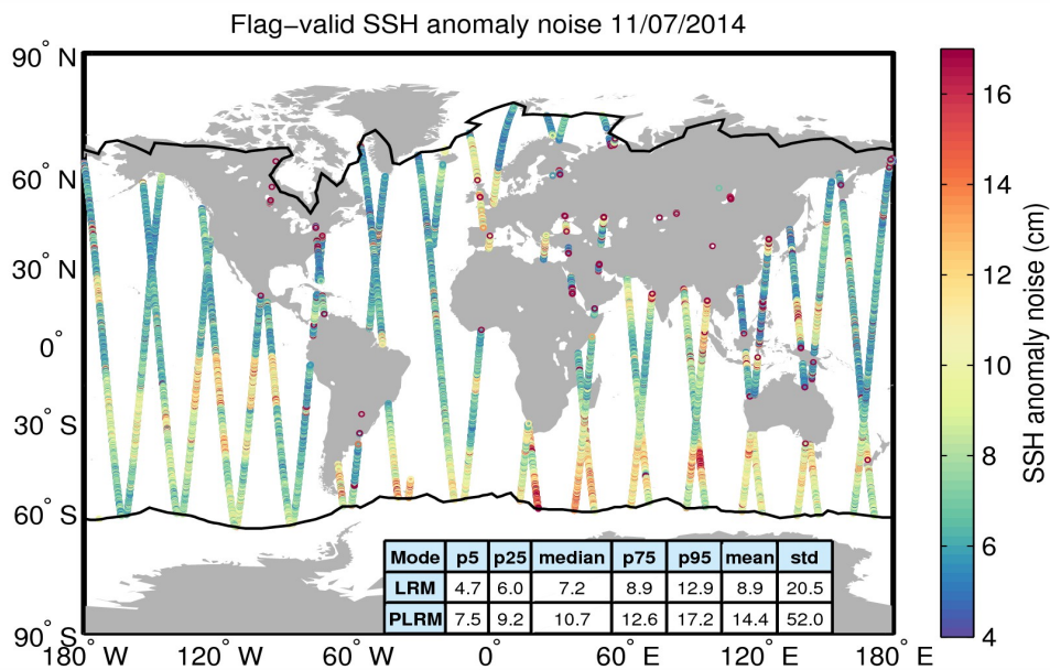
Figure 8. Geographical distribution of flag-valid 20-Hz SSH anomaly measurement noise over oceans and lakes for 11/07/2014. The statistical values shown in the table refer to the SSH anomaly noise and are calculated separately for LRM and PLRM regions. Measurements taken over polar polygons have been excluded from the computation of the statistical values. The black lines mark the outer limit of the Arctic and Antarctic polar polygons.
