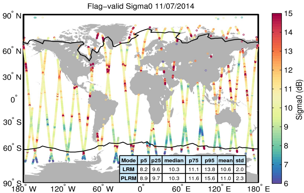
Figure 23. Geographical distribution of flag-valid sigma0 data over oceans and lakes for 11/07/2014. The statistical values shown in the table refer to the sigma0 in dB and are calculated separately for LRM and PLRM regions. Measurements taken over polar polygons have been excluded from the computation of the statistical values. The black lines mark the outer limit of the Arctic and Antarctic polar polygons.
