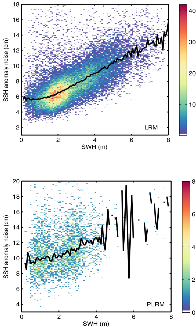
Figure 9. 2D histogram showing flag-valid SSH anomaly noise as a function of SWH for LRM (top) and PLRM (bottom) for 11/07/2014. The black line denotes the median SSH anomaly as a function of SWH.
