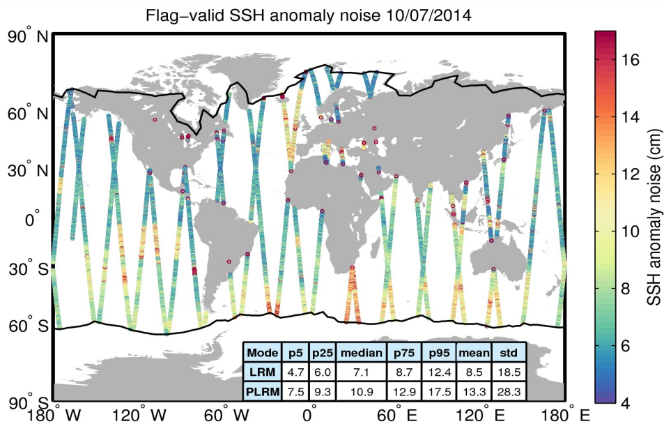
Figure 8. Geographical distribution of flag-valid 20-Hz SSH anomaly measurement noise over oceans and lakes for 10/07/2014. The statistical values shown in the table refer to the SSH anomaly noise and are calculated separately for LRM and PLRM regions. Measurements taken over polar polygons have been excluded from the computation of the statistical values. The black lines mark the outer limit of the Arctic and Antarctic polar polygons.
