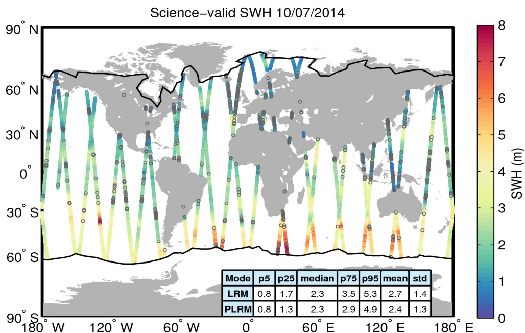
Figure 19. Geographical distribution of science-valid SWH data over oceans and lakes for 10/07/2014. The statistical values shown in the table refer to the SWH in m and are calculated separately for LRM and PLRM regions. The black lines mark the outer limit of the Arctic and Antarctic polar polygons. Gray circles denote records that have been rejected based on the editing criteria described in Table 3.
