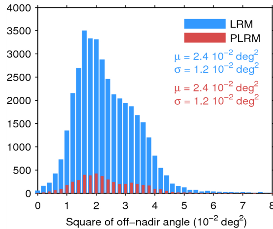
Figure 39. Histogram of flag-valid mispointing over oceans and lakes for LRM (blue) and PLRM (red) for 10/07/2014. Only positive values have been considered. The mean ( \mu ) and standard deviation ( \sigma ) are also shown. Note that values 8 \cdot 10^{-2} \text{ deg}^2 are excluded from the histogram for the sake of readability but not from the computation of \mu and \sigma .
