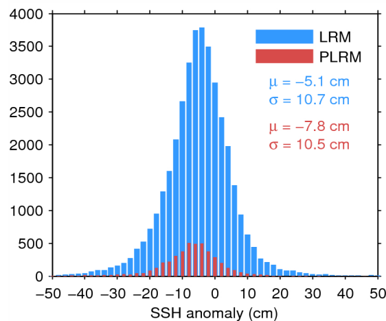
Figure 11. Histogram of science-valid SSH anomaly over oceans and lakes for LRM (blue) and PLRM (red) for 10/07/2014. The mean ( \mu ) and standard deviation ( \sigma ) are also shown. Note that values outside [-50 50] cm are excluded from the histogram for the sake of readability but not from the computation of \mu and \sigma .
