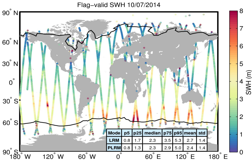
Figure 15. Geographical distribution of flag-valid SWH data over oceans and lakes for 10/07/2014. The statistical values shown in the table refer to the SWH in m and are calculated separately for LRM and PLRM regions. Measurements taken over polar polygons have been excluded from the computation of the statistical values. The black lines mark the outer limit of the Arctic and Antarctic polar polygons.
