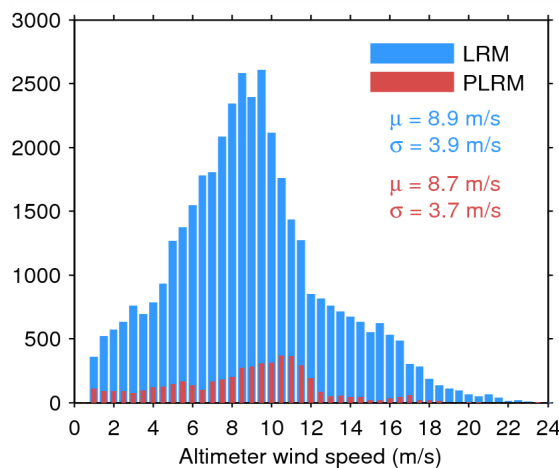
Figure 35. Histogram of science-valid wind over oceans and lakes for LRM (blue) and PLRM (red) for 10/07/2014. The mean ( \mu ) and standard deviation ( \sigma ) are also shown. Note that values larger than 24 m/s are excluded from the histogram for the sake of readability but not from the computation of \mu and \sigma .
