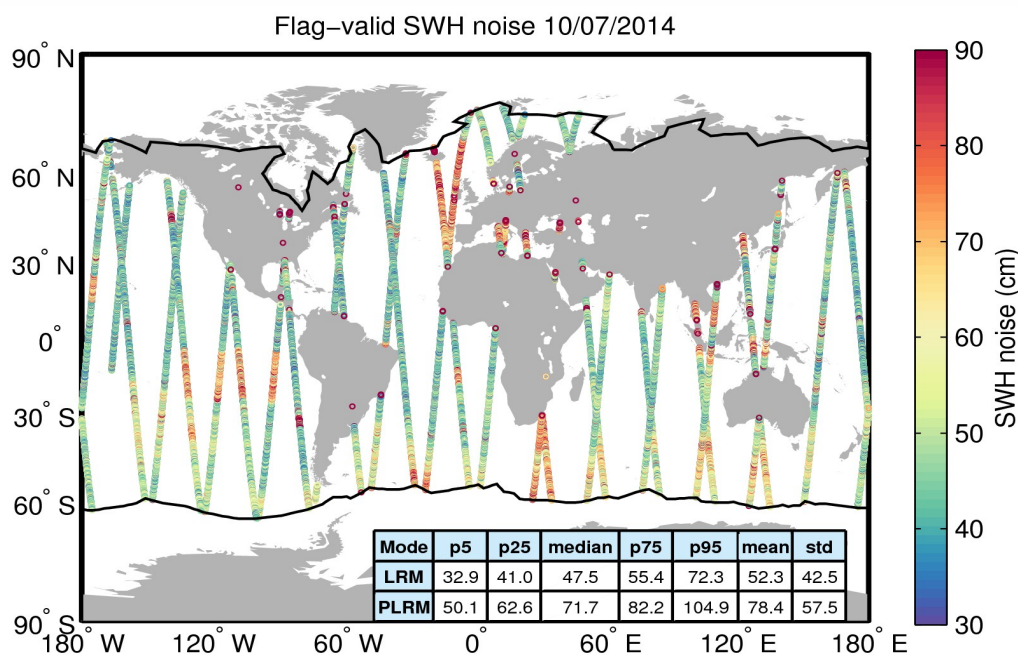
Figure 18. Geographical distribution of flag-valid 20-Hz SWH measurement noise over oceans and lakes for 10/07/2014. The statistical values shown in the table refer to the SWH noise and are calculated separately for LRM and PLRM regions. Measurements taken over polar polygons have been excluded from the computation of the statistical values. The black lines mark the outer limit of the Arctic and Antarctic polar polygons.
