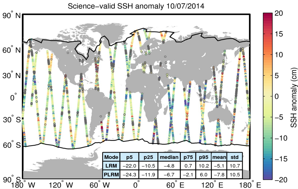
Figure 10. Geographical distribution of science-valid SSH anomaly data over oceans and lakes for 10/07/2014. The statistical values shown in the table refer to the SSH anomaly in cm and are calculated separately for LRM and PLRM regions. The black lines mark the outer limit of the Arctic and Antarctic polar polygons. Gray circles denote records that have been rejected based on the editing criteria described in Table 2.
