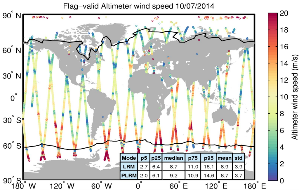
Figure 31. Geographical distribution of flag-valid wind data over oceans and lakes for 10/07/2014. The statistical values shown in the table refer to the wind in m/s and are calculated separately for LRM and PLRM regions. Measurements taken over polar polygons have been excluded from the computation of the statistical values. The black lines mark the outer limit of the Arctic and Antarctic polar polygons.
