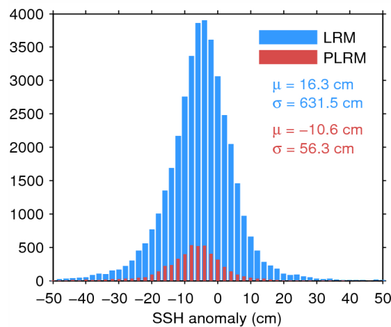
Figure 7. Histogram of flag-valid SSH anomaly over oceans and lakes for LRM (blue) and PLRM (red) for 10/07/2014. The mean ( \mu ) and standard deviation ( \sigma ) are also shown. Note that values outside [-50\ 50] cm are excluded from the histogram for the sake of readability but not from the computation of \mu and \sigma .
