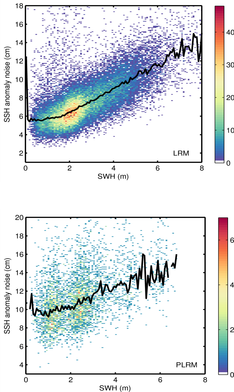
Figure 9. 2D histogram showing flag-valid SSH anomaly noise as a function of SWH for LRM (top) and PLRM (bottom) for 10/07/2014. The black line denotes the median SSH anomaly as a function of SWH.
