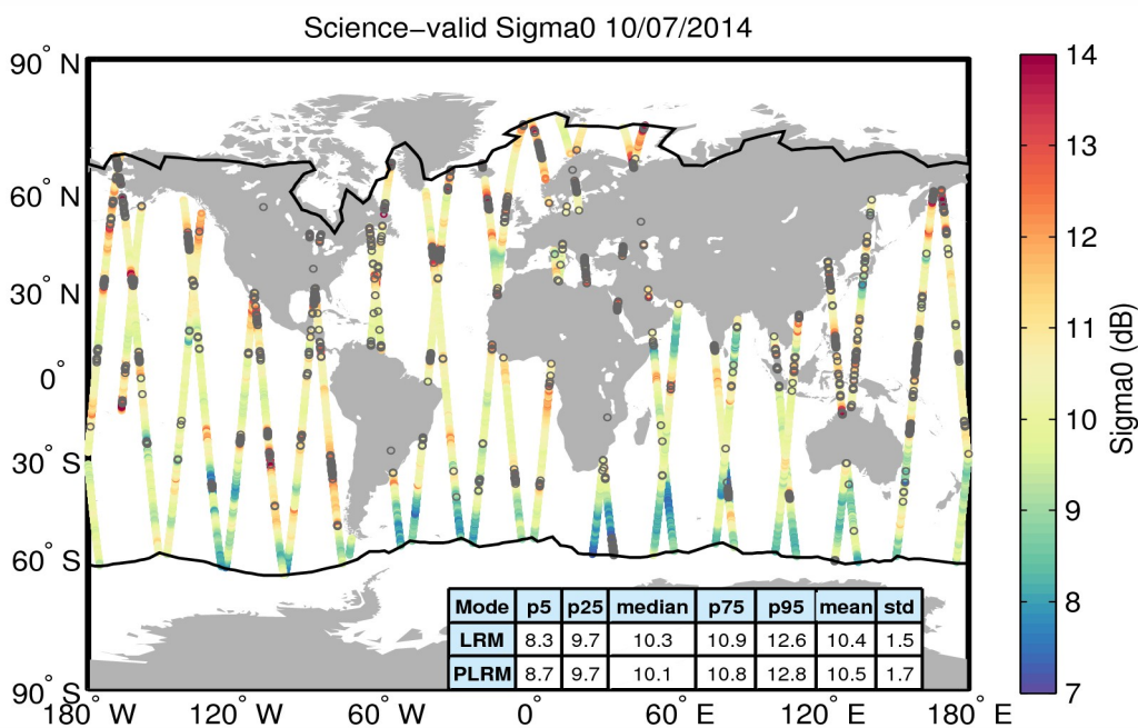
Figure 27. Geographical distribution of science-valid sigma0 data over oceans and lakes for 10/07/2014. The statistical values shown in the table refer to the sigma0 in dB and are calculated separately for LRM and PLRM regions. The black lines mark the outer limit of the Arctic and Antarctic polar polygons. Gray circles denote records that have been rejected based on the editing criteria described in Table 4.
