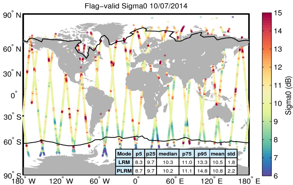
Figure 23. Geographical distribution of flag-valid sigma0 data over oceans and lakes for 10/07/2014. The statistical values shown in the table refer to the sigma0 in dB and are calculated separately for LRM and PLRM regions. Measurements taken over polar polygons have been excluded from the computation of the statistical values. The black lines mark the outer limit of the Arctic and Antarctic polar polygons.
