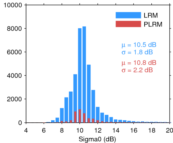
Figure 25. Histogram of flag-valid sigma0 over oceans and lakes for LRM (blue) and PLRM (red) for 10/07/2014. The mean ( \mu ) and standard deviation ( \sigma ) are also shown. Note that values outside [4 20] dB are excluded from the histogram for the sake of readability but not from the computation of \mu and \sigma .
