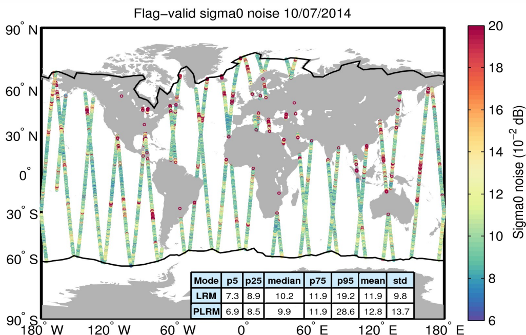
Figure 26. Geographical distribution of flag-valid 20-Hz sigma0 measurement noise over oceans and lakes for 10/07/2014. The statistical values shown in the table refer to the sigma0 noise and are calculated separately for LRM and PLRM regions. Measurements taken over polar polygons have been excluded from the computation of the statistical values. The black lines mark the outer limit of the Arctic and Antarctic polar polygons.
