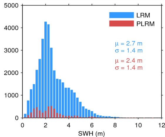
Figure 17. Histogram of flag-valid SWH over oceans and lakes for LRM (blue) and PLRM (red) for 10/07/2014. The mean ( \mu ) and standard deviation ( \sigma ) are also shown. Note that values larger than 12 m are excluded from the histogram for the sake of readability but not from the computation of \mu and \sigma .
