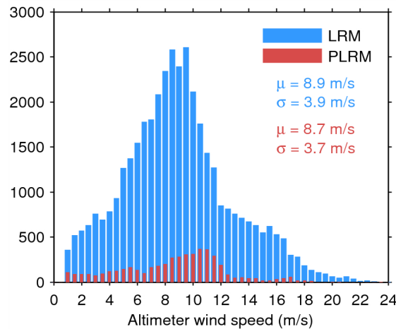
Figure 33. Histogram of flag-valid wind over oceans and lakes for LRM (blue) and PLRM (red) for 10/07/2014. The mean ( \mu ) and standard deviation ( \sigma ) are also shown. Note that values larger than 24 m/s are excluded from the histogram for the sake of readability but not from the computation of \mu and \sigma .
