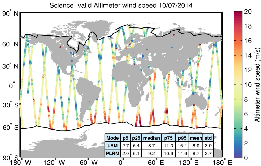
Figure 34. Geographical distribution of science-valid wind data over oceans and lakes for 10/07/2014. The statistical values shown in the table refer to the wind in m/s and are calculated separately for LRM and PLRM regions. The black lines mark the outer limit of the Arctic and Antarctic polar polygons. Gray circles denote records that have been rejected based on the editing criteria described in Table 5.
