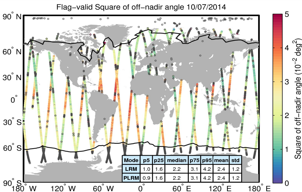
Figure 37. Geographical distribution of flag-valid mispointing data over oceans and lakes for 10/07/2014. The statistical values shown in the table refer to the mispointing in 10^{-2} \text{ deg}^2 and are calculated separately for LRM and PLRM regions. Measurements taken over polar polygons have been excluded from the computation of the statistical values. The black lines mark the outer limit of the Arctic and Antarctic polar polygons. Gray circles denote negative values.
