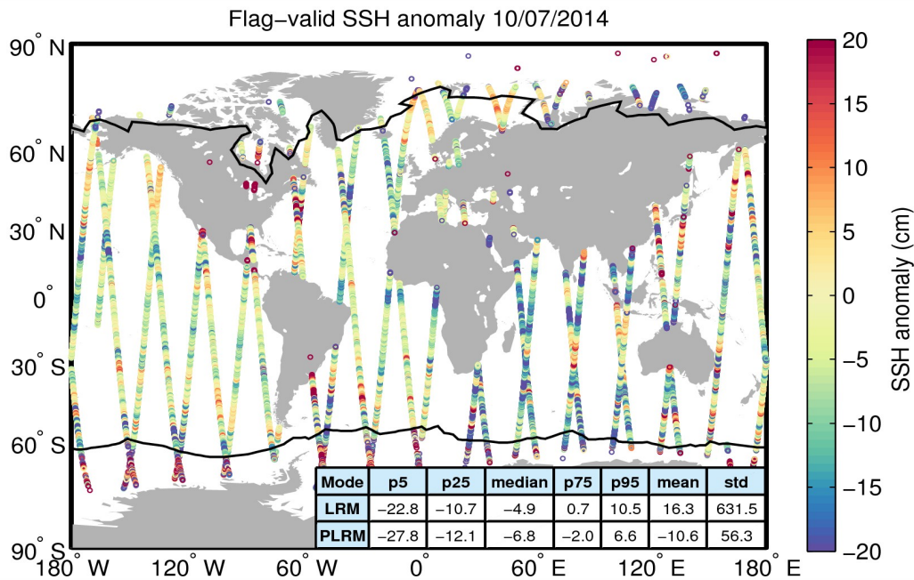
Figure 5. Geographical distribution of flag-valid 1-Hz SSH anomaly data over oceans and lakes for 10/07/2014. The statistical values shown in the table refer to the SSH anomaly in cm and are calculated separately for LRM and PLRM regions. Measurements taken over polar polygons have been excluded from the computation of the statistical values. The black lines mark the outer limit of the Arctic and Antarctic polar polygons.
