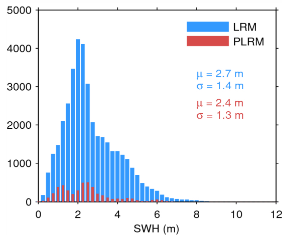
Figure 20. Histogram of science-valid SWH over oceans and lakes for LRM (blue) and PLRM (red) for 10/07/2014. The mean ( \mu ) and standard deviation ( \sigma ) are also shown. Note that values larger than 12 m are excluded from the histogram for the sake of readability but not from the computation of \mu and \sigma .
