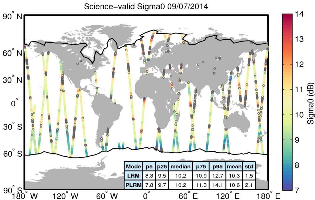
Figure 27. Geographical distribution of science-valid sigma0 data over oceans and lakes for 09/07/2014. The statistical values shown in the table refer to the sigma0 in dB and are calculated separately for LRM and PLRM regions. The black lines mark the outer limit of the Arctic and Antarctic polar polygons. Gray circles denote records that have been rejected based on the editing criteria described in Table 4.
