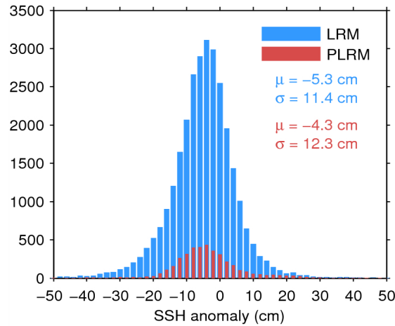
Figure 11. Histogram of science-valid SSH anomaly over oceans and lakes for LRM (blue) and PLRM (red) for 09/07/2014. The mean ( \mu ) and standard deviation ( \sigma ) are also shown. Note that values outside [-50\ 50] cm are excluded from the histogram for the sake of readability but not from the computation of \mu and \sigma .
