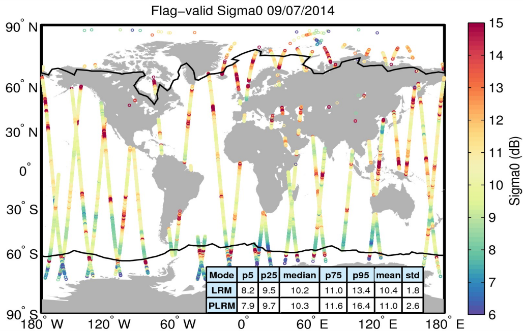
Figure 23. Geographical distribution of flag-valid sigma0 data over oceans and lakes for 09/07/2014. The statistical values shown in the table refer to the sigma0 in dB and are calculated separately for LRM and PLRM regions. Measurements taken over polar polygons have been excluded from the computation of the statistical values. The black lines mark the outer limit of the Arctic and Antarctic polar polygons.
