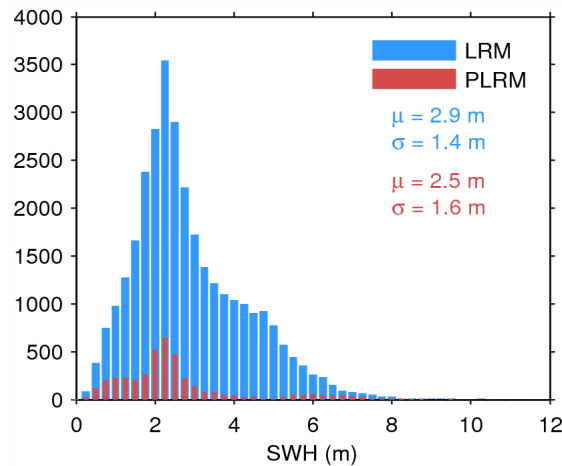
Figure 20. Histogram of science-valid SWH over oceans and lakes for LRM (blue) and PLRM (red) for 09/07/2014. The mean ( \mu ) and standard deviation ( \sigma ) are also shown. Note that values larger than 12 m are excluded from the histogram for the sake of readability but not from the computation of \mu and \sigma .
