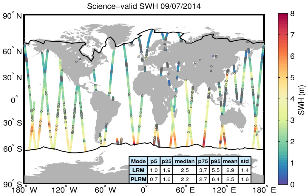
Figure 19. Geographical distribution of science-valid SWH data over oceans and lakes for 09/07/2014. The statistical values shown in the table refer to the SWH in m and are calculated separately for LRM and PLRM regions. The black lines mark the outer limit of the Arctic and Antarctic polar polygons. Gray circles denote records that have been rejected based on the editing criteria described in Table 3.
