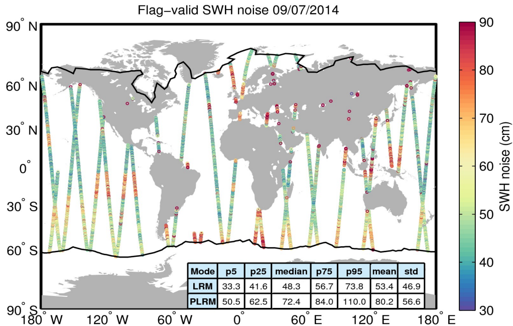
Figure 18. Geographical distribution of flag-valid 20-Hz SWH measurement noise over oceans and lakes for 09/07/2014. The statistical values shown in the table refer to the SWH noise and are calculated separately for LRM and PLRM regions. Measurements taken over polar polygons have been excluded from the computation of the statistical values. The black lines mark the outer limit of the Arctic and Antarctic polar polygons.
