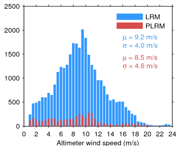
Figure 35. Histogram of science-valid wind over oceans and lakes for LRM (blue) and PLRM (red) for 09/07/2014. The mean ( \mu ) and standard deviation ( \sigma ) are also shown. Note that values larger than 24 m/s are excluded from the histogram for the sake of readability but not from the computation of \mu and \sigma .
