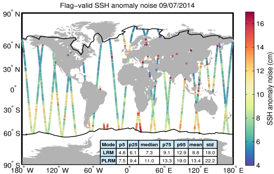
Figure 8. Geographical distribution of flag-valid 20-Hz SSH anomaly measurement noise over oceans and lakes for 09/07/2014. The statistical values shown in the table refer to the SSH anomaly noise and are calculated separately for LRM and PLRM regions. Measurements taken over polar polygons have been excluded from the computation of the statistical values. The black lines mark the outer limit of the Arctic and Antarctic polar polygons.
