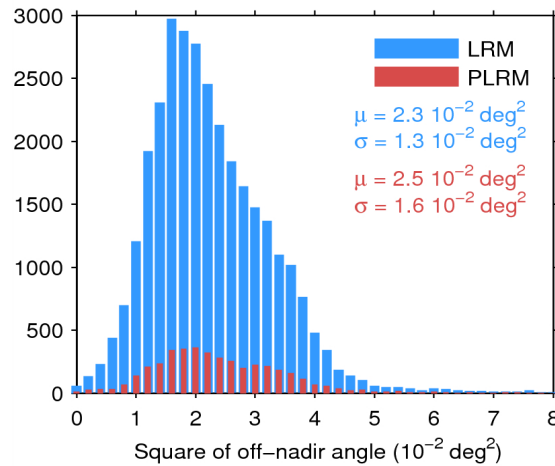
Figure 39. Histogram of flag-valid mispointing over oceans and lakes for LRM (blue) and PLRM (red) for 09/07/2014. Only positive values have been considered. The mean ( \mu ) and standard deviation ( \sigma ) are also shown. Note that values 8 \cdot 10^{-2} \text{ deg}^2 are excluded from the histogram for the sake of readability but not from the computation of \mu and \sigma .
