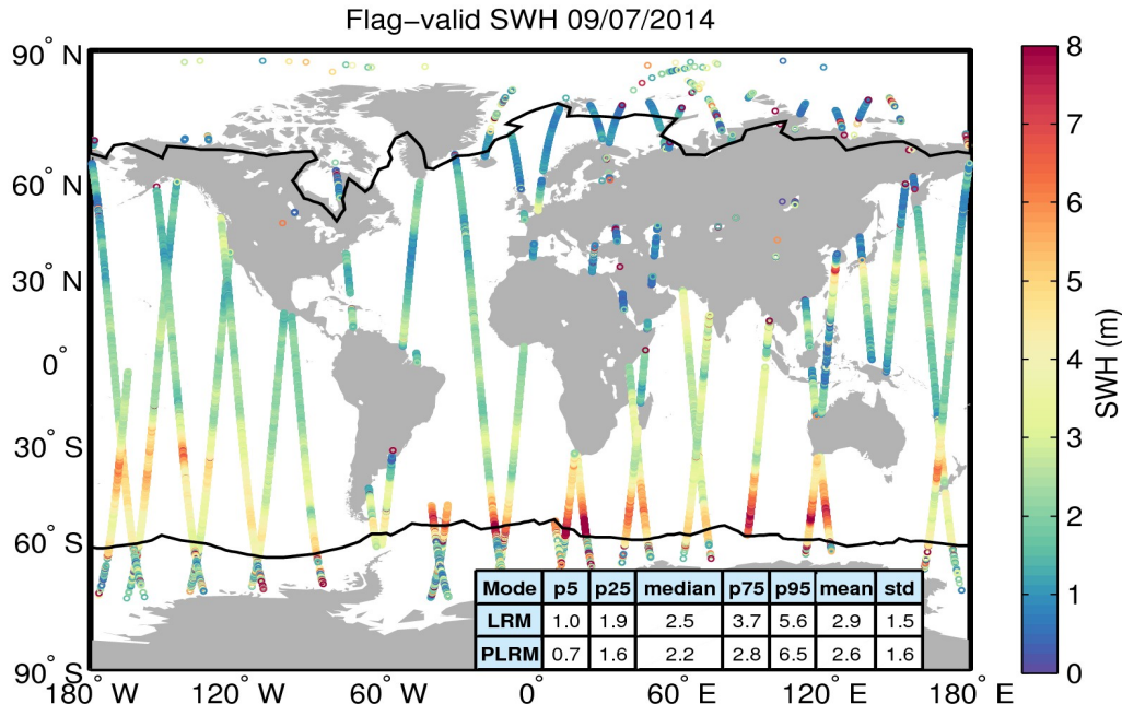
Figure 15. Geographical distribution of flag-valid SWH data over oceans and lakes for 09/07/2014. The statistical values shown in the table refer to the SWH in m and are calculated separately for LRM and PLRM regions. Measurements taken over polar polygons have been excluded from the computation of the statistical values. The black lines mark the outer limit of the Arctic and Antarctic polar polygons.
