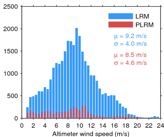
Figure 33. Histogram of flag-valid wind over oceans and lakes for LRM (blue) and PLRM (red) for 09/07/2014. The mean ( \mu ) and standard deviation ( \sigma ) are also shown. Note that values larger than 24 m/s are excluded from the histogram for the sake of readability but not from the computation of \mu and \sigma .
