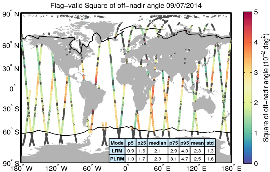
Figure 37. Geographical distribution of flag-valid mispointing data over oceans and lakes for 09/07/2014. The statistical values shown in the table refer to the mispointing in 10^{-2} \text{ deg}^2 and are calculated separately for LRM and PLRM regions. Measurements taken over polar polygons have been excluded from the computation of the statistical values. The black lines mark the outer limit of the Arctic and Antarctic polar polygons. Gray circles denote negative values.
