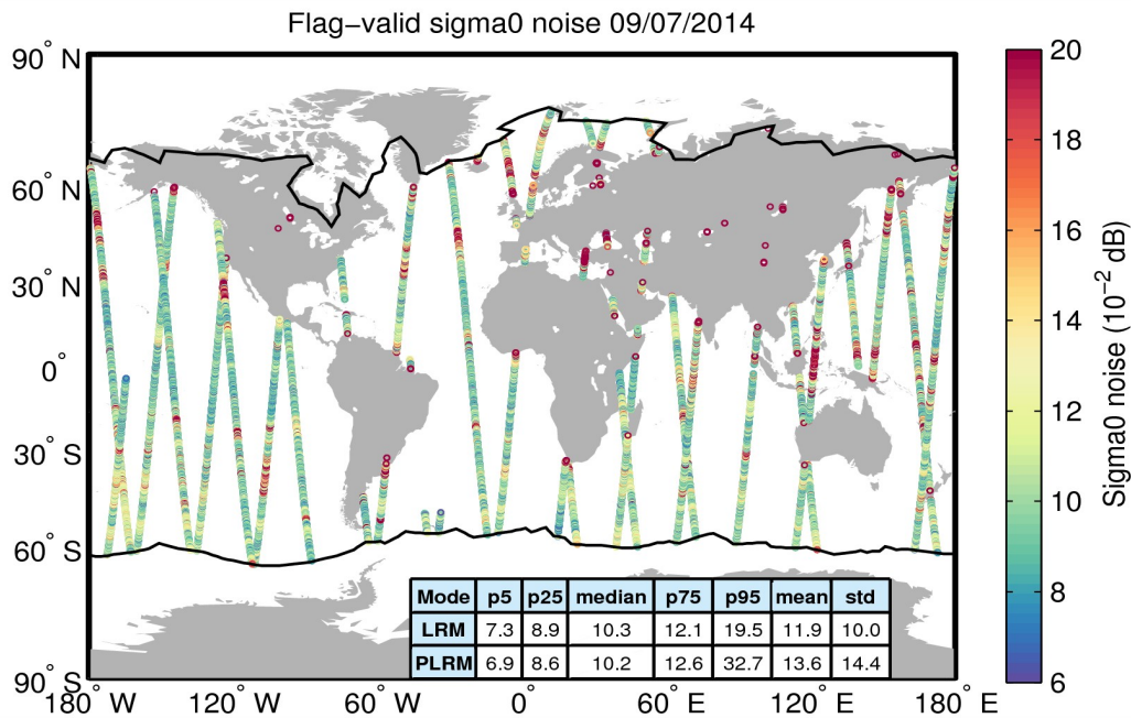
Figure 26. Geographical distribution of flag-valid 20-Hz sigma0 measurement noise over oceans and lakes for 09/07/2014. The statistical values shown in the table refer to the sigma0 noise and are calculated separately for LRM and PLRM regions. Measurements taken over polar polygons have been excluded from the computation of the statistical values. The black lines mark the outer limit of the Arctic and Antarctic polar polygons.
