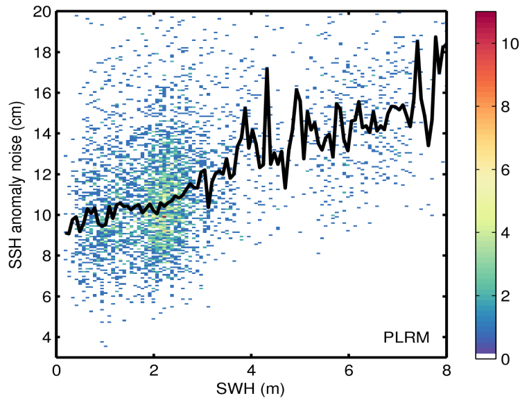
Figure 9. 2D histogram showing flag-valid SSH anomaly noise as a function of SWH for LRM (top) and PLRM (bottom) for 09/07/2014. The black line denotes the median SSH anomaly as a function of SWH.
