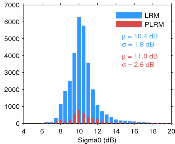
Figure 25. Histogram of flag-valid sigma0 over oceans and lakes for LRM (blue) and PLRM (red) for 09/07/2014. The mean ( \mu ) and standard deviation ( \sigma ) are also shown. Note that values outside [4 20] dB are excluded from the histogram for the sake of readability but not from the computation of \mu and \sigma .
