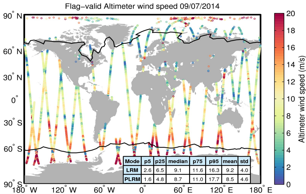
Figure 31. Geographical distribution of flag-valid wind data over oceans and lakes for 09/07/2014. The statistical values shown in the table refer to the wind in m/s and are calculated separately for LRM and PLRM regions. Measurements taken over polar polygons have been excluded from the computation of the statistical values. The black lines mark the outer limit of the Arctic and Antarctic polar polygons.
