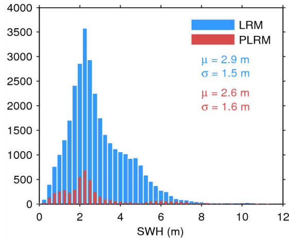
Figure 17. Histogram of flag-valid SWH over oceans and lakes for LRM (blue) and PLRM (red) for 09/07/2014. The mean ( \mu ) and standard deviation ( \sigma ) are also shown. Note that values larger than 12 m are excluded from the histogram for the sake of readability but not from the computation of \mu and \sigma .
