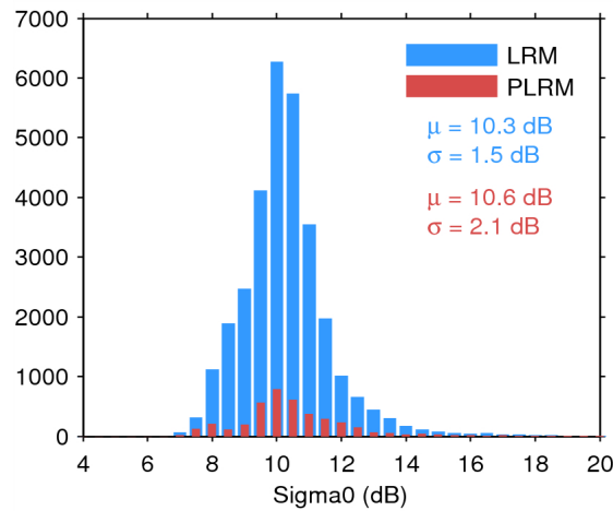
Figure 28. Histogram of science-valid sigma0 over oceans and lakes for LRM (blue) and PLRM (red) for 09/07/2014. The mean ( \mu ) and standard deviation ( \sigma ) are also shown. Note that values outside [4 20] dB are excluded from the histogram for the sake of readability but not from the computation of \mu and \sigma .
