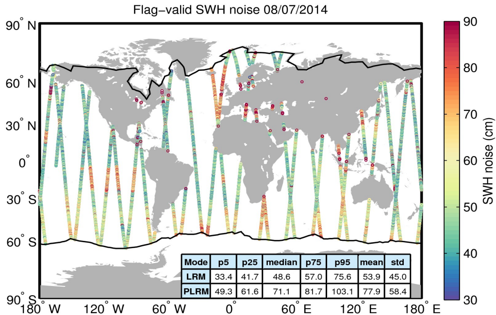
Figure 18. Geographical distribution of flag-valid 20-Hz SWH measurement noise over oceans and lakes for 08/07/2014. The statistical values shown in the table refer to the SWH noise and are calculated separately for LRM and PLRM regions. Measurements taken over polar polygons have been excluded from the computation of the statistical values. The black lines mark the outer limit of the Arctic and Antarctic polar polygons.
