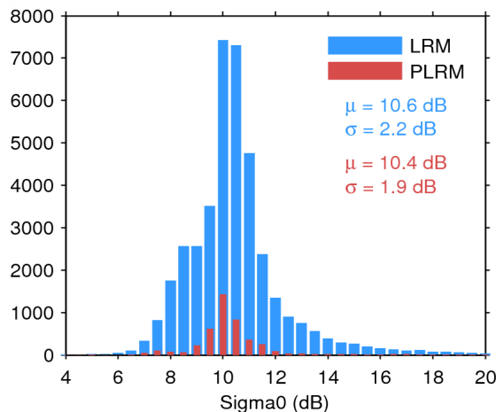
Figure 25. Histogram of flag-valid sigma0 over oceans and lakes for LRM (blue) and PLRM (red) for 08/07/2014. The mean ( \mu ) and standard deviation ( \sigma ) are also shown. Note that values outside [4 20] dB are excluded from the histogram for the sake of readability but not from the computation of \mu and \sigma .
