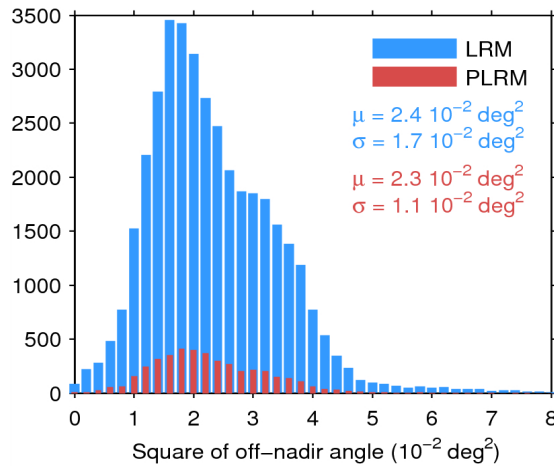
Figure 39. Histogram of flag-valid mispointing over oceans and lakes for LRM (blue) and PLRM (red) for 08/07/2014. Only positive values have been considered. The mean ( \mu ) and standard deviation ( \sigma ) are also shown. Note that values 8 \cdot 10^{-2} \text{ deg}^2 are excluded from the histogram for the sake of readability but not from the computation of \mu and \sigma .
