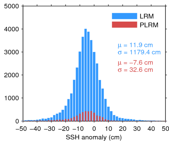
Figure 7. Histogram of flag-valid SSH anomaly over oceans and lakes for LRM (blue) and PLRM (red) for 08/07/2014. The mean ( \mu ) and standard deviation ( \sigma ) are also shown. Note that values outside [-50 50] cm are excluded from the histogram for the sake of readability but not from the computation of \mu and \sigma .
