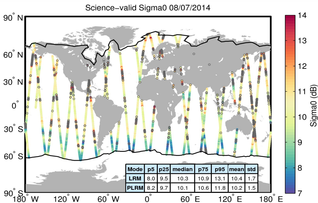
Figure 27. Geographical distribution of science-valid sigma0 data over oceans and lakes for 08/07/2014. The statistical values shown in the table refer to the sigma0 in dB and are calculated separately for LRM and PLRM regions. The black lines mark the outer limit of the Arctic and Antarctic polar polygons. Gray circles denote records that have been rejected based on the editing criteria described in Table 4.
