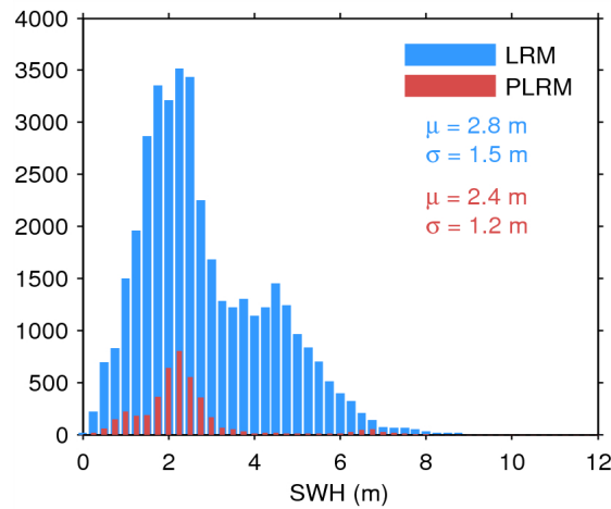
Figure 20. Histogram of science-valid SWH over oceans and lakes for LRM (blue) and PLRM (red) for 08/07/2014. The mean ( \mu ) and standard deviation ( \sigma ) are also shown. Note that values larger than 12 m are excluded from the histogram for the sake of readability but not from the computation of \mu and \sigma .
