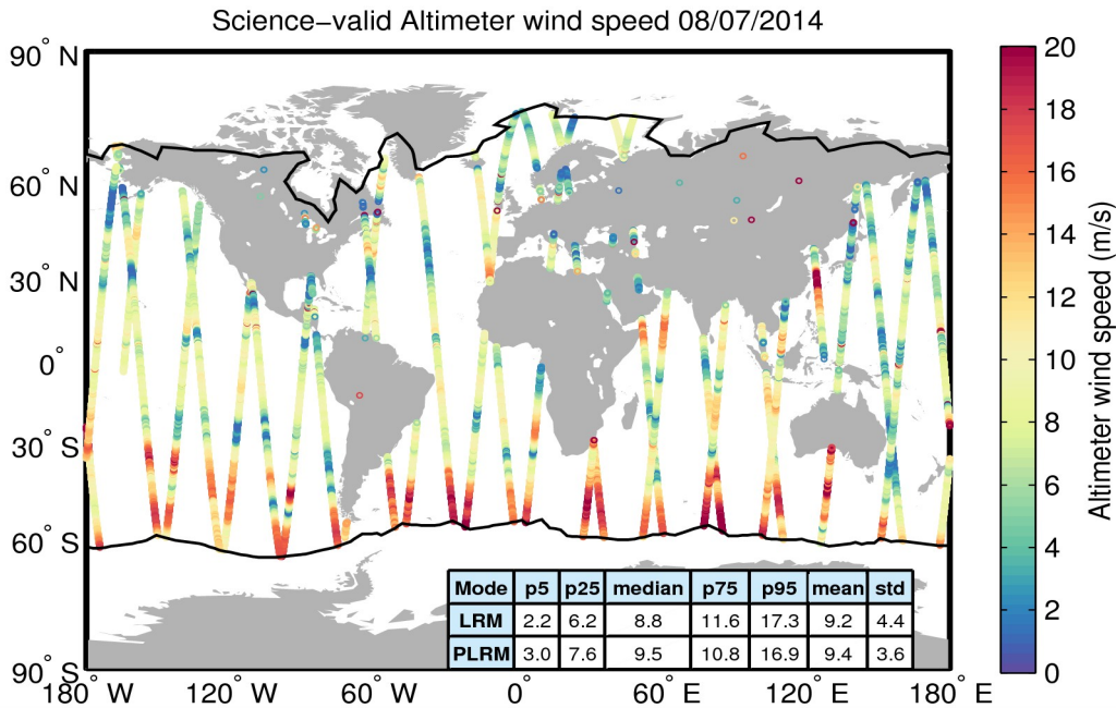
Figure 34. Geographical distribution of science-valid wind data over oceans and lakes for 08/07/2014. The statistical values shown in the table refer to the wind in m/s and are calculated separately for LRM and PLRM regions. The black lines mark the outer limit of the Arctic and Antarctic polar polygons. Gray circles denote records that have been rejected based on the editing criteria described in Table 5.
