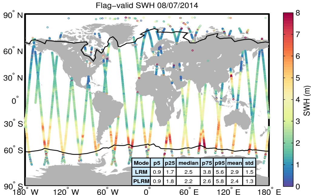
Figure 15. Geographical distribution of flag-valid SWH data over oceans and lakes for 08/07/2014. The statistical values shown in the table refer to the SWH in m and are calculated separately for LRM and PLRM regions. Measurements taken over polar polygons have been excluded from the computation of the statistical values. The black lines mark the outer limit of the Arctic and Antarctic polar polygons.
