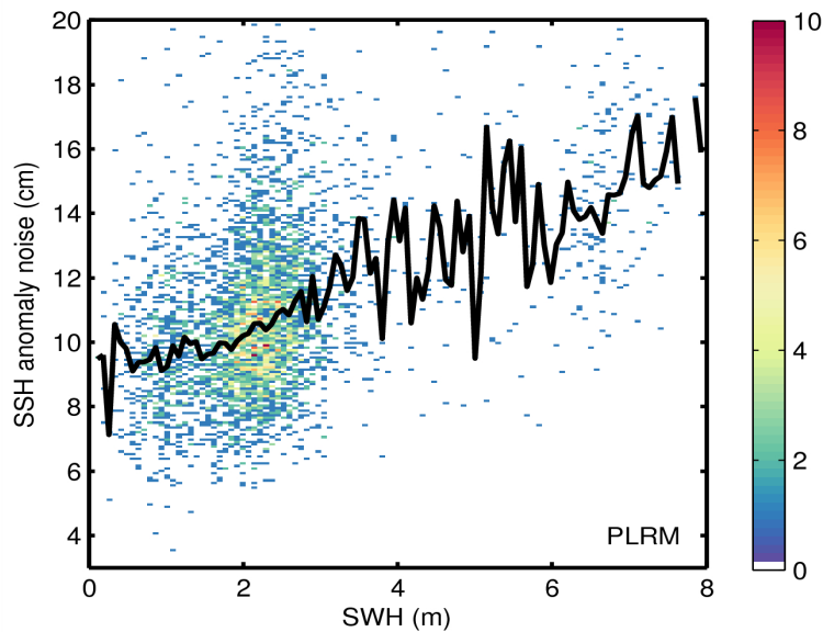
Figure 9. 2D histogram showing flag-valid SSH anomaly noise as a function of SWH for LRM (top) and PLRM (bottom) for 08/07/2014. The black line denotes the median SSH anomaly as a function of SWH.
