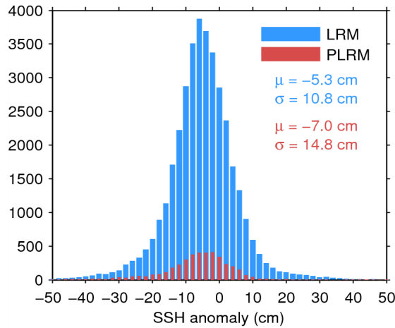
Figure 11. Histogram of science-valid SSH anomaly over oceans and lakes for LRM (blue) and PLRM (red) for 08/07/2014. The mean ( \mu ) and standard deviation ( \sigma ) are also shown. Note that values outside [-50 50] cm are excluded from the histogram for the sake of readability but not from the computation of \mu and \sigma .
