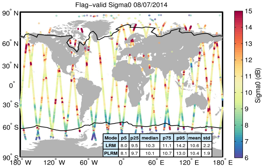
Figure 23. Geographical distribution of flag-valid sigma0 data over oceans and lakes for 08/07/2014. The statistical values shown in the table refer to the sigma0 in dB and are calculated separately for LRM and PLRM regions. Measurements taken over polar polygons have been excluded from the computation of the statistical values. The black lines mark the outer limit of the Arctic and Antarctic polar polygons.
