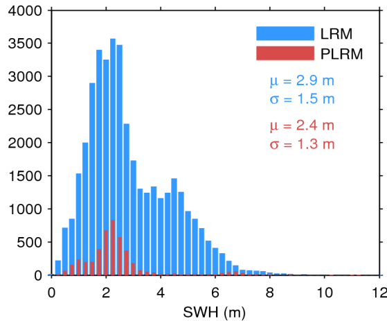
Figure 17. Histogram of flag-valid SWH over oceans and lakes for LRM (blue) and PLRM (red) for 08/07/2014. The mean ( \mu ) and standard deviation ( \sigma ) are also shown. Note that values larger than 12 m are excluded from the histogram for the sake of readability but not from the computation of \mu and \sigma .
