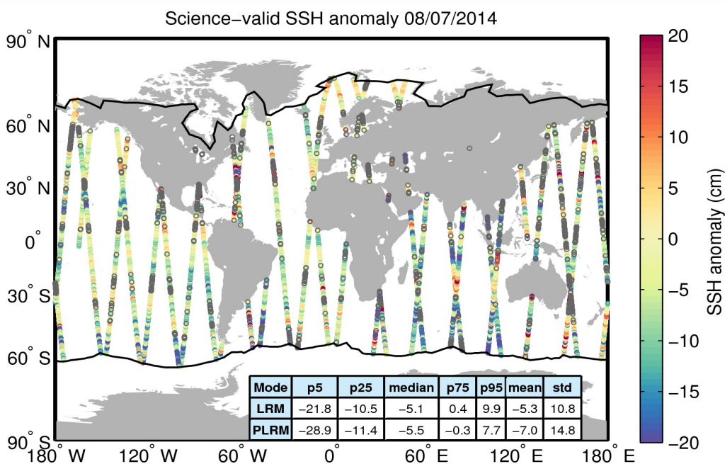
Figure 10. Geographical distribution of science-valid SSH anomaly data over oceans and lakes for 08/07/2014. The statistical values shown in the table refer to the SSH anomaly in cm and are calculated separately for LRM and PLRM regions. The black lines mark the outer limit of the Arctic and Antarctic polar polygons. Gray circles denote records that have been rejected based on the editing criteria described in Table 2.
