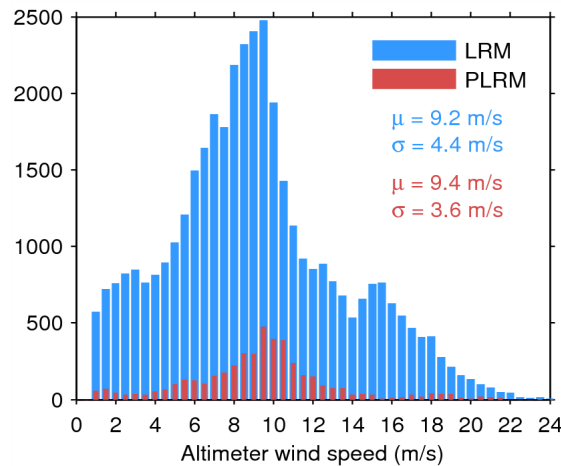
Figure 33. Histogram of flag-valid wind over oceans and lakes for LRM (blue) and PLRM (red) for 08/07/2014. The mean ( \mu ) and standard deviation ( \sigma ) are also shown. Note that values larger than 24 m/s are excluded from the histogram for the sake of readability but not from the computation of \mu and \sigma .
