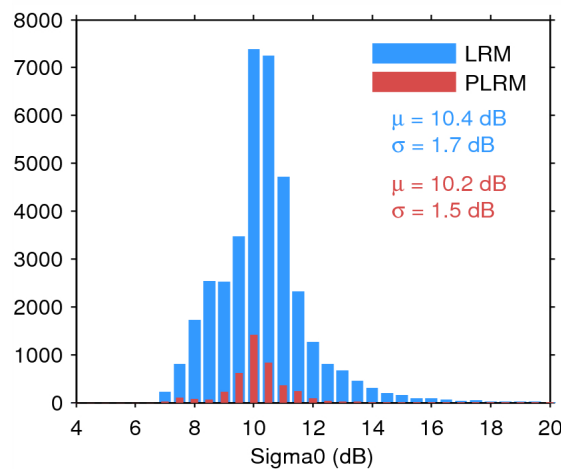
Figure 28. Histogram of science-valid sigma0 over oceans and lakes for LRM (blue) and PLRM (red) for 08/07/2014. The mean ( \mu ) and standard deviation ( \sigma ) are also shown. Note that values outside [4 20] dB are excluded from the histogram for the sake of readability but not from the computation of \mu and \sigma .
