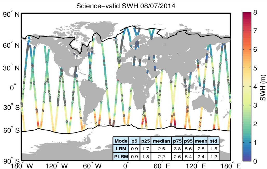
Figure 19. Geographical distribution of science-valid SWH data over oceans and lakes for 08/07/2014. The statistical values shown in the table refer to the SWH in m and are calculated separately for LRM and PLRM regions. The black lines mark the outer limit of the Arctic and Antarctic polar polygons. Gray circles denote records that have been rejected based on the editing criteria described in Table 3.
