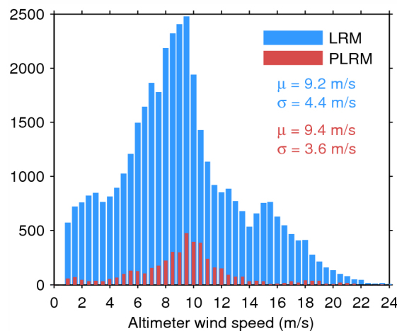
Figure 35. Histogram of science-valid wind over oceans and lakes for LRM (blue) and PLRM (red) for 08/07/2014. The mean ( \mu ) and standard deviation ( \sigma ) are also shown. Note that values larger than 24 m/s are excluded from the histogram for the sake of readability but not from the computation of \mu and \sigma .
