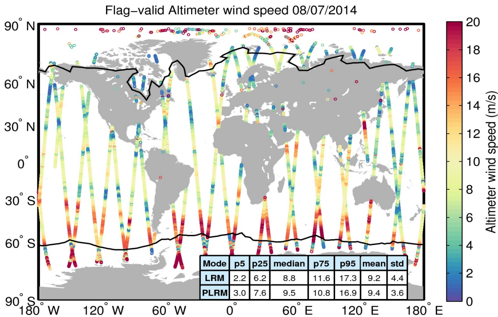
Figure 31. Geographical distribution of flag-valid wind data over oceans and lakes for 08/07/2014. The statistical values shown in the table refer to the wind in m/s and are calculated separately for LRM and PLRM regions. Measurements taken over polar polygons have been excluded from the computation of the statistical values. The black lines mark the outer limit of the Arctic and Antarctic polar polygons.
