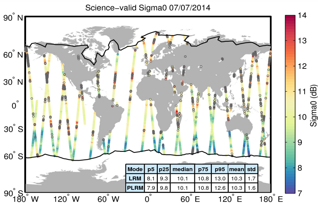
Figure 27. Geographical distribution of science-valid sigma0 data over oceans and lakes for 07/07/2014. The statistical values shown in the table refer to the sigma0 in dB and are calculated separately for LRM and PLRM regions. The black lines mark the outer limit of the Arctic and Antarctic polar polygons. Gray circles denote records that have been rejected based on the editing criteria described in Table 4.
