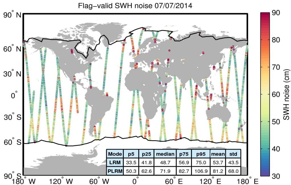
Figure 18. Geographical distribution of flag-valid 20-Hz SWH measurement noise over oceans and lakes for 07/07/2014. The statistical values shown in the table refer to the SWH noise and are calculated separately for LRM and PLRM regions. Measurements taken over polar polygons have been excluded from the computation of the statistical values. The black lines mark the outer limit of the Arctic and Antarctic polar polygons.
