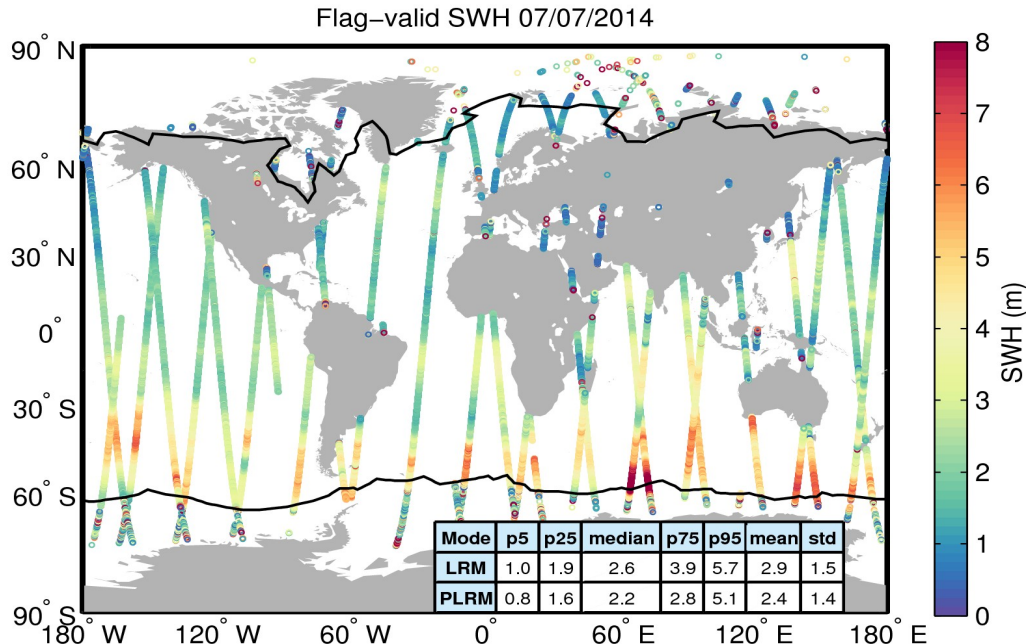
Figure 15. Geographical distribution of flag-valid SWH data over oceans and lakes for 07/07/2014. The statistical values shown in the table refer to the SWH in m and are calculated separately for LRM and PLRM regions. Measurements taken over polar polygons have been excluded from the computation of the statistical values. The black lines mark the outer limit of the Arctic and Antarctic polar polygons.
