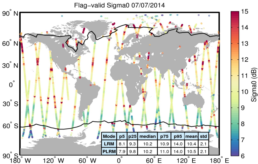
Figure 23. Geographical distribution of flag-valid sigma0 data over oceans and lakes for 07/07/2014. The statistical values shown in the table refer to the sigma0 in dB and are calculated separately for LRM and PLRM regions. Measurements taken over polar polygons have been excluded from the computation of the statistical values. The black lines mark the outer limit of the Arctic and Antarctic polar polygons.
