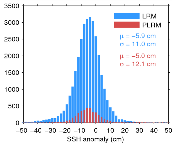
Figure 11. Histogram of science-valid SSH anomaly over oceans and lakes for LRM (blue) and PLRM (red) for 07/07/2014. The mean ( \mu ) and standard deviation ( \sigma ) are also shown. Note that values outside [-50\ 50] cm are excluded from the histogram for the sake of readability but not from the computation of \mu and \sigma .
