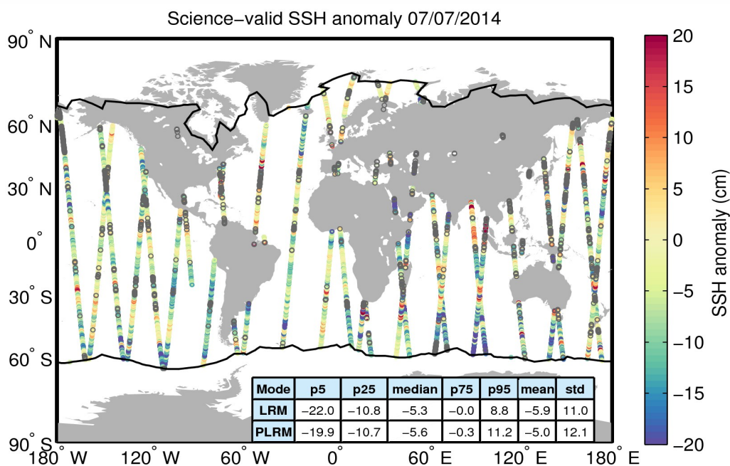
Figure 10. Geographical distribution of science-valid SSH anomaly data over oceans and lakes for 07/07/2014. The statistical values shown in the table refer to the SSH anomaly in cm and are calculated separately for LRM and PLRM regions. The black lines mark the outer limit of the Arctic and Antarctic polar polygons. Gray circles denote records that have been rejected based on the editing criteria described in Table 2.
