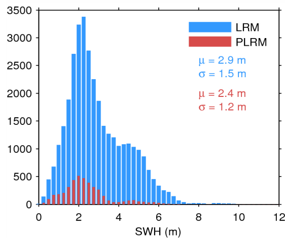
Figure 20. Histogram of science-valid SWH over oceans and lakes for LRM (blue) and PLRM (red) for 07/07/2014. The mean ( \mu ) and standard deviation ( \sigma ) are also shown. Note that values larger than 12 m are excluded from the histogram for the sake of readability but not from the computation of \mu and \sigma .
