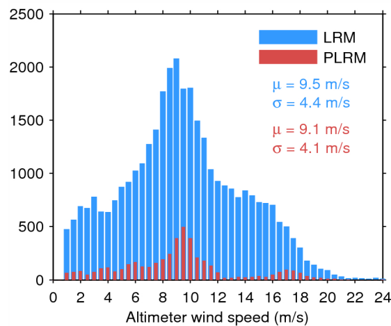
Figure 33. Histogram of flag-valid wind over oceans and lakes for LRM (blue) and PLRM (red) for 07/07/2014. The mean ( \mu ) and standard deviation ( \sigma ) are also shown. Note that values larger than 24 m/s are excluded from the histogram for the sake of readability but not from the computation of \mu and \sigma .
