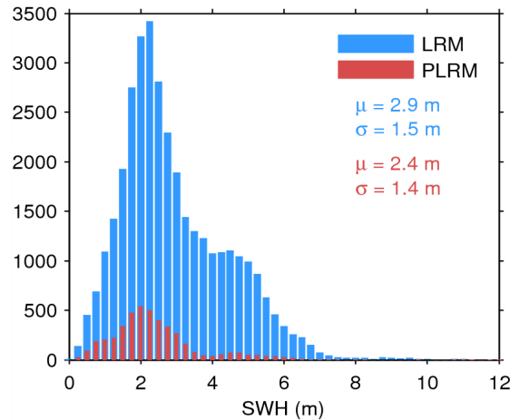
Figure 17. Histogram of flag-valid SWH over oceans and lakes for LRM (blue) and PLRM (red) for 07/07/2014. The mean ( \mu ) and standard deviation ( \sigma ) are also shown. Note that values larger than 12 m are excluded from the histogram for the sake of readability but not from the computation of \mu and \sigma .
