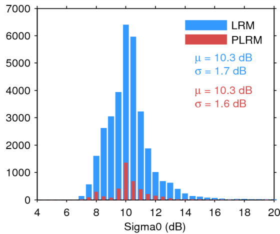
Figure 28. Histogram of science-valid sigma0 over oceans and lakes for LRM (blue) and PLRM (red) for 07/07/2014. The mean ( \mu ) and standard deviation ( \sigma ) are also shown. Note that values outside [4 20] dB are excluded from the histogram for the sake of readability but not from the computation of \mu and \sigma .
