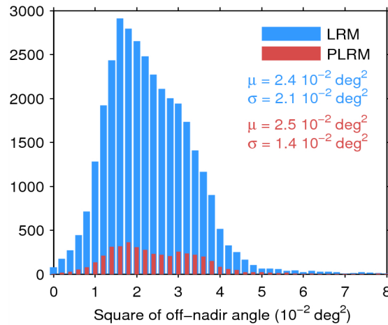
Figure 39. Histogram of flag-valid mispointing over oceans and lakes for LRM (blue) and PLRM (red) for 07/07/2014. Only positive values have been considered. The mean ( \mu ) and standard deviation ( \sigma ) are also shown. Note that values 8 \cdot 10^{-2} \text{ deg}^2 are excluded from the histogram for the sake of readability but not from the computation of \mu and \sigma .
