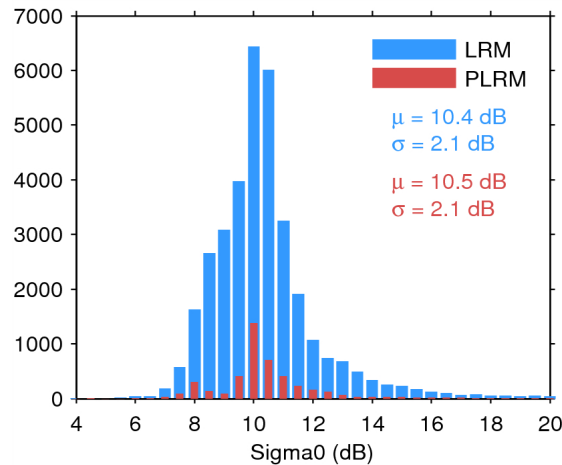
Figure 25. Histogram of flag-valid sigma0 over oceans and lakes for LRM (blue) and PLRM (red) for 07/07/2014. The mean ( \mu ) and standard deviation ( \sigma ) are also shown. Note that values outside [4 20] dB are excluded from the histogram for the sake of readability but not from the computation of \mu and \sigma .
