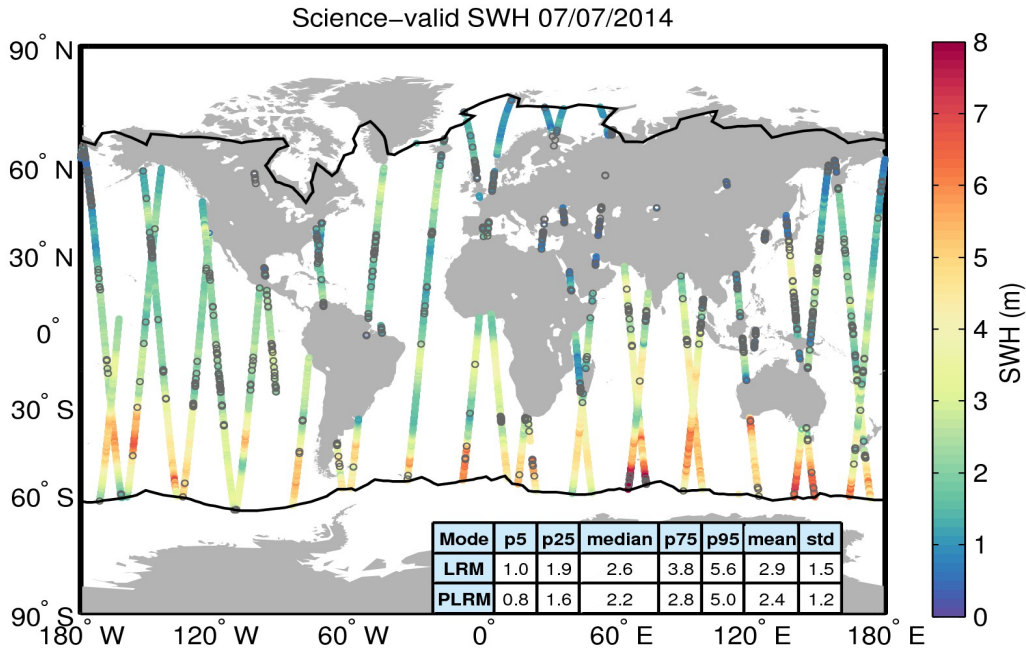
Figure 19. Geographical distribution of science-valid SWH data over oceans and lakes for 07/07/2014. The statistical values shown in the table refer to the SWH in m and are calculated separately for LRM and PLRM regions. The black lines mark the outer limit of the Arctic and Antarctic polar polygons. Gray circles denote records that have been rejected based on the editing criteria described in Table 3.
