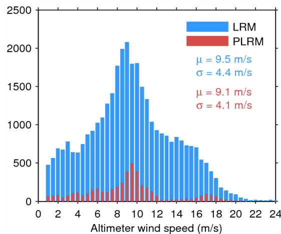
Figure 35. Histogram of science-valid wind over oceans and lakes for LRM (blue) and PLRM (red) for 07/07/2014. The mean ( \mu ) and standard deviation ( \sigma ) are also shown. Note that values larger than 24 m/s are excluded from the histogram for the sake of readability but not from the computation of \mu and \sigma .
