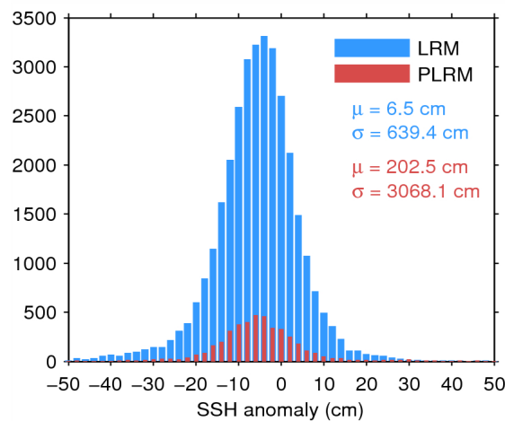
Figure 7. Histogram of flag-valid SSH anomaly over oceans and lakes for LRM (blue) and PLRM (red) for 07/07/2014. The mean ( \mu ) and standard deviation ( \sigma ) are also shown. Note that values outside [-50\ 50] cm are excluded from the histogram for the sake of readability but not from the computation of \mu and \sigma .
