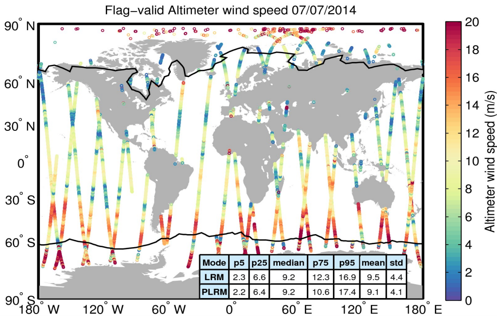
Figure 31. Geographical distribution of flag-valid wind data over oceans and lakes for 07/07/2014. The statistical values shown in the table refer to the wind in m/s and are calculated separately for LRM and PLRM regions. Measurements taken over polar polygons have been excluded from the computation of the statistical values. The black lines mark the outer limit of the Arctic and Antarctic polar polygons.
