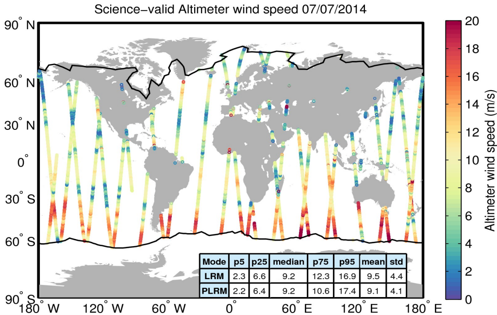
Figure 34. Geographical distribution of science-valid wind data over oceans and lakes for 07/07/2014. The statistical values shown in the table refer to the wind in m/s and are calculated separately for LRM and PLRM regions. The black lines mark the outer limit of the Arctic and Antarctic polar polygons. Gray circles denote records that have been rejected based on the editing criteria described in Table 5.
