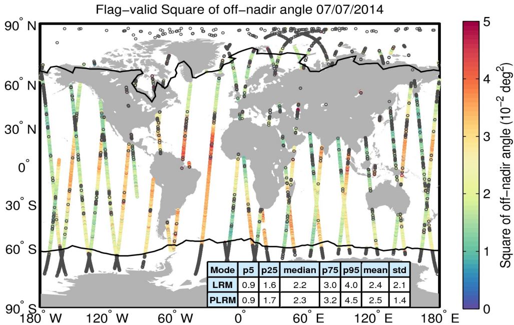
Figure 37. Geographical distribution of flag-valid mispointing data over oceans and lakes for 07/07/2014. The statistical values shown in the table refer to the mispointing in 10^{-2} deg 2 and are calculated separately for LRM and PLRM regions. Measurements taken over polar polygons have been excluded from the computation of the statistical values. The black lines mark the outer limit of the Arctic and Antarctic polar polygons. Gray circles denote negative values.
