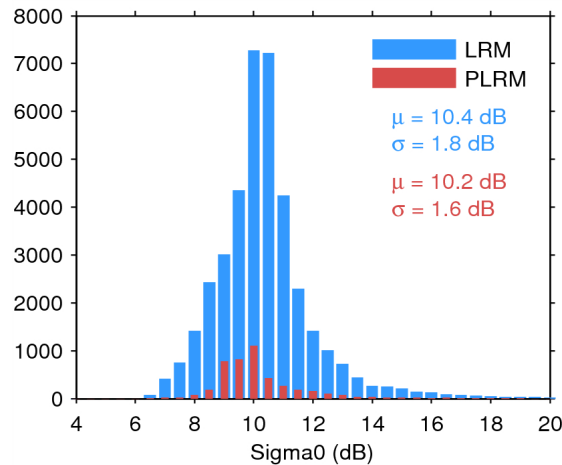
Figure 25. Histogram of flag-valid sigma0 over oceans and lakes for LRM (blue) and PLRM (red) for 05/07/2014. The mean ( \mu ) and standard deviation ( \sigma ) are also shown. Note that values outside [4 20] dB are excluded from the histogram for the sake of readability but not from the computation of \mu and \sigma .
