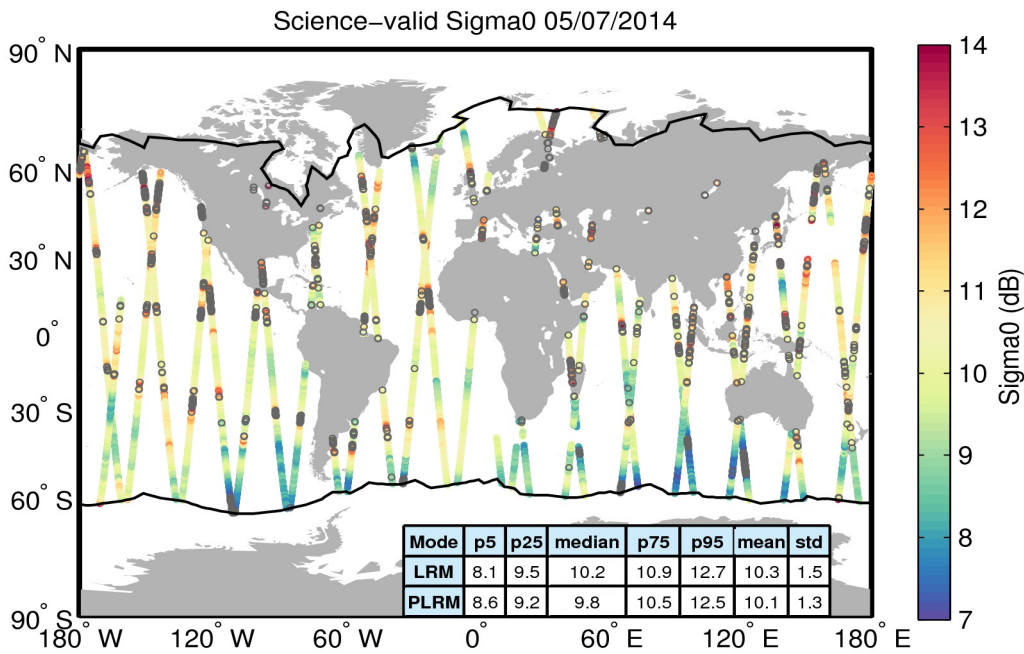
Figure 27. Geographical distribution of science-valid sigma0 data over oceans and lakes for 05/07/2014. The statistical values shown in the table refer to the sigma0 in dB and are calculated separately for LRM and PLRM regions. The black lines mark the outer limit of the Arctic and Antarctic polar polygons. Gray circles denote records that have been rejected based on the editing criteria described in Table 4.
