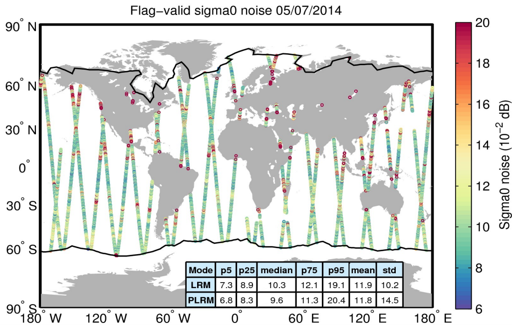
Figure 26. Geographical distribution of flag-valid 20-Hz sigma0 measurement noise over oceans and lakes for 05/07/2014. The statistical values shown in the table refer to the sigma0 noise and are calculated separately for LRM and PLRM regions. Measurements taken over polar polygons have been excluded from the computation of the statistical values. The black lines mark the outer limit of the Arctic and Antarctic polar polygons.
