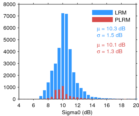
Figure 28. Histogram of science-valid sigma0 over oceans and lakes for LRM (blue) and PLRM (red) for 05/07/2014. The mean ( \mu ) and standard deviation ( \sigma ) are also shown. Note that values outside [4 20] dB are excluded from the histogram for the sake of readability but not from the computation of \mu and \sigma .
