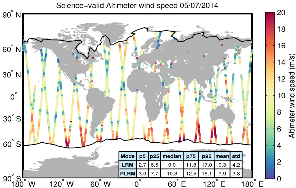
Figure 34. Geographical distribution of science-valid wind data over oceans and lakes for 05/07/2014. The statistical values shown in the table refer to the wind in m/s and are calculated separately for LRM and PLRM regions. The black lines mark the outer limit of the Arctic and Antarctic polar polygons. Gray circles denote records that have been rejected based on the editing criteria described in Table 5.
