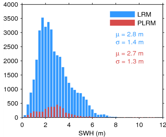
Figure 17. Histogram of flag-valid SWH over oceans and lakes for LRM (blue) and PLRM (red) for 05/07/2014. The mean ( \mu ) and standard deviation ( \sigma ) are also shown. Note that values larger than 12 m are excluded from the histogram for the sake of readability but not from the computation of \mu and \sigma .
