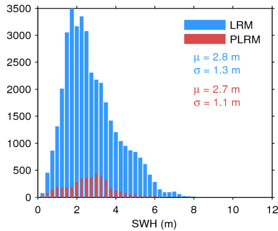
Figure 20. Histogram of science-valid SWH over oceans and lakes for LRM (blue) and PLRM (red) for 05/07/2014. The mean ( \mu ) and standard deviation ( \sigma ) are also shown. Note that values larger than 12 m are excluded from the histogram for the sake of readability but not from the computation of \mu and \sigma .
