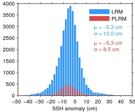
Figure 11. Histogram of science-valid SSH anomaly over oceans and lakes for LRM (blue) and PLRM (red) for 05/07/2014. The mean ( \mu ) and standard deviation ( \sigma ) are also shown. Note that values outside [-50 50] cm are excluded from the histogram for the sake of readability but not from the computation of \mu and \sigma .
