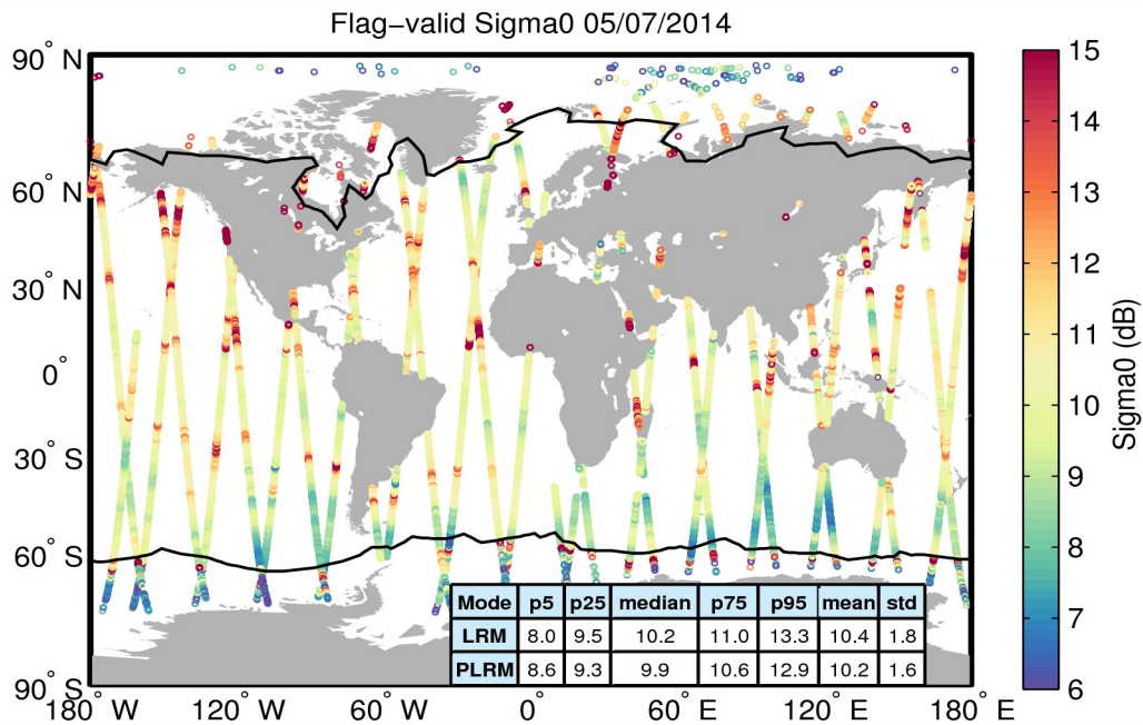
Figure 23. Geographical distribution of flag-valid sigma0 data over oceans and lakes for 05/07/2014. The statistical values shown in the table refer to the sigma0 in dB and are calculated separately for LRM and PLRM regions. Measurements taken over polar polygons have been excluded from the computation of the statistical values. The black lines mark the outer limit of the Arctic and Antarctic polar polygons.
