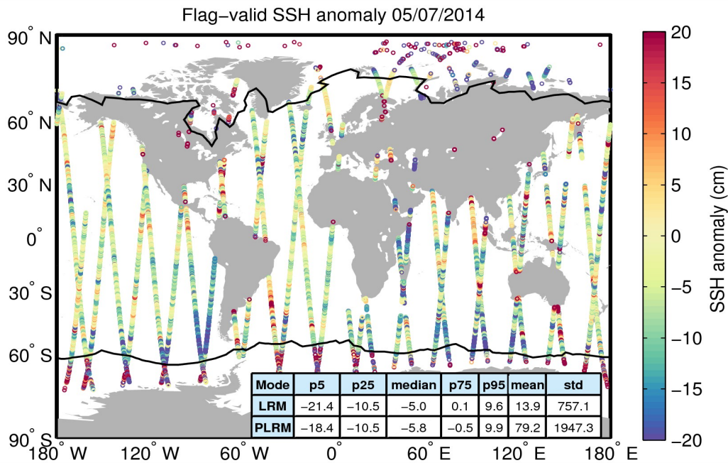
Figure 5. Geographical distribution of flag-valid 1-Hz SSH anomaly data over oceans and lakes for 05/07/2014. The statistical values shown in the table refer to the SSH anomaly in cm and are calculated separately for LRM and PLRM regions. Measurements taken over polar polygons have been excluded from the computation of the statistical values. The black lines mark the outer limit of the Arctic and Antarctic polar polygons.
