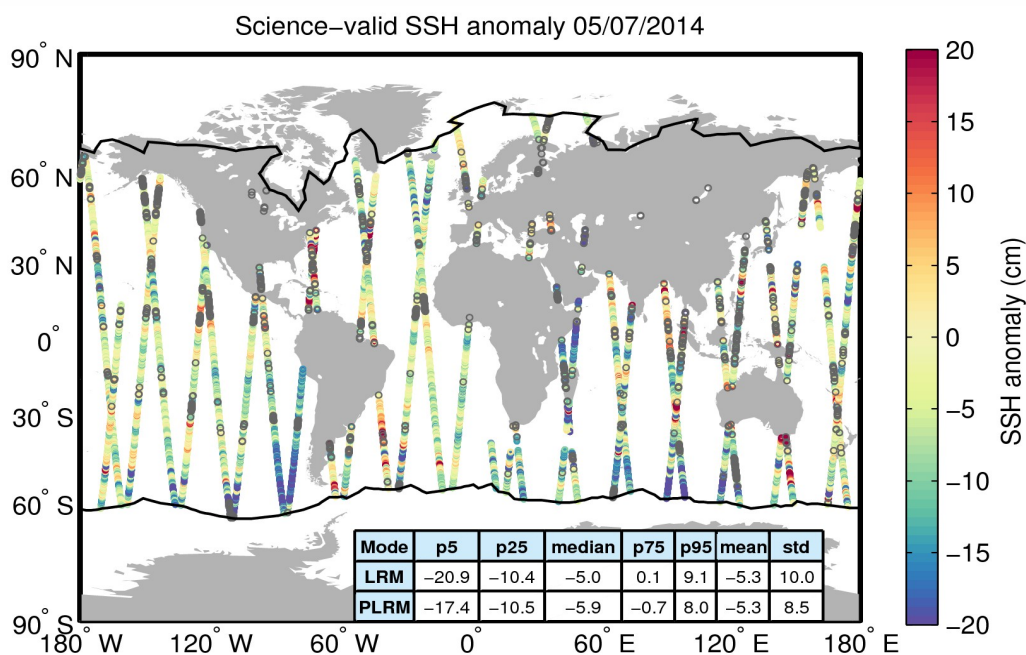
Figure 10. Geographical distribution of science-valid SSH anomaly data over oceans and lakes for 05/07/2014. The statistical values shown in the table refer to the SSH anomaly in cm and are calculated separately for LRM and PLRM regions. The black lines mark the outer limit of the Arctic and Antarctic polar polygons. Gray circles denote records that have been rejected based on the editing criteria described in Table 2.
