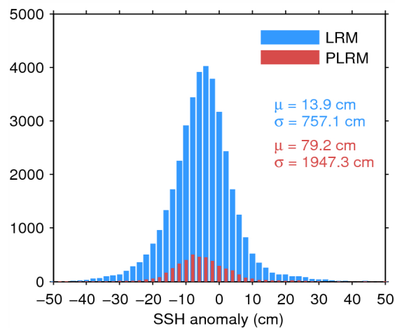
Figure 7. Histogram of flag-valid SSH anomaly over oceans and lakes for LRM (blue) and PLRM (red) for 05/07/2014. The mean ( \mu ) and standard deviation ( \sigma ) are also shown. Note that values outside [-50\ 50] cm are excluded from the histogram for the sake of readability but not from the computation of \mu and \sigma .
