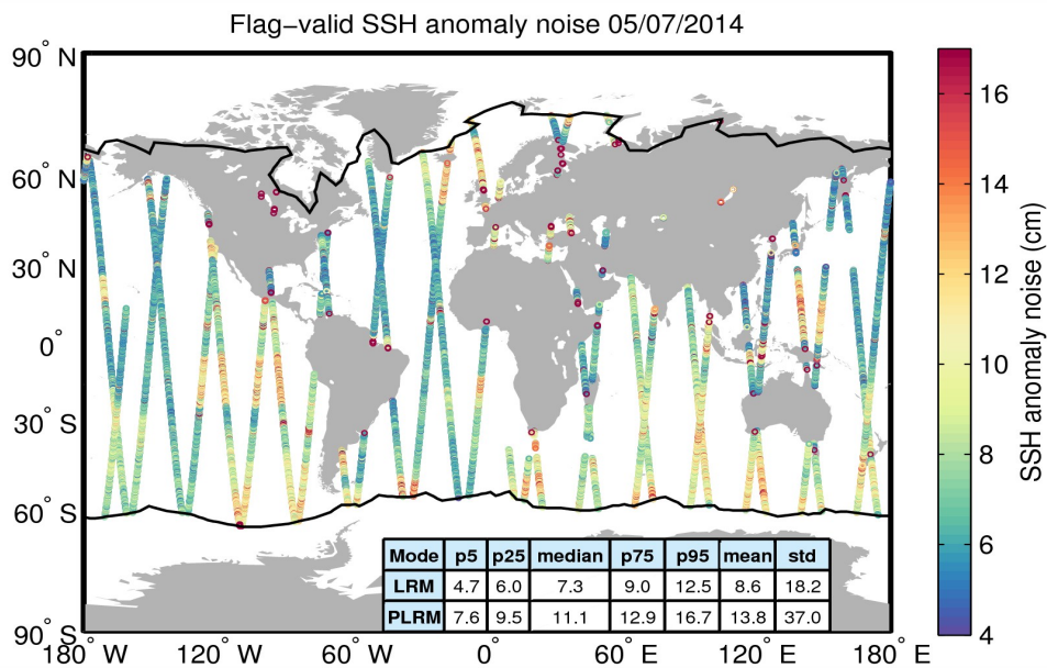
Figure 8. Geographical distribution of flag-valid 20-Hz SSH anomaly measurement noise over oceans and lakes for 05/07/2014. The statistical values shown in the table refer to the SSH anomaly noise and are calculated separately for LRM and PLRM regions. Measurements taken over polar polygons have been excluded from the computation of the statistical values. The black lines mark the outer limit of the Arctic and Antarctic polar polygons.
