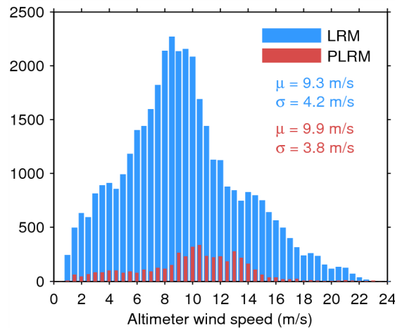
Figure 33. Histogram of flag-valid wind over oceans and lakes for LRM (blue) and PLRM (red) for 05/07/2014. The mean ( \mu ) and standard deviation ( \sigma ) are also shown. Note that values larger than 24 m/s are excluded from the histogram for the sake of readability but not from the computation of \mu and \sigma .
