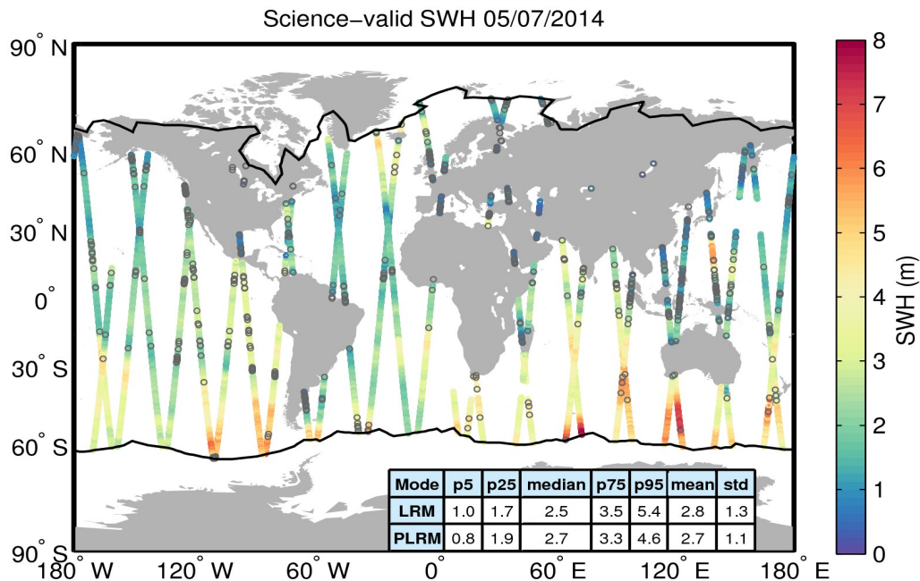
Figure 19. Geographical distribution of science-valid SWH data over oceans and lakes for 05/07/2014. The statistical values shown in the table refer to the SWH in m and are calculated separately for LRM and PLRM regions. The black lines mark the outer limit of the Arctic and Antarctic polar polygons. Gray circles denote records that have been rejected based on the editing criteria described in Table 3.
