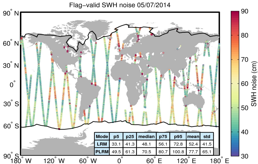
Figure 18. Geographical distribution of flag-valid 20-Hz SWH measurement noise over oceans and lakes for 05/07/2014. The statistical values shown in the table refer to the SWH noise and are calculated separately for LRM and PLRM regions. Measurements taken over polar polygons have been excluded from the computation of the statistical values. The black lines mark the outer limit of the Arctic and Antarctic polar polygons.
