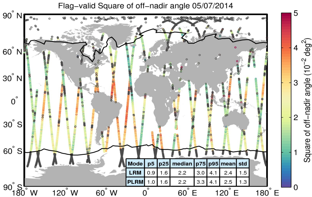
Figure 37. Geographical distribution of flag-valid mispointing data over oceans and lakes for 05/07/2014. The statistical values shown in the table refer to the mispointing in 10^{-2} deg 2 and are calculated separately for LRM and PLRM regions. Measurements taken over polar polygons have been excluded from the computation of the statistical values. The black lines mark the outer limit of the Arctic and Antarctic polar polygons. Gray circles denote negative values.
