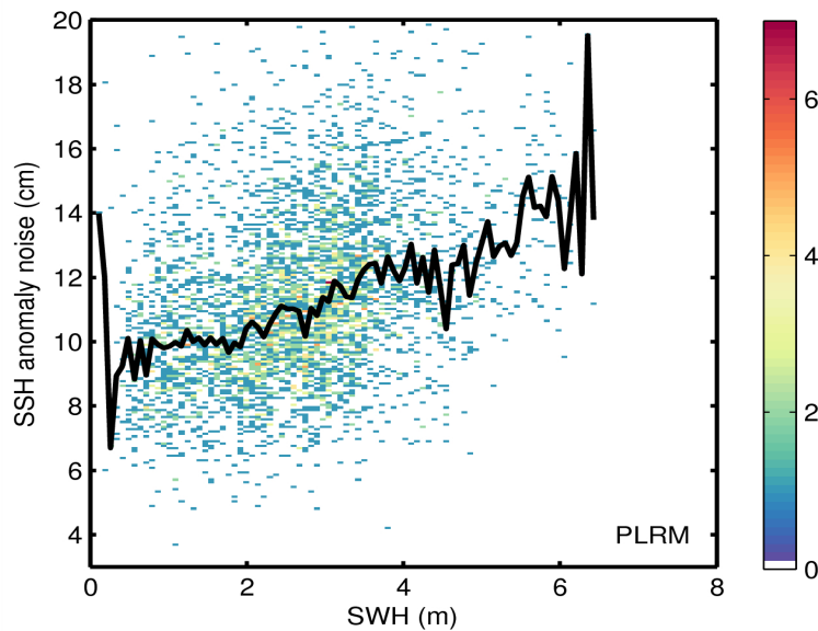
Figure 9. 2D histogram showing flag-valid SSH anomaly noise as a function of SWH for LRM (top) and PLRM (bottom) for 05/07/2014. The black line denotes the median SSH anomaly as a function of SWH.
