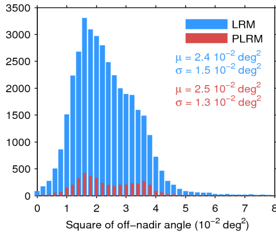
Figure 39. Histogram of flag-valid mispointing over oceans and lakes for LRM (blue) and PLRM (red) for 05/07/2014. Only positive values have been considered. The mean ( \mu ) and standard deviation ( \sigma ) are also shown. Note that values 8 \cdot 10^{-2} \text{ deg}^2 are excluded from the histogram for the sake of readability but not from the computation of \mu and \sigma .
