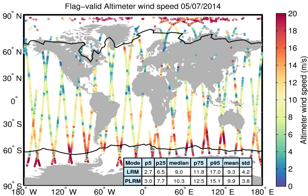
Figure 31. Geographical distribution of flag-valid wind data over oceans and lakes for 05/07/2014. The statistical values shown in the table refer to the wind in m/s and are calculated separately for LRM and PLRM regions. Measurements taken over polar polygons have been excluded from the computation of the statistical values. The black lines mark the outer limit of the Arctic and Antarctic polar polygons.
