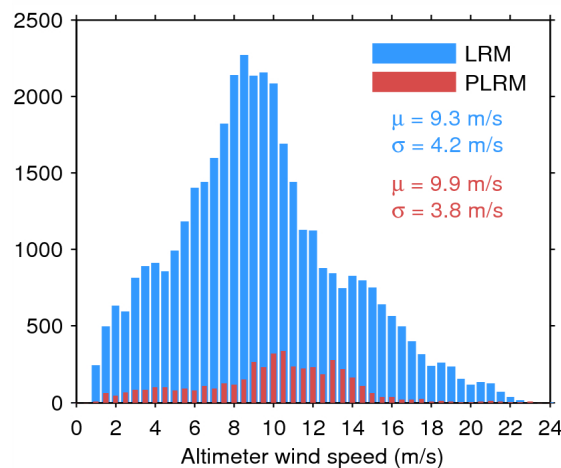
Figure 35. Histogram of science-valid wind over oceans and lakes for LRM (blue) and PLRM (red) for 05/07/2014. The mean ( \mu ) and standard deviation ( \sigma ) are also shown. Note that values larger than 24 m/s are excluded from the histogram for the sake of readability but not from the computation of \mu and \sigma .
