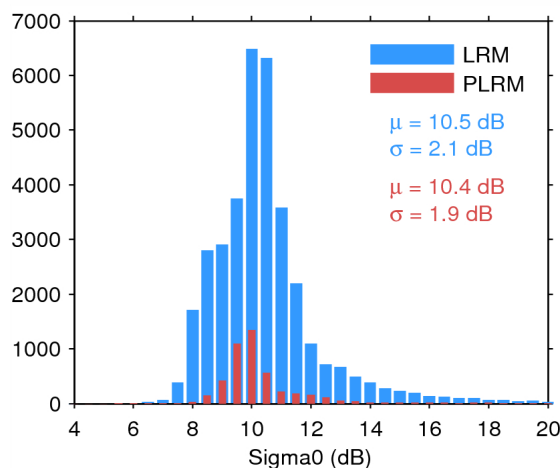
Figure 25. Histogram of flag-valid sigma0 over oceans and lakes for LRM (blue) and PLRM (red) for 04/07/2014. The mean ( \mu ) and standard deviation ( \sigma ) are also shown. Note that values outside [4 20] dB are excluded from the histogram for the sake of readability but not from the computation of \mu and \sigma .
