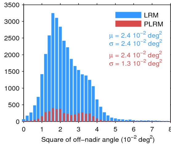
Figure 39. Histogram of flag-valid mispointing over oceans and lakes for LRM (blue) and PLRM (red) for 04/07/2014. Only positive values have been considered. The mean ( \mu ) and standard deviation ( \sigma ) are also shown. Note that values 8 \cdot 10^{-2} \text{ deg}^2 are excluded from the histogram for the sake of readability but not from the computation of \mu and \sigma .
