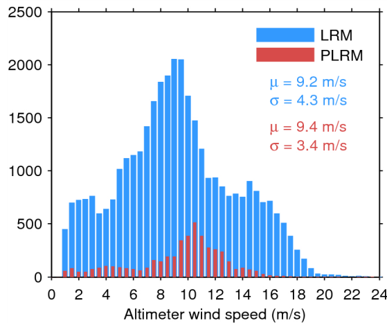
Figure 33. Histogram of flag-valid wind over oceans and lakes for LRM (blue) and PLRM (red) for 04/07/2014. The mean ( \mu ) and standard deviation ( \sigma ) are also shown. Note that values larger than 24 m/s are excluded from the histogram for the sake of readability but not from the computation of \mu and \sigma .
