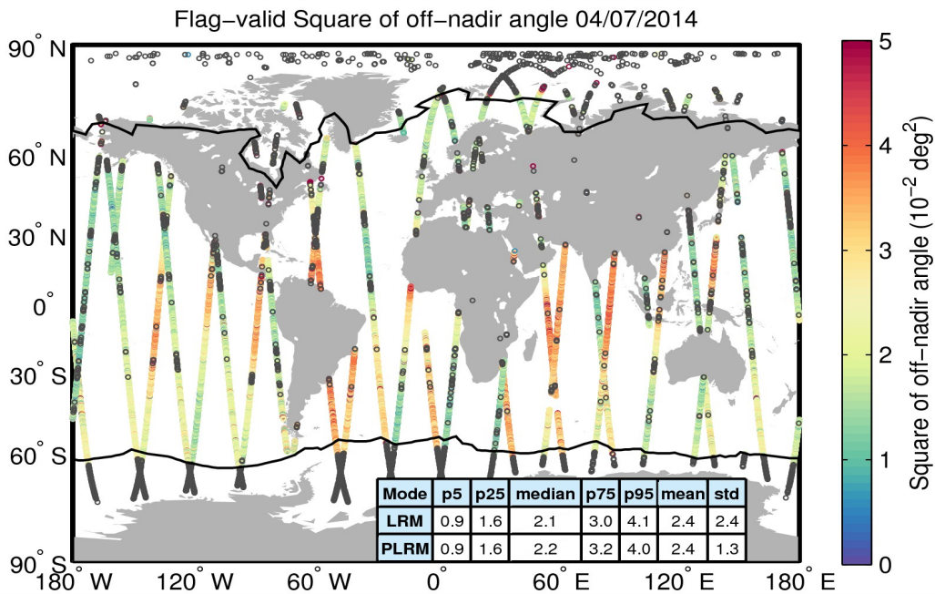
Figure 37. Geographical distribution of flag-valid mispointing data over oceans and lakes for 04/07/2014. The statistical values shown in the table refer to the mispointing in 10^{-2} \text{ deg}^2 and are calculated separately for LRM and PLRM regions. Measurements taken over polar polygons have been excluded from the computation of the statistical values. The black lines mark the outer limit of the Arctic and Antarctic polar polygons. Gray circles denote negative values.
