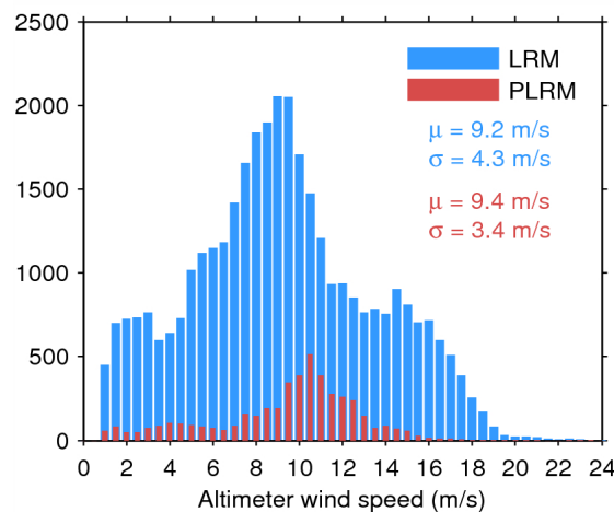
Figure 35. Histogram of science-valid wind over oceans and lakes for LRM (blue) and PLRM (red) for 04/07/2014. The mean ( \mu ) and standard deviation ( \sigma ) are also shown. Note that values larger than 24 m/s are excluded from the histogram for the sake of readability but not from the computation of \mu and \sigma .
