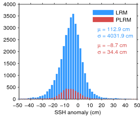
Figure 7. Histogram of flag-valid SSH anomaly over oceans and lakes for LRM (blue) and PLRM (red) for 04/07/2014. The mean ( \mu ) and standard deviation ( \sigma ) are also shown. Note that values outside [-50\ 50] cm are excluded from the histogram for the sake of readability but not from the computation of \mu and \sigma .
