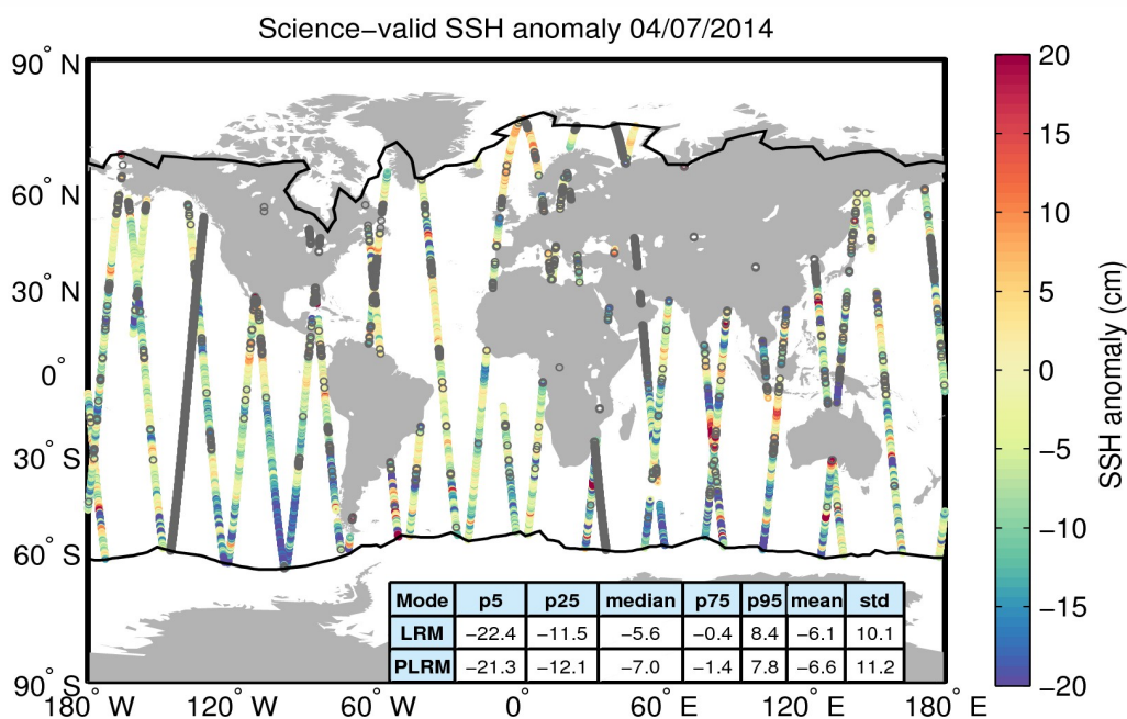
Figure 10. Geographical distribution of science-valid SSH anomaly data over oceans and lakes for 04/07/2014. The statistical values shown in the table refer to the SSH anomaly in cm and are calculated separately for LRM and PLRM regions. The black lines mark the outer limit of the Arctic and Antarctic polar polygons. Gray circles denote records that have been rejected based on the editing criteria described in Table 2.
