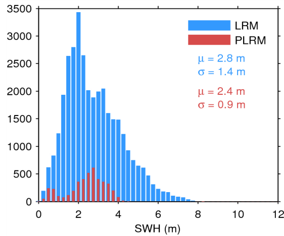
Figure 20. Histogram of science-valid SWH over oceans and lakes for LRM (blue) and PLRM (red) for 04/07/2014. The mean ( \mu ) and standard deviation ( \sigma ) are also shown. Note that values larger than 12 m are excluded from the histogram for the sake of readability but not from the computation of \mu and \sigma .
