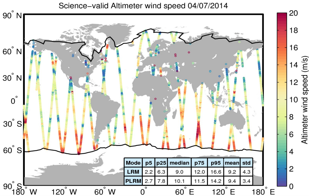
Figure 34. Geographical distribution of science-valid wind data over oceans and lakes for 04/07/2014. The statistical values shown in the table refer to the wind in m/s and are calculated separately for LRM and PLRM regions. The black lines mark the outer limit of the Arctic and Antarctic polar polygons. Gray circles denote records that have been rejected based on the editing criteria described in Table 5.
