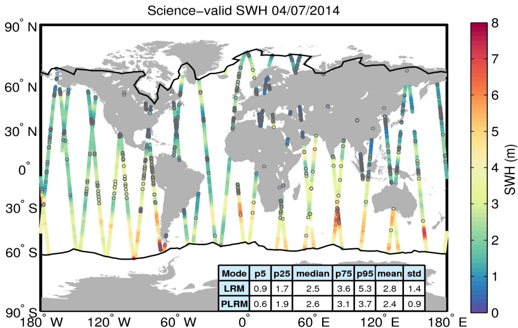
Figure 19. Geographical distribution of science-valid SWH data over oceans and lakes for 04/07/2014. The statistical values shown in the table refer to the SWH in m and are calculated separately for LRM and PLRM regions. The black lines mark the outer limit of the Arctic and Antarctic polar polygons. Gray circles denote records that have been rejected based on the editing criteria described in Table 3.
