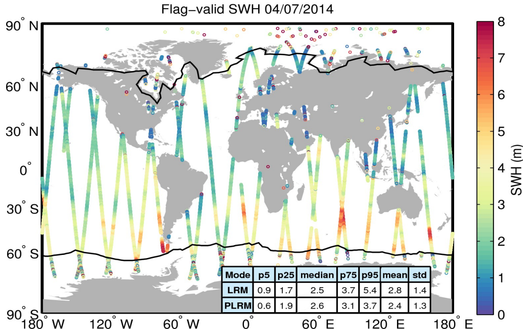
Figure 15. Geographical distribution of flag-valid SWH data over oceans and lakes for 04/07/2014. The statistical values shown in the table refer to the SWH in m and are calculated separately for LRM and PLRM regions. Measurements taken over polar polygons have been excluded from the computation of the statistical values. The black lines mark the outer limit of the Arctic and Antarctic polar polygons.
