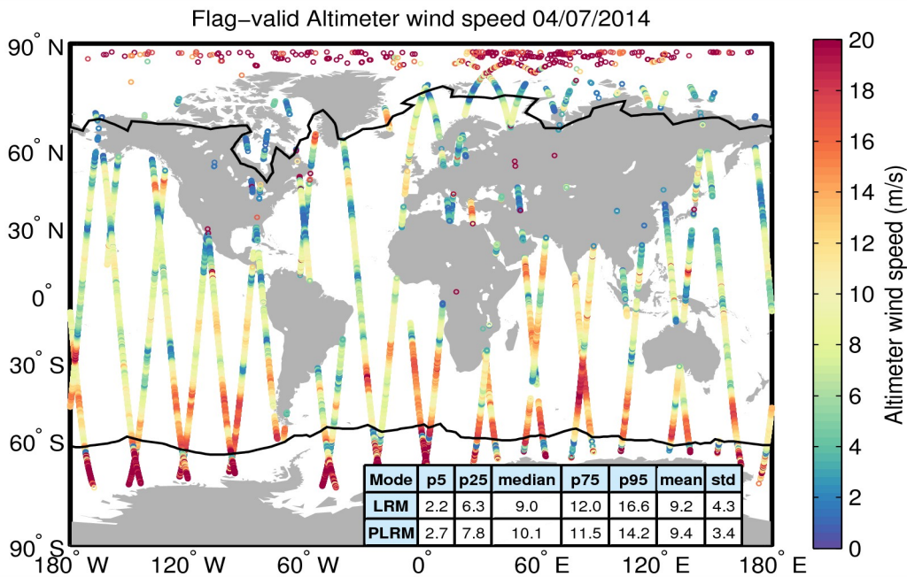
Figure 31. Geographical distribution of flag-valid wind data over oceans and lakes for 04/07/2014. The statistical values shown in the table refer to the wind in m/s and are calculated separately for LRM and PLRM regions. Measurements taken over polar polygons have been excluded from the computation of the statistical values. The black lines mark the outer limit of the Arctic and Antarctic polar polygons.
