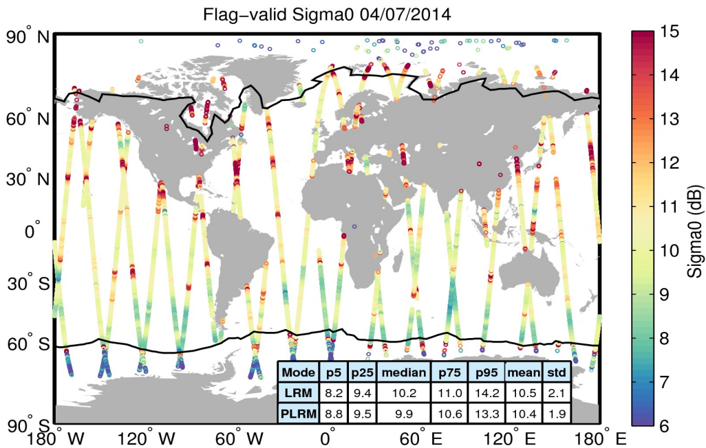
Figure 23. Geographical distribution of flag-valid sigma0 data over oceans and lakes for 04/07/2014. The statistical values shown in the table refer to the sigma0 in dB and are calculated separately for LRM and PLRM regions. Measurements taken over polar polygons have been excluded from the computation of the statistical values. The black lines mark the outer limit of the Arctic and Antarctic polar polygons.
