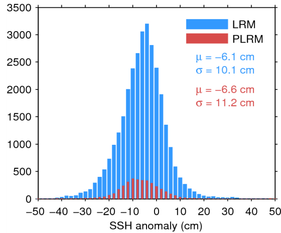
Figure 11. Histogram of science-valid SSH anomaly over oceans and lakes for LRM (blue) and PLRM (red) for 04/07/2014. The mean ( \mu ) and standard deviation ( \sigma ) are also shown. Note that values outside [-50\ 50] cm are excluded from the histogram for the sake of readability but not from the computation of \mu and \sigma .
