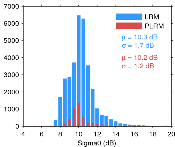
Figure 28. Histogram of science-valid sigma0 over oceans and lakes for LRM (blue) and PLRM (red) for 04/07/2014. The mean ( \mu ) and standard deviation ( \sigma ) are also shown. Note that values outside [4 20] dB are excluded from the histogram for the sake of readability but not from the computation of \mu and \sigma .
