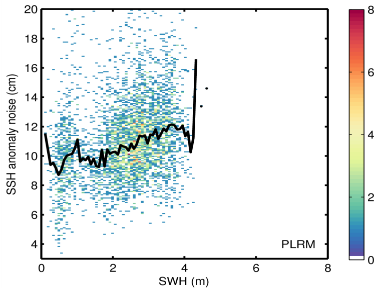
Figure 9. 2D histogram showing flag-valid SSH anomaly noise as a function of SWH for LRM (top) and PLRM (bottom) for 04/07/2014. The black line denotes the median SSH anomaly as a function of SWH.
