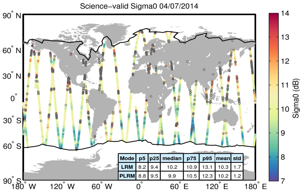
Figure 27. Geographical distribution of science-valid sigma0 data over oceans and lakes for 04/07/2014. The statistical values shown in the table refer to the sigma0 in dB and are calculated separately for LRM and PLRM regions. The black lines mark the outer limit of the Arctic and Antarctic polar polygons. Gray circles denote records that have been rejected based on the editing criteria described in Table 4.
