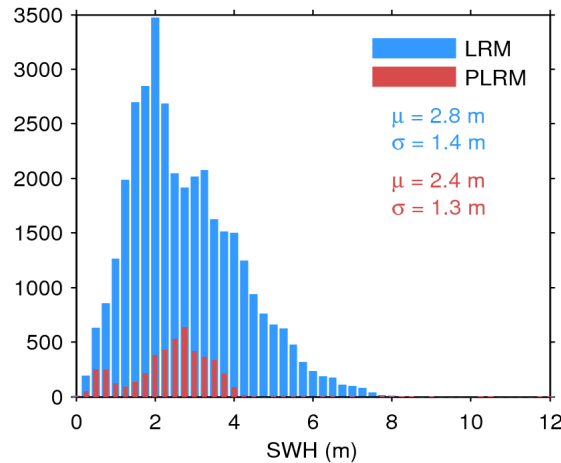
Figure 17. Histogram of flag-valid SWH over oceans and lakes for LRM (blue) and PLRM (red) for 04/07/2014. The mean ( \mu ) and standard deviation ( \sigma ) are also shown. Note that values larger than 12 m are excluded from the histogram for the sake of readability but not from the computation of \mu and \sigma .
