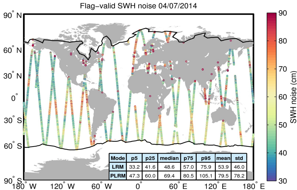
Figure 18. Geographical distribution of flag-valid 20-Hz SWH measurement noise over oceans and lakes for 04/07/2014. The statistical values shown in the table refer to the SWH noise and are calculated separately for LRM and PLRM regions. Measurements taken over polar polygons have been excluded from the computation of the statistical values. The black lines mark the outer limit of the Arctic and Antarctic polar polygons.
