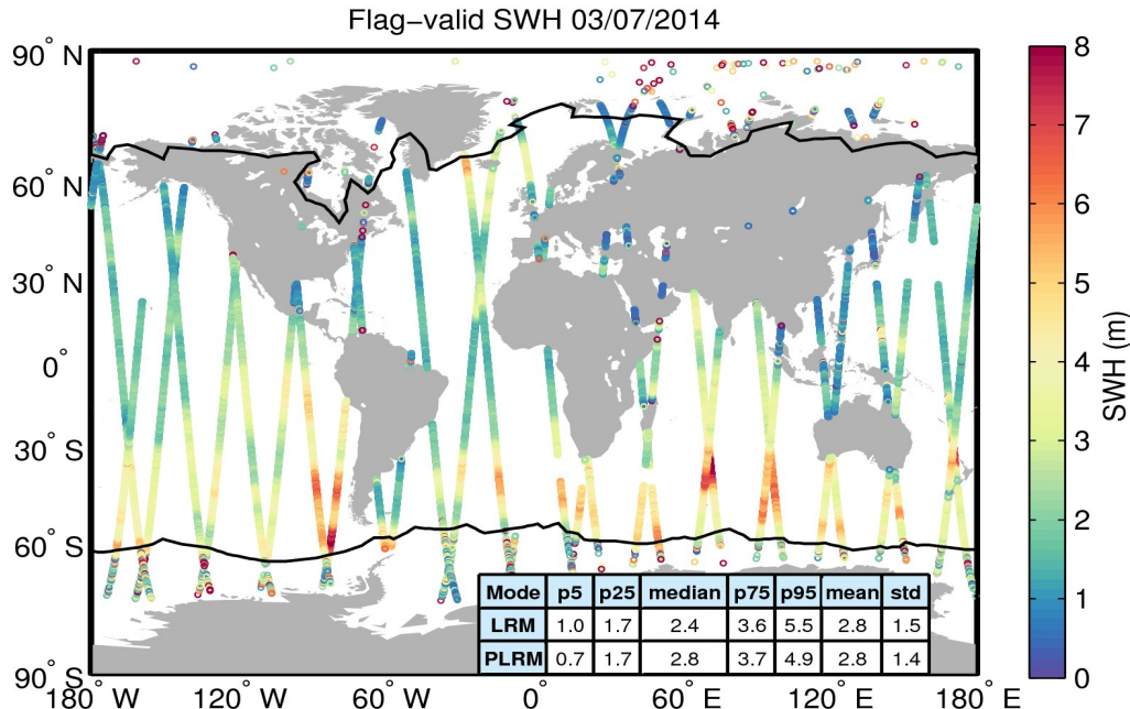
Figure 15. Geographical distribution of flag-valid SWH data over oceans and lakes for 03/07/2014. The statistical values shown in the table refer to the SWH in m and are calculated separately for LRM and PLRM regions. Measurements taken over polar polygons have been excluded from the computation of the statistical values. The black lines mark the outer limit of the Arctic and Antarctic polar polygons.
