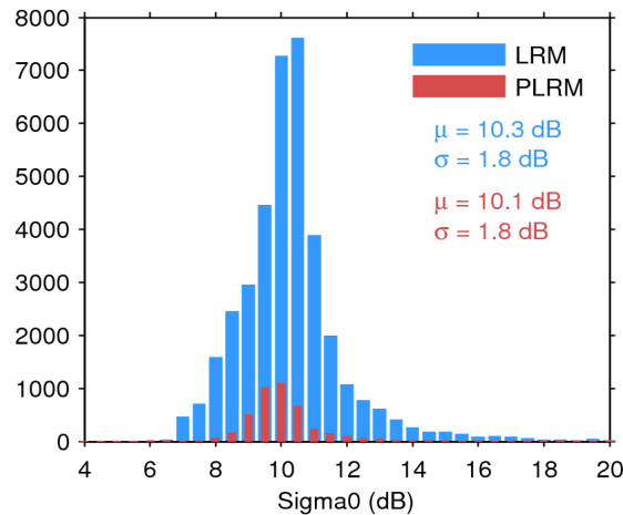
Figure 25. Histogram of flag-valid sigma0 over oceans and lakes for LRM (blue) and PLRM (red) for 03/07/2014. The mean ( \mu ) and standard deviation ( \sigma ) are also shown. Note that values outside [4 20] dB are excluded from the histogram for the sake of readability but not from the computation of \mu and \sigma .
