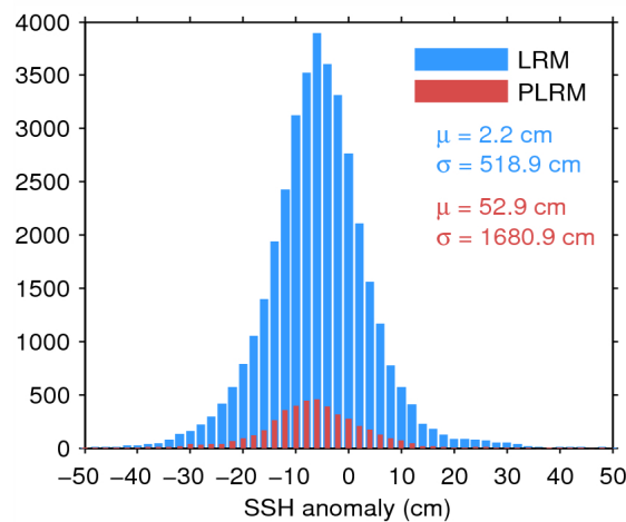
Figure 7. Histogram of flag-valid SSH anomaly over oceans and lakes for LRM (blue) and PLRM (red) for 03/07/2014. The mean ( \mu ) and standard deviation ( \sigma ) are also shown. Note that values outside [-50\ 50] cm are excluded from the histogram for the sake of readability but not from the computation of \mu and \sigma .
