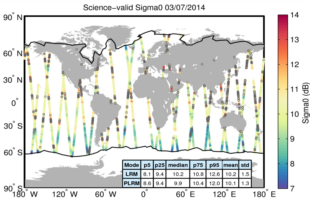
Figure 27. Geographical distribution of science-valid sigma0 data over oceans and lakes for 03/07/2014. The statistical values shown in the table refer to the sigma0 in dB and are calculated separately for LRM and PLRM regions. The black lines mark the outer limit of the Arctic and Antarctic polar polygons. Gray circles denote records that have been rejected based on the editing criteria described in Table 4.
