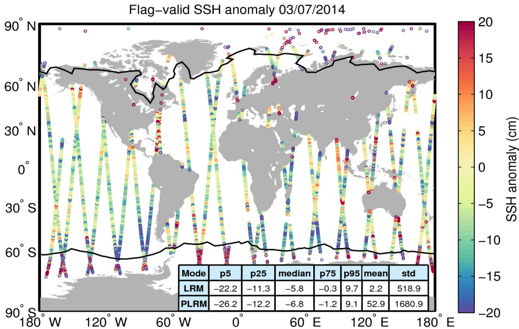
Figure 5. Geographical distribution of flag-valid 1-Hz SSH anomaly data over oceans and lakes for 03/07/2014. The statistical values shown in the table refer to the SSH anomaly in cm and are calculated separately for LRM and PLRM regions. Measurements taken over polar polygons have been excluded from the computation of the statistical values. The black lines mark the outer limit of the Arctic and Antarctic polar polygons.
