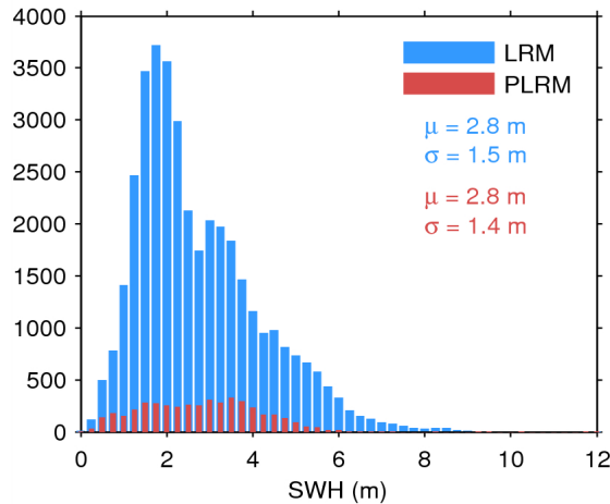
Figure 17. Histogram of flag-valid SWH over oceans and lakes for LRM (blue) and PLRM (red) for 03/07/2014. The mean ( \mu ) and standard deviation ( \sigma ) are also shown. Note that values larger than 12 m are excluded from the histogram for the sake of readability but not from the computation of \mu and \sigma .
