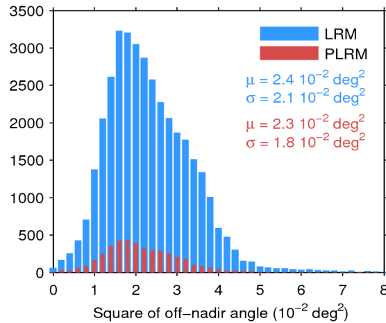
Figure 39. Histogram of flag-valid mispointing over oceans and lakes for LRM (blue) and PLRM (red) for 03/07/2014. Only positive values have been considered. The mean ( \mu ) and standard deviation ( \sigma ) are also shown. Note that values 8 \cdot 10^{-2} \text{ deg}^2 are excluded from the histogram for the sake of readability but not from the computation of \mu and \sigma .
