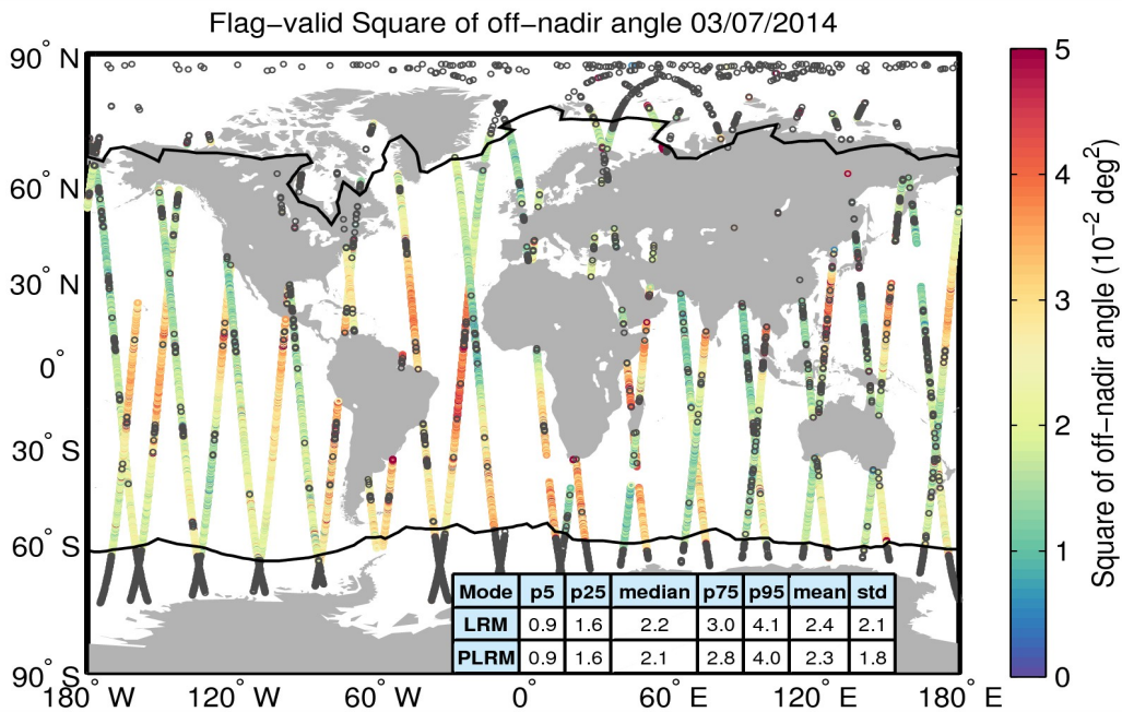
Figure 37. Geographical distribution of flag-valid mispointing data over oceans and lakes for 03/07/2014. The statistical values shown in the table refer to the mispointing in 10^{-2} \text{ deg}^2 and are calculated separately for LRM and PLRM regions. Measurements taken over polar polygons have been excluded from the computation of the statistical values. The black lines mark the outer limit of the Arctic and Antarctic polar polygons. Gray circles denote negative values.
