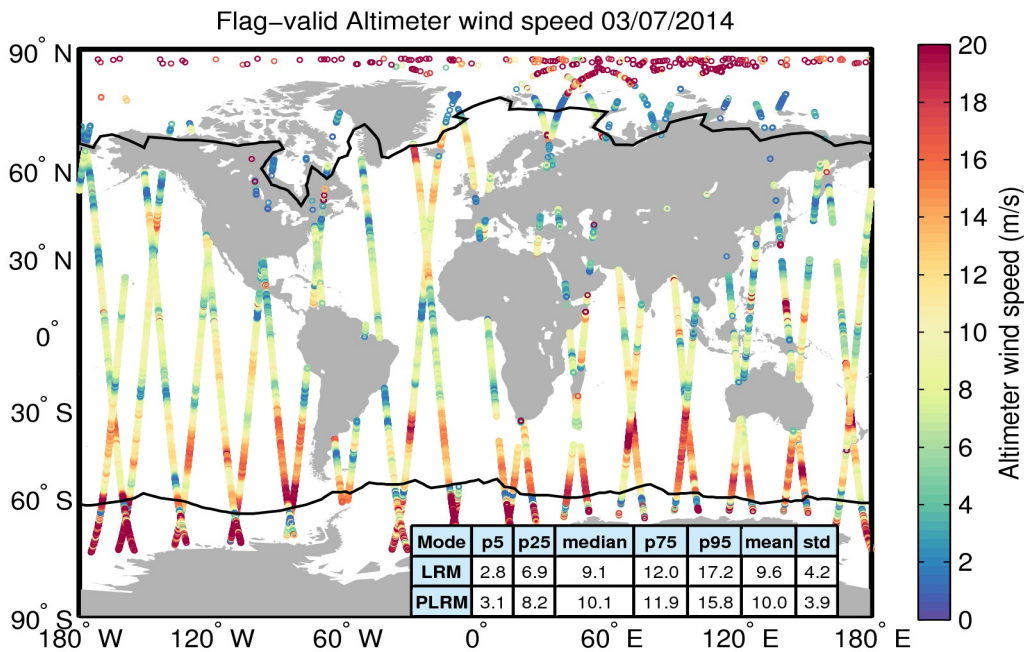
Figure 31. Geographical distribution of flag-valid wind data over oceans and lakes for 03/07/2014. The statistical values shown in the table refer to the wind in m/s and are calculated separately for LRM and PLRM regions. Measurements taken over polar polygons have been excluded from the computation of the statistical values. The black lines mark the outer limit of the Arctic and Antarctic polar polygons.
