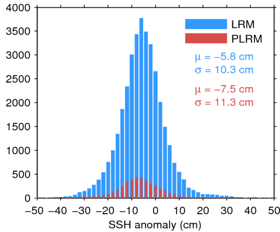
Figure 11. Histogram of science-valid SSH anomaly over oceans and lakes for LRM (blue) and PLRM (red) for 03/07/2014. The mean ( \mu ) and standard deviation ( \sigma ) are also shown. Note that values outside [-50 50] cm are excluded from the histogram for the sake of readability but not from the computation of \mu and \sigma .
