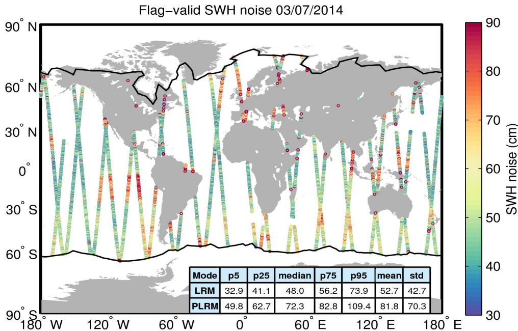
Figure 18. Geographical distribution of flag-valid 20-Hz SWH measurement noise over oceans and lakes for 03/07/2014. The statistical values shown in the table refer to the SWH noise and are calculated separately for LRM and PLRM regions. Measurements taken over polar polygons have been excluded from the computation of the statistical values. The black lines mark the outer limit of the Arctic and Antarctic polar polygons.
