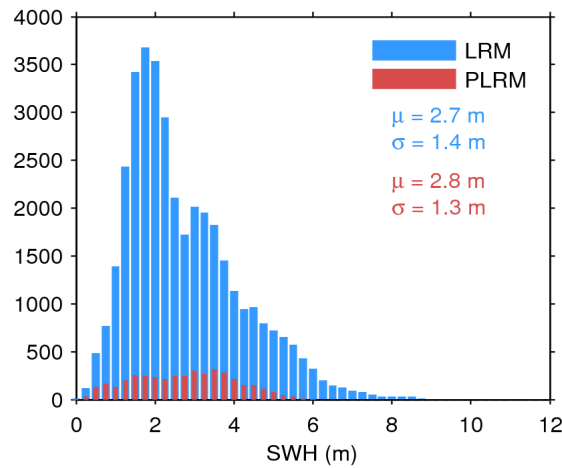
Figure 20. Histogram of science-valid SWH over oceans and lakes for LRM (blue) and PLRM (red) for 03/07/2014. The mean ( \mu ) and standard deviation ( \sigma ) are also shown. Note that values larger than 12 m are excluded from the histogram for the sake of readability but not from the computation of \mu and \sigma .
