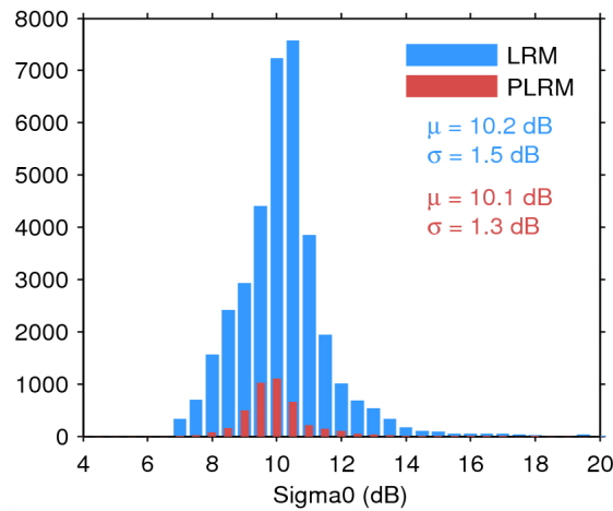
Figure 28. Histogram of science-valid sigma0 over oceans and lakes for LRM (blue) and PLRM (red) for 03/07/2014. The mean ( \mu ) and standard deviation ( \sigma ) are also shown. Note that values outside [4 20] dB are excluded from the histogram for the sake of readability but not from the computation of \mu and \sigma .
