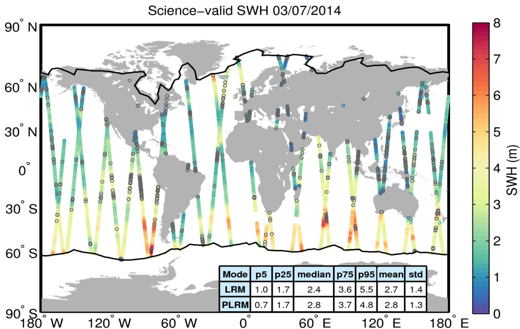
Figure 19. Geographical distribution of science-valid SWH data over oceans and lakes for 03/07/2014. The statistical values shown in the table refer to the SWH in m and are calculated separately for LRM and PLRM regions. The black lines mark the outer limit of the Arctic and Antarctic polar polygons. Gray circles denote records that have been rejected based on the editing criteria described in Table 3.
