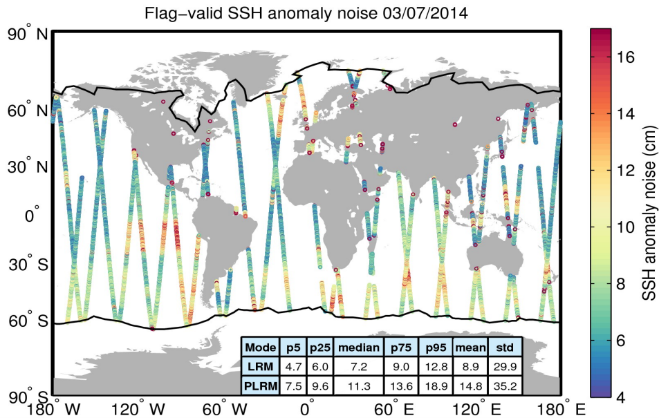
Figure 8. Geographical distribution of flag-valid 20-Hz SSH anomaly measurement noise over oceans and lakes for 03/07/2014. The statistical values shown in the table refer to the SSH anomaly noise and are calculated separately for LRM and PLRM regions. Measurements taken over polar polygons have been excluded from the computation of the statistical values. The black lines mark the outer limit of the Arctic and Antarctic polar polygons.
