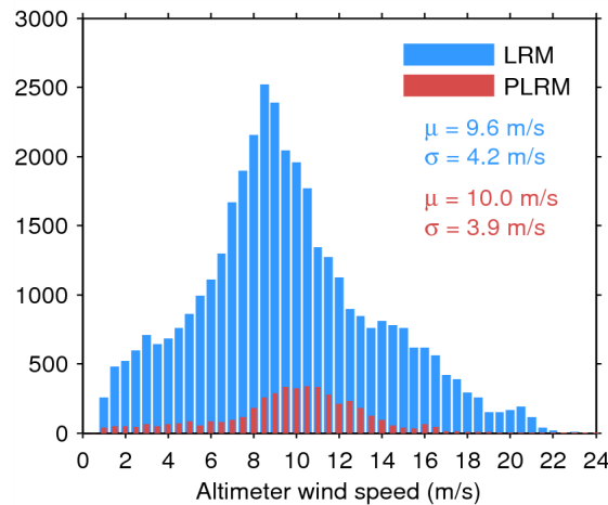
Figure 33. Histogram of flag-valid wind over oceans and lakes for LRM (blue) and PLRM (red) for 03/07/2014. The mean ( \mu ) and standard deviation ( \sigma ) are also shown. Note that values larger than 24 m/s are excluded from the histogram for the sake of readability but not from the computation of \mu and \sigma .
