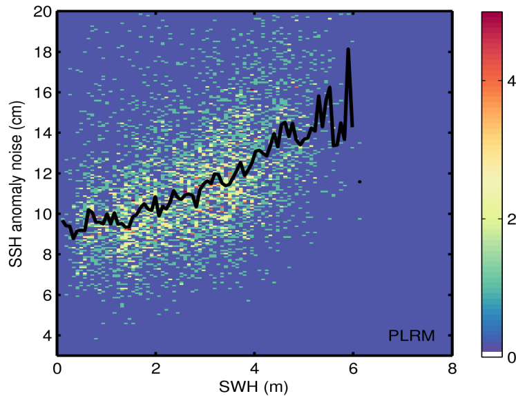
Figure 9. 2D histogram showing flag-valid SSH anomaly noise as a function of SWH for LRM (top) and PLRM (bottom) for 03/07/2014. The black line denotes the median SSH anomaly as a function of SWH.
