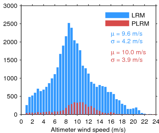
Figure 35. Histogram of science-valid wind over oceans and lakes for LRM (blue) and PLRM (red) for 03/07/2014. The mean ( \mu ) and standard deviation ( \sigma ) are also shown. Note that values larger than 24 m/s are excluded from the histogram for the sake of readability but not from the computation of \mu and \sigma .
