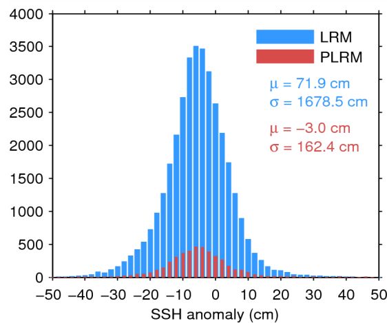
Figure 7. Histogram of flag-valid SSH anomaly over oceans and lakes for LRM (blue) and PLRM (red) for 02/07/2014. The mean ( \mu ) and standard deviation ( \sigma ) are also shown. Note that values outside [-50\ 50] cm are excluded from the histogram for the sake of readability but not from the computation of \mu and \sigma .
