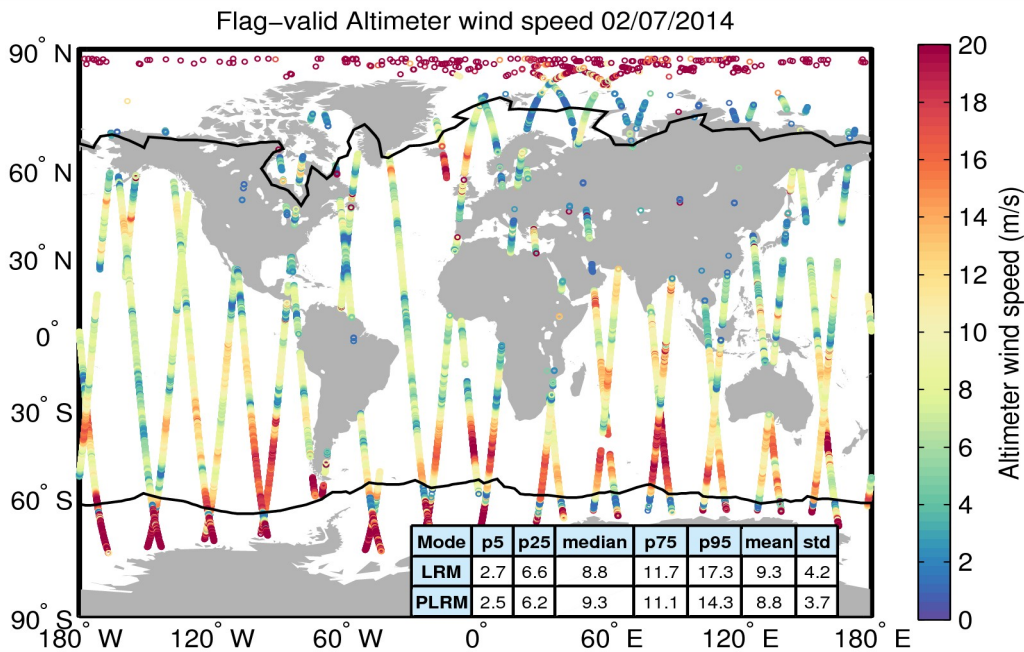
Figure 31. Geographical distribution of flag-valid wind data over oceans and lakes for 02/07/2014. The statistical values shown in the table refer to the wind in m/s and are calculated separately for LRM and PLRM regions. Measurements taken over polar polygons have been excluded from the computation of the statistical values. The black lines mark the outer limit of the Arctic and Antarctic polar polygons.
