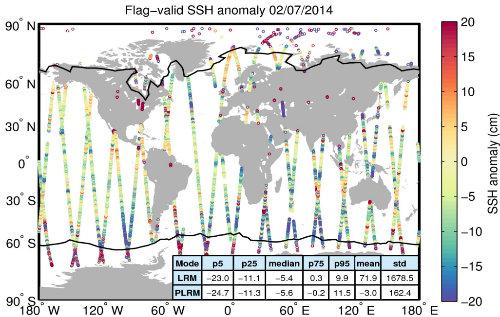
Figure 5. Geographical distribution of flag-valid 1-Hz SSH anomaly data over oceans and lakes for 02/07/2014. The statistical values shown in the table refer to the SSH anomaly in cm and are calculated separately for LRM and PLRM regions. Measurements taken over polar polygons have been excluded from the computation of the statistical values. The black lines mark the outer limit of the Arctic and Antarctic polar polygons.
