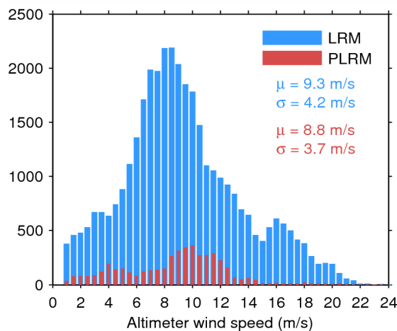
Figure 35. Histogram of science-valid wind over oceans and lakes for LRM (blue) and PLRM (red) for 02/07/2014. The mean ( \mu ) and standard deviation ( \sigma ) are also shown. Note that values larger than 24 m/s are excluded from the histogram for the sake of readability but not from the computation of \mu and \sigma .
