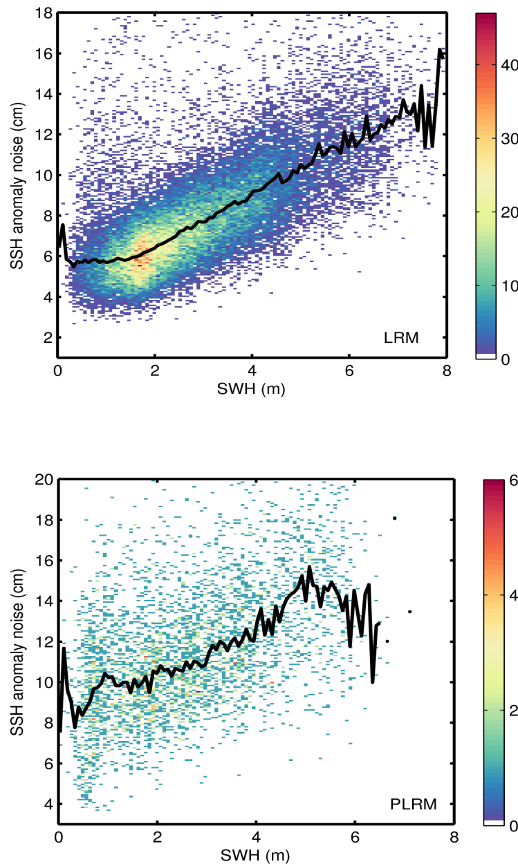
Figure 9. 2D histogram showing flag-valid SSH anomaly noise as a function of SWH for LRM (top) and PLRM (bottom) for 02/07/2014. The black line denotes the median SSH anomaly as a function of SWH.
