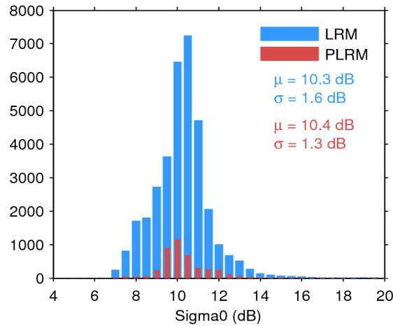
Figure 28. Histogram of science-valid sigma0 over oceans and lakes for LRM (blue) and PLRM (red) for 02/07/2014. The mean ( \mu ) and standard deviation ( \sigma ) are also shown. Note that values outside [4 20] dB are excluded from the histogram for the sake of readability but not from the computation of \mu and \sigma .
