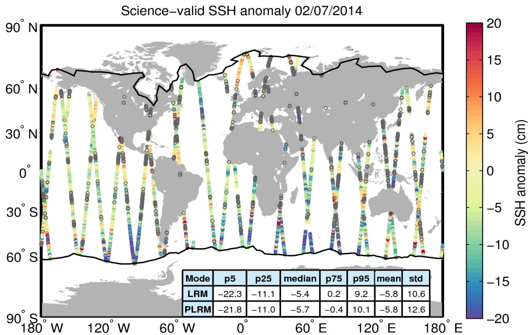
Figure 10. Geographical distribution of science-valid SSH anomaly data over oceans and lakes for 02/07/2014. The statistical values shown in the table refer to the SSH anomaly in cm and are calculated separately for LRM and PLRM regions. The black lines mark the outer limit of the Arctic and Antarctic polar polygons. Gray circles denote records that have been rejected based on the editing criteria described in Table 2.
