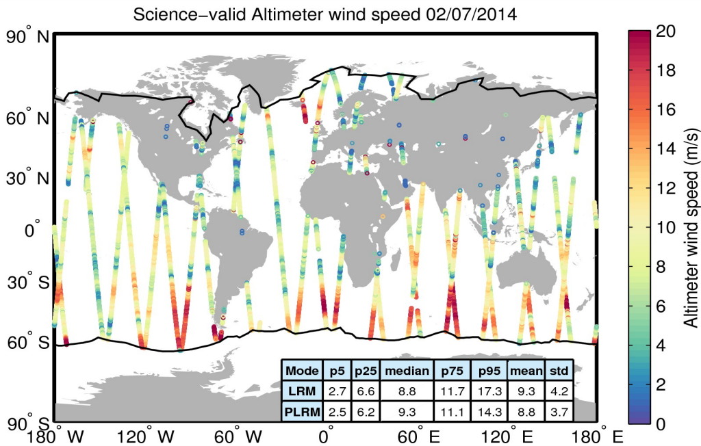
Figure 34. Geographical distribution of science-valid wind data over oceans and lakes for 02/07/2014. The statistical values shown in the table refer to the wind in m/s and are calculated separately for LRM and PLRM regions. The black lines mark the outer limit of the Arctic and Antarctic polar polygons. Gray circles denote records that have been rejected based on the editing criteria described in Table 5.
