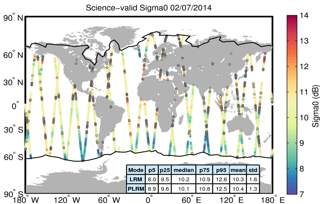
Figure 27. Geographical distribution of science-valid sigma0 data over oceans and lakes for 02/07/2014. The statistical values shown in the table refer to the sigma0 in dB and are calculated separately for LRM and PLRM regions. The black lines mark the outer limit of the Arctic and Antarctic polar polygons. Gray circles denote records that have been rejected based on the editing criteria described in Table 4.
