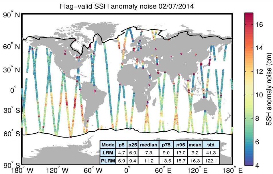
Figure 8. Geographical distribution of flag-valid 20-Hz SSH anomaly measurement noise over oceans and lakes for 02/07/2014. The statistical values shown in the table refer to the SSH anomaly noise and are calculated separately for LRM and PLRM regions. Measurements taken over polar polygons have been excluded from the computation of the statistical values. The black lines mark the outer limit of the Arctic and Antarctic polar polygons.
