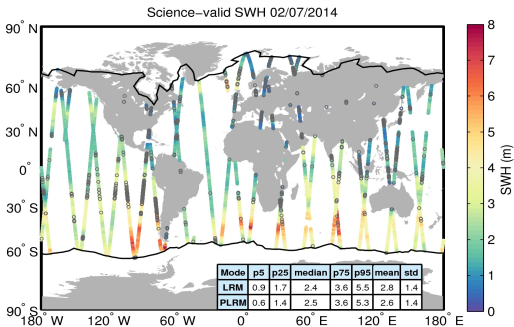
Figure 19. Geographical distribution of science-valid SWH data over oceans and lakes for 02/07/2014. The statistical values shown in the table refer to the SWH in m and are calculated separately for LRM and PLRM regions. The black lines mark the outer limit of the Arctic and Antarctic polar polygons. Gray circles denote records that have been rejected based on the editing criteria described in Table 3.
