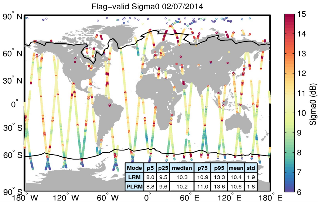
Figure 23. Geographical distribution of flag-valid sigma0 data over oceans and lakes for 02/07/2014. The statistical values shown in the table refer to the sigma0 in dB and are calculated separately for LRM and PLRM regions. Measurements taken over polar polygons have been excluded from the computation of the statistical values. The black lines mark the outer limit of the Arctic and Antarctic polar polygons.
