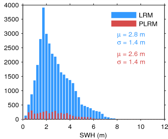
Figure 20. Histogram of science-valid SWH over oceans and lakes for LRM (blue) and PLRM (red) for 02/07/2014. The mean ( \mu ) and standard deviation ( \sigma ) are also shown. Note that values larger than 12 m are excluded from the histogram for the sake of readability but not from the computation of \mu and \sigma .
