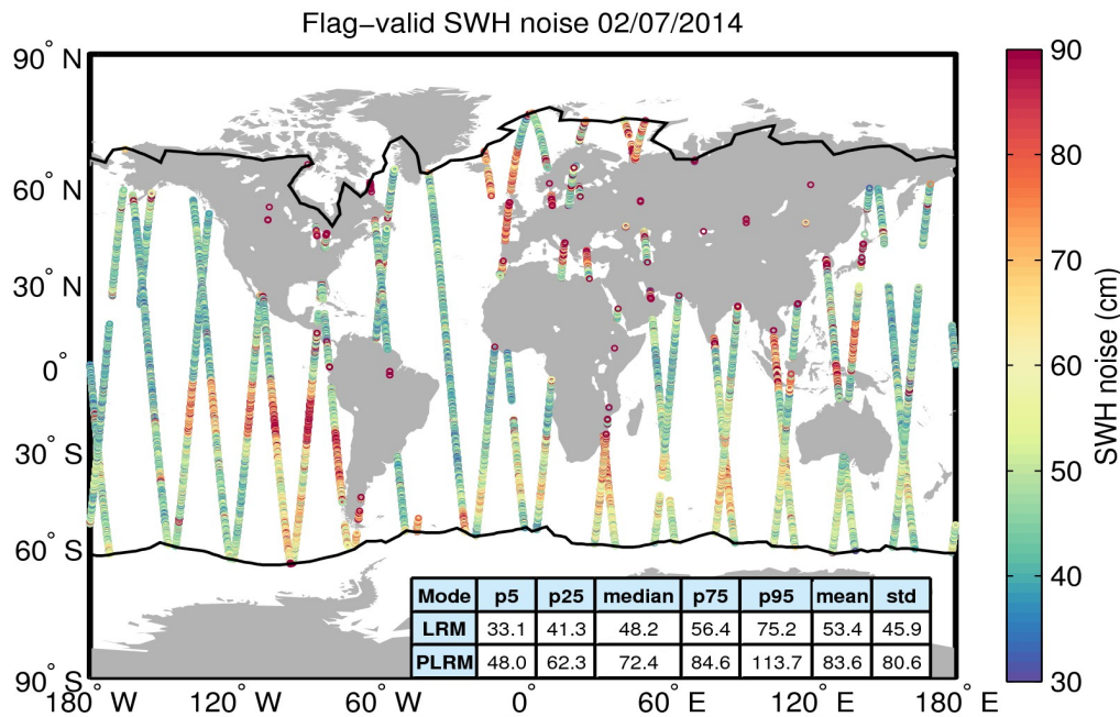
Figure 18. Geographical distribution of flag-valid 20-Hz SWH measurement noise over oceans and lakes for 02/07/2014. The statistical values shown in the table refer to the SWH noise and are calculated separately for LRM and PLRM regions. Measurements taken over polar polygons have been excluded from the computation of the statistical values. The black lines mark the outer limit of the Arctic and Antarctic polar polygons.
