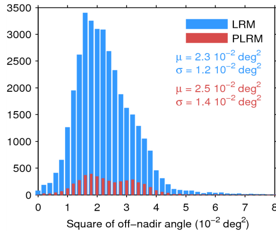
Figure 39. Histogram of flag-valid mispointing over oceans and lakes for LRM (blue) and PLRM (red) for 02/07/2014. Only positive values have been considered. The mean ( \mu ) and standard deviation ( \sigma ) are also shown. Note that values 8 \cdot 10^{-2} \text{ deg}^2 are excluded from the histogram for the sake of readability but not from the computation of \mu and \sigma .
