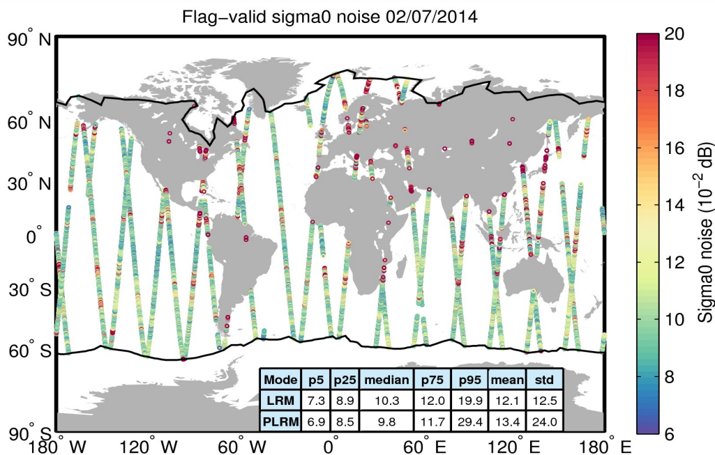
Figure 26. Geographical distribution of flag-valid 20-Hz sigma0 measurement noise over oceans and lakes for 02/07/2014. The statistical values shown in the table refer to the sigma0 noise and are calculated separately for LRM and PLRM regions. Measurements taken over polar polygons have been excluded from the computation of the statistical values. The black lines mark the outer limit of the Arctic and Antarctic polar polygons.
