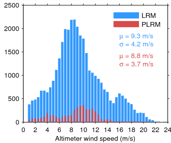
Figure 33. Histogram of flag-valid wind over oceans and lakes for LRM (blue) and PLRM (red) for 02/07/2014. The mean ( \mu ) and standard deviation ( \sigma ) are also shown. Note that values larger than 24 m/s are excluded from the histogram for the sake of readability but not from the computation of \mu and \sigma .
