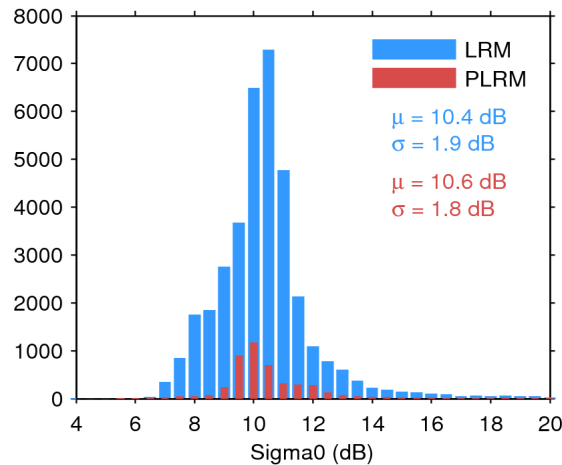
Figure 25. Histogram of flag-valid sigma0 over oceans and lakes for LRM (blue) and PLRM (red) for 02/07/2014. The mean ( \mu ) and standard deviation ( \sigma ) are also shown. Note that values outside [4 20] dB are excluded from the histogram for the sake of readability but not from the computation of \mu and \sigma .
