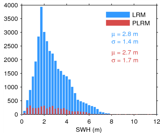
Figure 17. Histogram of flag-valid SWH over oceans and lakes for LRM (blue) and PLRM (red) for 02/07/2014. The mean ( \mu ) and standard deviation ( \sigma ) are also shown. Note that values larger than 12 m are excluded from the histogram for the sake of readability but not from the computation of \mu and \sigma .
