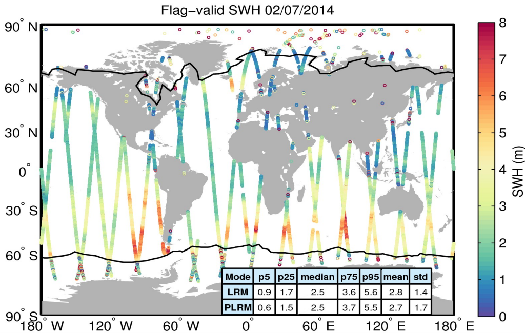
Figure 15. Geographical distribution of flag-valid SWH data over oceans and lakes for 02/07/2014. The statistical values shown in the table refer to the SWH in m and are calculated separately for LRM and PLRM regions. Measurements taken over polar polygons have been excluded from the computation of the statistical values. The black lines mark the outer limit of the Arctic and Antarctic polar polygons.
