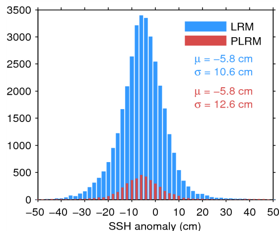
Figure 11. Histogram of science-valid SSH anomaly over oceans and lakes for LRM (blue) and PLRM (red) for 02/07/2014. The mean ( \mu ) and standard deviation ( \sigma ) are also shown. Note that values outside [-50 50] cm are excluded from the histogram for the sake of readability but not from the computation of \mu and \sigma .
