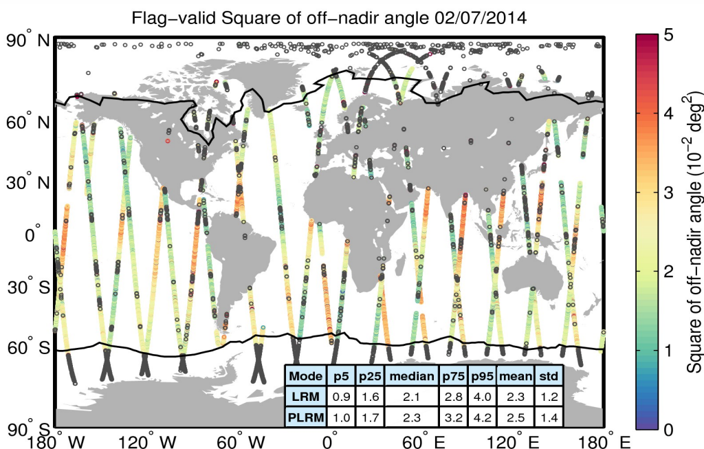
Figure 37. Geographical distribution of flag-valid mispointing data over oceans and lakes for 02/07/2014. The statistical values shown in the table refer to the mispointing in 10^{-2} \text{ deg}^2 and are calculated separately for LRM and PLRM regions. Measurements taken over polar polygons have been excluded from the computation of the statistical values. The black lines mark the outer limit of the Arctic and Antarctic polar polygons. Gray circles denote negative values.
