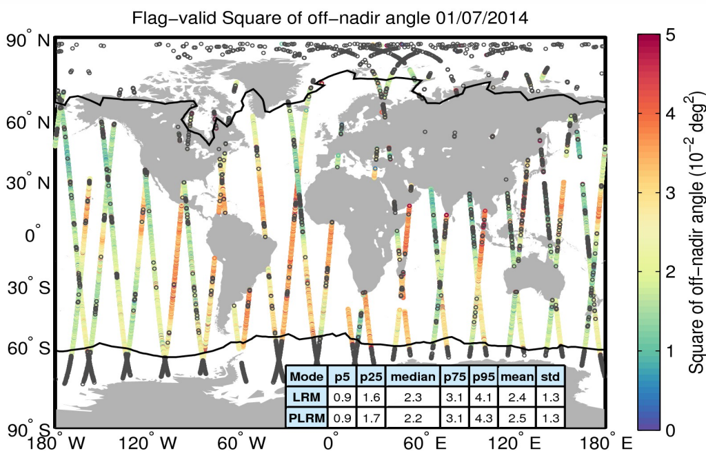
Figure 37. Geographical distribution of flag-valid mispointing data over oceans and lakes for 01/07/2014. The statistical values shown in the table refer to the mispointing in 10^{-2} \text{ deg}^2 and are calculated separately for LRM and PLRM regions. Measurements taken over polar polygons have been excluded from the computation of the statistical values. The black lines mark the outer limit of the Arctic and Antarctic polar polygons. Gray circles denote negative values.
