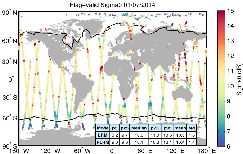
Figure 23. Geographical distribution of flag-valid sigma0 data over oceans and lakes for 01/07/2014. The statistical values shown in the table refer to the sigma0 in dB and are calculated separately for LRM and PLRM regions. Measurements taken over polar polygons have been excluded from the computation of the statistical values. The black lines mark the outer limit of the Arctic and Antarctic polar polygons.
