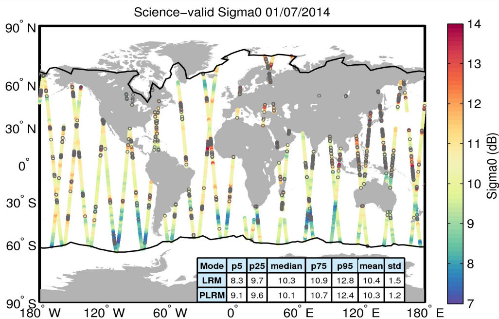
Figure 27. Geographical distribution of science-valid sigma0 data over oceans and lakes for 01/07/2014. The statistical values shown in the table refer to the sigma0 in dB and are calculated separately for LRM and PLRM regions. The black lines mark the outer limit of the Arctic and Antarctic polar polygons. Gray circles denote records that have been rejected based on the editing criteria described in Table 4.
