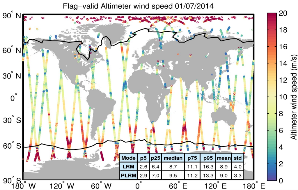
Figure 31. Geographical distribution of flag-valid wind data over oceans and lakes for 01/07/2014. The statistical values shown in the table refer to the wind in m/s and are calculated separately for LRM and PLRM regions. Measurements taken over polar polygons have been excluded from the computation of the statistical values. The black lines mark the outer limit of the Arctic and Antarctic polar polygons.
