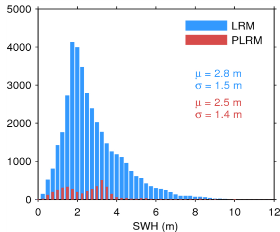
Figure 17. Histogram of flag-valid SWH over oceans and lakes for LRM (blue) and PLRM (red) for 01/07/2014. The mean ( \mu ) and standard deviation ( \sigma ) are also shown. Note that values larger than 12 m are excluded from the histogram for the sake of readability but not from the computation of \mu and \sigma .
