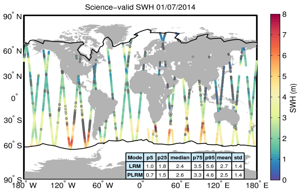
Figure 19. Geographical distribution of science-valid SWH data over oceans and lakes for 01/07/2014. The statistical values shown in the table refer to the SWH in m and are calculated separately for LRM and PLRM regions. The black lines mark the outer limit of the Arctic and Antarctic polar polygons. Gray circles denote records that have been rejected based on the editing criteria described in Table 3.
