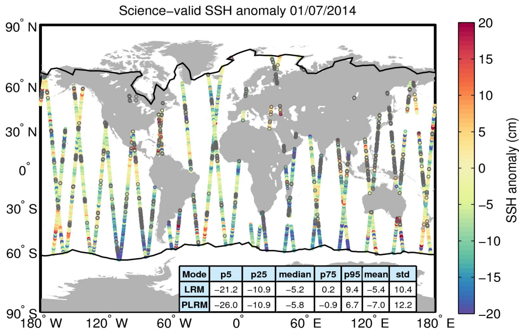
Figure 10. Geographical distribution of science-valid SSH anomaly data over oceans and lakes for 01/07/2014. The statistical values shown in the table refer to the SSH anomaly in cm and are calculated separately for LRM and PLRM regions. The black lines mark the outer limit of the Arctic and Antarctic polar polygons. Gray circles denote records that have been rejected based on the editing criteria described in Table 2.
