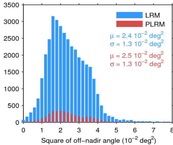
Figure 39. Histogram of flag-valid mispointing over oceans and lakes for LRM (blue) and PLRM (red) for 01/07/2014. Only positive values have been considered. The mean ( \mu ) and standard deviation ( \sigma ) are also shown. Note that values 8 \cdot 10^{-2} \text{ deg}^2 are excluded from the histogram for the sake of readability but not from the computation of \mu and \sigma .
