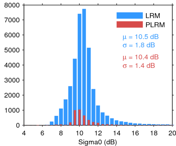
Figure 25. Histogram of flag-valid sigma0 over oceans and lakes for LRM (blue) and PLRM (red) for 01/07/2014. The mean ( \mu ) and standard deviation ( \sigma ) are also shown. Note that values outside [4 20] dB are excluded from the histogram for the sake of readability but not from the computation of \mu and \sigma .
