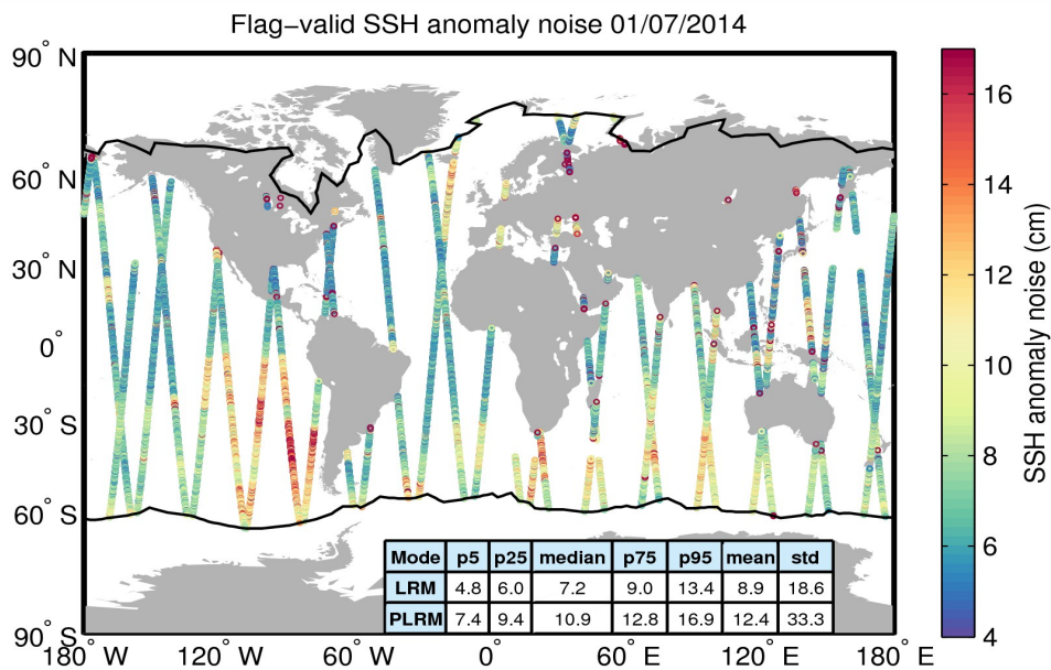
Figure 8. Geographical distribution of flag-valid 20-Hz SSH anomaly measurement noise over oceans and lakes for 01/07/2014. The statistical values shown in the table refer to the SSH anomaly noise and are calculated separately for LRM and PLRM regions. Measurements taken over polar polygons have been excluded from the computation of the statistical values. The black lines mark the outer limit of the Arctic and Antarctic polar polygons.
