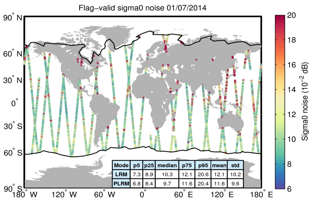
Figure 26. Geographical distribution of flag-valid 20-Hz sigma0 measurement noise over oceans and lakes for 01/07/2014. The statistical values shown in the table refer to the sigma0 noise and are calculated separately for LRM and PLRM regions. Measurements taken over polar polygons have been excluded from the computation of the statistical values. The black lines mark the outer limit of the Arctic and Antarctic polar polygons.
