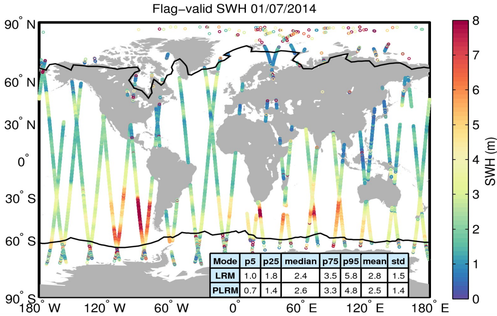
Figure 15. Geographical distribution of flag-valid SWH data over oceans and lakes for 01/07/2014. The statistical values shown in the table refer to the SWH in m and are calculated separately for LRM and PLRM regions. Measurements taken over polar polygons have been excluded from the computation of the statistical values. The black lines mark the outer limit of the Arctic and Antarctic polar polygons.
