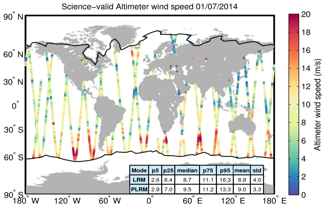
Figure 34. Geographical distribution of science-valid wind data over oceans and lakes for 01/07/2014. The statistical values shown in the table refer to the wind in m/s and are calculated separately for LRM and PLRM regions. The black lines mark the outer limit of the Arctic and Antarctic polar polygons. Gray circles denote records that have been rejected based on the editing criteria described in Table 5.
