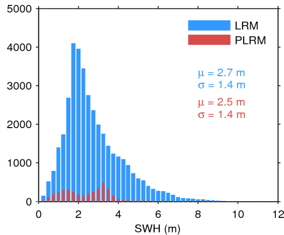
Figure 20. Histogram of science-valid SWH over oceans and lakes for LRM (blue) and PLRM (red) for 01/07/2014. The mean ( \mu ) and standard deviation ( \sigma ) are also shown. Note that values larger than 12 m are excluded from the histogram for the sake of readability but not from the computation of \mu and \sigma .
