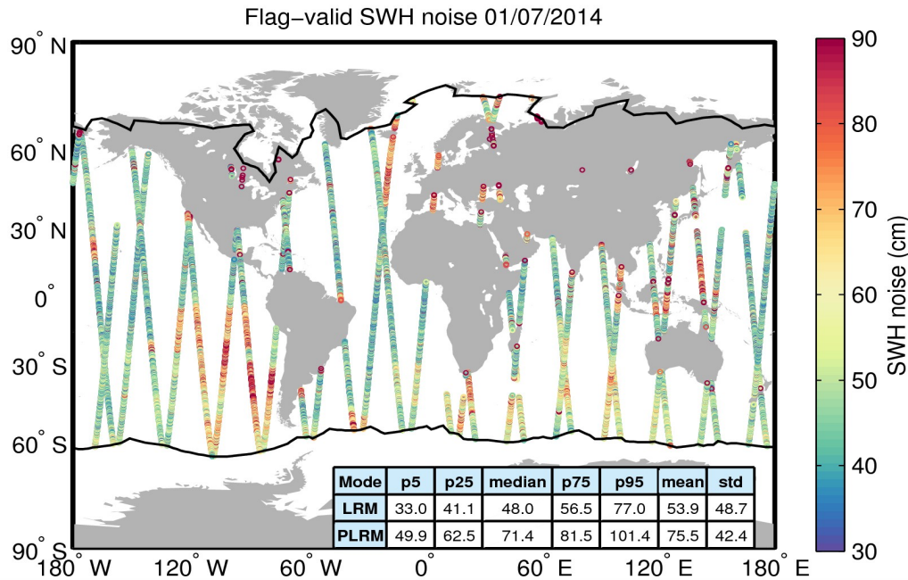
Figure 18. Geographical distribution of flag-valid 20-Hz SWH measurement noise over oceans and lakes for 01/07/2014. The statistical values shown in the table refer to the SWH noise and are calculated separately for LRM and PLRM regions. Measurements taken over polar polygons have been excluded from the computation of the statistical values. The black lines mark the outer limit of the Arctic and Antarctic polar polygons.
