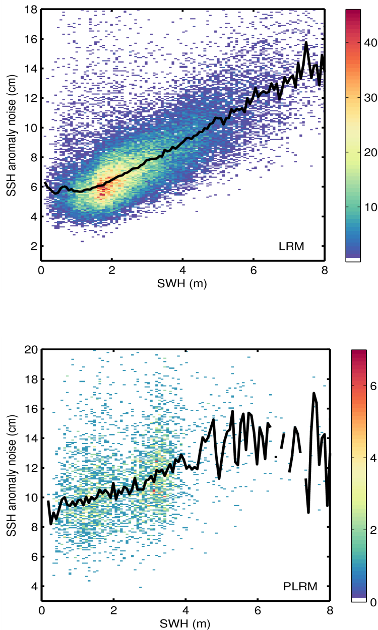
Figure 9. 2D histogram showing flag-valid SSH anomaly noise as a function of SWH for LRM (top) and PLRM (bottom) for 01/07/2014. The black line denotes the median SSH anomaly as a function of SWH.
