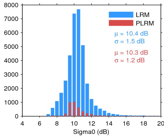
Figure 28. Histogram of science-valid sigma0 over oceans and lakes for LRM (blue) and PLRM (red) for 01/07/2014. The mean ( \mu ) and standard deviation ( \sigma ) are also shown. Note that values outside [4 20] dB are excluded from the histogram for the sake of readability but not from the computation of \mu and \sigma .
