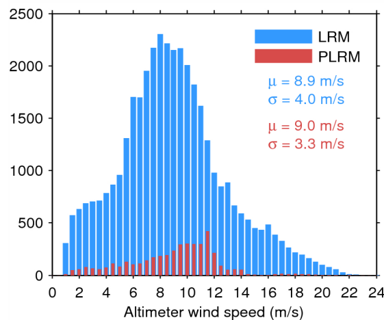
Figure 35. Histogram of science-valid wind over oceans and lakes for LRM (blue) and PLRM (red) for 01/07/2014. The mean ( \mu ) and standard deviation ( \sigma ) are also shown. Note that values larger than 24 m/s are excluded from the histogram for the sake of readability but not from the computation of \mu and \sigma .
