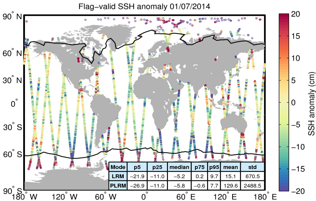
Figure 5. Geographical distribution of flag-valid 1-Hz SSH anomaly data over oceans and lakes for 01/07/2014. The statistical values shown in the table refer to the SSH anomaly in cm and are calculated separately for LRM and PLRM regions. Measurements taken over polar polygons have been excluded from the computation of the statistical values. The black lines mark the outer limit of the Arctic and Antarctic polar polygons.
