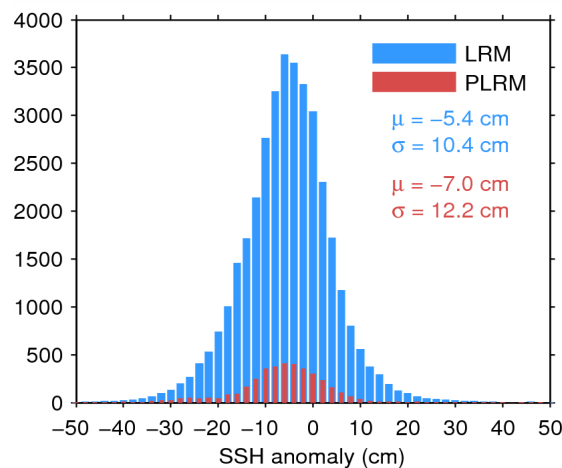
Figure 11. Histogram of science-valid SSH anomaly over oceans and lakes for LRM (blue) and PLRM (red) for 01/07/2014. The mean ( \mu ) and standard deviation ( \sigma ) are also shown. Note that values outside [-50 \ 50] cm are excluded from the histogram for the sake of readability but not from the computation of \mu and \sigma .
