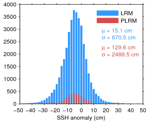
Figure 7. Histogram of flag-valid SSH anomaly over oceans and lakes for LRM (blue) and PLRM (red) for 01/07/2014. The mean ( \mu ) and standard deviation ( \sigma ) are also shown. Note that values outside [-50 \ 50] cm are excluded from the histogram for the sake of readability but not from the computation of \mu and \sigma .
