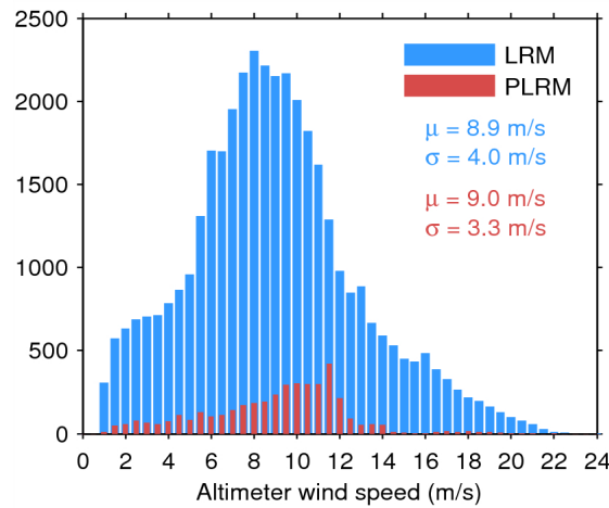
Figure 33. Histogram of flag-valid wind over oceans and lakes for LRM (blue) and PLRM (red) for 01/07/2014. The mean ( \mu ) and standard deviation ( \sigma ) are also shown. Note that values larger than 24 m/s are excluded from the histogram for the sake of readability but not from the computation of \mu and \sigma .
