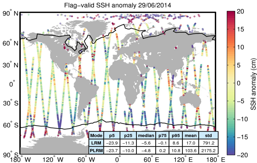
Figure 5. Geographical distribution of flag-valid 1-Hz SSH anomaly data over oceans and lakes for 29/06/2014. The statistical values shown in the table refer to the SSH anomaly in cm and are calculated separately for LRM and PLRM regions. Measurements taken over polar polygons have been excluded from the computation of the statistical values. The black lines mark the outer limit of the Arctic and Antarctic polar polygons.
