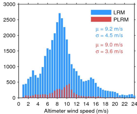
Figure 33. Histogram of flag-valid wind over oceans and lakes for LRM (blue) and PLRM (red) for 29/06/2014. The mean ( \mu ) and standard deviation ( \sigma ) are also shown. Note that values larger than 24 m/s are excluded from the histogram for the sake of readability but not from the computation of \mu and \sigma .
