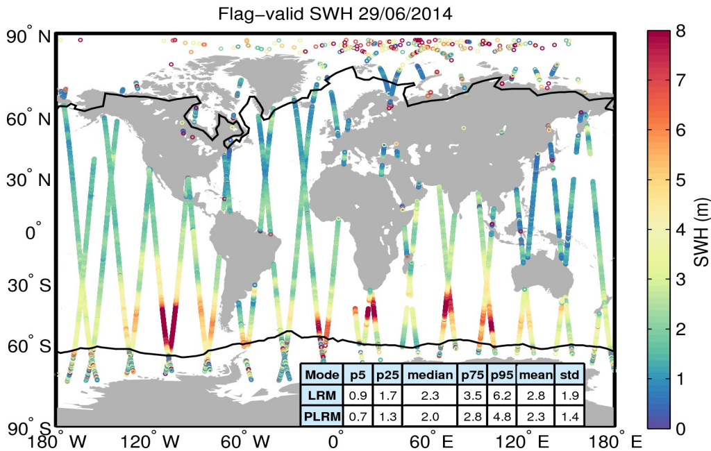
Figure 15. Geographical distribution of flag-valid SWH data over oceans and lakes for 29/06/2014. The statistical values shown in the table refer to the SWH in m and are calculated separately for LRM and PLRM regions. Measurements taken over polar polygons have been excluded from the computation of the statistical values. The black lines mark the outer limit of the Arctic and Antarctic polar polygons.
