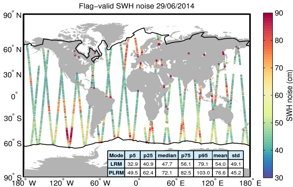
Figure 18. Geographical distribution of flag-valid 20-Hz SWH measurement noise over oceans and lakes for 29/06/2014. The statistical values shown in the table refer to the SWH noise and are calculated separately for LRM and PLRM regions. Measurements taken over polar polygons have been excluded from the computation of the statistical values. The black lines mark the outer limit of the Arctic and Antarctic polar polygons.
