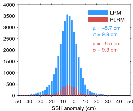
Figure 11. Histogram of science-valid SSH anomaly over oceans and lakes for LRM (blue) and PLRM (red) for 29/06/2014. The mean ( \mu ) and standard deviation ( \sigma ) are also shown. Note that values outside [-50 50] cm are excluded from the histogram for the sake of readability but not from the computation of \mu and \sigma .
