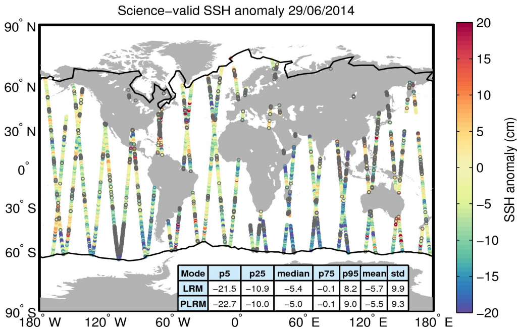
Figure 10. Geographical distribution of science-valid SSH anomaly data over oceans and lakes for 29/06/2014. The statistical values shown in the table refer to the SSH anomaly in cm and are calculated separately for LRM and PLRM regions. The black lines mark the outer limit of the Arctic and Antarctic polar polygons. Gray circles denote records that have been rejected based on the editing criteria described in Table 2.
