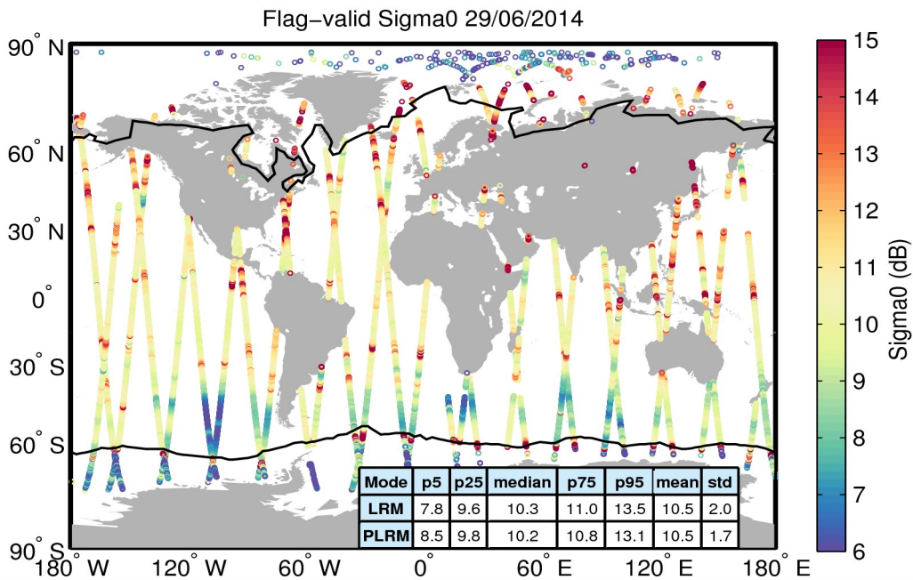
Figure 23. Geographical distribution of flag-valid sigma0 data over oceans and lakes for 29/06/2014. The statistical values shown in the table refer to the sigma0 in dB and are calculated separately for LRM and PLRM regions. Measurements taken over polar polygons have been excluded from the computation of the statistical values. The black lines mark the outer limit of the Arctic and Antarctic polar polygons.
