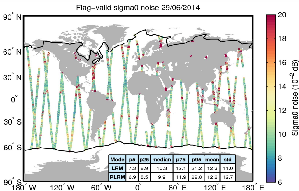
Figure 26. Geographical distribution of flag-valid 20-Hz sigma0 measurement noise over oceans and lakes for 29/06/2014. The statistical values shown in the table refer to the sigma0 noise and are calculated separately for LRM and PLRM regions. Measurements taken over polar polygons have been excluded from the computation of the statistical values. The black lines mark the outer limit of the Arctic and Antarctic polar polygons.
