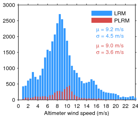
Figure 35. Histogram of science-valid wind over oceans and lakes for LRM (blue) and PLRM (red) for 29/06/2014. The mean ( \mu ) and standard deviation ( \sigma ) are also shown. Note that values larger than 24 m/s are excluded from the histogram for the sake of readability but not from the computation of \mu and \sigma .
