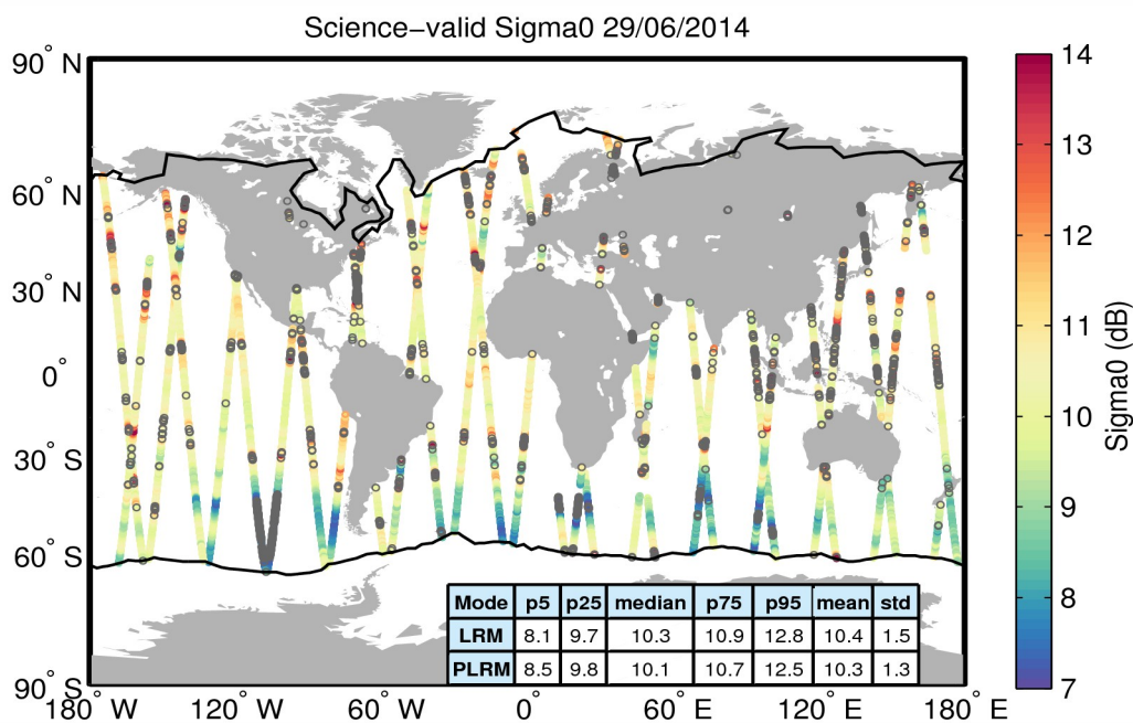
Figure 27. Geographical distribution of science-valid sigma0 data over oceans and lakes for 29/06/2014. The statistical values shown in the table refer to the sigma0 in dB and are calculated separately for LRM and PLRM regions. The black lines mark the outer limit of the Arctic and Antarctic polar polygons. Gray circles denote records that have been rejected based on the editing criteria described in Table 4.
