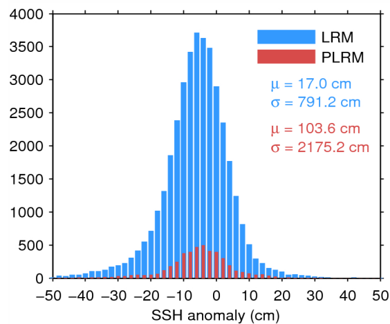
Figure 7. Histogram of flag-valid SSH anomaly over oceans and lakes for LRM (blue) and PLRM (red) for 29/06/2014. The mean ( \mu ) and standard deviation ( \sigma ) are also shown. Note that values outside [-50\ 50] cm are excluded from the histogram for the sake of readability but not from the computation of \mu and \sigma .
