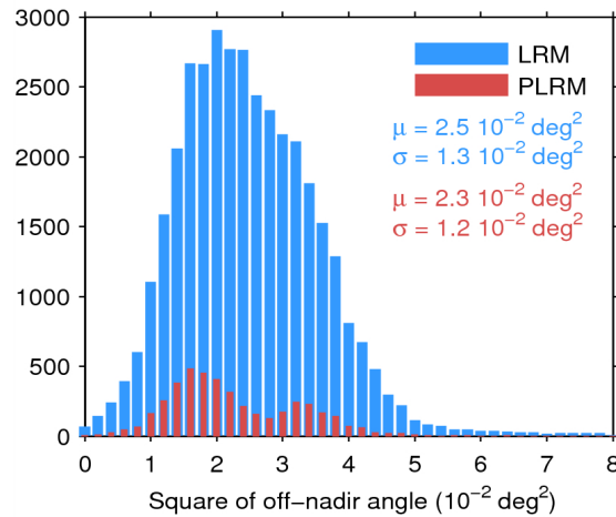
Figure 39. Histogram of flag-valid mispointing over oceans and lakes for LRM (blue) and PLRM (red) for 29/06/2014. Only positive values have been considered. The mean ( \mu ) and standard deviation ( \sigma ) are also shown. Note that values 8 \cdot 10^{-2} \text{ deg}^2 are excluded from the histogram for the sake of readability but not from the computation of \mu and \sigma .
