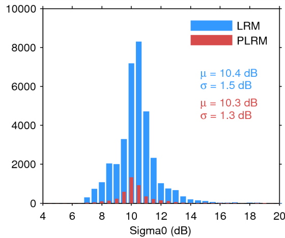
Figure 28. Histogram of science-valid sigma0 over oceans and lakes for LRM (blue) and PLRM (red) for 29/06/2014. The mean ( \mu ) and standard deviation ( \sigma ) are also shown. Note that values outside [4 20] dB are excluded from the histogram for the sake of readability but not from the computation of \mu and \sigma .
