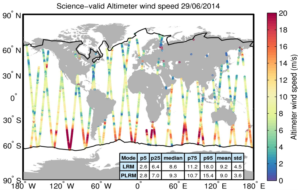
Figure 34. Geographical distribution of science-valid wind data over oceans and lakes for 29/06/2014. The statistical values shown in the table refer to the wind in m/s and are calculated separately for LRM and PLRM regions. The black lines mark the outer limit of the Arctic and Antarctic polar polygons. Gray circles denote records that have been rejected based on the editing criteria described in Table 5.
