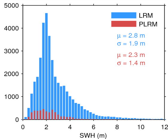
Figure 17. Histogram of flag-valid SWH over oceans and lakes for LRM (blue) and PLRM (red) for 29/06/2014. The mean ( \mu ) and standard deviation ( \sigma ) are also shown. Note that values larger than 12 m are excluded from the histogram for the sake of readability but not from the computation of \mu and \sigma .
