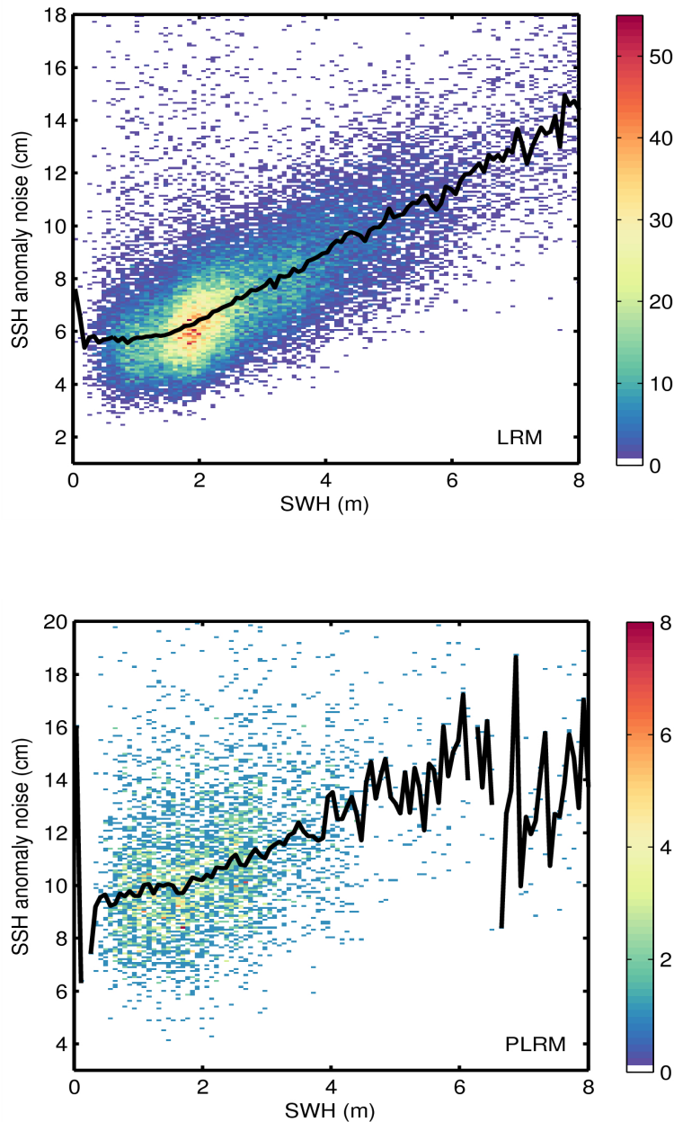
Figure 9. 2D histogram showing flag-valid SSH anomaly noise as a function of SWH for LRM (top) and PLRM (bottom) for 29/06/2014. The black line denotes the median SSH anomaly as a function of SWH.
