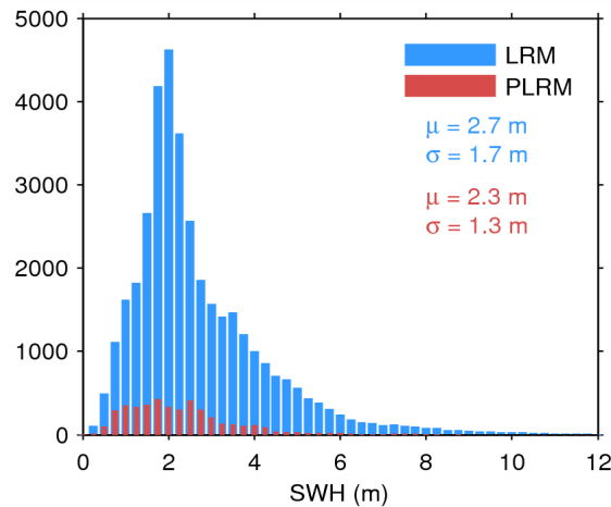
Figure 20. Histogram of science-valid SWH over oceans and lakes for LRM (blue) and PLRM (red) for 29/06/2014. The mean ( \mu ) and standard deviation ( \sigma ) are also shown. Note that values larger than 12 m are excluded from the histogram for the sake of readability but not from the computation of \mu and \sigma .
