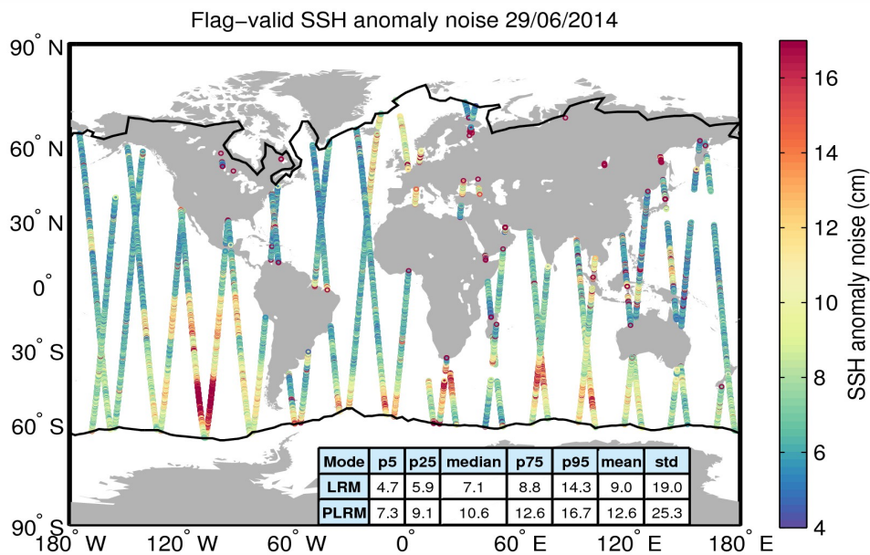
Figure 8. Geographical distribution of flag-valid 20-Hz SSH anomaly measurement noise over oceans and lakes for 29/06/2014. The statistical values shown in the table refer to the SSH anomaly noise and are calculated separately for LRM and PLRM regions. Measurements taken over polar polygons have been excluded from the computation of the statistical values. The black lines mark the outer limit of the Arctic and Antarctic polar polygons.
