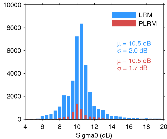
Figure 25. Histogram of flag-valid sigma0 over oceans and lakes for LRM (blue) and PLRM (red) for 29/06/2014. The mean ( \mu ) and standard deviation ( \sigma ) are also shown. Note that values outside [4 20] dB are excluded from the histogram for the sake of readability but not from the computation of \mu and \sigma .
