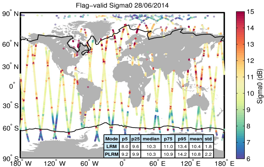
Figure 23. Geographical distribution of flag-valid sigma0 data over oceans and lakes for 28/06/2014. The statistical values shown in the table refer to the sigma0 in dB and are calculated separately for LRM and PLRM regions. Measurements taken over polar polygons have been excluded from the computation of the statistical values. The black lines mark the outer limit of the Arctic and Antarctic polar polygons.
