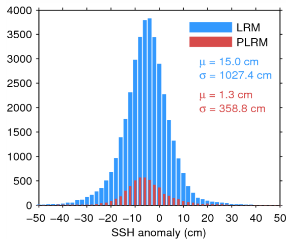
Figure 7. Histogram of flag-valid SSH anomaly over oceans and lakes for LRM (blue) and PLRM (red) for 28/06/2014. The mean ( \mu ) and standard deviation ( \sigma ) are also shown. Note that values outside [-50\ 50] cm are excluded from the histogram for the sake of readability but not from the computation of \mu and \sigma .
