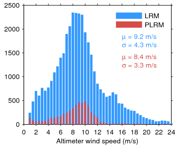
Figure 33. Histogram of flag-valid wind over oceans and lakes for LRM (blue) and PLRM (red) for 28/06/2014. The mean ( \mu ) and standard deviation ( \sigma ) are also shown. Note that values larger than 24 m/s are excluded from the histogram for the sake of readability but not from the computation of \mu and \sigma .
