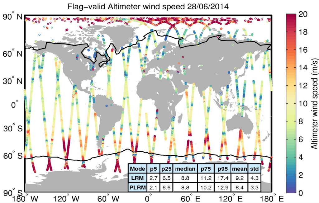
Figure 31. Geographical distribution of flag-valid wind data over oceans and lakes for 28/06/2014. The statistical values shown in the table refer to the wind in m/s and are calculated separately for LRM and PLRM regions. Measurements taken over polar polygons have been excluded from the computation of the statistical values. The black lines mark the outer limit of the Arctic and Antarctic polar polygons.
