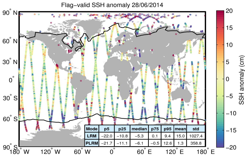
Figure 5. Geographical distribution of flag-valid 1-Hz SSH anomaly data over oceans and lakes for 28/06/2014. The statistical values shown in the table refer to the SSH anomaly in cm and are calculated separately for LRM and PLRM regions. Measurements taken over polar polygons have been excluded from the computation of the statistical values. The black lines mark the outer limit of the Arctic and Antarctic polar polygons.
