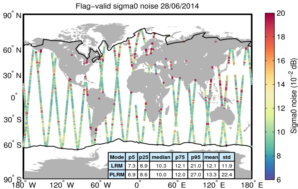
Figure 26. Geographical distribution of flag-valid 20-Hz sigma0 measurement noise over oceans and lakes for 28/06/2014. The statistical values shown in the table refer to the sigma0 noise and are calculated separately for LRM and PLRM regions. Measurements taken over polar polygons have been excluded from the computation of the statistical values. The black lines mark the outer limit of the Arctic and Antarctic polar polygons.
