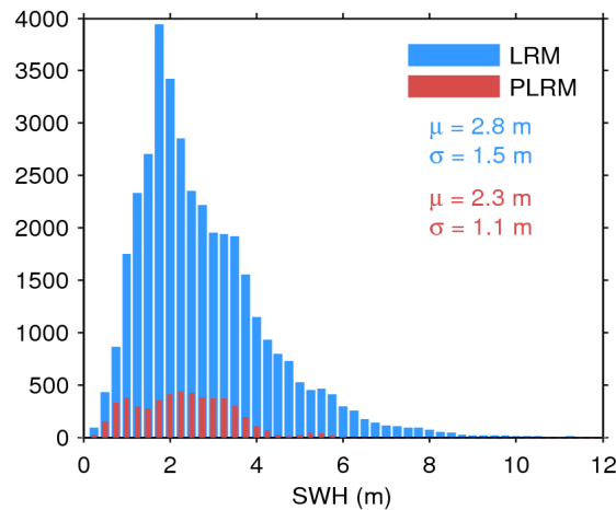
Figure 20. Histogram of science-valid SWH over oceans and lakes for LRM (blue) and PLRM (red) for 28/06/2014. The mean ( \mu ) and standard deviation ( \sigma ) are also shown. Note that values larger than 12 m are excluded from the histogram for the sake of readability but not from the computation of \mu and \sigma .
