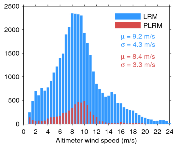
Figure 35. Histogram of science-valid wind over oceans and lakes for LRM (blue) and PLRM (red) for 28/06/2014. The mean ( \mu ) and standard deviation ( \sigma ) are also shown. Note that values larger than 24 m/s are excluded from the histogram for the sake of readability but not from the computation of \mu and \sigma .
