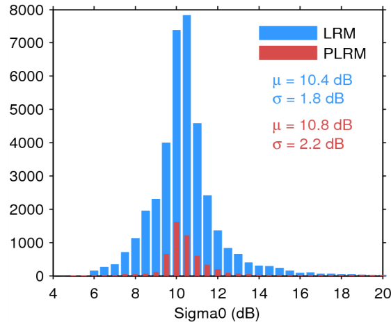
Figure 25. Histogram of flag-valid sigma0 over oceans and lakes for LRM (blue) and PLRM (red) for 28/06/2014. The mean ( \mu ) and standard deviation ( \sigma ) are also shown. Note that values outside [4 20] dB are excluded from the histogram for the sake of readability but not from the computation of \mu and \sigma .
