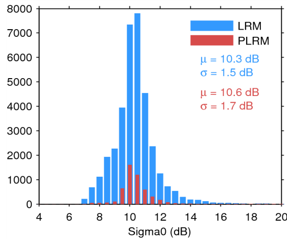
Figure 28. Histogram of science-valid sigma0 over oceans and lakes for LRM (blue) and PLRM (red) for 28/06/2014. The mean ( \mu ) and standard deviation ( \sigma ) are also shown. Note that values outside [4 20] dB are excluded from the histogram for the sake of readability but not from the computation of \mu and \sigma .
