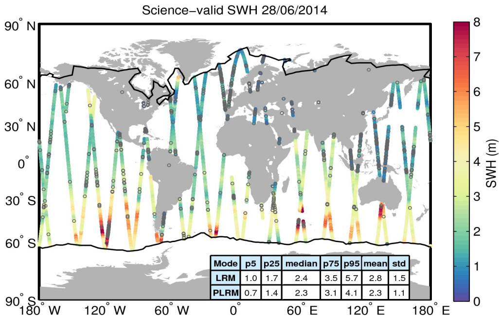
Figure 19. Geographical distribution of science-valid SWH data over oceans and lakes for 28/06/2014. The statistical values shown in the table refer to the SWH in m and are calculated separately for LRM and PLRM regions. The black lines mark the outer limit of the Arctic and Antarctic polar polygons. Gray circles denote records that have been rejected based on the editing criteria described in Table 3.
