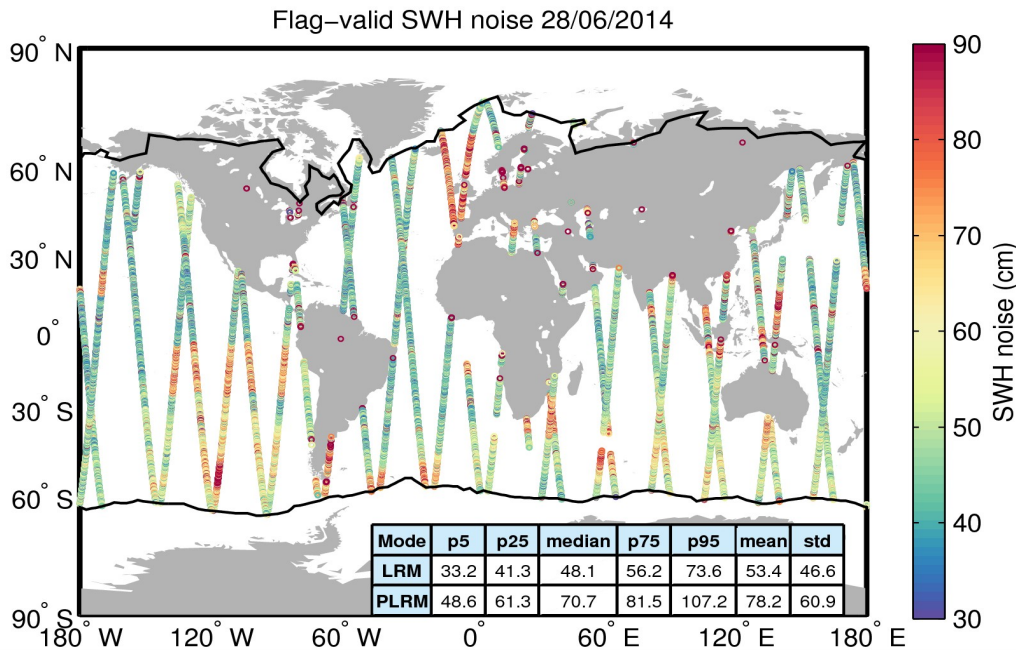
Figure 18. Geographical distribution of flag-valid 20-Hz SWH measurement noise over oceans and lakes for 28/06/2014. The statistical values shown in the table refer to the SWH noise and are calculated separately for LRM and PLRM regions. Measurements taken over polar polygons have been excluded from the computation of the statistical values. The black lines mark the outer limit of the Arctic and Antarctic polar polygons.
