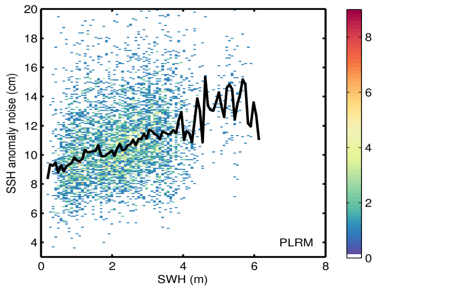
Figure 9. 2D histogram showing flag-valid SSH anomaly noise as a function of SWH for LRM (top) and PLRM (bottom) for 28/06/2014. The black line denotes the median SSH anomaly as a function of SWH.
