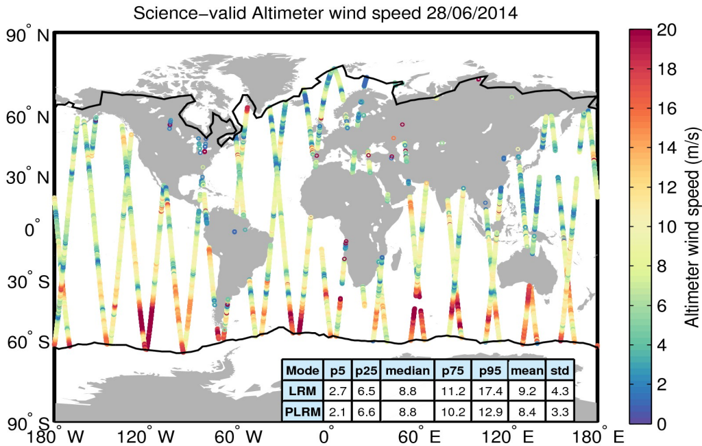
Figure 34. Geographical distribution of science-valid wind data over oceans and lakes for 28/06/2014. The statistical values shown in the table refer to the wind in m/s and are calculated separately for LRM and PLRM regions. The black lines mark the outer limit of the Arctic and Antarctic polar polygons. Gray circles denote records that have been rejected based on the editing criteria described in Table 5.
