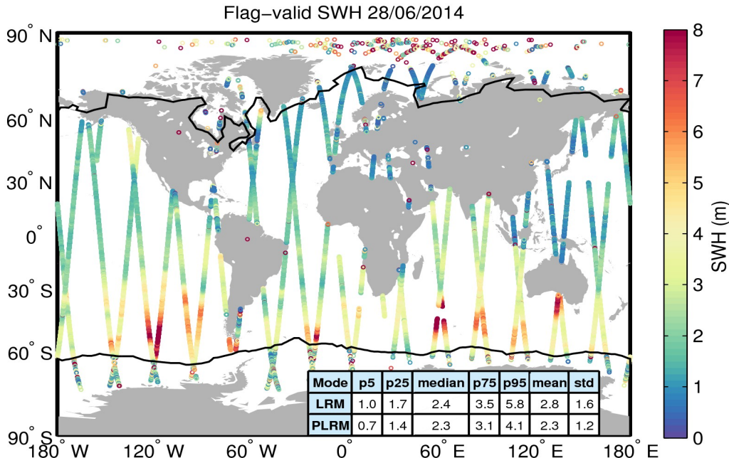
Figure 15. Geographical distribution of flag-valid SWH data over oceans and lakes for 28/06/2014. The statistical values shown in the table refer to the SWH in m and are calculated separately for LRM and PLRM regions. Measurements taken over polar polygons have been excluded from the computation of the statistical values. The black lines mark the outer limit of the Arctic and Antarctic polar polygons.
