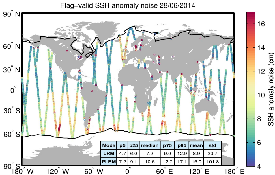
Figure 8. Geographical distribution of flag-valid 20-Hz SSH anomaly measurement noise over oceans and lakes for 28/06/2014. The statistical values shown in the table refer to the SSH anomaly noise and are calculated separately for LRM and PLRM regions. Measurements taken over polar polygons have been excluded from the computation of the statistical values. The black lines mark the outer limit of the Arctic and Antarctic polar polygons.
