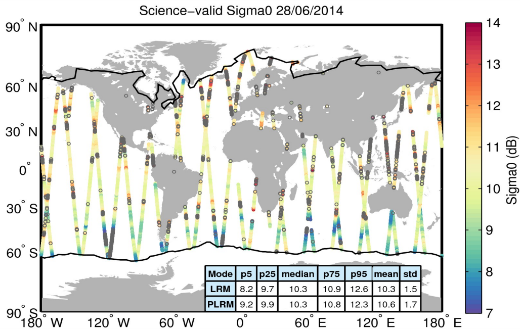
Figure 27. Geographical distribution of science-valid sigma0 data over oceans and lakes for 28/06/2014. The statistical values shown in the table refer to the sigma0 in dB and are calculated separately for LRM and PLRM regions. The black lines mark the outer limit of the Arctic and Antarctic polar polygons. Gray circles denote records that have been rejected based on the editing criteria described in Table 4.
