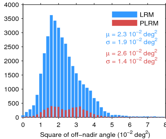
Figure 39. Histogram of flag-valid mispointing over oceans and lakes for LRM (blue) and PLRM (red) for 28/06/2014. Only positive values have been considered. The mean ( \mu ) and standard deviation ( \sigma ) are also shown. Note that values 8 \cdot 10^{-2} \text{ deg}^2 are excluded from the histogram for the sake of readability but not from the computation of \mu and \sigma .
