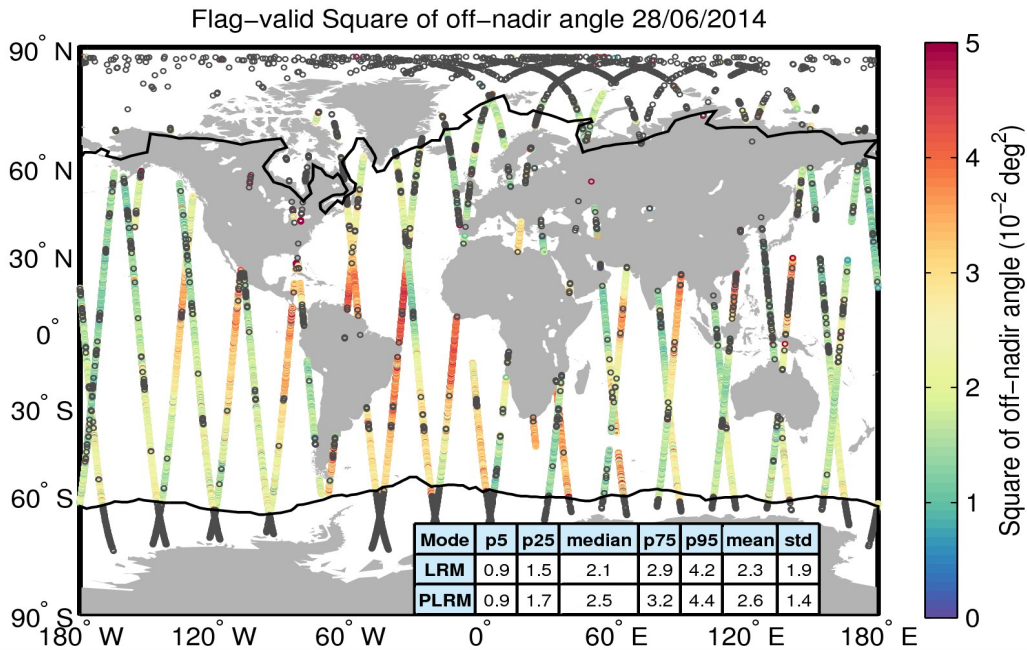
Figure 37. Geographical distribution of flag-valid mispointing data over oceans and lakes for 28/06/2014. The statistical values shown in the table refer to the mispointing in 10^{-2} \text{ deg}^2 and are calculated separately for LRM and PLRM regions. Measurements taken over polar polygons have been excluded from the computation of the statistical values. The black lines mark the outer limit of the Arctic and Antarctic polar polygons. Gray circles denote negative values.
