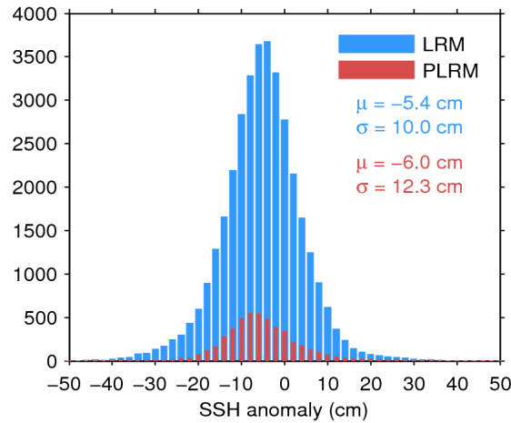
Figure 11. Histogram of science-valid SSH anomaly over oceans and lakes for LRM (blue) and PLRM (red) for 28/06/2014. The mean ( \mu ) and standard deviation ( \sigma ) are also shown. Note that values outside [-50 50] cm are excluded from the histogram for the sake of readability but not from the computation of \mu and \sigma .
