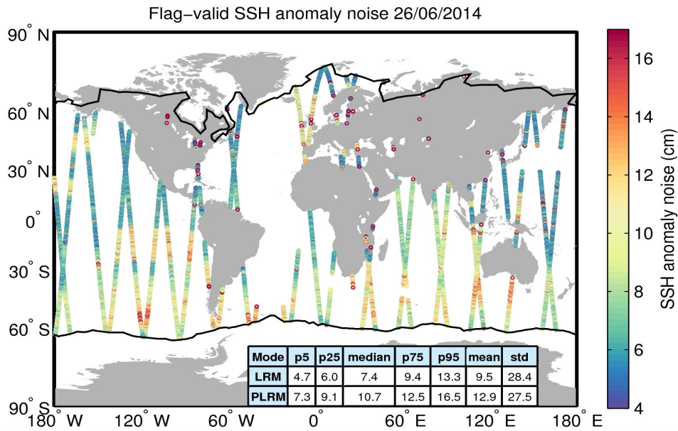
Figure 8. Geographical distribution of flag-valid 20-Hz SSH anomaly measurement noise over oceans and lakes for 26/06/2014. The statistical values shown in the table refer to the SSH anomaly noise and are calculated separately for LRM and PLRM regions. Measurements taken over polar polygons have been excluded from the computation of the statistical values. The black lines mark the outer limit of the Arctic and Antarctic polar polygons.
