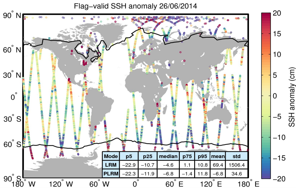
Figure 5. Geographical distribution of flag-valid 1-Hz SSH anomaly data over oceans and lakes for 26/06/2014. The statistical values shown in the table refer to the SSH anomaly in cm and are calculated separately for LRM and PLRM regions. Measurements taken over polar polygons have been excluded from the computation of the statistical values. The black lines mark the outer limit of the Arctic and Antarctic polar polygons.
