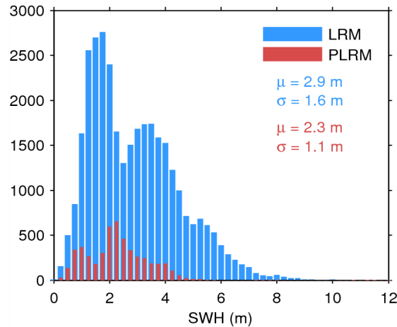
Figure 17. Histogram of flag-valid SWH over oceans and lakes for LRM (blue) and PLRM (red) for 26/06/2014. The mean ( \mu ) and standard deviation ( \sigma ) are also shown. Note that values larger than 12 m are excluded from the histogram for the sake of readability but not from the computation of \mu and \sigma .
