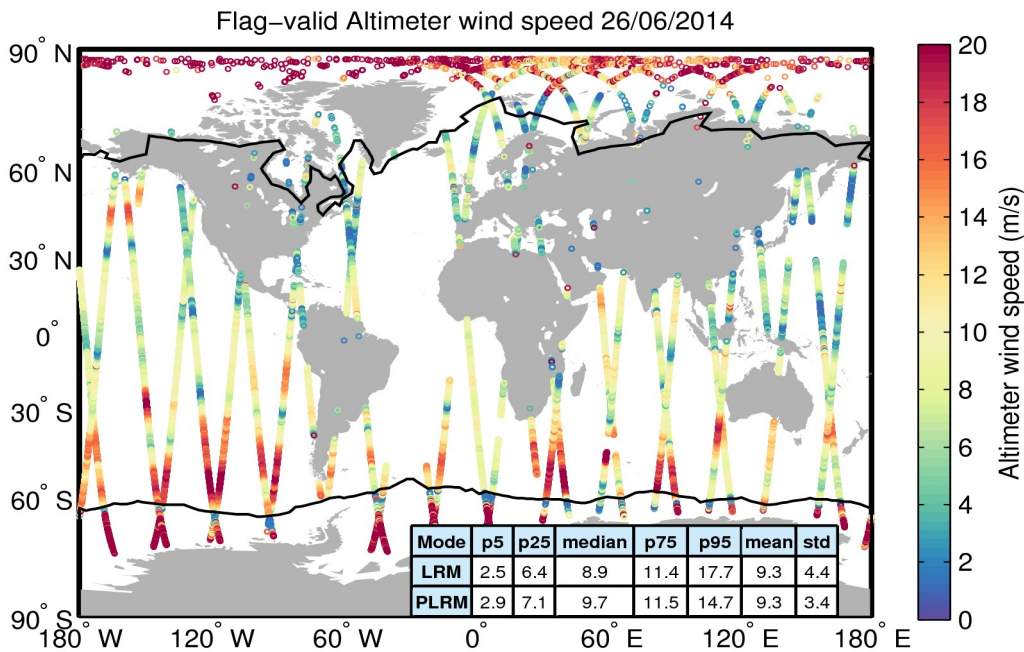
Figure 31. Geographical distribution of flag-valid wind data over oceans and lakes for 26/06/2014. The statistical values shown in the table refer to the wind in m/s and are calculated separately for LRM and PLRM regions. Measurements taken over polar polygons have been excluded from the computation of the statistical values. The black lines mark the outer limit of the Arctic and Antarctic polar polygons.
