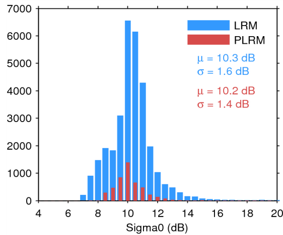
Figure 28. Histogram of science-valid sigma0 over oceans and lakes for LRM (blue) and PLRM (red) for 26/06/2014. The mean ( \mu ) and standard deviation ( \sigma ) are also shown. Note that values outside [4 20] dB are excluded from the histogram for the sake of readability but not from the computation of \mu and \sigma .
