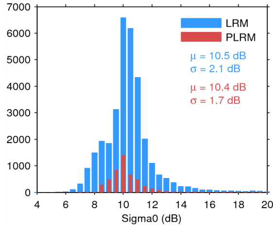
Figure 25. Histogram of flag-valid sigma0 over oceans and lakes for LRM (blue) and PLRM (red) for 26/06/2014. The mean ( \mu ) and standard deviation ( \sigma ) are also shown. Note that values outside [4 20] dB are excluded from the histogram for the sake of readability but not from the computation of \mu and \sigma .
