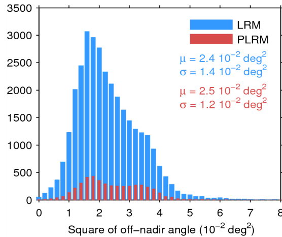
Figure 39. Histogram of flag-valid mispointing over oceans and lakes for LRM (blue) and PLRM (red) for 26/06/2014. Only positive values have been considered. The mean ( \mu ) and standard deviation ( \sigma ) are also shown. Note that values 8 \cdot 10^{-2} \text{ deg}^2 are excluded from the histogram for the sake of readability but not from the computation of \mu and \sigma .
