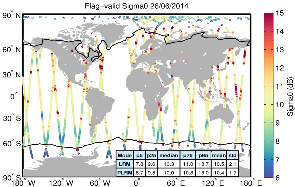
Figure 23. Geographical distribution of flag-valid sigma0 data over oceans and lakes for 26/06/2014. The statistical values shown in the table refer to the sigma0 in dB and are calculated separately for LRM and PLRM regions. Measurements taken over polar polygons have been excluded from the computation of the statistical values. The black lines mark the outer limit of the Arctic and Antarctic polar polygons.
