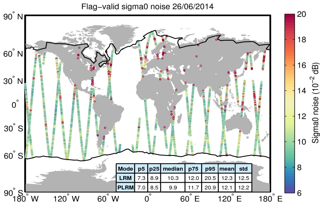
Figure 26. Geographical distribution of flag-valid 20-Hz sigma0 measurement noise over oceans and lakes for 26/06/2014. The statistical values shown in the table refer to the sigma0 noise and are calculated separately for LRM and PLRM regions. Measurements taken over polar polygons have been excluded from the computation of the statistical values. The black lines mark the outer limit of the Arctic and Antarctic polar polygons.
