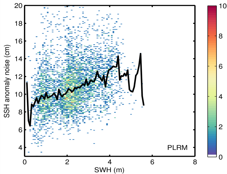
Figure 9. 2D histogram showing flag-valid SSH anomaly noise as a function of SWH for LRM (top) and PLRM (bottom) for 26/06/2014. The black line denotes the median SSH anomaly as a function of SWH.
