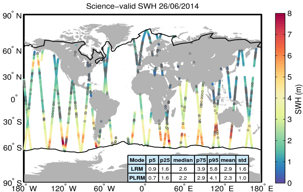
Figure 19. Geographical distribution of science-valid SWH data over oceans and lakes for 26/06/2014. The statistical values shown in the table refer to the SWH in m and are calculated separately for LRM and PLRM regions. The black lines mark the outer limit of the Arctic and Antarctic polar polygons. Gray circles denote records that have been rejected based on the editing criteria described in Table 3.
