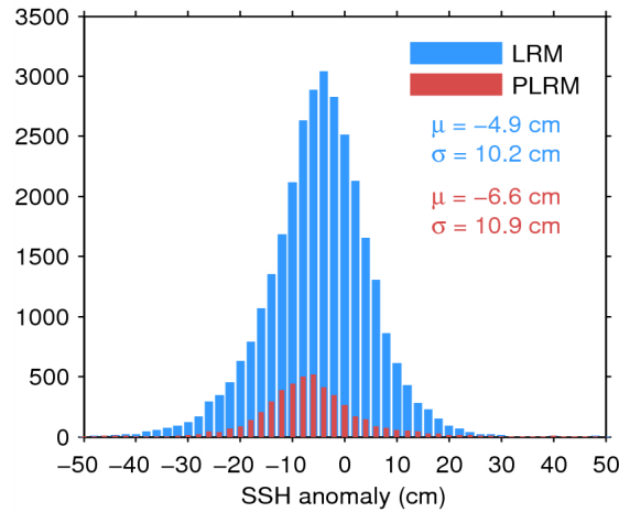
Figure 11. Histogram of science-valid SSH anomaly over oceans and lakes for LRM (blue) and PLRM (red) for 26/06/2014. The mean ( \mu ) and standard deviation ( \sigma ) are also shown. Note that values outside [-50 50] cm are excluded from the histogram for the sake of readability but not from the computation of \mu and \sigma .
