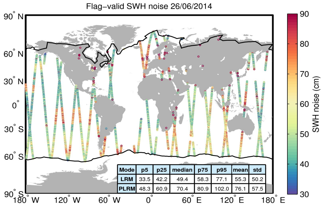
Figure 18. Geographical distribution of flag-valid 20-Hz SWH measurement noise over oceans and lakes for 26/06/2014. The statistical values shown in the table refer to the SWH noise and are calculated separately for LRM and PLRM regions. Measurements taken over polar polygons have been excluded from the computation of the statistical values. The black lines mark the outer limit of the Arctic and Antarctic polar polygons.
