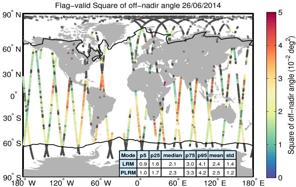
Figure 37. Geographical distribution of flag-valid mispointing data over oceans and lakes for 26/06/2014. The statistical values shown in the table refer to the mispointing in 10^{-2} \text{ deg}^2 and are calculated separately for LRM and PLRM regions. Measurements taken over polar polygons have been excluded from the computation of the statistical values. The black lines mark the outer limit of the Arctic and Antarctic polar polygons. Gray circles denote negative values.
