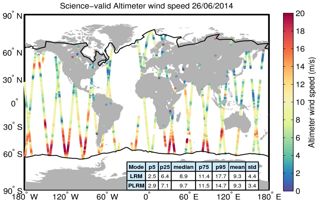
Figure 34. Geographical distribution of science-valid wind data over oceans and lakes for 26/06/2014. The statistical values shown in the table refer to the wind in m/s and are calculated separately for LRM and PLRM regions. The black lines mark the outer limit of the Arctic and Antarctic polar polygons. Gray circles denote records that have been rejected based on the editing criteria described in Table 5.
