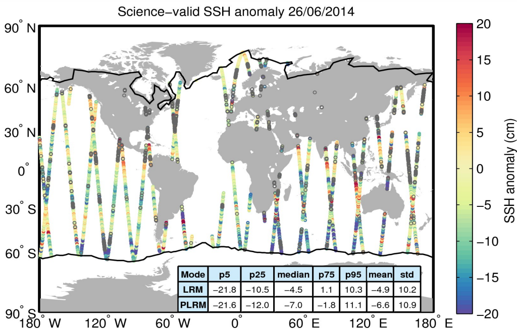
Figure 10. Geographical distribution of science-valid SSH anomaly data over oceans and lakes for 26/06/2014. The statistical values shown in the table refer to the SSH anomaly in cm and are calculated separately for LRM and PLRM regions. The black lines mark the outer limit of the Arctic and Antarctic polar polygons. Gray circles denote records that have been rejected based on the editing criteria described in Table 2.
