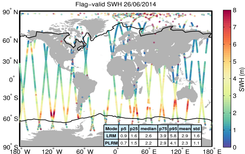
Figure 15. Geographical distribution of flag-valid SWH data over oceans and lakes for 26/06/2014. The statistical values shown in the table refer to the SWH in m and are calculated separately for LRM and PLRM regions. Measurements taken over polar polygons have been excluded from the computation of the statistical values. The black lines mark the outer limit of the Arctic and Antarctic polar polygons.
