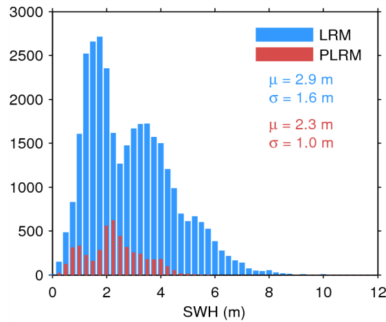
Figure 20. Histogram of science-valid SWH over oceans and lakes for LRM (blue) and PLRM (red) for 26/06/2014. The mean ( \mu ) and standard deviation ( \sigma ) are also shown. Note that values larger than 12 m are excluded from the histogram for the sake of readability but not from the computation of \mu and \sigma .
