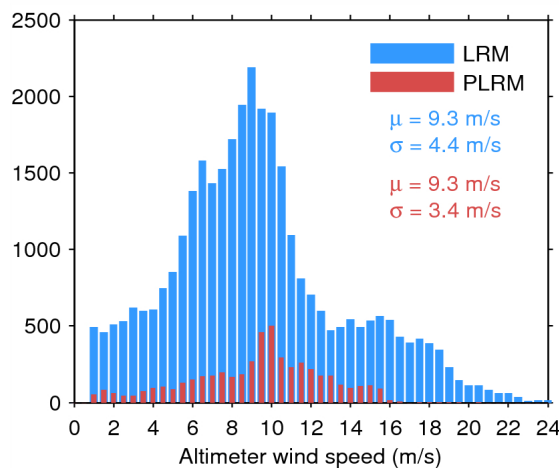
Figure 35. Histogram of science-valid wind over oceans and lakes for LRM (blue) and PLRM (red) for 26/06/2014. The mean ( \mu ) and standard deviation ( \sigma ) are also shown. Note that values larger than 24 m/s are excluded from the histogram for the sake of readability but not from the computation of \mu and \sigma .
