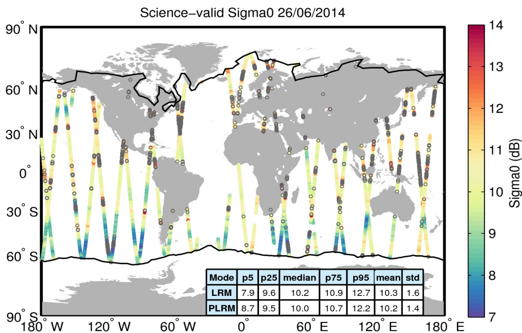
Figure 27. Geographical distribution of science-valid sigma0 data over oceans and lakes for 26/06/2014. The statistical values shown in the table refer to the sigma0 in dB and are calculated separately for LRM and PLRM regions. The black lines mark the outer limit of the Arctic and Antarctic polar polygons. Gray circles denote records that have been rejected based on the editing criteria described in Table 4.
