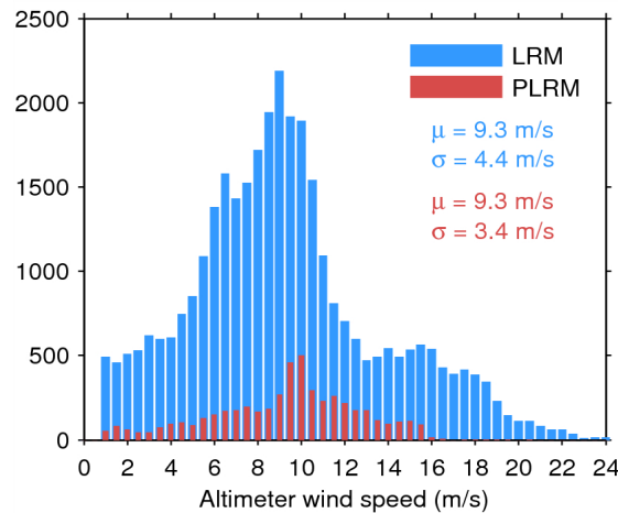
Figure 33. Histogram of flag-valid wind over oceans and lakes for LRM (blue) and PLRM (red) for 26/06/2014. The mean ( \mu ) and standard deviation ( \sigma ) are also shown. Note that values larger than 24 m/s are excluded from the histogram for the sake of readability but not from the computation of \mu and \sigma .
