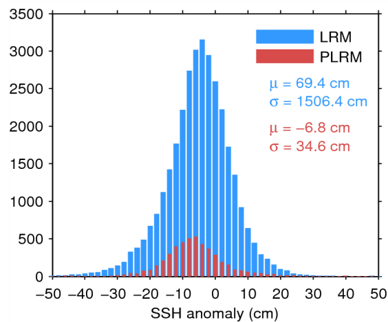
Figure 7. Histogram of flag-valid SSH anomaly over oceans and lakes for LRM (blue) and PLRM (red) for 26/06/2014. The mean ( \mu ) and standard deviation ( \sigma ) are also shown. Note that values outside [-50\ 50] cm are excluded from the histogram for the sake of readability but not from the computation of \mu and \sigma .
