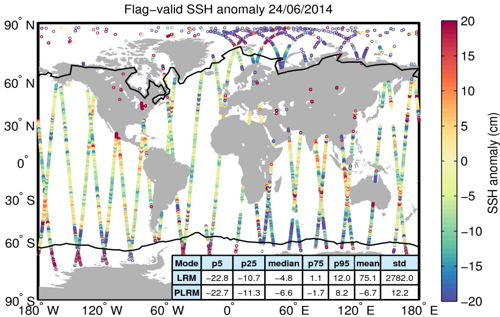
Figure 5. Geographical distribution of flag-valid 1-Hz SSH anomaly data over oceans and lakes for 24/06/2014. The statistical values shown in the table refer to the SSH anomaly in cm and are calculated separately for LRM and PLRM regions. Measurements taken over polar polygons have been excluded from the computation of the statistical values. The black lines mark the outer limit of the Arctic and Antarctic polar polygons.
