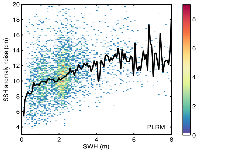
Figure 9. 2D histogram showing flag-valid SSH anomaly noise as a function of SWH for LRM (top) and PLRM (bottom) for 24/06/2014. The black line denotes the median SSH anomaly as a function of SWH.
