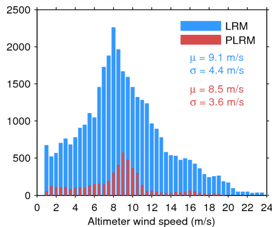
Figure 35. Histogram of science-valid wind over oceans and lakes for LRM (blue) and PLRM (red) for 24/06/2014. The mean ( \mu ) and standard deviation ( \sigma ) are also shown. Note that values larger than 24 m/s are excluded from the histogram for the sake of readability but not from the computation of \mu and \sigma .
