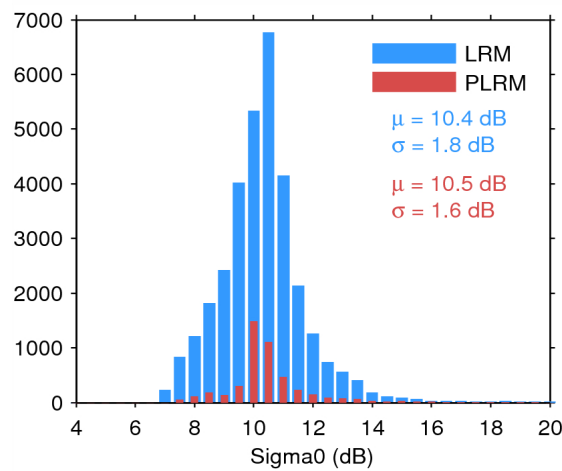
Figure 28. Histogram of science-valid sigma0 over oceans and lakes for LRM (blue) and PLRM (red) for 24/06/2014. The mean ( \mu ) and standard deviation ( \sigma ) are also shown. Note that values outside [4 20] dB are excluded from the histogram for the sake of readability but not from the computation of \mu and \sigma .
