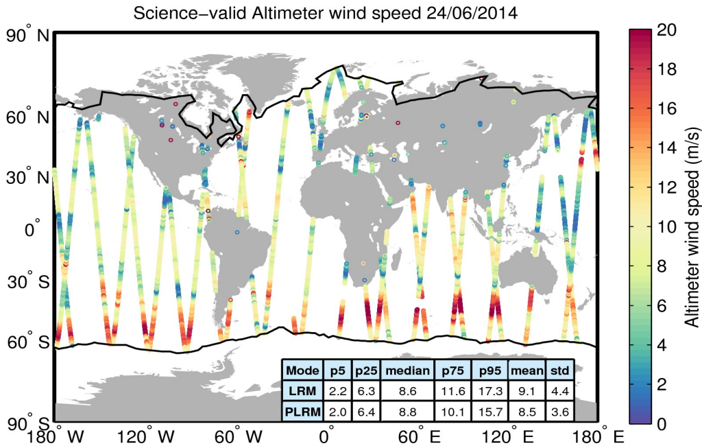
Figure 34. Geographical distribution of science-valid wind data over oceans and lakes for 24/06/2014. The statistical values shown in the table refer to the wind in m/s and are calculated separately for LRM and PLRM regions. The black lines mark the outer limit of the Arctic and Antarctic polar polygons. Gray circles denote records that have been rejected based on the editing criteria described in Table 5.
