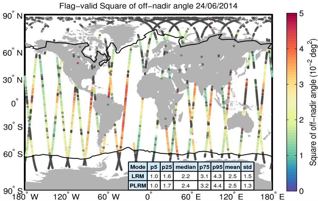
Figure 37. Geographical distribution of flag-valid mispointing data over oceans and lakes for 24/06/2014. The statistical values shown in the table refer to the mispointing in 10^{-2} \text{ deg}^2 and are calculated separately for LRM and PLRM regions. Measurements taken over polar polygons have been excluded from the computation of the statistical values. The black lines mark the outer limit of the Arctic and Antarctic polar polygons. Gray circles denote negative values.
