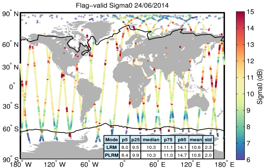
Figure 23. Geographical distribution of flag-valid sigma0 data over oceans and lakes for 24/06/2014. The statistical values shown in the table refer to the sigma0 in dB and are calculated separately for LRM and PLRM regions. Measurements taken over polar polygons have been excluded from the computation of the statistical values. The black lines mark the outer limit of the Arctic and Antarctic polar polygons.
