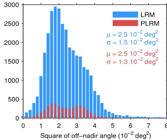
Figure 39. Histogram of flag-valid mispointing over oceans and lakes for LRM (blue) and PLRM (red) for 24/06/2014. Only positive values have been considered. The mean ( \mu ) and standard deviation ( \sigma ) are also shown. Note that values 8 \cdot 10^{-2} \text{ deg}^2 are excluded from the histogram for the sake of readability but not from the computation of \mu and \sigma .
