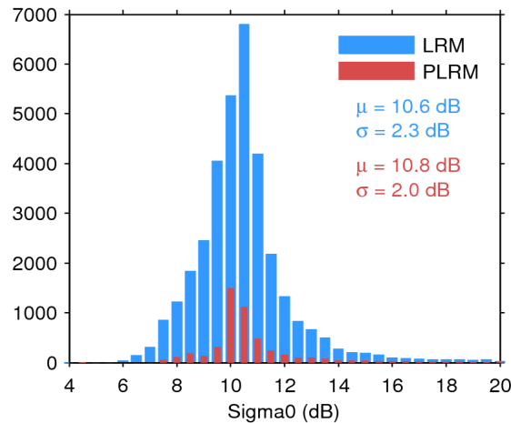
Figure 25. Histogram of flag-valid sigma0 over oceans and lakes for LRM (blue) and PLRM (red) for 24/06/2014. The mean ( \mu ) and standard deviation ( \sigma ) are also shown. Note that values outside [4 20] dB are excluded from the histogram for the sake of readability but not from the computation of \mu and \sigma .
