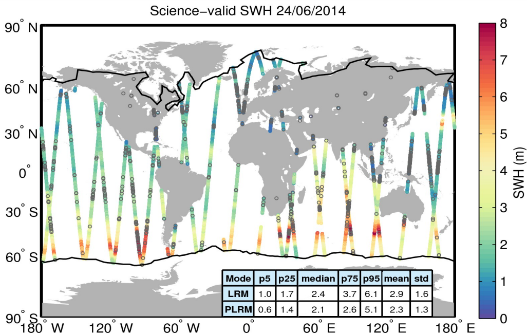
Figure 19. Geographical distribution of science-valid SWH data over oceans and lakes for 24/06/2014. The statistical values shown in the table refer to the SWH in m and are calculated separately for LRM and PLRM regions. The black lines mark the outer limit of the Arctic and Antarctic polar polygons. Gray circles denote records that have been rejected based on the editing criteria described in Table 3.
