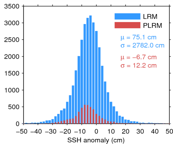
Figure 7. Histogram of flag-valid SSH anomaly over oceans and lakes for LRM (blue) and PLRM (red) for 24/06/2014. The mean ( \mu ) and standard deviation ( \sigma ) are also shown. Note that values outside [-50\ 50] cm are excluded from the histogram for the sake of readability but not from the computation of \mu and \sigma .
