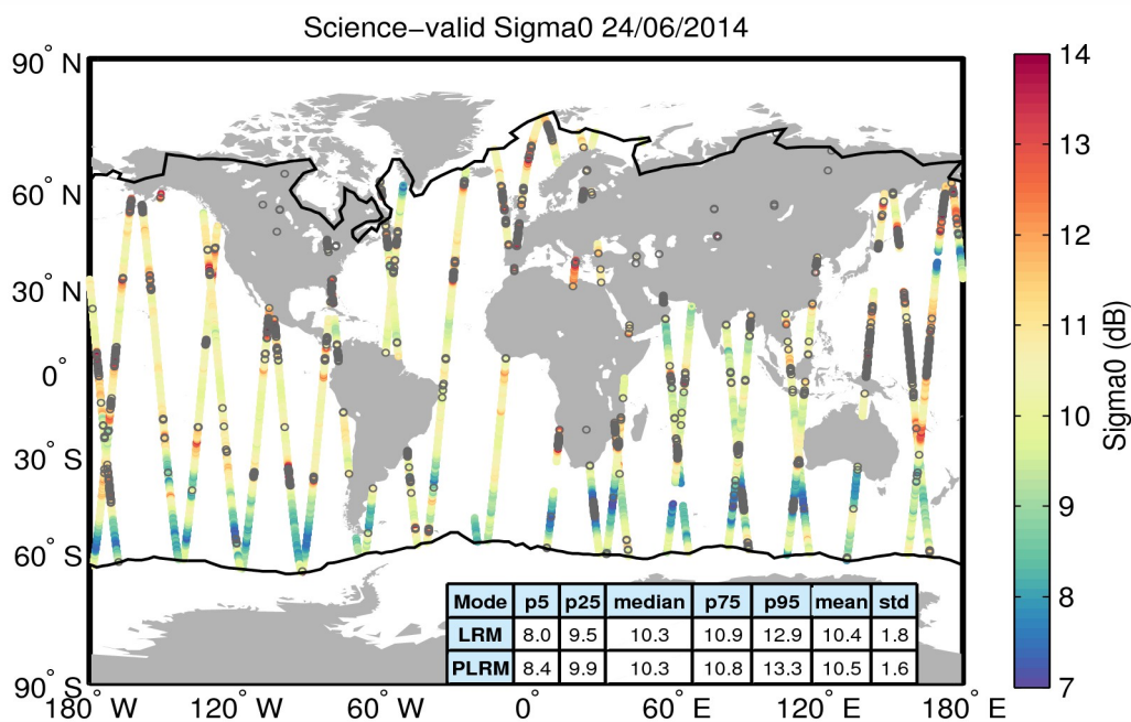
Figure 27. Geographical distribution of science-valid sigma0 data over oceans and lakes for 24/06/2014. The statistical values shown in the table refer to the sigma0 in dB and are calculated separately for LRM and PLRM regions. The black lines mark the outer limit of the Arctic and Antarctic polar polygons. Gray circles denote records that have been rejected based on the editing criteria described in Table 4.
