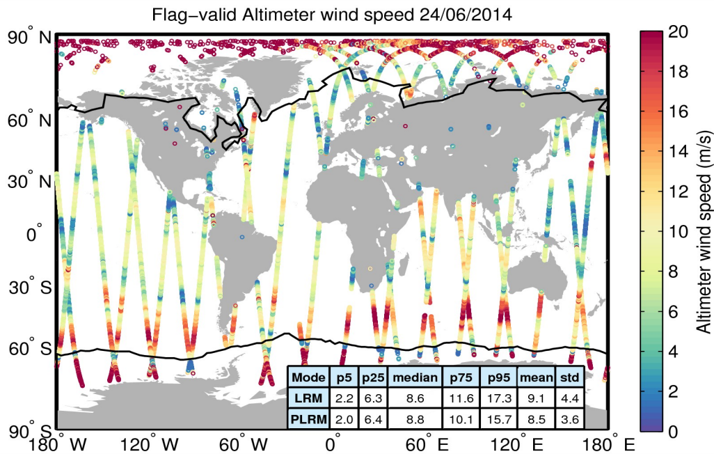
Figure 31. Geographical distribution of flag-valid wind data over oceans and lakes for 24/06/2014. The statistical values shown in the table refer to the wind in m/s and are calculated separately for LRM and PLRM regions. Measurements taken over polar polygons have been excluded from the computation of the statistical values. The black lines mark the outer limit of the Arctic and Antarctic polar polygons.
