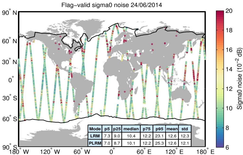
Figure 26. Geographical distribution of flag-valid 20-Hz sigma0 measurement noise over oceans and lakes for 24/06/2014. The statistical values shown in the table refer to the sigma0 noise and are calculated separately for LRM and PLRM regions. Measurements taken over polar polygons have been excluded from the computation of the statistical values. The black lines mark the outer limit of the Arctic and Antarctic polar polygons.
