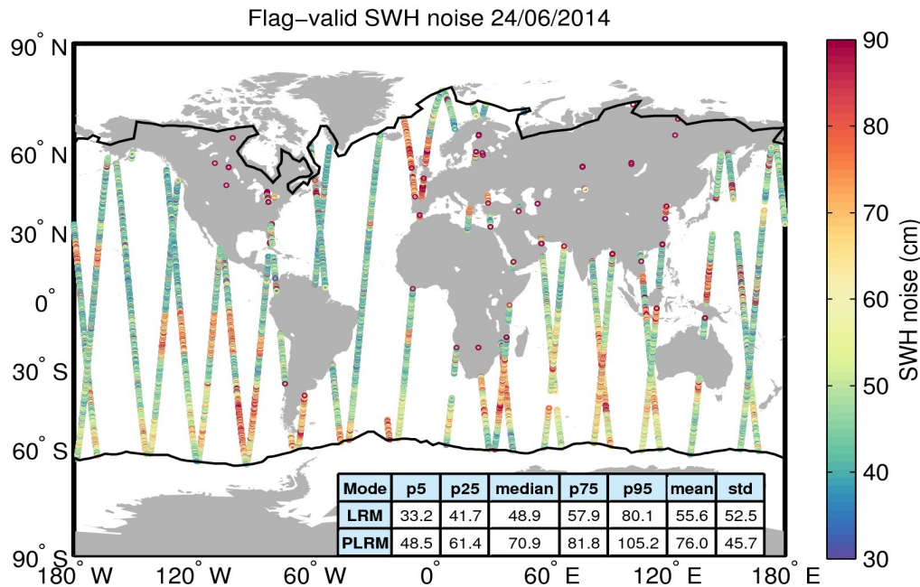
Figure 18. Geographical distribution of flag-valid 20-Hz SWH measurement noise over oceans and lakes for 24/06/2014. The statistical values shown in the table refer to the SWH noise and are calculated separately for LRM and PLRM regions. Measurements taken over polar polygons have been excluded from the computation of the statistical values. The black lines mark the outer limit of the Arctic and Antarctic polar polygons.
