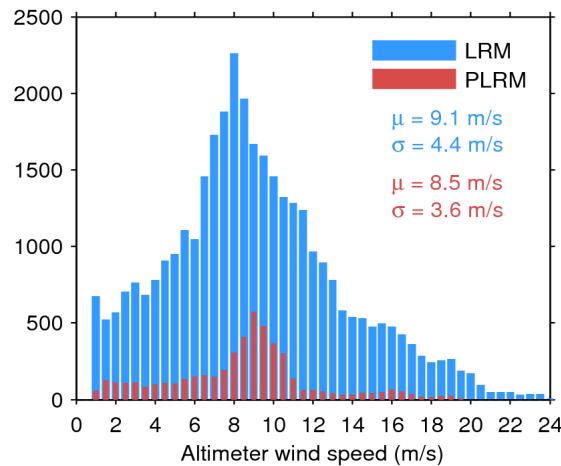
Figure 33. Histogram of flag-valid wind over oceans and lakes for LRM (blue) and PLRM (red) for 24/06/2014. The mean ( \mu ) and standard deviation ( \sigma ) are also shown. Note that values larger than 24 m/s are excluded from the histogram for the sake of readability but not from the computation of \mu and \sigma .
