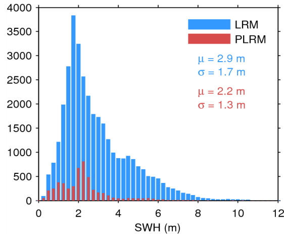
Figure 17. Histogram of flag-valid SWH over oceans and lakes for LRM (blue) and PLRM (red) for 24/06/2014. The mean ( \mu ) and standard deviation ( \sigma ) are also shown. Note that values larger than 12 m are excluded from the histogram for the sake of readability but not from the computation of \mu and \sigma .
