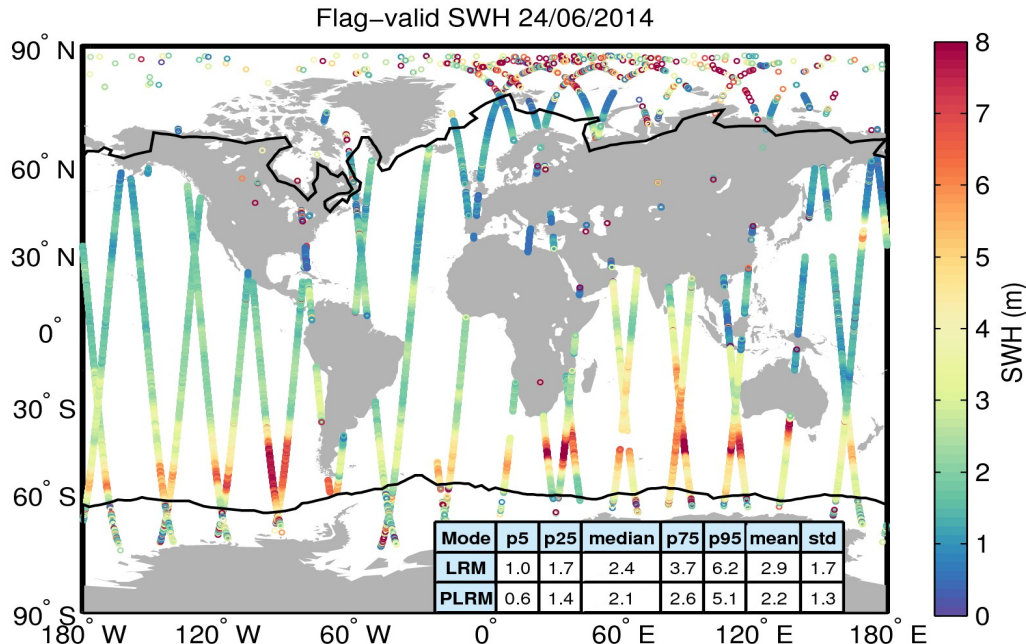
Figure 15. Geographical distribution of flag-valid SWH data over oceans and lakes for 24/06/2014. The statistical values shown in the table refer to the SWH in m and are calculated separately for LRM and PLRM regions. Measurements taken over polar polygons have been excluded from the computation of the statistical values. The black lines mark the outer limit of the Arctic and Antarctic polar polygons.
