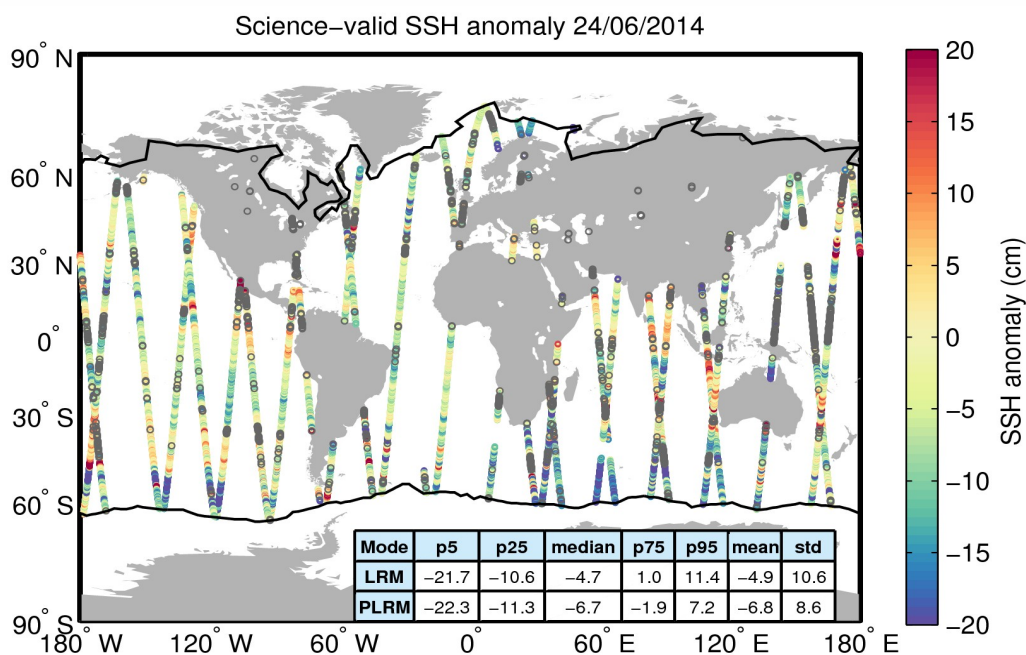
Figure 10. Geographical distribution of science-valid SSH anomaly data over oceans and lakes for 24/06/2014. The statistical values shown in the table refer to the SSH anomaly in cm and are calculated separately for LRM and PLRM regions. The black lines mark the outer limit of the Arctic and Antarctic polar polygons. Gray circles denote records that have been rejected based on the editing criteria described in Table 2.
