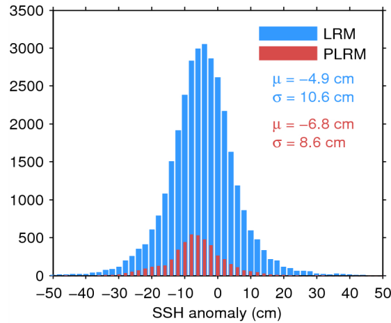
Figure 11. Histogram of science-valid SSH anomaly over oceans and lakes for LRM (blue) and PLRM (red) for 24/06/2014. The mean ( \mu ) and standard deviation ( \sigma ) are also shown. Note that values outside [-50 50] cm are excluded from the histogram for the sake of readability but not from the computation of \mu and \sigma .
