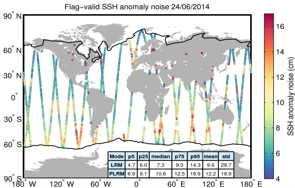
Figure 8. Geographical distribution of flag-valid 20-Hz SSH anomaly measurement noise over oceans and lakes for 24/06/2014. The statistical values shown in the table refer to the SSH anomaly noise and are calculated separately for LRM and PLRM regions. Measurements taken over polar polygons have been excluded from the computation of the statistical values. The black lines mark the outer limit of the Arctic and Antarctic polar polygons.
