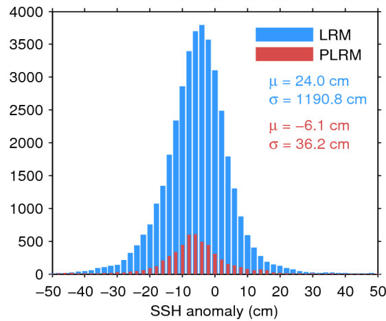
Figure 7. Histogram of flag-valid SSH anomaly over oceans and lakes for LRM (blue) and PLRM (red) for 21/06/2014. The mean ( \mu ) and standard deviation ( \sigma ) are also shown. Note that values outside [-50\ 50] cm are excluded from the histogram for the sake of readability but not from the computation of \mu and \sigma .
