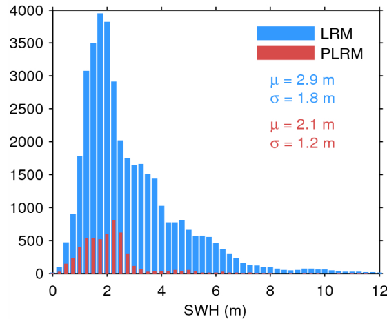
Figure 17. Histogram of flag-valid SWH over oceans and lakes for LRM (blue) and PLRM (red) for 21/06/2014. The mean ( \mu ) and standard deviation ( \sigma ) are also shown. Note that values larger than 12 m are excluded from the histogram for the sake of readability but not from the computation of \mu and \sigma .
