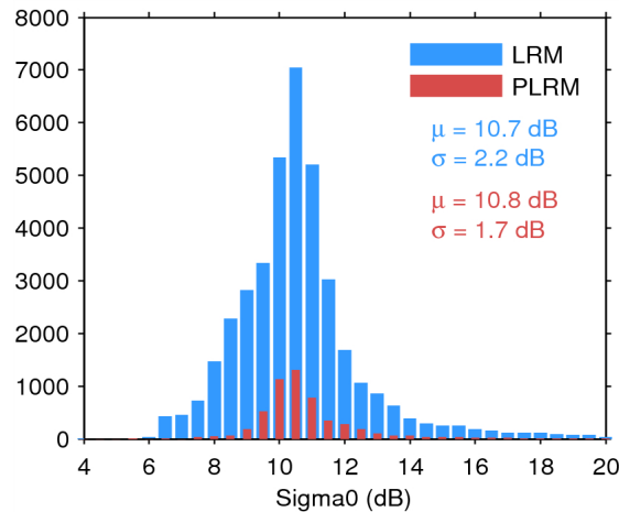
Figure 25. Histogram of flag-valid sigma0 over oceans and lakes for LRM (blue) and PLRM (red) for 21/06/2014. The mean ( \mu ) and standard deviation ( \sigma ) are also shown. Note that values outside [4 20] dB are excluded from the histogram for the sake of readability but not from the computation of \mu and \sigma .
