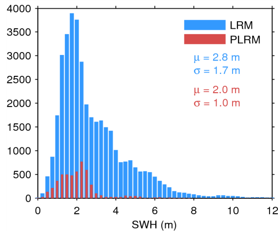
Figure 20. Histogram of science-valid SWH over oceans and lakes for LRM (blue) and PLRM (red) for 21/06/2014. The mean ( \mu ) and standard deviation ( \sigma ) are also shown. Note that values larger than 12 m are excluded from the histogram for the sake of readability but not from the computation of \mu and \sigma .
