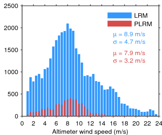
Figure 35. Histogram of science-valid wind over oceans and lakes for LRM (blue) and PLRM (red) for 21/06/2014. The mean ( \mu ) and standard deviation ( \sigma ) are also shown. Note that values larger than 24 m/s are excluded from the histogram for the sake of readability but not from the computation of \mu and \sigma .
