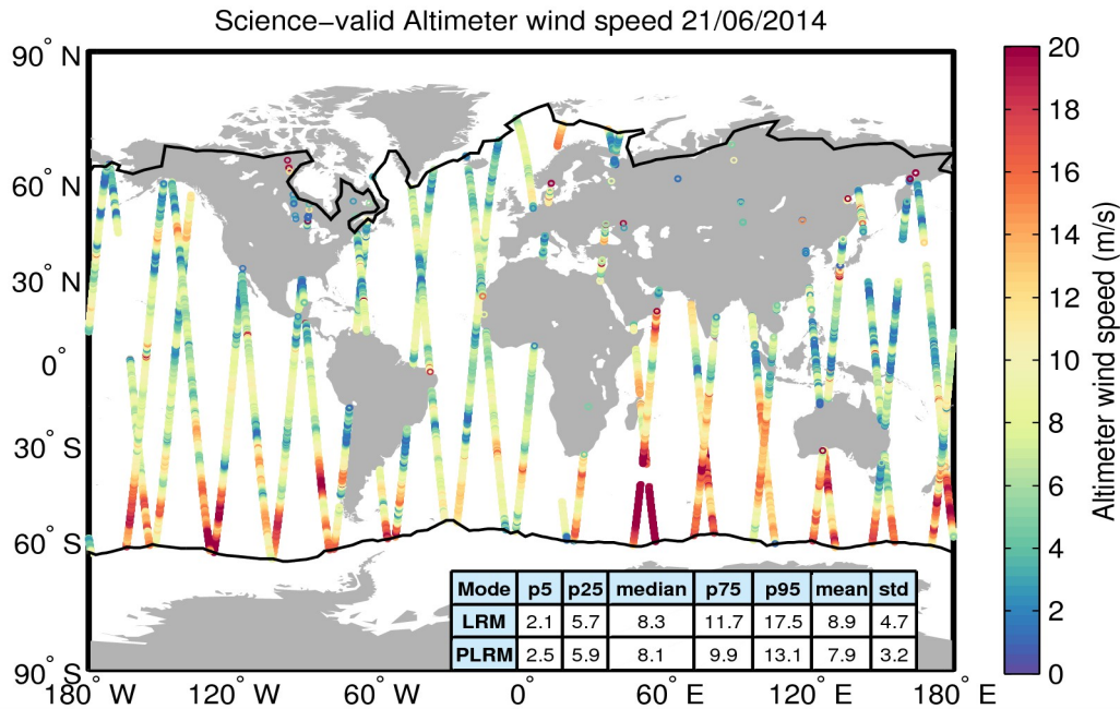
Figure 34. Geographical distribution of science-valid wind data over oceans and lakes for 21/06/2014. The statistical values shown in the table refer to the wind in m/s and are calculated separately for LRM and PLRM regions. The black lines mark the outer limit of the Arctic and Antarctic polar polygons. Gray circles denote records that have been rejected based on the editing criteria described in Table 5.
