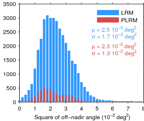
Figure 39. Histogram of flag-valid mispointing over oceans and lakes for LRM (blue) and PLRM (red) for 21/06/2014. Only positive values have been considered. The mean ( \mu ) and standard deviation ( \sigma ) are also shown. Note that values 8 \cdot 10^{-2} \text{ deg}^2 are excluded from the histogram for the sake of readability but not from the computation of \mu and \sigma .
