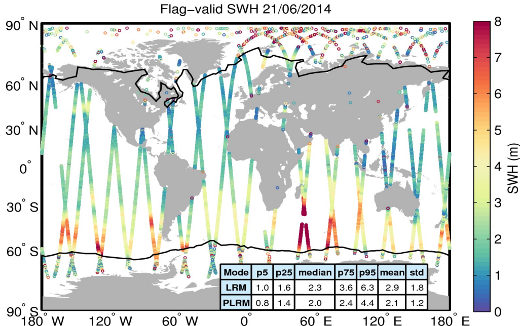
Figure 15. Geographical distribution of flag-valid SWH data over oceans and lakes for 21/06/2014. The statistical values shown in the table refer to the SWH in m and are calculated separately for LRM and PLRM regions. Measurements taken over polar polygons have been excluded from the computation of the statistical values. The black lines mark the outer limit of the Arctic and Antarctic polar polygons.
