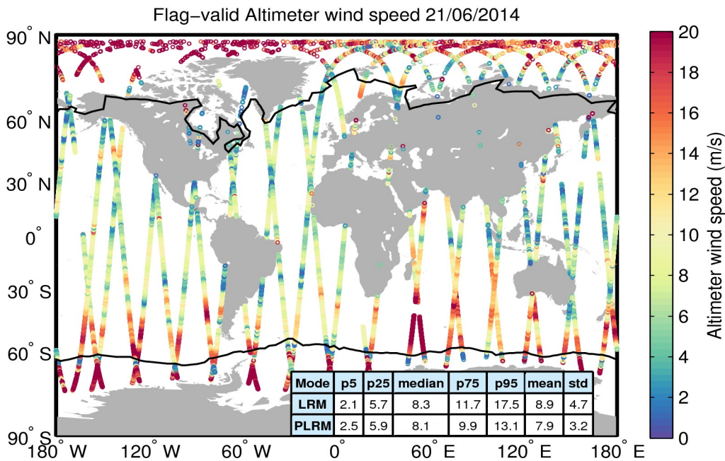
Figure 31. Geographical distribution of flag-valid wind data over oceans and lakes for 21/06/2014. The statistical values shown in the table refer to the wind in m/s and are calculated separately for LRM and PLRM regions. Measurements taken over polar polygons have been excluded from the computation of the statistical values. The black lines mark the outer limit of the Arctic and Antarctic polar polygons.
