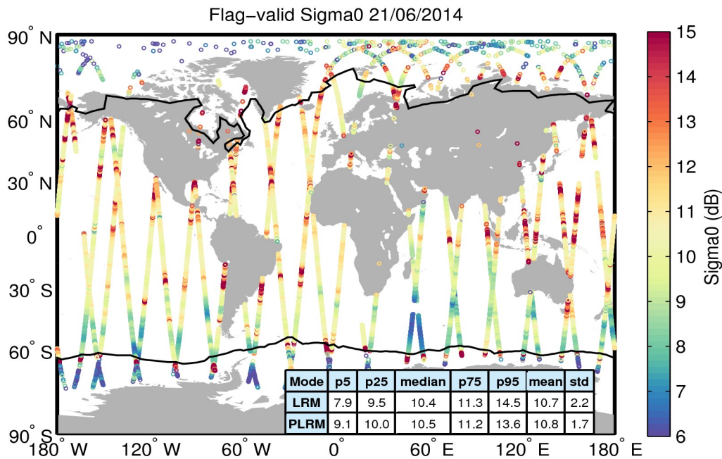
Figure 23. Geographical distribution of flag-valid sigma0 data over oceans and lakes for 21/06/2014. The statistical values shown in the table refer to the sigma0 in dB and are calculated separately for LRM and PLRM regions. Measurements taken over polar polygons have been excluded from the computation of the statistical values. The black lines mark the outer limit of the Arctic and Antarctic polar polygons.
