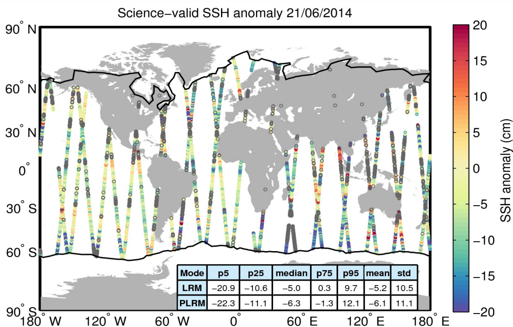
Figure 10. Geographical distribution of science-valid SSH anomaly data over oceans and lakes for 21/06/2014. The statistical values shown in the table refer to the SSH anomaly in cm and are calculated separately for LRM and PLRM regions. The black lines mark the outer limit of the Arctic and Antarctic polar polygons. Gray circles denote records that have been rejected based on the editing criteria described in Table 2.
