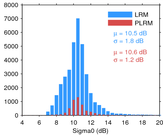
Figure 28. Histogram of science-valid sigma0 over oceans and lakes for LRM (blue) and PLRM (red) for 21/06/2014. The mean ( \mu ) and standard deviation ( \sigma ) are also shown. Note that values outside [4 20] dB are excluded from the histogram for the sake of readability but not from the computation of \mu and \sigma .
