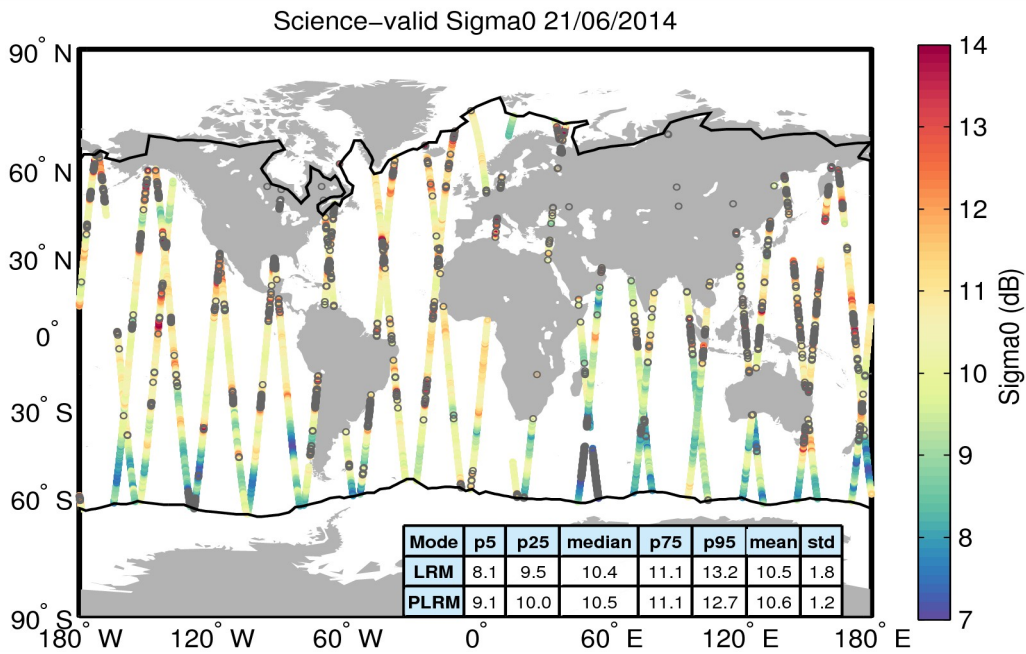
Figure 27. Geographical distribution of science-valid sigma0 data over oceans and lakes for 21/06/2014. The statistical values shown in the table refer to the sigma0 in dB and are calculated separately for LRM and PLRM regions. The black lines mark the outer limit of the Arctic and Antarctic polar polygons. Gray circles denote records that have been rejected based on the editing criteria described in Table 4.
