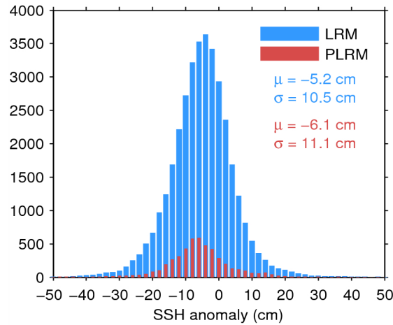
Figure 11. Histogram of science-valid SSH anomaly over oceans and lakes for LRM (blue) and PLRM (red) for 21/06/2014. The mean ( \mu ) and standard deviation ( \sigma ) are also shown. Note that values outside [-50 50] cm are excluded from the histogram for the sake of readability but not from the computation of \mu and \sigma .
