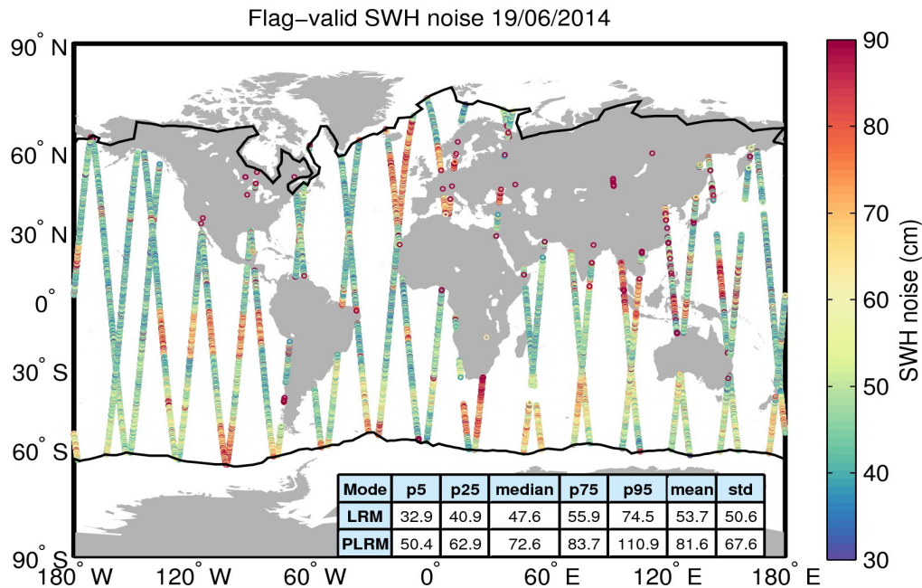
Figure 18. Geographical distribution of flag-valid 20-Hz SWH measurement noise over oceans and lakes for 19/06/2014. The statistical values shown in the table refer to the SWH noise and are calculated separately for LRM and PLRM regions. Measurements taken over polar polygons have been excluded from the computation of the statistical values. The black lines mark the outer limit of the Arctic and Antarctic polar polygons.
