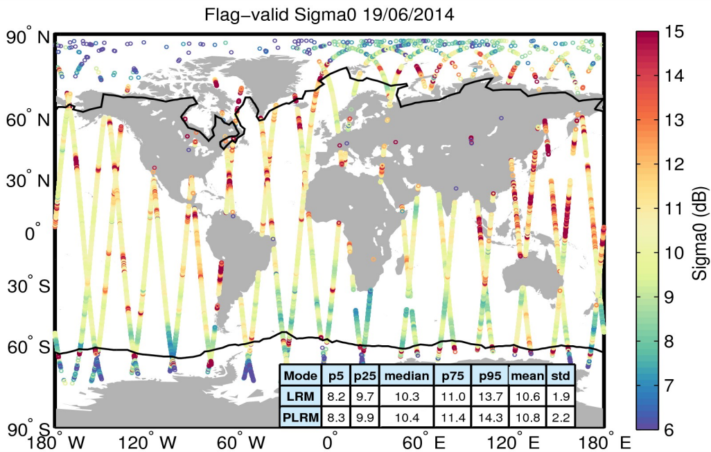
Figure 23. Geographical distribution of flag-valid sigma0 data over oceans and lakes for 19/06/2014. The statistical values shown in the table refer to the sigma0 in dB and are calculated separately for LRM and PLRM regions. Measurements taken over polar polygons have been excluded from the computation of the statistical values. The black lines mark the outer limit of the Arctic and Antarctic polar polygons.
