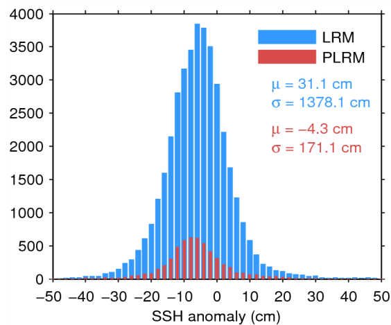
Figure 7. Histogram of flag-valid SSH anomaly over oceans and lakes for LRM (blue) and PLRM (red) for 19/06/2014. The mean ( \mu ) and standard deviation ( \sigma ) are also shown. Note that values outside [-50\ 50] cm are excluded from the histogram for the sake of readability but not from the computation of \mu and \sigma .
