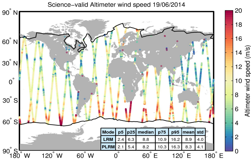
Figure 34. Geographical distribution of science-valid wind data over oceans and lakes for 19/06/2014. The statistical values shown in the table refer to the wind in m/s and are calculated separately for LRM and PLRM regions. The black lines mark the outer limit of the Arctic and Antarctic polar polygons. Gray circles denote records that have been rejected based on the editing criteria described in Table 5.
