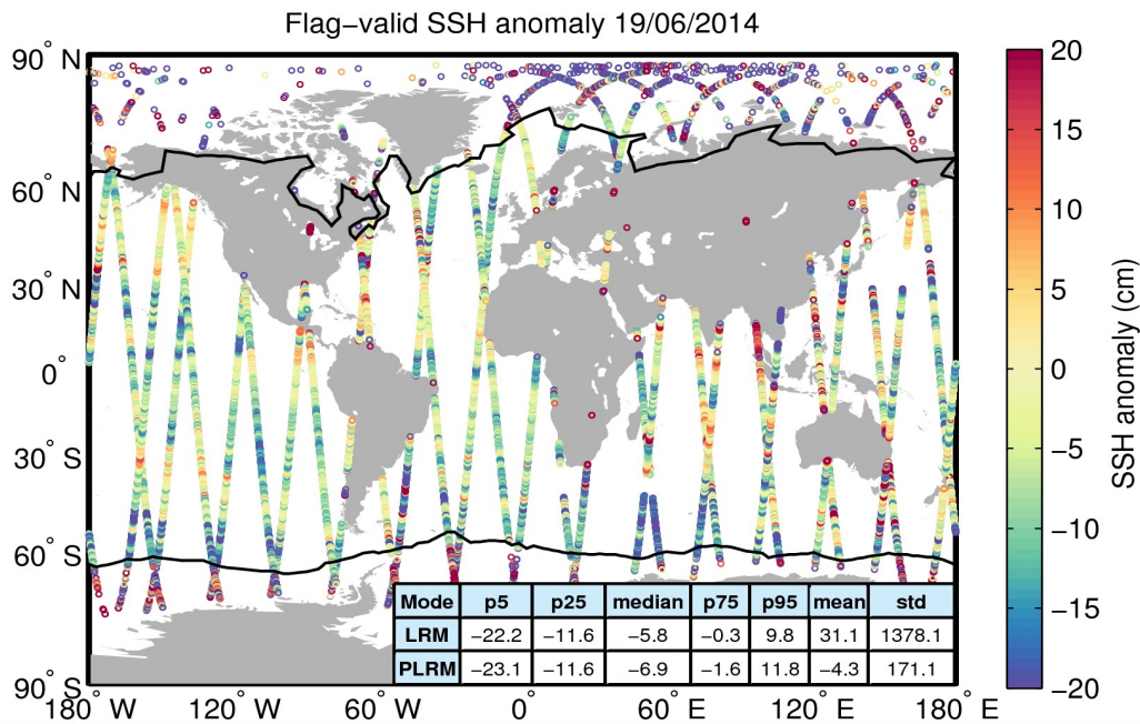
Figure 5. Geographical distribution of flag-valid 1-Hz SSH anomaly data over oceans and lakes for 19/06/2014. The statistical values shown in the table refer to the SSH anomaly in cm and are calculated separately for LRM and PLRM regions. Measurements taken over polar polygons have been excluded from the computation of the statistical values. The black lines mark the outer limit of the Arctic and Antarctic polar polygons.
