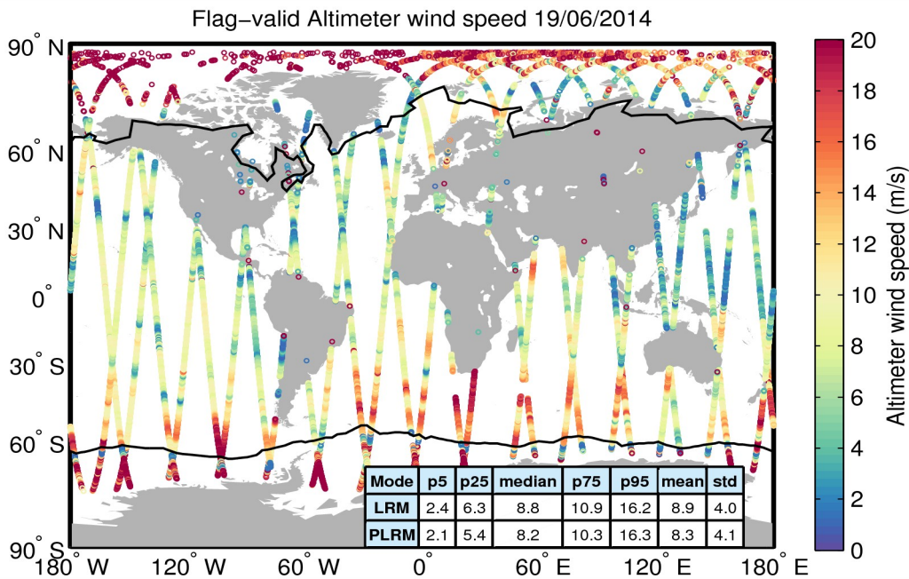
Figure 31. Geographical distribution of flag-valid wind data over oceans and lakes for 19/06/2014. The statistical values shown in the table refer to the wind in m/s and are calculated separately for LRM and PLRM regions. Measurements taken over polar polygons have been excluded from the computation of the statistical values. The black lines mark the outer limit of the Arctic and Antarctic polar polygons.
