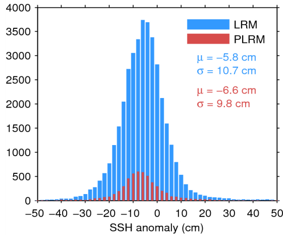
Figure 11. Histogram of science-valid SSH anomaly over oceans and lakes for LRM (blue) and PLRM (red) for 19/06/2014. The mean ( \mu ) and standard deviation ( \sigma ) are also shown. Note that values outside [-50\ 50] cm are excluded from the histogram for the sake of readability but not from the computation of \mu and \sigma .
