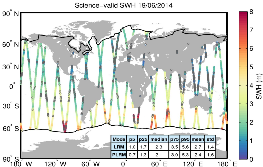
Figure 19. Geographical distribution of science-valid SWH data over oceans and lakes for 19/06/2014. The statistical values shown in the table refer to the SWH in m and are calculated separately for LRM and PLRM regions. The black lines mark the outer limit of the Arctic and Antarctic polar polygons. Gray circles denote records that have been rejected based on the editing criteria described in Table 3.
