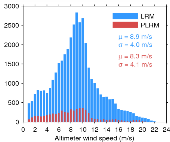
Figure 33. Histogram of flag-valid wind over oceans and lakes for LRM (blue) and PLRM (red) for 19/06/2014. The mean ( \mu ) and standard deviation ( \sigma ) are also shown. Note that values larger than 24 m/s are excluded from the histogram for the sake of readability but not from the computation of \mu and \sigma .
