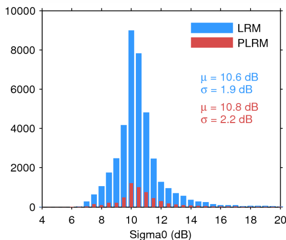
Figure 25. Histogram of flag-valid sigma0 over oceans and lakes for LRM (blue) and PLRM (red) for 19/06/2014. The mean ( \mu ) and standard deviation ( \sigma ) are also shown. Note that values outside [4 20] dB are excluded from the histogram for the sake of readability but not from the computation of \mu and \sigma .
