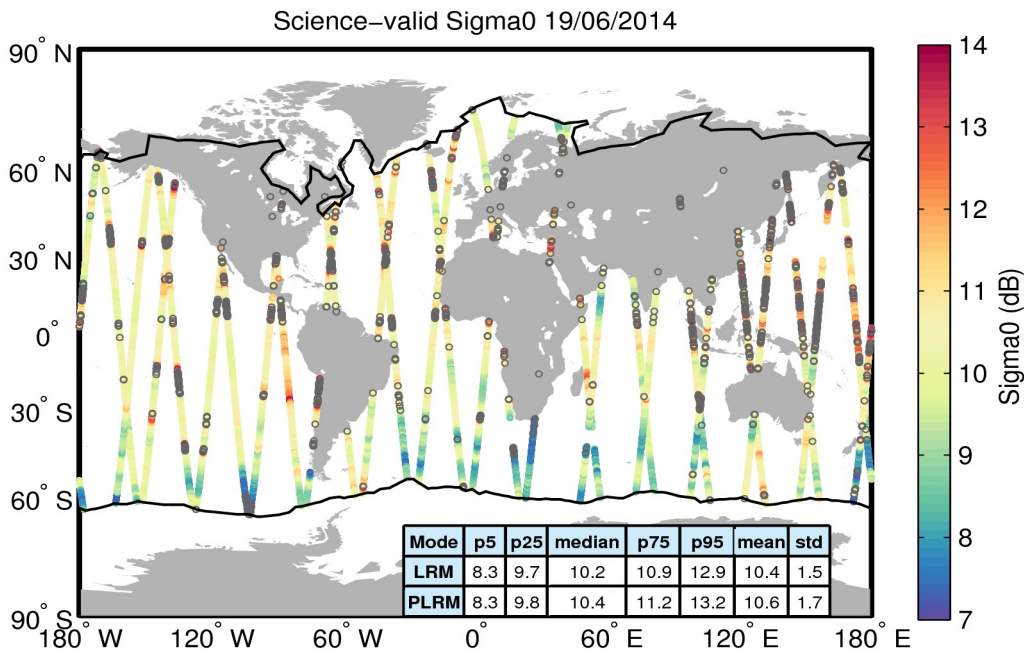
Figure 27. Geographical distribution of science-valid sigma0 data over oceans and lakes for 19/06/2014. The statistical values shown in the table refer to the sigma0 in dB and are calculated separately for LRM and PLRM regions. The black lines mark the outer limit of the Arctic and Antarctic polar polygons. Gray circles denote records that have been rejected based on the editing criteria described in Table 4.
