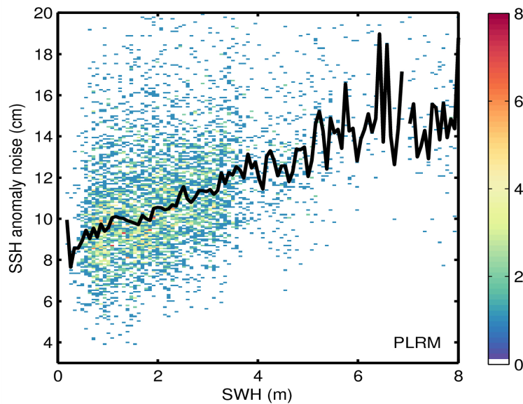
Figure 9. 2D histogram showing flag-valid SSH anomaly noise as a function of SWH for LRM (top) and PLRM (bottom) for 19/06/2014. The black line denotes the median SSH anomaly as a function of SWH.
