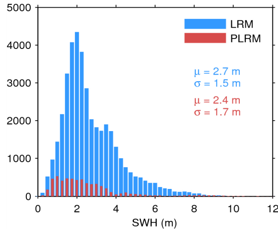
Figure 17. Histogram of flag-valid SWH over oceans and lakes for LRM (blue) and PLRM (red) for 19/06/2014. The mean ( \mu ) and standard deviation ( \sigma ) are also shown. Note that values larger than 12 m are excluded from the histogram for the sake of readability but not from the computation of \mu and \sigma .
