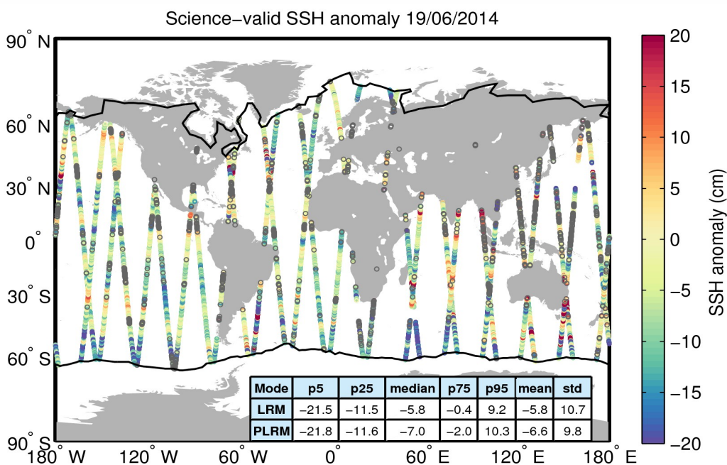
Figure 10. Geographical distribution of science-valid SSH anomaly data over oceans and lakes for 19/06/2014. The statistical values shown in the table refer to the SSH anomaly in cm and are calculated separately for LRM and PLRM regions. The black lines mark the outer limit of the Arctic and Antarctic polar polygons. Gray circles denote records that have been rejected based on the editing criteria described in Table 2.
