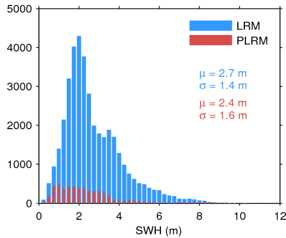
Figure 20. Histogram of science-valid SWH over oceans and lakes for LRM (blue) and PLRM (red) for 19/06/2014. The mean ( \mu ) and standard deviation ( \sigma ) are also shown. Note that values larger than 12 m are excluded from the histogram for the sake of readability but not from the computation of \mu and \sigma .
