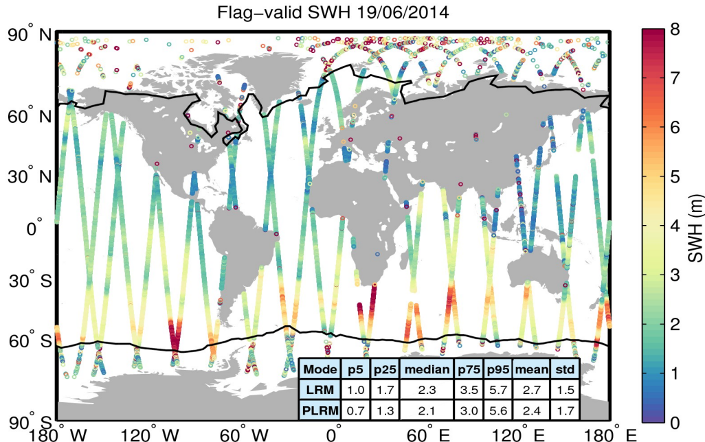
Figure 15. Geographical distribution of flag-valid SWH data over oceans and lakes for 19/06/2014. The statistical values shown in the table refer to the SWH in m and are calculated separately for LRM and PLRM regions. Measurements taken over polar polygons have been excluded from the computation of the statistical values. The black lines mark the outer limit of the Arctic and Antarctic polar polygons.
