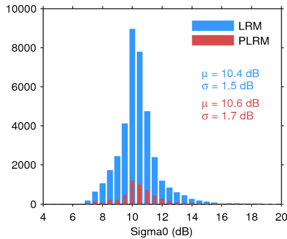
Figure 28. Histogram of science-valid sigma0 over oceans and lakes for LRM (blue) and PLRM (red) for 19/06/2014. The mean ( \mu ) and standard deviation ( \sigma ) are also shown. Note that values outside [4 20] dB are excluded from the histogram for the sake of readability but not from the computation of \mu and \sigma .
