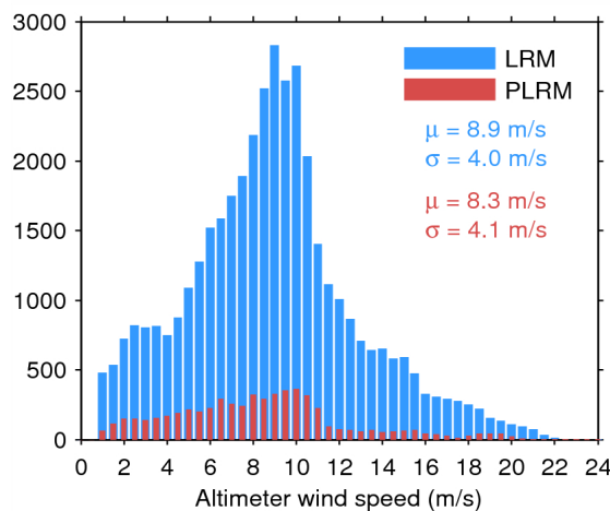
Figure 35. Histogram of science-valid wind over oceans and lakes for LRM (blue) and PLRM (red) for 19/06/2014. The mean ( \mu ) and standard deviation ( \sigma ) are also shown. Note that values larger than 24 m/s are excluded from the histogram for the sake of readability but not from the computation of \mu and \sigma .
