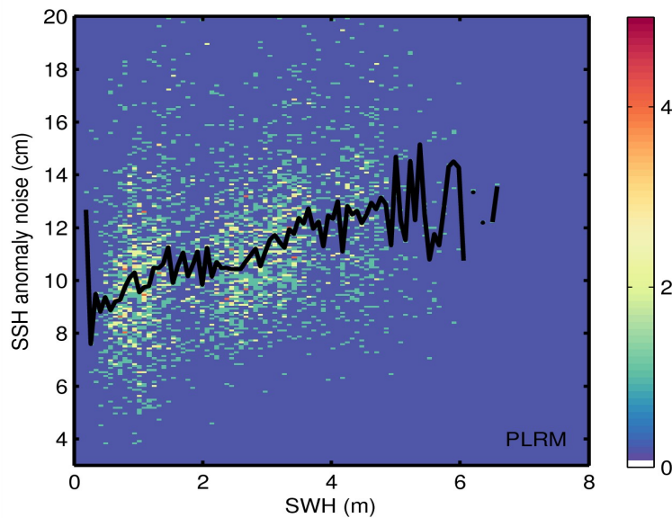
Figure 9. 2D histogram showing flag-valid SSH anomaly noise as a function of SWH for LRM (top) and PLRM (bottom) for 18/06/2014. The black line denotes the median SSH anomaly as a function of SWH.
