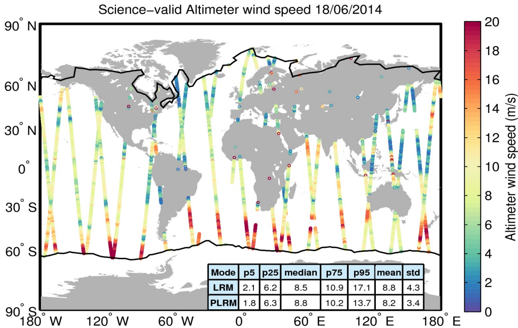
Figure 34. Geographical distribution of science-valid wind data over oceans and lakes for 18/06/2014. The statistical values shown in the table refer to the wind in m/s and are calculated separately for LRM and PLRM regions. The black lines mark the outer limit of the Arctic and Antarctic polar polygons. Gray circles denote records that have been rejected based on the editing criteria described in Table 5.
