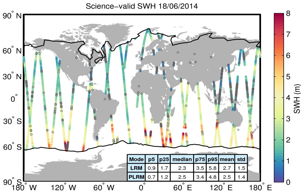
Figure 19. Geographical distribution of science-valid SWH data over oceans and lakes for 18/06/2014. The statistical values shown in the table refer to the SWH in m and are calculated separately for LRM and PLRM regions. The black lines mark the outer limit of the Arctic and Antarctic polar polygons. Gray circles denote records that have been rejected based on the editing criteria described in Table 3.
