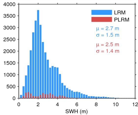
Figure 20. Histogram of science-valid SWH over oceans and lakes for LRM (blue) and PLRM (red) for 18/06/2014. The mean ( \mu ) and standard deviation ( \sigma ) are also shown. Note that values larger than 12 m are excluded from the histogram for the sake of readability but not from the computation of \mu and \sigma .
