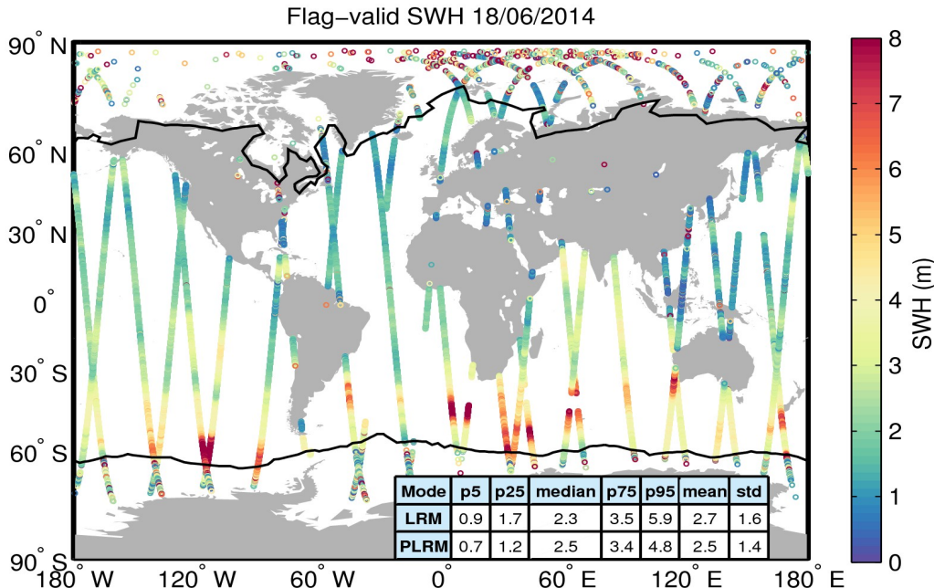
Figure 15. Geographical distribution of flag-valid SWH data over oceans and lakes for 18/06/2014. The statistical values shown in the table refer to the SWH in m and are calculated separately for LRM and PLRM regions. Measurements taken over polar polygons have been excluded from the computation of the statistical values. The black lines mark the outer limit of the Arctic and Antarctic polar polygons.
