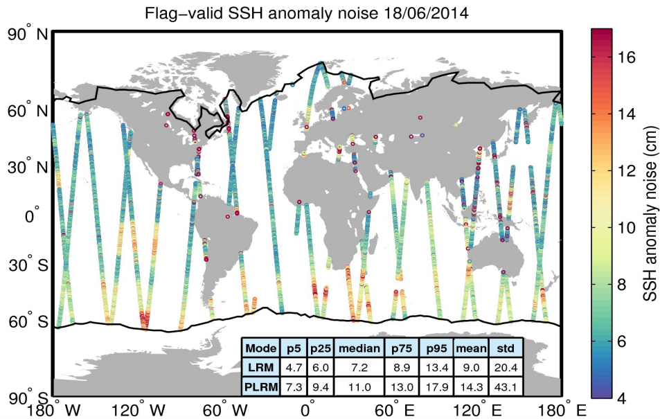
Figure 8. Geographical distribution of flag-valid 20-Hz SSH anomaly measurement noise over oceans and lakes for 18/06/2014. The statistical values shown in the table refer to the SSH anomaly noise and are calculated separately for LRM and PLRM regions. Measurements taken over polar polygons have been excluded from the computation of the statistical values. The black lines mark the outer limit of the Arctic and Antarctic polar polygons.
