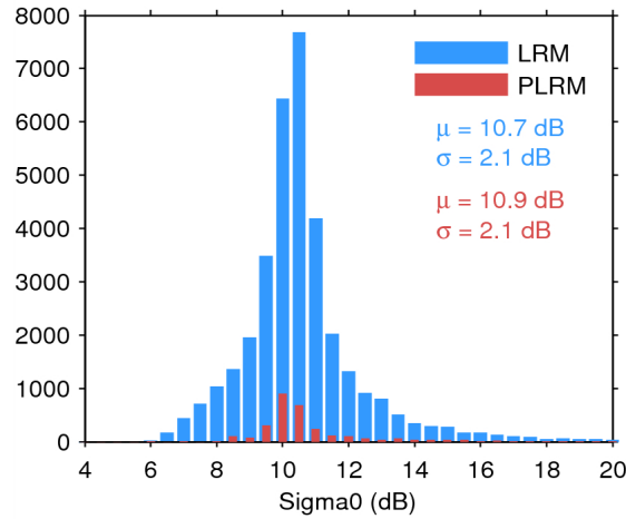
Figure 25. Histogram of flag-valid sigma0 over oceans and lakes for LRM (blue) and PLRM (red) for 18/06/2014. The mean ( \mu ) and standard deviation ( \sigma ) are also shown. Note that values outside [4 20] dB are excluded from the histogram for the sake of readability but not from the computation of \mu and \sigma .
