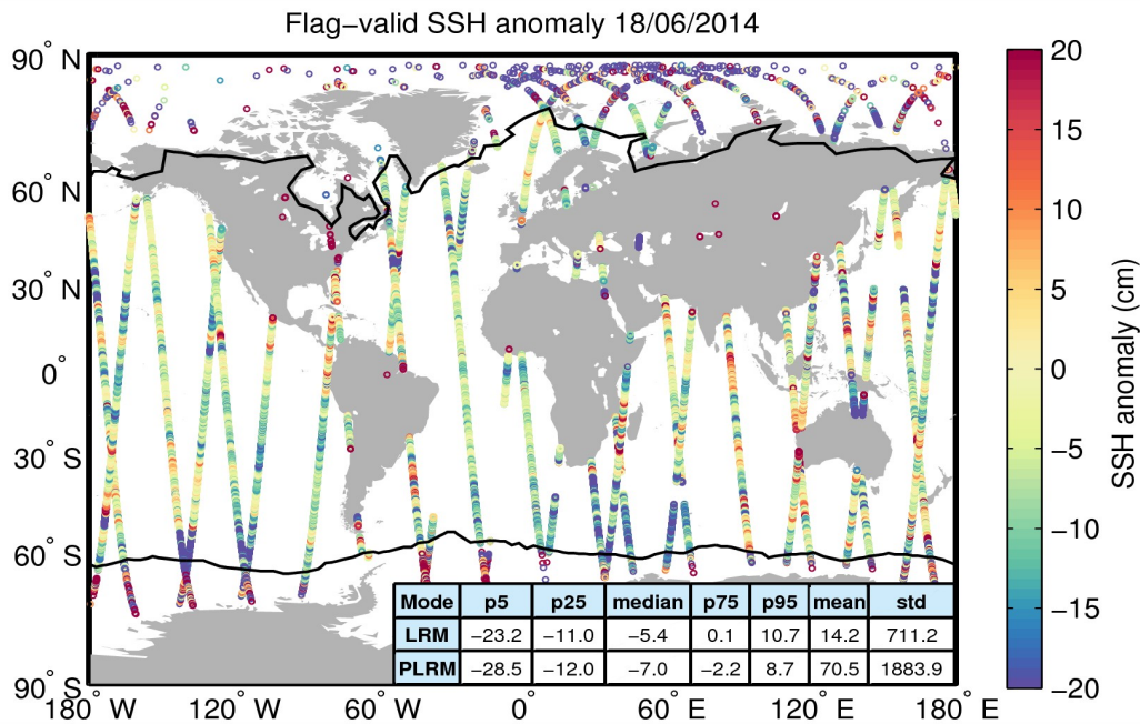
Figure 5. Geographical distribution of flag-valid 1-Hz SSH anomaly data over oceans and lakes for 18/06/2014. The statistical values shown in the table refer to the SSH anomaly in cm and are calculated separately for LRM and PLRM regions. Measurements taken over polar polygons have been excluded from the computation of the statistical values. The black lines mark the outer limit of the Arctic and Antarctic polar polygons.
