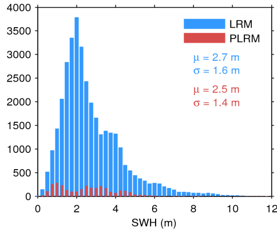
Figure 17. Histogram of flag-valid SWH over oceans and lakes for LRM (blue) and PLRM (red) for 18/06/2014. The mean ( \mu ) and standard deviation ( \sigma ) are also shown. Note that values larger than 12 m are excluded from the histogram for the sake of readability but not from the computation of \mu and \sigma .
