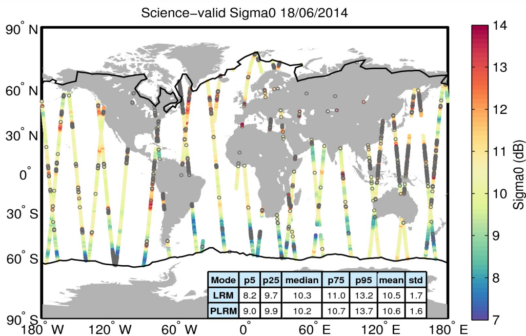
Figure 27. Geographical distribution of science-valid sigma0 data over oceans and lakes for 18/06/2014. The statistical values shown in the table refer to the sigma0 in dB and are calculated separately for LRM and PLRM regions. The black lines mark the outer limit of the Arctic and Antarctic polar polygons. Gray circles denote records that have been rejected based on the editing criteria described in Table 4.
