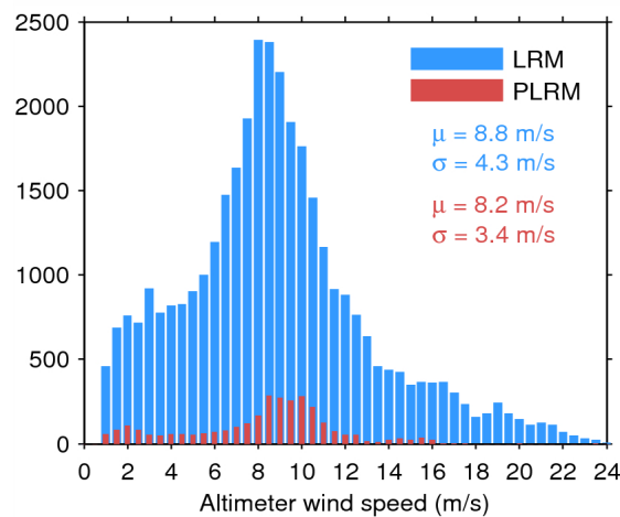
Figure 33. Histogram of flag-valid wind over oceans and lakes for LRM (blue) and PLRM (red) for 18/06/2014. The mean ( \mu ) and standard deviation ( \sigma ) are also shown. Note that values larger than 24 m/s are excluded from the histogram for the sake of readability but not from the computation of \mu and \sigma .
