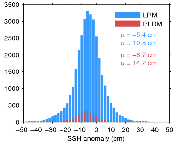
Figure 11. Histogram of science-valid SSH anomaly over oceans and lakes for LRM (blue) and PLRM (red) for 18/06/2014. The mean ( \mu ) and standard deviation ( \sigma ) are also shown. Note that values outside [-50 50] cm are excluded from the histogram for the sake of readability but not from the computation of \mu and \sigma .
