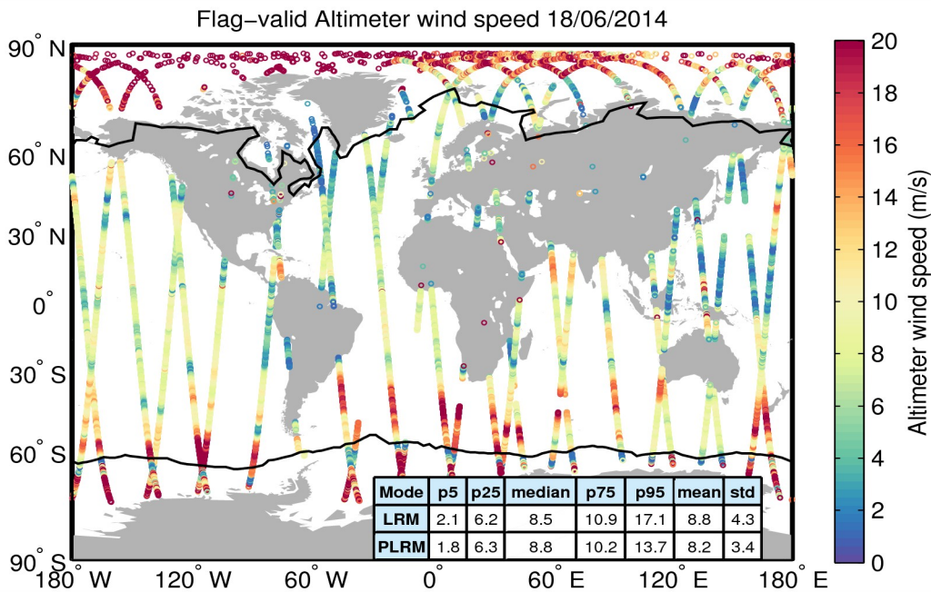
Figure 31. Geographical distribution of flag-valid wind data over oceans and lakes for 18/06/2014. The statistical values shown in the table refer to the wind in m/s and are calculated separately for LRM and PLRM regions. Measurements taken over polar polygons have been excluded from the computation of the statistical values. The black lines mark the outer limit of the Arctic and Antarctic polar polygons.
