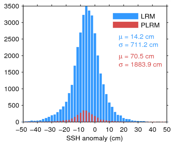
Figure 7. Histogram of flag-valid SSH anomaly over oceans and lakes for LRM (blue) and PLRM (red) for 18/06/2014. The mean ( \mu ) and standard deviation ( \sigma ) are also shown. Note that values outside [-50\ 50] cm are excluded from the histogram for the sake of readability but not from the computation of \mu and \sigma .
