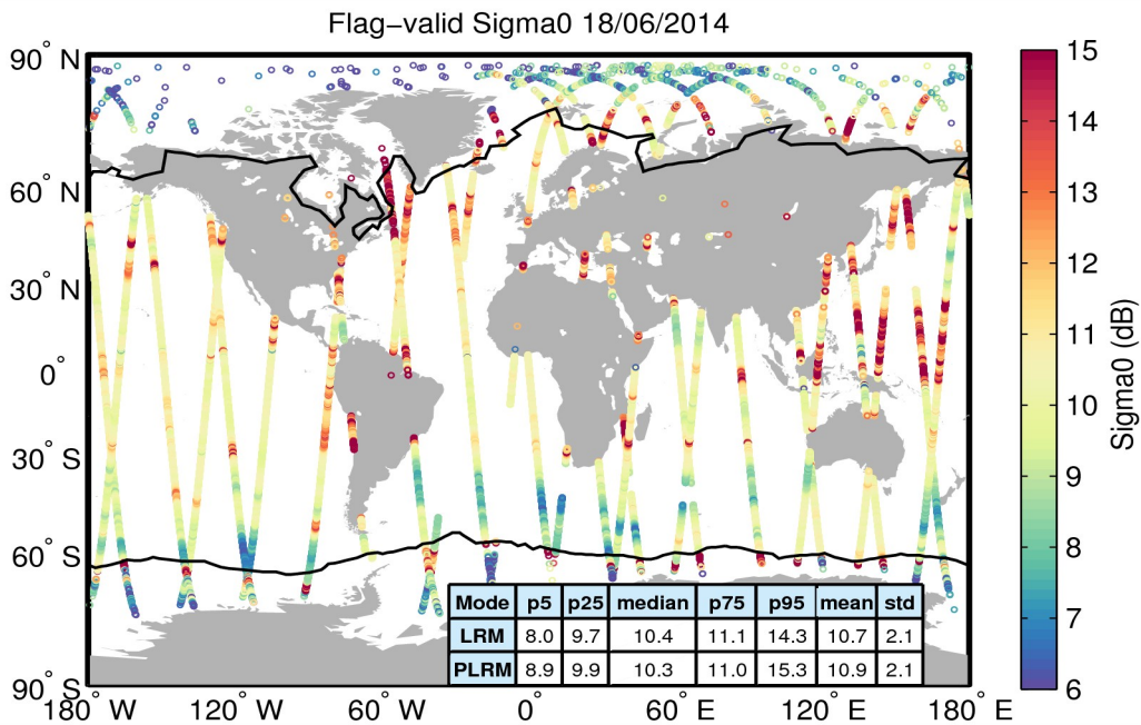
Figure 23. Geographical distribution of flag-valid sigma0 data over oceans and lakes for 18/06/2014. The statistical values shown in the table refer to the sigma0 in dB and are calculated separately for LRM and PLRM regions. Measurements taken over polar polygons have been excluded from the computation of the statistical values. The black lines mark the outer limit of the Arctic and Antarctic polar polygons.
