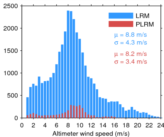
Figure 35. Histogram of science-valid wind over oceans and lakes for LRM (blue) and PLRM (red) for 18/06/2014. The mean ( \mu ) and standard deviation ( \sigma ) are also shown. Note that values larger than 24 m/s are excluded from the histogram for the sake of readability but not from the computation of \mu and \sigma .
