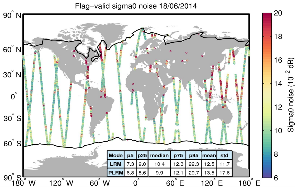
Figure 26. Geographical distribution of flag-valid 20-Hz sigma0 measurement noise over oceans and lakes for 18/06/2014. The statistical values shown in the table refer to the sigma0 noise and are calculated separately for LRM and PLRM regions. Measurements taken over polar polygons have been excluded from the computation of the statistical values. The black lines mark the outer limit of the Arctic and Antarctic polar polygons.
