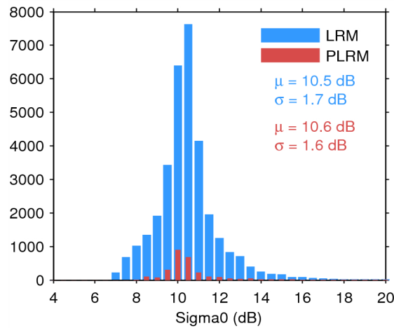
Figure 28. Histogram of science-valid sigma0 over oceans and lakes for LRM (blue) and PLRM (red) for 18/06/2014. The mean ( \mu ) and standard deviation ( \sigma ) are also shown. Note that values outside [4 20] dB are excluded from the histogram for the sake of readability but not from the computation of \mu and \sigma .
