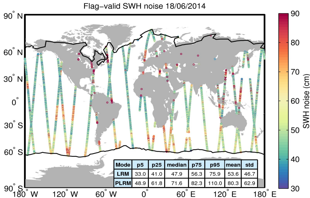
Figure 18. Geographical distribution of flag-valid 20-Hz SWH measurement noise over oceans and lakes for 18/06/2014. The statistical values shown in the table refer to the SWH noise and are calculated separately for LRM and PLRM regions. Measurements taken over polar polygons have been excluded from the computation of the statistical values. The black lines mark the outer limit of the Arctic and Antarctic polar polygons.
