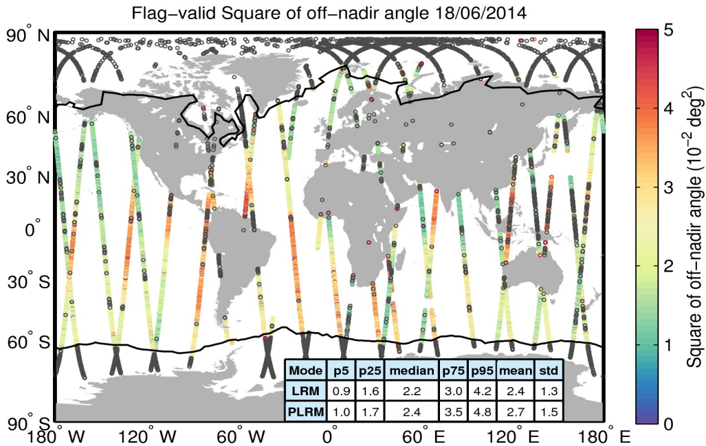
Figure 37. Geographical distribution of flag-valid mispointing data over oceans and lakes for 18/06/2014. The statistical values shown in the table refer to the mispointing in 10^{-2} deg 2 and are calculated separately for LRM and PLRM regions. Measurements taken over polar polygons have been excluded from the computation of the statistical values. The black lines mark the outer limit of the Arctic and Antarctic polar polygons. Gray circles denote negative values.
