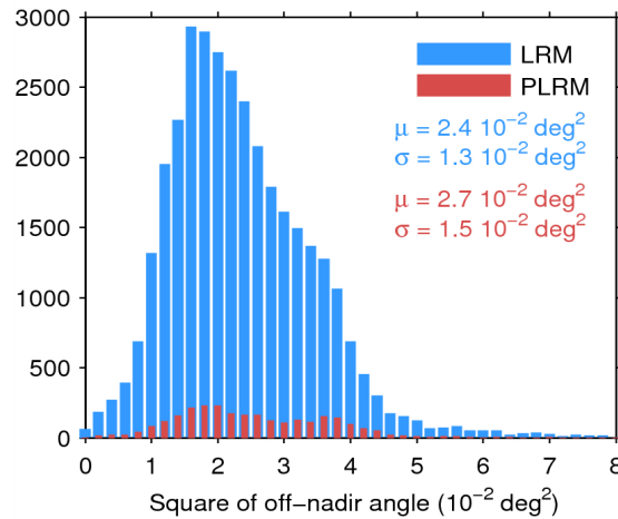
Figure 39. Histogram of flag-valid mispointing over oceans and lakes for LRM (blue) and PLRM (red) for 18/06/2014. Only positive values have been considered. The mean ( \mu ) and standard deviation ( \sigma ) are also shown. Note that values 8 \cdot 10^{-2} \text{ deg}^2 are excluded from the histogram for the sake of readability but not from the computation of \mu and \sigma .
