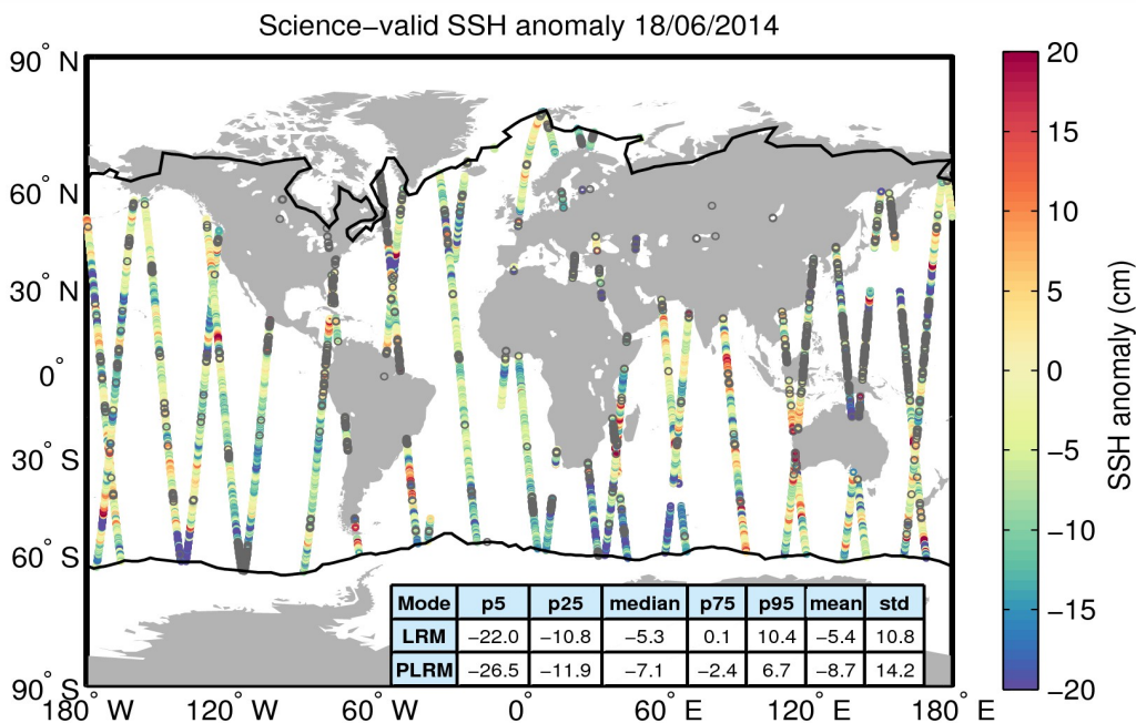
Figure 10. Geographical distribution of science-valid SSH anomaly data over oceans and lakes for 18/06/2014. The statistical values shown in the table refer to the SSH anomaly in cm and are calculated separately for LRM and PLRM regions. The black lines mark the outer limit of the Arctic and Antarctic polar polygons. Gray circles denote records that have been rejected based on the editing criteria described in Table 2.
