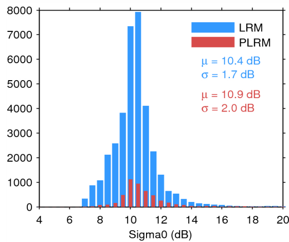
Figure 28. Histogram of science-valid sigma0 over oceans and lakes for LRM (blue) and PLRM (red) for 17/06/2014. The mean ( \mu ) and standard deviation ( \sigma ) are also shown. Note that values outside [4 20] dB are excluded from the histogram for the sake of readability but not from the computation of \mu and \sigma .
