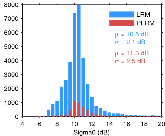
Figure 25. Histogram of flag-valid sigma0 over oceans and lakes for LRM (blue) and PLRM (red) for 17/06/2014. The mean ( \mu ) and standard deviation ( \sigma ) are also shown. Note that values outside [4 20] dB are excluded from the histogram for the sake of readability but not from the computation of \mu and \sigma .
