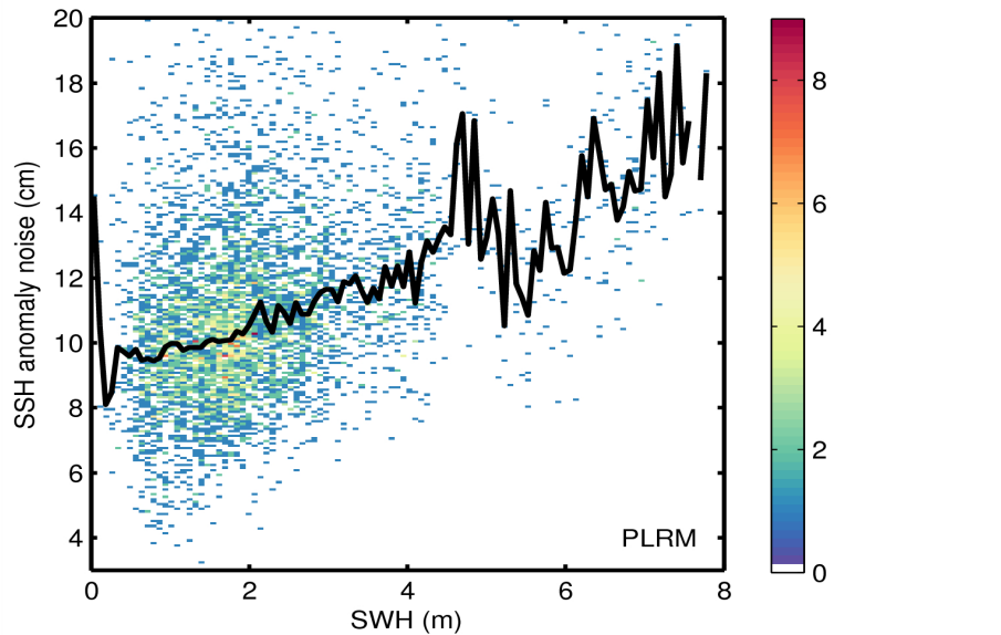
Figure 9. 2D histogram showing flag-valid SSH anomaly noise as a function of SWH for LRM (top) and PLRM (bottom) for 17/06/2014. The black line denotes the median SSH anomaly as a function of SWH.
