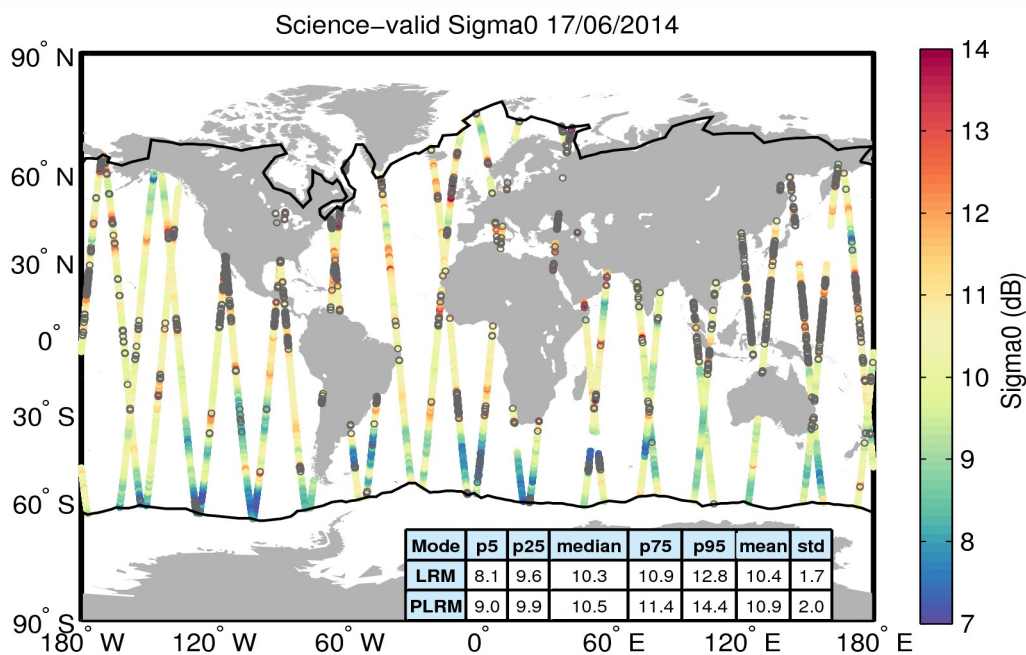
Figure 27. Geographical distribution of science-valid sigma0 data over oceans and lakes for 17/06/2014. The statistical values shown in the table refer to the sigma0 in dB and are calculated separately for LRM and PLRM regions. The black lines mark the outer limit of the Arctic and Antarctic polar polygons. Gray circles denote records that have been rejected based on the editing criteria described in Table 4.
