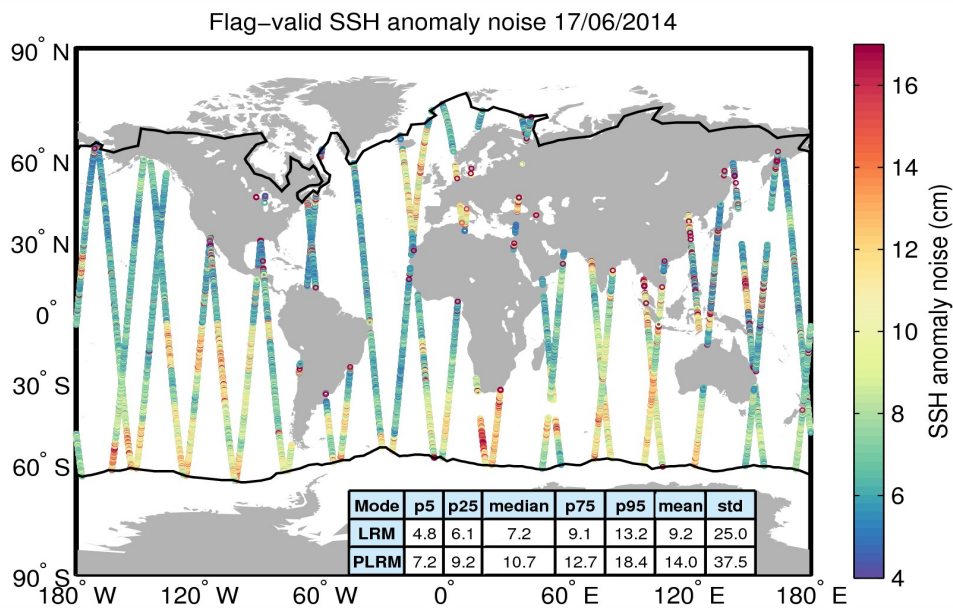
Figure 8. Geographical distribution of flag-valid 20-Hz SSH anomaly measurement noise over oceans and lakes for 17/06/2014. The statistical values shown in the table refer to the SSH anomaly noise and are calculated separately for LRM and PLRM regions. Measurements taken over polar polygons have been excluded from the computation of the statistical values. The black lines mark the outer limit of the Arctic and Antarctic polar polygons.
