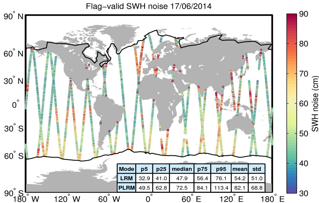
Figure 18. Geographical distribution of flag-valid 20-Hz SWH measurement noise over oceans and lakes for 17/06/2014. The statistical values shown in the table refer to the SWH noise and are calculated separately for LRM and PLRM regions. Measurements taken over polar polygons have been excluded from the computation of the statistical values. The black lines mark the outer limit of the Arctic and Antarctic polar polygons.
