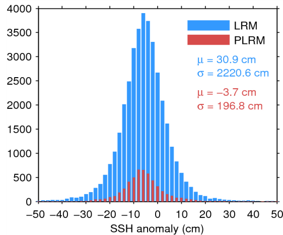
Figure 7. Histogram of flag-valid SSH anomaly over oceans and lakes for LRM (blue) and PLRM (red) for 17/06/2014. The mean ( \mu ) and standard deviation ( \sigma ) are also shown. Note that values outside [-50\ 50] cm are excluded from the histogram for the sake of readability but not from the computation of \mu and \sigma .
