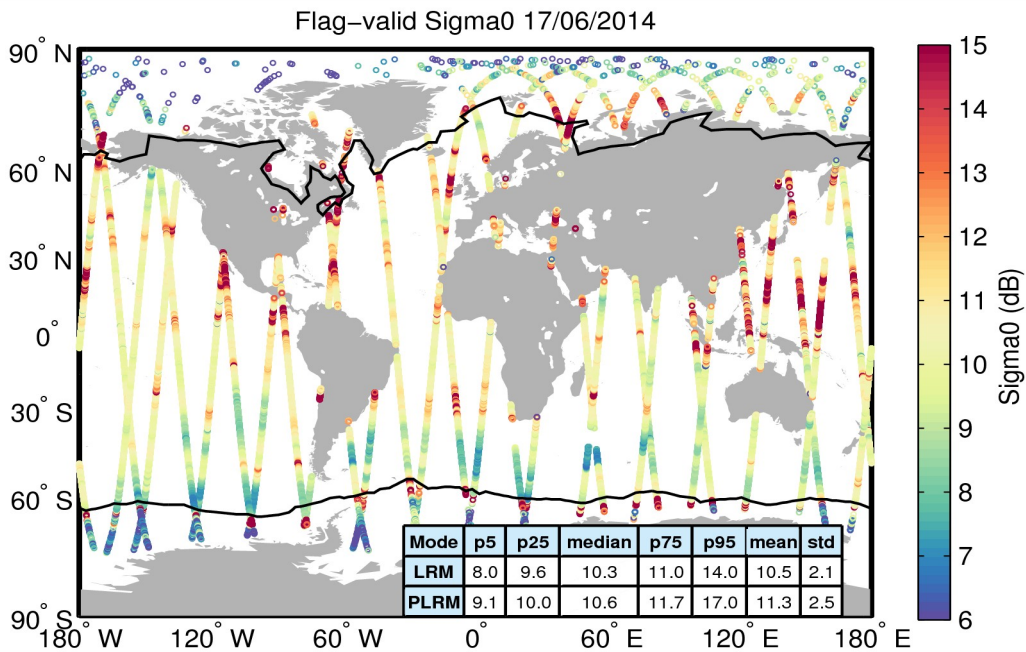
Figure 23. Geographical distribution of flag-valid sigma0 data over oceans and lakes for 17/06/2014. The statistical values shown in the table refer to the sigma0 in dB and are calculated separately for LRM and PLRM regions. Measurements taken over polar polygons have been excluded from the computation of the statistical values. The black lines mark the outer limit of the Arctic and Antarctic polar polygons.
