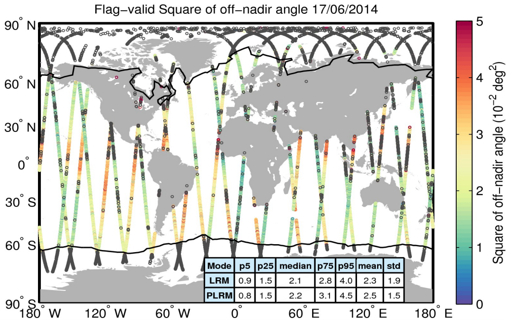
Figure 37. Geographical distribution of flag-valid mispointing data over oceans and lakes for 17/06/2014. The statistical values shown in the table refer to the mispointing in 10^{-2} \text{ deg}^2 and are calculated separately for LRM and PLRM regions. Measurements taken over polar polygons have been excluded from the computation of the statistical values. The black lines mark the outer limit of the Arctic and Antarctic polar polygons. Gray circles denote negative values.
