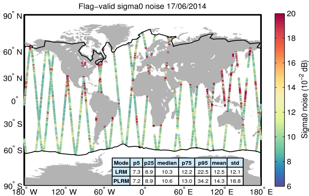
Figure 26. Geographical distribution of flag-valid 20-Hz sigma0 measurement noise over oceans and lakes for 17/06/2014. The statistical values shown in the table refer to the sigma0 noise and are calculated separately for LRM and PLRM regions. Measurements taken over polar polygons have been excluded from the computation of the statistical values. The black lines mark the outer limit of the Arctic and Antarctic polar polygons.
