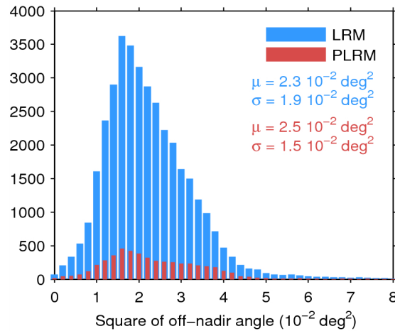
Figure 39. Histogram of flag-valid mispointing over oceans and lakes for LRM (blue) and PLRM (red) for 17/06/2014. Only positive values have been considered. The mean ( \mu ) and standard deviation ( \sigma ) are also shown. Note that values 8 \cdot 10^{-2} \text{ deg}^2 are excluded from the histogram for the sake of readability but not from the computation of \mu and \sigma .
