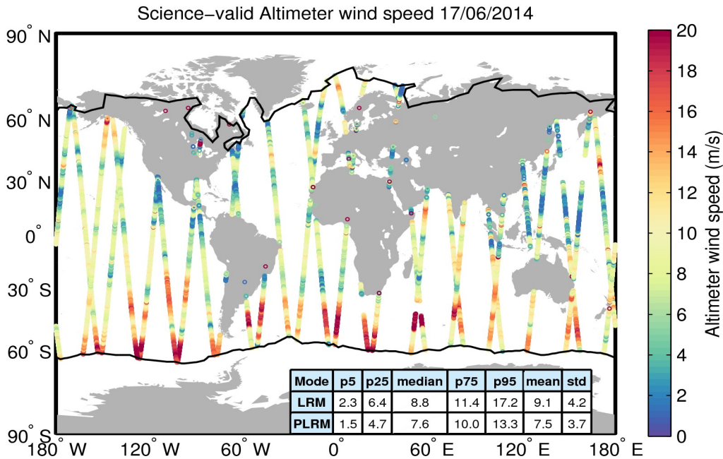
Figure 34. Geographical distribution of science-valid wind data over oceans and lakes for 17/06/2014. The statistical values shown in the table refer to the wind in m/s and are calculated separately for LRM and PLRM regions. The black lines mark the outer limit of the Arctic and Antarctic polar polygons. Gray circles denote records that have been rejected based on the editing criteria described in Table 5.
