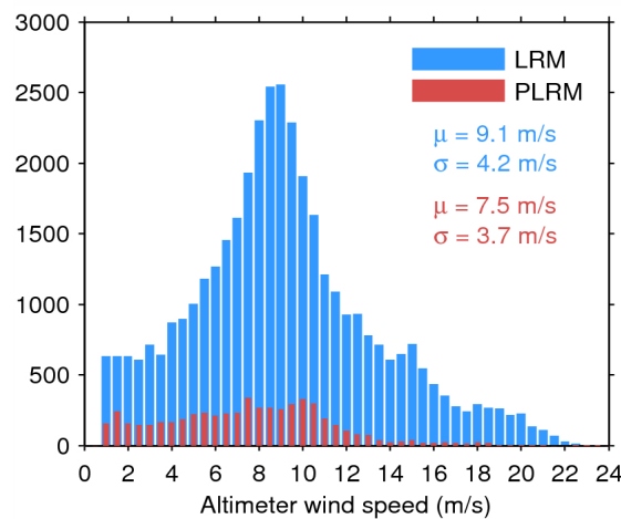
Figure 33. Histogram of flag-valid wind over oceans and lakes for LRM (blue) and PLRM (red) for 17/06/2014. The mean ( \mu ) and standard deviation ( \sigma ) are also shown. Note that values larger than 24 m/s are excluded from the histogram for the sake of readability but not from the computation of \mu and \sigma .
