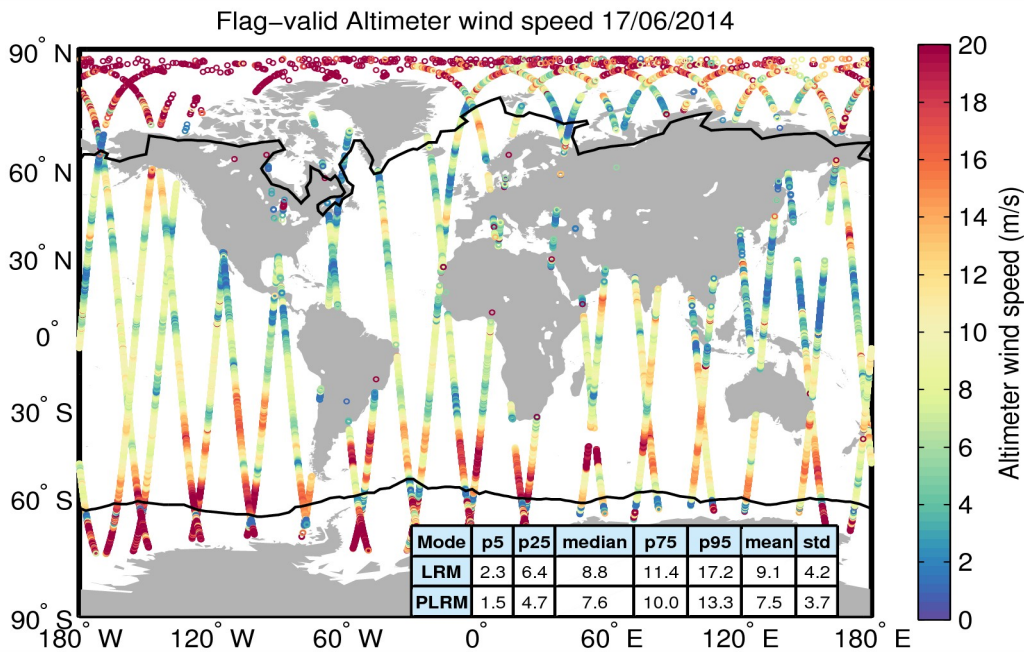
Figure 31. Geographical distribution of flag-valid wind data over oceans and lakes for 17/06/2014. The statistical values shown in the table refer to the wind in m/s and are calculated separately for LRM and PLRM regions. Measurements taken over polar polygons have been excluded from the computation of the statistical values. The black lines mark the outer limit of the Arctic and Antarctic polar polygons.
