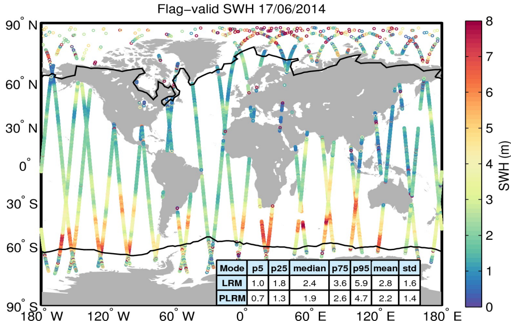
Figure 15. Geographical distribution of flag-valid SWH data over oceans and lakes for 17/06/2014. The statistical values shown in the table refer to the SWH in m and are calculated separately for LRM and PLRM regions. Measurements taken over polar polygons have been excluded from the computation of the statistical values. The black lines mark the outer limit of the Arctic and Antarctic polar polygons.
