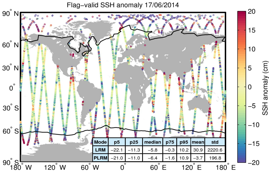
Figure 5. Geographical distribution of flag-valid 1-Hz SSH anomaly data over oceans and lakes for 17/06/2014. The statistical values shown in the table refer to the SSH anomaly in cm and are calculated separately for LRM and PLRM regions. Measurements taken over polar polygons have been excluded from the computation of the statistical values. The black lines mark the outer limit of the Arctic and Antarctic polar polygons.
