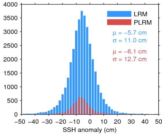
Figure 11. Histogram of science-valid SSH anomaly over oceans and lakes for LRM (blue) and PLRM (red) for 17/06/2014. The mean ( \mu ) and standard deviation ( \sigma ) are also shown. Note that values outside [-50 50] cm are excluded from the histogram for the sake of readability but not from the computation of \mu and \sigma .
