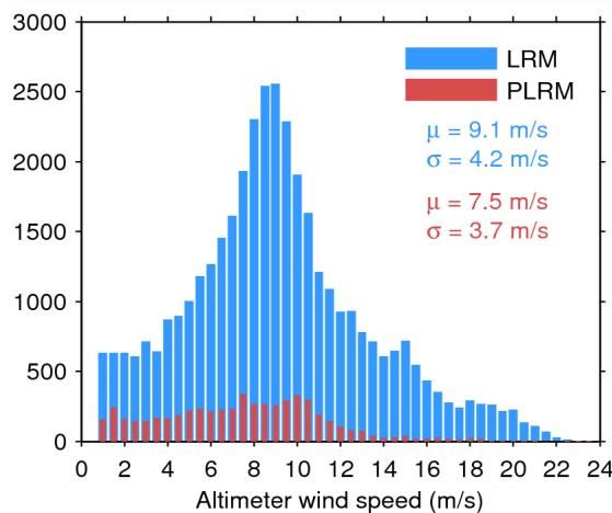
Figure 35. Histogram of science-valid wind over oceans and lakes for LRM (blue) and PLRM (red) for 17/06/2014. The mean ( \mu ) and standard deviation ( \sigma ) are also shown. Note that values larger than 24 m/s are excluded from the histogram for the sake of readability but not from the computation of \mu and \sigma .
