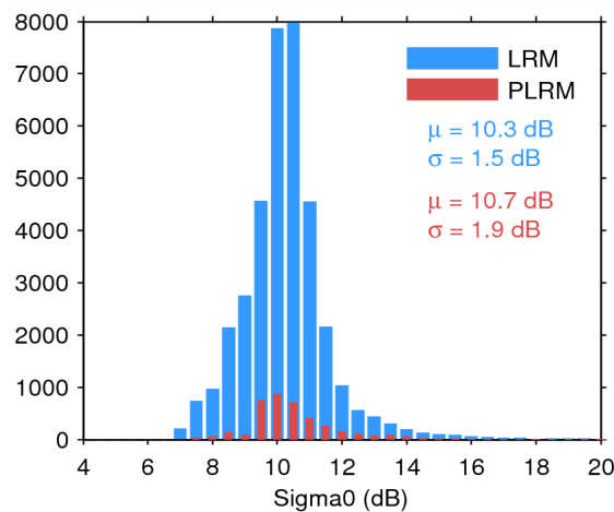
Figure 28. Histogram of science-valid sigma0 over oceans and lakes for LRM (blue) and PLRM (red) for 13/06/2014. The mean ( \mu ) and standard deviation ( \sigma ) are also shown. Note that values outside [4 20] dB are excluded from the histogram for the sake of readability but not from the computation of \mu and \sigma .
