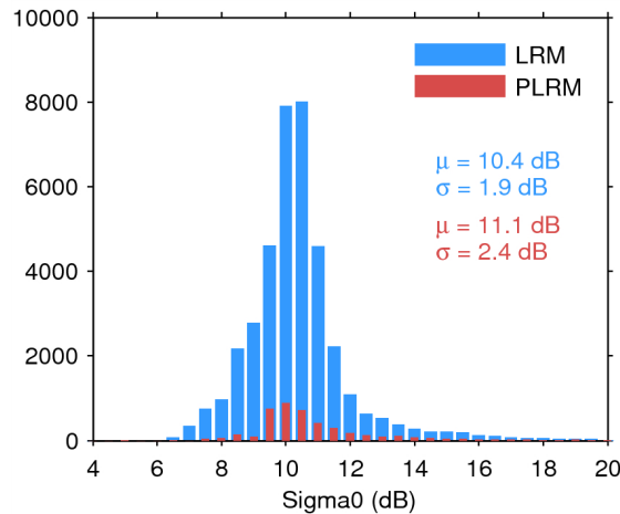
Figure 25. Histogram of flag-valid sigma0 over oceans and lakes for LRM (blue) and PLRM (red) for 13/06/2014. The mean ( \mu ) and standard deviation ( \sigma ) are also shown. Note that values outside [4 20] dB are excluded from the histogram for the sake of readability but not from the computation of \mu and \sigma .
