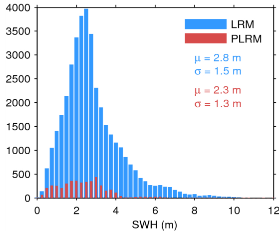
Figure 17. Histogram of flag-valid SWH over oceans and lakes for LRM (blue) and PLRM (red) for 13/06/2014. The mean ( \mu ) and standard deviation ( \sigma ) are also shown. Note that values larger than 12 m are excluded from the histogram for the sake of readability but not from the computation of \mu and \sigma .
