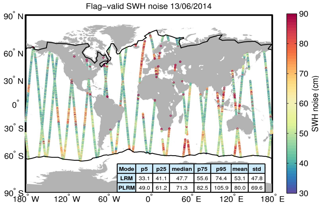
Figure 18. Geographical distribution of flag-valid 20-Hz SWH measurement noise over oceans and lakes for 13/06/2014. The statistical values shown in the table refer to the SWH noise and are calculated separately for LRM and PLRM regions. Measurements taken over polar polygons have been excluded from the computation of the statistical values. The black lines mark the outer limit of the Arctic and Antarctic polar polygons.
