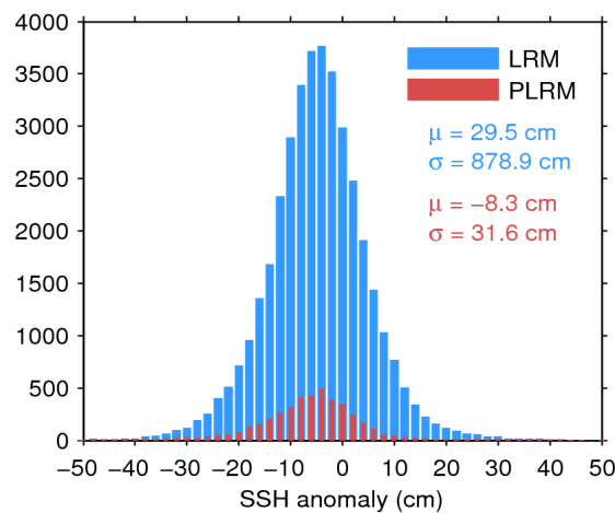
Figure 7. Histogram of flag-valid SSH anomaly over oceans and lakes for LRM (blue) and PLRM (red) for 13/06/2014. The mean ( \mu ) and standard deviation ( \sigma ) are also shown. Note that values outside [-50\ 50] cm are excluded from the histogram for the sake of readability but not from the computation of \mu and \sigma .
