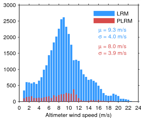
Figure 35. Histogram of science-valid wind over oceans and lakes for LRM (blue) and PLRM (red) for 13/06/2014. The mean ( \mu ) and standard deviation ( \sigma ) are also shown. Note that values larger than 24 m/s are excluded from the histogram for the sake of readability but not from the computation of \mu and \sigma .
