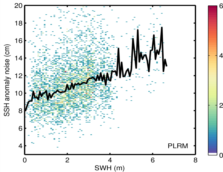
Figure 9. 2D histogram showing flag-valid SSH anomaly noise as a function of SWH for LRM (top) and PLRM (bottom) for 13/06/2014. The black line denotes the median SSH anomaly as a function of SWH.
