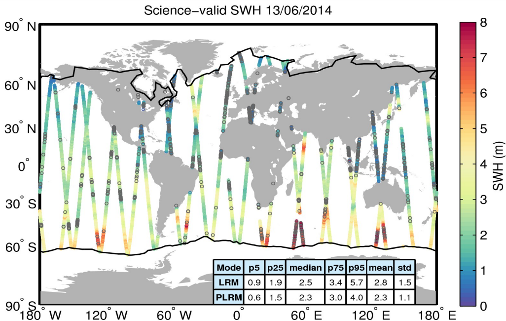
Figure 19. Geographical distribution of science-valid SWH data over oceans and lakes for 13/06/2014. The statistical values shown in the table refer to the SWH in m and are calculated separately for LRM and PLRM regions. The black lines mark the outer limit of the Arctic and Antarctic polar polygons. Gray circles denote records that have been rejected based on the editing criteria described in Table 3.
