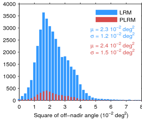
Figure 39. Histogram of flag-valid mispointing over oceans and lakes for LRM (blue) and PLRM (red) for 13/06/2014. Only positive values have been considered. The mean ( \mu ) and standard deviation ( \sigma ) are also shown. Note that values 8 \cdot 10^{-2} \text{ deg}^2 are excluded from the histogram for the sake of readability but not from the computation of \mu and \sigma .
