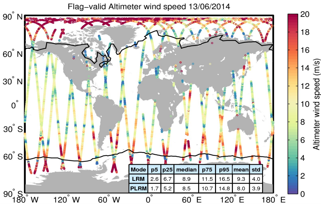
Figure 31. Geographical distribution of flag-valid wind data over oceans and lakes for 13/06/2014. The statistical values shown in the table refer to the wind in m/s and are calculated separately for LRM and PLRM regions. Measurements taken over polar polygons have been excluded from the computation of the statistical values. The black lines mark the outer limit of the Arctic and Antarctic polar polygons.
