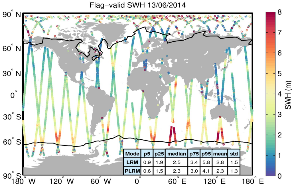
Figure 15. Geographical distribution of flag-valid SWH data over oceans and lakes for 13/06/2014. The statistical values shown in the table refer to the SWH in m and are calculated separately for LRM and PLRM regions. Measurements taken over polar polygons have been excluded from the computation of the statistical values. The black lines mark the outer limit of the Arctic and Antarctic polar polygons.
