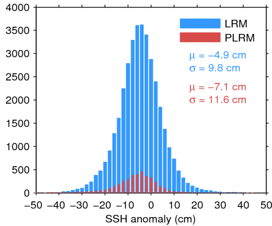
Figure 11. Histogram of science-valid SSH anomaly over oceans and lakes for LRM (blue) and PLRM (red) for 13/06/2014. The mean ( \mu ) and standard deviation ( \sigma ) are also shown. Note that values outside [-50 50] cm are excluded from the histogram for the sake of readability but not from the computation of \mu and \sigma .
