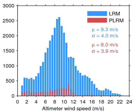
Figure 33. Histogram of flag-valid wind over oceans and lakes for LRM (blue) and PLRM (red) for 13/06/2014. The mean ( \mu ) and standard deviation ( \sigma ) are also shown. Note that values larger than 24 m/s are excluded from the histogram for the sake of readability but not from the computation of \mu and \sigma .
