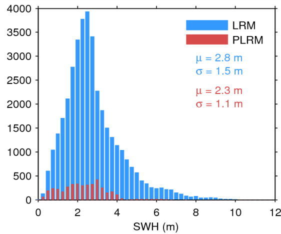
Figure 20. Histogram of science-valid SWH over oceans and lakes for LRM (blue) and PLRM (red) for 13/06/2014. The mean ( \mu ) and standard deviation ( \sigma ) are also shown. Note that values larger than 12 m are excluded from the histogram for the sake of readability but not from the computation of \mu and \sigma .
