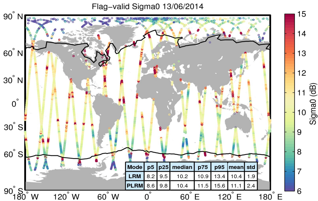
Figure 23. Geographical distribution of flag-valid sigma0 data over oceans and lakes for 13/06/2014. The statistical values shown in the table refer to the sigma0 in dB and are calculated separately for LRM and PLRM regions. Measurements taken over polar polygons have been excluded from the computation of the statistical values. The black lines mark the outer limit of the Arctic and Antarctic polar polygons.
