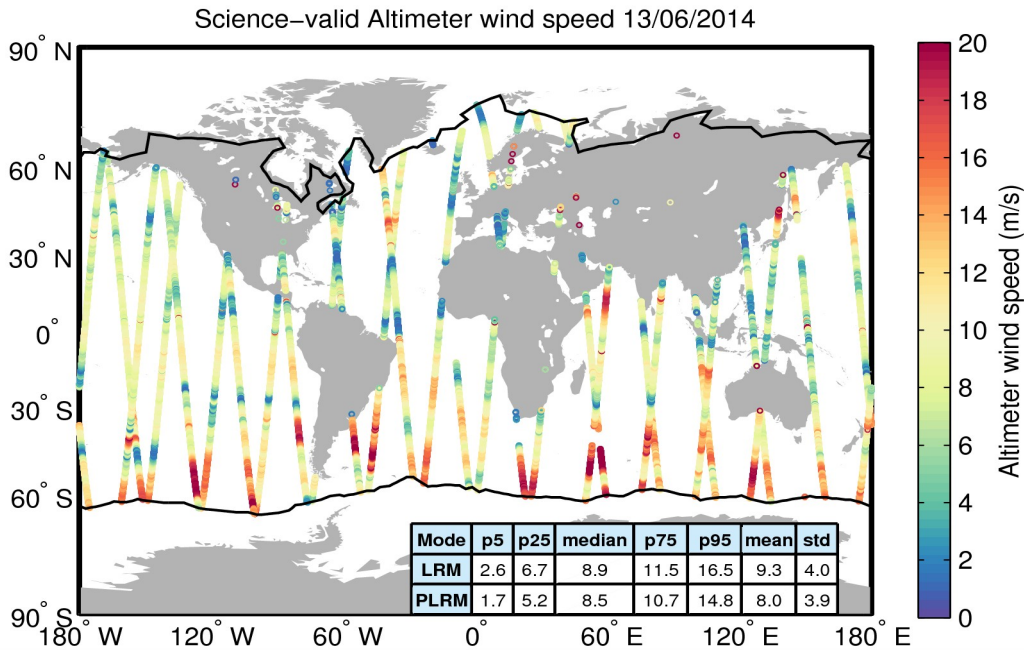
Figure 34. Geographical distribution of science-valid wind data over oceans and lakes for 13/06/2014. The statistical values shown in the table refer to the wind in m/s and are calculated separately for LRM and PLRM regions. The black lines mark the outer limit of the Arctic and Antarctic polar polygons. Gray circles denote records that have been rejected based on the editing criteria described in Table 5.
