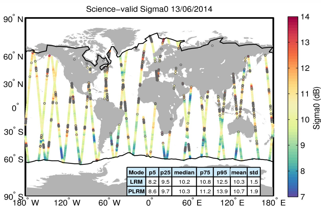
Figure 27. Geographical distribution of science-valid sigma0 data over oceans and lakes for 13/06/2014. The statistical values shown in the table refer to the sigma0 in dB and are calculated separately for LRM and PLRM regions. The black lines mark the outer limit of the Arctic and Antarctic polar polygons. Gray circles denote records that have been rejected based on the editing criteria described in Table 4.
