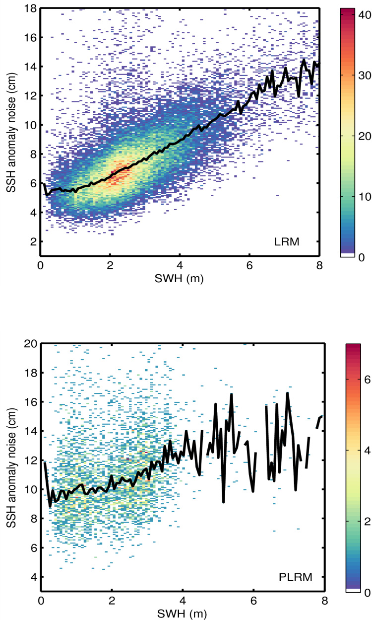
Figure 9. 2D histogram showing flag-valid SSH anomaly noise as a function of SWH for LRM (top) and PLRM (bottom) for 12/06/2014. The black line denotes the median SSH anomaly as a function of SWH.
