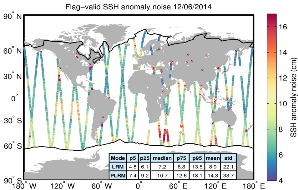
Figure 8. Geographical distribution of flag-valid 20-Hz SSH anomaly measurement noise over oceans and lakes for 12/06/2014. The statistical values shown in the table refer to the SSH anomaly noise and are calculated separately for LRM and PLRM regions. Measurements taken over polar polygons have been excluded from the computation of the statistical values. The black lines mark the outer limit of the Arctic and Antarctic polar polygons.
