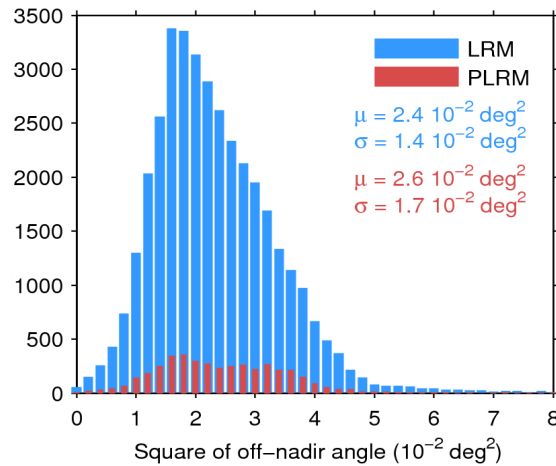
Figure 39. Histogram of flag-valid mispointing over oceans and lakes for LRM (blue) and PLRM (red) for 12/06/2014. Only positive values have been considered. The mean ( \mu ) and standard deviation ( \sigma ) are also shown. Note that values 8 \cdot 10^{-2} \text{ deg}^2 are excluded from the histogram for the sake of readability but not from the computation of \mu and \sigma .
