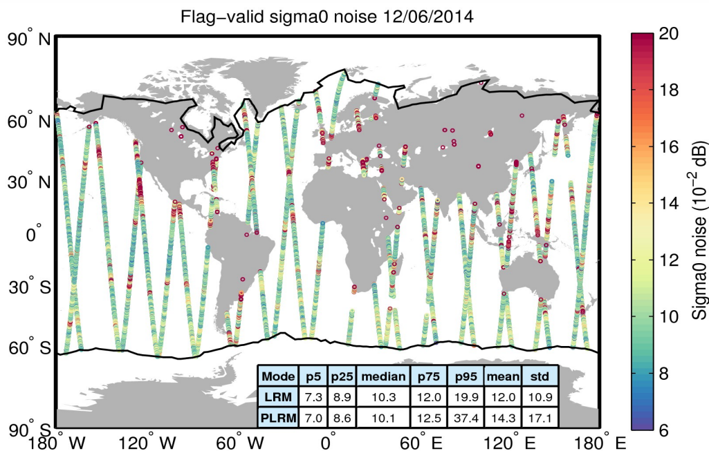
Figure 26. Geographical distribution of flag-valid 20-Hz sigma0 measurement noise over oceans and lakes for 12/06/2014. The statistical values shown in the table refer to the sigma0 noise and are calculated separately for LRM and PLRM regions. Measurements taken over polar polygons have been excluded from the computation of the statistical values. The black lines mark the outer limit of the Arctic and Antarctic polar polygons.
