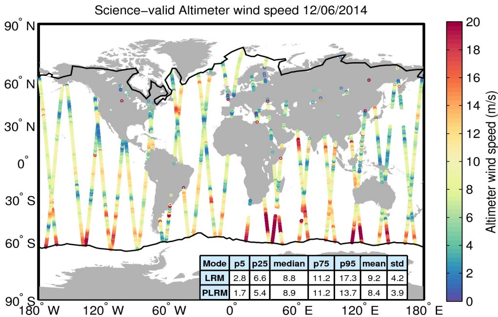
Figure 34. Geographical distribution of science-valid wind data over oceans and lakes for 12/06/2014. The statistical values shown in the table refer to the wind in m/s and are calculated separately for LRM and PLRM regions. The black lines mark the outer limit of the Arctic and Antarctic polar polygons. Gray circles denote records that have been rejected based on the editing criteria described in Table 5.
