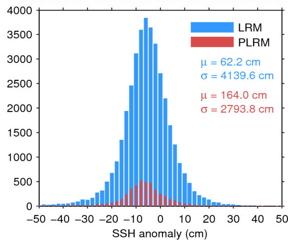
Figure 7. Histogram of flag-valid SSH anomaly over oceans and lakes for LRM (blue) and PLRM (red) for 12/06/2014. The mean ( \mu ) and standard deviation ( \sigma ) are also shown. Note that values outside [-50\ 50] cm are excluded from the histogram for the sake of readability but not from the computation of \mu and \sigma .
