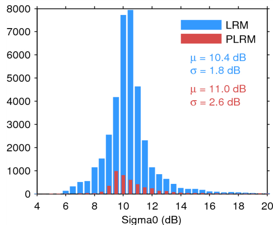
Figure 25. Histogram of flag-valid sigma0 over oceans and lakes for LRM (blue) and PLRM (red) for 12/06/2014. The mean ( \mu ) and standard deviation ( \sigma ) are also shown. Note that values outside [4 20] dB are excluded from the histogram for the sake of readability but not from the computation of \mu and \sigma .
