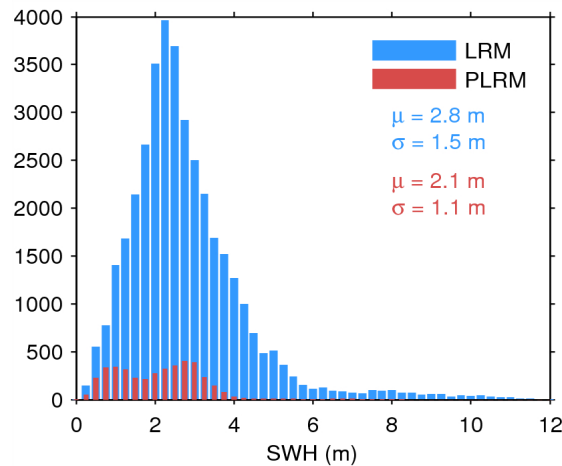
Figure 20. Histogram of science-valid SWH over oceans and lakes for LRM (blue) and PLRM (red) for 12/06/2014. The mean ( \mu ) and standard deviation ( \sigma ) are also shown. Note that values larger than 12 m are excluded from the histogram for the sake of readability but not from the computation of \mu and \sigma .
