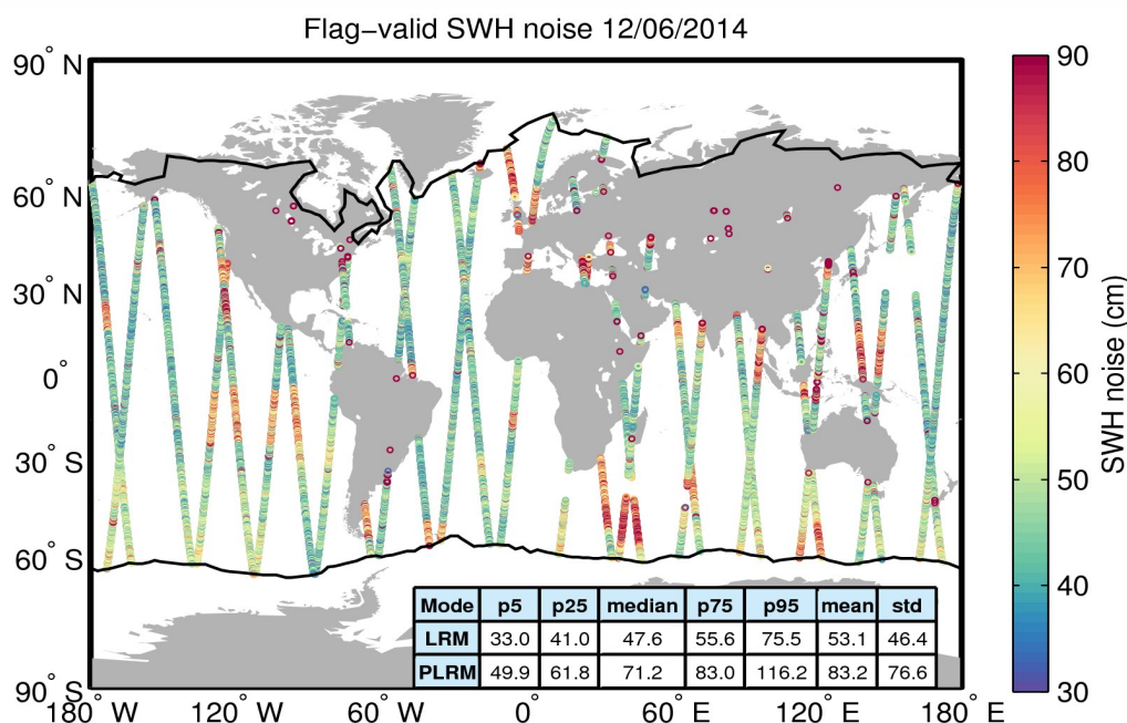
Figure 18. Geographical distribution of flag-valid 20-Hz SWH measurement noise over oceans and lakes for 12/06/2014. The statistical values shown in the table refer to the SWH noise and are calculated separately for LRM and PLRM regions. Measurements taken over polar polygons have been excluded from the computation of the statistical values. The black lines mark the outer limit of the Arctic and Antarctic polar polygons.
