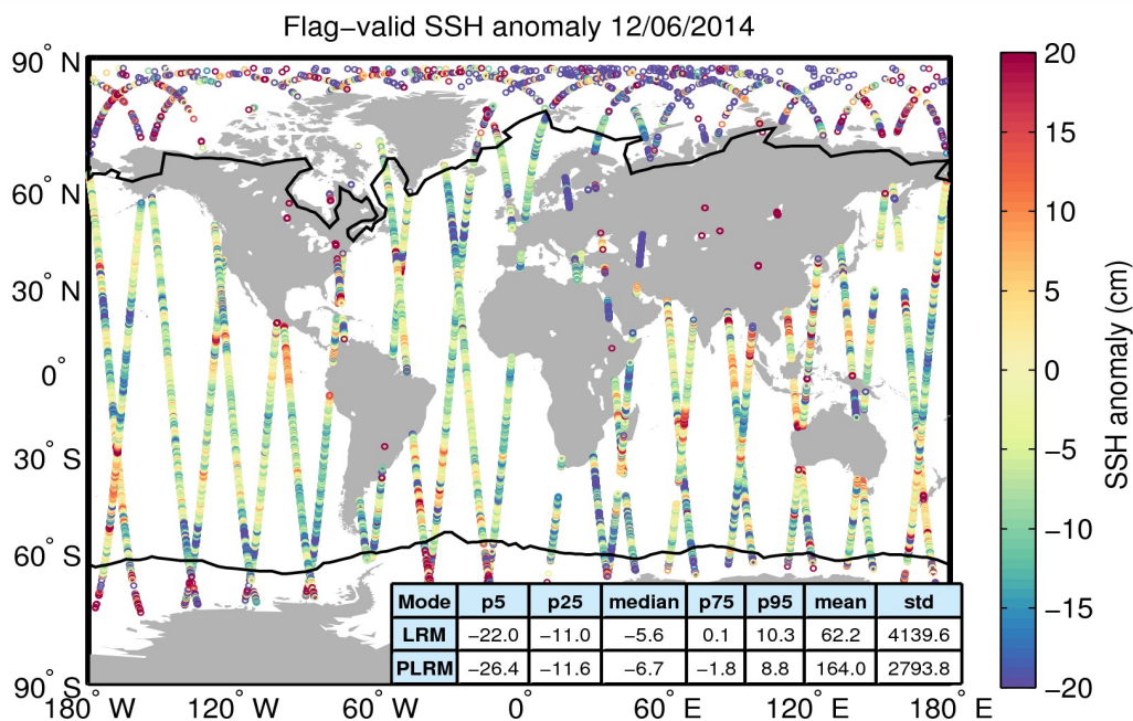
Figure 5. Geographical distribution of flag-valid 1-Hz SSH anomaly data over oceans and lakes for 12/06/2014. The statistical values shown in the table refer to the SSH anomaly in cm and are calculated separately for LRM and PLRM regions. Measurements taken over polar polygons have been excluded from the computation of the statistical values. The black lines mark the outer limit of the Arctic and Antarctic polar polygons.
