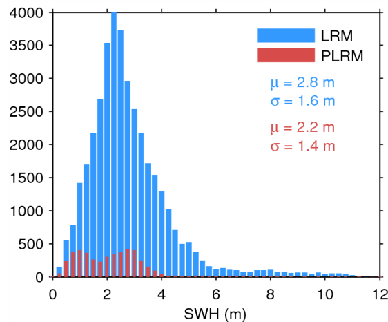
Figure 17. Histogram of flag-valid SWH over oceans and lakes for LRM (blue) and PLRM (red) for 12/06/2014. The mean ( \mu ) and standard deviation ( \sigma ) are also shown. Note that values larger than 12 m are excluded from the histogram for the sake of readability but not from the computation of \mu and \sigma .
