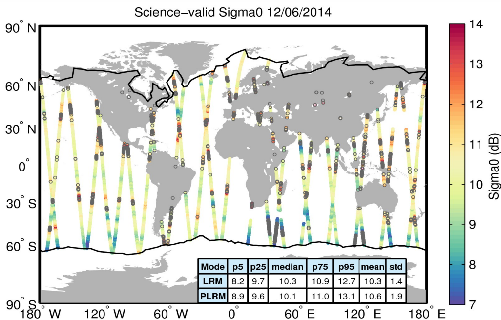
Figure 27. Geographical distribution of science-valid sigma0 data over oceans and lakes for 12/06/2014. The statistical values shown in the table refer to the sigma0 in dB and are calculated separately for LRM and PLRM regions. The black lines mark the outer limit of the Arctic and Antarctic polar polygons. Gray circles denote records that have been rejected based on the editing criteria described in Table 4.
