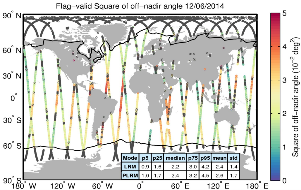
Figure 37. Geographical distribution of flag-valid mispointing data over oceans and lakes for 12/06/2014. The statistical values shown in the table refer to the mispointing in 10^{-2} \text{ deg}^2 and are calculated separately for LRM and PLRM regions. Measurements taken over polar polygons have been excluded from the computation of the statistical values. The black lines mark the outer limit of the Arctic and Antarctic polar polygons. Gray circles denote negative values.
