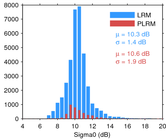
Figure 28. Histogram of science-valid sigma0 over oceans and lakes for LRM (blue) and PLRM (red) for 12/06/2014. The mean ( \mu ) and standard deviation ( \sigma ) are also shown. Note that values outside [4 20] dB are excluded from the histogram for the sake of readability but not from the computation of \mu and \sigma .
