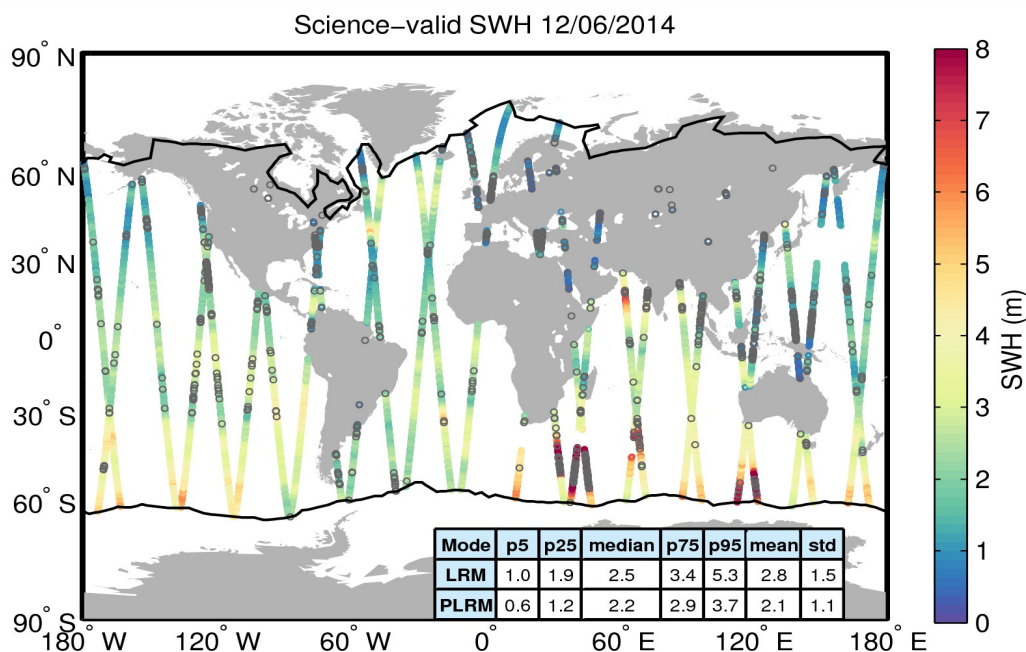
Figure 19. Geographical distribution of science-valid SWH data over oceans and lakes for 12/06/2014. The statistical values shown in the table refer to the SWH in m and are calculated separately for LRM and PLRM regions. The black lines mark the outer limit of the Arctic and Antarctic polar polygons. Gray circles denote records that have been rejected based on the editing criteria described in Table 3.
