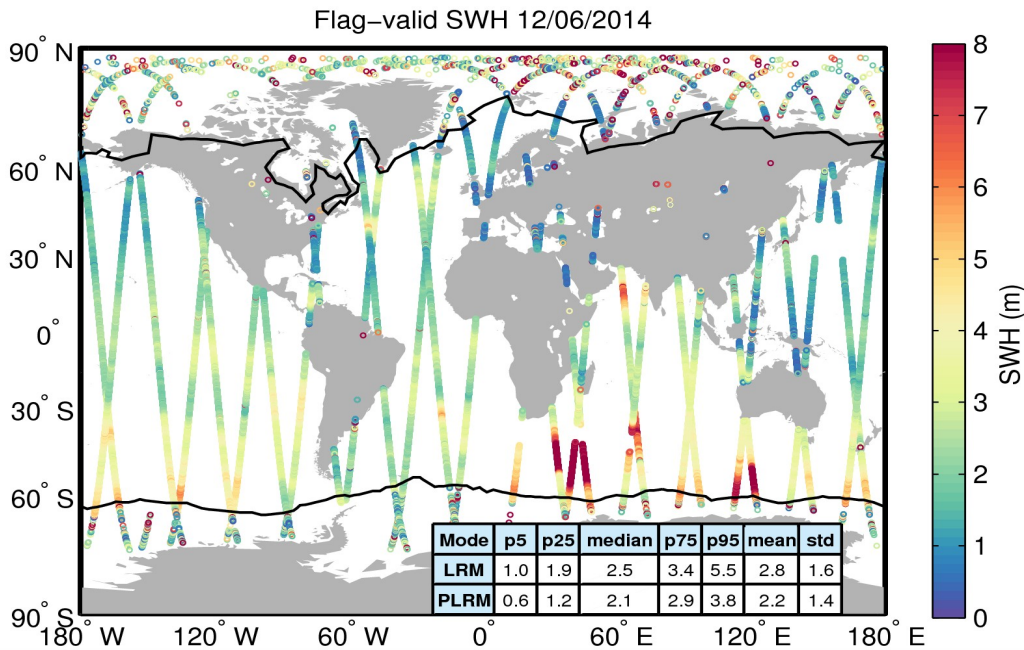
Figure 15. Geographical distribution of flag-valid SWH data over oceans and lakes for 12/06/2014. The statistical values shown in the table refer to the SWH in m and are calculated separately for LRM and PLRM regions. Measurements taken over polar polygons have been excluded from the computation of the statistical values. The black lines mark the outer limit of the Arctic and Antarctic polar polygons.
