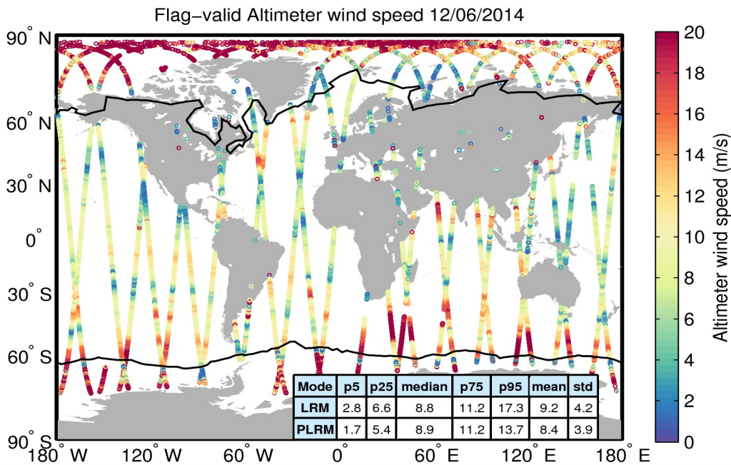
Figure 31. Geographical distribution of flag-valid wind data over oceans and lakes for 12/06/2014. The statistical values shown in the table refer to the wind in m/s and are calculated separately for LRM and PLRM regions. Measurements taken over polar polygons have been excluded from the computation of the statistical values. The black lines mark the outer limit of the Arctic and Antarctic polar polygons.
