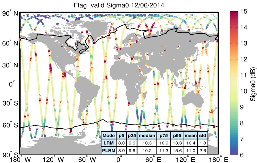
Figure 23. Geographical distribution of flag-valid sigma0 data over oceans and lakes for 12/06/2014. The statistical values shown in the table refer to the sigma0 in dB and are calculated separately for LRM and PLRM regions. Measurements taken over polar polygons have been excluded from the computation of the statistical values. The black lines mark the outer limit of the Arctic and Antarctic polar polygons.
