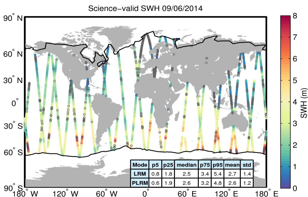
Figure 19. Geographical distribution of science-valid SWH data over oceans and lakes for 09/06/2014. The statistical values shown in the table refer to the SWH in m and are calculated separately for LRM and PLRM regions. The black lines mark the outer limit of the Arctic and Antarctic polar polygons. Gray circles denote records that have been rejected based on the editing criteria described in Table 3.
