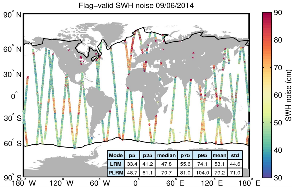
Figure 18. Geographical distribution of flag-valid 20-Hz SWH measurement noise over oceans and lakes for 09/06/2014. The statistical values shown in the table refer to the SWH noise and are calculated separately for LRM and PLRM regions. Measurements taken over polar polygons have been excluded from the computation of the statistical values. The black lines mark the outer limit of the Arctic and Antarctic polar polygons.
