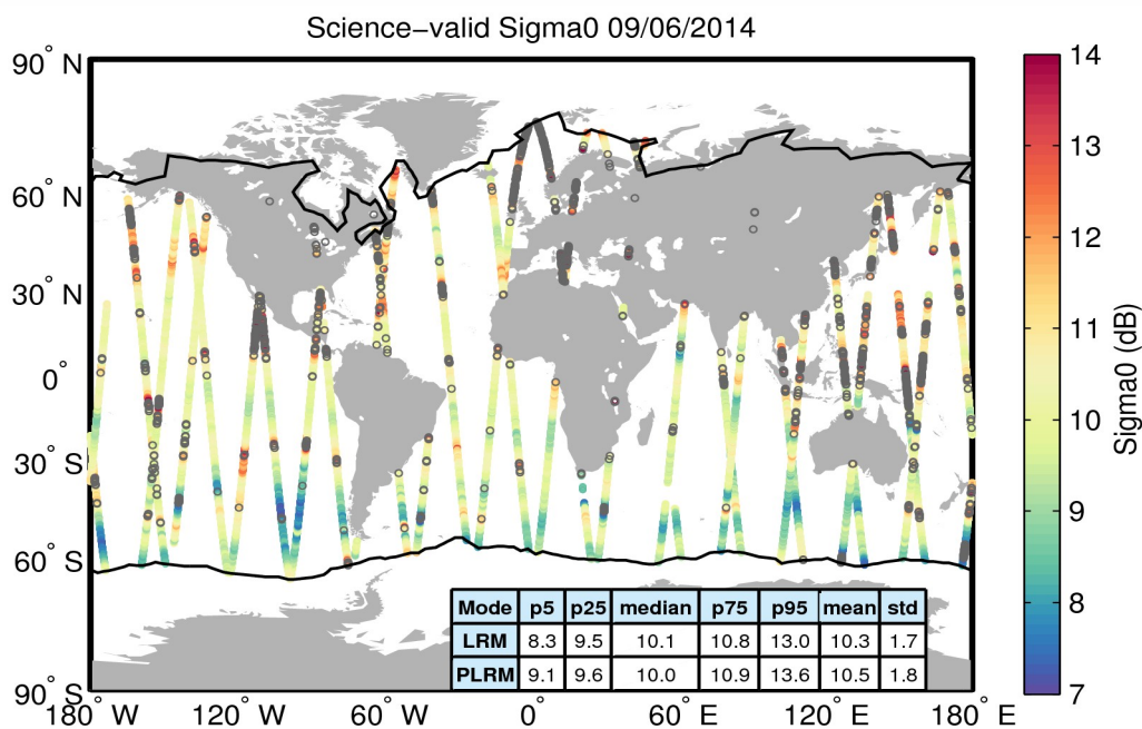
Figure 27. Geographical distribution of science-valid sigma0 data over oceans and lakes for 09/06/2014. The statistical values shown in the table refer to the sigma0 in dB and are calculated separately for LRM and PLRM regions. The black lines mark the outer limit of the Arctic and Antarctic polar polygons. Gray circles denote records that have been rejected based on the editing criteria described in Table 4.
