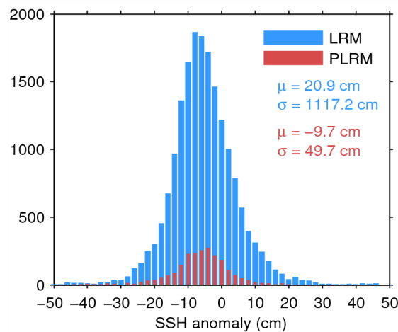
Figure 7. Histogram of flag-valid SSH anomaly over oceans and lakes for LRM (blue) and PLRM (red) for 09/06/2014. The mean ( \mu ) and standard deviation ( \sigma ) are also shown. Note that values outside [-50\ 50] cm are excluded from the histogram for the sake of readability but not from the computation of \mu and \sigma .
