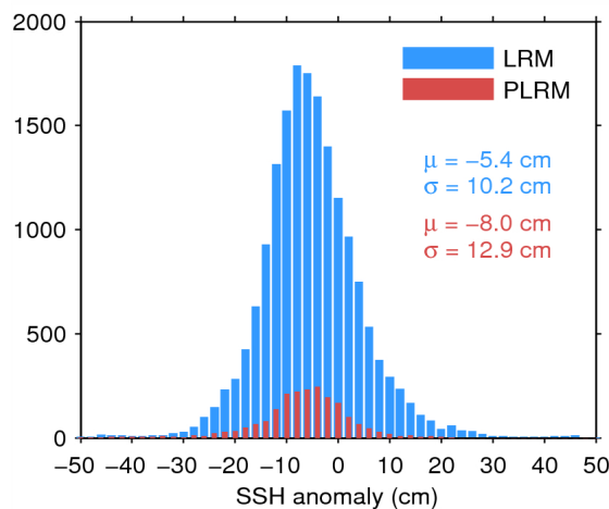
Figure 11. Histogram of science-valid SSH anomaly over oceans and lakes for LRM (blue) and PLRM (red) for 09/06/2014. The mean ( \mu ) and standard deviation ( \sigma ) are also shown. Note that values outside [-50 50] cm are excluded from the histogram for the sake of readability but not from the computation of \mu and \sigma .
