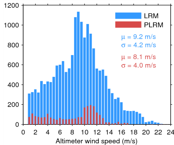
Figure 33. Histogram of flag-valid wind over oceans and lakes for LRM (blue) and PLRM (red) for 09/06/2014. The mean ( \mu ) and standard deviation ( \sigma ) are also shown. Note that values larger than 24 m/s are excluded from the histogram for the sake of readability but not from the computation of \mu and \sigma .
