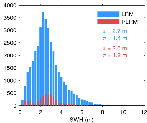
Figure 20. Histogram of science-valid SWH over oceans and lakes for LRM (blue) and PLRM (red) for 09/06/2014. The mean ( \mu ) and standard deviation ( \sigma ) are also shown. Note that values larger than 12 m are excluded from the histogram for the sake of readability but not from the computation of \mu and \sigma .
