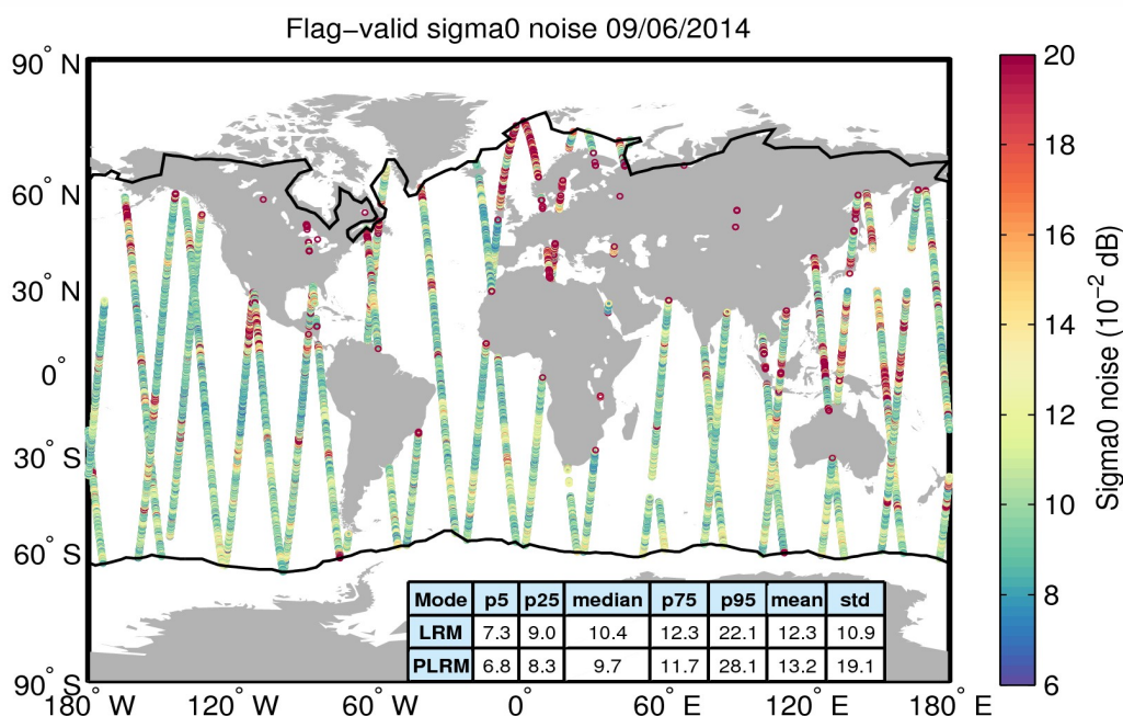
Figure 26. Geographical distribution of flag-valid 20-Hz sigma0 measurement noise over oceans and lakes for 09/06/2014. The statistical values shown in the table refer to the sigma0 noise and are calculated separately for LRM and PLRM regions. Measurements taken over polar polygons have been excluded from the computation of the statistical values. The black lines mark the outer limit of the Arctic and Antarctic polar polygons.
