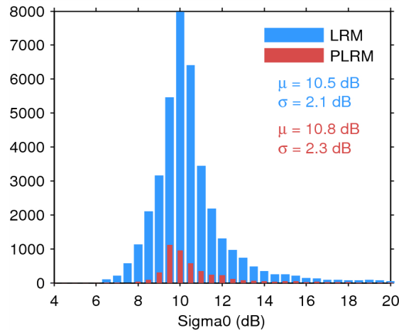
Figure 25. Histogram of flag-valid sigma0 over oceans and lakes for LRM (blue) and PLRM (red) for 09/06/2014. The mean ( \mu ) and standard deviation ( \sigma ) are also shown. Note that values outside [4 20] dB are excluded from the histogram for the sake of readability but not from the computation of \mu and \sigma .
