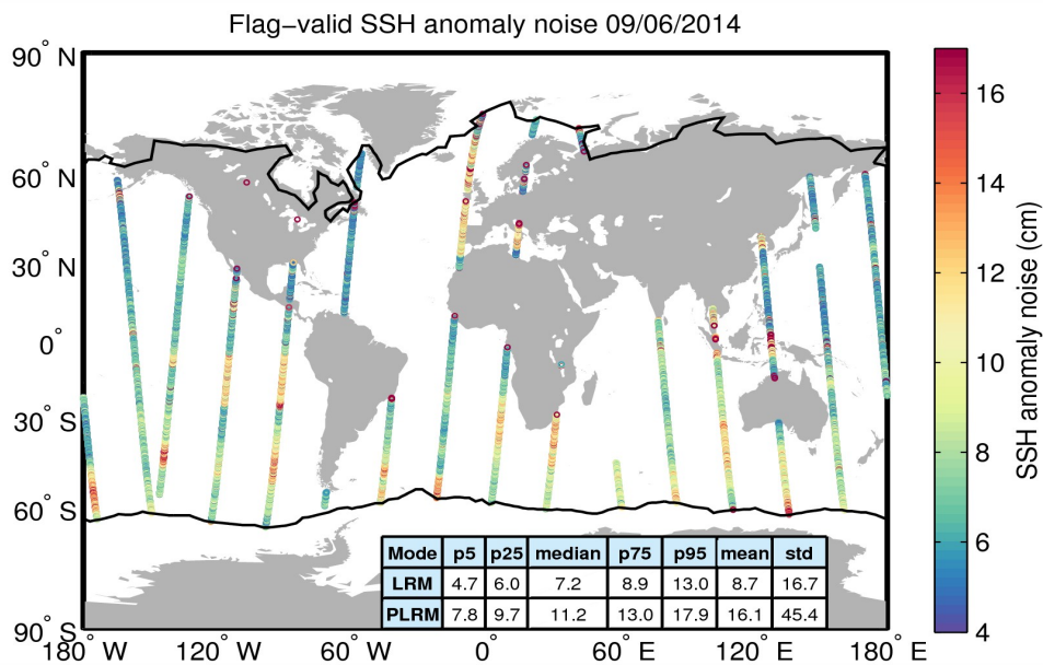
Figure 8. Geographical distribution of flag-valid 20-Hz SSH anomaly measurement noise over oceans and lakes for 09/06/2014. The statistical values shown in the table refer to the SSH anomaly noise and are calculated separately for LRM and PLRM regions. Measurements taken over polar polygons have been excluded from the computation of the statistical values. The black lines mark the outer limit of the Arctic and Antarctic polar polygons.
