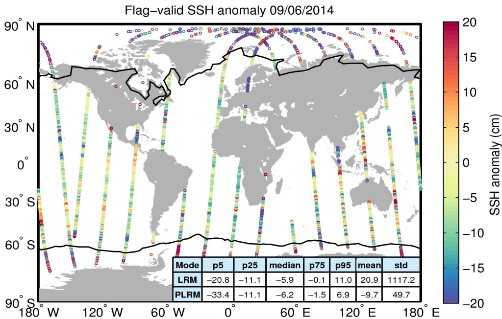
Figure 5. Geographical distribution of flag-valid 1-Hz SSH anomaly data over oceans and lakes for 09/06/2014. The statistical values shown in the table refer to the SSH anomaly in cm and are calculated separately for LRM and PLRM regions. Measurements taken over polar polygons have been excluded from the computation of the statistical values. The black lines mark the outer limit of the Arctic and Antarctic polar polygons.
