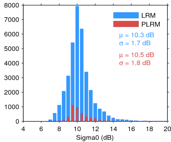
Figure 28. Histogram of science-valid sigma0 over oceans and lakes for LRM (blue) and PLRM (red) for 09/06/2014. The mean ( \mu ) and standard deviation ( \sigma ) are also shown. Note that values outside [4 20] dB are excluded from the histogram for the sake of readability but not from the computation of \mu and \sigma .
