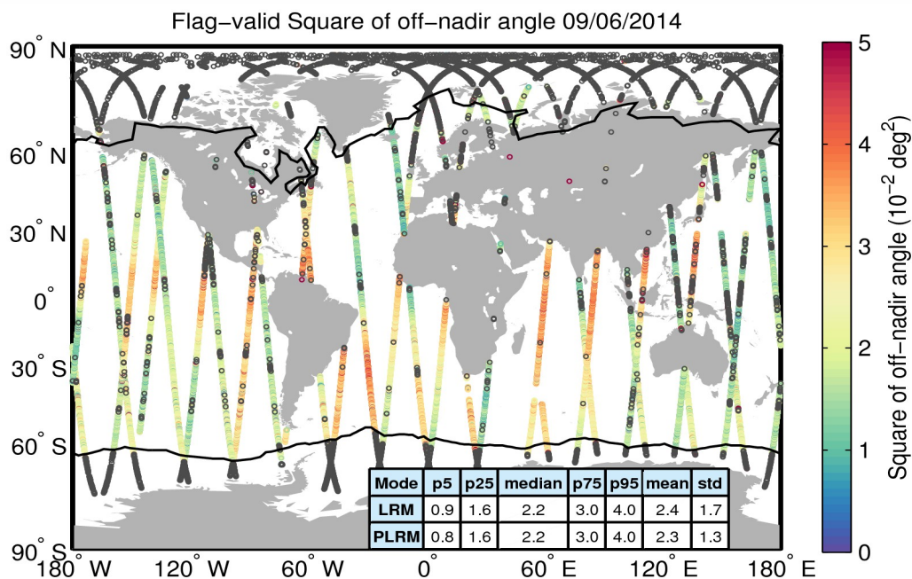
Figure 37. Geographical distribution of flag-valid mispointing data over oceans and lakes for 09/06/2014. The statistical values shown in the table refer to the mispointing in 10^{-2} \text{ deg}^2 and are calculated separately for LRM and PLRM regions. Measurements taken over polar polygons have been excluded from the computation of the statistical values. The black lines mark the outer limit of the Arctic and Antarctic polar polygons. Gray circles denote negative values.
