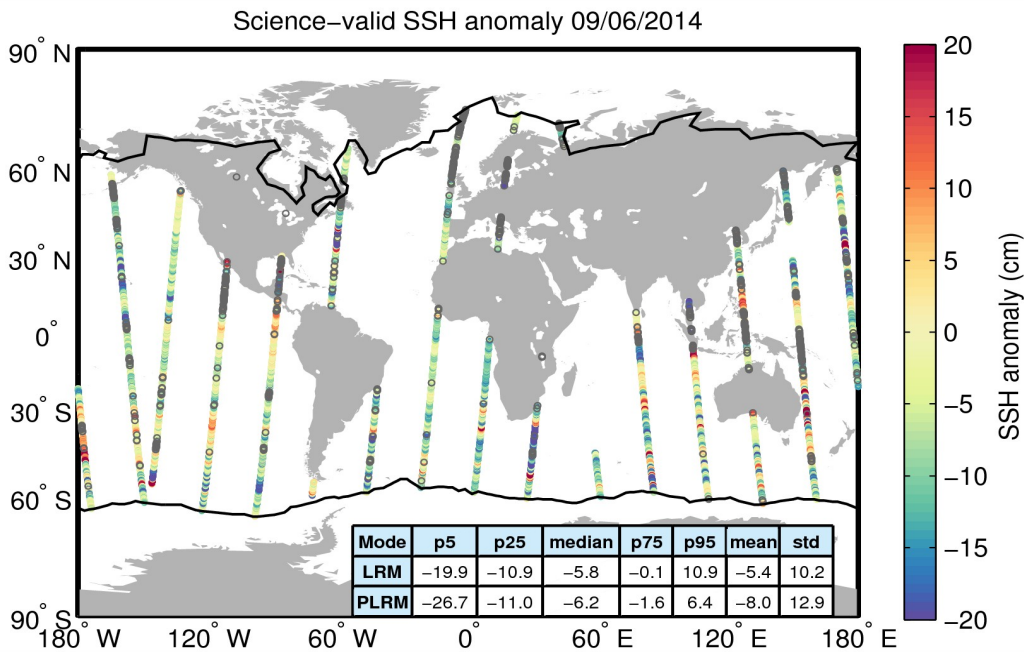
Figure 10. Geographical distribution of science-valid SSH anomaly data over oceans and lakes for 09/06/2014. The statistical values shown in the table refer to the SSH anomaly in cm and are calculated separately for LRM and PLRM regions. The black lines mark the outer limit of the Arctic and Antarctic polar polygons. Gray circles denote records that have been rejected based on the editing criteria described in Table 2.
