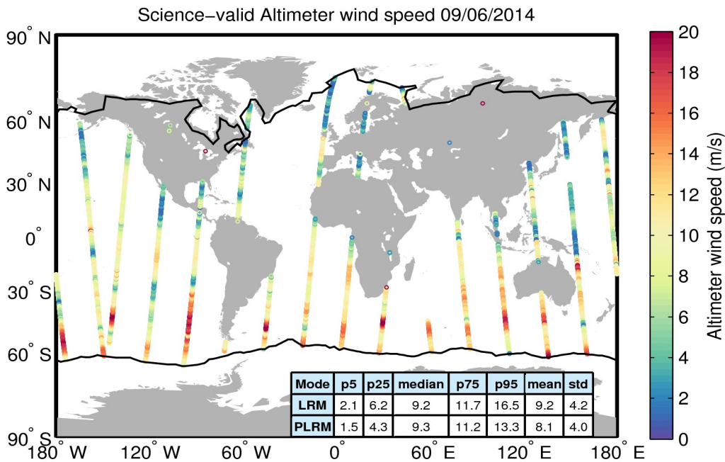
Figure 34. Geographical distribution of science-valid wind data over oceans and lakes for 09/06/2014. The statistical values shown in the table refer to the wind in m/s and are calculated separately for LRM and PLRM regions. The black lines mark the outer limit of the Arctic and Antarctic polar polygons. Gray circles denote records that have been rejected based on the editing criteria described in Table 5.
