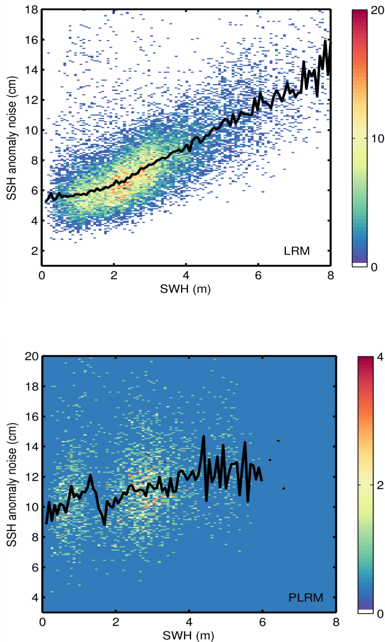
Figure 9. 2D histogram showing flag-valid SSH anomaly noise as a function of SWH for LRM (top) and PLRM (bottom) for 09/06/2014. The black line denotes the median SSH anomaly as a function of SWH.
