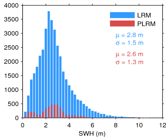
Figure 17. Histogram of flag-valid SWH over oceans and lakes for LRM (blue) and PLRM (red) for 09/06/2014. The mean ( \mu ) and standard deviation ( \sigma ) are also shown. Note that values larger than 12 m are excluded from the histogram for the sake of readability but not from the computation of \mu and \sigma .
