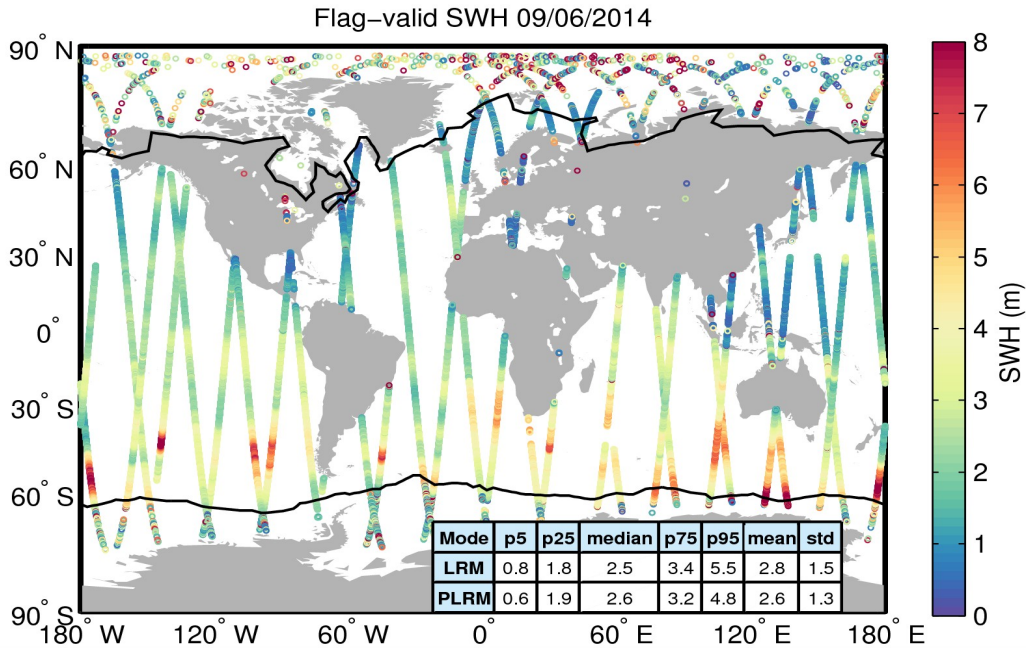
Figure 15. Geographical distribution of flag-valid SWH data over oceans and lakes for 09/06/2014. The statistical values shown in the table refer to the SWH in m and are calculated separately for LRM and PLRM regions. Measurements taken over polar polygons have been excluded from the computation of the statistical values. The black lines mark the outer limit of the Arctic and Antarctic polar polygons.
