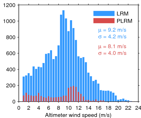
Figure 35. Histogram of science-valid wind over oceans and lakes for LRM (blue) and PLRM (red) for 09/06/2014. The mean ( \mu ) and standard deviation ( \sigma ) are also shown. Note that values larger than 24 m/s are excluded from the histogram for the sake of readability but not from the computation of \mu and \sigma .
