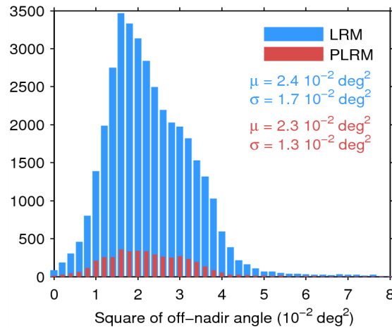
Figure 39. Histogram of flag-valid mispointing over oceans and lakes for LRM (blue) and PLRM (red) for 09/06/2014. Only positive values have been considered. The mean ( \mu ) and standard deviation ( \sigma ) are also shown. Note that values 8 \cdot 10^{-2} \text{ deg}^2 are excluded from the histogram for the sake of readability but not from the computation of \mu and \sigma .
