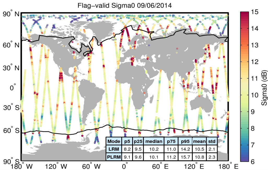
Figure 23. Geographical distribution of flag-valid sigma0 data over oceans and lakes for 09/06/2014. The statistical values shown in the table refer to the sigma0 in dB and are calculated separately for LRM and PLRM regions. Measurements taken over polar polygons have been excluded from the computation of the statistical values. The black lines mark the outer limit of the Arctic and Antarctic polar polygons.
