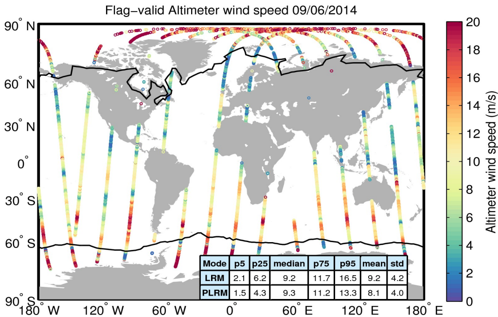
Figure 31. Geographical distribution of flag-valid wind data over oceans and lakes for 09/06/2014. The statistical values shown in the table refer to the wind in m/s and are calculated separately for LRM and PLRM regions. Measurements taken over polar polygons have been excluded from the computation of the statistical values. The black lines mark the outer limit of the Arctic and Antarctic polar polygons.
