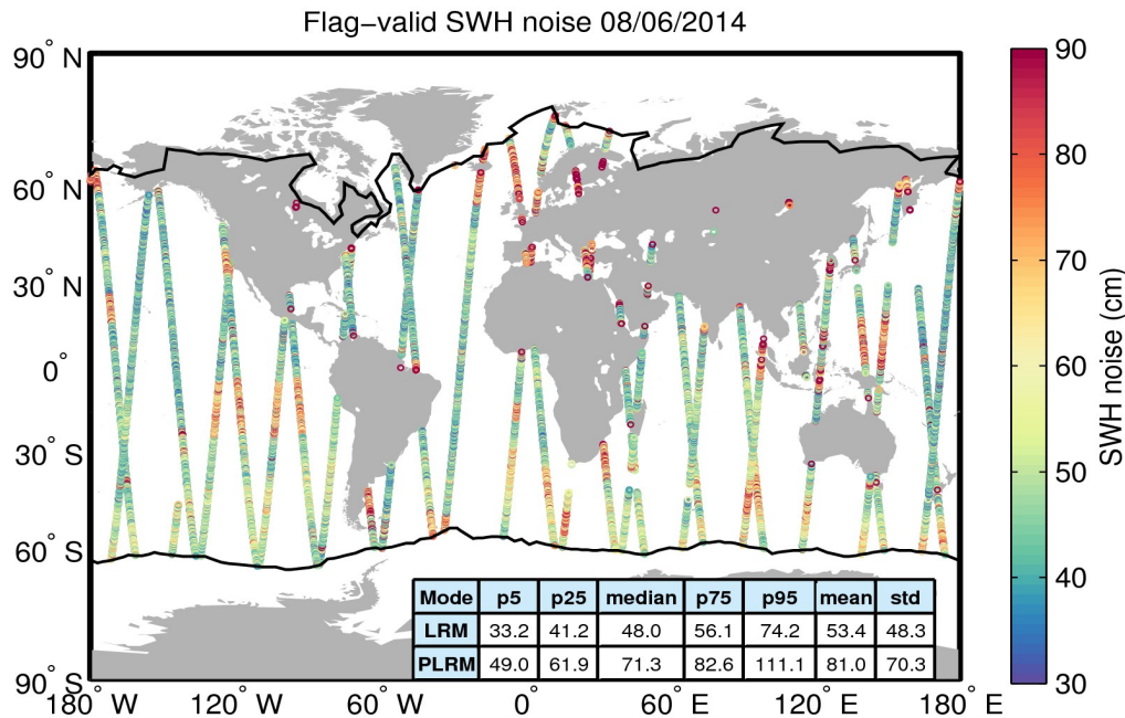
Figure 18. Geographical distribution of flag-valid 20-Hz SWH measurement noise over oceans and lakes for 08/06/2014. The statistical values shown in the table refer to the SWH noise and are calculated separately for LRM and PLRM regions. Measurements taken over polar polygons have been excluded from the computation of the statistical values. The black lines mark the outer limit of the Arctic and Antarctic polar polygons.
