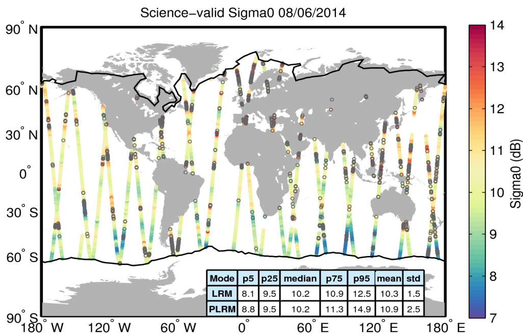
Figure 27. Geographical distribution of science-valid sigma0 data over oceans and lakes for 08/06/2014. The statistical values shown in the table refer to the sigma0 in dB and are calculated separately for LRM and PLRM regions. The black lines mark the outer limit of the Arctic and Antarctic polar polygons. Gray circles denote records that have been rejected based on the editing criteria described in Table 4.
