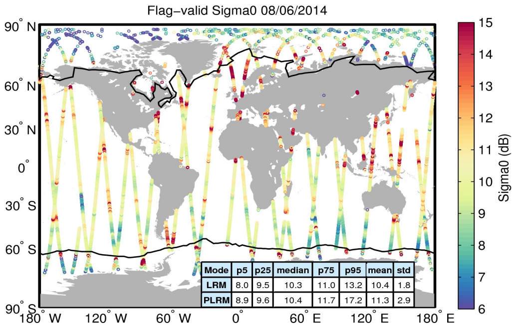
Figure 23. Geographical distribution of flag-valid sigma0 data over oceans and lakes for 08/06/2014. The statistical values shown in the table refer to the sigma0 in dB and are calculated separately for LRM and PLRM regions. Measurements taken over polar polygons have been excluded from the computation of the statistical values. The black lines mark the outer limit of the Arctic and Antarctic polar polygons.
