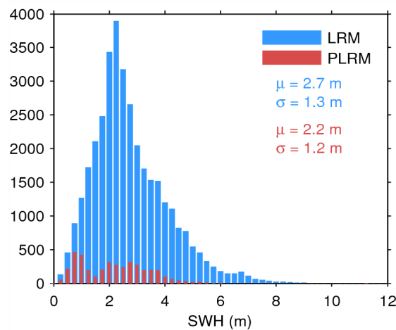
Figure 20. Histogram of science-valid SWH over oceans and lakes for LRM (blue) and PLRM (red) for 08/06/2014. The mean ( \mu ) and standard deviation ( \sigma ) are also shown. Note that values larger than 12 m are excluded from the histogram for the sake of readability but not from the computation of \mu and \sigma .
