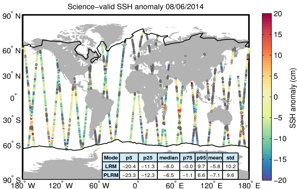
Figure 10. Geographical distribution of science-valid SSH anomaly data over oceans and lakes for 08/06/2014. The statistical values shown in the table refer to the SSH anomaly in cm and are calculated separately for LRM and PLRM regions. The black lines mark the outer limit of the Arctic and Antarctic polar polygons. Gray circles denote records that have been rejected based on the editing criteria described in Table 2.
