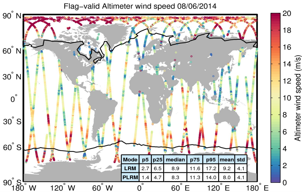
Figure 31. Geographical distribution of flag-valid wind data over oceans and lakes for 08/06/2014. The statistical values shown in the table refer to the wind in m/s and are calculated separately for LRM and PLRM regions. Measurements taken over polar polygons have been excluded from the computation of the statistical values. The black lines mark the outer limit of the Arctic and Antarctic polar polygons.
