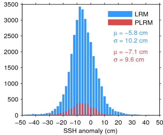
Figure 11. Histogram of science-valid SSH anomaly over oceans and lakes for LRM (blue) and PLRM (red) for 08/06/2014. The mean ( \mu ) and standard deviation ( \sigma ) are also shown. Note that values outside [-50\ 50] cm are excluded from the histogram for the sake of readability but not from the computation of \mu and \sigma .
