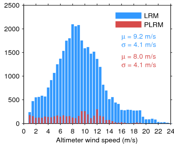
Figure 33. Histogram of flag-valid wind over oceans and lakes for LRM (blue) and PLRM (red) for 08/06/2014. The mean ( \mu ) and standard deviation ( \sigma ) are also shown. Note that values larger than 24 m/s are excluded from the histogram for the sake of readability but not from the computation of \mu and \sigma .
