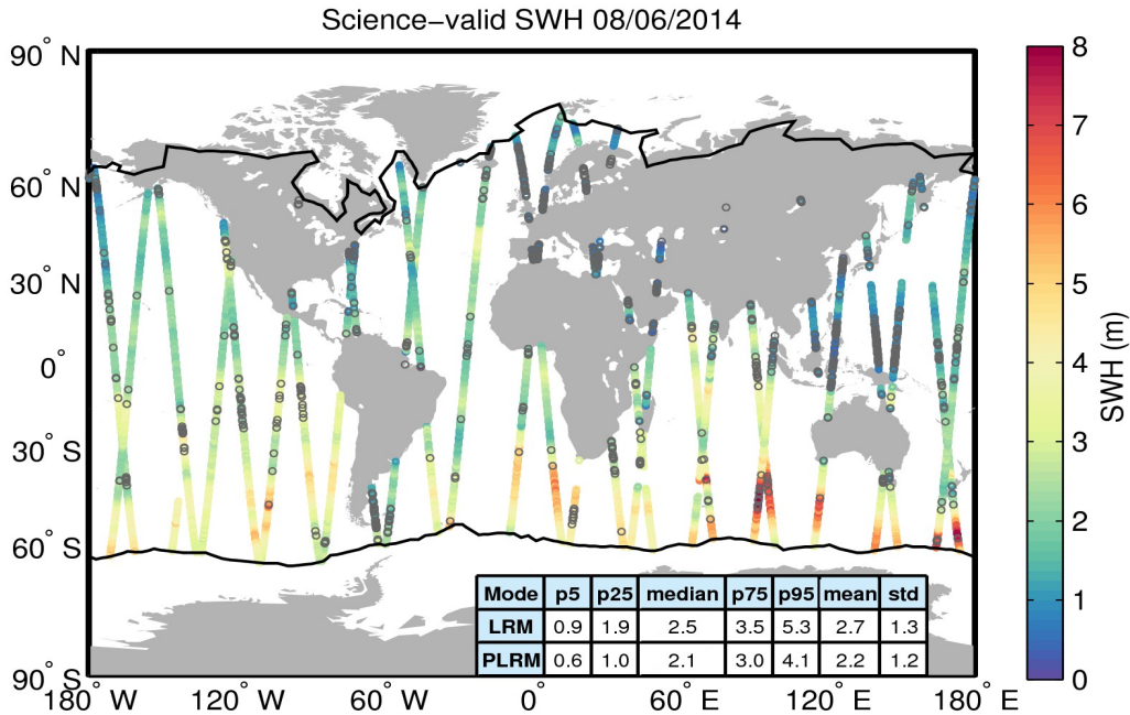
Figure 19. Geographical distribution of science-valid SWH data over oceans and lakes for 08/06/2014. The statistical values shown in the table refer to the SWH in m and are calculated separately for LRM and PLRM regions. The black lines mark the outer limit of the Arctic and Antarctic polar polygons. Gray circles denote records that have been rejected based on the editing criteria described in Table 3.
