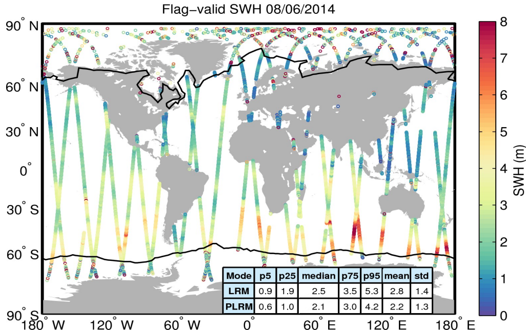
Figure 15. Geographical distribution of flag-valid SWH data over oceans and lakes for 08/06/2014. The statistical values shown in the table refer to the SWH in m and are calculated separately for LRM and PLRM regions. Measurements taken over polar polygons have been excluded from the computation of the statistical values. The black lines mark the outer limit of the Arctic and Antarctic polar polygons.
