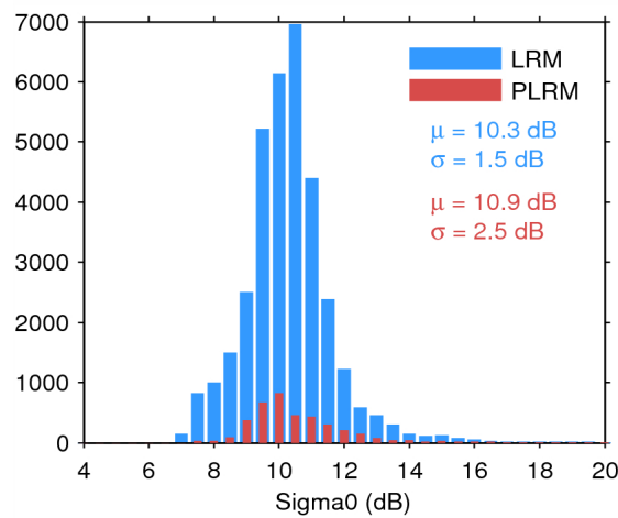
Figure 28. Histogram of science-valid sigma0 over oceans and lakes for LRM (blue) and PLRM (red) for 08/06/2014. The mean ( \mu ) and standard deviation ( \sigma ) are also shown. Note that values outside [4 20] dB are excluded from the histogram for the sake of readability but not from the computation of \mu and \sigma .
