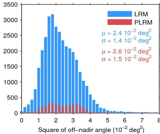
Figure 39. Histogram of flag-valid mispointing over oceans and lakes for LRM (blue) and PLRM (red) for 08/06/2014. Only positive values have been considered. The mean ( \mu ) and standard deviation ( \sigma ) are also shown. Note that values 8 \cdot 10^{-2} \text{ deg}^2 are excluded from the histogram for the sake of readability but not from the computation of \mu and \sigma .
