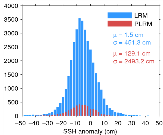
Figure 7. Histogram of flag-valid SSH anomaly over oceans and lakes for LRM (blue) and PLRM (red) for 08/06/2014. The mean ( \mu ) and standard deviation ( \sigma ) are also shown. Note that values outside [-50\ 50] cm are excluded from the histogram for the sake of readability but not from the computation of \mu and \sigma .
