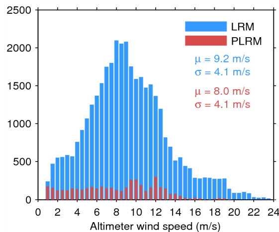
Figure 35. Histogram of science-valid wind over oceans and lakes for LRM (blue) and PLRM (red) for 08/06/2014. The mean ( \mu ) and standard deviation ( \sigma ) are also shown. Note that values larger than 24 m/s are excluded from the histogram for the sake of readability but not from the computation of \mu and \sigma .
