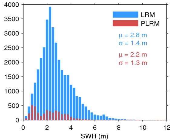
Figure 17. Histogram of flag-valid SWH over oceans and lakes for LRM (blue) and PLRM (red) for 08/06/2014. The mean ( \mu ) and standard deviation ( \sigma ) are also shown. Note that values larger than 12 m are excluded from the histogram for the sake of readability but not from the computation of \mu and \sigma .
