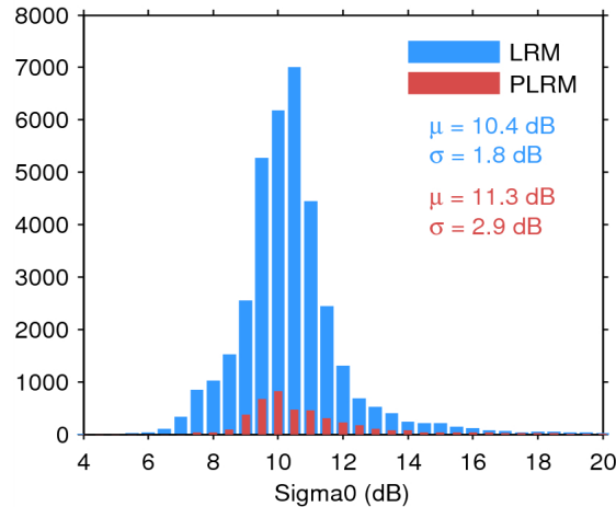
Figure 25. Histogram of flag-valid sigma0 over oceans and lakes for LRM (blue) and PLRM (red) for 08/06/2014. The mean ( \mu ) and standard deviation ( \sigma ) are also shown. Note that values outside [4 20] dB are excluded from the histogram for the sake of readability but not from the computation of \mu and \sigma .
