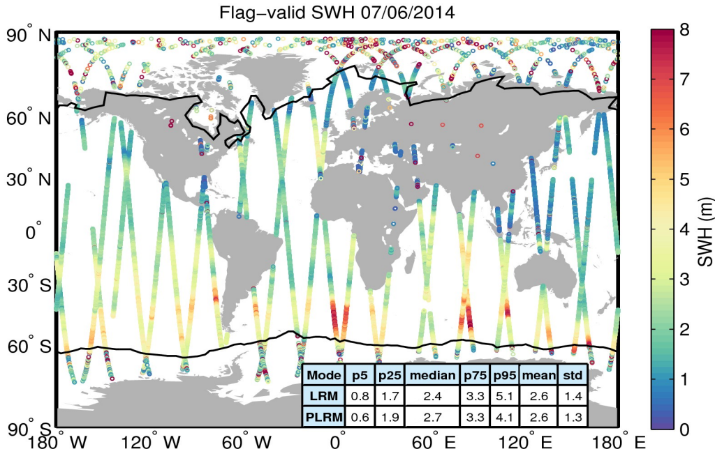
Figure 15. Geographical distribution of flag-valid SWH data over oceans and lakes for 07/06/2014. The statistical values shown in the table refer to the SWH in m and are calculated separately for LRM and PLRM regions. Measurements taken over polar polygons have been excluded from the computation of the statistical values. The black lines mark the outer limit of the Arctic and Antarctic polar polygons.
