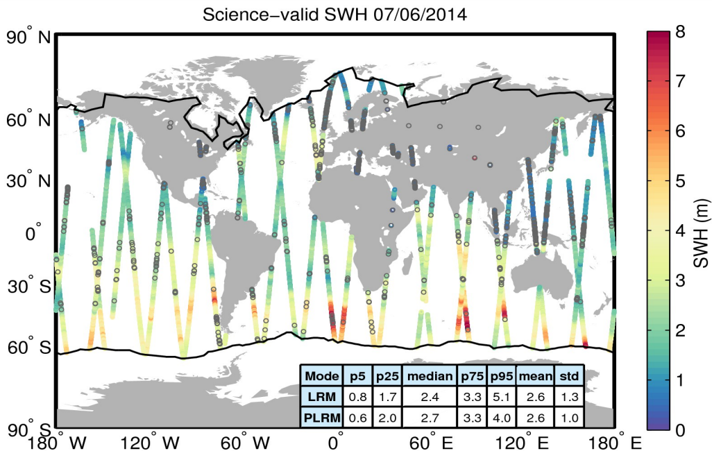
Figure 19. Geographical distribution of science-valid SWH data over oceans and lakes for 07/06/2014. The statistical values shown in the table refer to the SWH in m and are calculated separately for LRM and PLRM regions. The black lines mark the outer limit of the Arctic and Antarctic polar polygons. Gray circles denote records that have been rejected based on the editing criteria described in Table 3.
