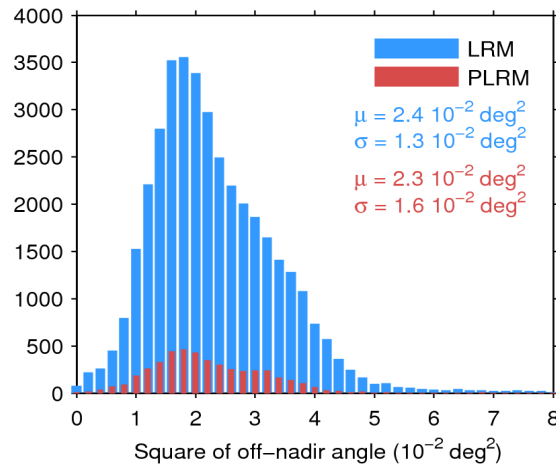
Figure 39. Histogram of flag-valid mispointing over oceans and lakes for LRM (blue) and PLRM (red) for 07/06/2014. Only positive values have been considered. The mean ( \mu ) and standard deviation ( \sigma ) are also shown. Note that values 8 \cdot 10^{-2} \text{ deg}^2 are excluded from the histogram for the sake of readability but not from the computation of \mu and \sigma .
