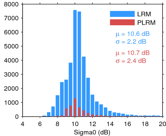
Figure 25. Histogram of flag-valid sigma0 over oceans and lakes for LRM (blue) and PLRM (red) for 07/06/2014. The mean ( \mu ) and standard deviation ( \sigma ) are also shown. Note that values outside [4 20] dB are excluded from the histogram for the sake of readability but not from the computation of \mu and \sigma .
