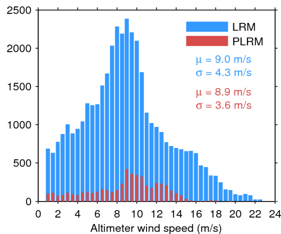
Figure 35. Histogram of science-valid wind over oceans and lakes for LRM (blue) and PLRM (red) for 07/06/2014. The mean ( \mu ) and standard deviation ( \sigma ) are also shown. Note that values larger than 24 m/s are excluded from the histogram for the sake of readability but not from the computation of \mu and \sigma .
