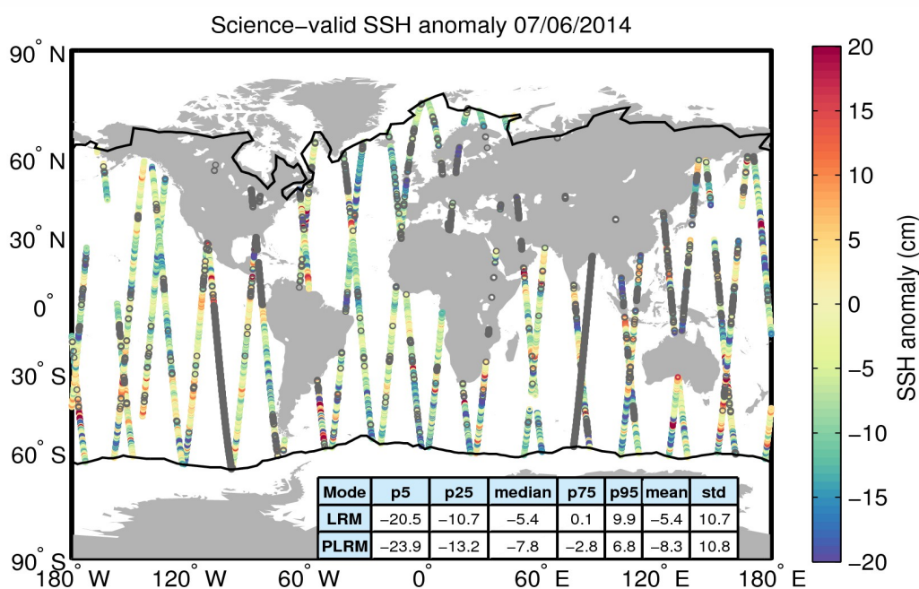
Figure 10. Geographical distribution of science-valid SSH anomaly data over oceans and lakes for 07/06/2014. The statistical values shown in the table refer to the SSH anomaly in cm and are calculated separately for LRM and PLRM regions. The black lines mark the outer limit of the Arctic and Antarctic polar polygons. Gray circles denote records that have been rejected based on the editing criteria described in Table 2.
