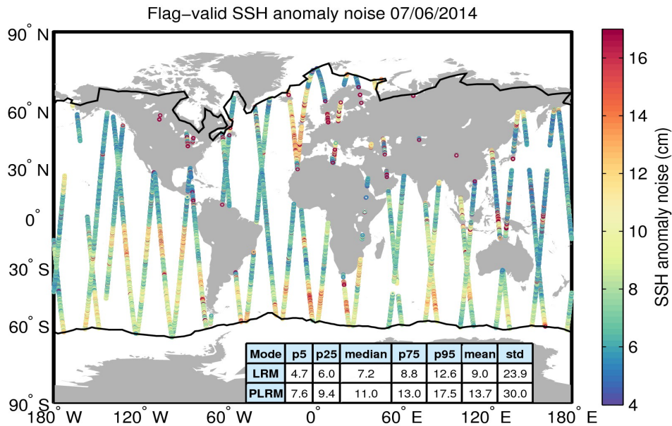
Figure 8. Geographical distribution of flag-valid 20-Hz SSH anomaly measurement noise over oceans and lakes for 07/06/2014. The statistical values shown in the table refer to the SSH anomaly noise and are calculated separately for LRM and PLRM regions. Measurements taken over polar polygons have been excluded from the computation of the statistical values. The black lines mark the outer limit of the Arctic and Antarctic polar polygons.
