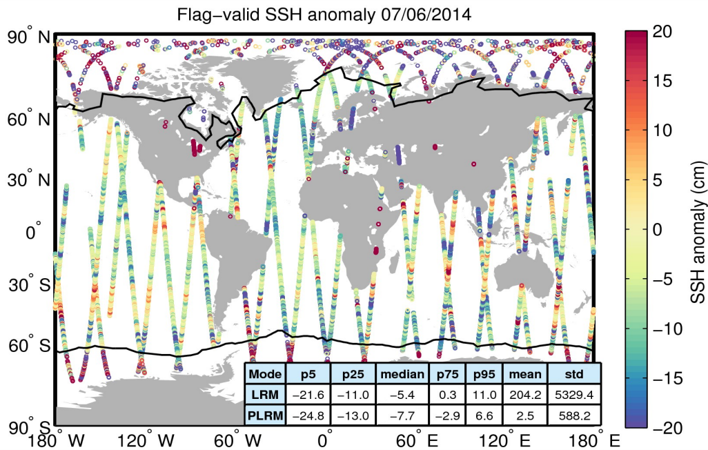
Figure 5. Geographical distribution of flag-valid 1-Hz SSH anomaly data over oceans and lakes for 07/06/2014. The statistical values shown in the table refer to the SSH anomaly in cm and are calculated separately for LRM and PLRM regions. Measurements taken over polar polygons have been excluded from the computation of the statistical values. The black lines mark the outer limit of the Arctic and Antarctic polar polygons.
