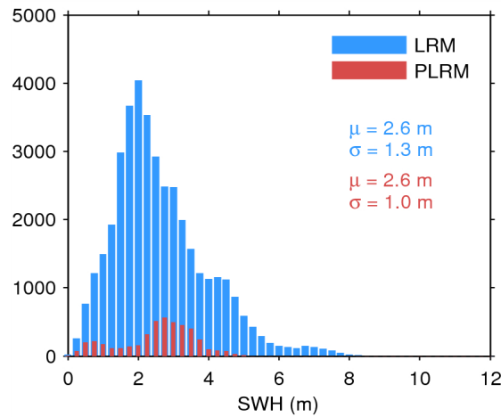
Figure 20. Histogram of science-valid SWH over oceans and lakes for LRM (blue) and PLRM (red) for 07/06/2014. The mean ( \mu ) and standard deviation ( \sigma ) are also shown. Note that values larger than 12 m are excluded from the histogram for the sake of readability but not from the computation of \mu and \sigma .
