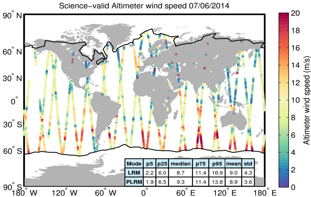
Figure 34. Geographical distribution of science-valid wind data over oceans and lakes for 07/06/2014. The statistical values shown in the table refer to the wind in m/s and are calculated separately for LRM and PLRM regions. The black lines mark the outer limit of the Arctic and Antarctic polar polygons. Gray circles denote records that have been rejected based on the editing criteria described in Table 5.
