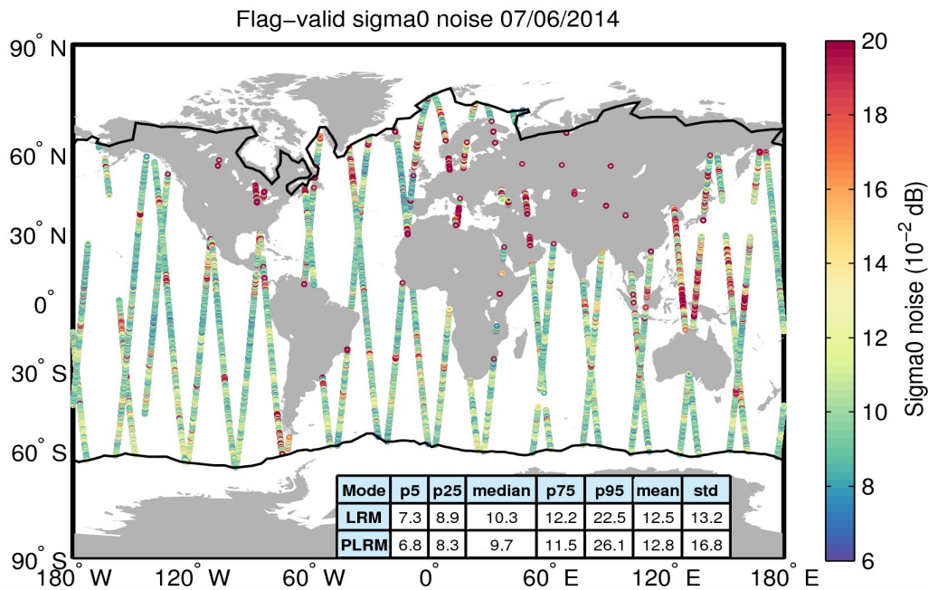
Figure 26. Geographical distribution of flag-valid 20-Hz sigma0 measurement noise over oceans and lakes for 07/06/2014. The statistical values shown in the table refer to the sigma0 noise and are calculated separately for LRM and PLRM regions. Measurements taken over polar polygons have been excluded from the computation of the statistical values. The black lines mark the outer limit of the Arctic and Antarctic polar polygons.
