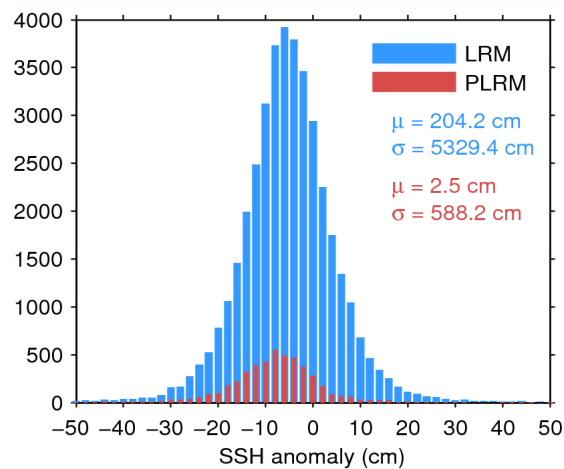
Figure 7. Histogram of flag-valid SSH anomaly over oceans and lakes for LRM (blue) and PLRM (red) for 07/06/2014. The mean ( \mu ) and standard deviation ( \sigma ) are also shown. Note that values outside [-50\ 50] cm are excluded from the histogram for the sake of readability but not from the computation of \mu and \sigma .
