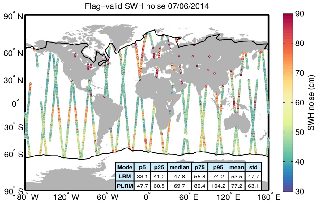
Figure 18. Geographical distribution of flag-valid 20-Hz SWH measurement noise over oceans and lakes for 07/06/2014. The statistical values shown in the table refer to the SWH noise and are calculated separately for LRM and PLRM regions. Measurements taken over polar polygons have been excluded from the computation of the statistical values. The black lines mark the outer limit of the Arctic and Antarctic polar polygons.
