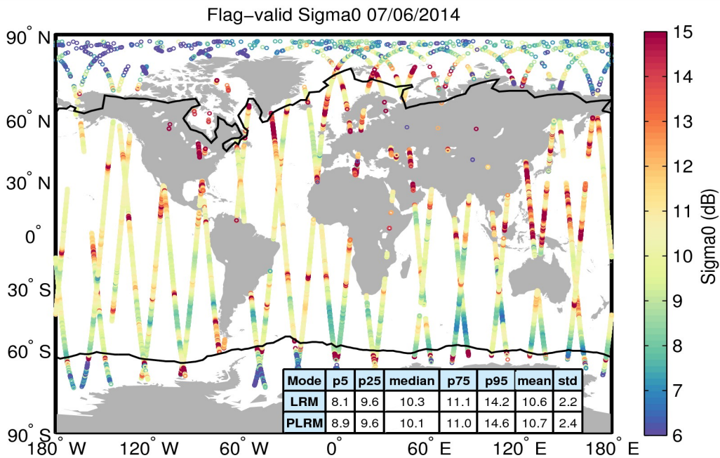
Figure 23. Geographical distribution of flag-valid sigma0 data over oceans and lakes for 07/06/2014. The statistical values shown in the table refer to the sigma0 in dB and are calculated separately for LRM and PLRM regions. Measurements taken over polar polygons have been excluded from the computation of the statistical values. The black lines mark the outer limit of the Arctic and Antarctic polar polygons.
