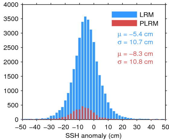
Figure 11. Histogram of science-valid SSH anomaly over oceans and lakes for LRM (blue) and PLRM (red) for 07/06/2014. The mean ( \mu ) and standard deviation ( \sigma ) are also shown. Note that values outside [-50\ 50] cm are excluded from the histogram for the sake of readability but not from the computation of \mu and \sigma .
