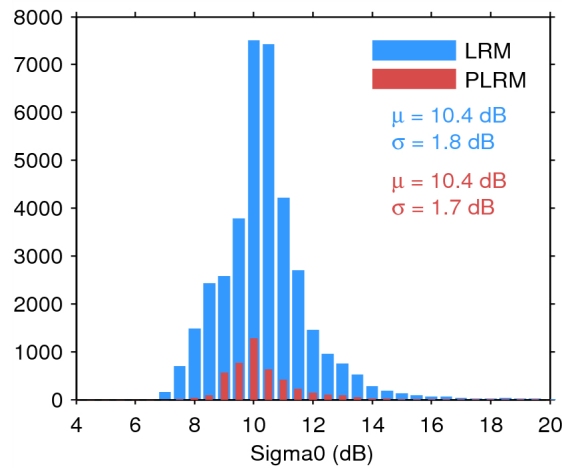
Figure 28. Histogram of science-valid sigma0 over oceans and lakes for LRM (blue) and PLRM (red) for 07/06/2014. The mean ( \mu ) and standard deviation ( \sigma ) are also shown. Note that values outside [4 20] dB are excluded from the histogram for the sake of readability but not from the computation of \mu and \sigma .
