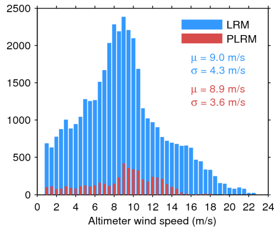
Figure 33. Histogram of flag-valid wind over oceans and lakes for LRM (blue) and PLRM (red) for 07/06/2014. The mean ( \mu ) and standard deviation ( \sigma ) are also shown. Note that values larger than 24 m/s are excluded from the histogram for the sake of readability but not from the computation of \mu and \sigma .
