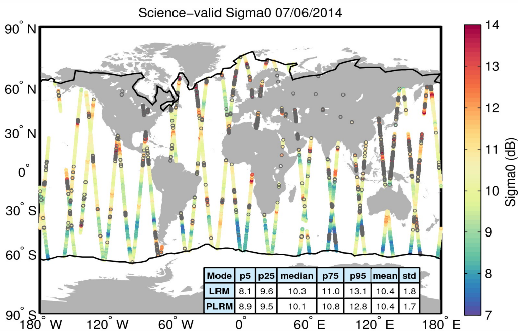
Figure 27. Geographical distribution of science-valid sigma0 data over oceans and lakes for 07/06/2014. The statistical values shown in the table refer to the sigma0 in dB and are calculated separately for LRM and PLRM regions. The black lines mark the outer limit of the Arctic and Antarctic polar polygons. Gray circles denote records that have been rejected based on the editing criteria described in Table 4.
