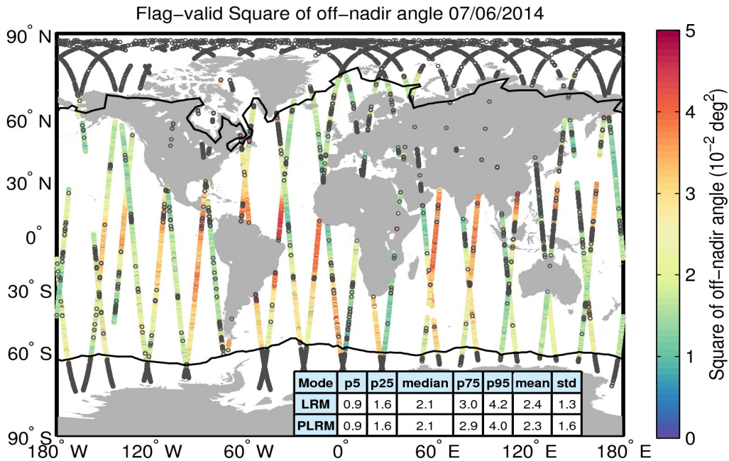
Figure 37. Geographical distribution of flag-valid mispointing data over oceans and lakes for 07/06/2014. The statistical values shown in the table refer to the mispointing in 10^{-2} \text{ deg}^2 and are calculated separately for LRM and PLRM regions. Measurements taken over polar polygons have been excluded from the computation of the statistical values. The black lines mark the outer limit of the Arctic and Antarctic polar polygons. Gray circles denote negative values.
