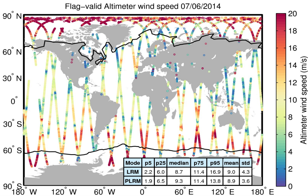
Figure 31. Geographical distribution of flag-valid wind data over oceans and lakes for 07/06/2014. The statistical values shown in the table refer to the wind in m/s and are calculated separately for LRM and PLRM regions. Measurements taken over polar polygons have been excluded from the computation of the statistical values. The black lines mark the outer limit of the Arctic and Antarctic polar polygons.
