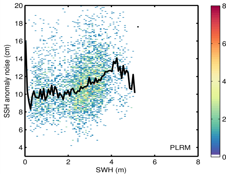
Figure 9. 2D histogram showing flag-valid SSH anomaly noise as a function of SWH for LRM (top) and PLRM (bottom) for 07/06/2014. The black line denotes the median SSH anomaly as a function of SWH.
