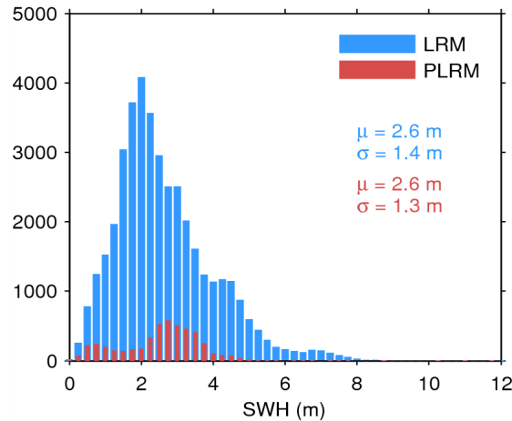
Figure 17. Histogram of flag-valid SWH over oceans and lakes for LRM (blue) and PLRM (red) for 07/06/2014. The mean ( \mu ) and standard deviation ( \sigma ) are also shown. Note that values larger than 12 m are excluded from the histogram for the sake of readability but not from the computation of \mu and \sigma .
