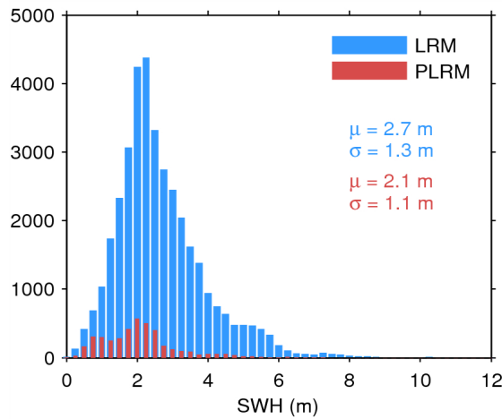
Figure 20. Histogram of science-valid SWH over oceans and lakes for LRM (blue) and PLRM (red) for 04/06/2014. The mean ( \mu ) and standard deviation ( \sigma ) are also shown. Note that values larger than 12 m are excluded from the histogram for the sake of readability but not from the computation of \mu and \sigma .
