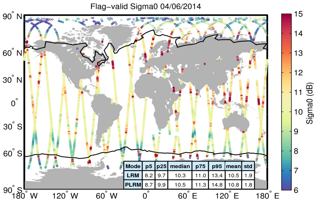
Figure 23. Geographical distribution of flag-valid sigma0 data over oceans and lakes for 04/06/2014. The statistical values shown in the table refer to the sigma0 in dB and are calculated separately for LRM and PLRM regions. Measurements taken over polar polygons have been excluded from the computation of the statistical values. The black lines mark the outer limit of the Arctic and Antarctic polar polygons.
