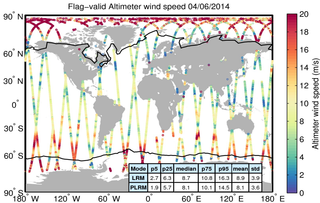
Figure 31. Geographical distribution of flag-valid wind data over oceans and lakes for 04/06/2014. The statistical values shown in the table refer to the wind in m/s and are calculated separately for LRM and PLRM regions. Measurements taken over polar polygons have been excluded from the computation of the statistical values. The black lines mark the outer limit of the Arctic and Antarctic polar polygons.
