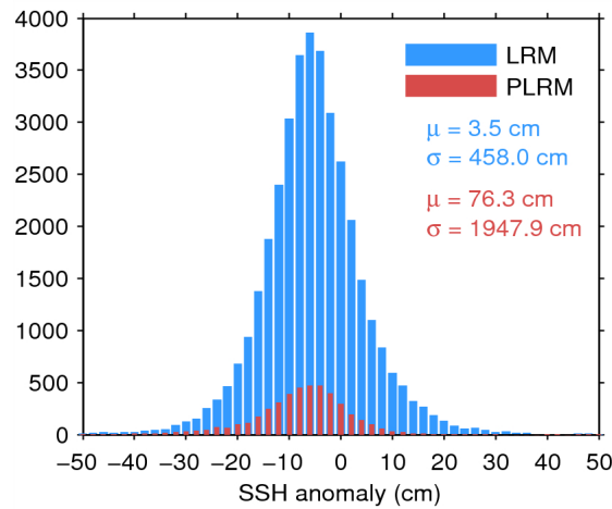
Figure 7. Histogram of flag-valid SSH anomaly over oceans and lakes for LRM (blue) and PLRM (red) for 04/06/2014. The mean ( \mu ) and standard deviation ( \sigma ) are also shown. Note that values outside [-50\ 50] cm are excluded from the histogram for the sake of readability but not from the computation of \mu and \sigma .
