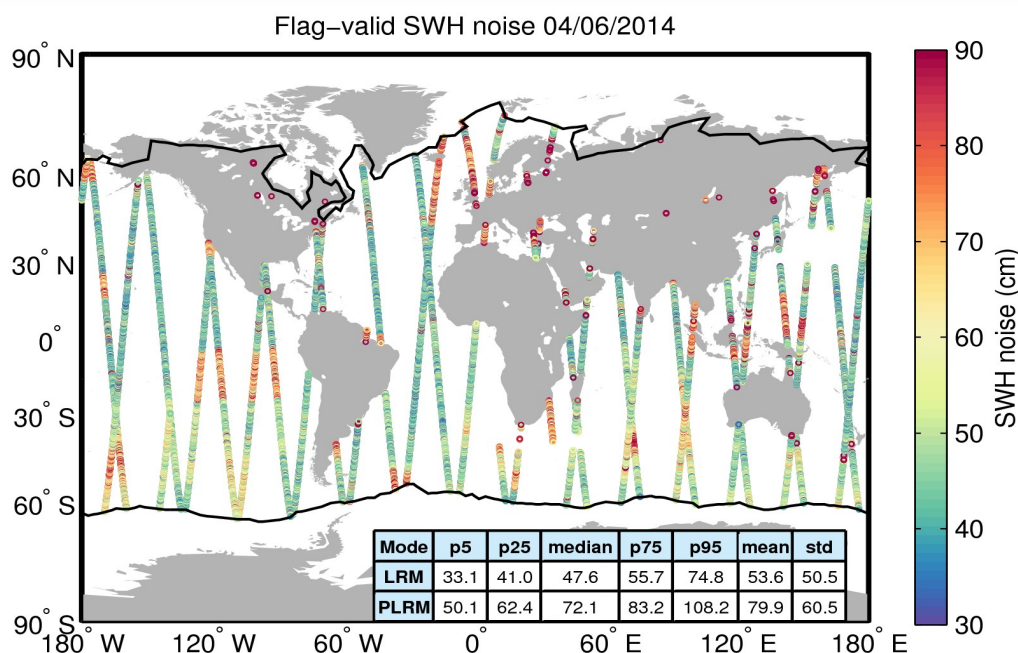
Figure 18. Geographical distribution of flag-valid 20-Hz SWH measurement noise over oceans and lakes for 04/06/2014. The statistical values shown in the table refer to the SWH noise and are calculated separately for LRM and PLRM regions. Measurements taken over polar polygons have been excluded from the computation of the statistical values. The black lines mark the outer limit of the Arctic and Antarctic polar polygons.
