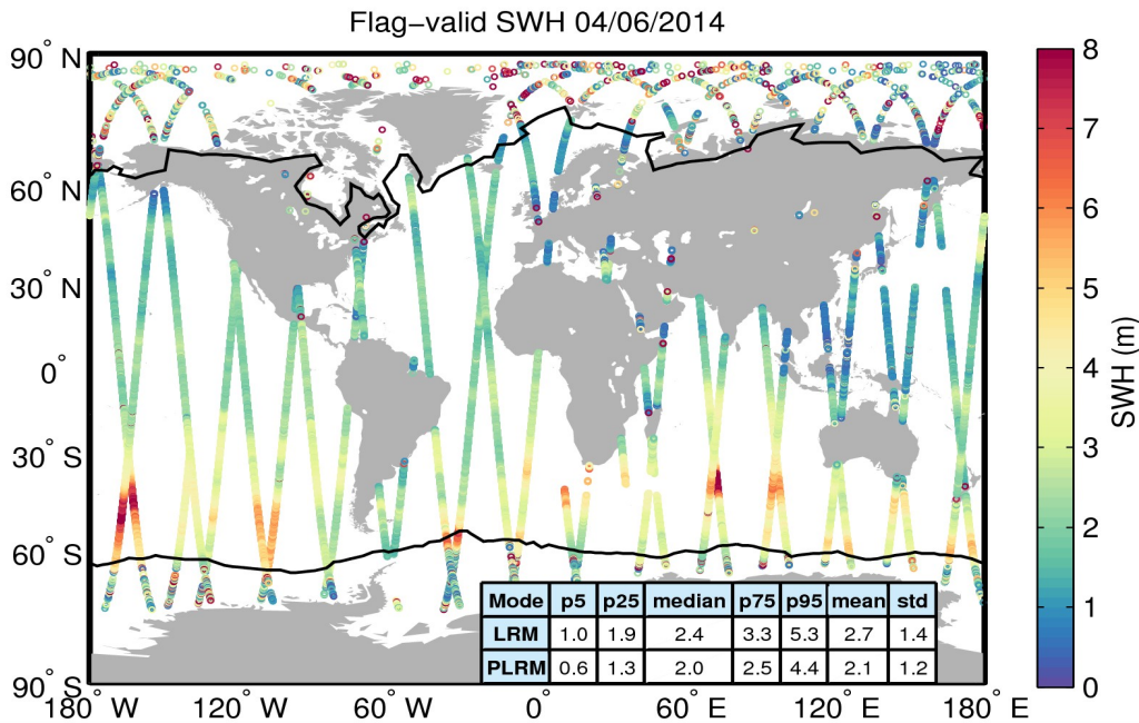
Figure 15. Geographical distribution of flag-valid SWH data over oceans and lakes for 04/06/2014. The statistical values shown in the table refer to the SWH in m and are calculated separately for LRM and PLRM regions. Measurements taken over polar polygons have been excluded from the computation of the statistical values. The black lines mark the outer limit of the Arctic and Antarctic polar polygons.
