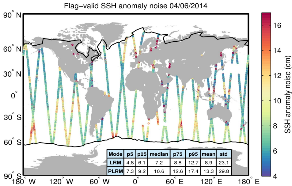
Figure 8. Geographical distribution of flag-valid 20-Hz SSH anomaly measurement noise over oceans and lakes for 04/06/2014. The statistical values shown in the table refer to the SSH anomaly noise and are calculated separately for LRM and PLRM regions. Measurements taken over polar polygons have been excluded from the computation of the statistical values. The black lines mark the outer limit of the Arctic and Antarctic polar polygons.
