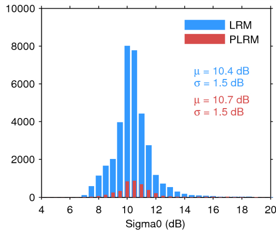
Figure 28. Histogram of science-valid sigma0 over oceans and lakes for LRM (blue) and PLRM (red) for 04/06/2014. The mean ( \mu ) and standard deviation ( \sigma ) are also shown. Note that values outside [4 20] dB are excluded from the histogram for the sake of readability but not from the computation of \mu and \sigma .
