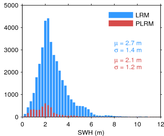
Figure 17. Histogram of flag-valid SWH over oceans and lakes for LRM (blue) and PLRM (red) for 04/06/2014. The mean ( \mu ) and standard deviation ( \sigma ) are also shown. Note that values larger than 12 m are excluded from the histogram for the sake of readability but not from the computation of \mu and \sigma .
