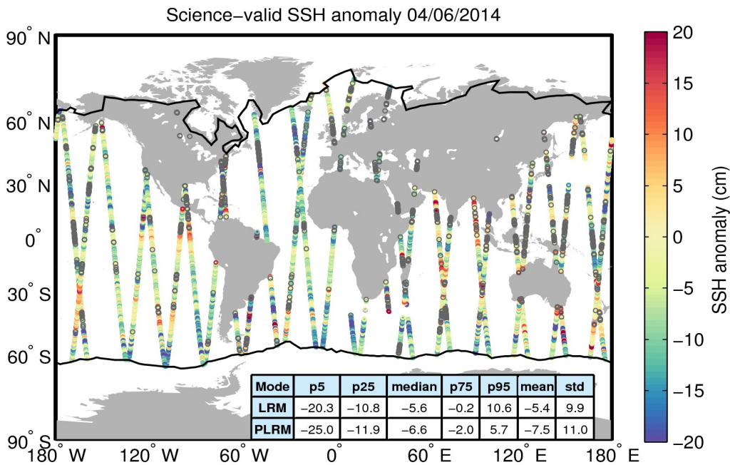
Figure 10. Geographical distribution of science-valid SSH anomaly data over oceans and lakes for 04/06/2014. The statistical values shown in the table refer to the SSH anomaly in cm and are calculated separately for LRM and PLRM regions. The black lines mark the outer limit of the Arctic and Antarctic polar polygons. Gray circles denote records that have been rejected based on the editing criteria described in Table 2.
