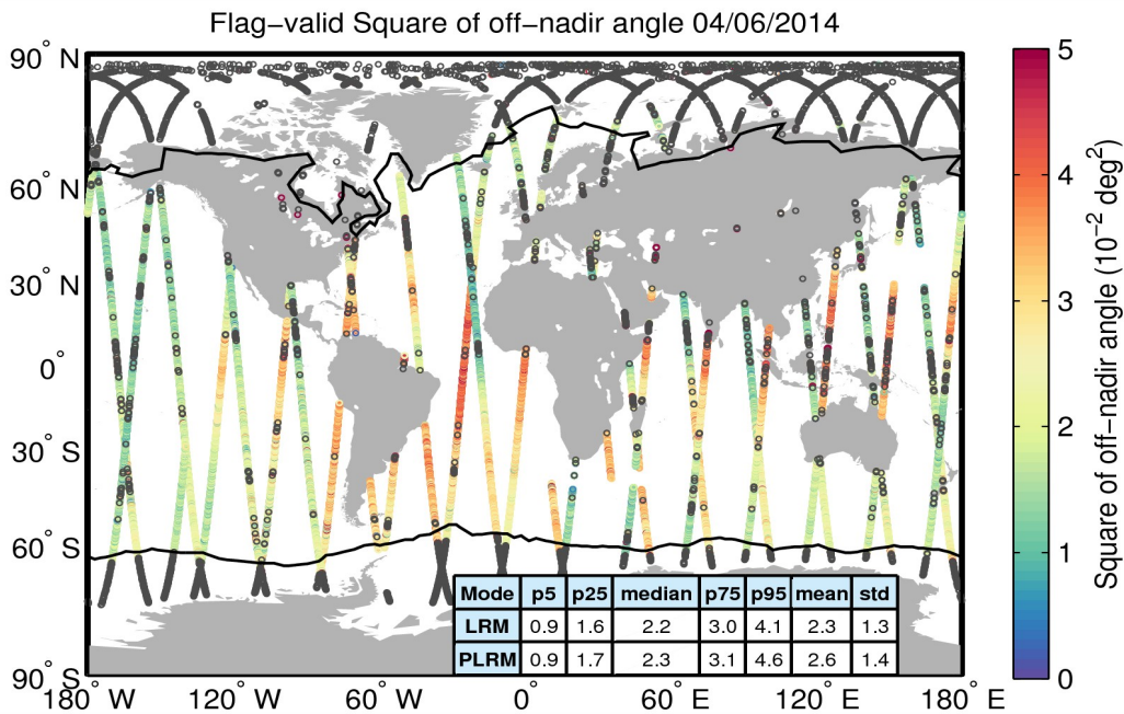
Figure 37. Geographical distribution of flag-valid mispointing data over oceans and lakes for 04/06/2014. The statistical values shown in the table refer to the mispointing in 10^{-2} \text{ deg}^2 and are calculated separately for LRM and PLRM regions. Measurements taken over polar polygons have been excluded from the computation of the statistical values. The black lines mark the outer limit of the Arctic and Antarctic polar polygons. Gray circles denote negative values.
