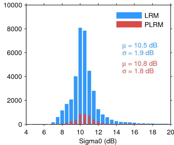
Figure 25. Histogram of flag-valid sigma0 over oceans and lakes for LRM (blue) and PLRM (red) for 04/06/2014. The mean ( \mu ) and standard deviation ( \sigma ) are also shown. Note that values outside [4 20] dB are excluded from the histogram for the sake of readability but not from the computation of \mu and \sigma .
