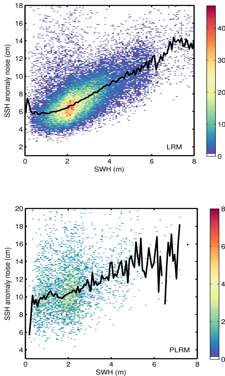
Figure 9. 2D histogram showing flag-valid SSH anomaly noise as a function of SWH for LRM (top) and PLRM (bottom) for 04/06/2014. The black line denotes the median SSH anomaly as a function of SWH.
