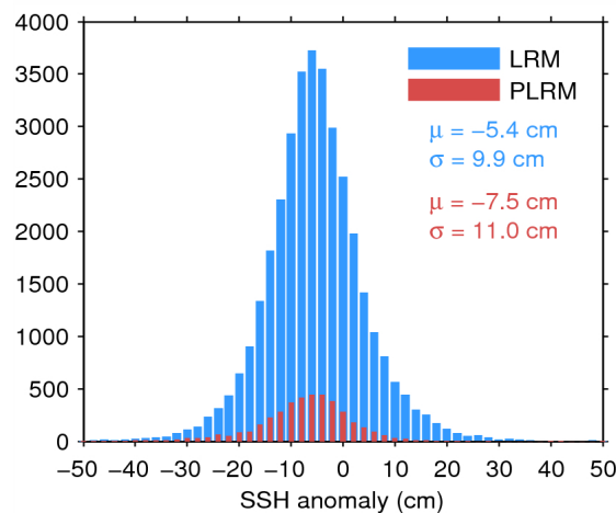
Figure 11. Histogram of science-valid SSH anomaly over oceans and lakes for LRM (blue) and PLRM (red) for 04/06/2014. The mean ( \mu ) and standard deviation ( \sigma ) are also shown. Note that values outside [-50 50] cm are excluded from the histogram for the sake of readability but not from the computation of \mu and \sigma .
