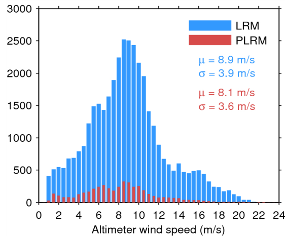
Figure 33. Histogram of flag-valid wind over oceans and lakes for LRM (blue) and PLRM (red) for 04/06/2014. The mean ( \mu ) and standard deviation ( \sigma ) are also shown. Note that values larger than 24 m/s are excluded from the histogram for the sake of readability but not from the computation of \mu and \sigma .
