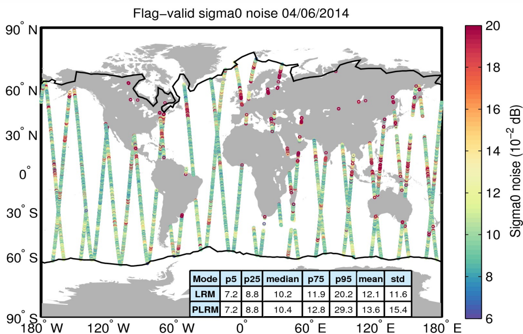
Figure 26. Geographical distribution of flag-valid 20-Hz sigma0 measurement noise over oceans and lakes for 04/06/2014. The statistical values shown in the table refer to the sigma0 noise and are calculated separately for LRM and PLRM regions. Measurements taken over polar polygons have been excluded from the computation of the statistical values. The black lines mark the outer limit of the Arctic and Antarctic polar polygons.
