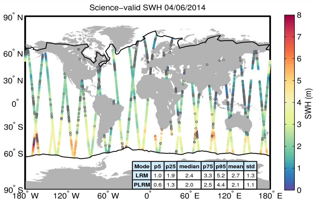
Figure 19. Geographical distribution of science-valid SWH data over oceans and lakes for 04/06/2014. The statistical values shown in the table refer to the SWH in m and are calculated separately for LRM and PLRM regions. The black lines mark the outer limit of the Arctic and Antarctic polar polygons. Gray circles denote records that have been rejected based on the editing criteria described in Table 3.
