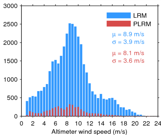
Figure 35. Histogram of science-valid wind over oceans and lakes for LRM (blue) and PLRM (red) for 04/06/2014. The mean ( \mu ) and standard deviation ( \sigma ) are also shown. Note that values larger than 24 m/s are excluded from the histogram for the sake of readability but not from the computation of \mu and \sigma .
