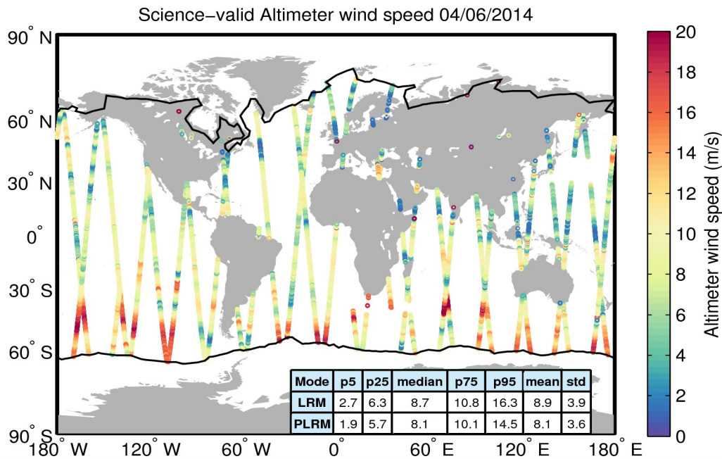
Figure 34. Geographical distribution of science-valid wind data over oceans and lakes for 04/06/2014. The statistical values shown in the table refer to the wind in m/s and are calculated separately for LRM and PLRM regions. The black lines mark the outer limit of the Arctic and Antarctic polar polygons. Gray circles denote records that have been rejected based on the editing criteria described in Table 5.
