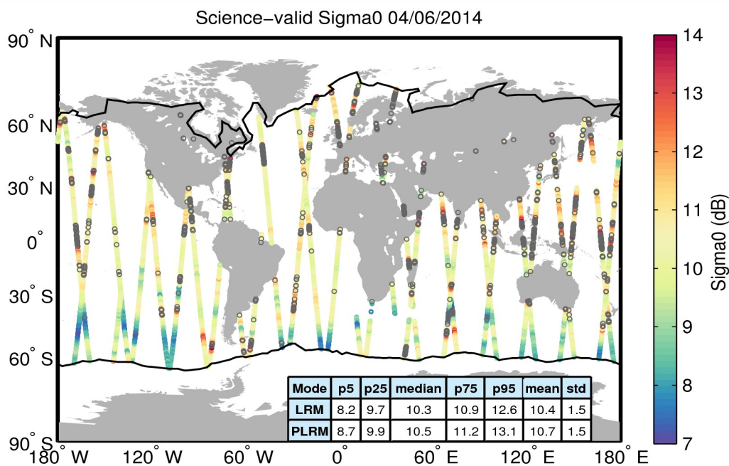
Figure 27. Geographical distribution of science-valid sigma0 data over oceans and lakes for 04/06/2014. The statistical values shown in the table refer to the sigma0 in dB and are calculated separately for LRM and PLRM regions. The black lines mark the outer limit of the Arctic and Antarctic polar polygons. Gray circles denote records that have been rejected based on the editing criteria described in Table 4.
