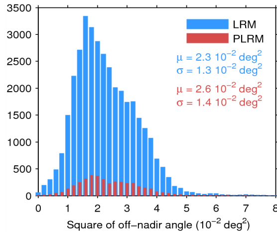
Figure 39. Histogram of flag-valid mispointing over oceans and lakes for LRM (blue) and PLRM (red) for 04/06/2014. Only positive values have been considered. The mean ( \mu ) and standard deviation ( \sigma ) are also shown. Note that values 8 \cdot 10^{-2} \text{ deg}^2 are excluded from the histogram for the sake of readability but not from the computation of \mu and \sigma .
