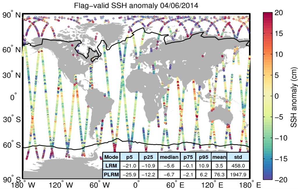
Figure 5. Geographical distribution of flag-valid 1-Hz SSH anomaly data over oceans and lakes for 04/06/2014. The statistical values shown in the table refer to the SSH anomaly in cm and are calculated separately for LRM and PLRM regions. Measurements taken over polar polygons have been excluded from the computation of the statistical values. The black lines mark the outer limit of the Arctic and Antarctic polar polygons.
