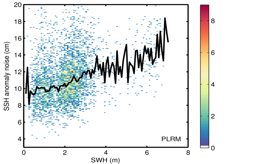
Figure 9. 2D histogram showing flag-valid SSH anomaly noise as a function of SWH for LRM (top) and PLRM (bottom) for 02/06/2014. The black line denotes the median SSH anomaly as a function of SWH.
