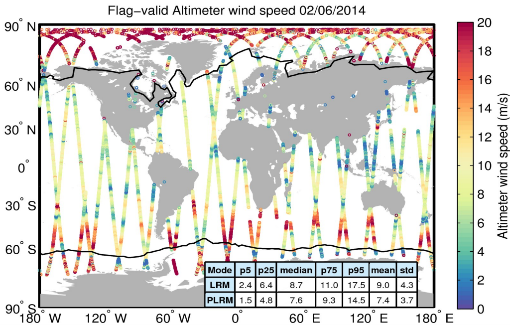
Figure 31. Geographical distribution of flag-valid wind data over oceans and lakes for 02/06/2014. The statistical values shown in the table refer to the wind in m/s and are calculated separately for LRM and PLRM regions. Measurements taken over polar polygons have been excluded from the computation of the statistical values. The black lines mark the outer limit of the Arctic and Antarctic polar polygons.
