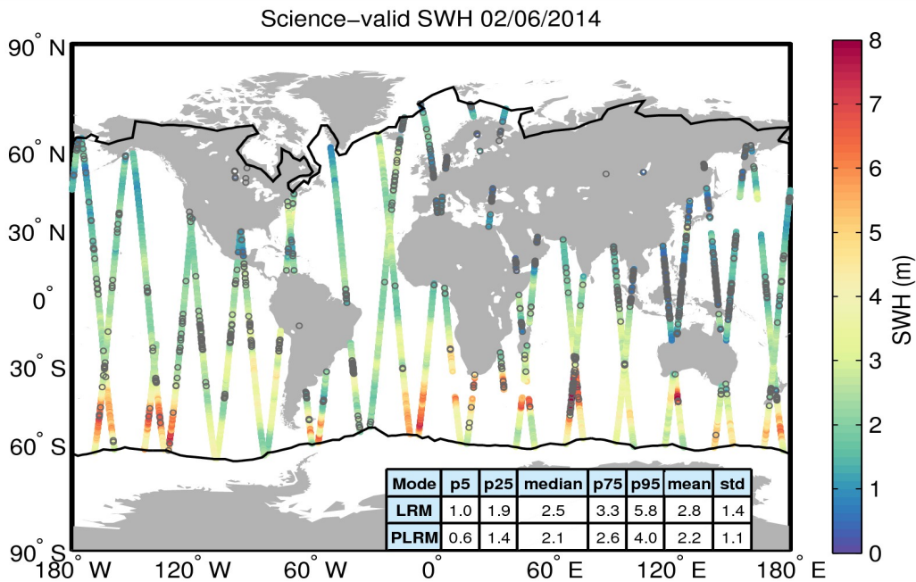
Figure 19. Geographical distribution of science-valid SWH data over oceans and lakes for 02/06/2014. The statistical values shown in the table refer to the SWH in m and are calculated separately for LRM and PLRM regions. The black lines mark the outer limit of the Arctic and Antarctic polar polygons. Gray circles denote records that have been rejected based on the editing criteria described in Table 3.
