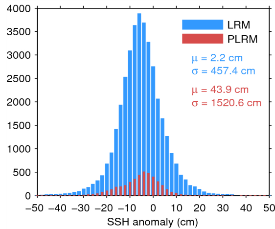
Figure 7. Histogram of flag-valid SSH anomaly over oceans and lakes for LRM (blue) and PLRM (red) for 02/06/2014. The mean ( \mu ) and standard deviation ( \sigma ) are also shown. Note that values outside [-50\ 50] cm are excluded from the histogram for the sake of readability but not from the computation of \mu and \sigma .
