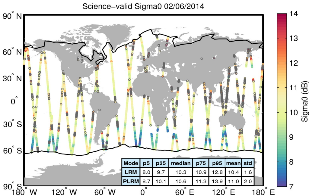
Figure 27. Geographical distribution of science-valid sigma0 data over oceans and lakes for 02/06/2014. The statistical values shown in the table refer to the sigma0 in dB and are calculated separately for LRM and PLRM regions. The black lines mark the outer limit of the Arctic and Antarctic polar polygons. Gray circles denote records that have been rejected based on the editing criteria described in Table 4.
