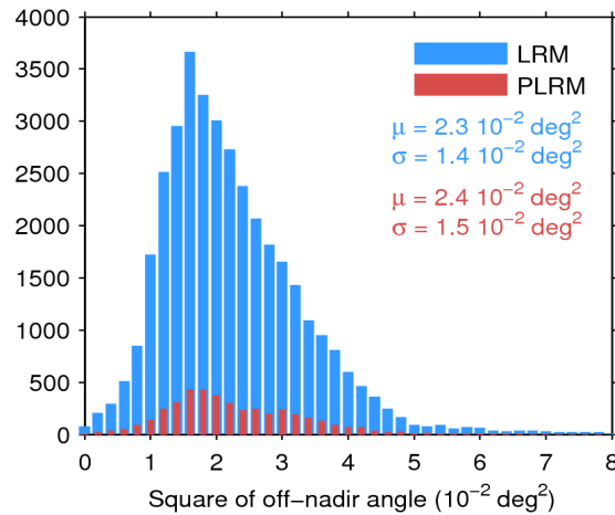
Figure 39. Histogram of flag-valid mispointing over oceans and lakes for LRM (blue) and PLRM (red) for 02/06/2014. Only positive values have been considered. The mean ( \mu ) and standard deviation ( \sigma ) are also shown. Note that values 8 \cdot 10^{-2} \text{ deg}^2 are excluded from the histogram for the sake of readability but not from the computation of \mu and \sigma .
