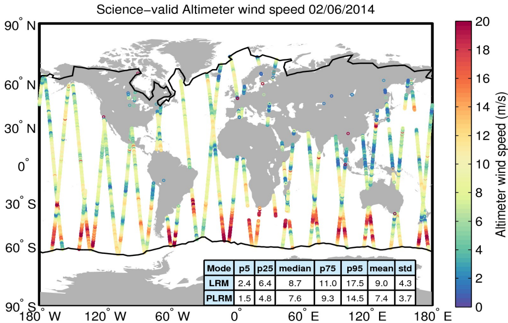
Figure 34. Geographical distribution of science-valid wind data over oceans and lakes for 02/06/2014. The statistical values shown in the table refer to the wind in m/s and are calculated separately for LRM and PLRM regions. The black lines mark the outer limit of the Arctic and Antarctic polar polygons. Gray circles denote records that have been rejected based on the editing criteria described in Table 5.
