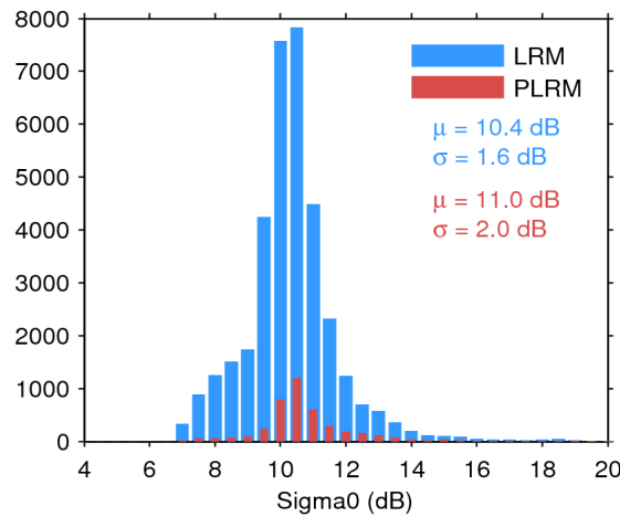
Figure 28. Histogram of science-valid sigma0 over oceans and lakes for LRM (blue) and PLRM (red) for 02/06/2014. The mean ( \mu ) and standard deviation ( \sigma ) are also shown. Note that values outside [4 20] dB are excluded from the histogram for the sake of readability but not from the computation of \mu and \sigma .
