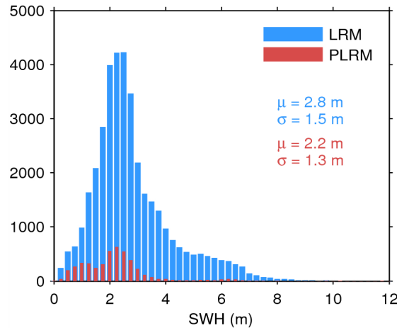
Figure 17. Histogram of flag-valid SWH over oceans and lakes for LRM (blue) and PLRM (red) for 02/06/2014. The mean ( \mu ) and standard deviation ( \sigma ) are also shown. Note that values larger than 12 m are excluded from the histogram for the sake of readability but not from the computation of \mu and \sigma .
