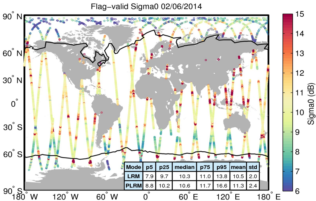
Figure 23. Geographical distribution of flag-valid sigma0 data over oceans and lakes for 02/06/2014. The statistical values shown in the table refer to the sigma0 in dB and are calculated separately for LRM and PLRM regions. Measurements taken over polar polygons have been excluded from the computation of the statistical values. The black lines mark the outer limit of the Arctic and Antarctic polar polygons.
