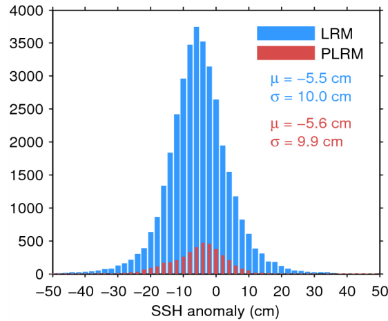
Figure 11. Histogram of science-valid SSH anomaly over oceans and lakes for LRM (blue) and PLRM (red) for 02/06/2014. The mean ( \mu ) and standard deviation ( \sigma ) are also shown. Note that values outside [-50\ 50] cm are excluded from the histogram for the sake of readability but not from the computation of \mu and \sigma .
