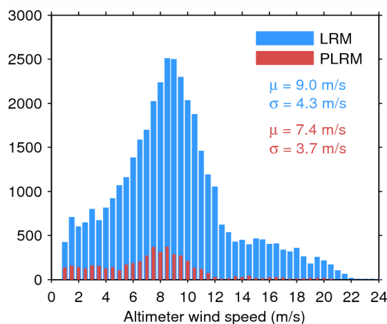
Figure 33. Histogram of flag-valid wind over oceans and lakes for LRM (blue) and PLRM (red) for 02/06/2014. The mean ( \mu ) and standard deviation ( \sigma ) are also shown. Note that values larger than 24 m/s are excluded from the histogram for the sake of readability but not from the computation of \mu and \sigma .
