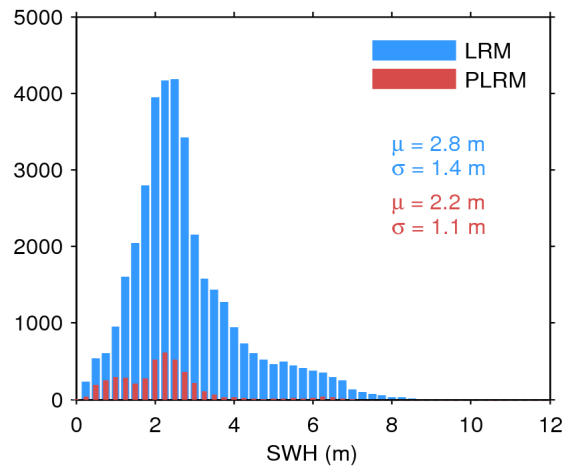
Figure 20. Histogram of science-valid SWH over oceans and lakes for LRM (blue) and PLRM (red) for 02/06/2014. The mean ( \mu ) and standard deviation ( \sigma ) are also shown. Note that values larger than 12 m are excluded from the histogram for the sake of readability but not from the computation of \mu and \sigma .
