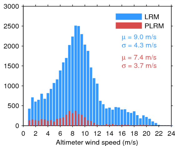
Figure 35. Histogram of science-valid wind over oceans and lakes for LRM (blue) and PLRM (red) for 02/06/2014. The mean ( \mu ) and standard deviation ( \sigma ) are also shown. Note that values larger than 24 m/s are excluded from the histogram for the sake of readability but not from the computation of \mu and \sigma .
