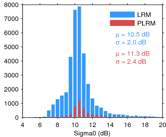
Figure 25. Histogram of flag-valid sigma0 over oceans and lakes for LRM (blue) and PLRM (red) for 02/06/2014. The mean ( \mu ) and standard deviation ( \sigma ) are also shown. Note that values outside [4 20] dB are excluded from the histogram for the sake of readability but not from the computation of \mu and \sigma .
