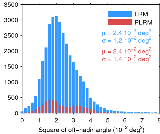
Figure 39. Histogram of flag-valid mispointing over oceans and lakes for LRM (blue) and PLRM (red) for 31/05/2014. Only positive values have been considered. The mean ( \mu ) and standard deviation ( \sigma ) are also shown. Note that values 8 \cdot 10^{-2} \text{ deg}^2 are excluded from the histogram for the sake of readability but not from the computation of \mu and \sigma .
