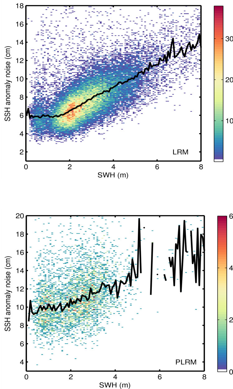
Figure 9. 2D histogram showing flag-valid SSH anomaly noise as a function of SWH for LRM (top) and PLRM (bottom) for 31/05/2014. The black line denotes the median SSH anomaly as a function of SWH.
