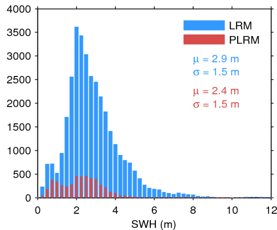
Figure 17. Histogram of flag-valid SWH over oceans and lakes for LRM (blue) and PLRM (red) for 31/05/2014. The mean ( \mu ) and standard deviation ( \sigma ) are also shown. Note that values larger than 12 m are excluded from the histogram for the sake of readability but not from the computation of \mu and \sigma .
