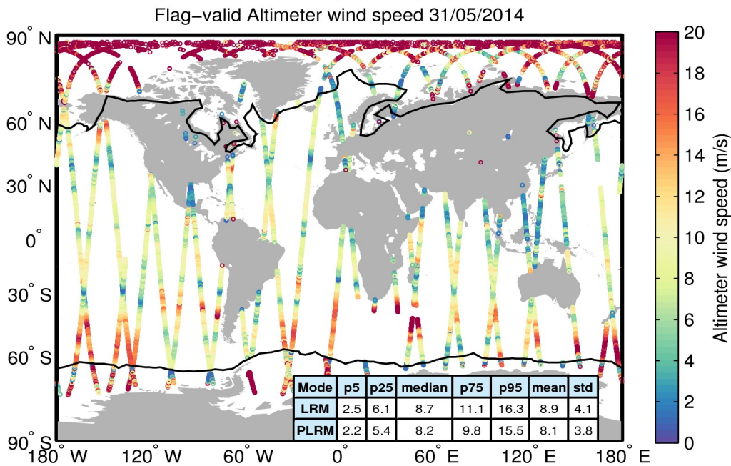
Figure 31. Geographical distribution of flag-valid wind data over oceans and lakes for 31/05/2014. The statistical values shown in the table refer to the wind in m/s and are calculated separately for LRM and PLRM regions. Measurements taken over polar polygons have been excluded from the computation of the statistical values. The black lines mark the outer limit of the Arctic and Antarctic polar polygons.
