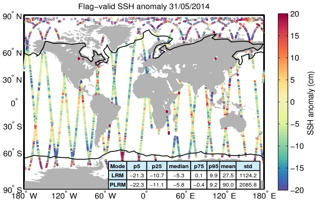
Figure 5. Geographical distribution of flag-valid 1-Hz SSH anomaly data over oceans and lakes for 31/05/2014. The statistical values shown in the table refer to the SSH anomaly in cm and are calculated separately for LRM and PLRM regions. Measurements taken over polar polygons have been excluded from the computation of the statistical values. The black lines mark the outer limit of the Arctic and Antarctic polar polygons.
