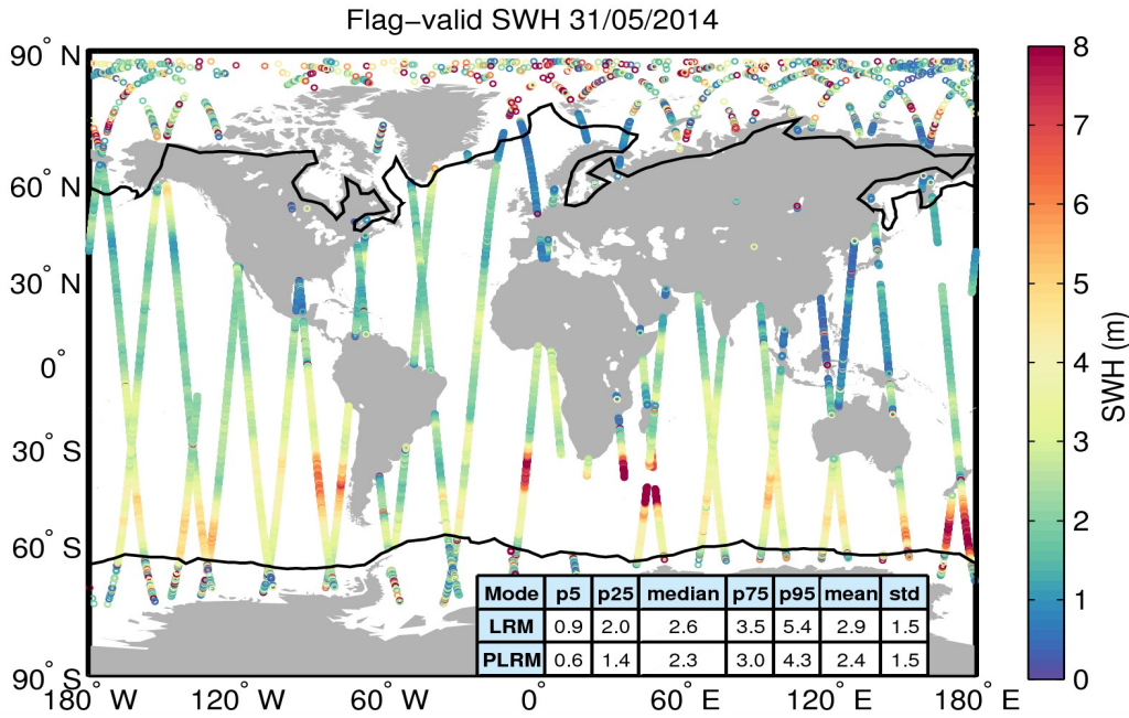
Figure 15. Geographical distribution of flag-valid SWH data over oceans and lakes for 31/05/2014. The statistical values shown in the table refer to the SWH in m and are calculated separately for LRM and PLRM regions. Measurements taken over polar polygons have been excluded from the computation of the statistical values. The black lines mark the outer limit of the Arctic and Antarctic polar polygons.
