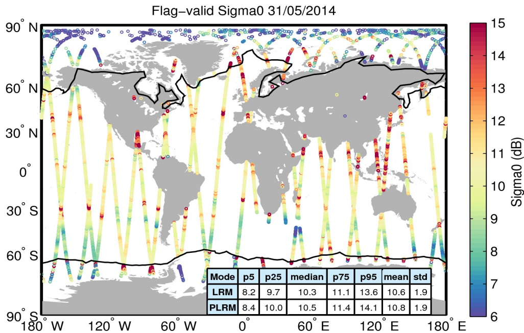
Figure 23. Geographical distribution of flag-valid sigma0 data over oceans and lakes for 31/05/2014. The statistical values shown in the table refer to the sigma0 in dB and are calculated separately for LRM and PLRM regions. Measurements taken over polar polygons have been excluded from the computation of the statistical values. The black lines mark the outer limit of the Arctic and Antarctic polar polygons.
