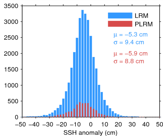
Figure 11. Histogram of science-valid SSH anomaly over oceans and lakes for LRM (blue) and PLRM (red) for 31/05/2014. The mean ( \mu ) and standard deviation ( \sigma ) are also shown. Note that values outside [-50 50] cm are excluded from the histogram for the sake of readability but not from the computation of \mu and \sigma .
