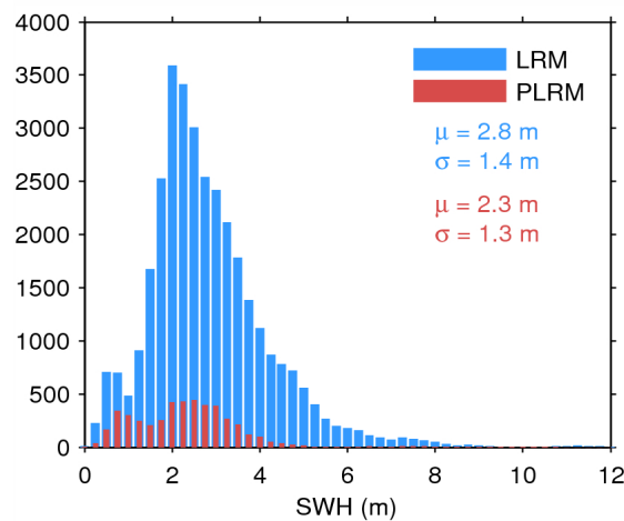
Figure 20. Histogram of science-valid SWH over oceans and lakes for LRM (blue) and PLRM (red) for 31/05/2014. The mean ( \mu ) and standard deviation ( \sigma ) are also shown. Note that values larger than 12 m are excluded from the histogram for the sake of readability but not from the computation of \mu and \sigma .
