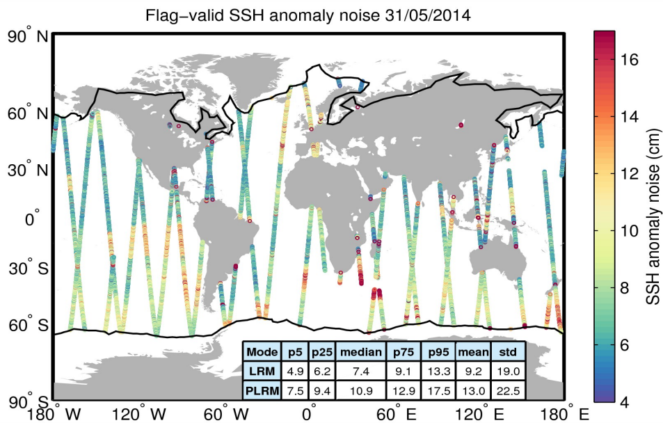
Figure 8. Geographical distribution of flag-valid 20-Hz SSH anomaly measurement noise over oceans and lakes for 31/05/2014. The statistical values shown in the table refer to the SSH anomaly noise and are calculated separately for LRM and PLRM regions. Measurements taken over polar polygons have been excluded from the computation of the statistical values. The black lines mark the outer limit of the Arctic and Antarctic polar polygons.
