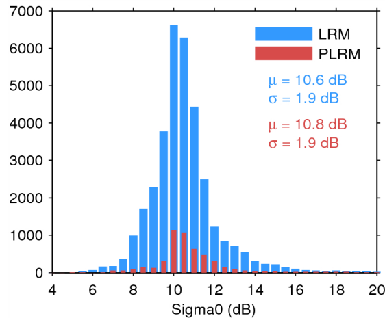
Figure 25. Histogram of flag-valid sigma0 over oceans and lakes for LRM (blue) and PLRM (red) for 31/05/2014. The mean ( \mu ) and standard deviation ( \sigma ) are also shown. Note that values outside [4 20] dB are excluded from the histogram for the sake of readability but not from the computation of \mu and \sigma .
