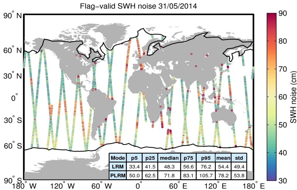
Figure 18. Geographical distribution of flag-valid 20-Hz SWH measurement noise over oceans and lakes for 31/05/2014. The statistical values shown in the table refer to the SWH noise and are calculated separately for LRM and PLRM regions. Measurements taken over polar polygons have been excluded from the computation of the statistical values. The black lines mark the outer limit of the Arctic and Antarctic polar polygons.
