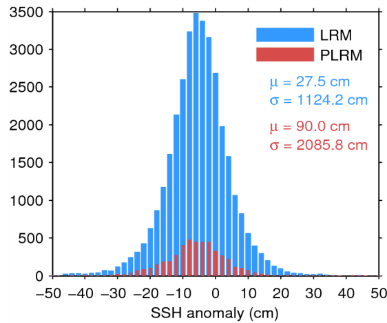
Figure 7. Histogram of flag-valid SSH anomaly over oceans and lakes for LRM (blue) and PLRM (red) for 31/05/2014. The mean ( \mu ) and standard deviation ( \sigma ) are also shown. Note that values outside [-50\ 50] cm are excluded from the histogram for the sake of readability but not from the computation of \mu and \sigma .
