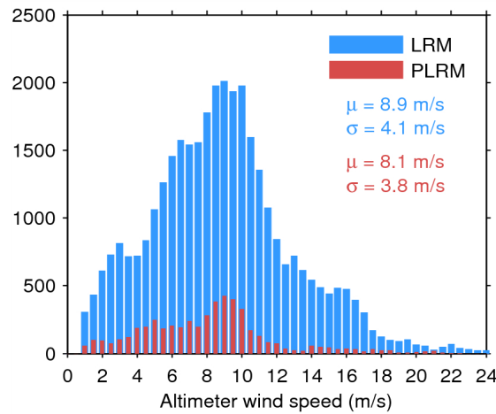
Figure 33. Histogram of flag-valid wind over oceans and lakes for LRM (blue) and PLRM (red) for 31/05/2014. The mean ( \mu ) and standard deviation ( \sigma ) are also shown. Note that values larger than 24 m/s are excluded from the histogram for the sake of readability but not from the computation of \mu and \sigma .
