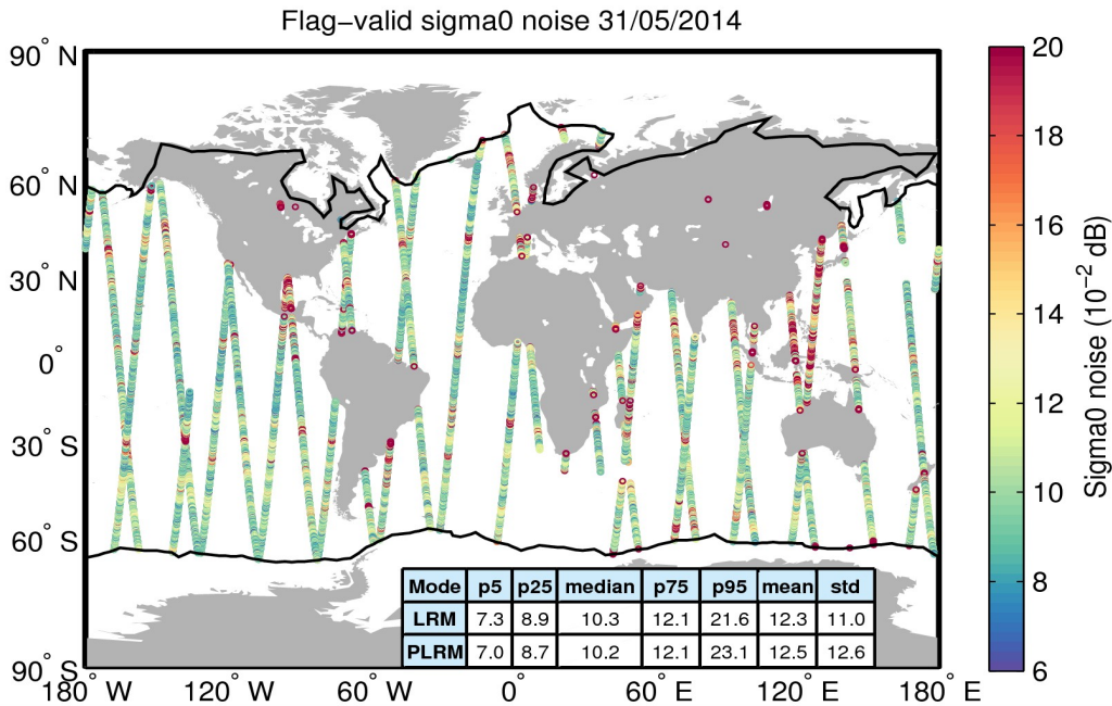
Figure 26. Geographical distribution of flag-valid 20-Hz sigma0 measurement noise over oceans and lakes for 31/05/2014. The statistical values shown in the table refer to the sigma0 noise and are calculated separately for LRM and PLRM regions. Measurements taken over polar polygons have been excluded from the computation of the statistical values. The black lines mark the outer limit of the Arctic and Antarctic polar polygons.
