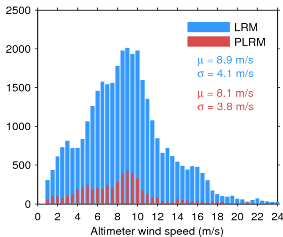
Figure 35. Histogram of science-valid wind over oceans and lakes for LRM (blue) and PLRM (red) for 31/05/2014. The mean ( \mu ) and standard deviation ( \sigma ) are also shown. Note that values larger than 24 m/s are excluded from the histogram for the sake of readability but not from the computation of \mu and \sigma .
