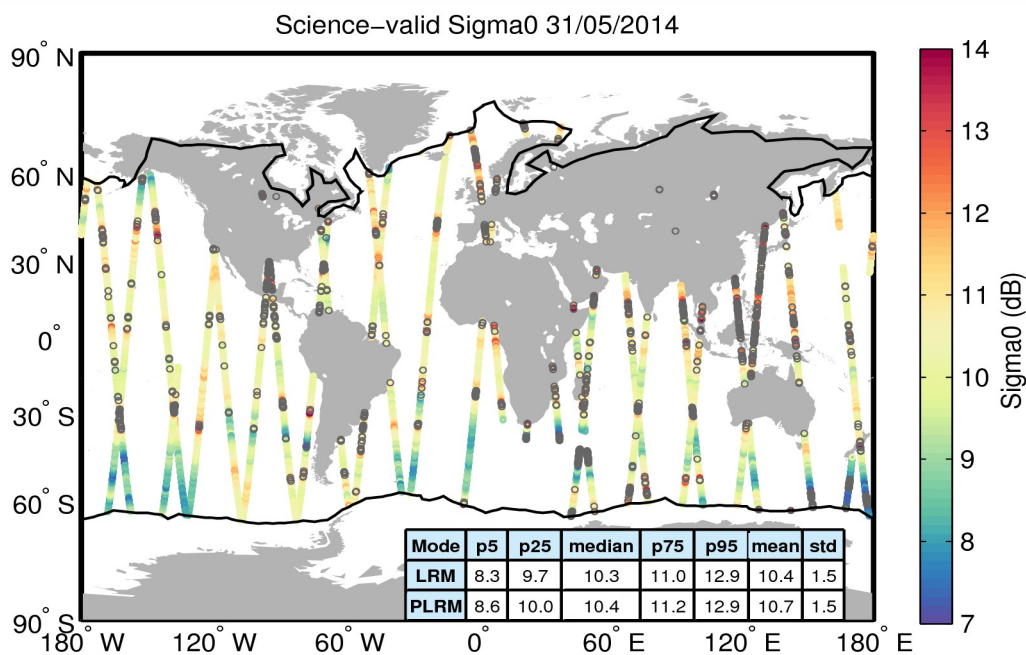
Figure 27. Geographical distribution of science-valid sigma0 data over oceans and lakes for 31/05/2014. The statistical values shown in the table refer to the sigma0 in dB and are calculated separately for LRM and PLRM regions. The black lines mark the outer limit of the Arctic and Antarctic polar polygons. Gray circles denote records that have been rejected based on the editing criteria described in Table 4.
