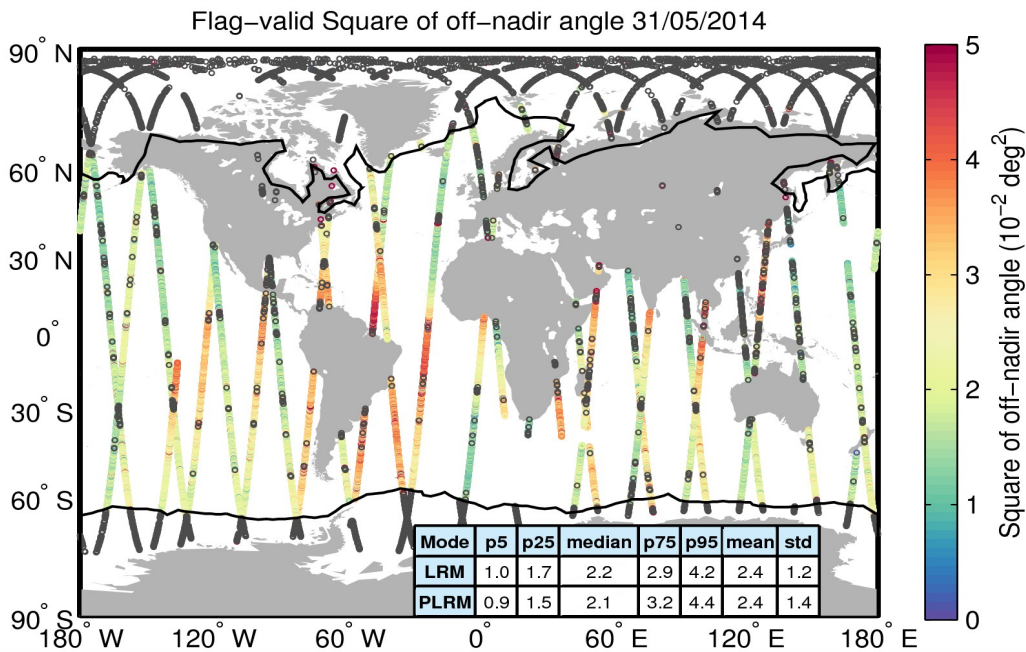
Figure 37. Geographical distribution of flag-valid mispointing data over oceans and lakes for 31/05/2014. The statistical values shown in the table refer to the mispointing in 10^{-2} \text{ deg}^2 and are calculated separately for LRM and PLRM regions. Measurements taken over polar polygons have been excluded from the computation of the statistical values. The black lines mark the outer limit of the Arctic and Antarctic polar polygons. Gray circles denote negative values.
