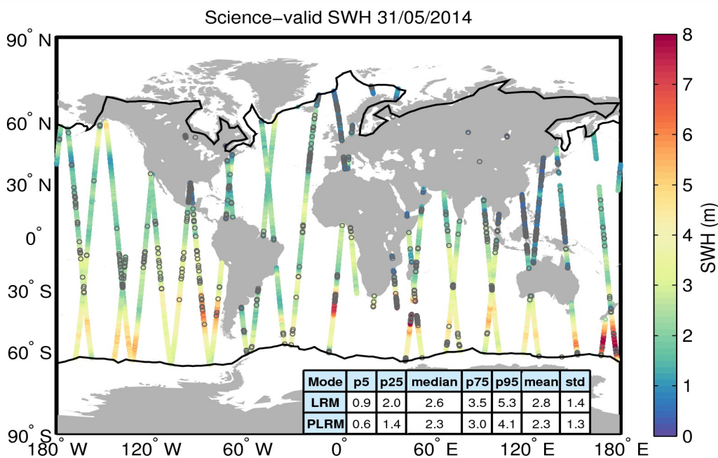
Figure 19. Geographical distribution of science-valid SWH data over oceans and lakes for 31/05/2014. The statistical values shown in the table refer to the SWH in m and are calculated separately for LRM and PLRM regions. The black lines mark the outer limit of the Arctic and Antarctic polar polygons. Gray circles denote records that have been rejected based on the editing criteria described in Table 3.
