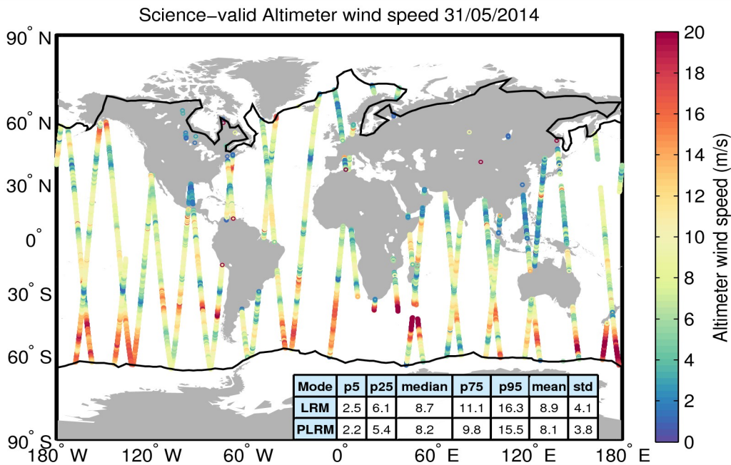
Figure 34. Geographical distribution of science-valid wind data over oceans and lakes for 31/05/2014. The statistical values shown in the table refer to the wind in m/s and are calculated separately for LRM and PLRM regions. The black lines mark the outer limit of the Arctic and Antarctic polar polygons. Gray circles denote records that have been rejected based on the editing criteria described in Table 5.
