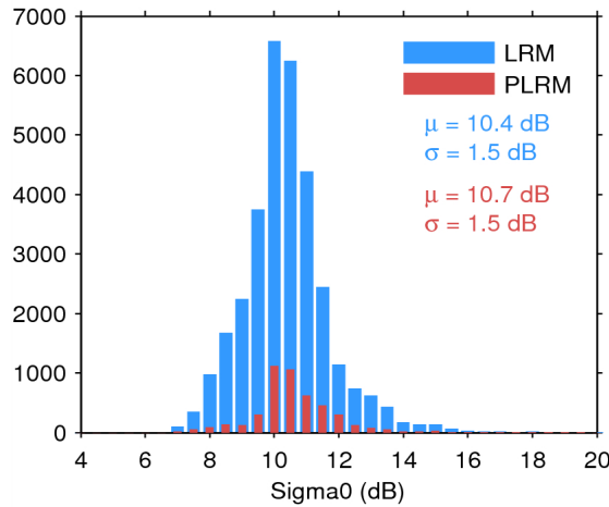
Figure 28. Histogram of science-valid sigma0 over oceans and lakes for LRM (blue) and PLRM (red) for 31/05/2014. The mean ( \mu ) and standard deviation ( \sigma ) are also shown. Note that values outside [4 20] dB are excluded from the histogram for the sake of readability but not from the computation of \mu and \sigma .
