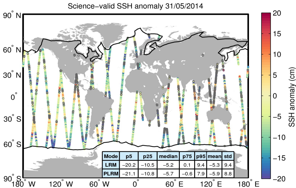
Figure 10. Geographical distribution of science-valid SSH anomaly data over oceans and lakes for 31/05/2014. The statistical values shown in the table refer to the SSH anomaly in cm and are calculated separately for LRM and PLRM regions. The black lines mark the outer limit of the Arctic and Antarctic polar polygons. Gray circles denote records that have been rejected based on the editing criteria described in Table 2.
