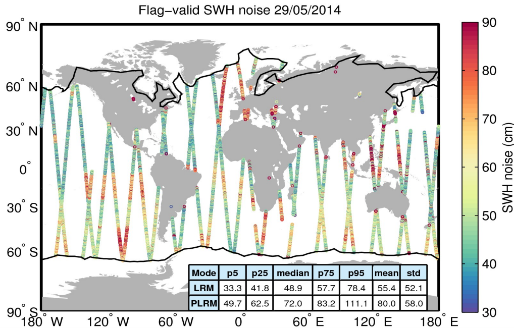
Figure 18. Geographical distribution of flag-valid 20-Hz SWH measurement noise over oceans and lakes for 29/05/2014. The statistical values shown in the table refer to the SWH noise and are calculated separately for LRM and PLRM regions. Measurements taken over polar polygons have been excluded from the computation of the statistical values. The black lines mark the outer limit of the Arctic and Antarctic polar polygons.
