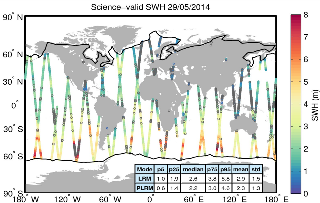
Figure 19. Geographical distribution of science-valid SWH data over oceans and lakes for 29/05/2014. The statistical values shown in the table refer to the SWH in m and are calculated separately for LRM and PLRM regions. The black lines mark the outer limit of the Arctic and Antarctic polar polygons. Gray circles denote records that have been rejected based on the editing criteria described in Table 3.
