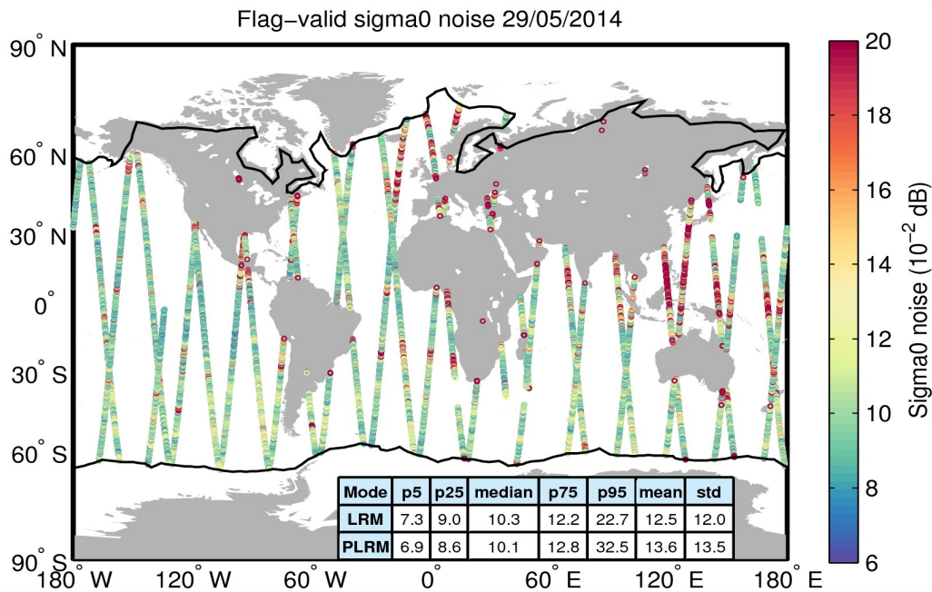
Figure 26. Geographical distribution of flag-valid 20-Hz sigma0 measurement noise over oceans and lakes for 29/05/2014. The statistical values shown in the table refer to the sigma0 noise and are calculated separately for LRM and PLRM regions. Measurements taken over polar polygons have been excluded from the computation of the statistical values. The black lines mark the outer limit of the Arctic and Antarctic polar polygons.
