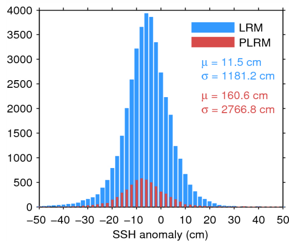
Figure 7. Histogram of flag-valid SSH anomaly over oceans and lakes for LRM (blue) and PLRM (red) for 29/05/2014. The mean ( \mu ) and standard deviation ( \sigma ) are also shown. Note that values outside [-50\ 50] cm are excluded from the histogram for the sake of readability but not from the computation of \mu and \sigma .
