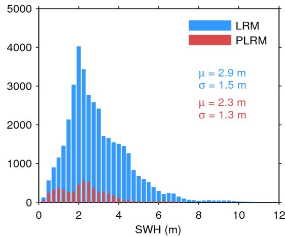
Figure 20. Histogram of science-valid SWH over oceans and lakes for LRM (blue) and PLRM (red) for 29/05/2014. The mean ( \mu ) and standard deviation ( \sigma ) are also shown. Note that values larger than 12 m are excluded from the histogram for the sake of readability but not from the computation of \mu and \sigma .
