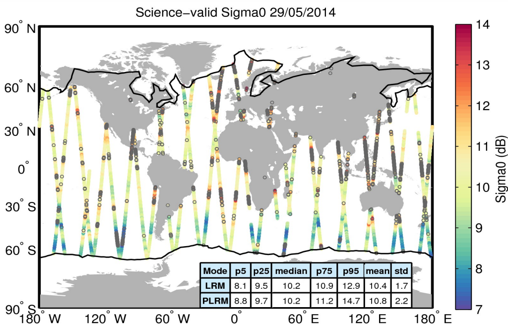
Figure 27. Geographical distribution of science-valid sigma0 data over oceans and lakes for 29/05/2014. The statistical values shown in the table refer to the sigma0 in dB and are calculated separately for LRM and PLRM regions. The black lines mark the outer limit of the Arctic and Antarctic polar polygons. Gray circles denote records that have been rejected based on the editing criteria described in Table 4.
