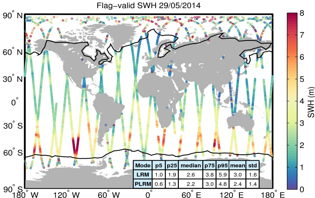
Figure 15. Geographical distribution of flag-valid SWH data over oceans and lakes for 29/05/2014. The statistical values shown in the table refer to the SWH in m and are calculated separately for LRM and PLRM regions. Measurements taken over polar polygons have been excluded from the computation of the statistical values. The black lines mark the outer limit of the Arctic and Antarctic polar polygons.
