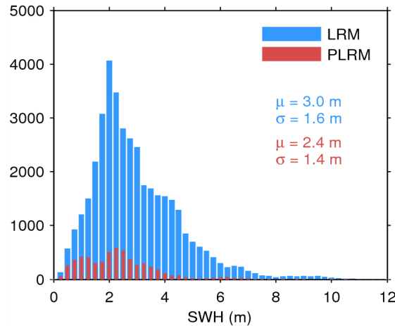
Figure 17. Histogram of flag-valid SWH over oceans and lakes for LRM (blue) and PLRM (red) for 29/05/2014. The mean ( \mu ) and standard deviation ( \sigma ) are also shown. Note that values larger than 12 m are excluded from the histogram for the sake of readability but not from the computation of \mu and \sigma .
