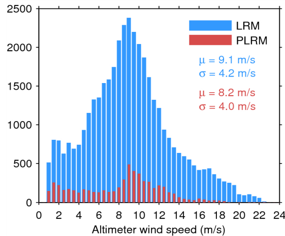
Figure 33. Histogram of flag-valid wind over oceans and lakes for LRM (blue) and PLRM (red) for 29/05/2014. The mean ( \mu ) and standard deviation ( \sigma ) are also shown. Note that values larger than 24 m/s are excluded from the histogram for the sake of readability but not from the computation of \mu and \sigma .
