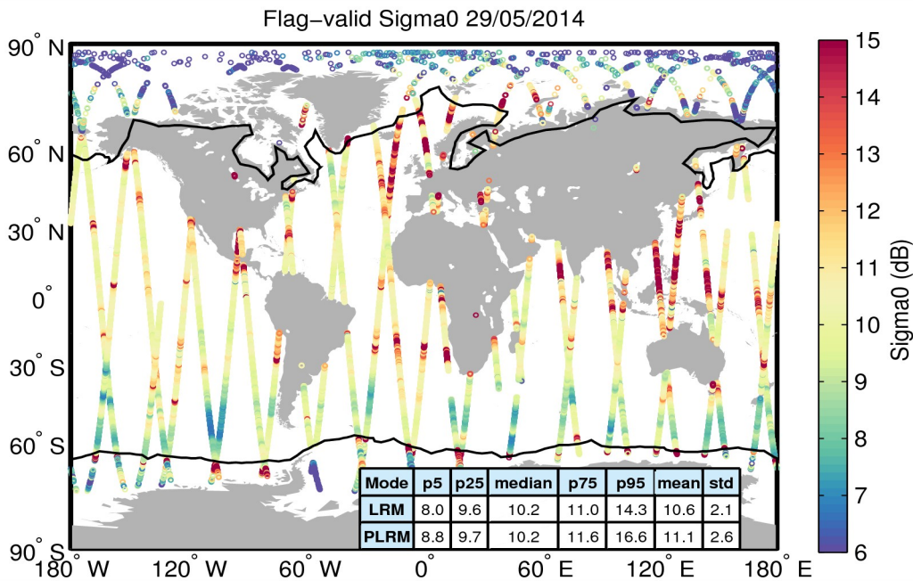
Figure 23. Geographical distribution of flag-valid sigma0 data over oceans and lakes for 29/05/2014. The statistical values shown in the table refer to the sigma0 in dB and are calculated separately for LRM and PLRM regions. Measurements taken over polar polygons have been excluded from the computation of the statistical values. The black lines mark the outer limit of the Arctic and Antarctic polar polygons.
