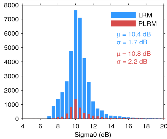
Figure 28. Histogram of science-valid sigma0 over oceans and lakes for LRM (blue) and PLRM (red) for 29/05/2014. The mean ( \mu ) and standard deviation ( \sigma ) are also shown. Note that values outside [4 20] dB are excluded from the histogram for the sake of readability but not from the computation of \mu and \sigma .
