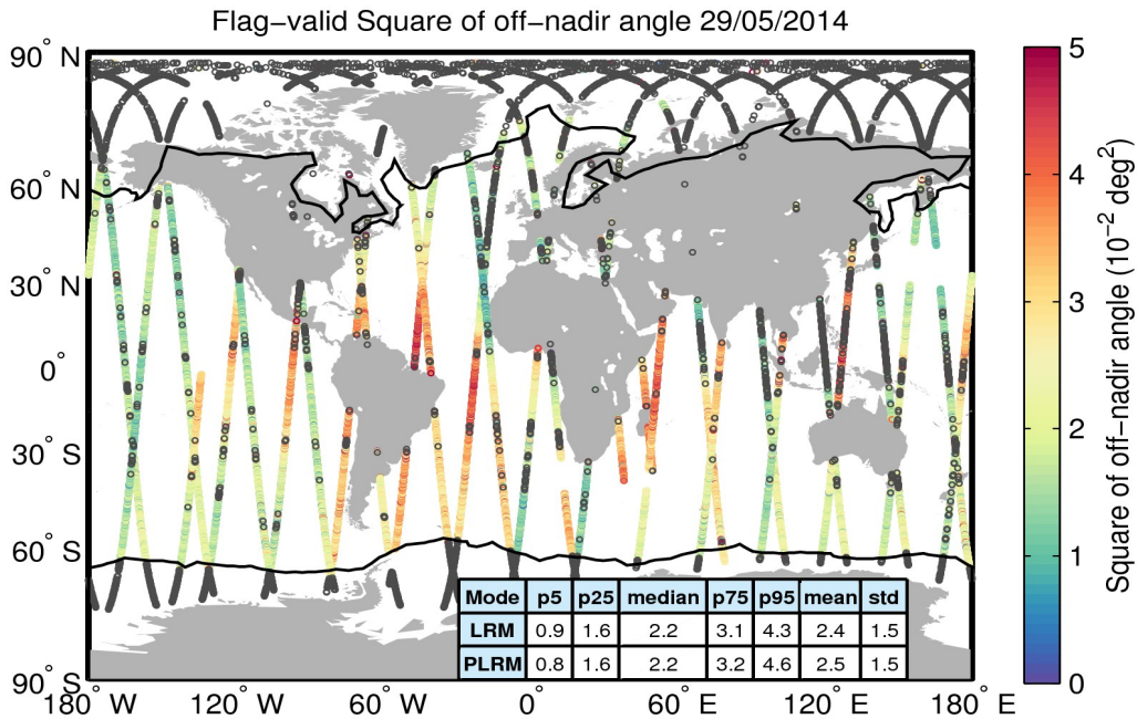
Figure 37. Geographical distribution of flag-valid mispointing data over oceans and lakes for 29/05/2014. The statistical values shown in the table refer to the mispointing in 10^{-2} \text{ deg}^2 and are calculated separately for LRM and PLRM regions. Measurements taken over polar polygons have been excluded from the computation of the statistical values. The black lines mark the outer limit of the Arctic and Antarctic polar polygons. Gray circles denote negative values.
