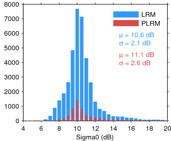
Figure 25. Histogram of flag-valid sigma0 over oceans and lakes for LRM (blue) and PLRM (red) for 29/05/2014. The mean ( \mu ) and standard deviation ( \sigma ) are also shown. Note that values outside [4 20] dB are excluded from the histogram for the sake of readability but not from the computation of \mu and \sigma .
