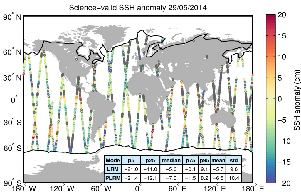
Figure 10. Geographical distribution of science-valid SSH anomaly data over oceans and lakes for 29/05/2014. The statistical values shown in the table refer to the SSH anomaly in cm and are calculated separately for LRM and PLRM regions. The black lines mark the outer limit of the Arctic and Antarctic polar polygons. Gray circles denote records that have been rejected based on the editing criteria described in Table 2.
