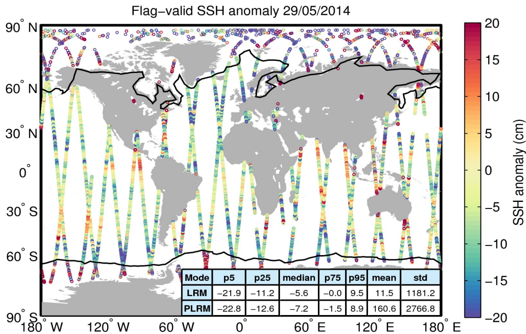
Figure 5. Geographical distribution of flag-valid 1-Hz SSH anomaly data over oceans and lakes for 29/05/2014. The statistical values shown in the table refer to the SSH anomaly in cm and are calculated separately for LRM and PLRM regions. Measurements taken over polar polygons have been excluded from the computation of the statistical values. The black lines mark the outer limit of the Arctic and Antarctic polar polygons.
