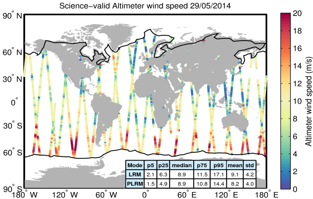
Figure 34. Geographical distribution of science-valid wind data over oceans and lakes for 29/05/2014. The statistical values shown in the table refer to the wind in m/s and are calculated separately for LRM and PLRM regions. The black lines mark the outer limit of the Arctic and Antarctic polar polygons. Gray circles denote records that have been rejected based on the editing criteria described in Table 5.
