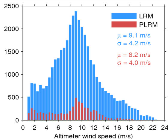
Figure 35. Histogram of science-valid wind over oceans and lakes for LRM (blue) and PLRM (red) for 29/05/2014. The mean ( \mu ) and standard deviation ( \sigma ) are also shown. Note that values larger than 24 m/s are excluded from the histogram for the sake of readability but not from the computation of \mu and \sigma .
