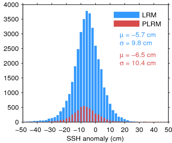
Figure 11. Histogram of science-valid SSH anomaly over oceans and lakes for LRM (blue) and PLRM (red) for 29/05/2014. The mean ( \mu ) and standard deviation ( \sigma ) are also shown. Note that values outside [-50 50] cm are excluded from the histogram for the sake of readability but not from the computation of \mu and \sigma .
