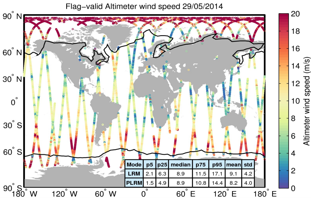
Figure 31. Geographical distribution of flag-valid wind data over oceans and lakes for 29/05/2014. The statistical values shown in the table refer to the wind in m/s and are calculated separately for LRM and PLRM regions. Measurements taken over polar polygons have been excluded from the computation of the statistical values. The black lines mark the outer limit of the Arctic and Antarctic polar polygons.
