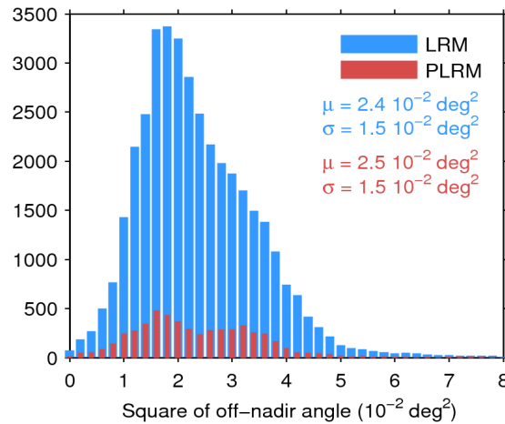
Figure 39. Histogram of flag-valid mispointing over oceans and lakes for LRM (blue) and PLRM (red) for 29/05/2014. Only positive values have been considered. The mean ( \mu ) and standard deviation ( \sigma ) are also shown. Note that values 8 \cdot 10^{-2} \text{ deg}^2 are excluded from the histogram for the sake of readability but not from the computation of \mu and \sigma .
