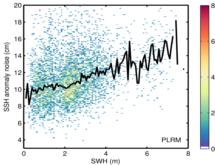
Figure 9. 2D histogram showing flag-valid SSH anomaly noise as a function of SWH for LRM (top) and PLRM (bottom) for 29/05/2014. The black line denotes the median SSH anomaly as a function of SWH.
