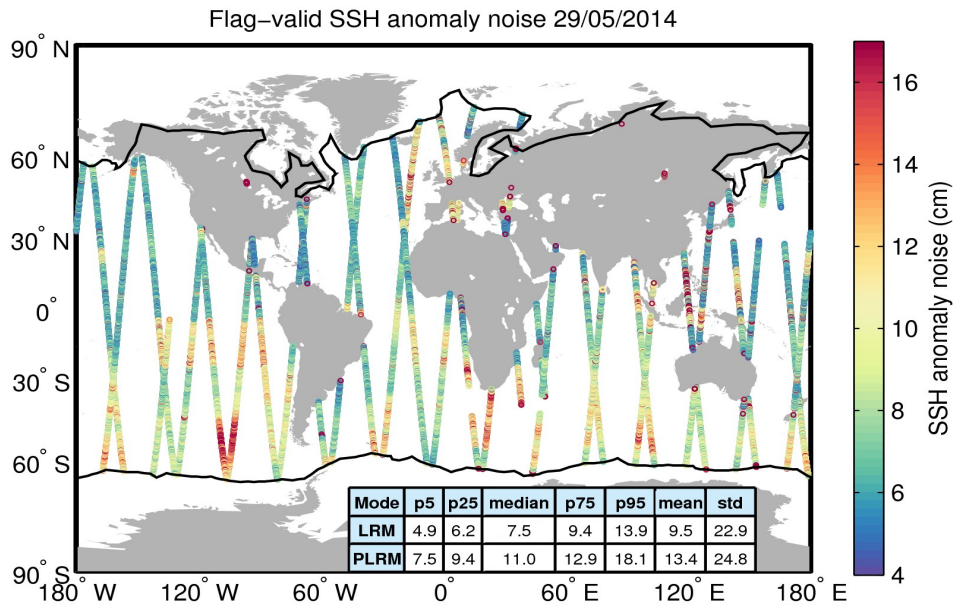
Figure 8. Geographical distribution of flag-valid 20-Hz SSH anomaly measurement noise over oceans and lakes for 29/05/2014. The statistical values shown in the table refer to the SSH anomaly noise and are calculated separately for LRM and PLRM regions. Measurements taken over polar polygons have been excluded from the computation of the statistical values. The black lines mark the outer limit of the Arctic and Antarctic polar polygons.
