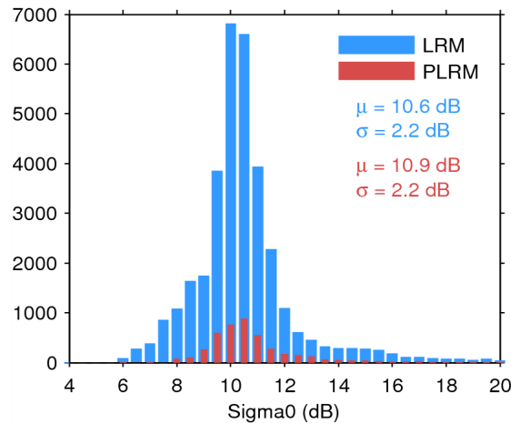
Figure 25. Histogram of flag-valid sigma0 over oceans and lakes for LRM (blue) and PLRM (red) for 28/05/2014. The mean ( \mu ) and standard deviation ( \sigma ) are also shown. Note that values outside [4 20] dB are excluded from the histogram for the sake of readability but not from the computation of \mu and \sigma .
