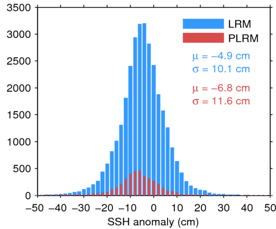
Figure 11. Histogram of science-valid SSH anomaly over oceans and lakes for LRM (blue) and PLRM (red) for 28/05/2014. The mean ( \mu ) and standard deviation ( \sigma ) are also shown. Note that values outside [-50 50] cm are excluded from the histogram for the sake of readability but not from the computation of \mu and \sigma .
