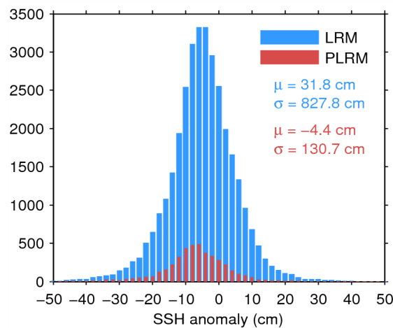
Figure 7. Histogram of flag-valid SSH anomaly over oceans and lakes for LRM (blue) and PLRM (red) for 28/05/2014. The mean ( \mu ) and standard deviation ( \sigma ) are also shown. Note that values outside [-50\ 50] cm are excluded from the histogram for the sake of readability but not from the computation of \mu and \sigma .
