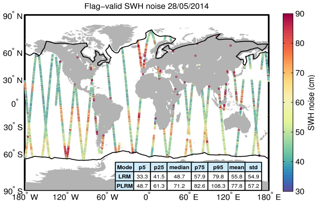
Figure 18. Geographical distribution of flag-valid 20-Hz SWH measurement noise over oceans and lakes for 28/05/2014. The statistical values shown in the table refer to the SWH noise and are calculated separately for LRM and PLRM regions. Measurements taken over polar polygons have been excluded from the computation of the statistical values. The black lines mark the outer limit of the Arctic and Antarctic polar polygons.
