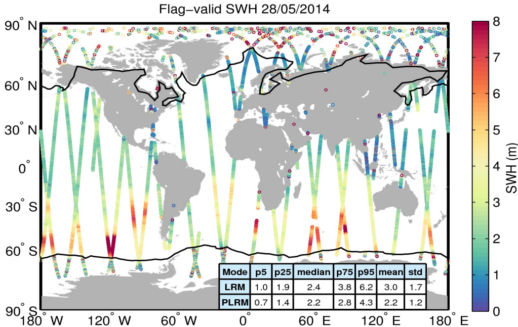
Figure 15. Geographical distribution of flag-valid SWH data over oceans and lakes for 28/05/2014. The statistical values shown in the table refer to the SWH in m and are calculated separately for LRM and PLRM regions. Measurements taken over polar polygons have been excluded from the computation of the statistical values. The black lines mark the outer limit of the Arctic and Antarctic polar polygons.
