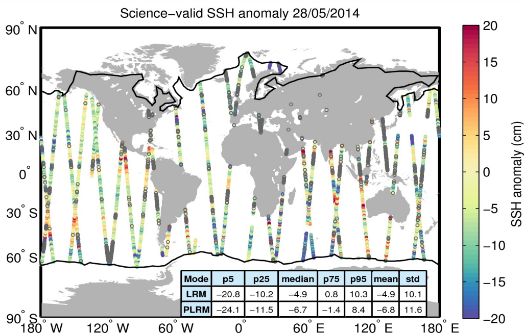
Figure 10. Geographical distribution of science-valid SSH anomaly data over oceans and lakes for 28/05/2014. The statistical values shown in the table refer to the SSH anomaly in cm and are calculated separately for LRM and PLRM regions. The black lines mark the outer limit of the Arctic and Antarctic polar polygons. Gray circles denote records that have been rejected based on the editing criteria described in Table 2.
