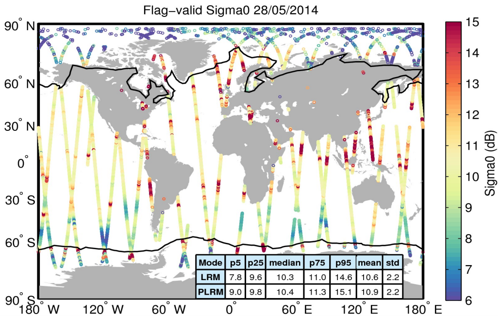
Figure 23. Geographical distribution of flag-valid sigma0 data over oceans and lakes for 28/05/2014. The statistical values shown in the table refer to the sigma0 in dB and are calculated separately for LRM and PLRM regions. Measurements taken over polar polygons have been excluded from the computation of the statistical values. The black lines mark the outer limit of the Arctic and Antarctic polar polygons.
