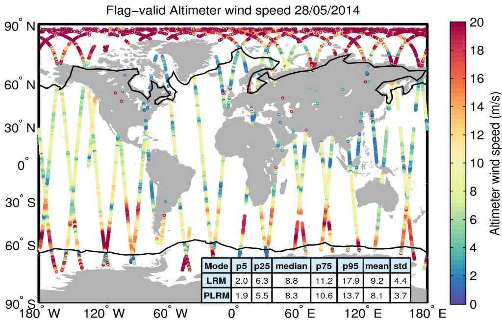
Figure 31. Geographical distribution of flag-valid wind data over oceans and lakes for 28/05/2014. The statistical values shown in the table refer to the wind in m/s and are calculated separately for LRM and PLRM regions. Measurements taken over polar polygons have been excluded from the computation of the statistical values. The black lines mark the outer limit of the Arctic and Antarctic polar polygons.
