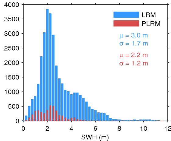
Figure 17. Histogram of flag-valid SWH over oceans and lakes for LRM (blue) and PLRM (red) for 28/05/2014. The mean ( \mu ) and standard deviation ( \sigma ) are also shown. Note that values larger than 12 m are excluded from the histogram for the sake of readability but not from the computation of \mu and \sigma .
