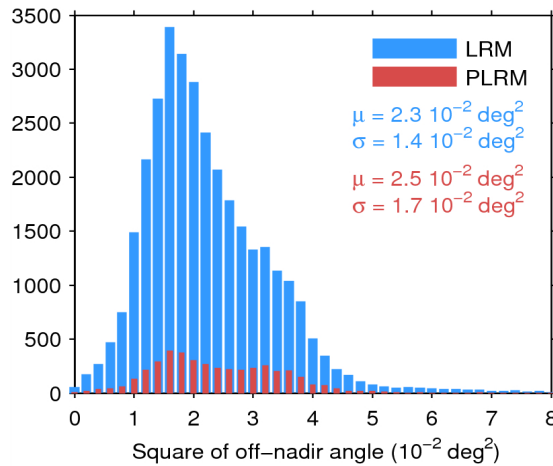
Figure 39. Histogram of flag-valid mispointing over oceans and lakes for LRM (blue) and PLRM (red) for 28/05/2014. Only positive values have been considered. The mean ( \mu ) and standard deviation ( \sigma ) are also shown. Note that values 8 \cdot 10^{-2} \text{ deg}^2 are excluded from the histogram for the sake of readability but not from the computation of \mu and \sigma .
