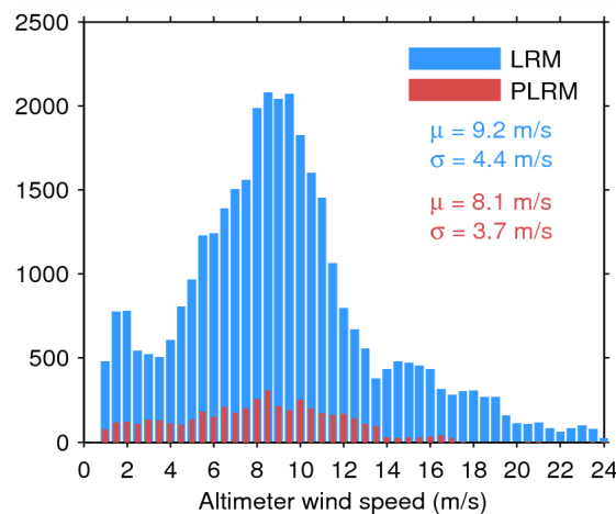
Figure 35. Histogram of science-valid wind over oceans and lakes for LRM (blue) and PLRM (red) for 28/05/2014. The mean ( \mu ) and standard deviation ( \sigma ) are also shown. Note that values larger than 24 m/s are excluded from the histogram for the sake of readability but not from the computation of \mu and \sigma .
