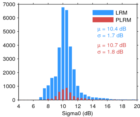
Figure 28. Histogram of science-valid sigma0 over oceans and lakes for LRM (blue) and PLRM (red) for 28/05/2014. The mean ( \mu ) and standard deviation ( \sigma ) are also shown. Note that values outside [4 20] dB are excluded from the histogram for the sake of readability but not from the computation of \mu and \sigma .
