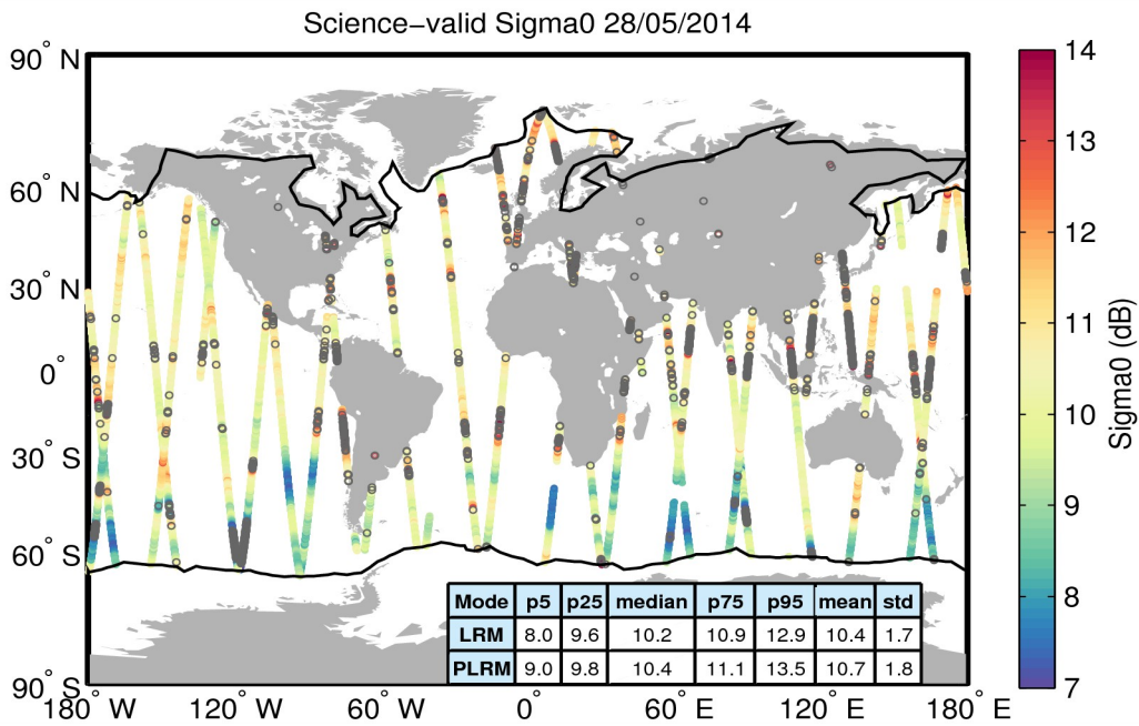
Figure 27. Geographical distribution of science-valid sigma0 data over oceans and lakes for 28/05/2014. The statistical values shown in the table refer to the sigma0 in dB and are calculated separately for LRM and PLRM regions. The black lines mark the outer limit of the Arctic and Antarctic polar polygons. Gray circles denote records that have been rejected based on the editing criteria described in Table 4.
