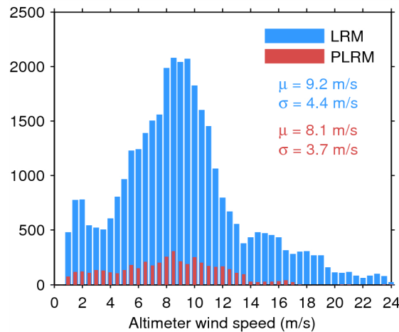
Figure 33. Histogram of flag-valid wind over oceans and lakes for LRM (blue) and PLRM (red) for 28/05/2014. The mean ( \mu ) and standard deviation ( \sigma ) are also shown. Note that values larger than 24 m/s are excluded from the histogram for the sake of readability but not from the computation of \mu and \sigma .
