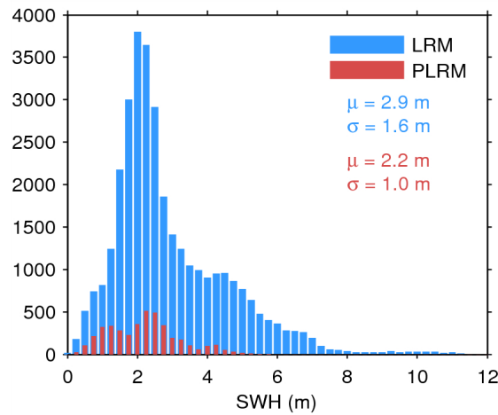
Figure 20. Histogram of science-valid SWH over oceans and lakes for LRM (blue) and PLRM (red) for 28/05/2014. The mean ( \mu ) and standard deviation ( \sigma ) are also shown. Note that values larger than 12 m are excluded from the histogram for the sake of readability but not from the computation of \mu and \sigma .
