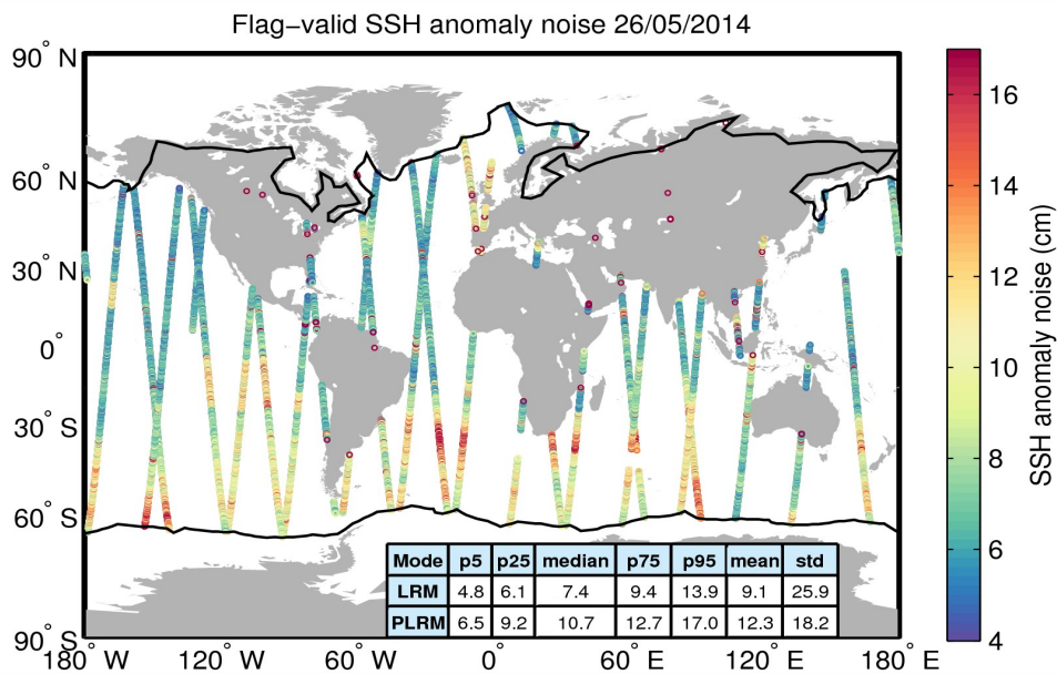
Figure 8. Geographical distribution of flag-valid 20-Hz SSH anomaly measurement noise over oceans and lakes for 26/05/2014. The statistical values shown in the table refer to the SSH anomaly noise and are calculated separately for LRM and PLRM regions. Measurements taken over polar polygons have been excluded from the computation of the statistical values. The black lines mark the outer limit of the Arctic and Antarctic polar polygons.
