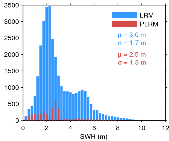
Figure 20. Histogram of science-valid SWH over oceans and lakes for LRM (blue) and PLRM (red) for 26/05/2014. The mean ( \mu ) and standard deviation ( \sigma ) are also shown. Note that values larger than 12 m are excluded from the histogram for the sake of readability but not from the computation of \mu and \sigma .
