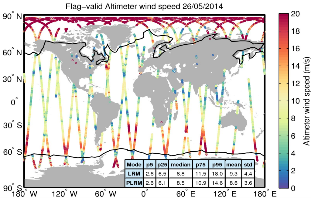
Figure 31. Geographical distribution of flag-valid wind data over oceans and lakes for 26/05/2014. The statistical values shown in the table refer to the wind in m/s and are calculated separately for LRM and PLRM regions. Measurements taken over polar polygons have been excluded from the computation of the statistical values. The black lines mark the outer limit of the Arctic and Antarctic polar polygons.
