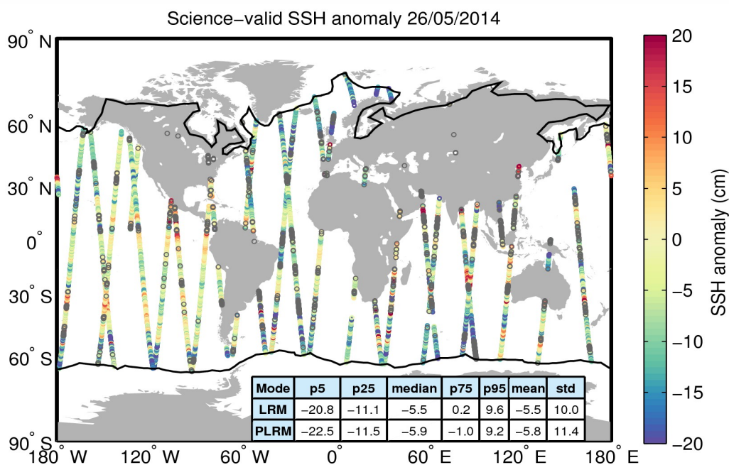
Figure 10. Geographical distribution of science-valid SSH anomaly data over oceans and lakes for 26/05/2014. The statistical values shown in the table refer to the SSH anomaly in cm and are calculated separately for LRM and PLRM regions. The black lines mark the outer limit of the Arctic and Antarctic polar polygons. Gray circles denote records that have been rejected based on the editing criteria described in Table 2.
