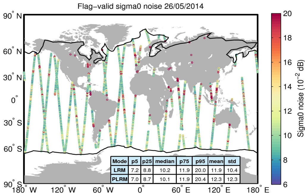
Figure 26. Geographical distribution of flag-valid 20-Hz sigma0 measurement noise over oceans and lakes for 26/05/2014. The statistical values shown in the table refer to the sigma0 noise and are calculated separately for LRM and PLRM regions. Measurements taken over polar polygons have been excluded from the computation of the statistical values. The black lines mark the outer limit of the Arctic and Antarctic polar polygons.
