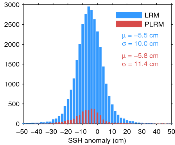
Figure 11. Histogram of science-valid SSH anomaly over oceans and lakes for LRM (blue) and PLRM (red) for 26/05/2014. The mean ( \mu ) and standard deviation ( \sigma ) are also shown. Note that values outside [-50 50] cm are excluded from the histogram for the sake of readability but not from the computation of \mu and \sigma .
