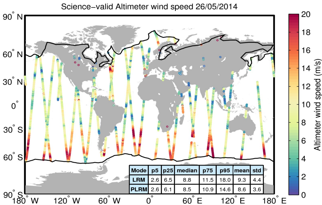
Figure 34. Geographical distribution of science-valid wind data over oceans and lakes for 26/05/2014. The statistical values shown in the table refer to the wind in m/s and are calculated separately for LRM and PLRM regions. The black lines mark the outer limit of the Arctic and Antarctic polar polygons. Gray circles denote records that have been rejected based on the editing criteria described in Table 5.
