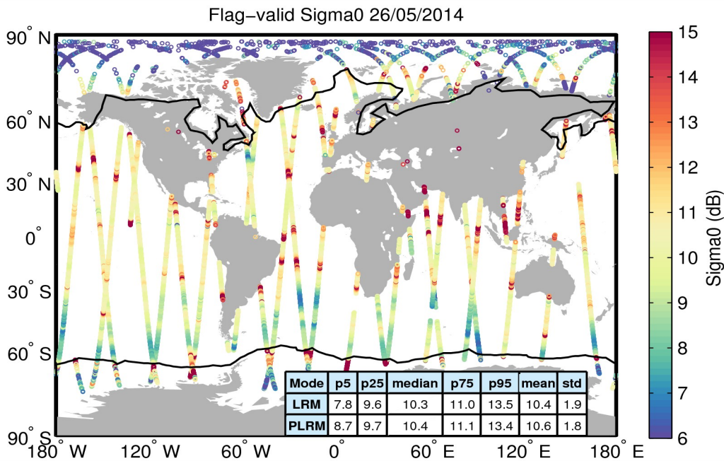
Figure 23. Geographical distribution of flag-valid sigma0 data over oceans and lakes for 26/05/2014. The statistical values shown in the table refer to the sigma0 in dB and are calculated separately for LRM and PLRM regions. Measurements taken over polar polygons have been excluded from the computation of the statistical values. The black lines mark the outer limit of the Arctic and Antarctic polar polygons.
