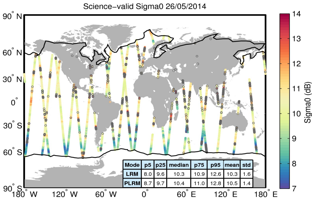
Figure 27. Geographical distribution of science-valid sigma0 data over oceans and lakes for 26/05/2014. The statistical values shown in the table refer to the sigma0 in dB and are calculated separately for LRM and PLRM regions. The black lines mark the outer limit of the Arctic and Antarctic polar polygons. Gray circles denote records that have been rejected based on the editing criteria described in Table 4.
