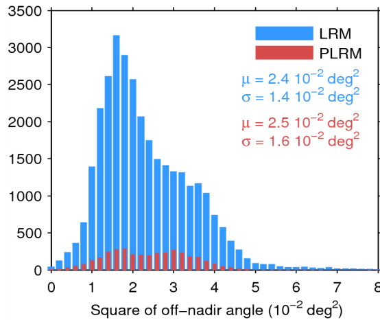
Figure 39. Histogram of flag-valid mispointing over oceans and lakes for LRM (blue) and PLRM (red) for 26/05/2014. Only positive values have been considered. The mean ( \mu ) and standard deviation ( \sigma ) are also shown. Note that values 8 \cdot 10^{-2} \text{ deg}^2 are excluded from the histogram for the sake of readability but not from the computation of \mu and \sigma .
