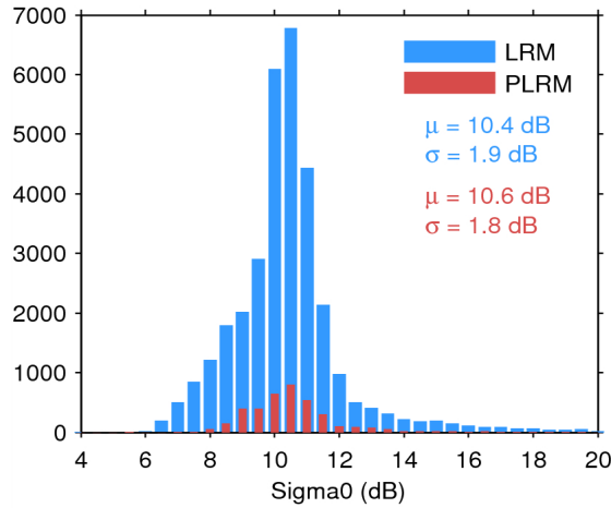
Figure 25. Histogram of flag-valid sigma0 over oceans and lakes for LRM (blue) and PLRM (red) for 26/05/2014. The mean ( \mu ) and standard deviation ( \sigma ) are also shown. Note that values outside [4 20] dB are excluded from the histogram for the sake of readability but not from the computation of \mu and \sigma .
