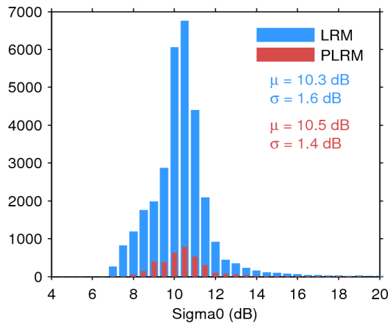
Figure 28. Histogram of science-valid sigma0 over oceans and lakes for LRM (blue) and PLRM (red) for 26/05/2014. The mean ( \mu ) and standard deviation ( \sigma ) are also shown. Note that values outside [4 20] dB are excluded from the histogram for the sake of readability but not from the computation of \mu and \sigma .
