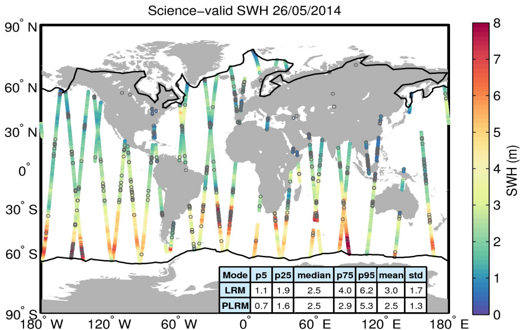
Figure 19. Geographical distribution of science-valid SWH data over oceans and lakes for 26/05/2014. The statistical values shown in the table refer to the SWH in m and are calculated separately for LRM and PLRM regions. The black lines mark the outer limit of the Arctic and Antarctic polar polygons. Gray circles denote records that have been rejected based on the editing criteria described in Table 3.
