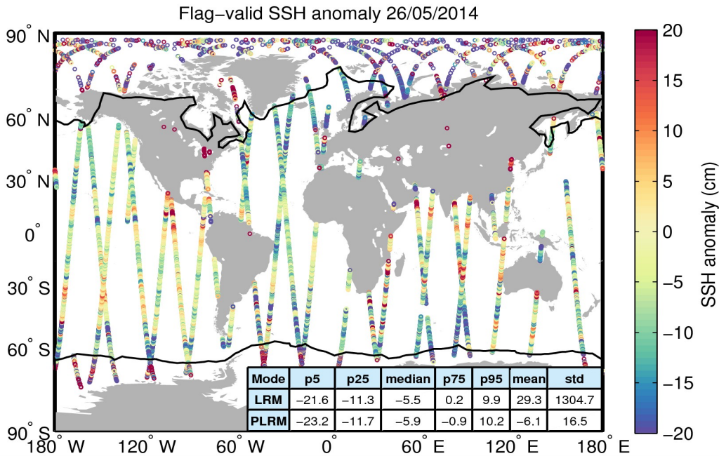
Figure 5. Geographical distribution of flag-valid 1-Hz SSH anomaly data over oceans and lakes for 26/05/2014. The statistical values shown in the table refer to the SSH anomaly in cm and are calculated separately for LRM and PLRM regions. Measurements taken over polar polygons have been excluded from the computation of the statistical values. The black lines mark the outer limit of the Arctic and Antarctic polar polygons.
