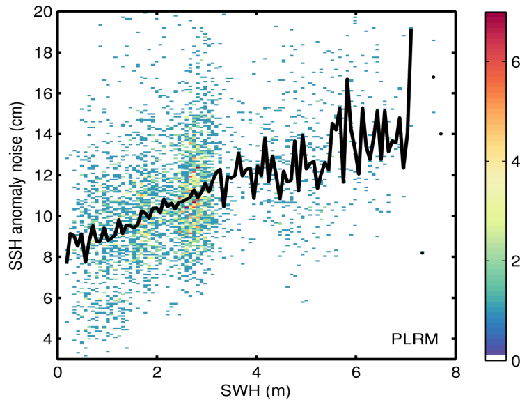
Figure 9. 2D histogram showing flag-valid SSH anomaly noise as a function of SWH for LRM (top) and PLRM (bottom) for 26/05/2014. The black line denotes the median SSH anomaly as a function of SWH.
