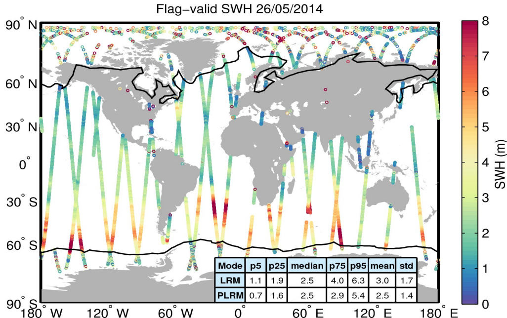
Figure 15. Geographical distribution of flag-valid SWH data over oceans and lakes for 26/05/2014. The statistical values shown in the table refer to the SWH in m and are calculated separately for LRM and PLRM regions. Measurements taken over polar polygons have been excluded from the computation of the statistical values. The black lines mark the outer limit of the Arctic and Antarctic polar polygons.
