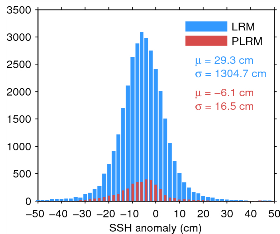
Figure 7. Histogram of flag-valid SSH anomaly over oceans and lakes for LRM (blue) and PLRM (red) for 26/05/2014. The mean ( \mu ) and standard deviation ( \sigma ) are also shown. Note that values outside [-50\ 50] cm are excluded from the histogram for the sake of readability but not from the computation of \mu and \sigma .
