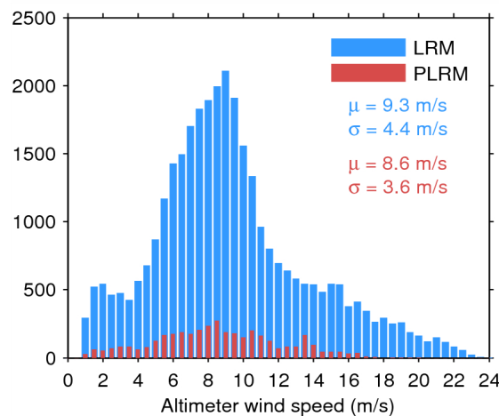
Figure 35. Histogram of science-valid wind over oceans and lakes for LRM (blue) and PLRM (red) for 26/05/2014. The mean ( \mu ) and standard deviation ( \sigma ) are also shown. Note that values larger than 24 m/s are excluded from the histogram for the sake of readability but not from the computation of \mu and \sigma .
