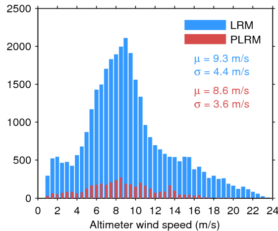
Figure 33. Histogram of flag-valid wind over oceans and lakes for LRM (blue) and PLRM (red) for 26/05/2014. The mean ( \mu ) and standard deviation ( \sigma ) are also shown. Note that values larger than 24 m/s are excluded from the histogram for the sake of readability but not from the computation of \mu and \sigma .
