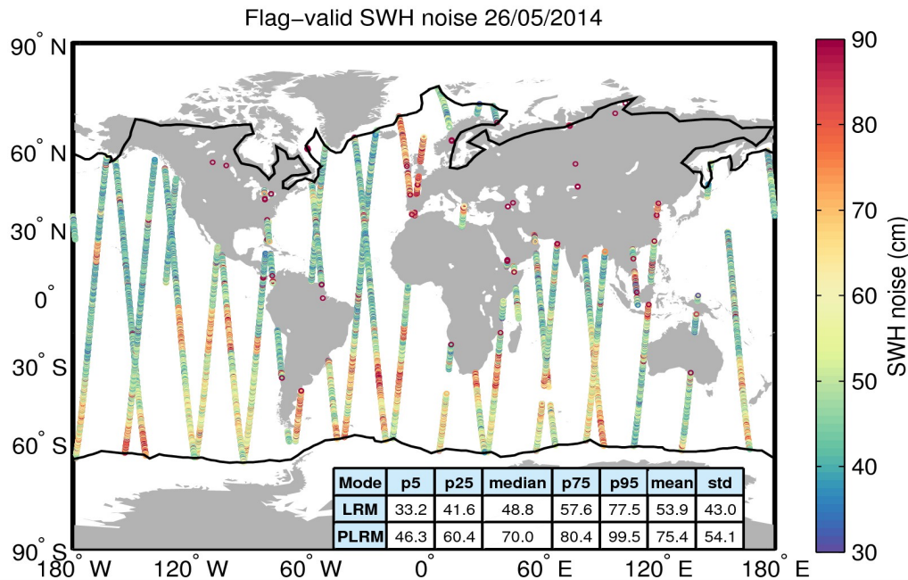
Figure 18. Geographical distribution of flag-valid 20-Hz SWH measurement noise over oceans and lakes for 26/05/2014. The statistical values shown in the table refer to the SWH noise and are calculated separately for LRM and PLRM regions. Measurements taken over polar polygons have been excluded from the computation of the statistical values. The black lines mark the outer limit of the Arctic and Antarctic polar polygons.
