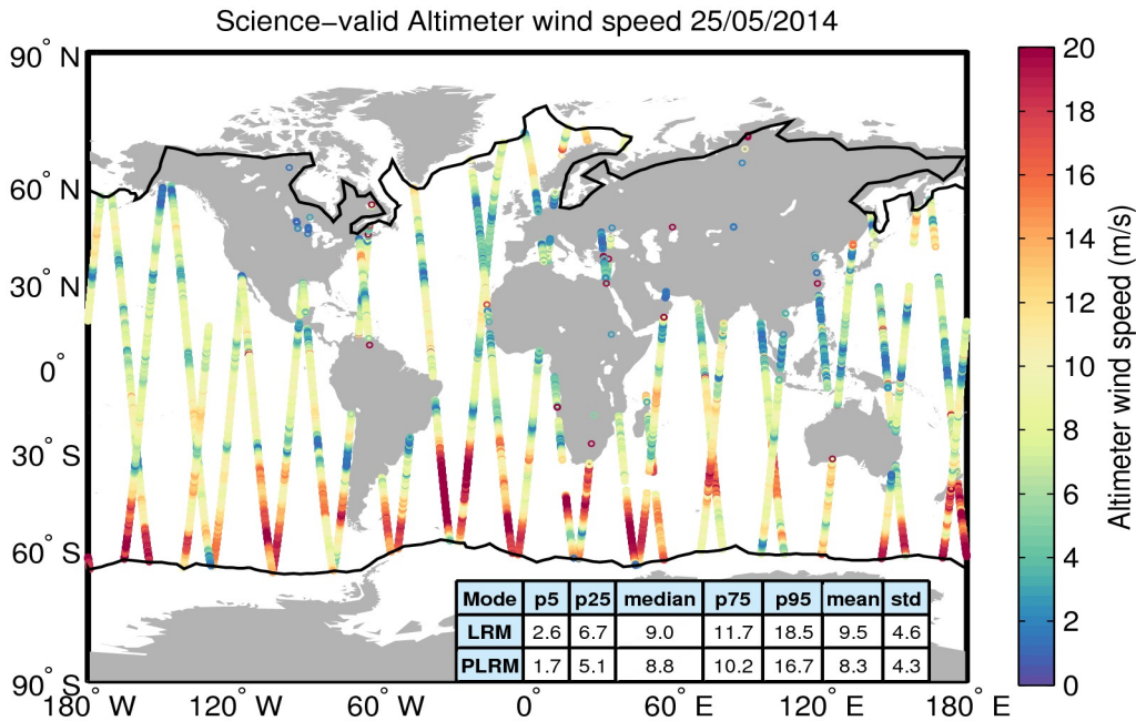
Figure 34. Geographical distribution of science-valid wind data over oceans and lakes for 25/05/2014. The statistical values shown in the table refer to the wind in m/s and are calculated separately for LRM and PLRM regions. The black lines mark the outer limit of the Arctic and Antarctic polar polygons. Gray circles denote records that have been rejected based on the editing criteria described in Table 5.
