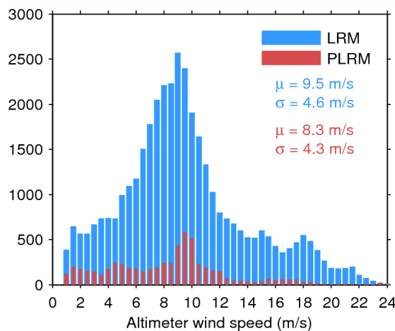
Figure 35. Histogram of science-valid wind over oceans and lakes for LRM (blue) and PLRM (red) for 25/05/2014. The mean ( \mu ) and standard deviation ( \sigma ) are also shown. Note that values larger than 24 m/s are excluded from the histogram for the sake of readability but not from the computation of \mu and \sigma .
