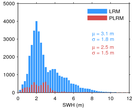
Figure 17. Histogram of flag-valid SWH over oceans and lakes for LRM (blue) and PLRM (red) for 25/05/2014. The mean ( \mu ) and standard deviation ( \sigma ) are also shown. Note that values larger than 12 m are excluded from the histogram for the sake of readability but not from the computation of \mu and \sigma .
