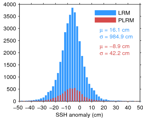
Figure 7. Histogram of flag-valid SSH anomaly over oceans and lakes for LRM (blue) and PLRM (red) for 25/05/2014. The mean ( \mu ) and standard deviation ( \sigma ) are also shown. Note that values outside [-50\ 50] cm are excluded from the histogram for the sake of readability but not from the computation of \mu and \sigma .
