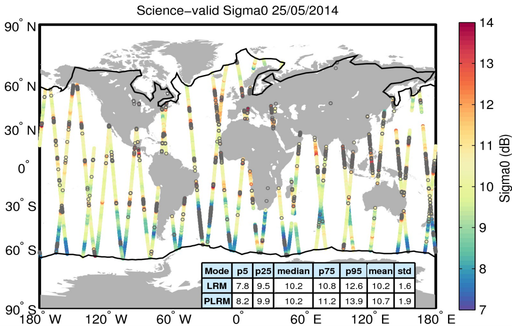
Figure 27. Geographical distribution of science-valid sigma0 data over oceans and lakes for 25/05/2014. The statistical values shown in the table refer to the sigma0 in dB and are calculated separately for LRM and PLRM regions. The black lines mark the outer limit of the Arctic and Antarctic polar polygons. Gray circles denote records that have been rejected based on the editing criteria described in Table 4.
