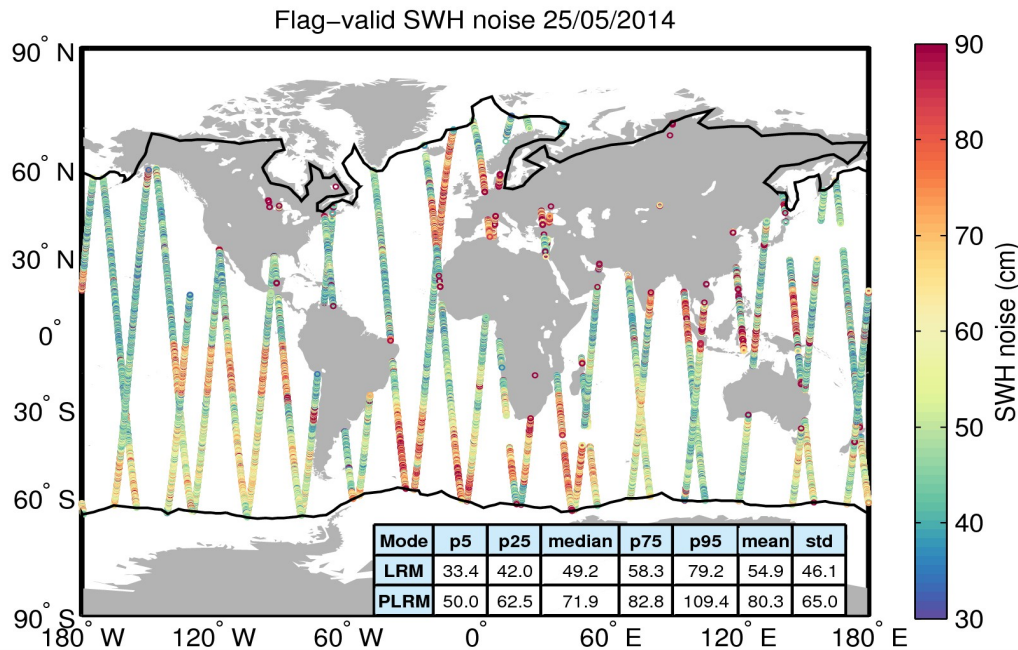
Figure 18. Geographical distribution of flag-valid 20-Hz SWH measurement noise over oceans and lakes for 25/05/2014. The statistical values shown in the table refer to the SWH noise and are calculated separately for LRM and PLRM regions. Measurements taken over polar polygons have been excluded from the computation of the statistical values. The black lines mark the outer limit of the Arctic and Antarctic polar polygons.
