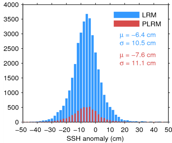
Figure 11. Histogram of science-valid SSH anomaly over oceans and lakes for LRM (blue) and PLRM (red) for 25/05/2014. The mean ( \mu ) and standard deviation ( \sigma ) are also shown. Note that values outside [-50\ 50] cm are excluded from the histogram for the sake of readability but not from the computation of \mu and \sigma .
