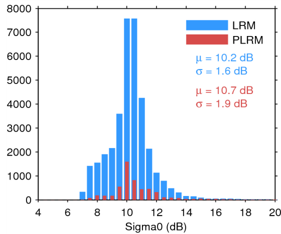
Figure 28. Histogram of science-valid sigma0 over oceans and lakes for LRM (blue) and PLRM (red) for 25/05/2014. The mean ( \mu ) and standard deviation ( \sigma ) are also shown. Note that values outside [4 20] dB are excluded from the histogram for the sake of readability but not from the computation of \mu and \sigma .
