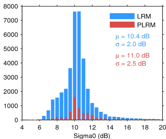
Figure 25. Histogram of flag-valid sigma0 over oceans and lakes for LRM (blue) and PLRM (red) for 25/05/2014. The mean ( \mu ) and standard deviation ( \sigma ) are also shown. Note that values outside [4 20] dB are excluded from the histogram for the sake of readability but not from the computation of \mu and \sigma .
