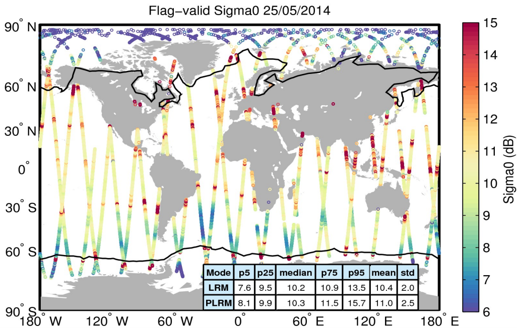
Figure 23. Geographical distribution of flag-valid sigma0 data over oceans and lakes for 25/05/2014. The statistical values shown in the table refer to the sigma0 in dB and are calculated separately for LRM and PLRM regions. Measurements taken over polar polygons have been excluded from the computation of the statistical values. The black lines mark the outer limit of the Arctic and Antarctic polar polygons.
