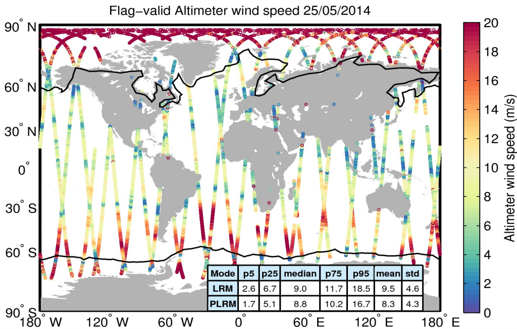
Figure 31. Geographical distribution of flag-valid wind data over oceans and lakes for 25/05/2014. The statistical values shown in the table refer to the wind in m/s and are calculated separately for LRM and PLRM regions. Measurements taken over polar polygons have been excluded from the computation of the statistical values. The black lines mark the outer limit of the Arctic and Antarctic polar polygons.
