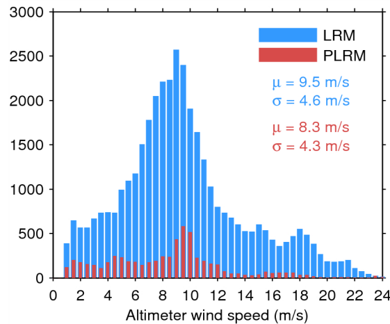
Figure 33. Histogram of flag-valid wind over oceans and lakes for LRM (blue) and PLRM (red) for 25/05/2014. The mean ( \mu ) and standard deviation ( \sigma ) are also shown. Note that values larger than 24 m/s are excluded from the histogram for the sake of readability but not from the computation of \mu and \sigma .
