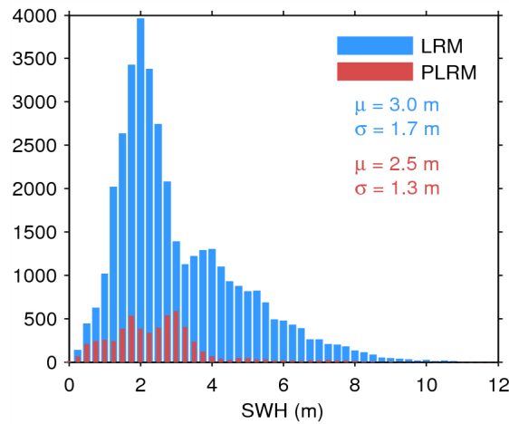
Figure 20. Histogram of science-valid SWH over oceans and lakes for LRM (blue) and PLRM (red) for 25/05/2014. The mean ( \mu ) and standard deviation ( \sigma ) are also shown. Note that values larger than 12 m are excluded from the histogram for the sake of readability but not from the computation of \mu and \sigma .
