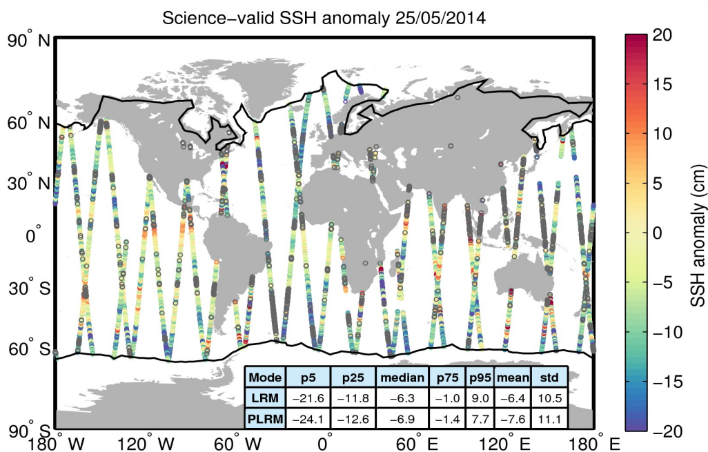
Figure 10. Geographical distribution of science-valid SSH anomaly data over oceans and lakes for 25/05/2014. The statistical values shown in the table refer to the SSH anomaly in cm and are calculated separately for LRM and PLRM regions. The black lines mark the outer limit of the Arctic and Antarctic polar polygons. Gray circles denote records that have been rejected based on the editing criteria described in Table 2.
