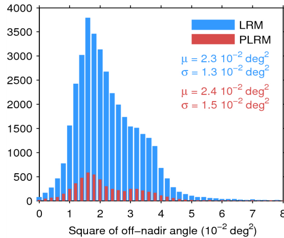
Figure 39. Histogram of flag-valid mispointing over oceans and lakes for LRM (blue) and PLRM (red) for 25/05/2014. Only positive values have been considered. The mean ( \mu ) and standard deviation ( \sigma ) are also shown. Note that values 8 \cdot 10^{-2} \text{ deg}^2 are excluded from the histogram for the sake of readability but not from the computation of \mu and \sigma .
