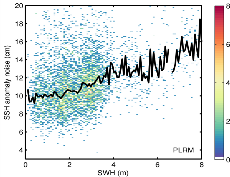
Figure 9. 2D histogram showing flag-valid SSH anomaly noise as a function of SWH for LRM (top) and PLRM (bottom) for 25/05/2014. The black line denotes the median SSH anomaly as a function of SWH.
