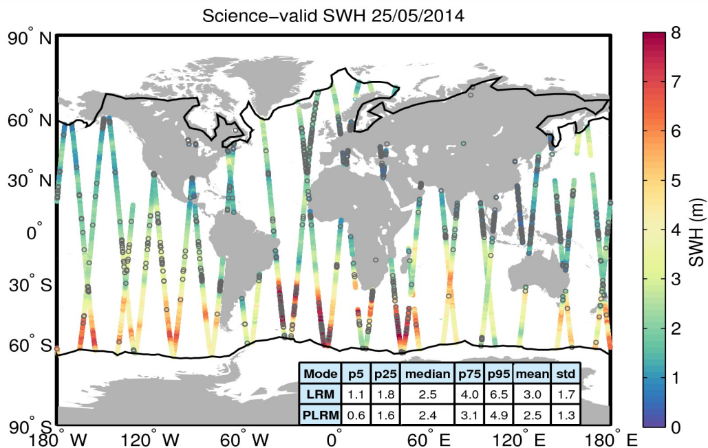
Figure 19. Geographical distribution of science-valid SWH data over oceans and lakes for 25/05/2014. The statistical values shown in the table refer to the SWH in m and are calculated separately for LRM and PLRM regions. The black lines mark the outer limit of the Arctic and Antarctic polar polygons. Gray circles denote records that have been rejected based on the editing criteria described in Table 3.
