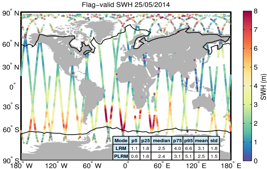
Figure 15. Geographical distribution of flag-valid SWH data over oceans and lakes for 25/05/2014. The statistical values shown in the table refer to the SWH in m and are calculated separately for LRM and PLRM regions. Measurements taken over polar polygons have been excluded from the computation of the statistical values. The black lines mark the outer limit of the Arctic and Antarctic polar polygons.
