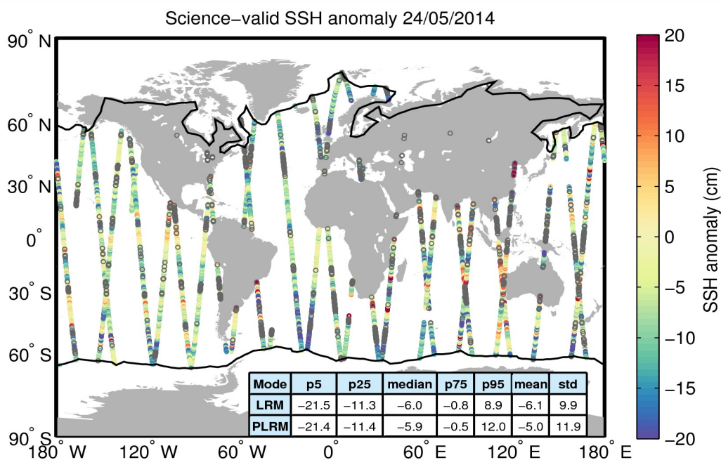
Figure 10. Geographical distribution of science-valid SSH anomaly data over oceans and lakes for 24/05/2014. The statistical values shown in the table refer to the SSH anomaly in cm and are calculated separately for LRM and PLRM regions. The black lines mark the outer limit of the Arctic and Antarctic polar polygons. Gray circles denote records that have been rejected based on the editing criteria described in Table 2.
