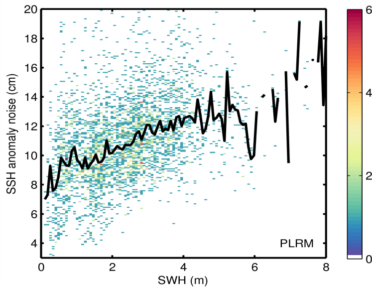
Figure 9. 2D histogram showing flag-valid SSH anomaly noise as a function of SWH for LRM (top) and PLRM (bottom) for 24/05/2014. The black line denotes the median SSH anomaly as a function of SWH.
