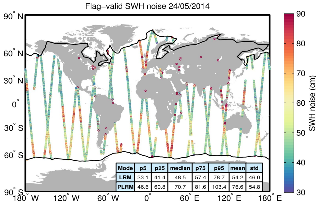
Figure 18. Geographical distribution of flag-valid 20-Hz SWH measurement noise over oceans and lakes for 24/05/2014. The statistical values shown in the table refer to the SWH noise and are calculated separately for LRM and PLRM regions. Measurements taken over polar polygons have been excluded from the computation of the statistical values. The black lines mark the outer limit of the Arctic and Antarctic polar polygons.
