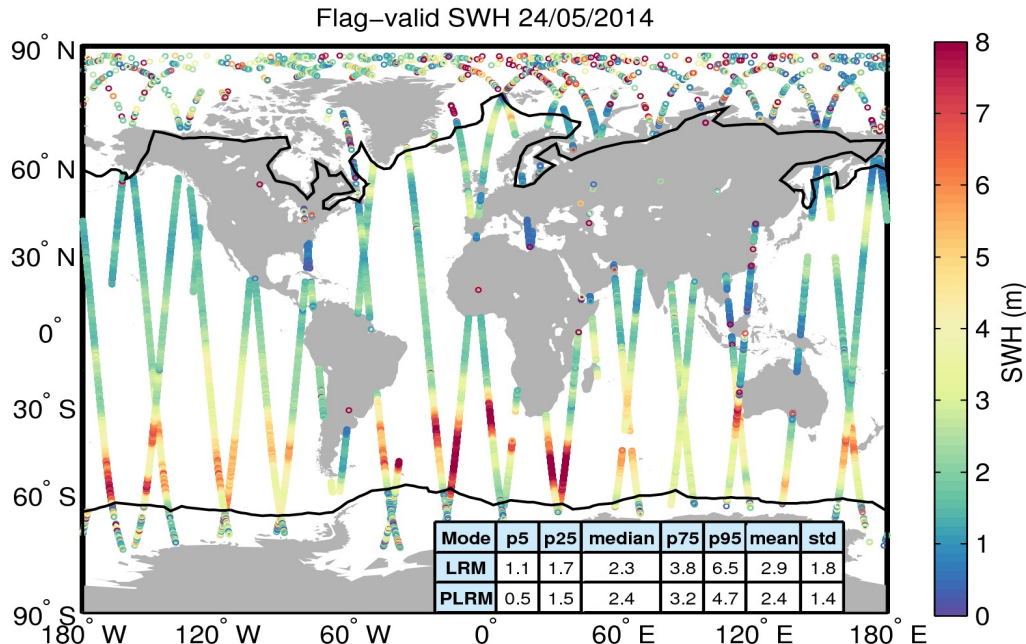
Figure 15. Geographical distribution of flag-valid SWH data over oceans and lakes for 24/05/2014. The statistical values shown in the table refer to the SWH in m and are calculated separately for LRM and PLRM regions. Measurements taken over polar polygons have been excluded from the computation of the statistical values. The black lines mark the outer limit of the Arctic and Antarctic polar polygons.
