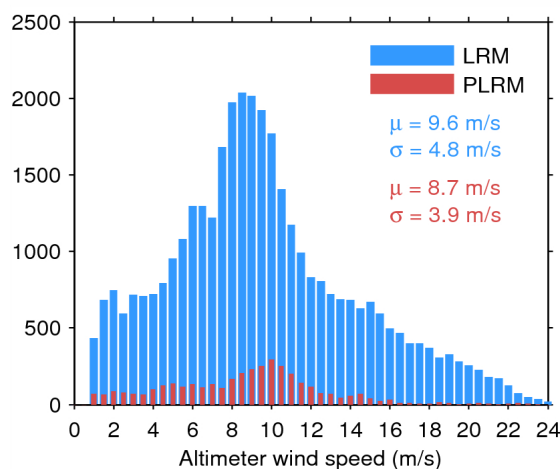
Figure 33. Histogram of flag-valid wind over oceans and lakes for LRM (blue) and PLRM (red) for 24/05/2014. The mean ( \mu ) and standard deviation ( \sigma ) are also shown. Note that values larger than 24 m/s are excluded from the histogram for the sake of readability but not from the computation of \mu and \sigma .
