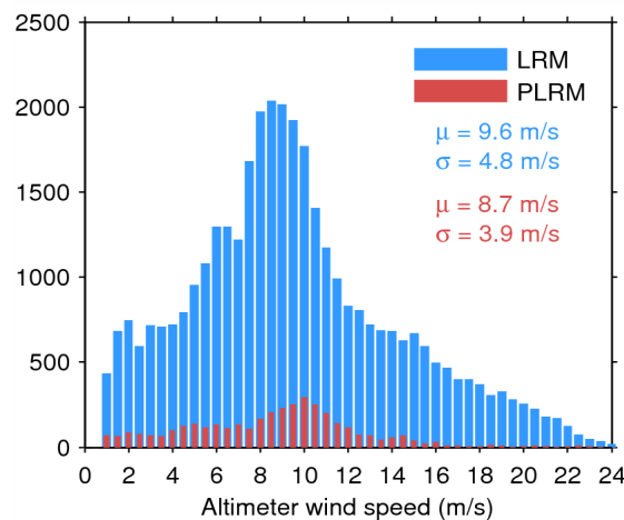
Figure 35. Histogram of science-valid wind over oceans and lakes for LRM (blue) and PLRM (red) for 24/05/2014. The mean ( \mu ) and standard deviation ( \sigma ) are also shown. Note that values larger than 24 m/s are excluded from the histogram for the sake of readability but not from the computation of \mu and \sigma .
