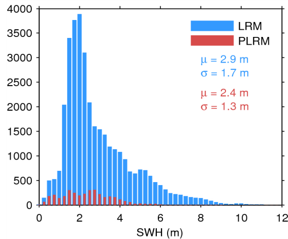
Figure 20. Histogram of science-valid SWH over oceans and lakes for LRM (blue) and PLRM (red) for 24/05/2014. The mean ( \mu ) and standard deviation ( \sigma ) are also shown. Note that values larger than 12 m are excluded from the histogram for the sake of readability but not from the computation of \mu and \sigma .
