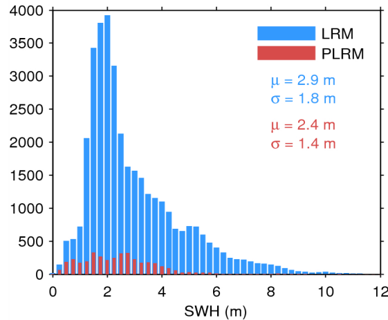
Figure 17. Histogram of flag-valid SWH over oceans and lakes for LRM (blue) and PLRM (red) for 24/05/2014. The mean ( \mu ) and standard deviation ( \sigma ) are also shown. Note that values larger than 12 m are excluded from the histogram for the sake of readability but not from the computation of \mu and \sigma .
