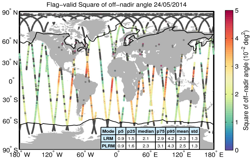
Figure 37. Geographical distribution of flag-valid mispointing data over oceans and lakes for 24/05/2014. The statistical values shown in the table refer to the mispointing in 10^{-2} deg 2 and are calculated separately for LRM and PLRM regions. Measurements taken over polar polygons have been excluded from the computation of the statistical values. The black lines mark the outer limit of the Arctic and Antarctic polar polygons. Gray circles denote negative values.
