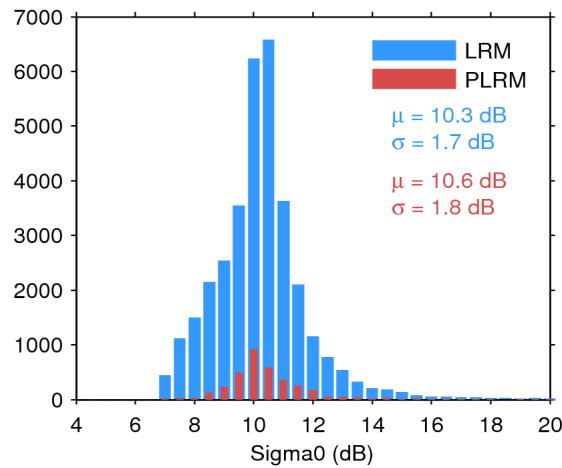
Figure 28. Histogram of science-valid sigma0 over oceans and lakes for LRM (blue) and PLRM (red) for 24/05/2014. The mean ( \mu ) and standard deviation ( \sigma ) are also shown. Note that values outside [4 20] dB are excluded from the histogram for the sake of readability but not from the computation of \mu and \sigma .
