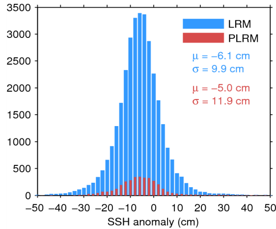
Figure 11. Histogram of science-valid SSH anomaly over oceans and lakes for LRM (blue) and PLRM (red) for 24/05/2014. The mean ( \mu ) and standard deviation ( \sigma ) are also shown. Note that values outside [-50 50] cm are excluded from the histogram for the sake of readability but not from the computation of \mu and \sigma .
