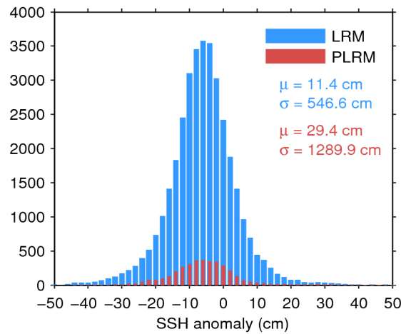
Figure 7. Histogram of flag-valid SSH anomaly over oceans and lakes for LRM (blue) and PLRM (red) for 24/05/2014. The mean ( \mu ) and standard deviation ( \sigma ) are also shown. Note that values outside [-50\ 50] cm are excluded from the histogram for the sake of readability but not from the computation of \mu and \sigma .
