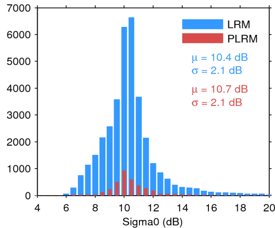
Figure 25. Histogram of flag-valid sigma0 over oceans and lakes for LRM (blue) and PLRM (red) for 24/05/2014. The mean ( \mu ) and standard deviation ( \sigma ) are also shown. Note that values outside [4 20] dB are excluded from the histogram for the sake of readability but not from the computation of \mu and \sigma .
