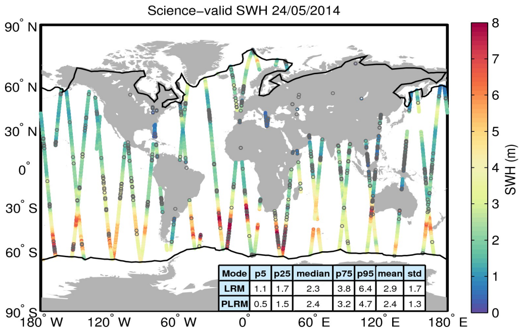
Figure 19. Geographical distribution of science-valid SWH data over oceans and lakes for 24/05/2014. The statistical values shown in the table refer to the SWH in m and are calculated separately for LRM and PLRM regions. The black lines mark the outer limit of the Arctic and Antarctic polar polygons. Gray circles denote records that have been rejected based on the editing criteria described in Table 3.
