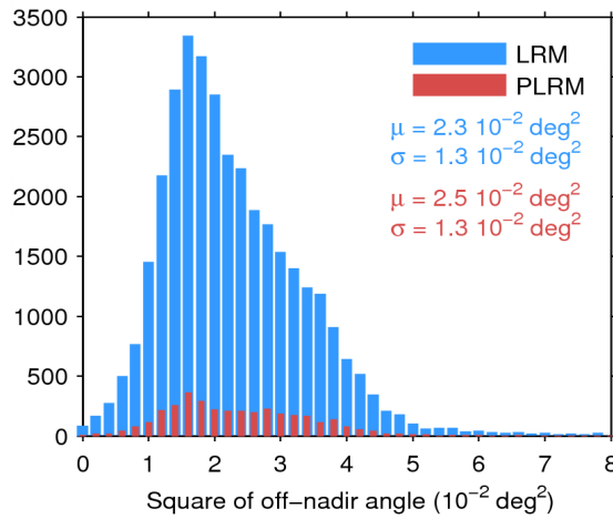
Figure 39. Histogram of flag-valid mispointing over oceans and lakes for LRM (blue) and PLRM (red) for 24/05/2014. Only positive values have been considered. The mean ( \mu ) and standard deviation ( \sigma ) are also shown. Note that values 8 \cdot 10^{-2} \text{ deg}^2 are excluded from the histogram for the sake of readability but not from the computation of \mu and \sigma .
