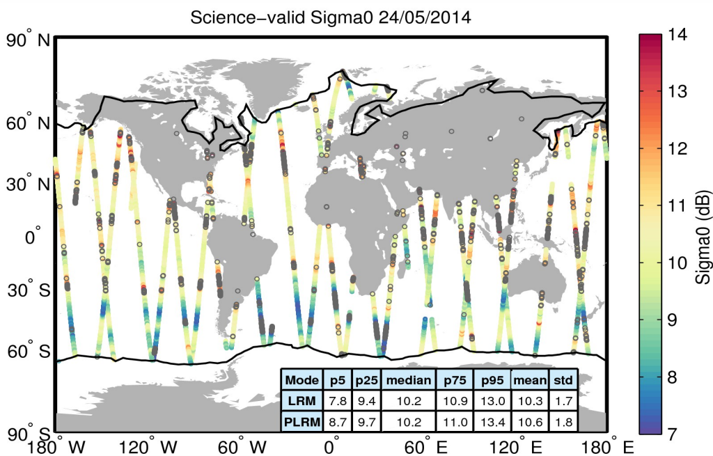
Figure 27. Geographical distribution of science-valid sigma0 data over oceans and lakes for 24/05/2014. The statistical values shown in the table refer to the sigma0 in dB and are calculated separately for LRM and PLRM regions. The black lines mark the outer limit of the Arctic and Antarctic polar polygons. Gray circles denote records that have been rejected based on the editing criteria described in Table 4.
