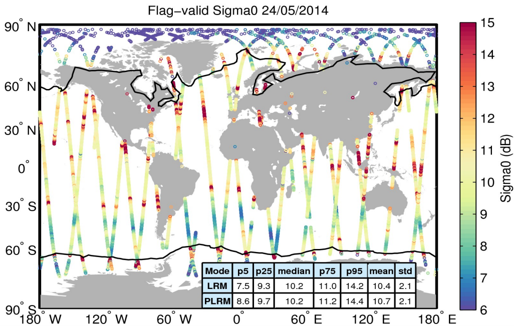
Figure 23. Geographical distribution of flag-valid sigma0 data over oceans and lakes for 24/05/2014. The statistical values shown in the table refer to the sigma0 in dB and are calculated separately for LRM and PLRM regions. Measurements taken over polar polygons have been excluded from the computation of the statistical values. The black lines mark the outer limit of the Arctic and Antarctic polar polygons.
