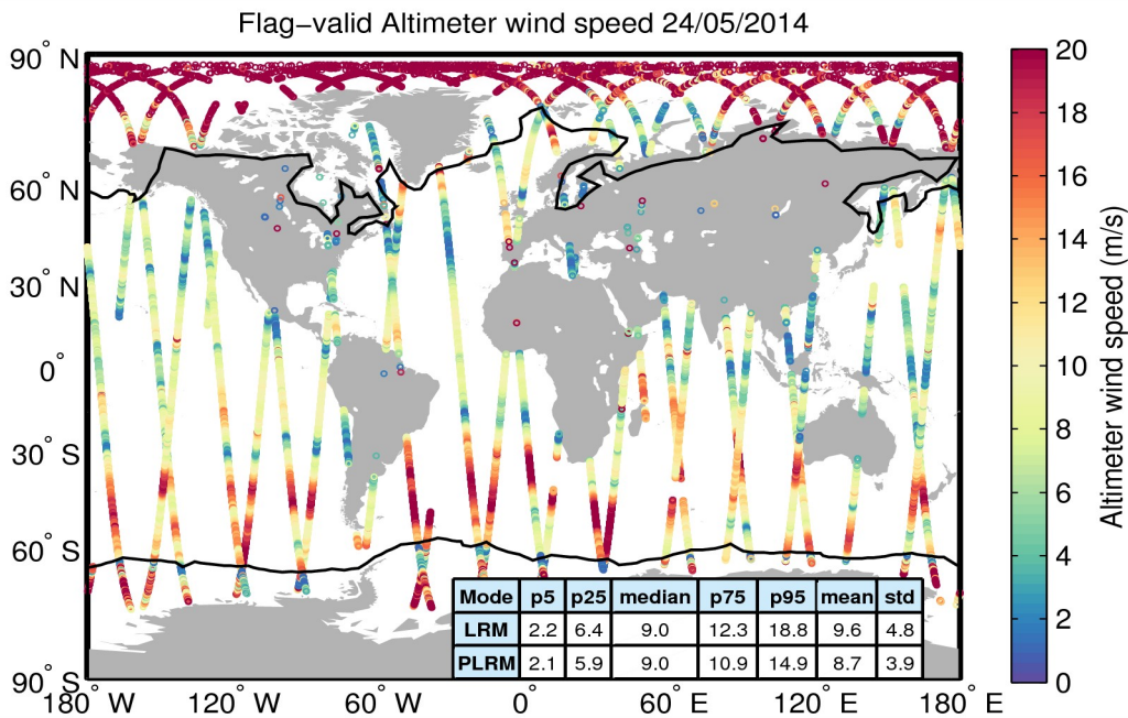
Figure 31. Geographical distribution of flag-valid wind data over oceans and lakes for 24/05/2014. The statistical values shown in the table refer to the wind in m/s and are calculated separately for LRM and PLRM regions. Measurements taken over polar polygons have been excluded from the computation of the statistical values. The black lines mark the outer limit of the Arctic and Antarctic polar polygons.
