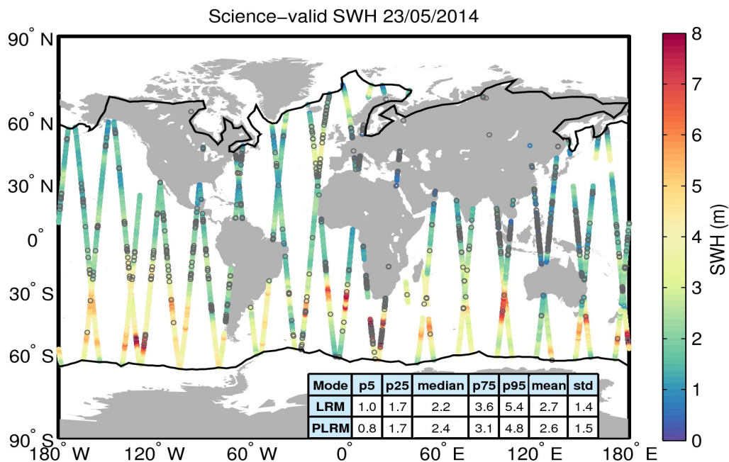
Figure 19. Geographical distribution of science-valid SWH data over oceans and lakes for 23/05/2014. The statistical values shown in the table refer to the SWH in m and are calculated separately for LRM and PLRM regions. The black lines mark the outer limit of the Arctic and Antarctic polar polygons. Gray circles denote records that have been rejected based on the editing criteria described in Table 3.
