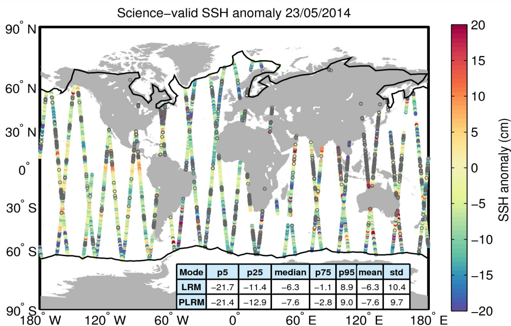
Figure 10. Geographical distribution of science-valid SSH anomaly data over oceans and lakes for 23/05/2014. The statistical values shown in the table refer to the SSH anomaly in cm and are calculated separately for LRM and PLRM regions. The black lines mark the outer limit of the Arctic and Antarctic polar polygons. Gray circles denote records that have been rejected based on the editing criteria described in Table 2.
