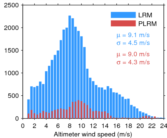
Figure 33. Histogram of flag-valid wind over oceans and lakes for LRM (blue) and PLRM (red) for 23/05/2014. The mean ( \mu ) and standard deviation ( \sigma ) are also shown. Note that values larger than 24 m/s are excluded from the histogram for the sake of readability but not from the computation of \mu and \sigma .
