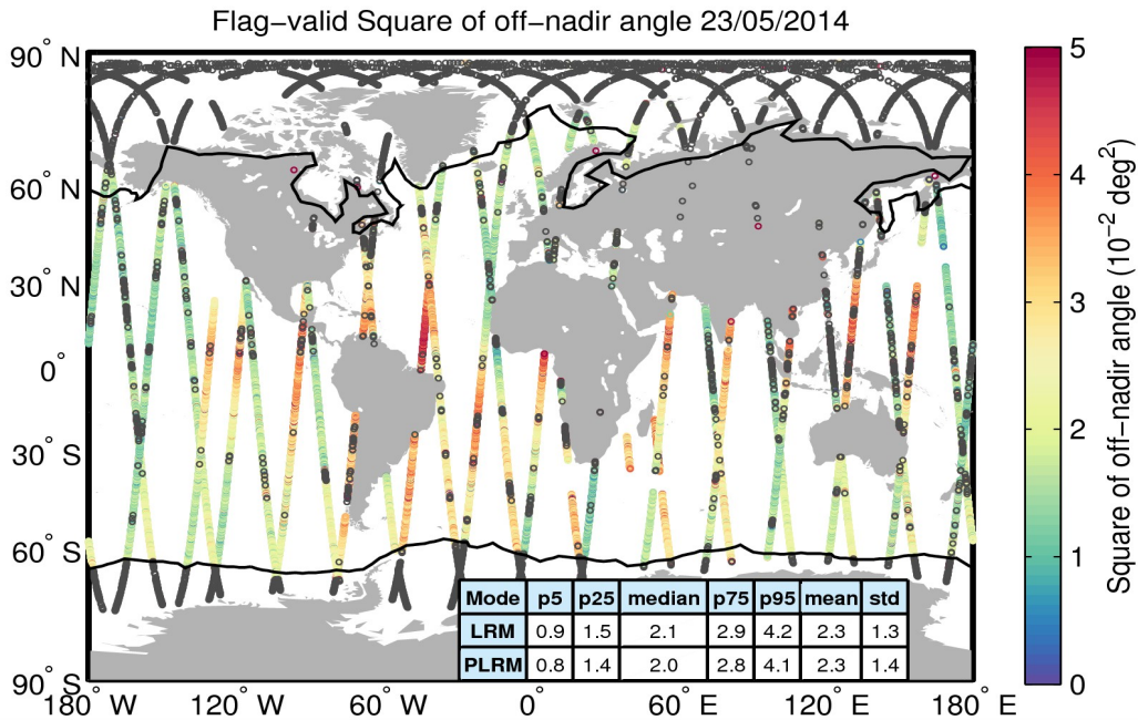
Figure 37. Geographical distribution of flag-valid mispointing data over oceans and lakes for 23/05/2014. The statistical values shown in the table refer to the mispointing in 10^{-2} \text{ deg}^2 and are calculated separately for LRM and PLRM regions. Measurements taken over polar polygons have been excluded from the computation of the statistical values. The black lines mark the outer limit of the Arctic and Antarctic polar polygons. Gray circles denote negative values.
