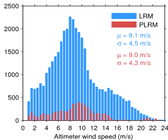
Figure 35. Histogram of science-valid wind over oceans and lakes for LRM (blue) and PLRM (red) for 23/05/2014. The mean ( \mu ) and standard deviation ( \sigma ) are also shown. Note that values larger than 24 m/s are excluded from the histogram for the sake of readability but not from the computation of \mu and \sigma .
