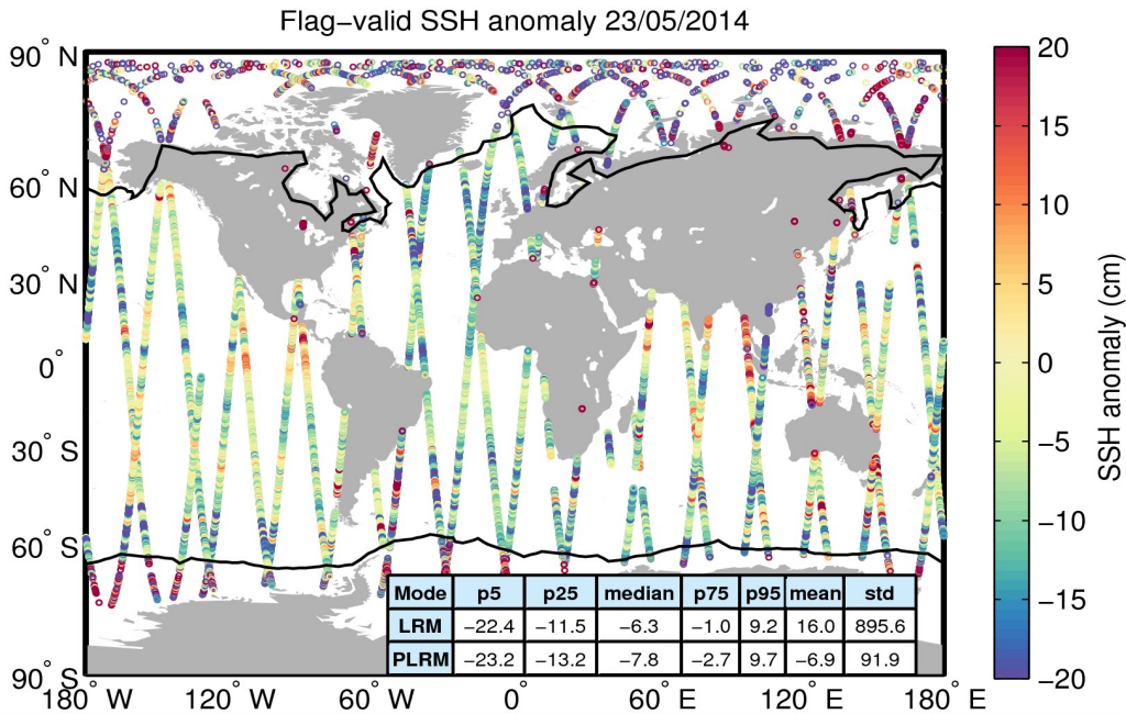
Figure 5. Geographical distribution of flag-valid 1-Hz SSH anomaly data over oceans and lakes for 23/05/2014. The statistical values shown in the table refer to the SSH anomaly in cm and are calculated separately for LRM and PLRM regions. Measurements taken over polar polygons have been excluded from the computation of the statistical values. The black lines mark the outer limit of the Arctic and Antarctic polar polygons.
