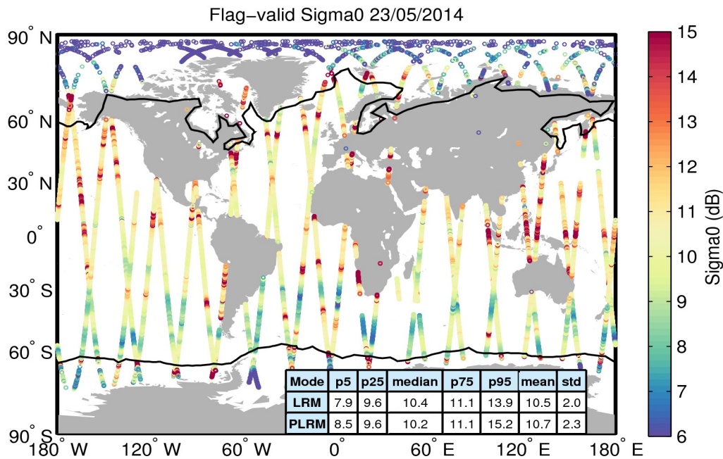
Figure 23. Geographical distribution of flag-valid sigma0 data over oceans and lakes for 23/05/2014. The statistical values shown in the table refer to the sigma0 in dB and are calculated separately for LRM and PLRM regions. Measurements taken over polar polygons have been excluded from the computation of the statistical values. The black lines mark the outer limit of the Arctic and Antarctic polar polygons.
