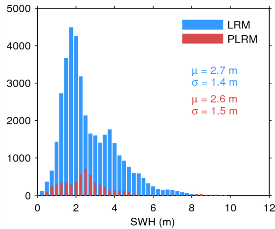
Figure 20. Histogram of science-valid SWH over oceans and lakes for LRM (blue) and PLRM (red) for 23/05/2014. The mean ( \mu ) and standard deviation ( \sigma ) are also shown. Note that values larger than 12 m are excluded from the histogram for the sake of readability but not from the computation of \mu and \sigma .
