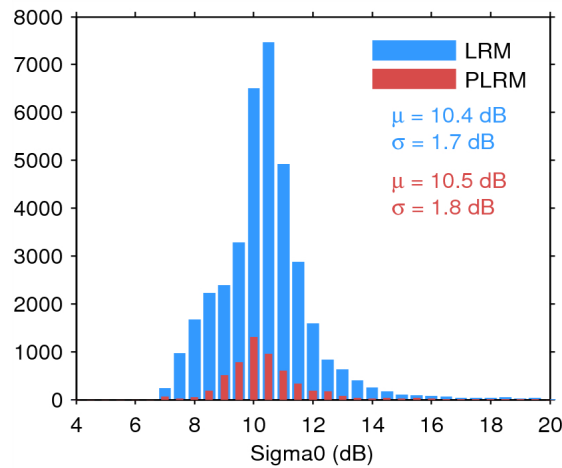
Figure 28. Histogram of science-valid sigma0 over oceans and lakes for LRM (blue) and PLRM (red) for 23/05/2014. The mean ( \mu ) and standard deviation ( \sigma ) are also shown. Note that values outside [4 20] dB are excluded from the histogram for the sake of readability but not from the computation of \mu and \sigma .
