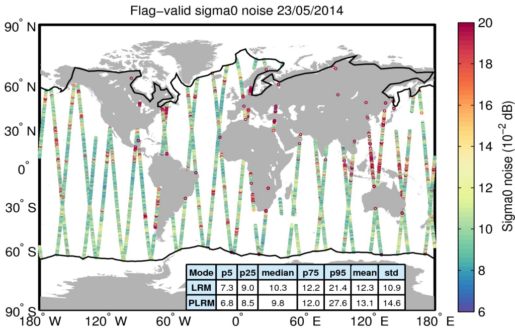
Figure 26. Geographical distribution of flag-valid 20-Hz sigma0 measurement noise over oceans and lakes for 23/05/2014. The statistical values shown in the table refer to the sigma0 noise and are calculated separately for LRM and PLRM regions. Measurements taken over polar polygons have been excluded from the computation of the statistical values. The black lines mark the outer limit of the Arctic and Antarctic polar polygons.
