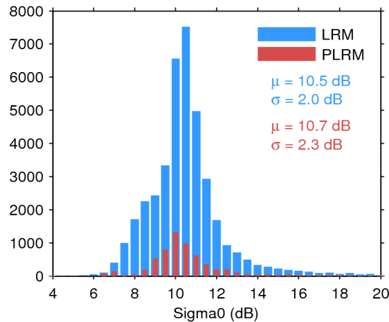
Figure 25. Histogram of flag-valid sigma0 over oceans and lakes for LRM (blue) and PLRM (red) for 23/05/2014. The mean ( \mu ) and standard deviation ( \sigma ) are also shown. Note that values outside [4 20] dB are excluded from the histogram for the sake of readability but not from the computation of \mu and \sigma .
