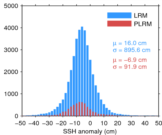
Figure 7. Histogram of flag-valid SSH anomaly over oceans and lakes for LRM (blue) and PLRM (red) for 23/05/2014. The mean ( \mu ) and standard deviation ( \sigma ) are also shown. Note that values outside [-50\ 50] cm are excluded from the histogram for the sake of readability but not from the computation of \mu and \sigma .
