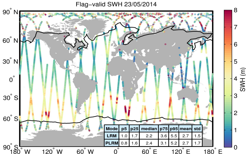
Figure 15. Geographical distribution of flag-valid SWH data over oceans and lakes for 23/05/2014. The statistical values shown in the table refer to the SWH in m and are calculated separately for LRM and PLRM regions. Measurements taken over polar polygons have been excluded from the computation of the statistical values. The black lines mark the outer limit of the Arctic and Antarctic polar polygons.
