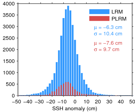
Figure 11. Histogram of science-valid SSH anomaly over oceans and lakes for LRM (blue) and PLRM (red) for 23/05/2014. The mean ( \mu ) and standard deviation ( \sigma ) are also shown. Note that values outside [-50 50] cm are excluded from the histogram for the sake of readability but not from the computation of \mu and \sigma .
