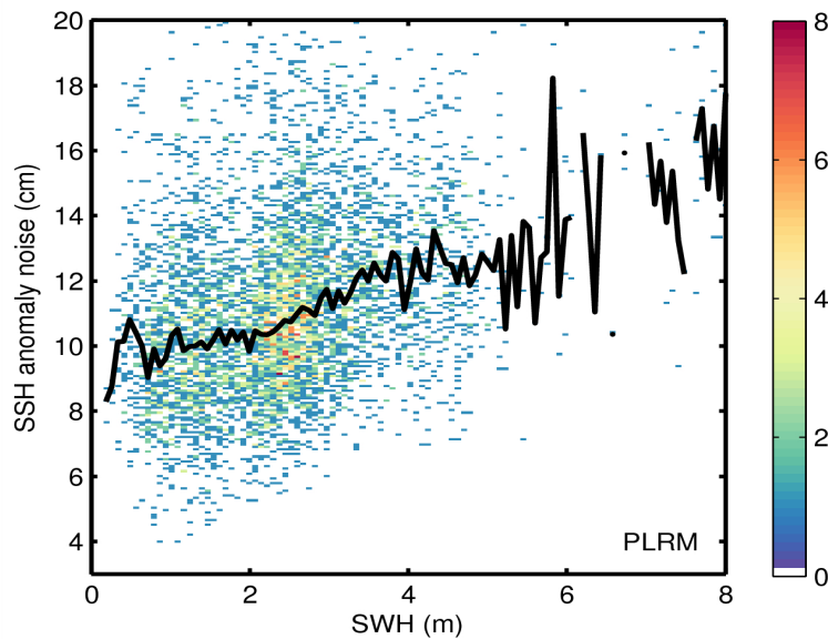
Figure 9. 2D histogram showing flag-valid SSH anomaly noise as a function of SWH for LRM (top) and PLRM (bottom) for 23/05/2014. The black line denotes the median SSH anomaly as a function of SWH.
