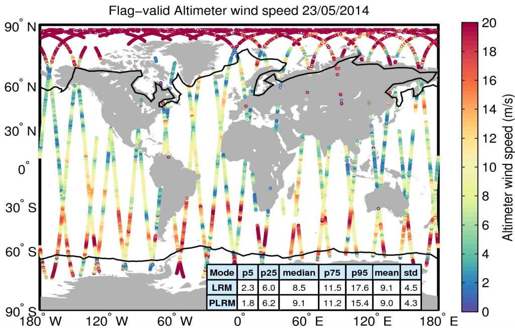
Figure 31. Geographical distribution of flag-valid wind data over oceans and lakes for 23/05/2014. The statistical values shown in the table refer to the wind in m/s and are calculated separately for LRM and PLRM regions. Measurements taken over polar polygons have been excluded from the computation of the statistical values. The black lines mark the outer limit of the Arctic and Antarctic polar polygons.
