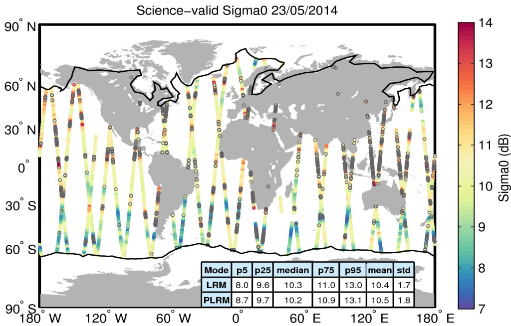
Figure 27. Geographical distribution of science-valid sigma0 data over oceans and lakes for 23/05/2014. The statistical values shown in the table refer to the sigma0 in dB and are calculated separately for LRM and PLRM regions. The black lines mark the outer limit of the Arctic and Antarctic polar polygons. Gray circles denote records that have been rejected based on the editing criteria described in Table 4.
