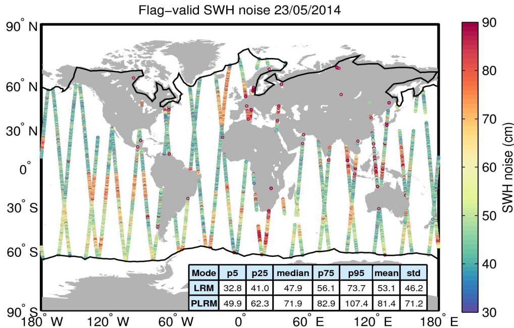
Figure 18. Geographical distribution of flag-valid 20-Hz SWH measurement noise over oceans and lakes for 23/05/2014. The statistical values shown in the table refer to the SWH noise and are calculated separately for LRM and PLRM regions. Measurements taken over polar polygons have been excluded from the computation of the statistical values. The black lines mark the outer limit of the Arctic and Antarctic polar polygons.
