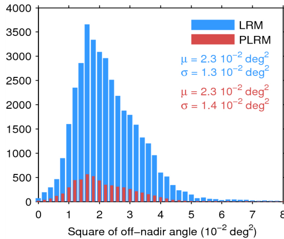
Figure 39. Histogram of flag-valid mispointing over oceans and lakes for LRM (blue) and PLRM (red) for 23/05/2014. Only positive values have been considered. The mean ( \mu ) and standard deviation ( \sigma ) are also shown. Note that values 8 \cdot 10^{-2} \text{ deg}^2 are excluded from the histogram for the sake of readability but not from the computation of \mu and \sigma .
