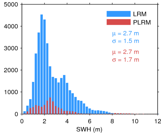
Figure 17. Histogram of flag-valid SWH over oceans and lakes for LRM (blue) and PLRM (red) for 23/05/2014. The mean ( \mu ) and standard deviation ( \sigma ) are also shown. Note that values larger than 12 m are excluded from the histogram for the sake of readability but not from the computation of \mu and \sigma .
