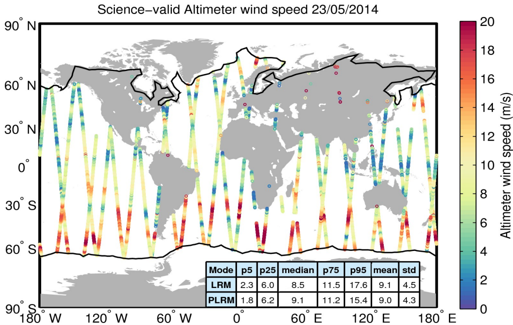
Figure 34. Geographical distribution of science-valid wind data over oceans and lakes for 23/05/2014. The statistical values shown in the table refer to the wind in m/s and are calculated separately for LRM and PLRM regions. The black lines mark the outer limit of the Arctic and Antarctic polar polygons. Gray circles denote records that have been rejected based on the editing criteria described in Table 5.
