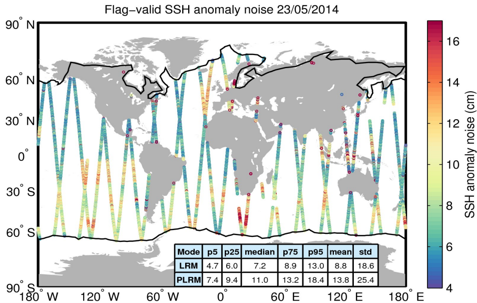
Figure 8. Geographical distribution of flag-valid 20-Hz SSH anomaly measurement noise over oceans and lakes for 23/05/2014. The statistical values shown in the table refer to the SSH anomaly noise and are calculated separately for LRM and PLRM regions. Measurements taken over polar polygons have been excluded from the computation of the statistical values. The black lines mark the outer limit of the Arctic and Antarctic polar polygons.
