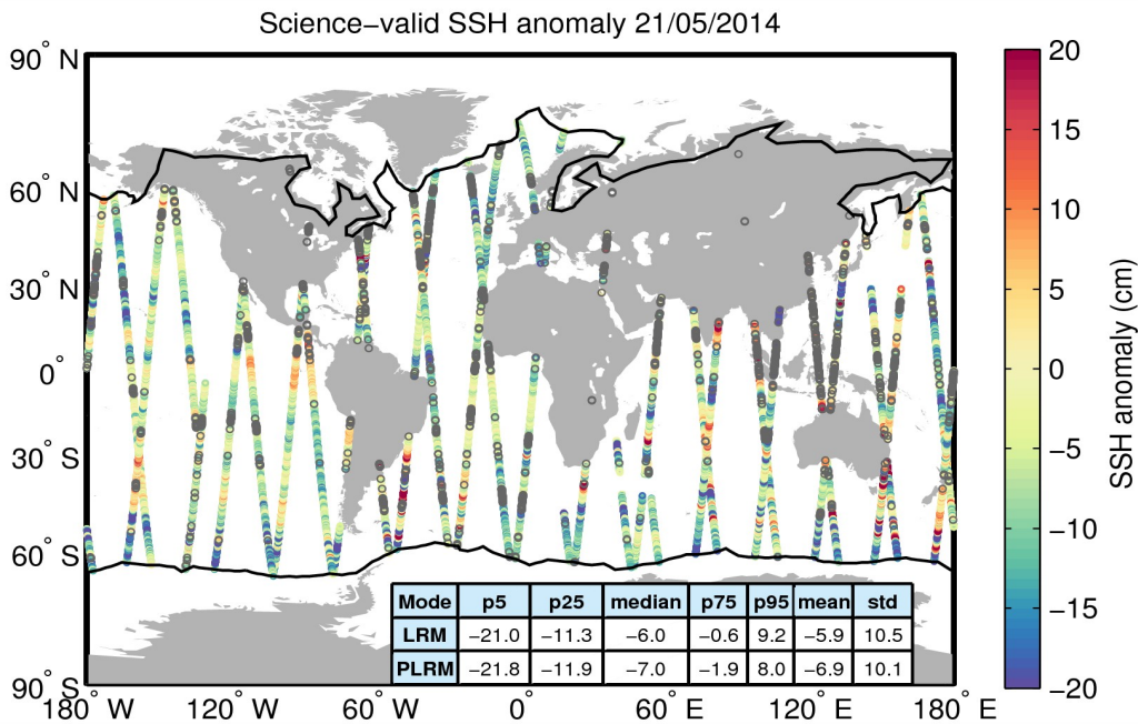
Figure 10. Geographical distribution of science-valid SSH anomaly data over oceans and lakes for 21/05/2014. The statistical values shown in the table refer to the SSH anomaly in cm and are calculated separately for LRM and PLRM regions. The black lines mark the outer limit of the Arctic and Antarctic polar polygons. Gray circles denote records that have been rejected based on the editing criteria described in Table 2.
