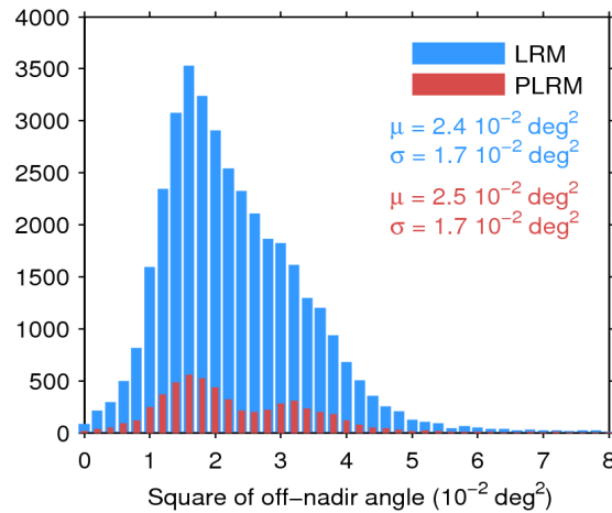
Figure 39. Histogram of flag-valid mispointing over oceans and lakes for LRM (blue) and PLRM (red) for 21/05/2014. Only positive values have been considered. The mean ( \mu ) and standard deviation ( \sigma ) are also shown. Note that values 8 \cdot 10^{-2} \text{ deg}^2 are excluded from the histogram for the sake of readability but not from the computation of \mu and \sigma .
