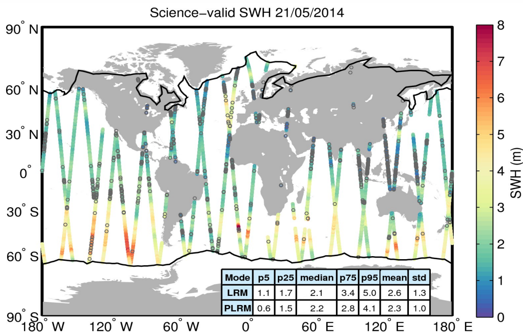
Figure 19. Geographical distribution of science-valid SWH data over oceans and lakes for 21/05/2014. The statistical values shown in the table refer to the SWH in m and are calculated separately for LRM and PLRM regions. The black lines mark the outer limit of the Arctic and Antarctic polar polygons. Gray circles denote records that have been rejected based on the editing criteria described in Table 3.
