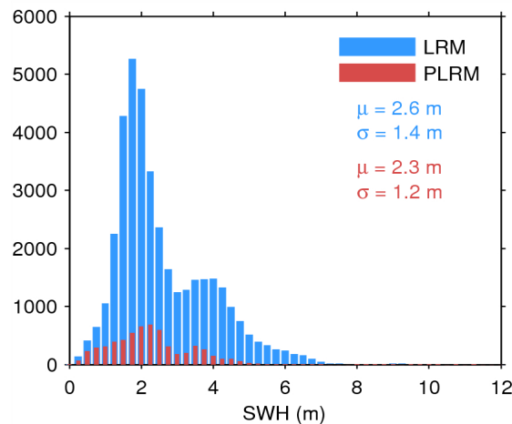
Figure 17. Histogram of flag-valid SWH over oceans and lakes for LRM (blue) and PLRM (red) for 21/05/2014. The mean ( \mu ) and standard deviation ( \sigma ) are also shown. Note that values larger than 12 m are excluded from the histogram for the sake of readability but not from the computation of \mu and \sigma .
