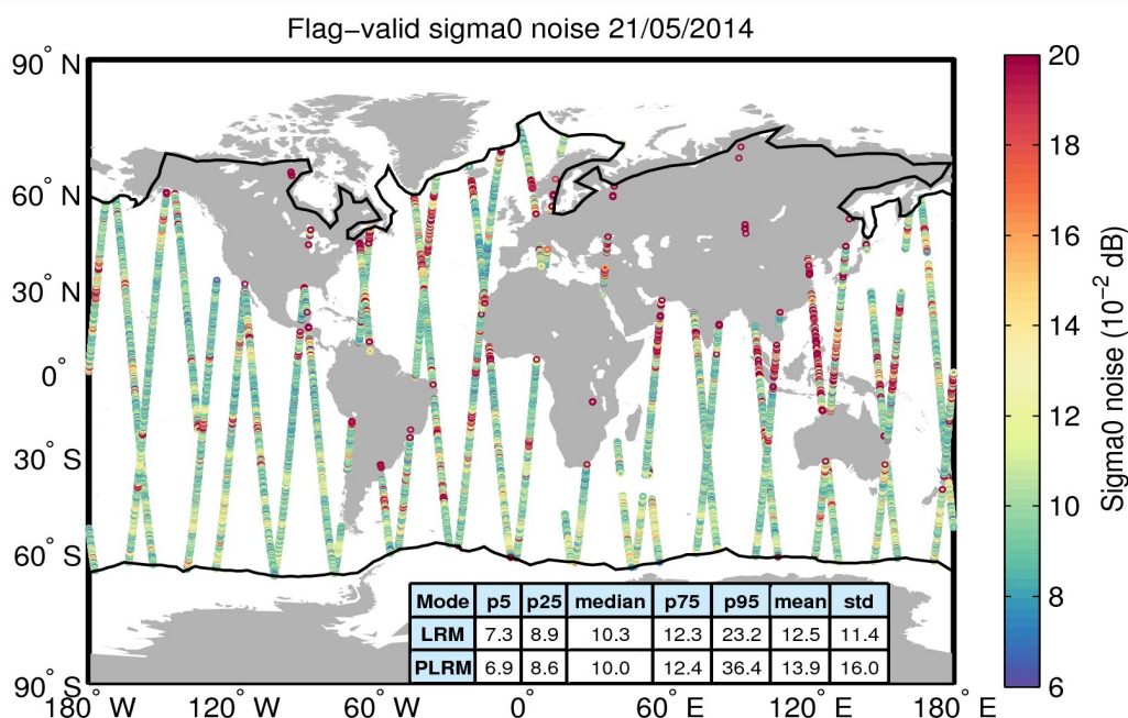
Figure 26. Geographical distribution of flag-valid 20-Hz sigma0 measurement noise over oceans and lakes for 21/05/2014. The statistical values shown in the table refer to the sigma0 noise and are calculated separately for LRM and PLRM regions. Measurements taken over polar polygons have been excluded from the computation of the statistical values. The black lines mark the outer limit of the Arctic and Antarctic polar polygons.
