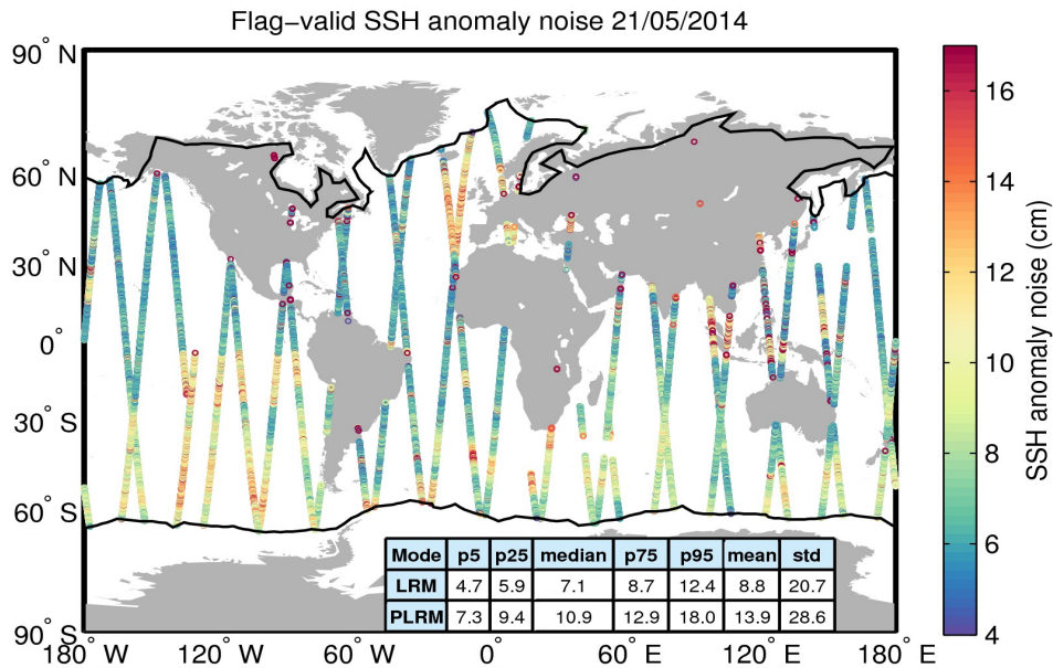
Figure 8. Geographical distribution of flag-valid 20-Hz SSH anomaly measurement noise over oceans and lakes for 21/05/2014. The statistical values shown in the table refer to the SSH anomaly noise and are calculated separately for LRM and PLRM regions. Measurements taken over polar polygons have been excluded from the computation of the statistical values. The black lines mark the outer limit of the Arctic and Antarctic polar polygons.
