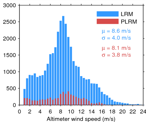
Figure 35. Histogram of science-valid wind over oceans and lakes for LRM (blue) and PLRM (red) for 21/05/2014. The mean ( \mu ) and standard deviation ( \sigma ) are also shown. Note that values larger than 24 m/s are excluded from the histogram for the sake of readability but not from the computation of \mu and \sigma .
