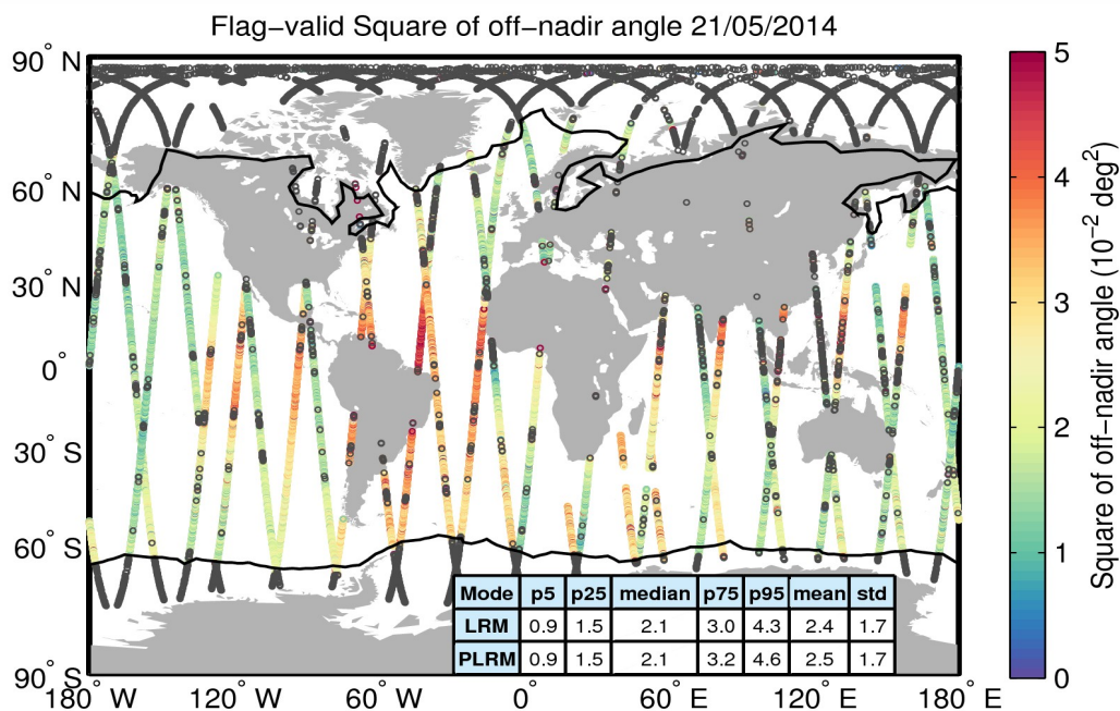
Figure 37. Geographical distribution of flag-valid mispointing data over oceans and lakes for 21/05/2014. The statistical values shown in the table refer to the mispointing in 10^{-2} \text{ deg}^2 and are calculated separately for LRM and PLRM regions. Measurements taken over polar polygons have been excluded from the computation of the statistical values. The black lines mark the outer limit of the Arctic and Antarctic polar polygons. Gray circles denote negative values.
