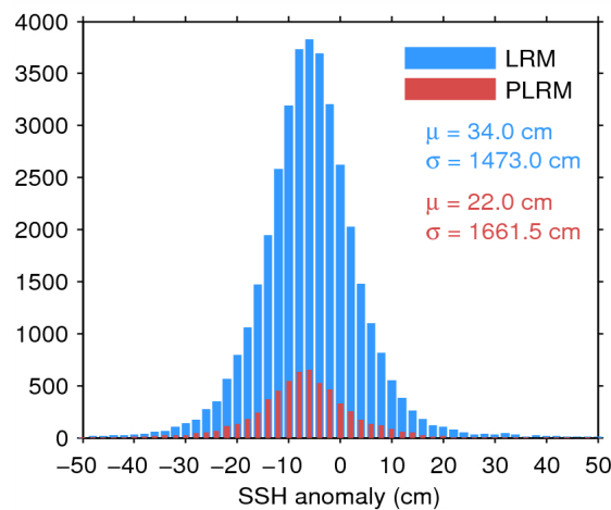
Figure 7. Histogram of flag-valid SSH anomaly over oceans and lakes for LRM (blue) and PLRM (red) for 21/05/2014. The mean ( \mu ) and standard deviation ( \sigma ) are also shown. Note that values outside [-50\ 50] cm are excluded from the histogram for the sake of readability but not from the computation of \mu and \sigma .
