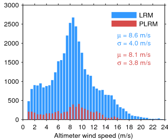
Figure 33. Histogram of flag-valid wind over oceans and lakes for LRM (blue) and PLRM (red) for 21/05/2014. The mean ( \mu ) and standard deviation ( \sigma ) are also shown. Note that values larger than 24 m/s are excluded from the histogram for the sake of readability but not from the computation of \mu and \sigma .
