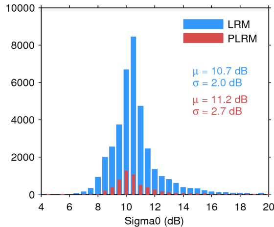
Figure 25. Histogram of flag-valid sigma0 over oceans and lakes for LRM (blue) and PLRM (red) for 21/05/2014. The mean ( \mu ) and standard deviation ( \sigma ) are also shown. Note that values outside [4 20] dB are excluded from the histogram for the sake of readability but not from the computation of \mu and \sigma .
