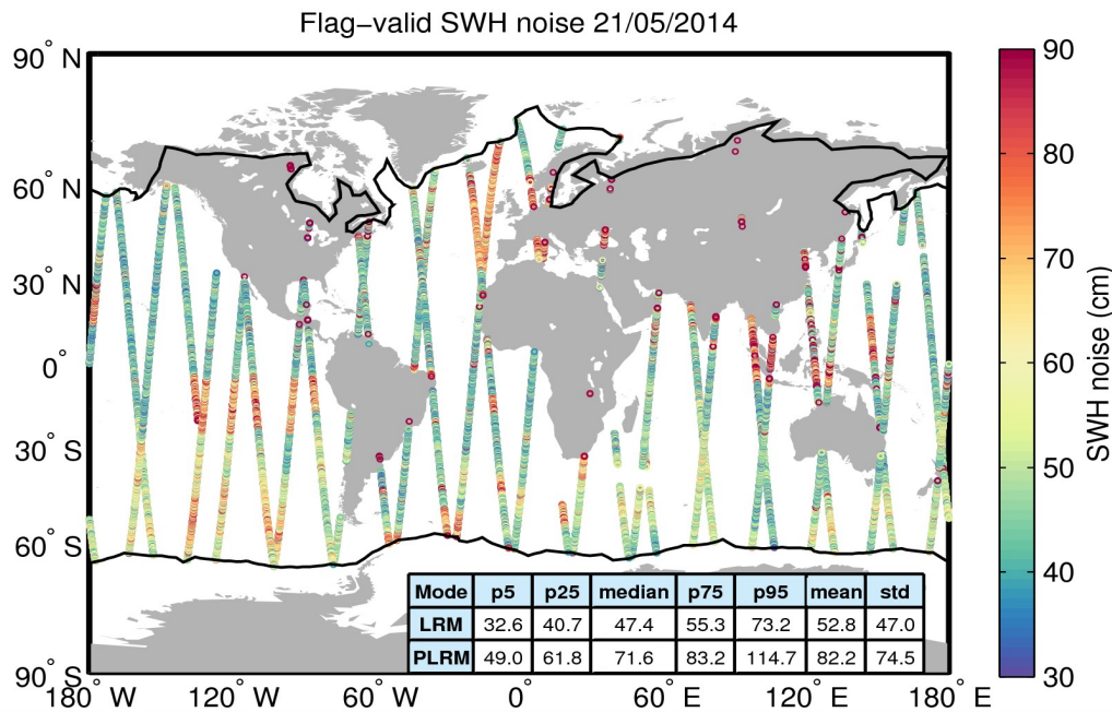
Figure 18. Geographical distribution of flag-valid 20-Hz SWH measurement noise over oceans and lakes for 21/05/2014. The statistical values shown in the table refer to the SWH noise and are calculated separately for LRM and PLRM regions. Measurements taken over polar polygons have been excluded from the computation of the statistical values. The black lines mark the outer limit of the Arctic and Antarctic polar polygons.
