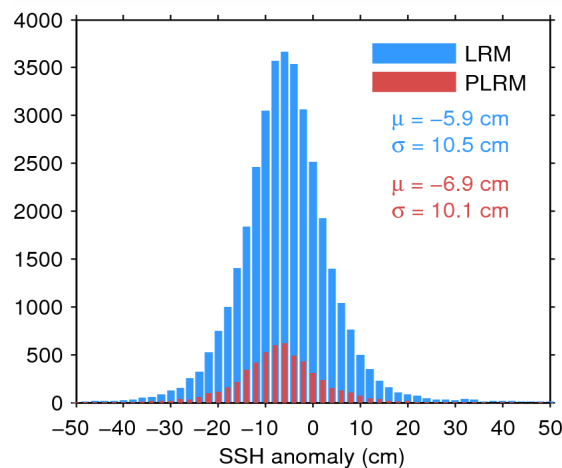
Figure 11. Histogram of science-valid SSH anomaly over oceans and lakes for LRM (blue) and PLRM (red) for 21/05/2014. The mean ( \mu ) and standard deviation ( \sigma ) are also shown. Note that values outside [-50 50] cm are excluded from the histogram for the sake of readability but not from the computation of \mu and \sigma .
