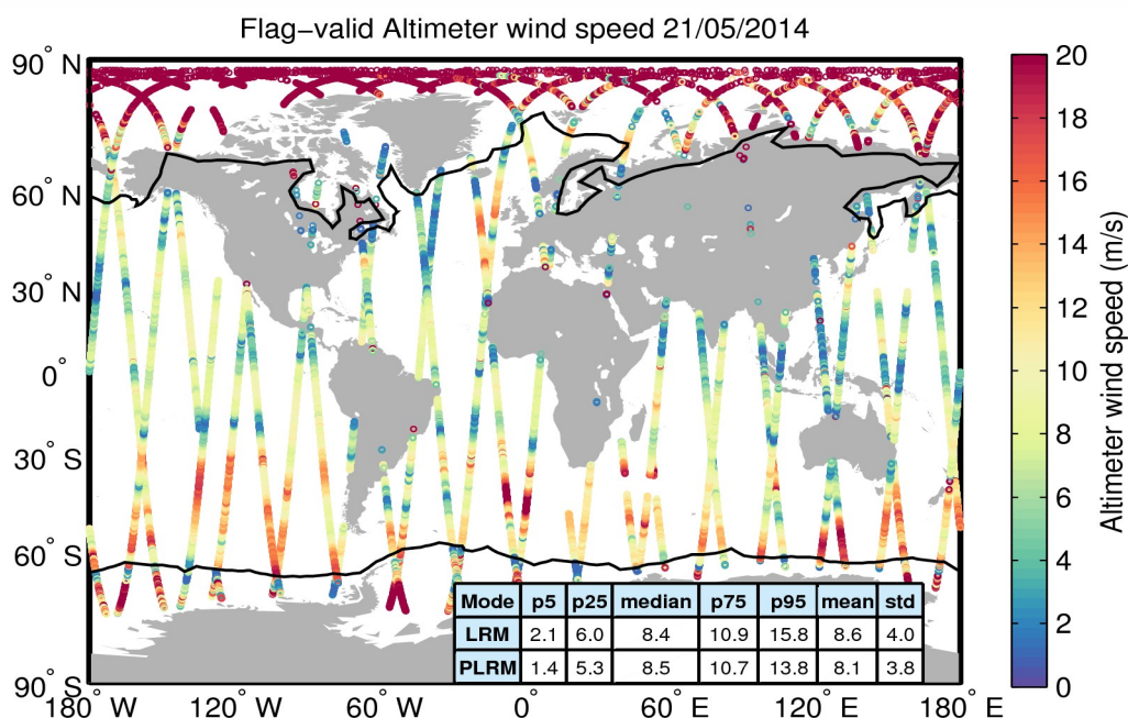
Figure 31. Geographical distribution of flag-valid wind data over oceans and lakes for 21/05/2014. The statistical values shown in the table refer to the wind in m/s and are calculated separately for LRM and PLRM regions. Measurements taken over polar polygons have been excluded from the computation of the statistical values. The black lines mark the outer limit of the Arctic and Antarctic polar polygons.
