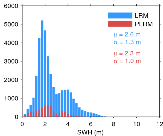
Figure 20. Histogram of science-valid SWH over oceans and lakes for LRM (blue) and PLRM (red) for 21/05/2014. The mean ( \mu ) and standard deviation ( \sigma ) are also shown. Note that values larger than 12 m are excluded from the histogram for the sake of readability but not from the computation of \mu and \sigma .
