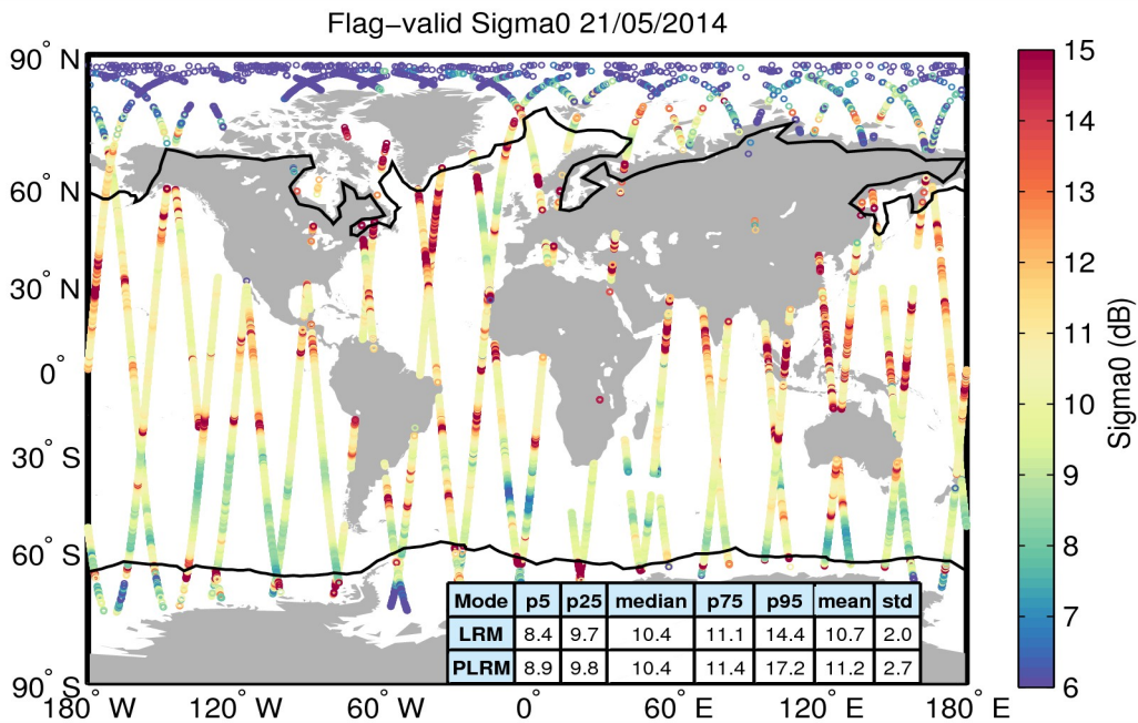
Figure 23. Geographical distribution of flag-valid sigma0 data over oceans and lakes for 21/05/2014. The statistical values shown in the table refer to the sigma0 in dB and are calculated separately for LRM and PLRM regions. Measurements taken over polar polygons have been excluded from the computation of the statistical values. The black lines mark the outer limit of the Arctic and Antarctic polar polygons.
