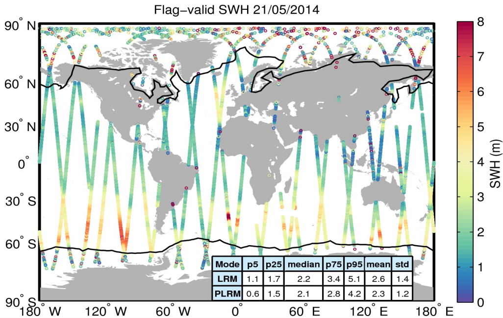
Figure 15. Geographical distribution of flag-valid SWH data over oceans and lakes for 21/05/2014. The statistical values shown in the table refer to the SWH in m and are calculated separately for LRM and PLRM regions. Measurements taken over polar polygons have been excluded from the computation of the statistical values. The black lines mark the outer limit of the Arctic and Antarctic polar polygons.
