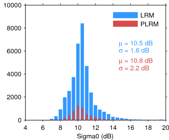
Figure 28. Histogram of science-valid sigma0 over oceans and lakes for LRM (blue) and PLRM (red) for 21/05/2014. The mean ( \mu ) and standard deviation ( \sigma ) are also shown. Note that values outside [4 20] dB are excluded from the histogram for the sake of readability but not from the computation of \mu and \sigma .
