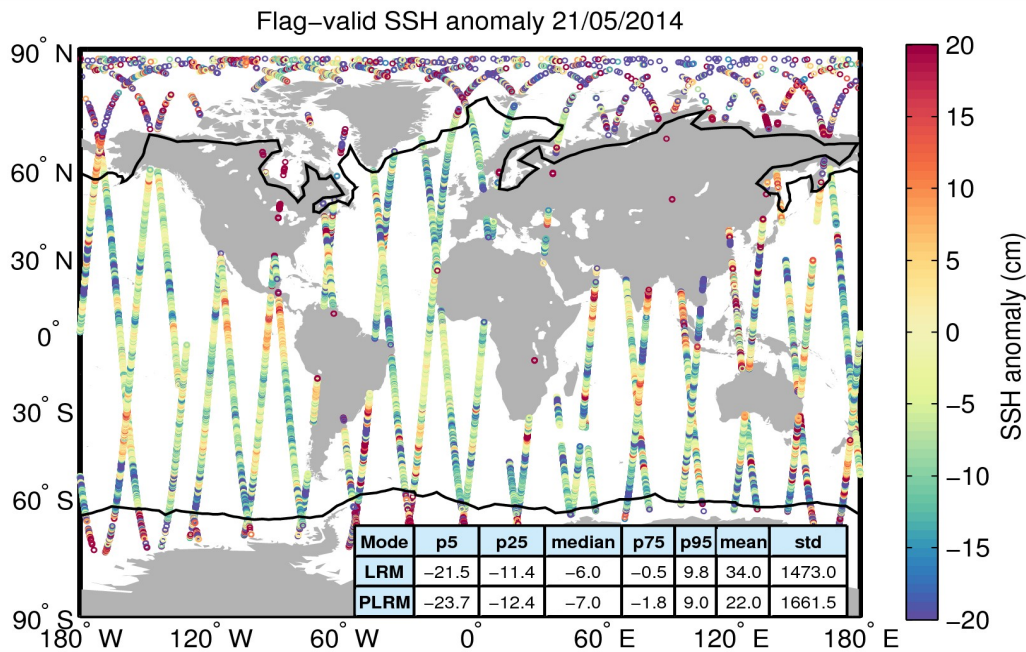
Figure 5. Geographical distribution of flag-valid 1-Hz SSH anomaly data over oceans and lakes for 21/05/2014. The statistical values shown in the table refer to the SSH anomaly in cm and are calculated separately for LRM and PLRM regions. Measurements taken over polar polygons have been excluded from the computation of the statistical values. The black lines mark the outer limit of the Arctic and Antarctic polar polygons.
