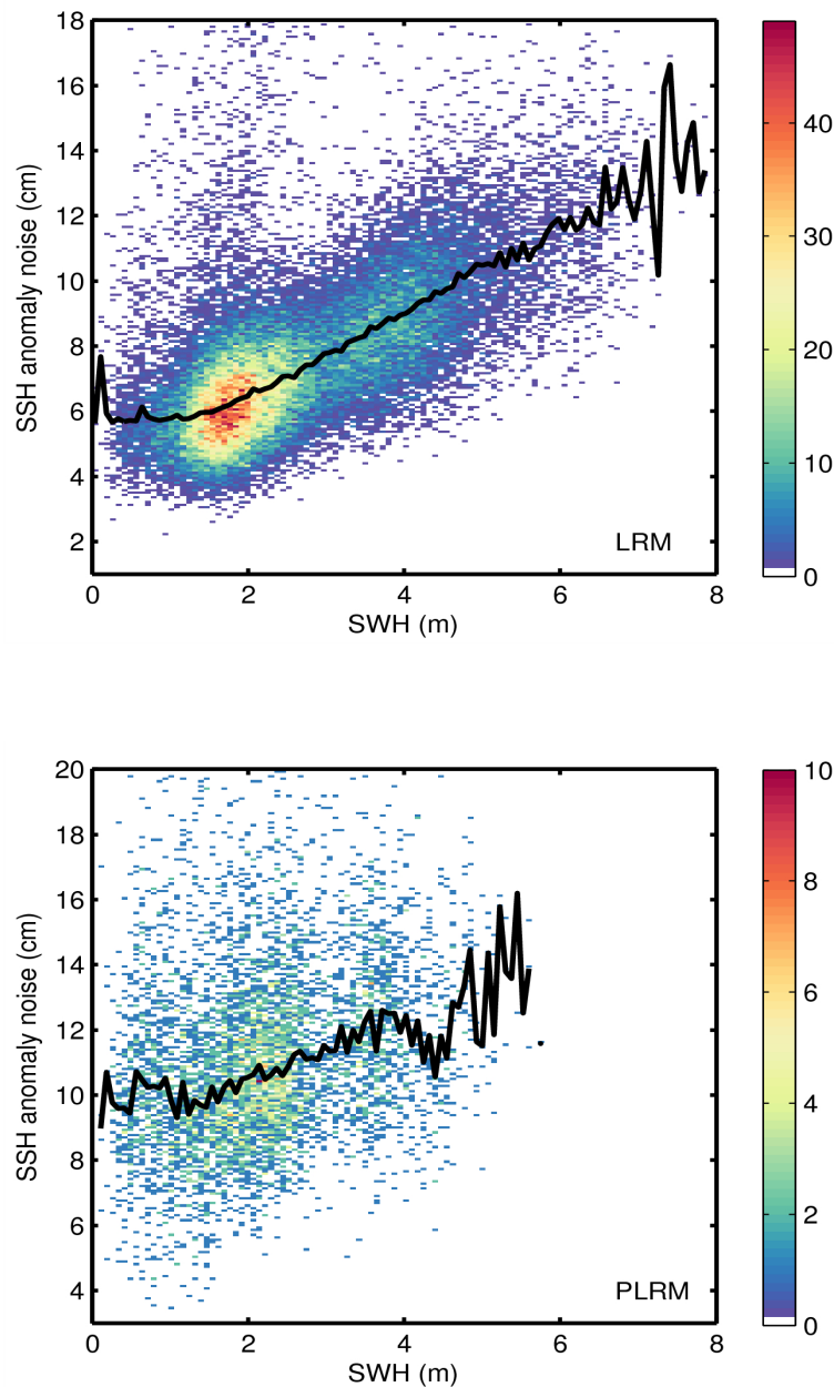
Figure 9. 2D histogram showing flag-valid SSH anomaly noise as a function of SWH for LRM (top) and PLRM (bottom) for 21/05/2014. The black line denotes the median SSH anomaly as a function of SWH.
