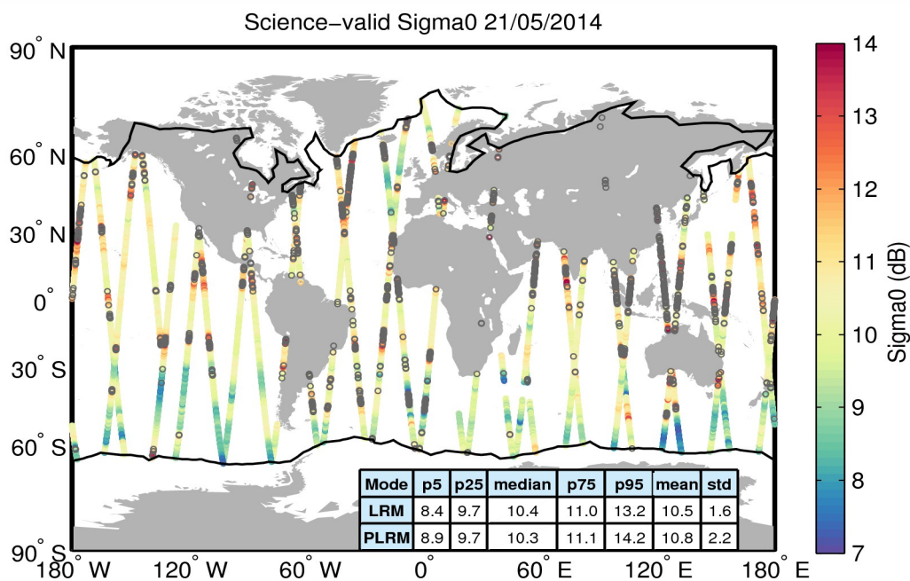
Figure 27. Geographical distribution of science-valid sigma0 data over oceans and lakes for 21/05/2014. The statistical values shown in the table refer to the sigma0 in dB and are calculated separately for LRM and PLRM regions. The black lines mark the outer limit of the Arctic and Antarctic polar polygons. Gray circles denote records that have been rejected based on the editing criteria described in Table 4.
