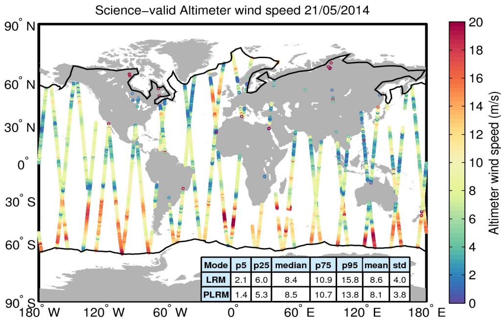
Figure 34. Geographical distribution of science-valid wind data over oceans and lakes for 21/05/2014. The statistical values shown in the table refer to the wind in m/s and are calculated separately for LRM and PLRM regions. The black lines mark the outer limit of the Arctic and Antarctic polar polygons. Gray circles denote records that have been rejected based on the editing criteria described in Table 5.
