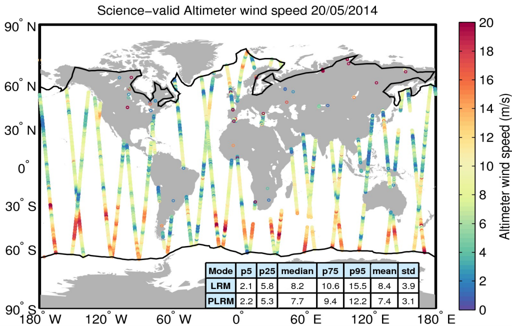
Figure 34. Geographical distribution of science-valid wind data over oceans and lakes for 20/05/2014. The statistical values shown in the table refer to the wind in m/s and are calculated separately for LRM and PLRM regions. The black lines mark the outer limit of the Arctic and Antarctic polar polygons. Gray circles denote records that have been rejected based on the editing criteria described in Table 5.
