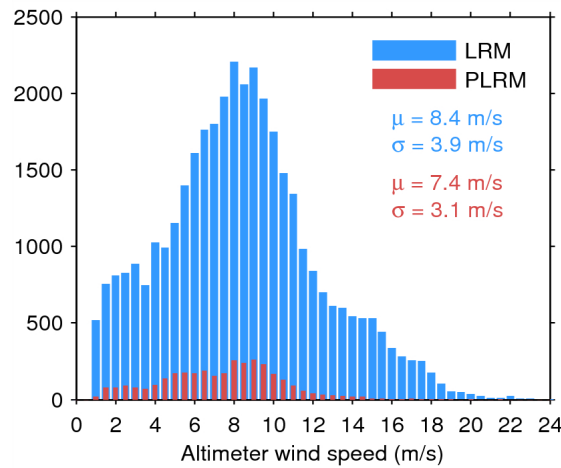
Figure 33. Histogram of flag-valid wind over oceans and lakes for LRM (blue) and PLRM (red) for 20/05/2014. The mean ( \mu ) and standard deviation ( \sigma ) are also shown. Note that values larger than 24 m/s are excluded from the histogram for the sake of readability but not from the computation of \mu and \sigma .
