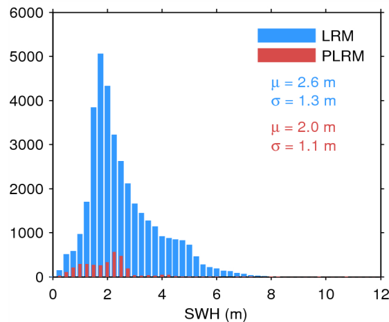
Figure 17. Histogram of flag-valid SWH over oceans and lakes for LRM (blue) and PLRM (red) for 20/05/2014. The mean ( \mu ) and standard deviation ( \sigma ) are also shown. Note that values larger than 12 m are excluded from the histogram for the sake of readability but not from the computation of \mu and \sigma .
