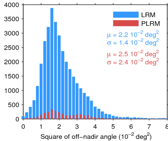
Figure 39. Histogram of flag-valid mispointing over oceans and lakes for LRM (blue) and PLRM (red) for 20/05/2014. Only positive values have been considered. The mean ( \mu ) and standard deviation ( \sigma ) are also shown. Note that values 8 \cdot 10^{-2} \text{ deg}^2 are excluded from the histogram for the sake of readability but not from the computation of \mu and \sigma .
