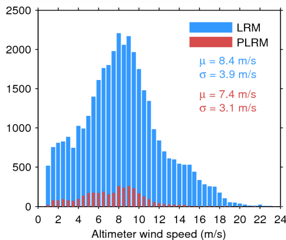
Figure 35. Histogram of science-valid wind over oceans and lakes for LRM (blue) and PLRM (red) for 20/05/2014. The mean ( \mu ) and standard deviation ( \sigma ) are also shown. Note that values larger than 24 m/s are excluded from the histogram for the sake of readability but not from the computation of \mu and \sigma .
