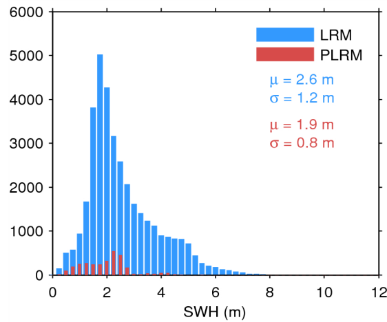
Figure 20. Histogram of science-valid SWH over oceans and lakes for LRM (blue) and PLRM (red) for 20/05/2014. The mean ( \mu ) and standard deviation ( \sigma ) are also shown. Note that values larger than 12 m are excluded from the histogram for the sake of readability but not from the computation of \mu and \sigma .
