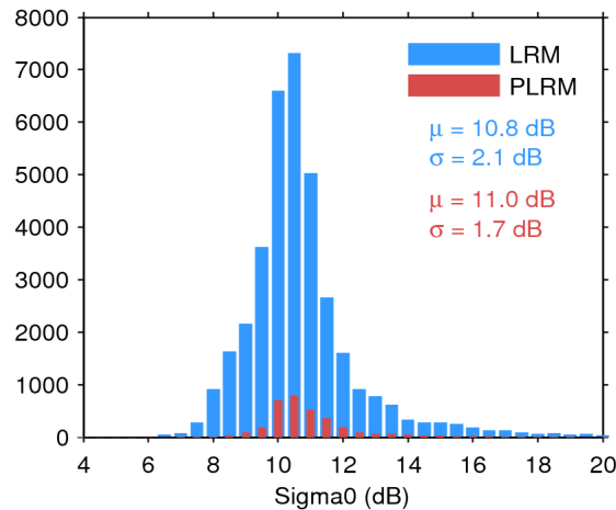
Figure 25. Histogram of flag-valid sigma0 over oceans and lakes for LRM (blue) and PLRM (red) for 20/05/2014. The mean ( \mu ) and standard deviation ( \sigma ) are also shown. Note that values outside [4 20] dB are excluded from the histogram for the sake of readability but not from the computation of \mu and \sigma .
