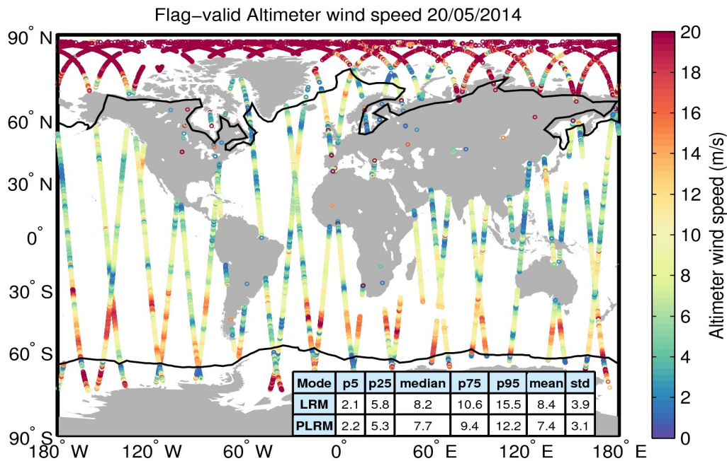
Figure 31. Geographical distribution of flag-valid wind data over oceans and lakes for 20/05/2014. The statistical values shown in the table refer to the wind in m/s and are calculated separately for LRM and PLRM regions. Measurements taken over polar polygons have been excluded from the computation of the statistical values. The black lines mark the outer limit of the Arctic and Antarctic polar polygons.
