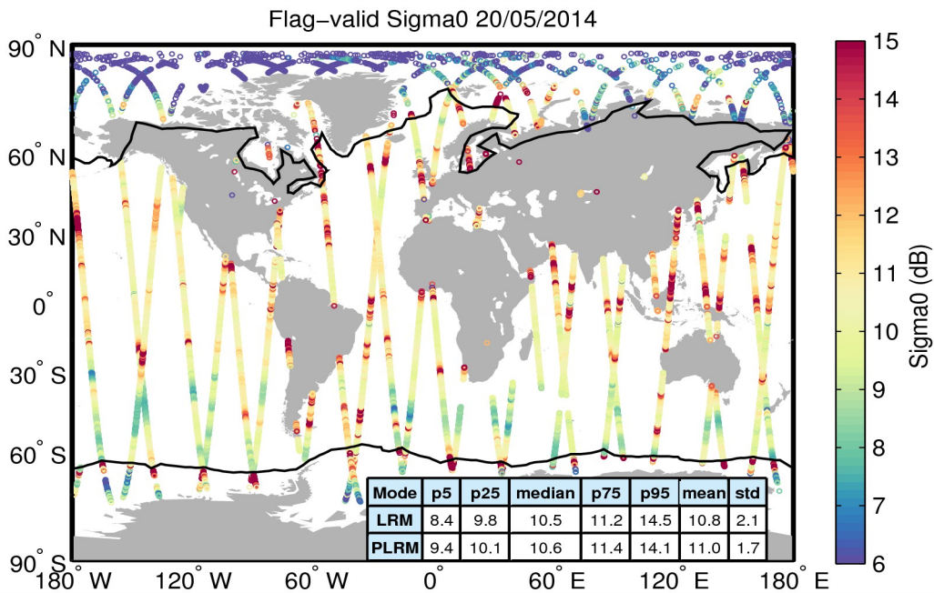
Figure 23. Geographical distribution of flag-valid sigma0 data over oceans and lakes for 20/05/2014. The statistical values shown in the table refer to the sigma0 in dB and are calculated separately for LRM and PLRM regions. Measurements taken over polar polygons have been excluded from the computation of the statistical values. The black lines mark the outer limit of the Arctic and Antarctic polar polygons.
