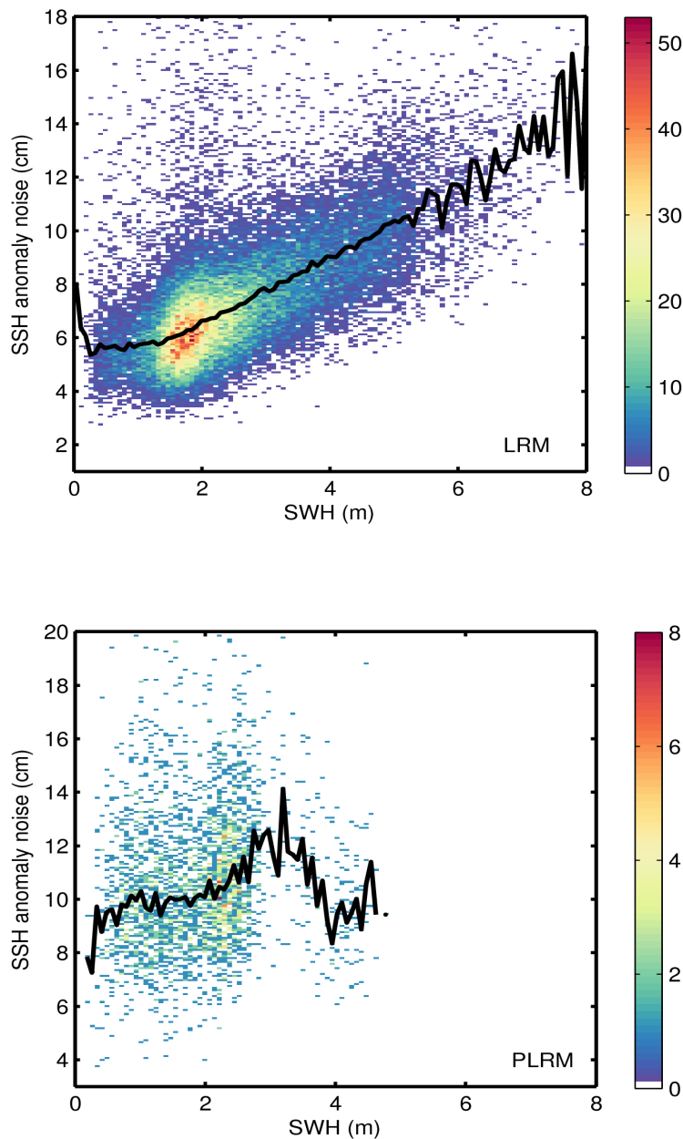
Figure 9. 2D histogram showing flag-valid SSH anomaly noise as a function of SWH for LRM (top) and PLRM (bottom) for 20/05/2014. The black line denotes the median SSH anomaly as a function of SWH.
