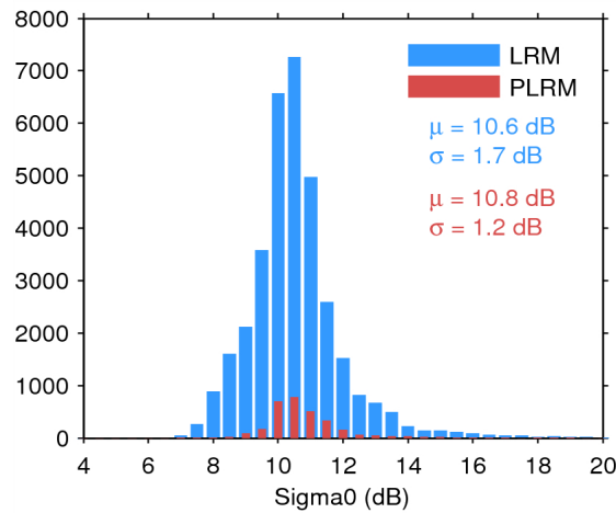
Figure 28. Histogram of science-valid sigma0 over oceans and lakes for LRM (blue) and PLRM (red) for 20/05/2014. The mean ( \mu ) and standard deviation ( \sigma ) are also shown. Note that values outside [4 20] dB are excluded from the histogram for the sake of readability but not from the computation of \mu and \sigma .
