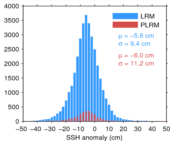
Figure 11. Histogram of science-valid SSH anomaly over oceans and lakes for LRM (blue) and PLRM (red) for 20/05/2014. The mean ( \mu ) and standard deviation ( \sigma ) are also shown. Note that values outside [-50 50] cm are excluded from the histogram for the sake of readability but not from the computation of \mu and \sigma .
