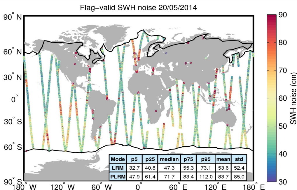
Figure 18. Geographical distribution of flag-valid 20-Hz SWH measurement noise over oceans and lakes for 20/05/2014. The statistical values shown in the table refer to the SWH noise and are calculated separately for LRM and PLRM regions. Measurements taken over polar polygons have been excluded from the computation of the statistical values. The black lines mark the outer limit of the Arctic and Antarctic polar polygons.
