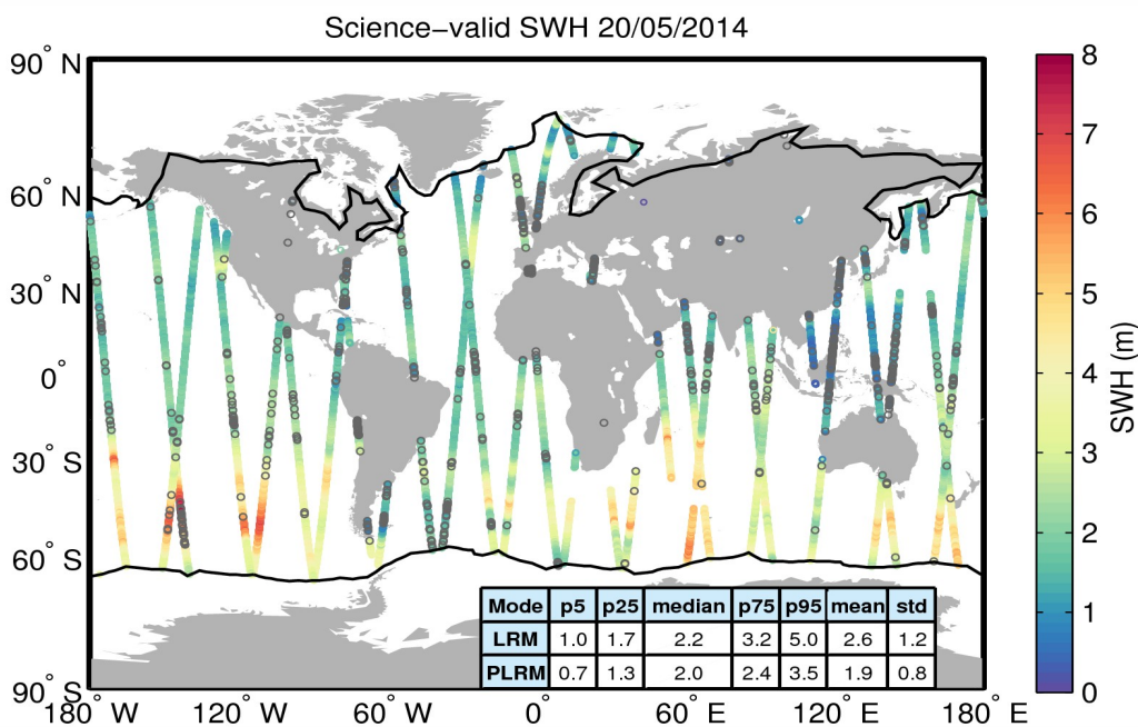
Figure 19. Geographical distribution of science-valid SWH data over oceans and lakes for 20/05/2014. The statistical values shown in the table refer to the SWH in m and are calculated separately for LRM and PLRM regions. The black lines mark the outer limit of the Arctic and Antarctic polar polygons. Gray circles denote records that have been rejected based on the editing criteria described in Table 3.
