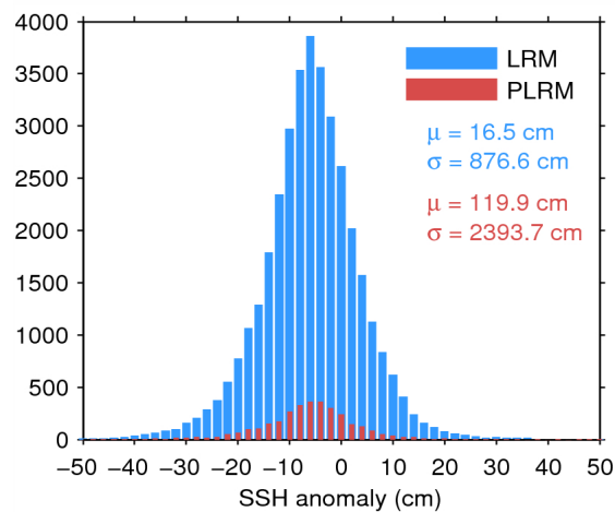
Figure 7. Histogram of flag-valid SSH anomaly over oceans and lakes for LRM (blue) and PLRM (red) for 20/05/2014. The mean ( \mu ) and standard deviation ( \sigma ) are also shown. Note that values outside [-50\ 50] cm are excluded from the histogram for the sake of readability but not from the computation of \mu and \sigma .
