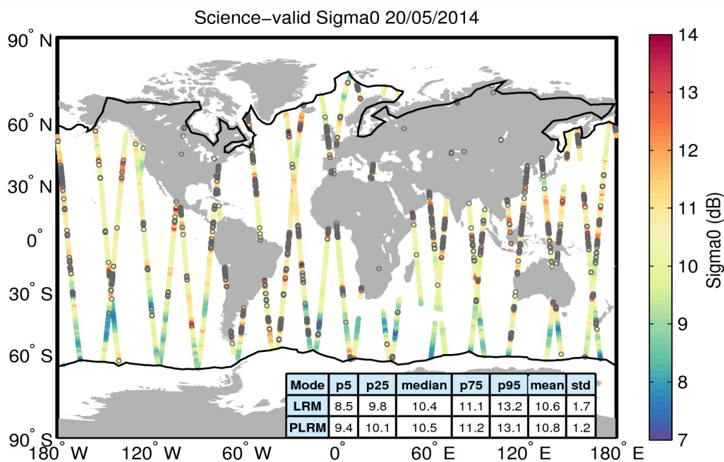
Figure 27. Geographical distribution of science-valid sigma0 data over oceans and lakes for 20/05/2014. The statistical values shown in the table refer to the sigma0 in dB and are calculated separately for LRM and PLRM regions. The black lines mark the outer limit of the Arctic and Antarctic polar polygons. Gray circles denote records that have been rejected based on the editing criteria described in Table 4.
