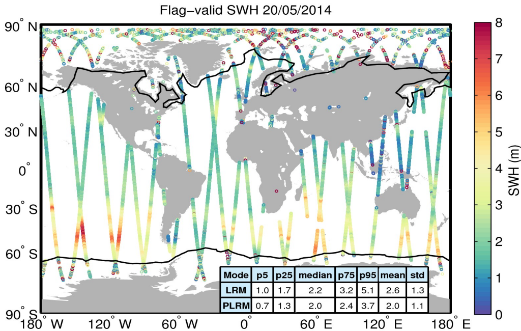
Figure 15. Geographical distribution of flag-valid SWH data over oceans and lakes for 20/05/2014. The statistical values shown in the table refer to the SWH in m and are calculated separately for LRM and PLRM regions. Measurements taken over polar polygons have been excluded from the computation of the statistical values. The black lines mark the outer limit of the Arctic and Antarctic polar polygons.
